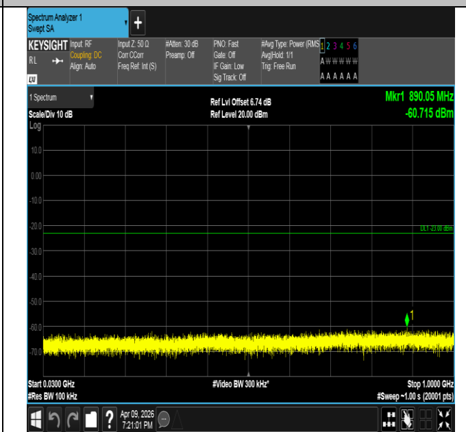
Band4-1.4MHz-16QAM-20393-6RB#0-30~1000-PASS
