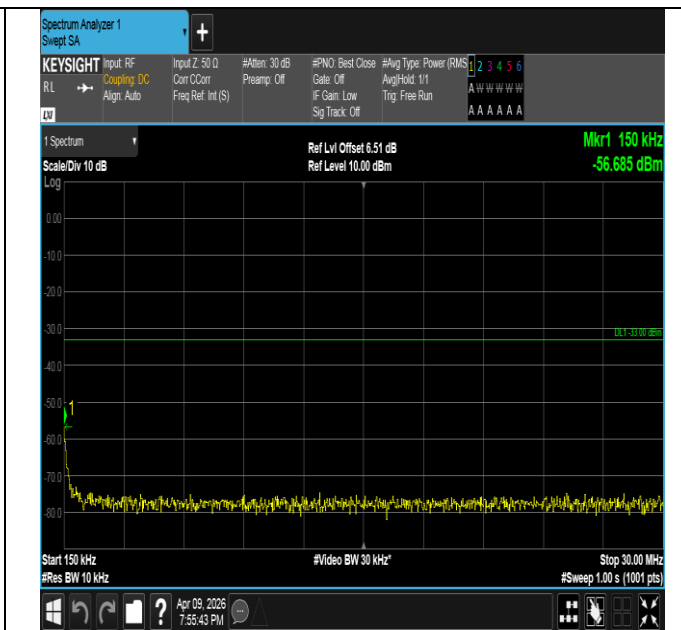
Band4-3MHz-QPSK-19965-15RB#0-0.15~30-PASS
