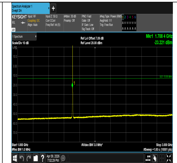
Band4-3MHz-QPSK-19965-1RB#0-1000~3000-PASS
