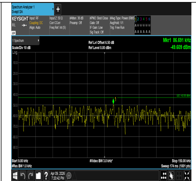
Band4-1.4MHz-16QAM-20393-6RB#0-0.009~0.15-PASS
