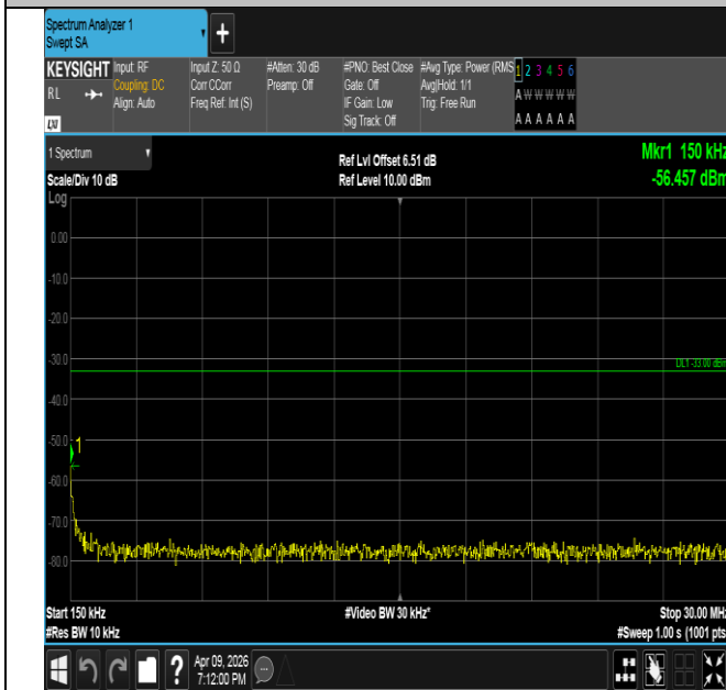
Band4-1.4MHz-16QAM-20175-1RB#0-0.15~30-PASS
