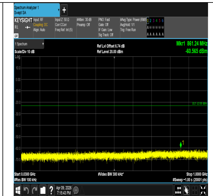
Band4-1.4MHz-16QAM-20175-6RB#0-30~1000-PASS
