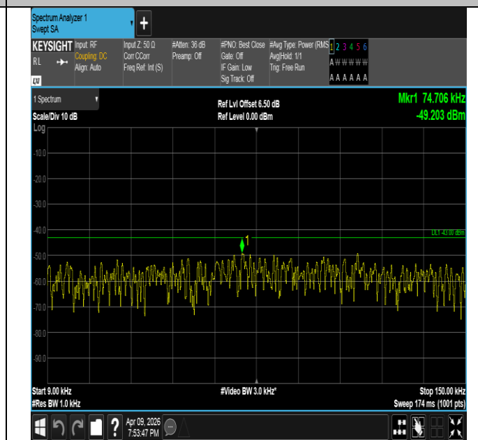
Band4-3MHz-QPSK-19965-1RB#14-0.009~0.15-PASS
