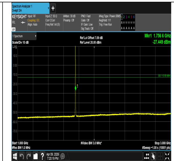
Band4-1.4MHz-QPSK-20393-6RB#0-1000~3000-PASS
