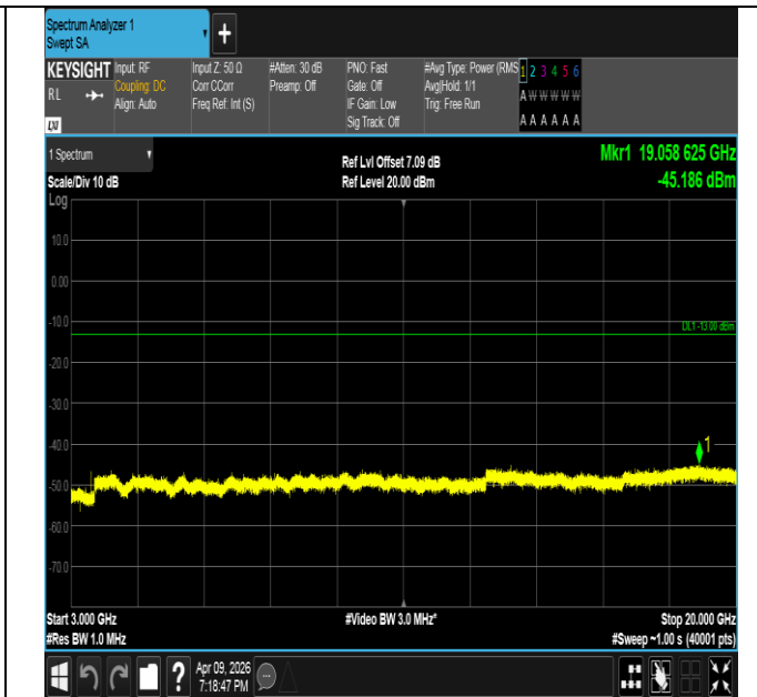
Band4-1.4MHz-QPSK-20393-1RB#5-3000~20000-PASS
