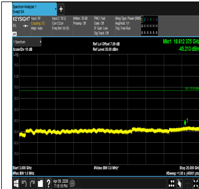
Band4-1.4MHz-QPSK-20175-6RB#0-3000~20000-PASS
