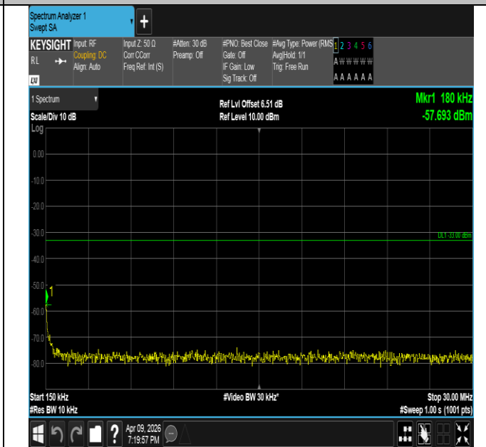
Band4-1.4MHz-QPSK-20393-6RB#0-0.15~30-PASS
