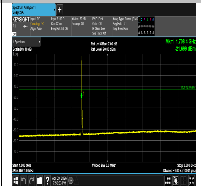
Band4-3MHz-QPSK-19965-15RB#0-1000~3000-PASS
