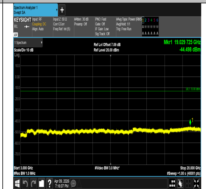
Band4-1.4MHz-16QAM-20175-6RB#0-3000~20000-PASS
