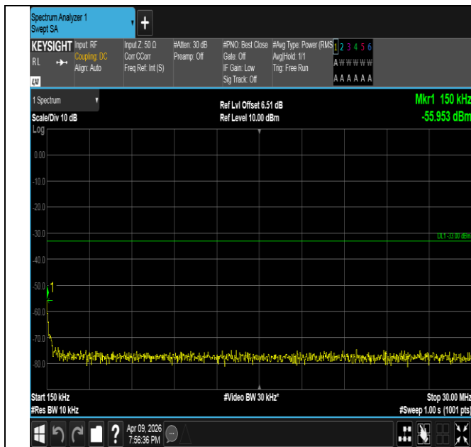
Band4-3MHz-16QAM-19965-15RB#0-0.15~30-PASS
