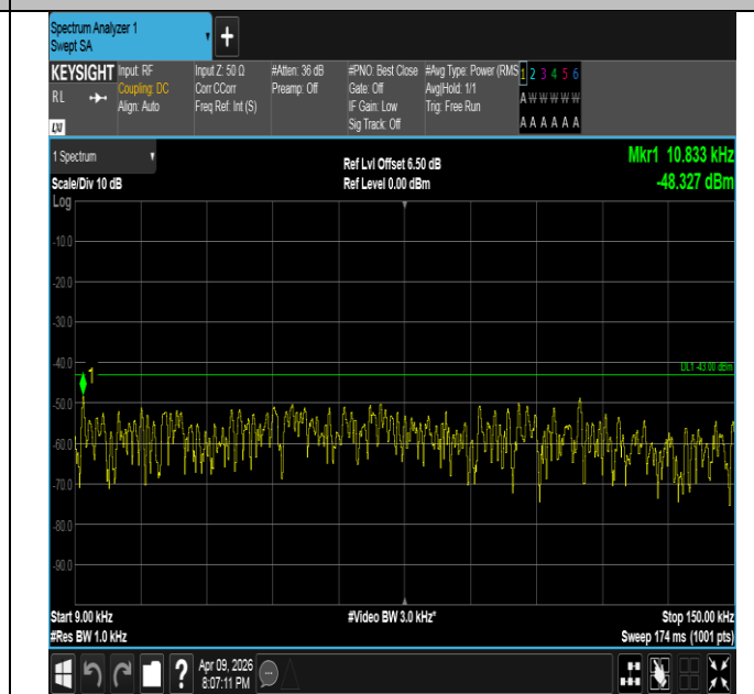
Band4-3MHz-16QAM-20385-15RB#0-0.009~0.15-PASS
