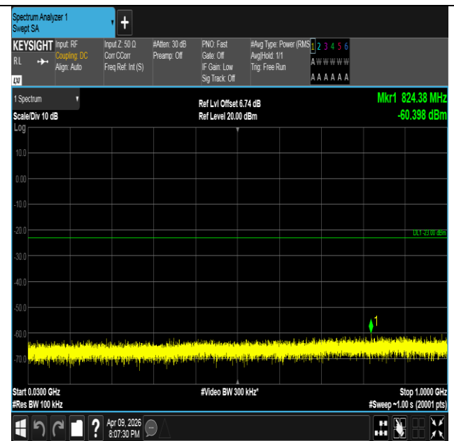
Band4-3MHz-16QAM-20385-15RB#0-30~1000-PASS
