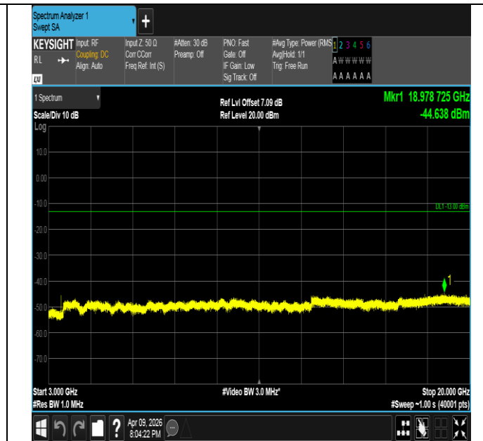
Band4-3MHz-16QAM-20385-1RB#0-3000~20000-PASS
