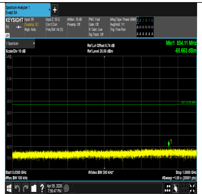
Band4-3MHz-16QAM-19965-15RB#0-30~1000-PASS
