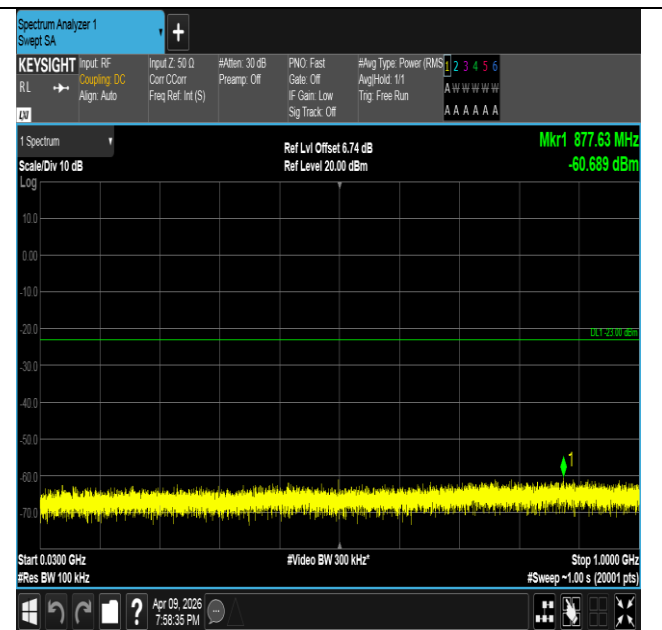
Band4-3MHz-16QAM-20175-1RB#0-30~1000-PASS
