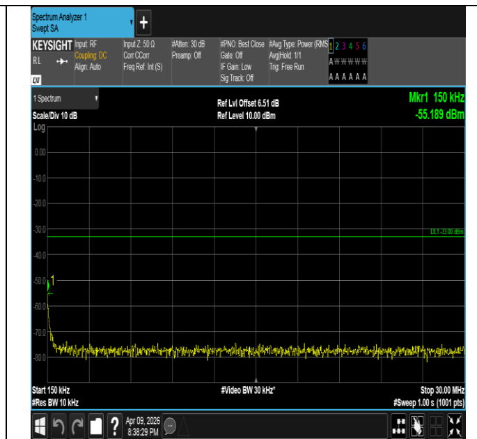
Band4-5MHz-QPSK-19975-1RB#0-0.15~30-PASS
