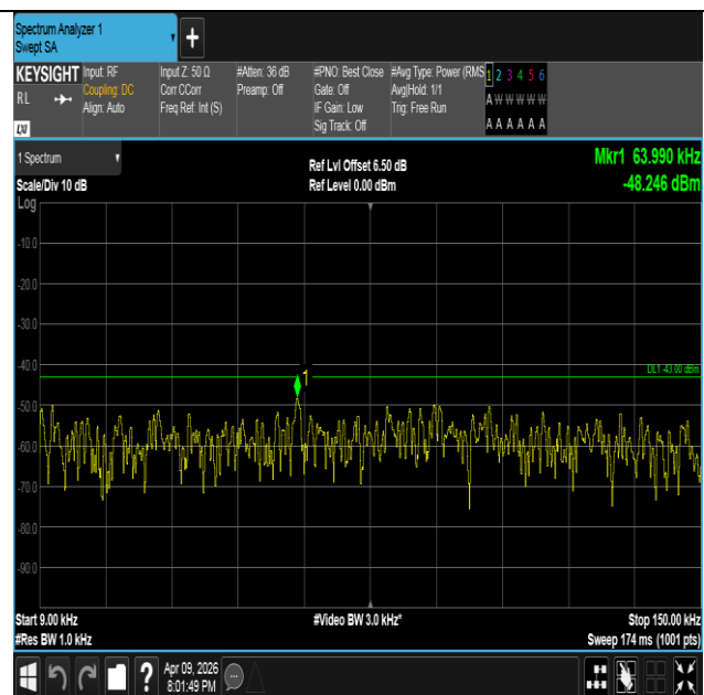
Band4-3MHz-16QAM-20175-15RB#0-0.009~0.15-PASS
