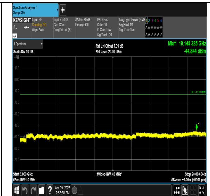
Band4-3MHz-16QAM-19965-1RB#0-3000~20000-PASS
