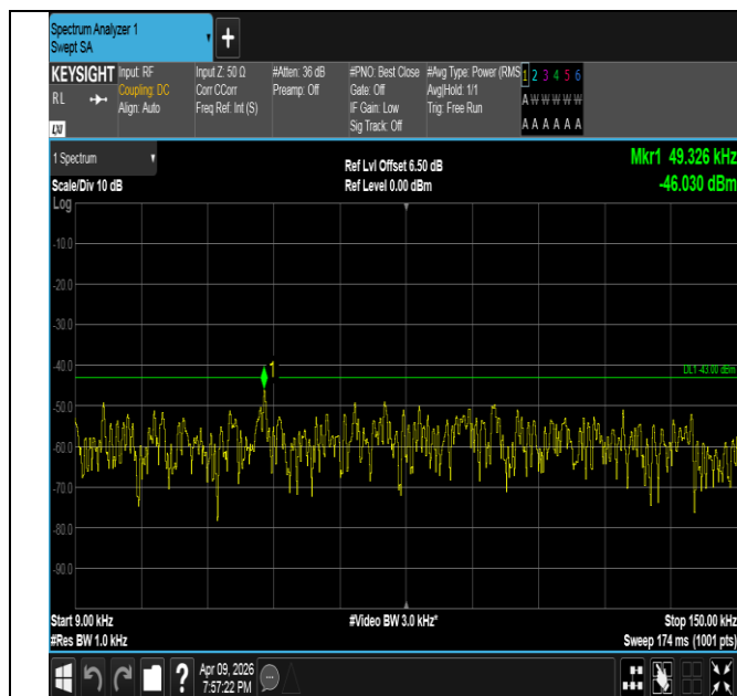
Band4-3MHz-QPSK-20175-1RB#0-0.009~0.15-PASS
