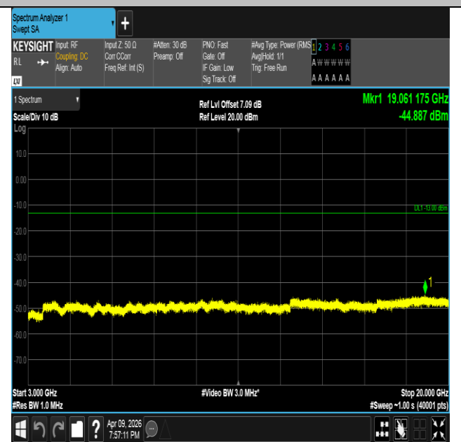
Band4-3MHz-16QAM-19965-15RB#0-3000~20000-PASS
