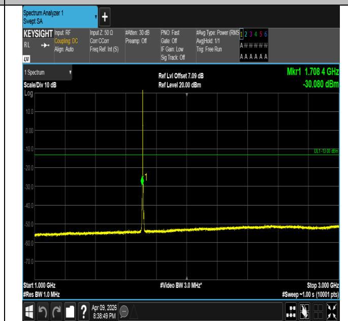
Band4-5MHz-QPSK-19975-1RB#0-1000~3000-PASS
