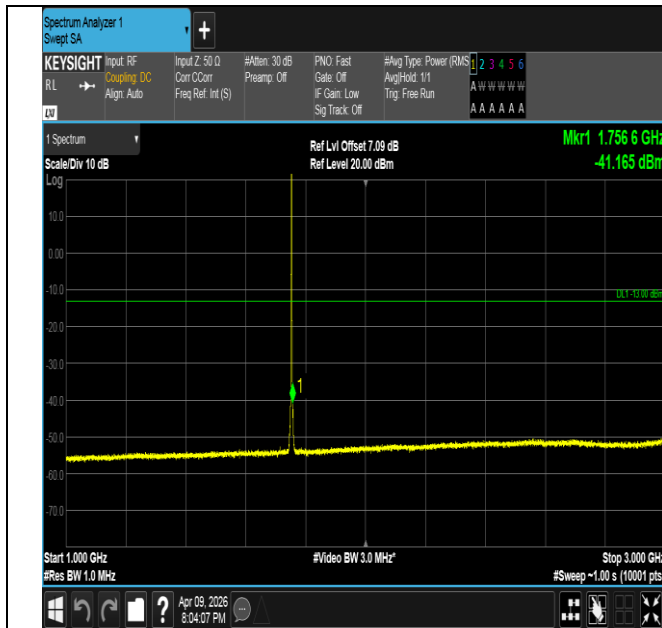
Band4-3MHz-16QAM-20385-1RB#0-1000~3000-PASS
