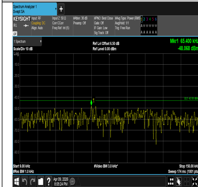
Band4-3MHz-16QAM-20385-1RB#14-0.009~0.15-PASS
