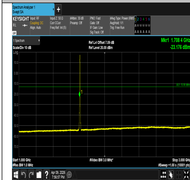
Band4-3MHz-16QAM-19965-15RB#0-1000~3000-PASS
