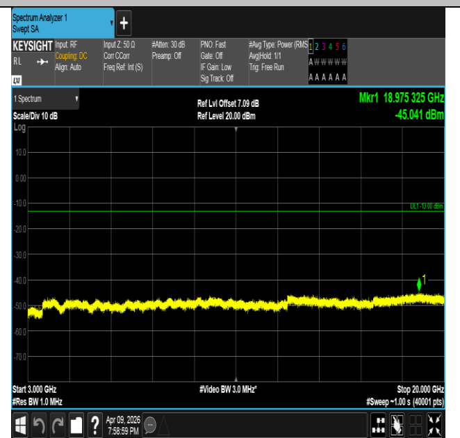
Band4-3MHz-16QAM-20175-1RB#0-3000~20000-PASS
