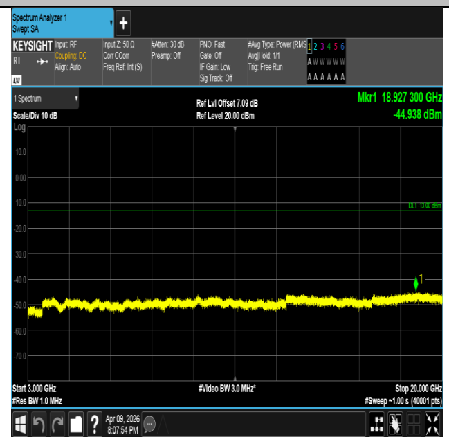
Band4-3MHz-16QAM-20385-15RB#0-3000~20000-PASS
