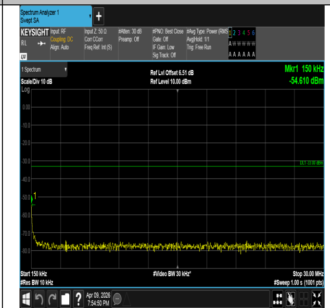
Band4-3MHz-16QAM-19965-1RB#14-0.15~30-PASS
