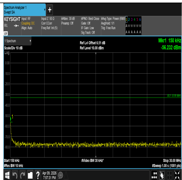
Band4-3MHz-QPSK-20175-1RB#0-0.15~30-PASS
