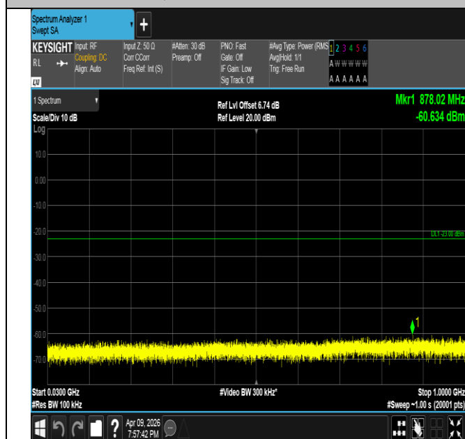
Band4-3MHz-QPSK-20175-1RB#0-30~1000-PASS
