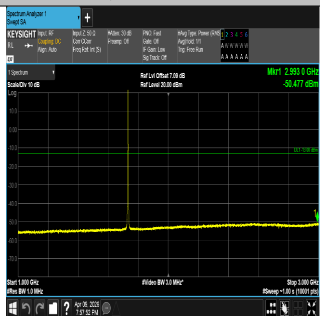
Band4-3MHz-QPSK-20175-1RB#0-1000~3000-PASS
