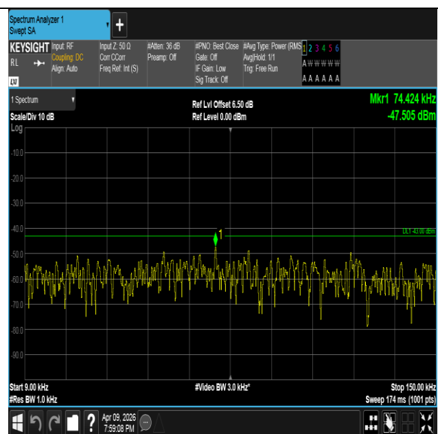
Band4-3MHz-QPSK-20175-1RB#14-0.009~0.15-PASS
