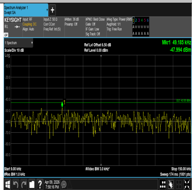
Band4-3MHz-16QAM-20175-1RB#0-0.009~0.15-PASS
