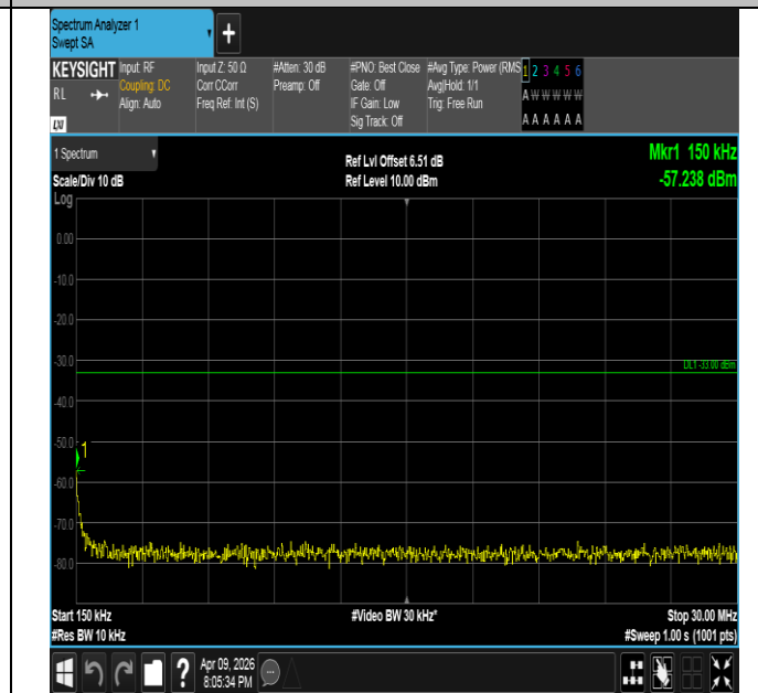
Band4-3MHz-16QAM-20385-1RB#14-0.15~30-PASS
