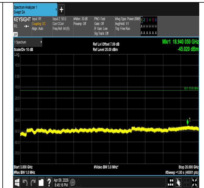
Band4-5MHz-16QAM-20175-1RB#0-3000~20000-PASS
