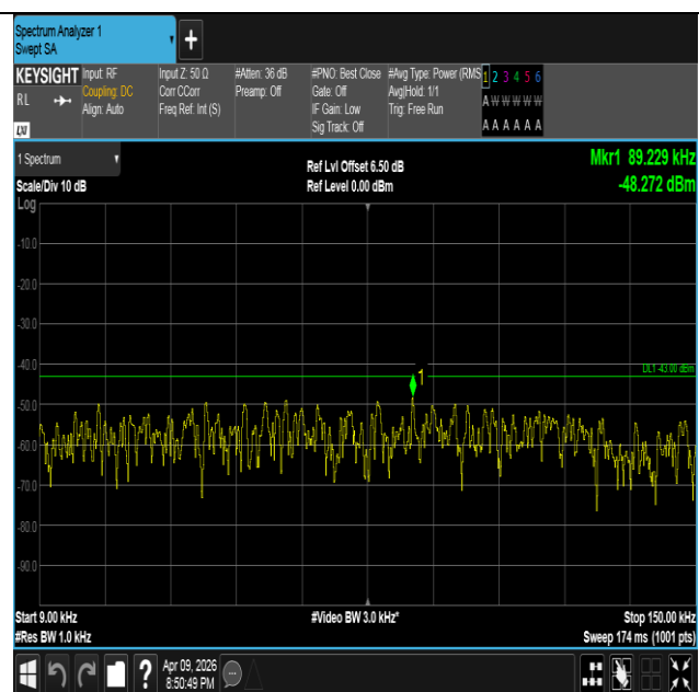
Band4-5MHz-QPSK-20375-1RB#24-0.009~0.15-PASS
