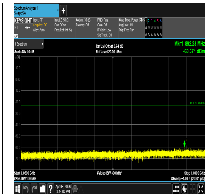
Band4-5MHz-QPSK-20175-1RB#0-30~1000-PASS
