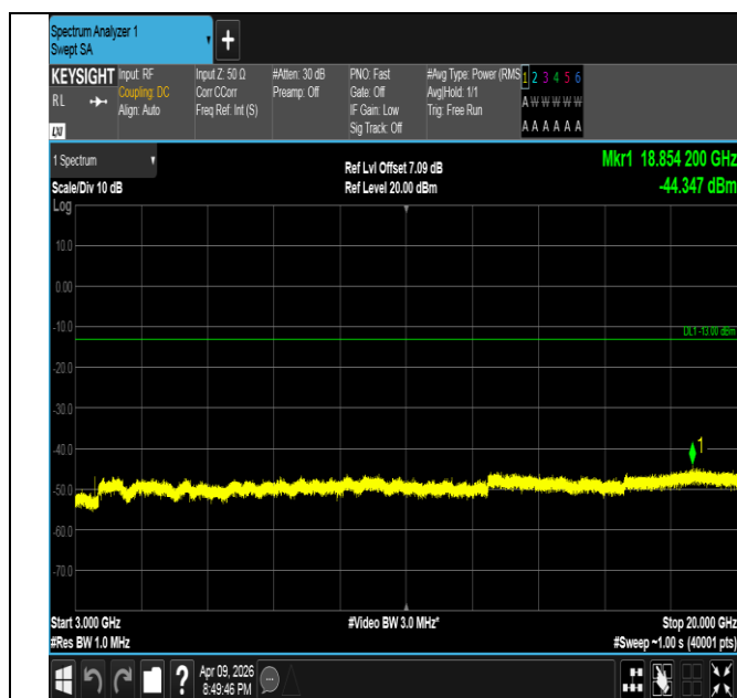
Band4-5MHz-QPSK-20375-1RB#0-3000~20000-PASS
