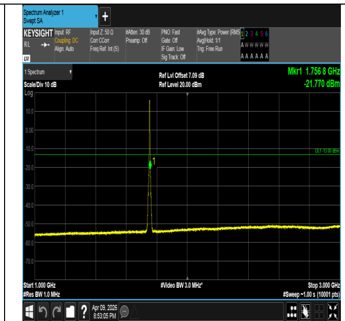
Band4-5MHz-QPSK-20375-25RB#0-1000~3000-PASS
