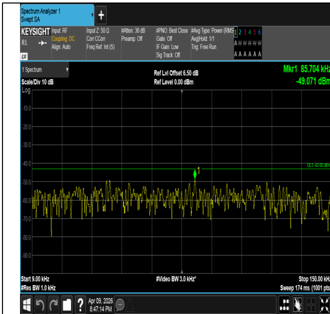
Band4-5MHz-QPSK-20175-25RB#0-0.009~0.15-PASS
