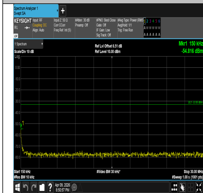
Band4-5MHz-QPSK-20375-1RB#24-0.15~30-PASS
