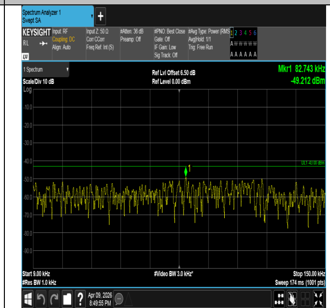
Band4-5MHz-16QAM-20375-1RB#0-0.009~0.15-PASS
