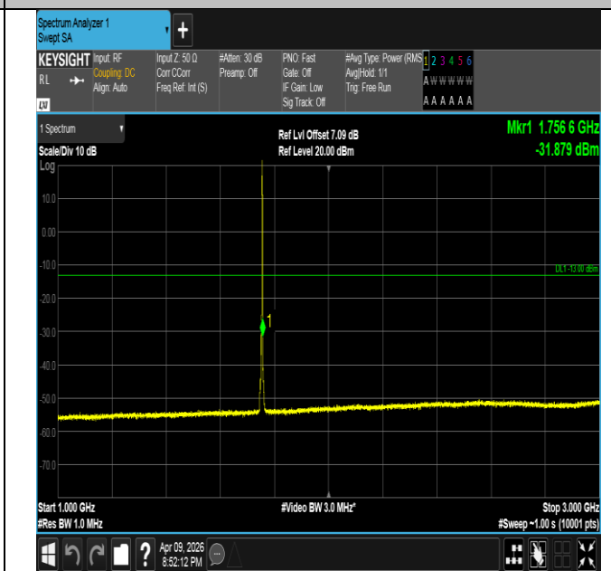
Band4-5MHz-16QAM-20375-1RB#24-1000~3000-PASS
