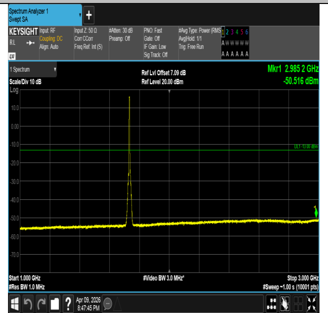
Band4-5MHz-QPSK-20175-25RB#0-1000~3000-PASS
