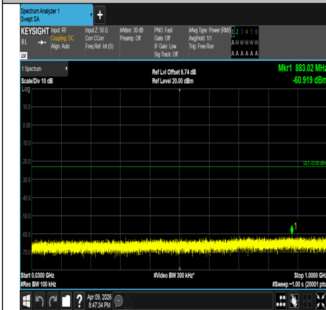
Band4-5MHz-QPSK-20175-25RB#0-30~1000-PASS
