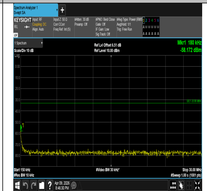
Band4-5MHz-16QAM-20175-1RB#24-0.15~30-PASS
