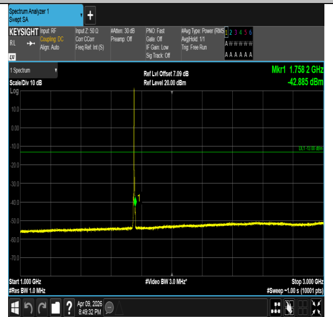
Band4-5MHz-QPSK-20375-1RB#0-1000~3000-PASS
