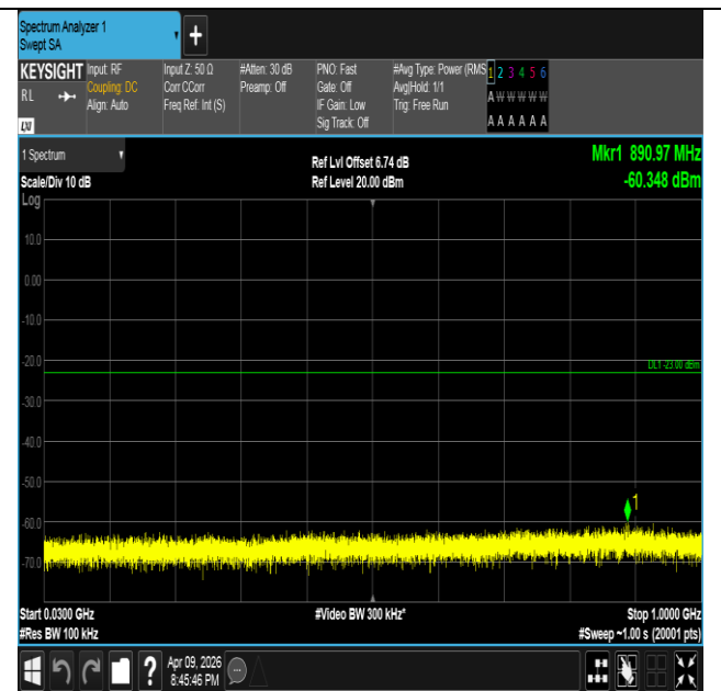
Band4-5MHz-QPSK-20175-1RB#24-30~1000-PASS
