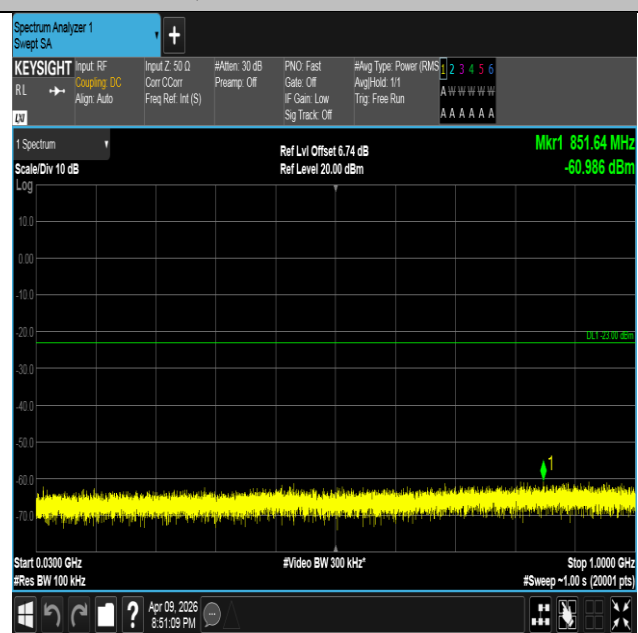
Band4-5MHz-QPSK-20375-1RB#24-30~1000-PASS
