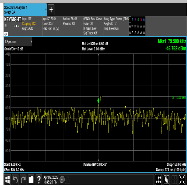
Band4-5MHz-QPSK-20175-1RB#24-0.009~0.15-PASS
