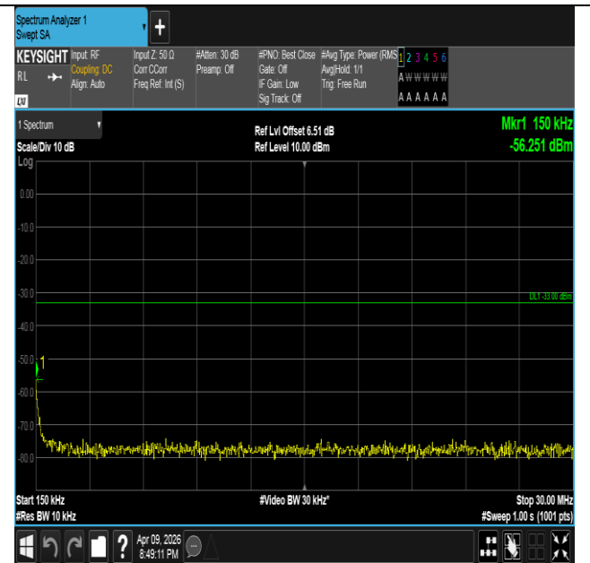
Band4-5MHz-QPSK-20375-1RB#0-0.15~30-PASS
