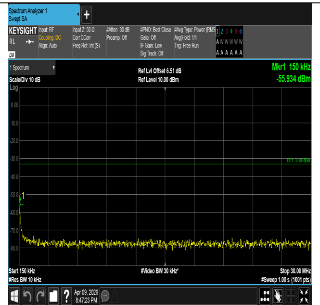
Band4-5MHz-QPSK-20175-25RB#0-0.15~30-PASS
