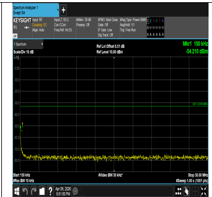
Band4-5MHz-16QAM-20375-1RB#24-0.15~30-PASS
