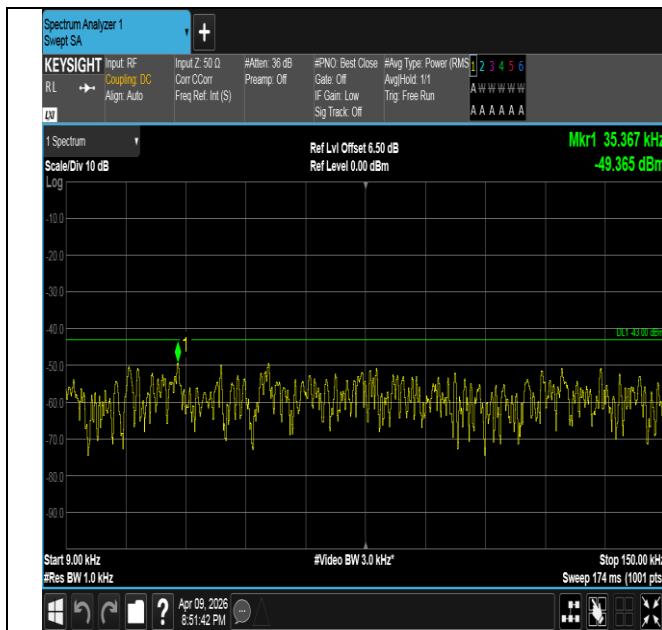
Band4-5MHz-16QAM-20375-1RB#24-0.009~0.15-PASS
