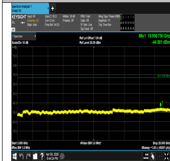
Band4-5MHz-QPSK-20175-1RB#0-3000~20000-PASS
