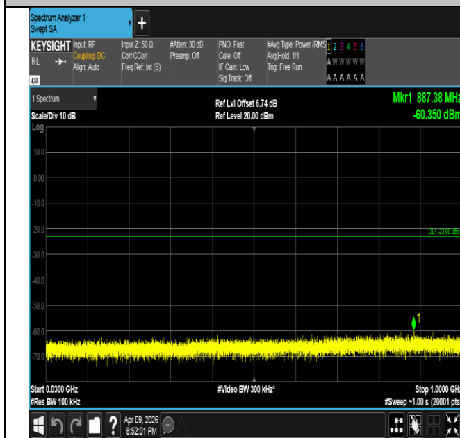
Band4-5MHz-16QAM-20375-1RB#24-30~1000-PASS
