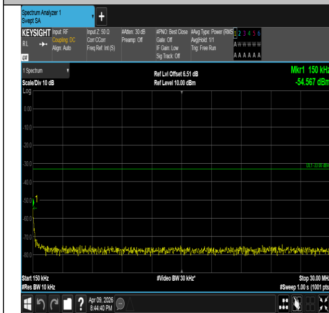
Band4-5MHz-16QAM-20175-1RB#0-0.15~30-PASS
