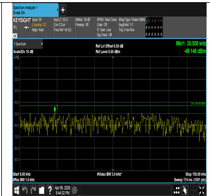
Band4-5MHz-16QAM-20175-1RB#0-0.009~0.15-PASS
