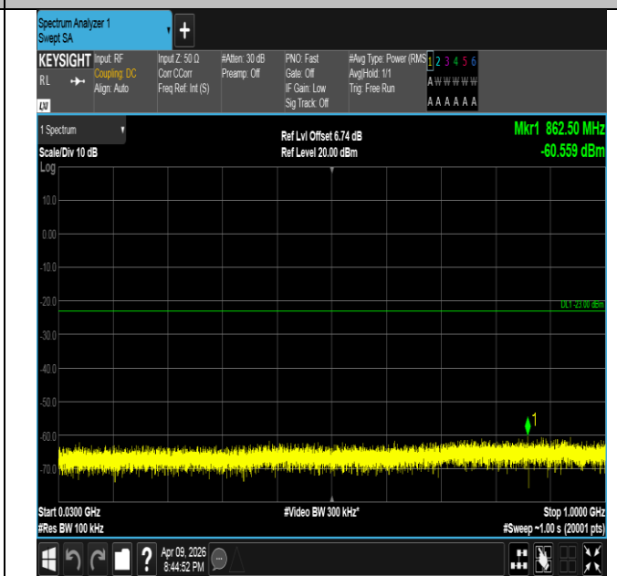
Band4-5MHz-16QAM-20175-1RB#0-30~1000-PASS
