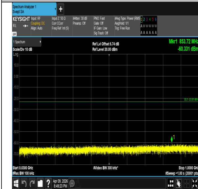
Band4-5MHz-QPSK-20375-1RB#0-30~1000-PASS
