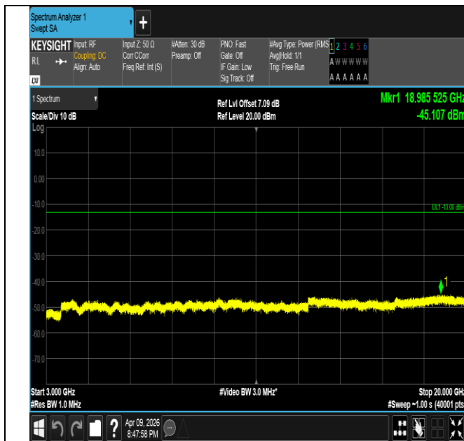
Band4-5MHz-QPSK-20175-25RB#0-3000~20000-PASS
