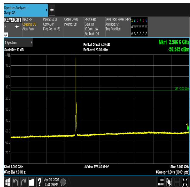
Band4-5MHz-QPSK-20175-1RB#0-1000~3000-PASS
