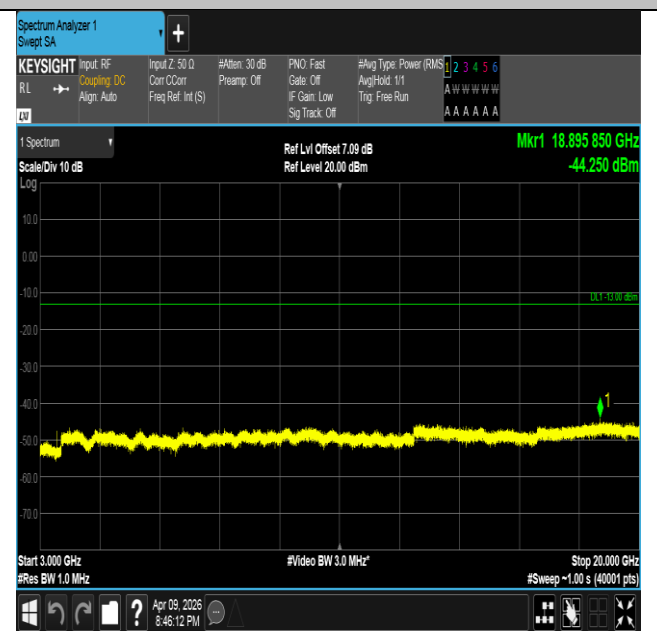
Band4-5MHz-QPSK-20175-1RB#24-3000~20000-PASS
