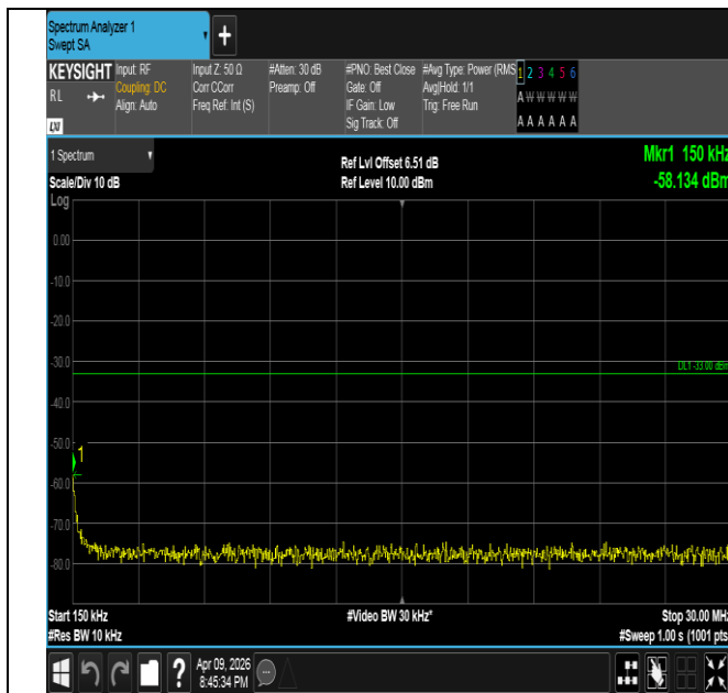
Band4-5MHz-QPSK-20175-1RB#24-0.15~30-PASS
