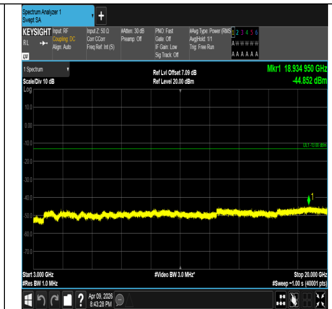
Band4-5MHz-16QAM-19975-25RB#0-3000~20000-PASS
