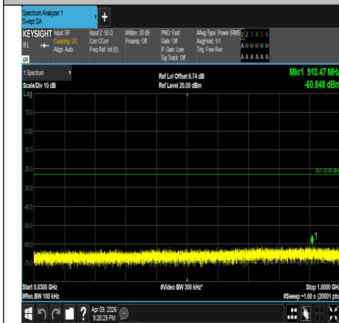
Band4-10MHz-QPSK-20000-50RB#0-30~1000-PASS
