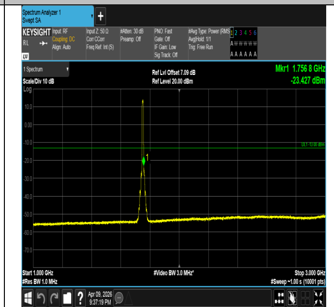
Band4-10MHz-QPSK-20350-50RB#0-1000~3000-PASS
