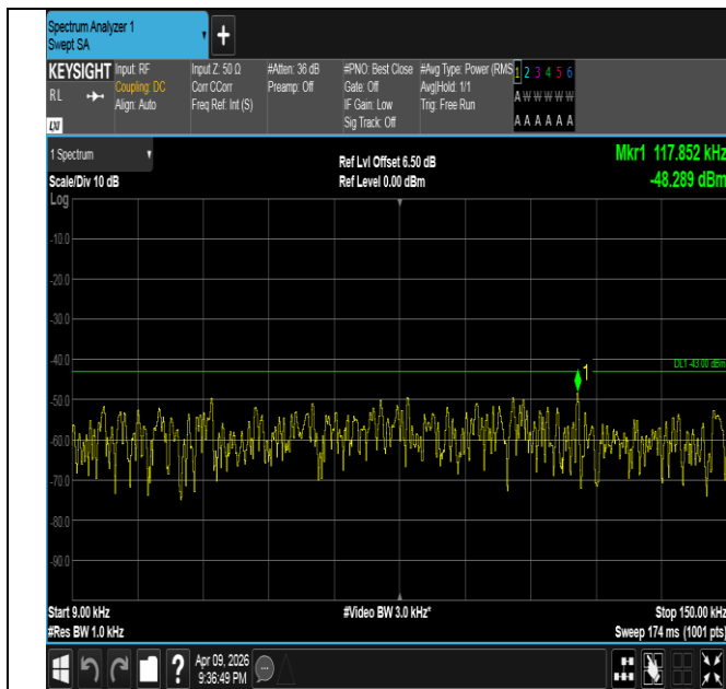
Band4-10MHz-QPSK-20350-50RB#0-0.009~0.15-PASS
