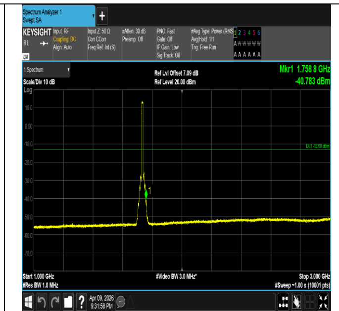
Band4-10MHz-QPSK-20175-50RB#0-1000~3000-PASS
