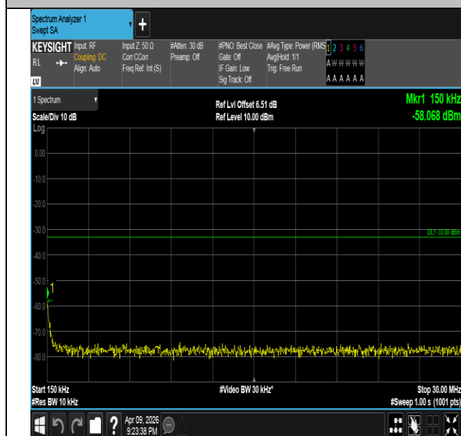
Band4-10MHz-16QAM-20000-1RB#0-0.15~30-PASS
