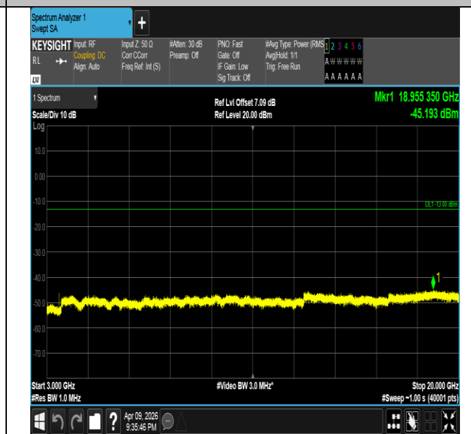
Band4-10MHz-QPSK-20350-1RB#49-3000~20000-PASS
