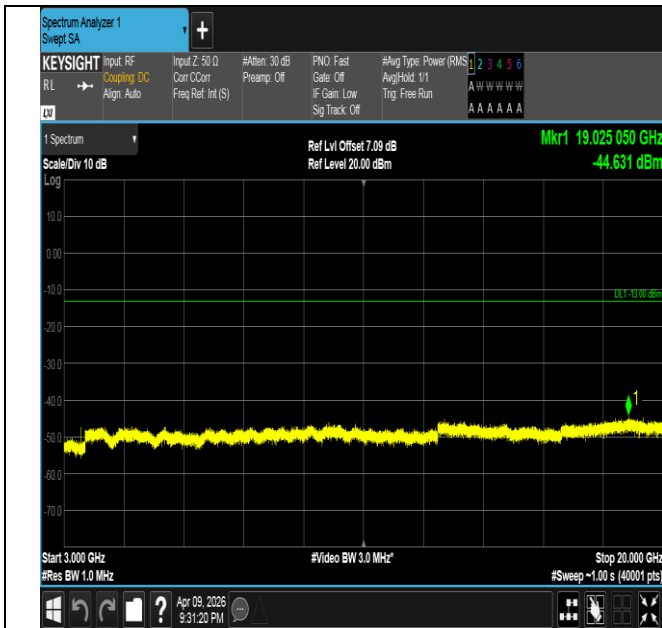
Band4-10MHz-16QAM-20175-1RB#49-3000~20000-PASS
