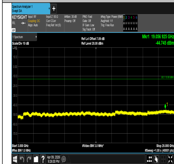
Band4-10MHz-16QAM-20000-1RB#49-3000~20000-PASS
