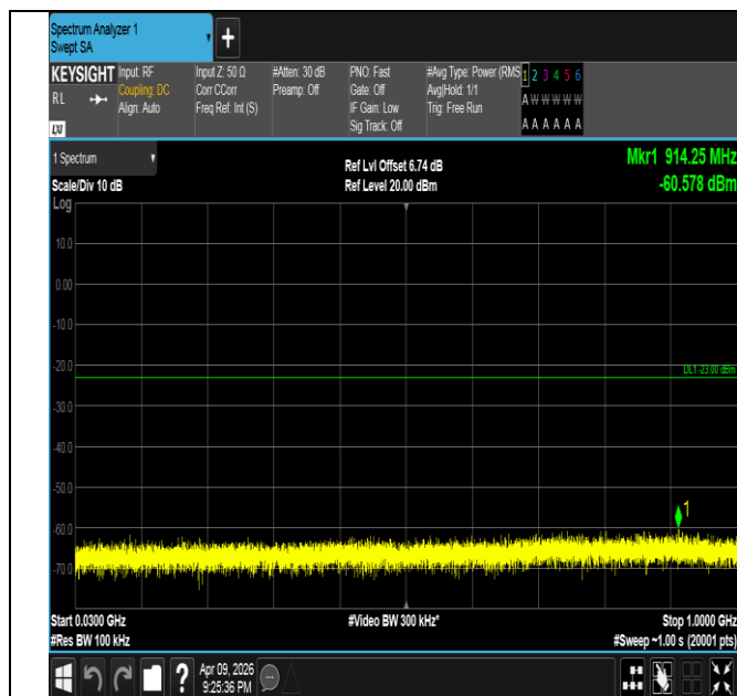
Band4-10MHz-16QAM-20000-1RB#49-30~1000-PASS
