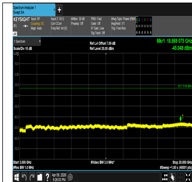
Band4-10MHz-QPSK-20000-50RB#0-3000~20000-PASS
