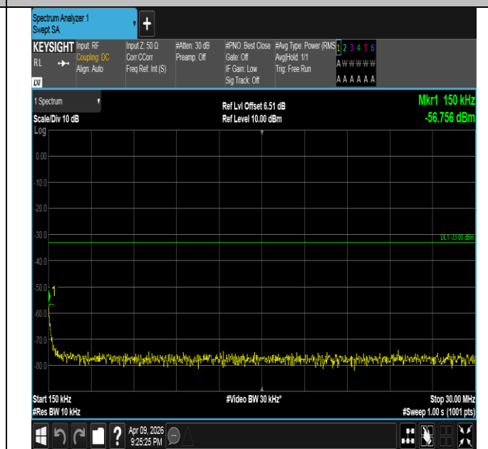
Band4-10MHz-16QAM-20000-1RB#49-0.15~30-PASS
