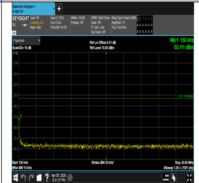
Band4-10MHz-QPSK-20175-50RB#0-0.15~30-PASS
