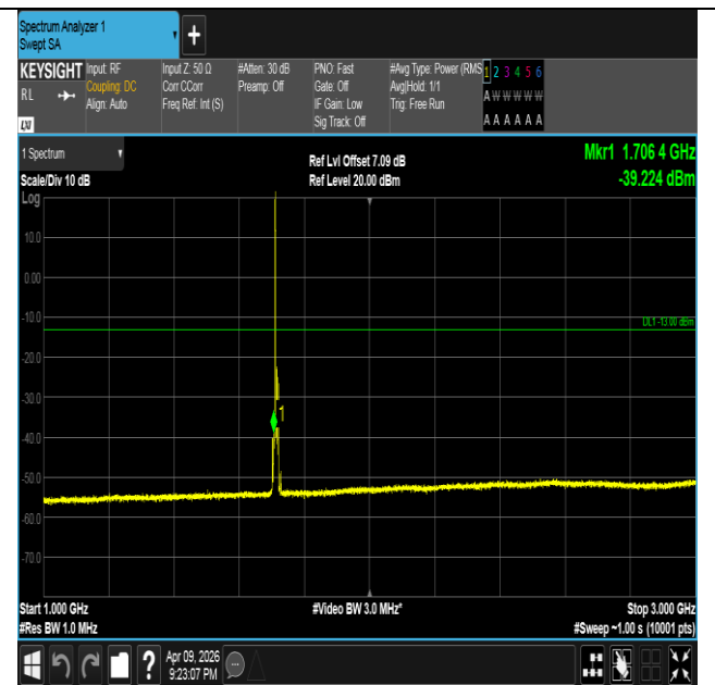
Band4-10MHz-QPSK-20000-1RB#0-1000~3000-PASS
