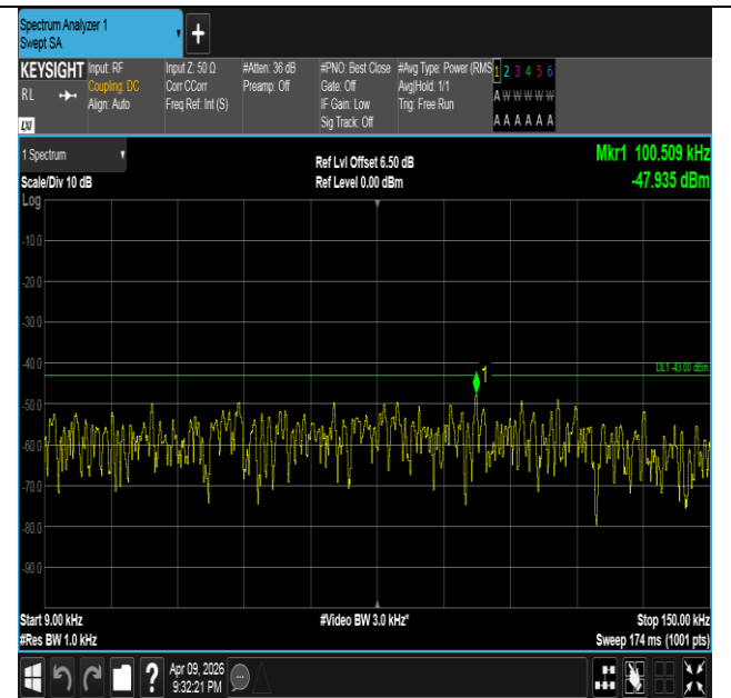
Band4-10MHz-16QAM-20175-50RB#0-0.009~0.15-PASS
