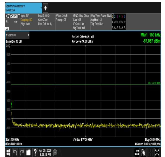
Band4-10MHz-QPSK-20000-50RB#0-0.15~30-PASS
