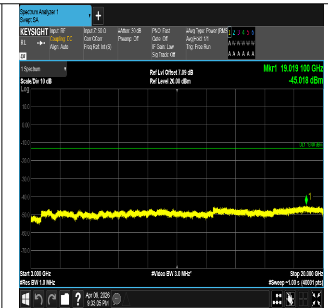
Band4-10MHz-16QAM-20175-50RB#0-3000~20000-PASS
