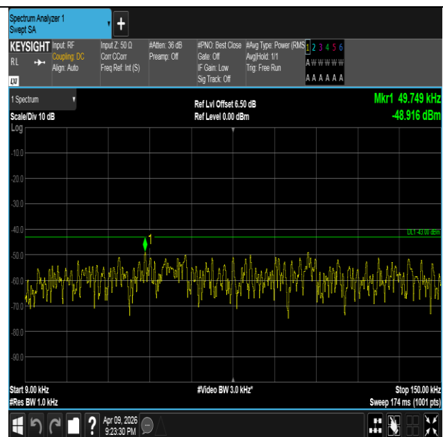
Band4-10MHz-16QAM-20000-1RB#0-0.009~0.15-PASS
