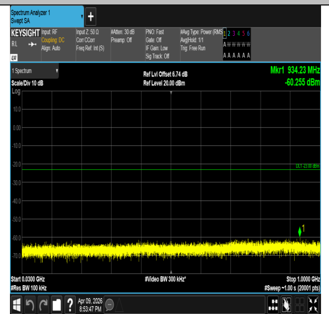
Band4-5MHz-16QAM-20375-25RB#0-30~1000-PASS
