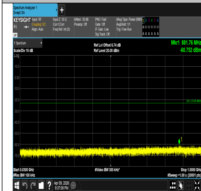
Band4-10MHz-QPSK-20350-50RB#0-30~1000-PASS
