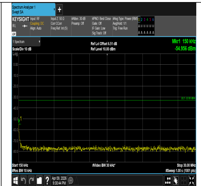
Band4-10MHz-16QAM-20175-1RB#49-0.15~30-PASS
