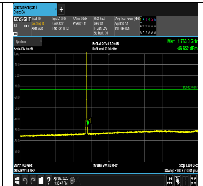
Band4-10MHz-QPSK-20350-1RB#0-1000~3000-PASS
