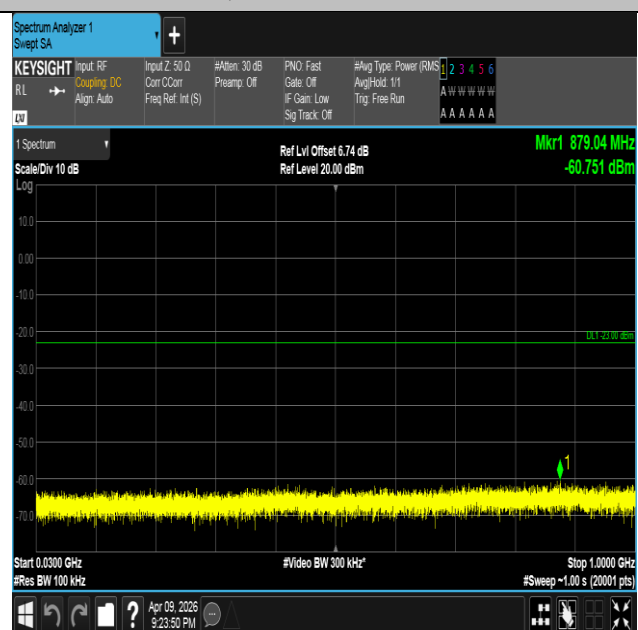
Band4-10MHz-16QAM-20000-1RB#0-30~1000-PASS
