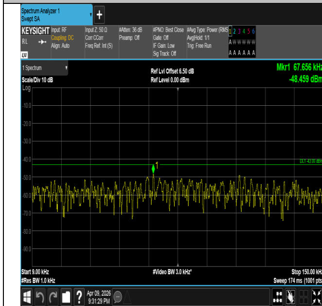
Band4-10MHz-QPSK-20175-50RB#0-0.009~0.15-PASS
