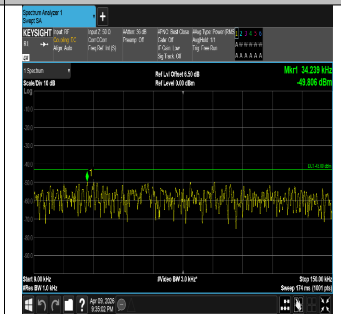
Band4-10MHz-QPSK-20350-1RB#49-0.009~0.15-PASS
