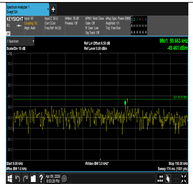
Band4-5MHz-16QAM-20375-25RB#0-0.009~0.15-PASS
