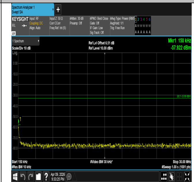
Band4-10MHz-QPSK-20350-1RB#0-0.15~30-PASS
