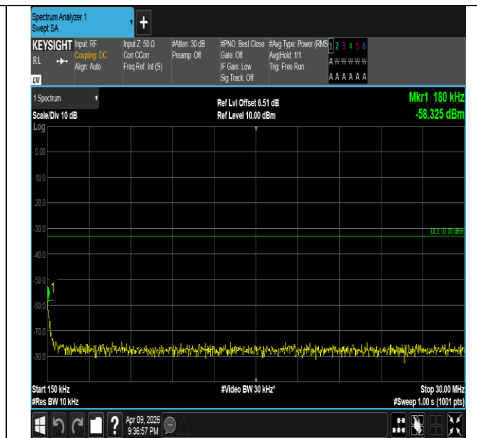
Band4-10MHz-QPSK-20350-50RB#0-0.15~30-PASS
