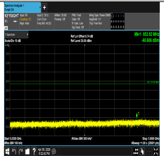
Band4-10MHz-16QAM-20175-50RB#0-30~1000-PASS
