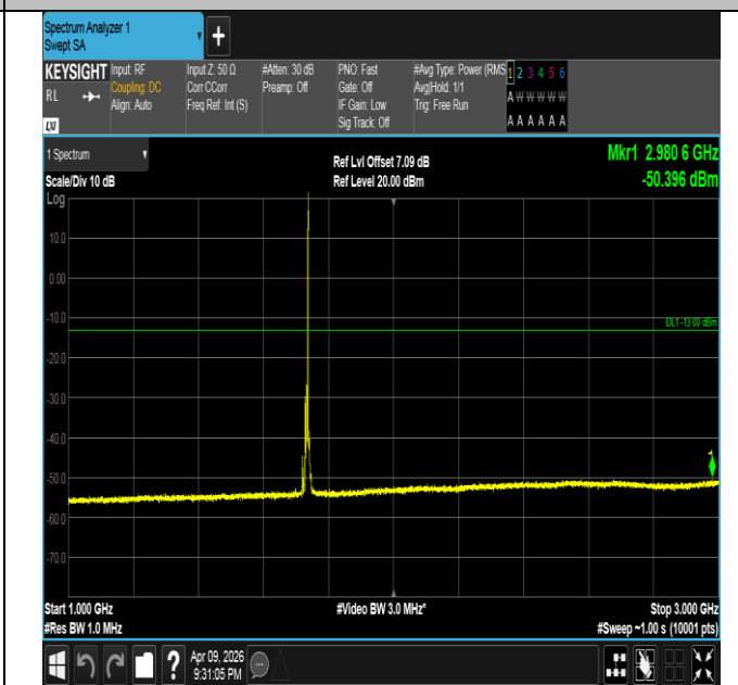
Band4-10MHz-16QAM-20175-1RB#49-1000~3000-PASS
