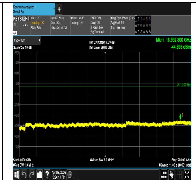
Band4-10MHz-16QAM-20000-1RB#0-3000~20000-PASS
