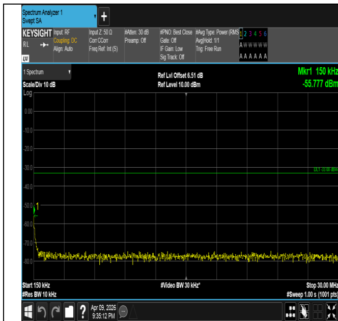
Band4-10MHz-QPSK-20350-1RB#49-0.15~30-PASS
