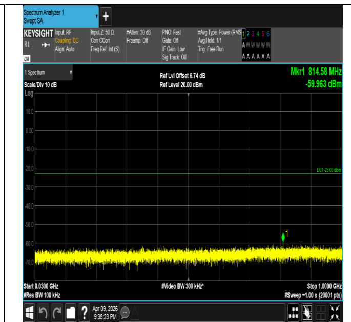
Band4-10MHz-QPSK-20350-1RB#49-30~1000-PASS
