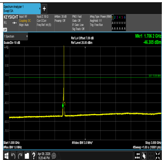
Band4-10MHz-16QAM-20000-1RB#49-1000~3000-PASS
