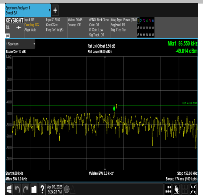
Band4-10MHz-QPSK-20000-1RB#49-0.009~0.15-PASS
