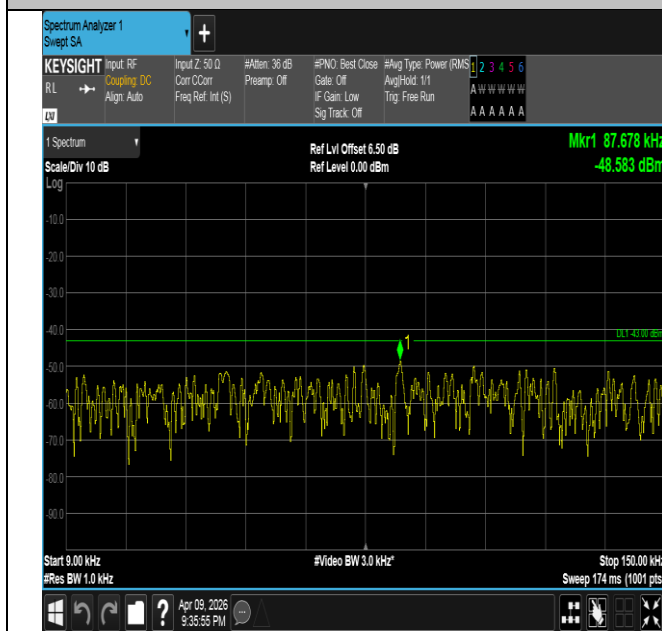
Band4-10MHz-16QAM-20350-1RB#49-0.009~0.15-PASS
