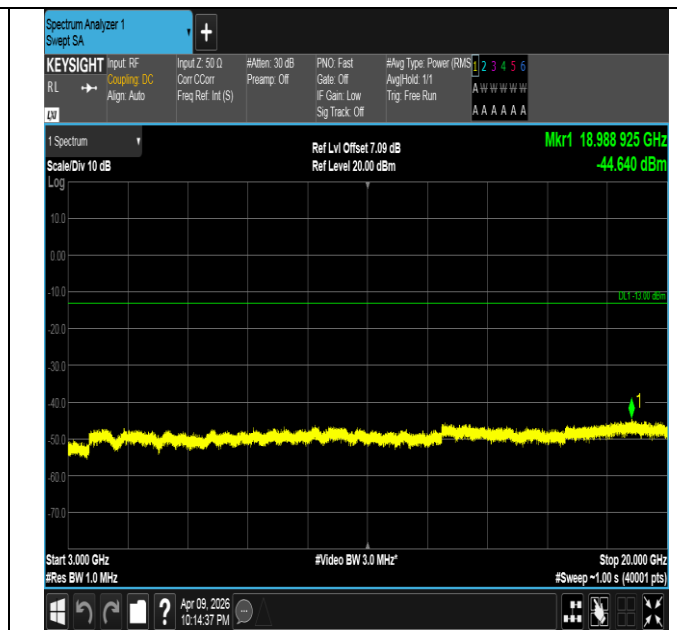
Band4-15MHz-16QAM-20175-1RB#0-3000~20000-PASS
