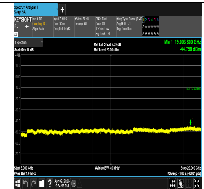
Band4-10MHz-16QAM-20350-1RB#0-3000~20000-PASS
