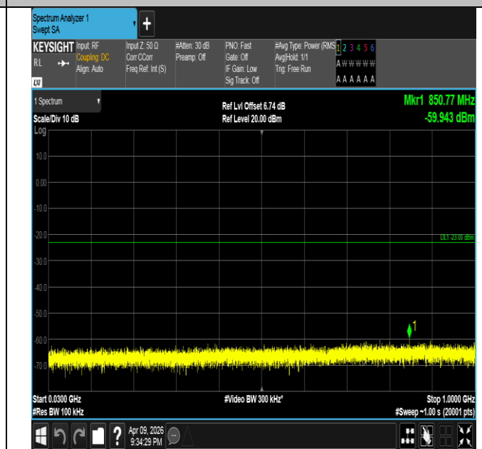
Band4-10MHz-16QAM-20350-1RB#0-30~1000-PASS
