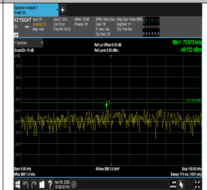
Band4-15MHz-16QAM-20025-1RB#0-0.009~0.15-PASS
