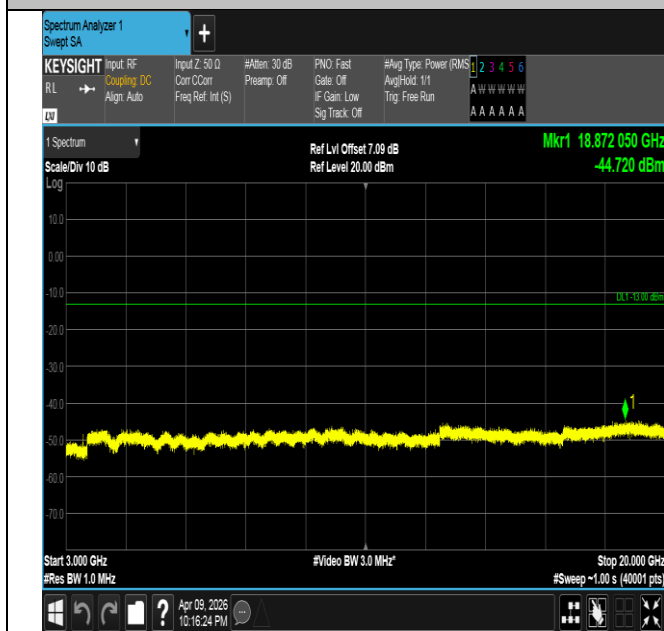
Band4-15MHz-16QAM-20175-1RB#74-3000~20000-PASS
