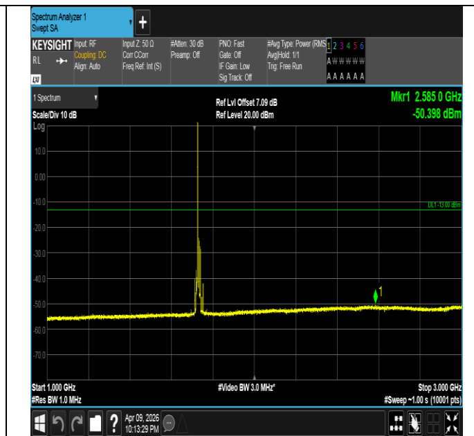
Band4-15MHz-QPSK-20175-1RB#0-1000~3000-PASS
