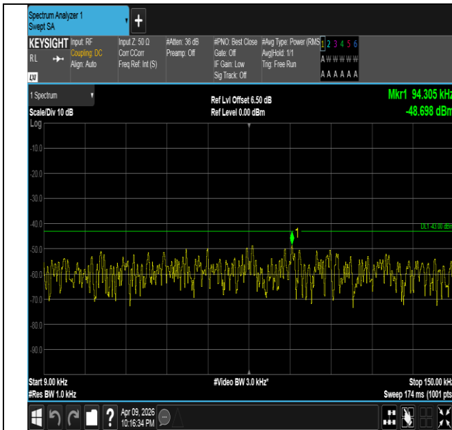
Band4-15MHz-QPSK-20175-75RB#0-0.009~0.15-PASS
