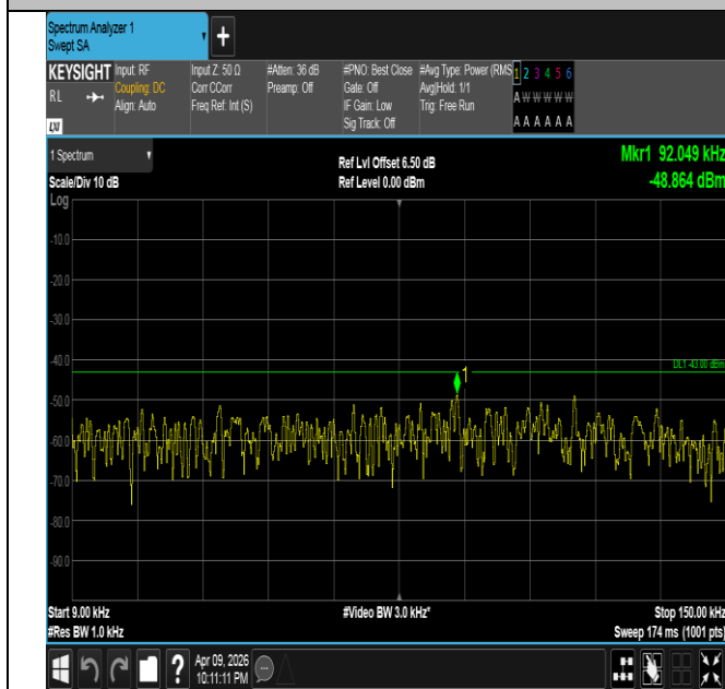
Band4-15MHz-QPSK-20025-75RB#0-0.009~0.15-PASS
