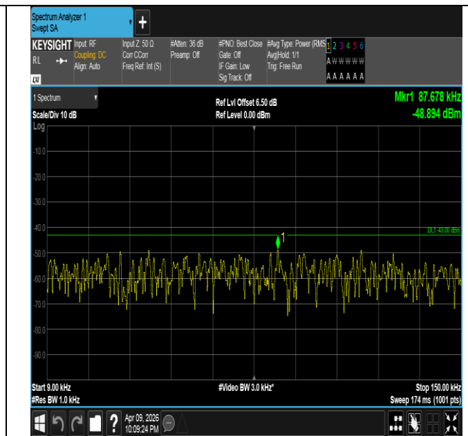
Band4-15MHz-QPSK-20025-1RB#74-0.009~0.15-PASS
