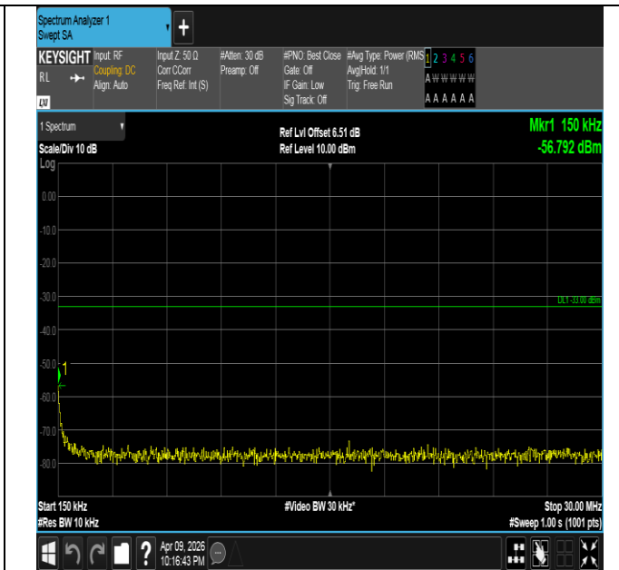
Band4-15MHz-QPSK-20175-75RB#0-0.15~30-PASS
