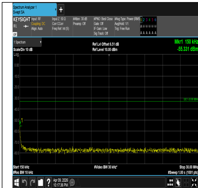
Band4-15MHz-16QAM-20175-75RB#0-0.15~30-PASS
