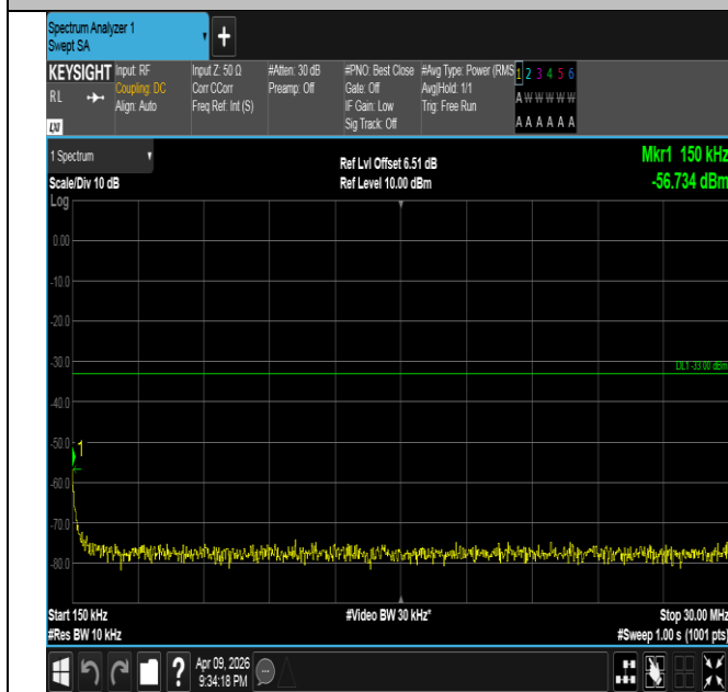
Band4-10MHz-16QAM-20350-1RB#0-0.15~30-PASS
