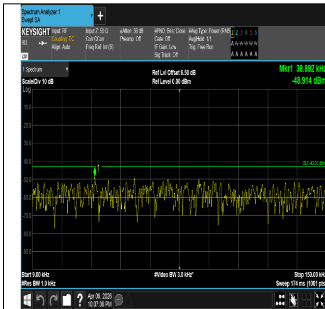
Band4-15MHz-QPSK-20025-1RB#0-0.009~0.15-PASS
