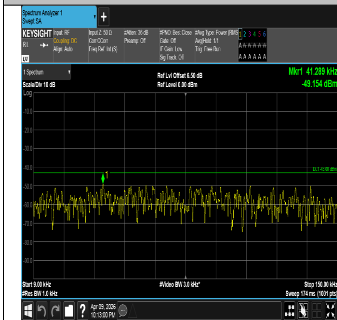
Band4-15MHz-QPSK-20175-1RB#0-0.009~0.15-PASS
