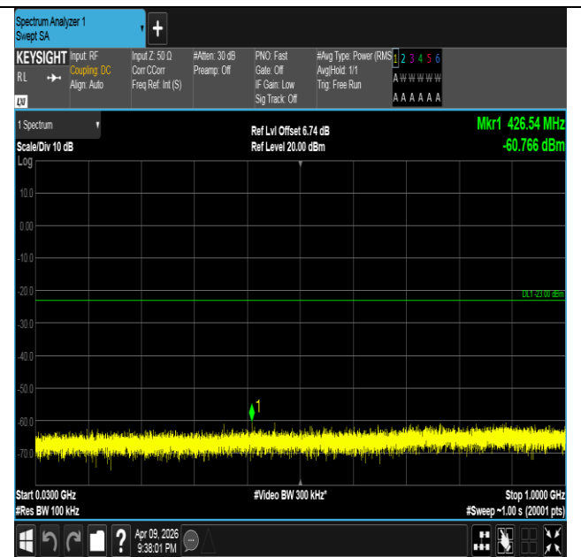
Band4-10MHz-16QAM-20350-50RB#0-30~1000-PASS
