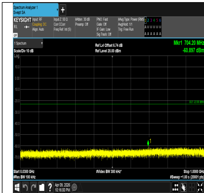
Band4-15MHz-16QAM-20175-1RB#74-30~1000-PASS
