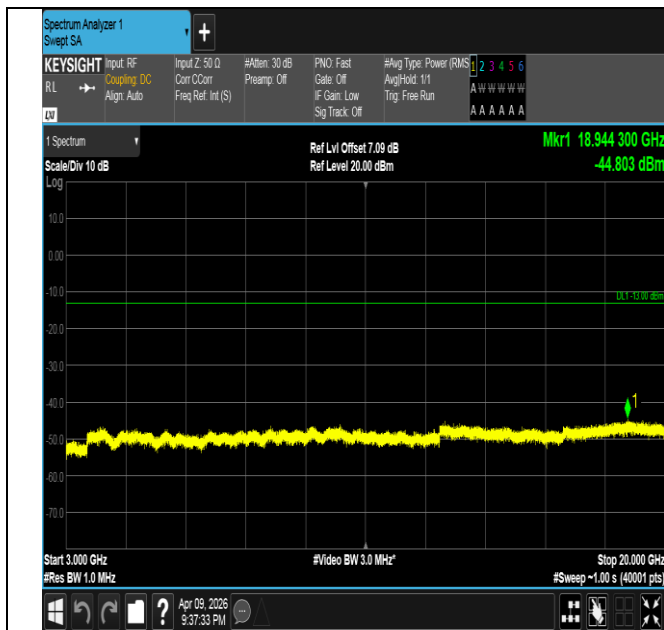
Band4-10MHz-QPSK-20350-50RB#0-3000~20000-PASS
