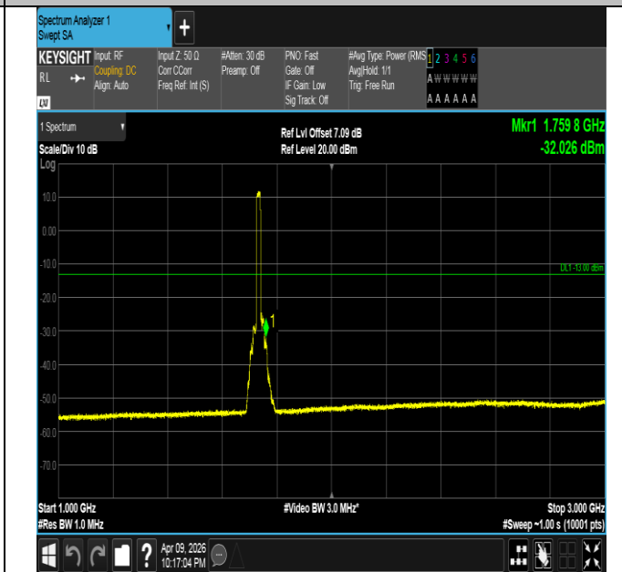
Band4-15MHz-QPSK-20175-75RB#0-1000~3000-PASS
