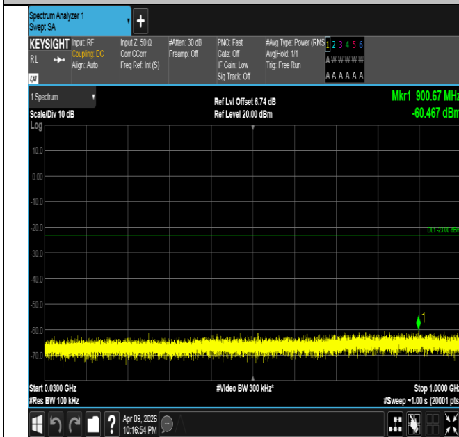
Band4-15MHz-QPSK-20175-75RB#0-30~1000-PASS
