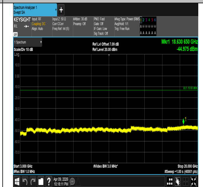
Band4-15MHz-16QAM-20175-75RB#0-3000~20000-PASS
