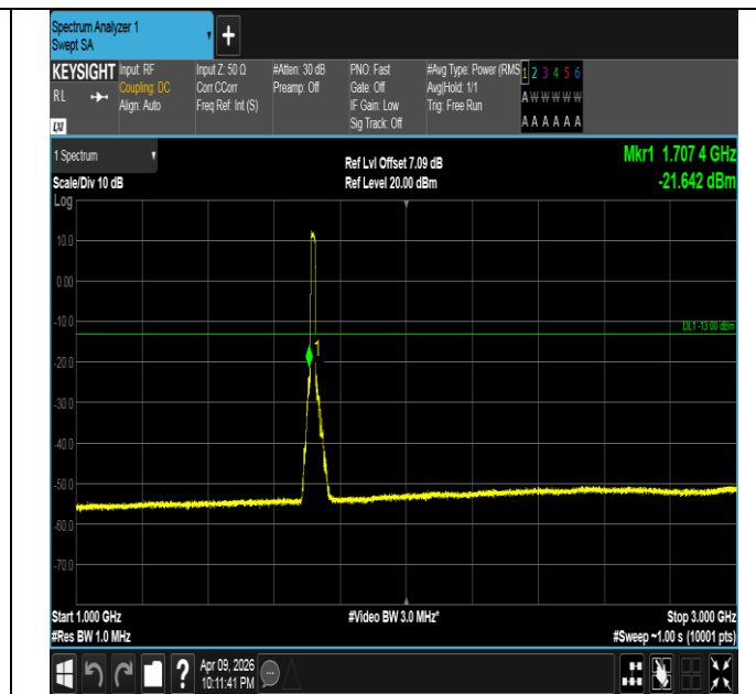
Band4-15MHz-QPSK-20025-75RB#0-1000~3000-PASS
