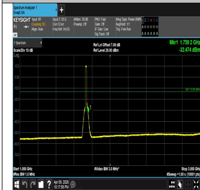
Band4-15MHz-16QAM-20175-75RB#0-1000~3000-PASS
