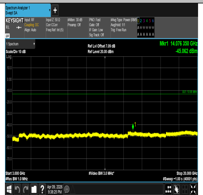
Band4-10MHz-16QAM-20350-50RB#0-3000~20000-PASS
