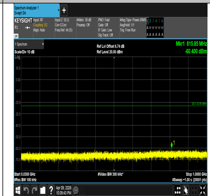
Band4-15MHz-QPSK-20025-1RB#74-30~1000-PASS
