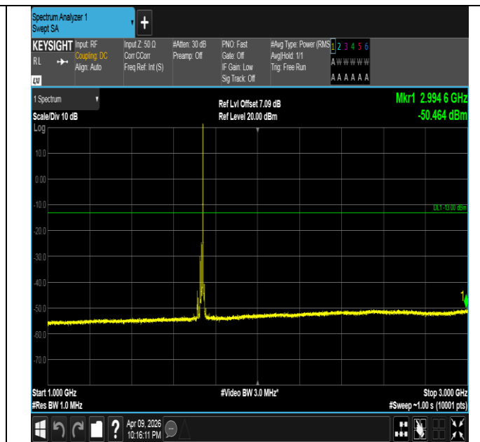
Band4-15MHz-16QAM-20175-1RB#74-1000~3000-PASS
