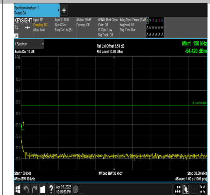
Band4-15MHz-16QAM-20175-1RB#74-0.15~30-PASS
