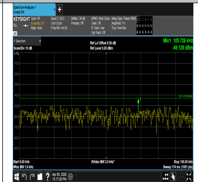
Band4-15MHz-16QAM-20175-75RB#0-0.009~0.15-PASS
