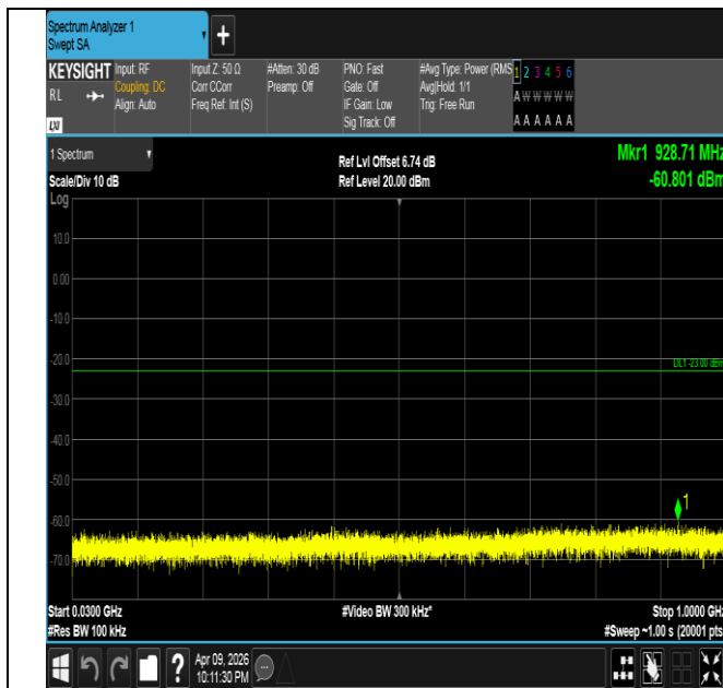
Band4-15MHz-QPSK-20025-75RB#0-30~1000-PASS
