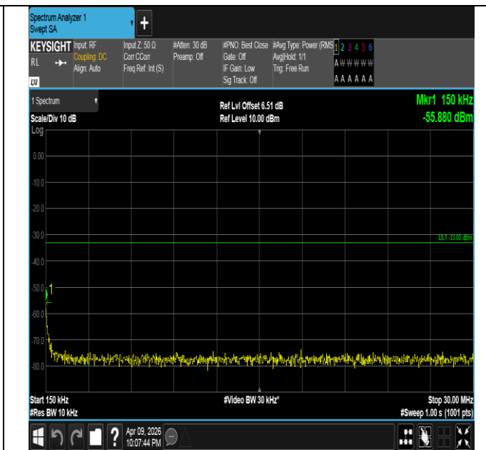
Band4-15MHz-QPSK-20025-1RB#0-0.15~30-PASS
