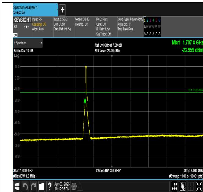
Band4-15MHz-16QAM-20025-75RB#0-1000~3000-PASS
