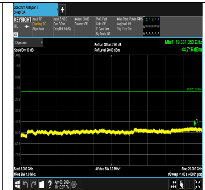
Band4-15MHz-QPSK-20025-1RB#74-3000~20000-PASS
