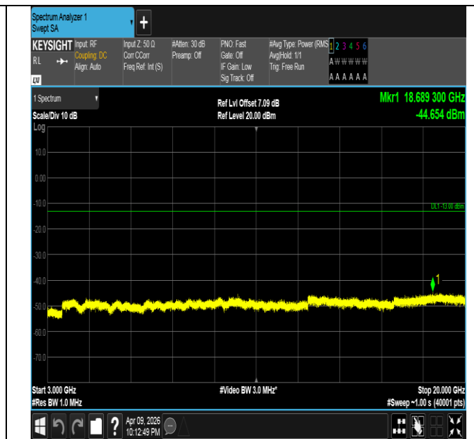
Band4-15MHz-16QAM-20025-75RB#0-3000~20000-PASS
