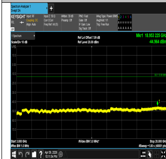
Band4-15MHz-QPSK-20025-75RB#0-3000~20000-PASS
