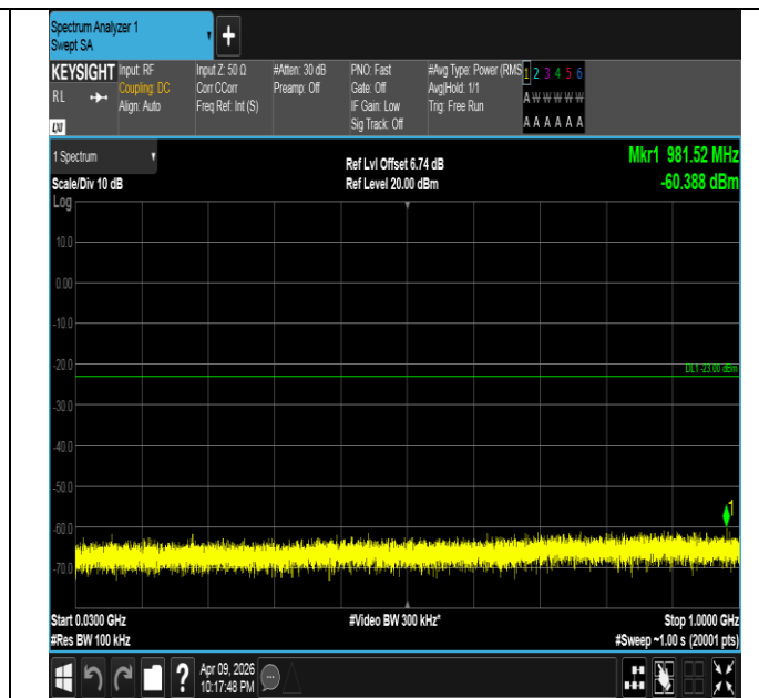
Band4-15MHz-16QAM-20175-75RB#0-30~1000-PASS
