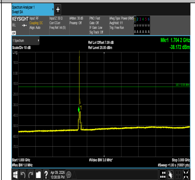
Band4-15MHz-QPSK-20025-1RB#0-1000~3000-PASS
