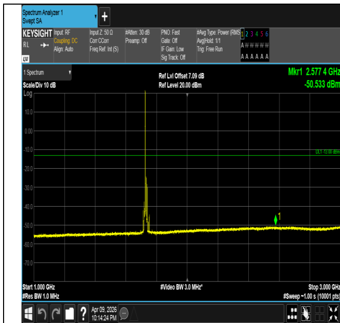
Band4-15MHz-16QAM-20175-1RB#0-1000~3000-PASS
