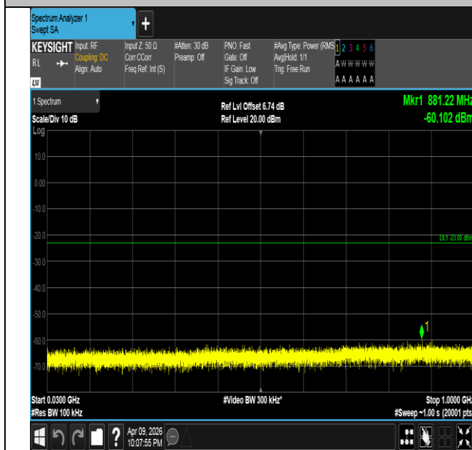
Band4-15MHz-QPSK-20025-1RB#0-30~1000-PASS
