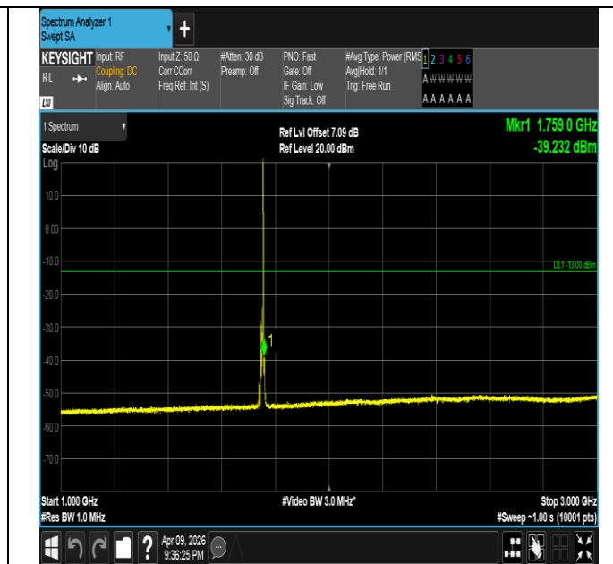
Band4-10MHz-16QAM-20350-1RB#49-1000~3000-PASS
