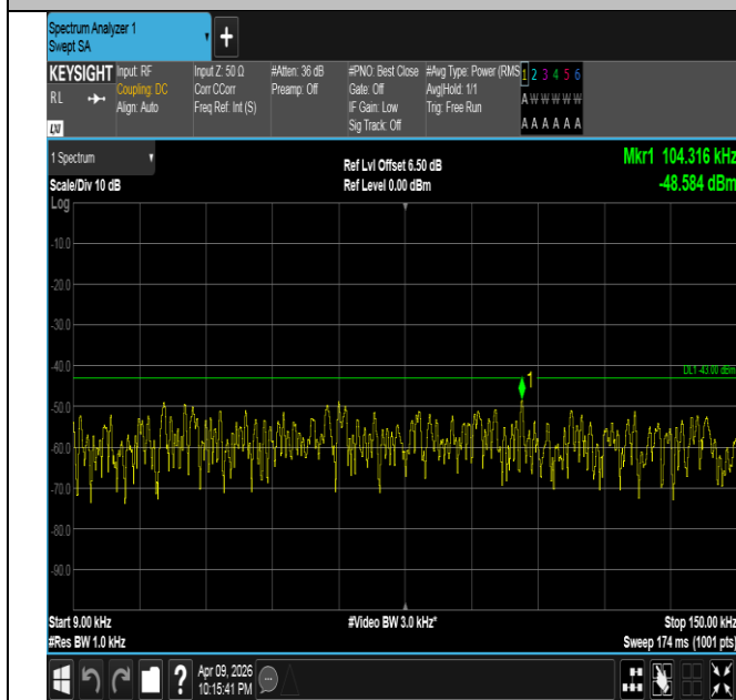
Band4-15MHz-16QAM-20175-1RB#74-0.009~0.15-PASS
