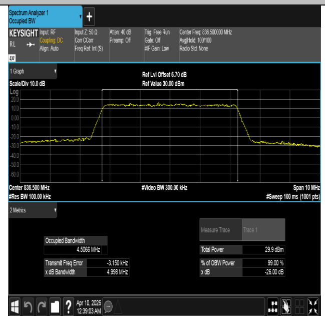
Band5-5MHz-16QAM-20525-25RB#0-PASS
