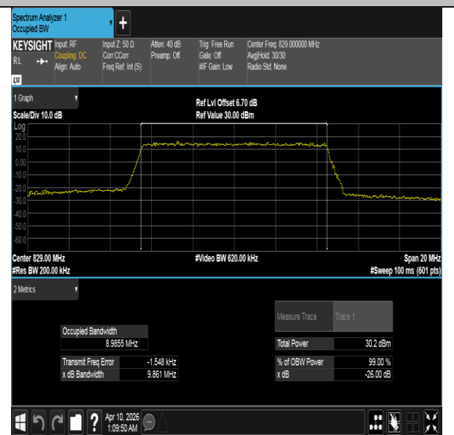
Band5-10MHz-16QAM-20450-50RB#0-PASS
