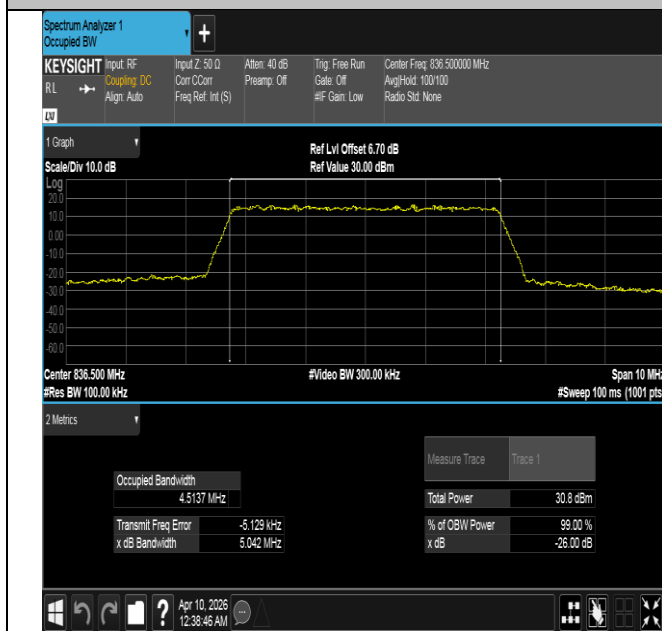
Band5-5MHz-QPSK-20525-25RB#0-PASS
