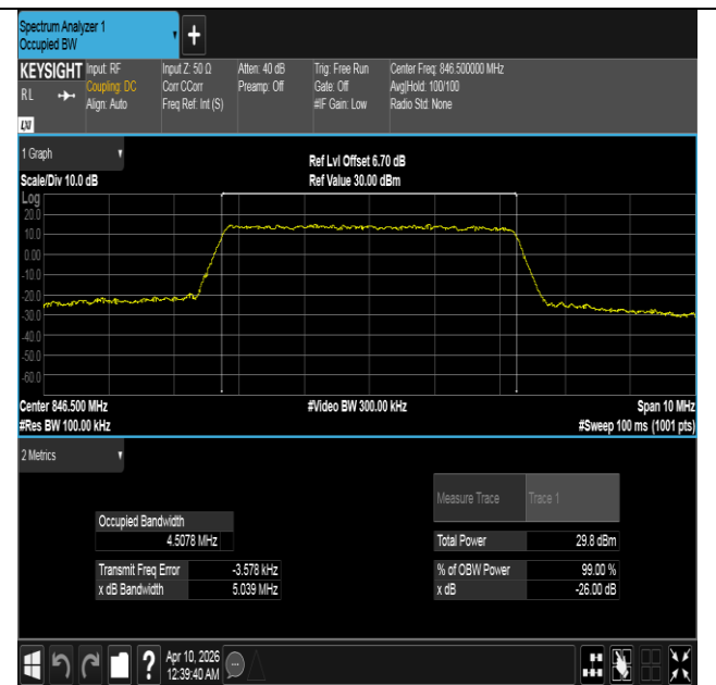
Band5-5MHz-16QAM-20625-25RB#0-PASS
