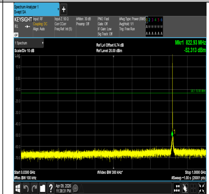
Band5-1.4MHz-16QAM-20407-1RB#0-30~1000-PASS
