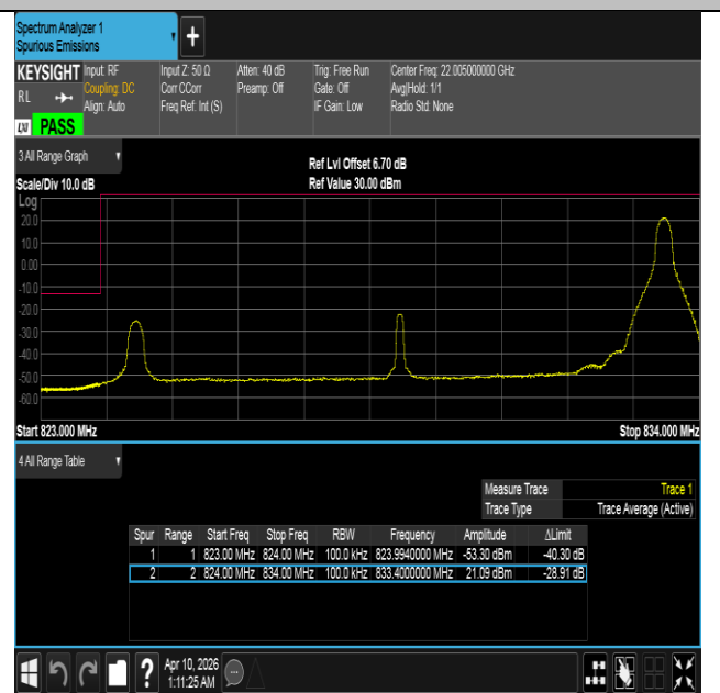
Band5-10MHz-QPSK-20450-1RB#49-PASS
