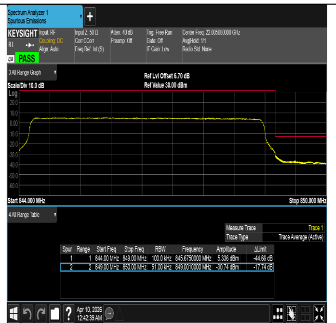
Band5-5MHz-16QAM-20625-25RB#0-PASS
