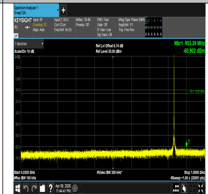
Band5-1.4MHz-QPSK-20525-1RB#5-30~1000-PASS
