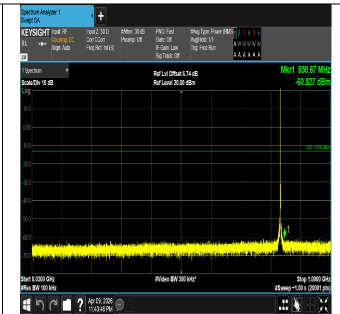
Band5-1.4MHz-16QAM-20525-1RB#0-30~1000-PASS
