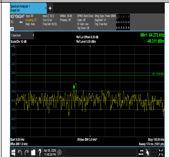
Band5-1.4MHz-QPSK-20643-1RB#5-0.009~0.15-PASS
