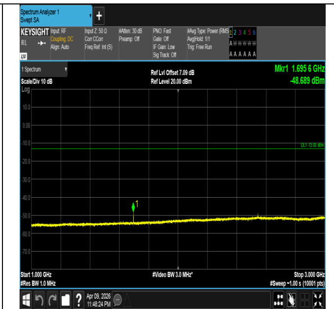
Band5-1.4MHz-QPSK-20643-1RB#0-1000~3000-PASS
