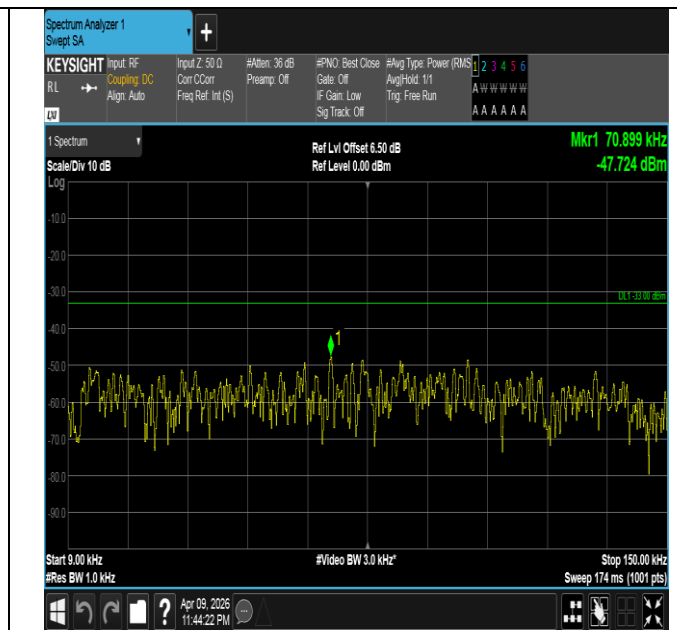
Band5-1.4MHz-QPSK-20525-1RB#5-0.009~0.15-PASS
