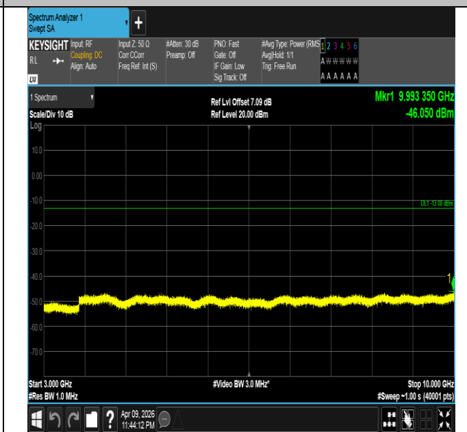
Band5-1.4MHz-16QAM-20525-1RB#0-3000~10000-PASS
