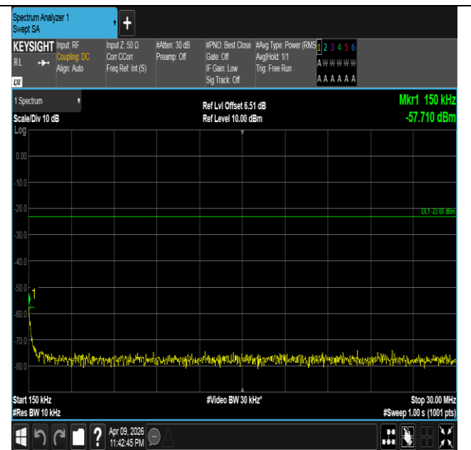
Band5-1.4MHz-QPSK-20525-1RB#0-0.15~30-PASS
