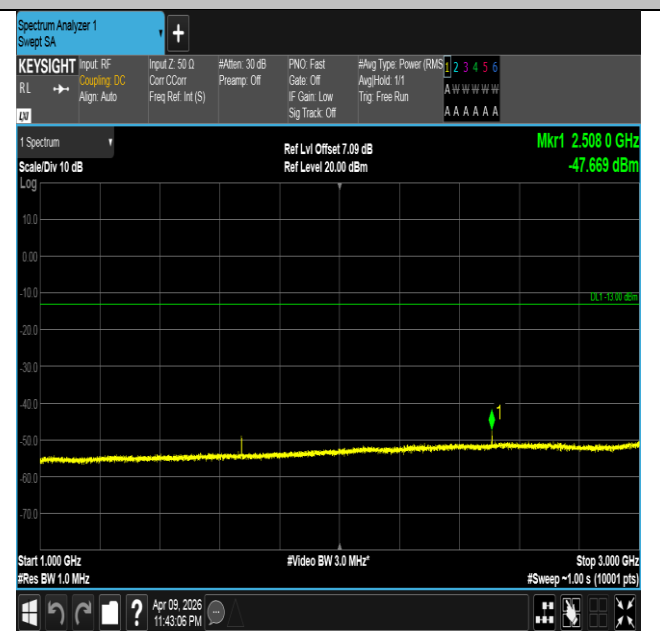
Band5-1.4MHz-QPSK-20525-1RB#0-1000~3000-PASS
