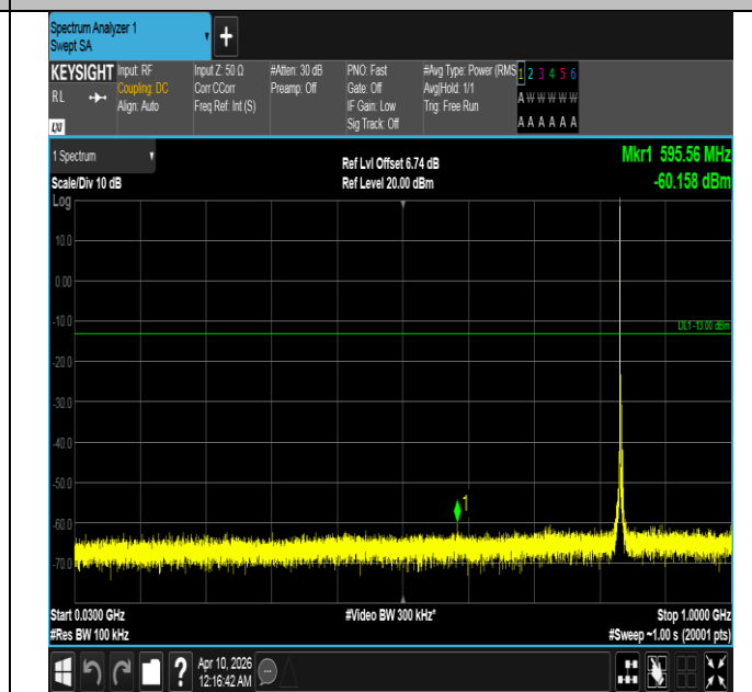
Band5-3MHz-16QAM-20525-1RB#0-30~1000-PASS
