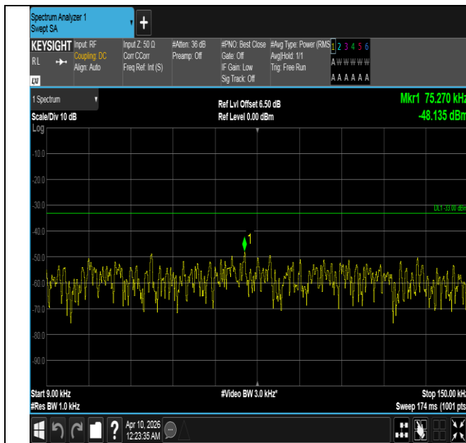
Band5-3MHz-16QAM-20635-1RB#14-0.009~0.15-PASS
