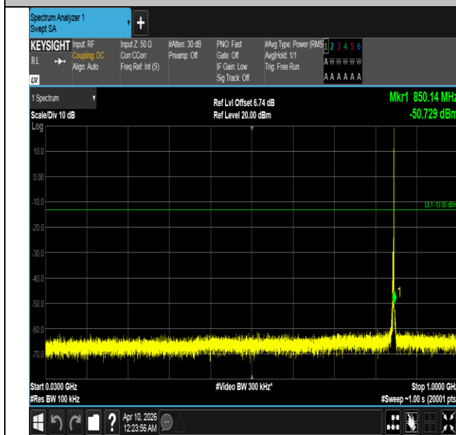
Band5-3MHz-16QAM-20635-1RB#14-30~1000-PASS
