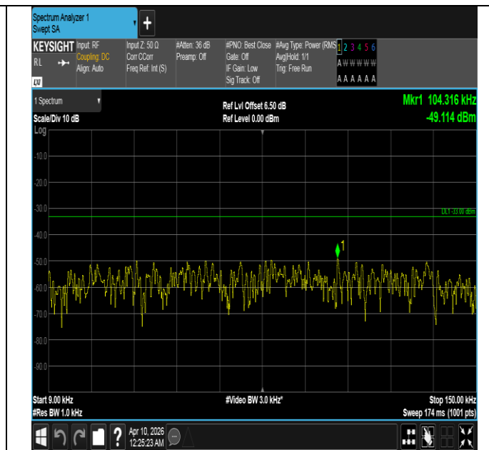
Band5-3MHz-16QAM-20635-15RB#0-0.009~0.15-PASS
