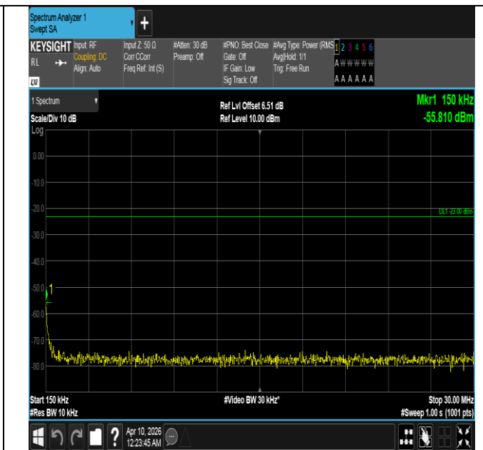
Band5-3MHz-16QAM-20635-1RB#14-0.15~30-PASS
