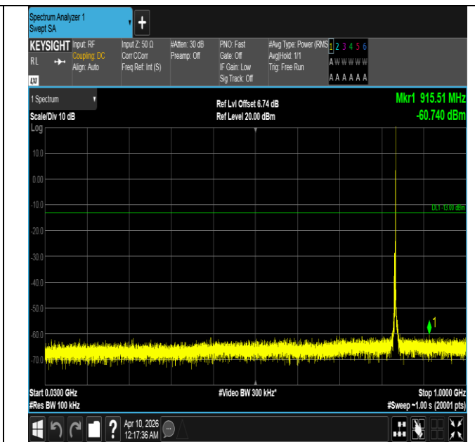
Band5-3MHz-QPSK-20525-1RB#14-30~1000-PASS
