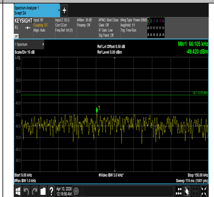
Band5-3MHz-16QAM-20525-15RB#0-0.009~0.15-PASS
