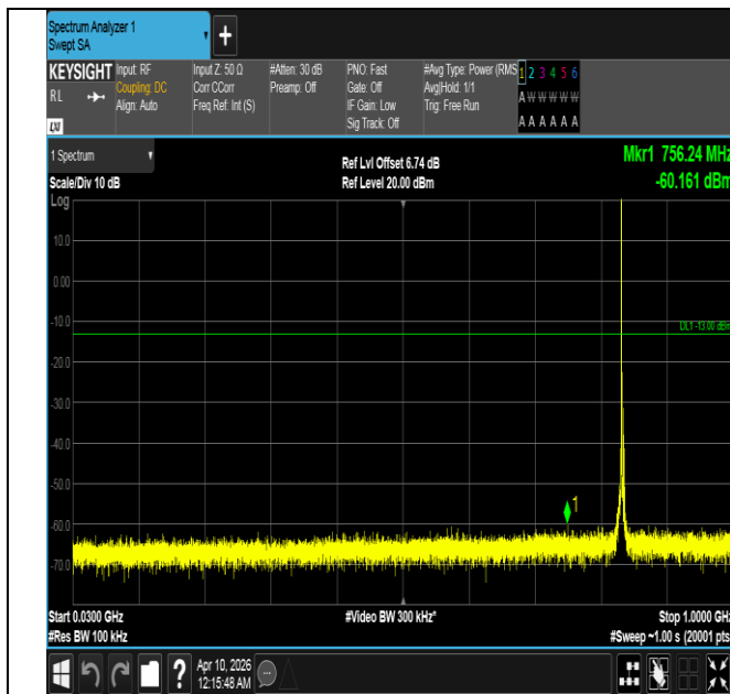
Band5-3MHz-QPSK-20525-1RB#0-30~1000-PASS
