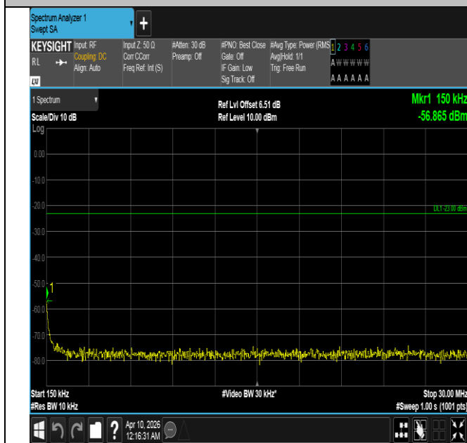
Band5-3MHz-16QAM-20525-1RB#0-0.15~30-PASS
