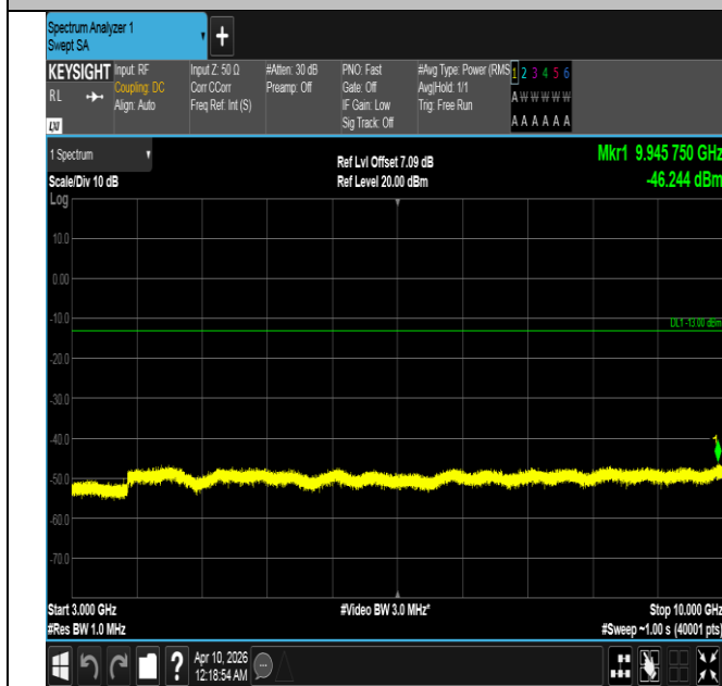
Band5-3MHz-16QAM-20525-1RB#14-3000~10000-PASS
