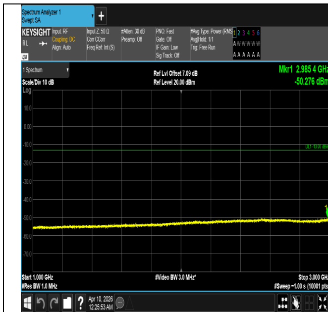
Band5-3MHz-16QAM-20635-15RB#0-1000~3000-PASS
