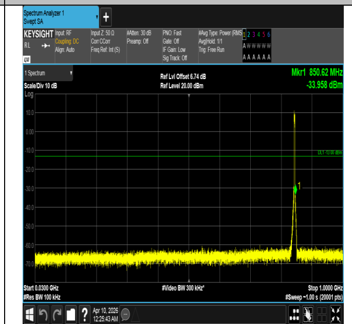
Band5-3MHz-16QAM-20635-15RB#0-30~1000-PASS
