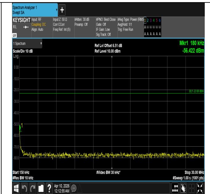
Band5-3MHz-16QAM-20415-1RB#14-0.15~30-PASS
