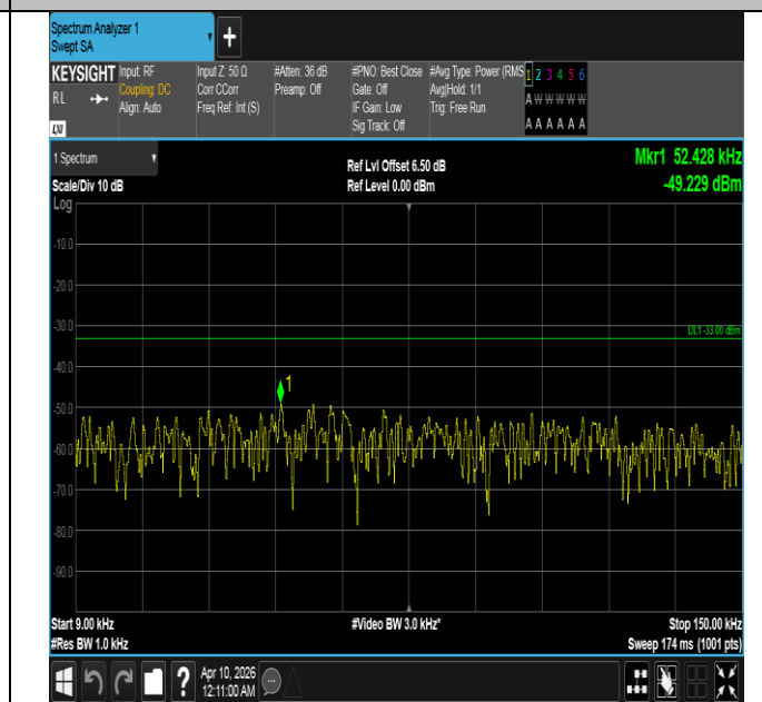
Band5-3MHz-16QAM-20415-1RB#0-0.009~0.15-PASS
