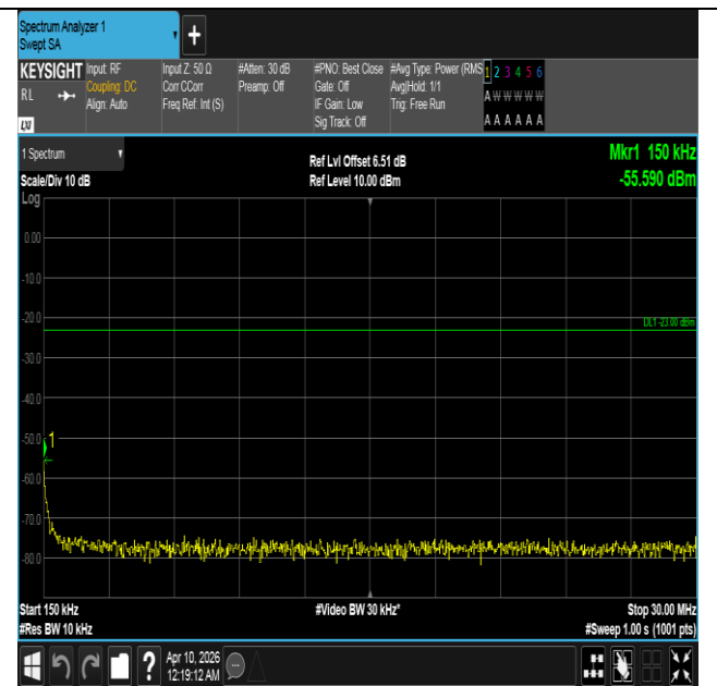
Band5-3MHz-QPSK-20525-15RB#0-0.15~30-PASS
