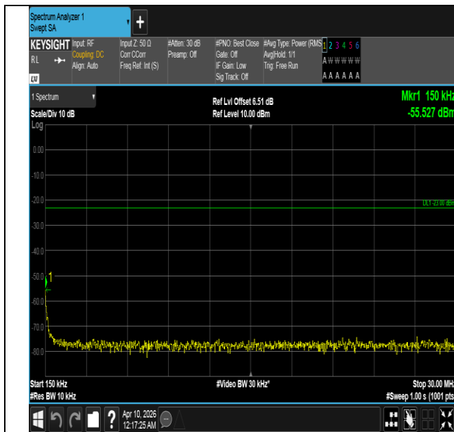
Band5-3MHz-QPSK-20525-1RB#14-0.15~30-PASS
