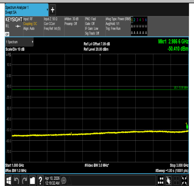
Band5-3MHz-QPSK-20525-15RB#0-1000~3000-PASS
