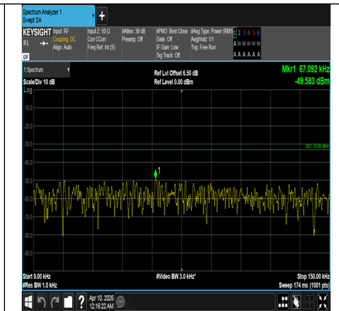
Band5-3MHz-16QAM-20525-1RB#0-0.009~0.15-PASS
