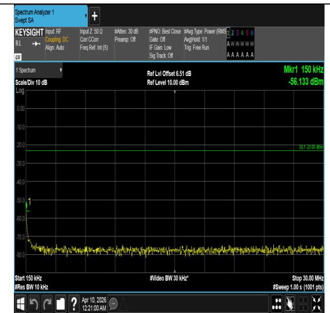
Band5-3MHz-QPSK-20635-1RB#0-0.15~30-PASS
