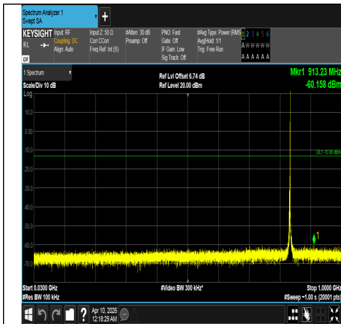
Band5-3MHz-16QAM-20525-1RB#14-30~1000-PASS
