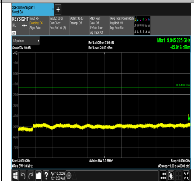
Band5-3MHz-QPSK-20525-1RB#14-3000~10000-PASS
