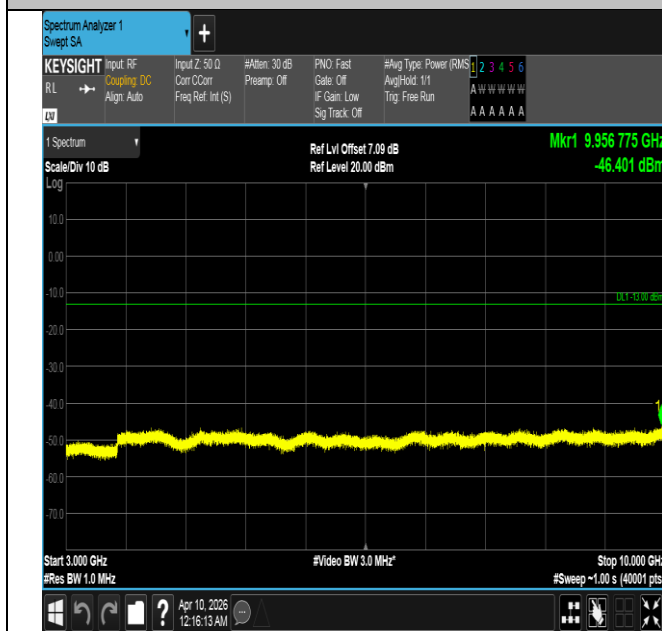
Band5-3MHz-QPSK-20525-1RB#0-3000~10000-PASS
