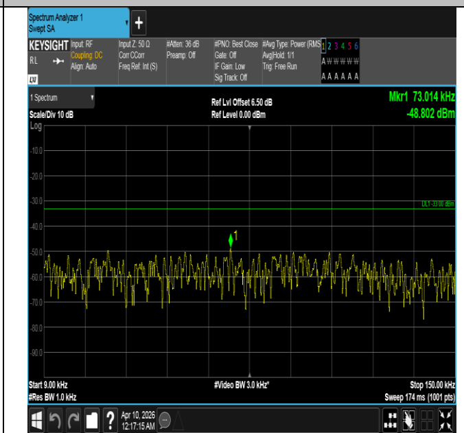
Band5-3MHz-QPSK-20525-1RB#14-0.009~0.15-PASS
