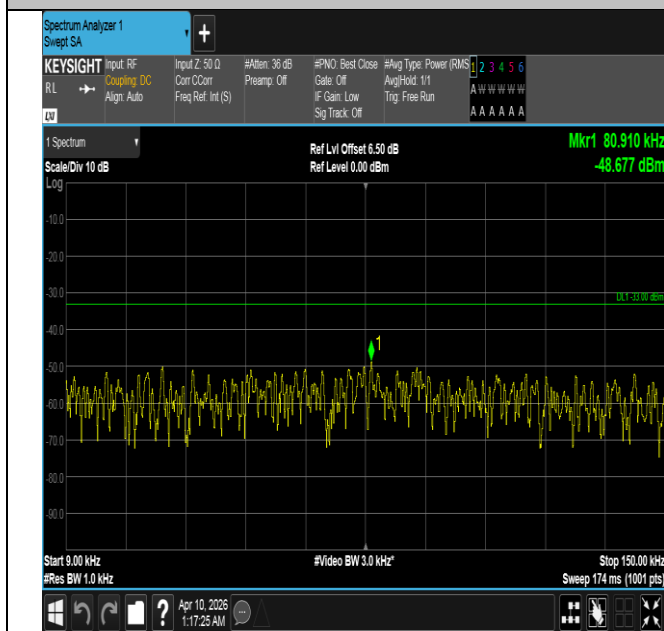
Band5-10MHz-QPSK-20450-50RB#0-0.009~0.15-PASS
