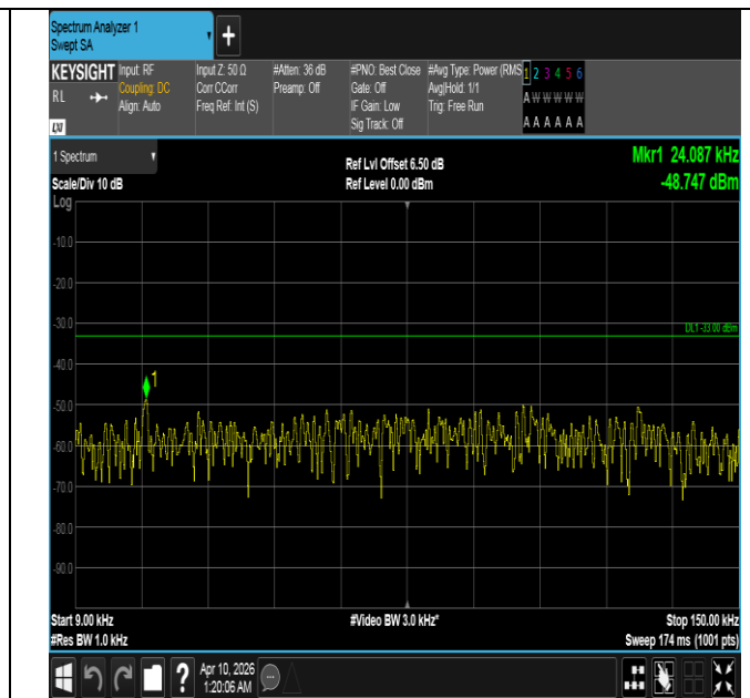
Band5-10MHz-16QAM-20525-1RB#0-0.009~0.15-PASS
