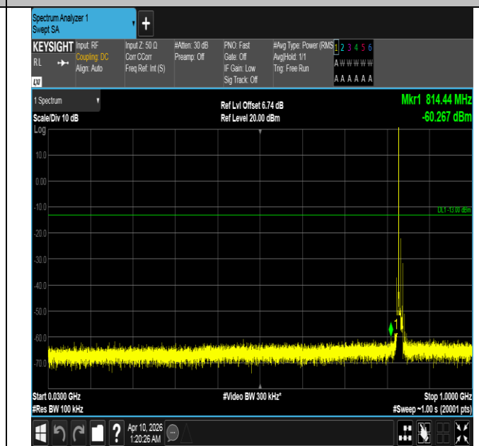
Band5-10MHz-16QAM-20525-1RB#0-30~1000-PASS
