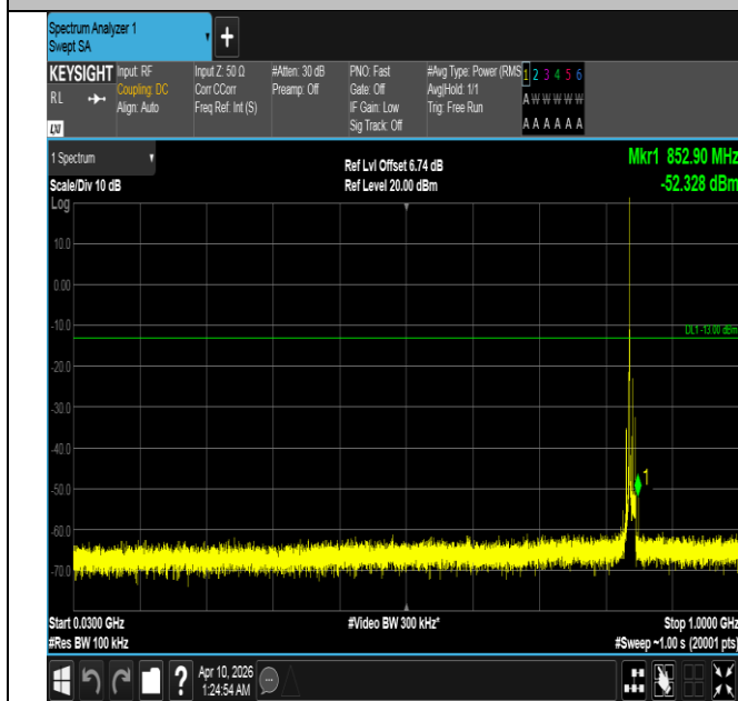
Band5-10MHz-QPSK-20600-1RB#0-30~1000-PASS
