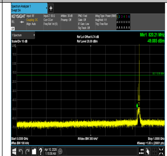
Band5-10MHz-QPSK-20450-1RB#49-30~1000-PASS
