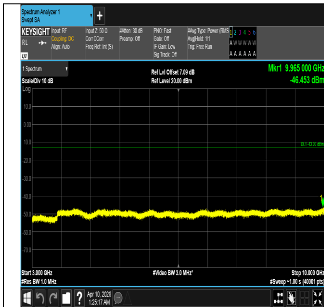
Band5-10MHz-QPSK-20600-1RB#0-3000~10000-PASS
