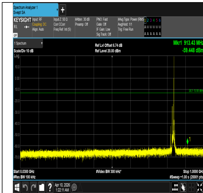
Band5-10MHz-16QAM-20525-1RB#49-30~1000-PASS
