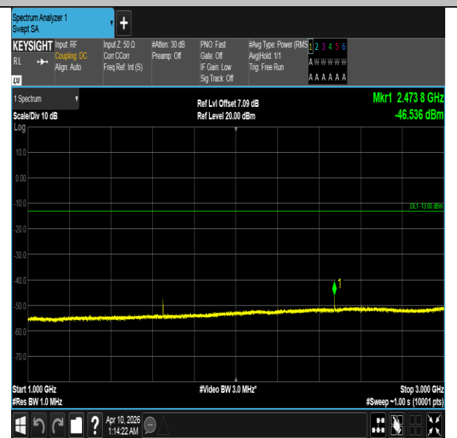
Band5-10MHz-QPSK-20450-1RB#0-1000~3000-PASS
