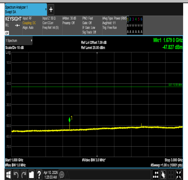
Band5-10MHz-QPSK-20600-1RB#0-1000~3000-PASS
