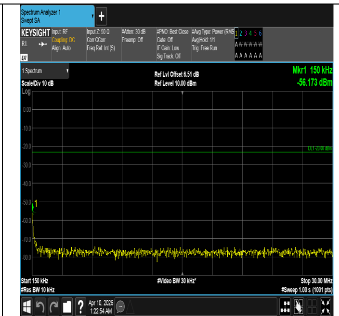
Band5-10MHz-QPSK-20525-50RB#0-0.15~30-PASS
