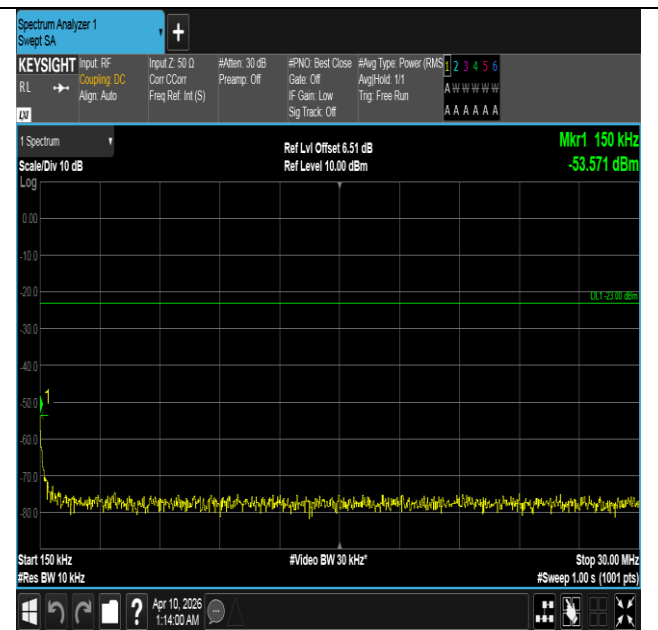
Band5-10MHz-QPSK-20450-1RB#0-0.15~30-PASS
