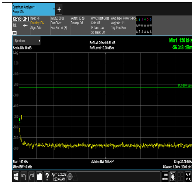
Band5-10MHz-16QAM-20525-50RB#0-0.15~30-PASS
