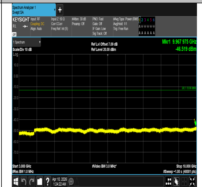
Band5-10MHz-16QAM-20525-50RB#0-3000~10000-PASS
