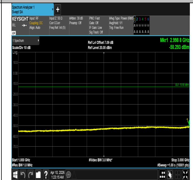
Band5-10MHz-QPSK-20525-50RB#0-1000~3000-PASS
