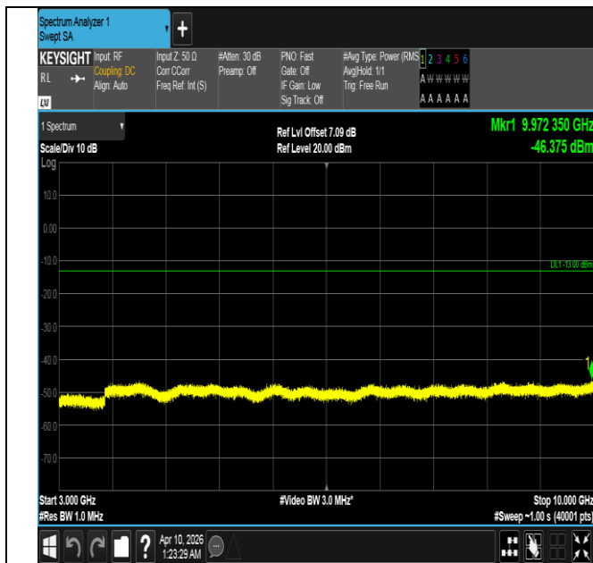
Band5-10MHz-QPSK-20525-50RB#0-3000~10000-PASS
