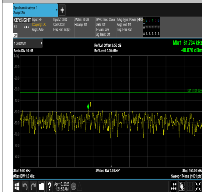
Band5-10MHz-16QAM-20525-1RB#49-0.009~0.15-PASS
