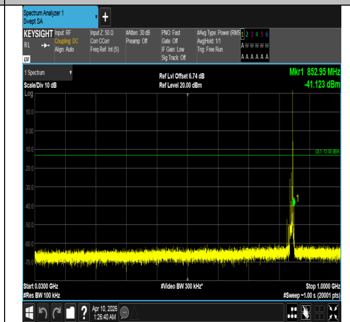
Band5-10MHz-QPSK-20600-1RB#49-30~1000-PASS
