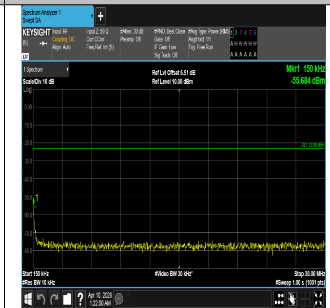
Band5-10MHz-16QAM-20525-1RB#49-0.15~30-PASS
