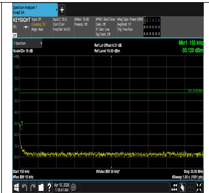
Band5-10MHz-16QAM-20450-1RB#49-0.15~30-PASS
