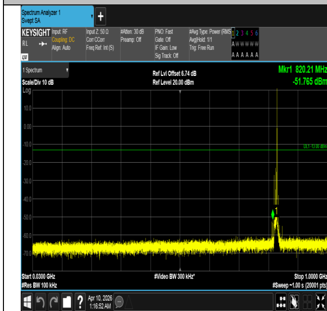
Band5-10MHz-16QAM-20450-1RB#49-30~1000-PASS
