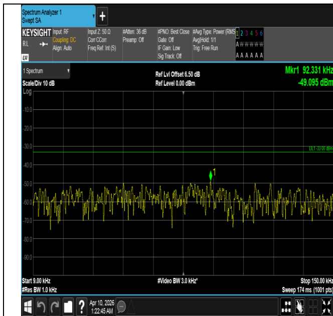
Band5-10MHz-QPSK-20525-50RB#0-0.009~0.15-PASS
