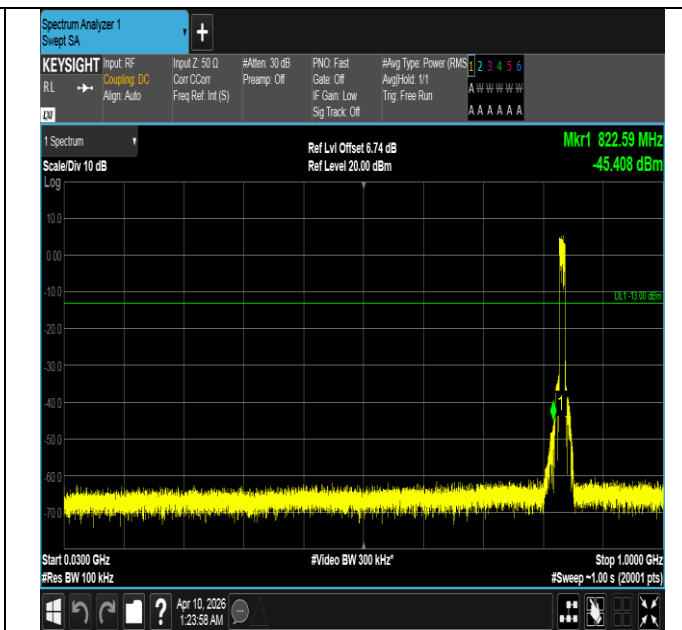
Band5-10MHz-16QAM-20525-50RB#0-30~1000-PASS
