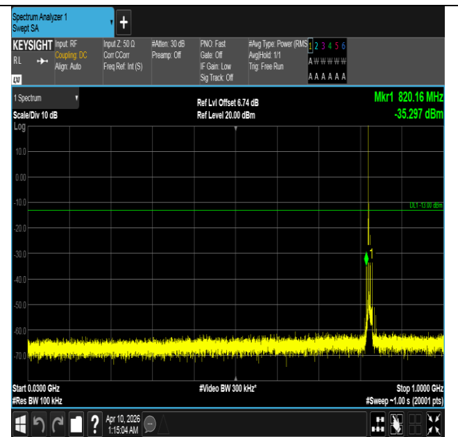
Band5-10MHz-16QAM-20450-1RB#0-30~1000-PASS
