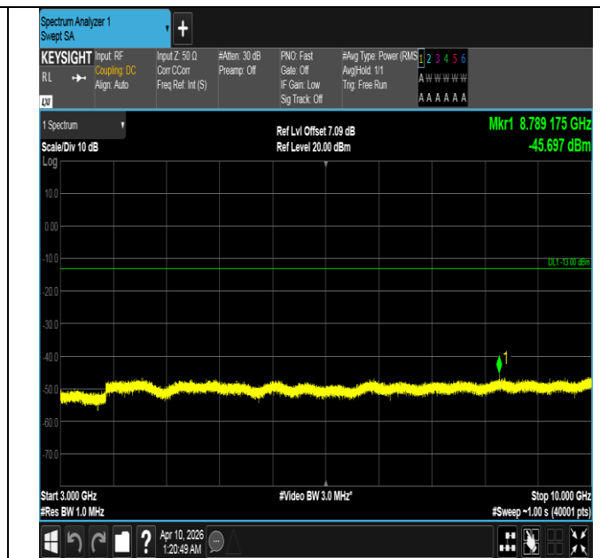
Band5-10MHz-16QAM-20525-1RB#0-3000~10000-PASS
