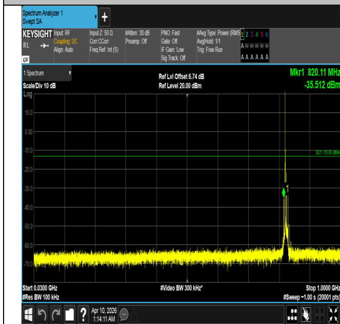
Band5-10MHz-QPSK-20450-1RB#0-30~1000-PASS
