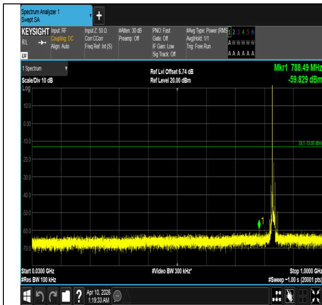
Band5-10MHz-QPSK-20525-1RB#0-30~1000-PASS
