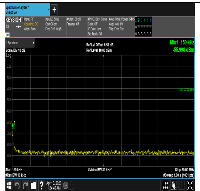
Band5-10MHz-QPSK-20600-1RB#0-0.15~30-PASS
