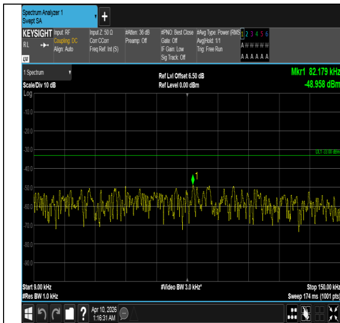
Band5-10MHz-16QAM-20450-1RB#49-0.009~0.15-PASS
