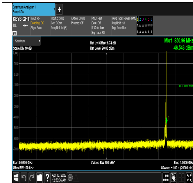
Band5-5MHz-16QAM-20625-1RB#24-30~1000-PASS
