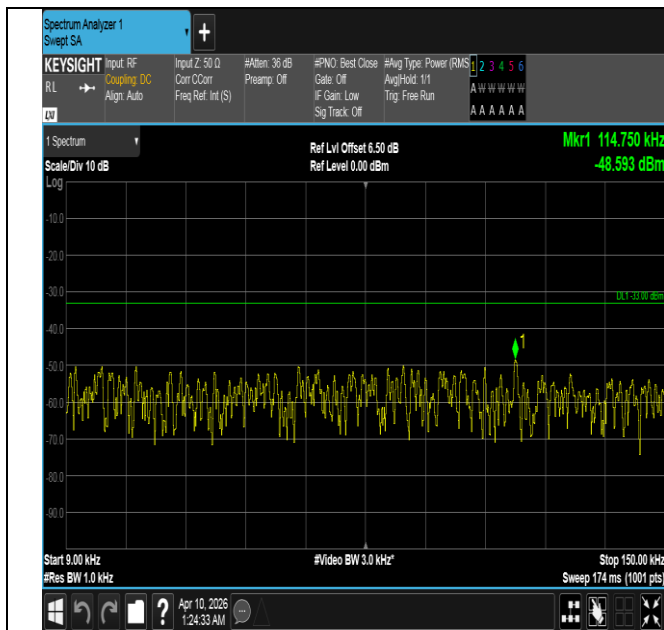
Band5-10MHz-QPSK-20600-1RB#0-0.009~0.15-PASS
