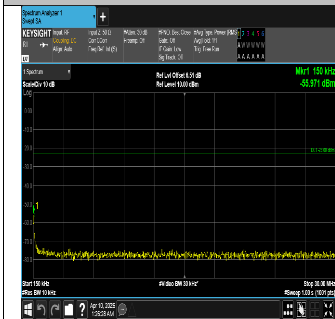
Band5-10MHz-QPSK-20600-1RB#49-0.15~30-PASS
