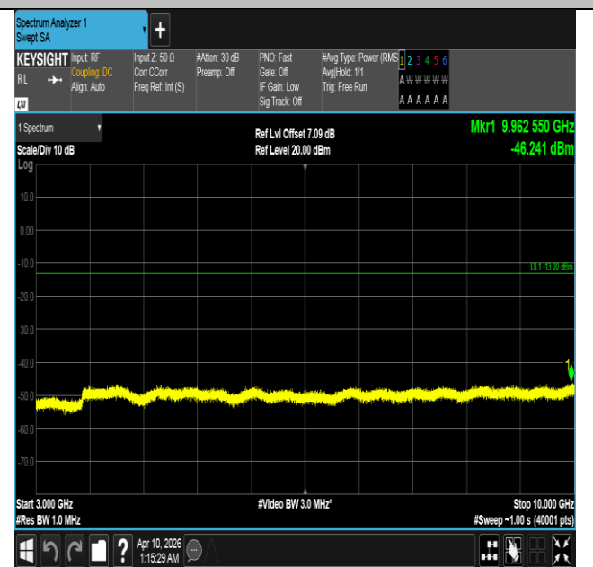
Band5-10MHz-16QAM-20450-1RB#0-3000~10000-PASS
