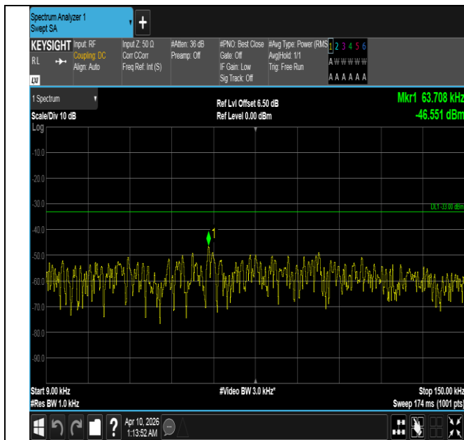
Band5-10MHz-QPSK-20450-1RB#0-0.009~0.15-PASS
