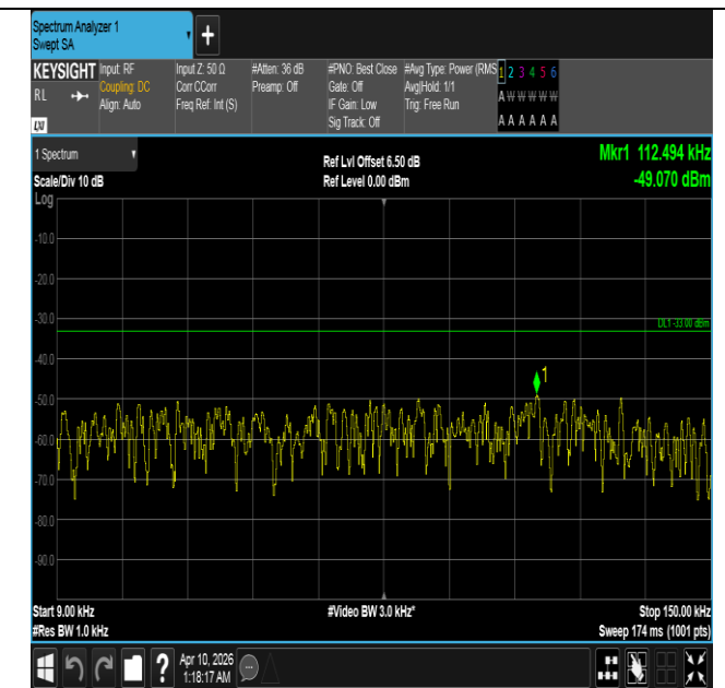
Band5-10MHz-16QAM-20450-50RB#0-0.009~0.15-PASS
