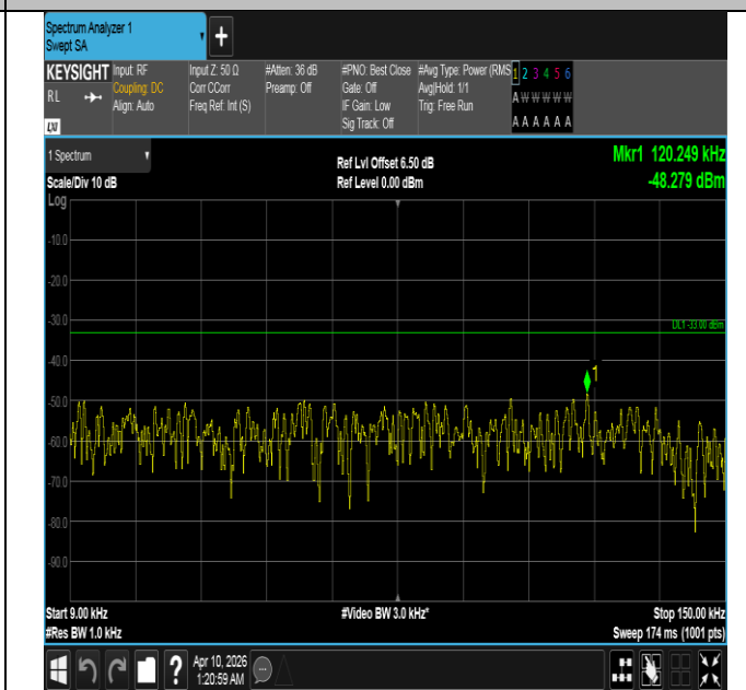
Band5-10MHz-QPSK-20525-1RB#49-0.009~0.15-PASS
