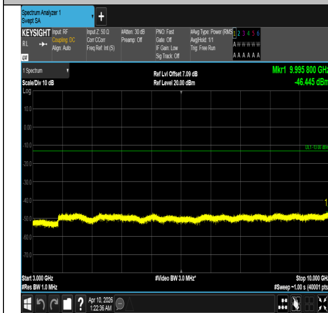
Band5-10MHz-16QAM-20525-1RB#49-3000~10000-PASS
