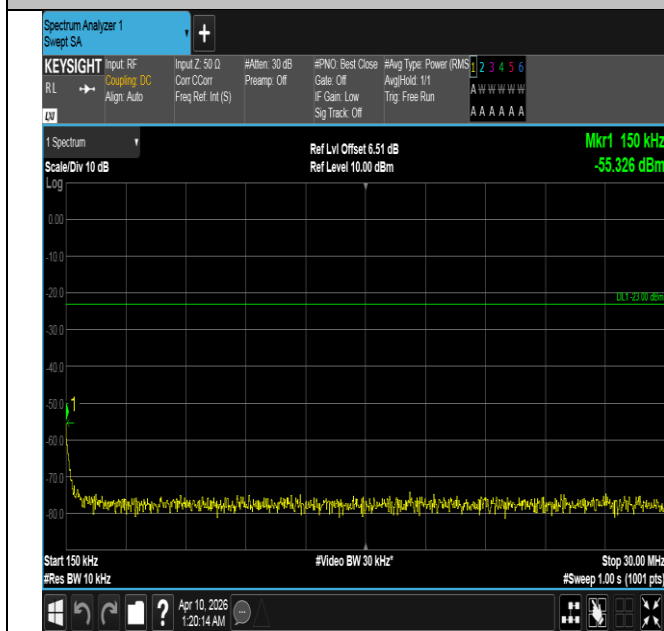
Band5-10MHz-16QAM-20525-1RB#0-0.15~30-PASS
