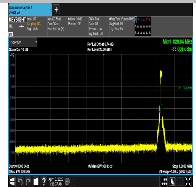
Band5-10MHz-16QAM-20450-50RB#0-30~1000-PASS
