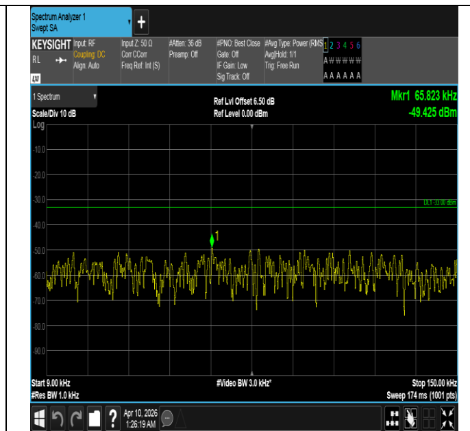
Band5-10MHz-QPSK-20600-1RB#49-0.009~0.15-PASS
