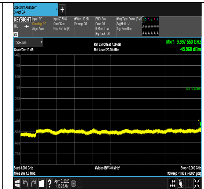
Band5-10MHz-QPSK-20450-1RB#49-3000~10000-PASS
