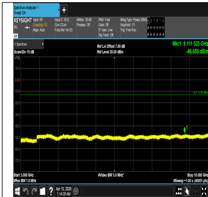
Band5-10MHz-QPSK-20450-1RB#0-3000~10000-PASS
