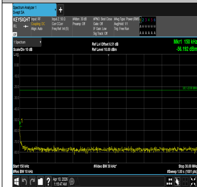
Band5-10MHz-QPSK-20450-1RB#49-0.15~30-PASS
