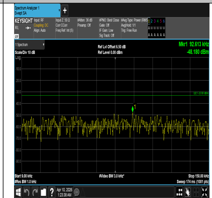
Band5-10MHz-16QAM-20525-50RB#0-0.009~0.15-PASS
