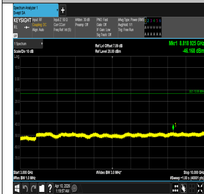
Band5-10MHz-QPSK-20525-1RB#0-3000~10000-PASS
