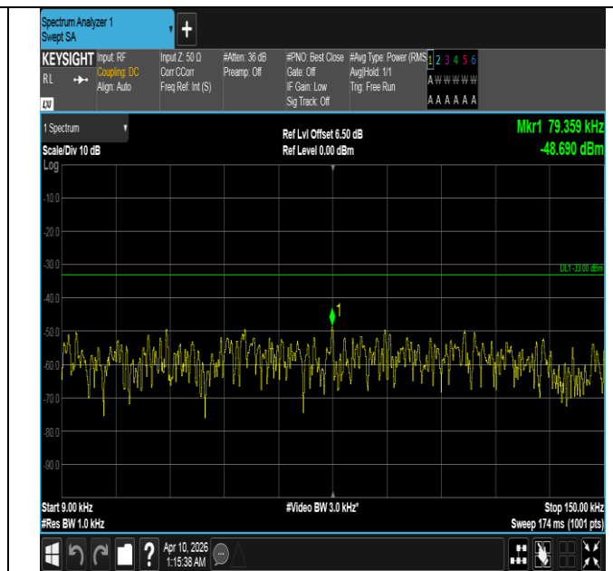
Band5-10MHz-QPSK-20450-1RB#49-0.009~0.15-PASS
