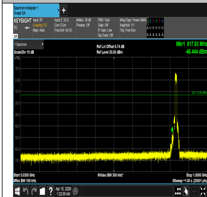
Band5-10MHz-QPSK-20525-50RB#0-30~1000-PASS
