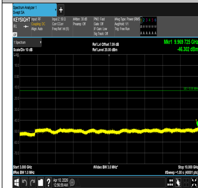
Band5-5MHz-16QAM-20625-1RB#24-3000~10000-PASS
