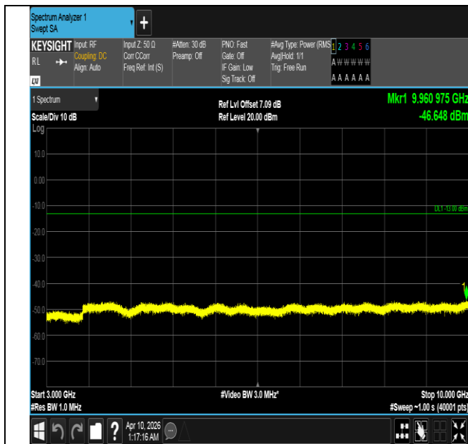
Band5-10MHz-16QAM-20450-1RB#49-3000~10000-PASS
