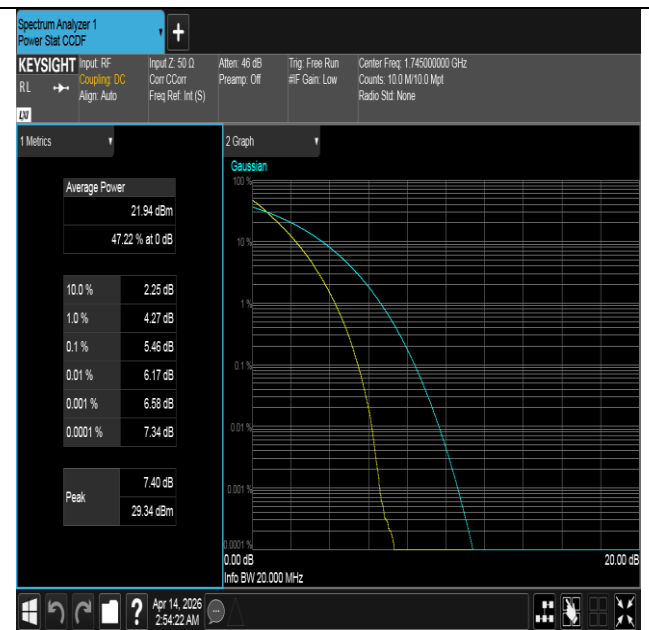
Band66-20MHz-QPSK-132322-100RB#0-PASS
