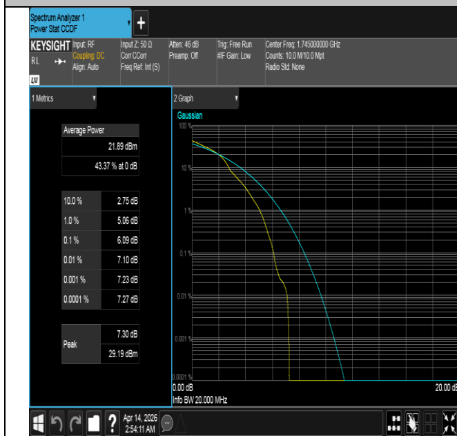
Band66-20MHz-16QAM-132322-1RB#0-PASS
