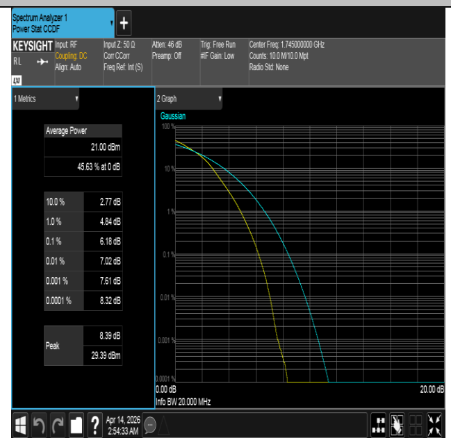
Band66-20MHz-16QAM-132322-100RB#0-PASS
