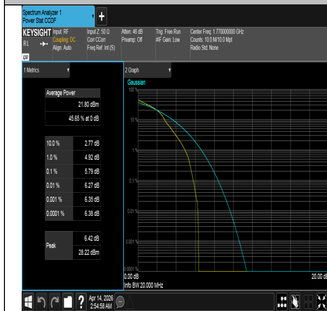
Band66-20MHz-16QAM-132572-1RB#0-PASS
