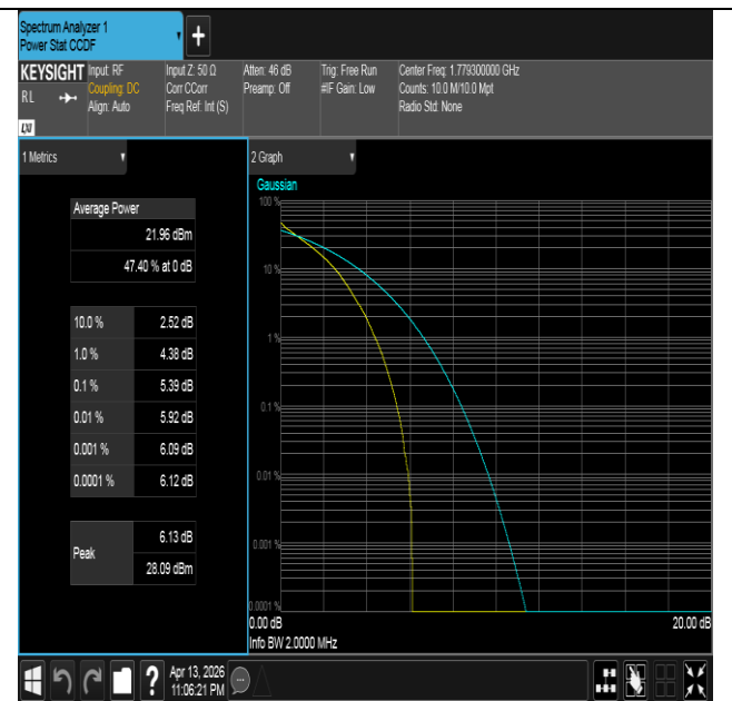
Band66-1.4MHz-QPSK-132665-6RB#0-PASS
