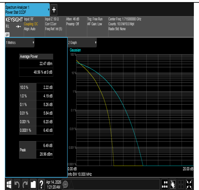
Band66-10MHz-QPSK-132022-50RB#0-PASS
