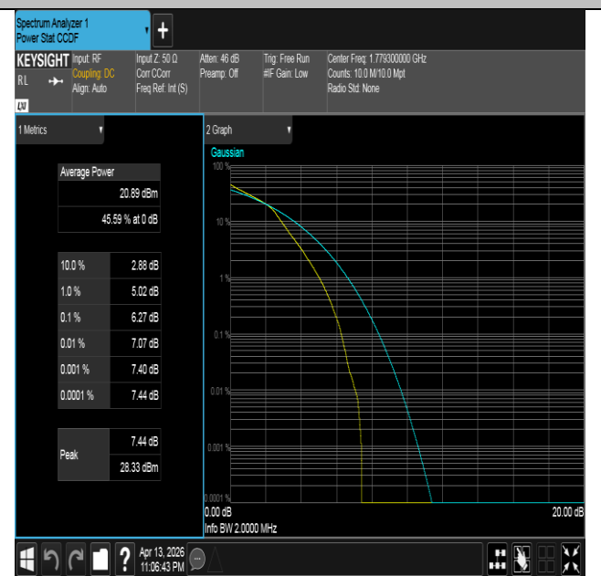
Band66-1.4MHz-16QAM-132665-6RB#0-PASS
