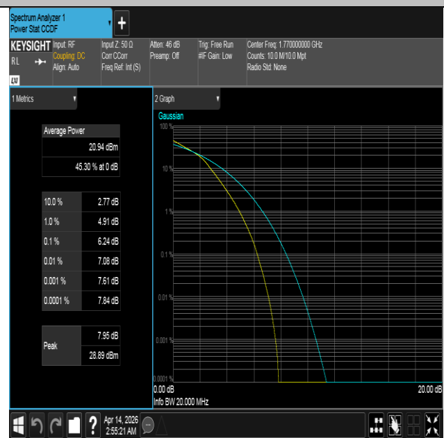
Band66-20MHz-16QAM-132572-100RB#0-PASS
