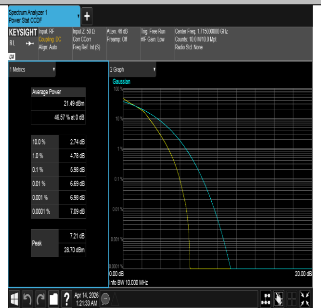
Band66-10MHz-16QAM-132022-50RB#0-PASS
