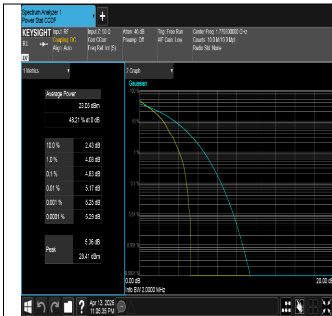
Band66-1.4MHz-QPSK-132665-1RB#0-PASS
