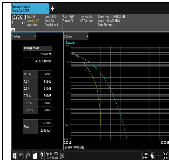
Band66-10MHz-QPSK-132622-1RB#0-PASS
