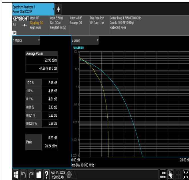
Band66-10MHz-QPSK-132022-1RB#0-PASS
