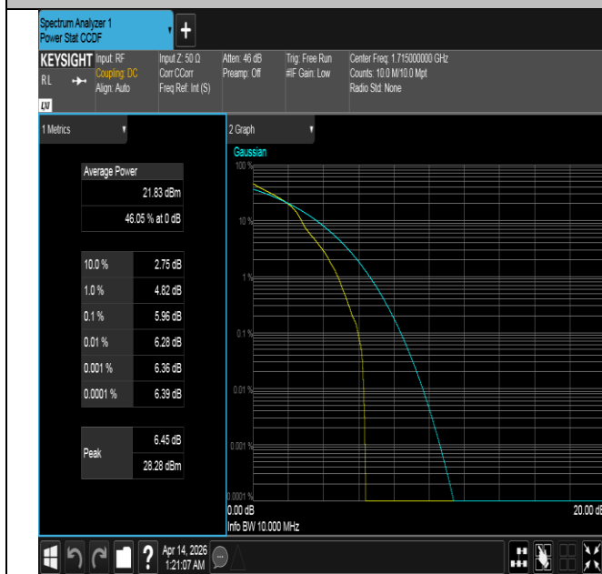
Band66-10MHz-16QAM-132022-1RB#0-PASS
