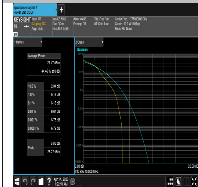
Band66-10MHz-16QAM-132622-1RB#0-PASS
