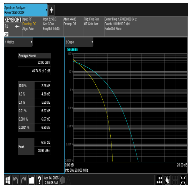
Band66-20MHz-QPSK-132572-100RB#0-PASS
