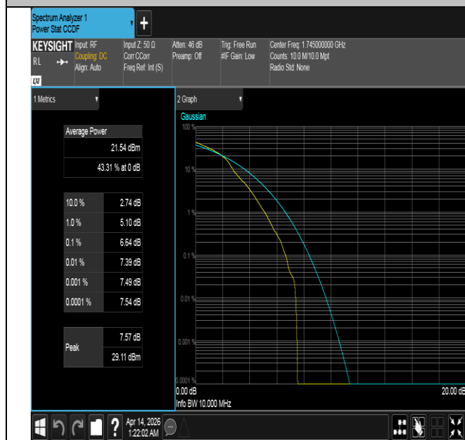
Band66-10MHz-16QAM-132322-1RB#0-PASS
