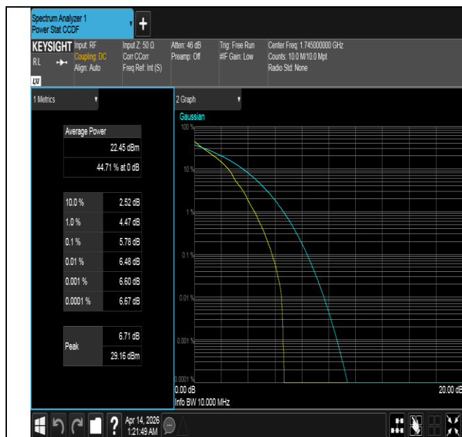
Band66-10MHz-QPSK-132322-1RB#0-PASS
