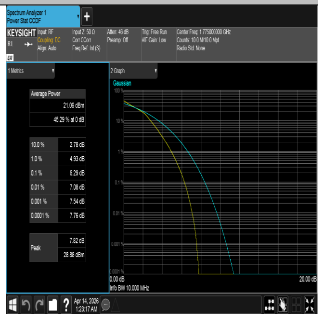
Band66-10MHz-16QAM-132622-50RB#0-PASS
