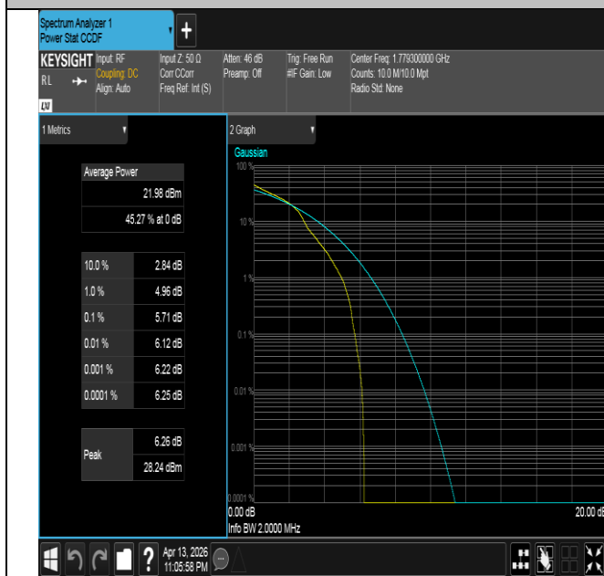
Band66-1.4MHz-16QAM-132665-1RB#0-PASS
