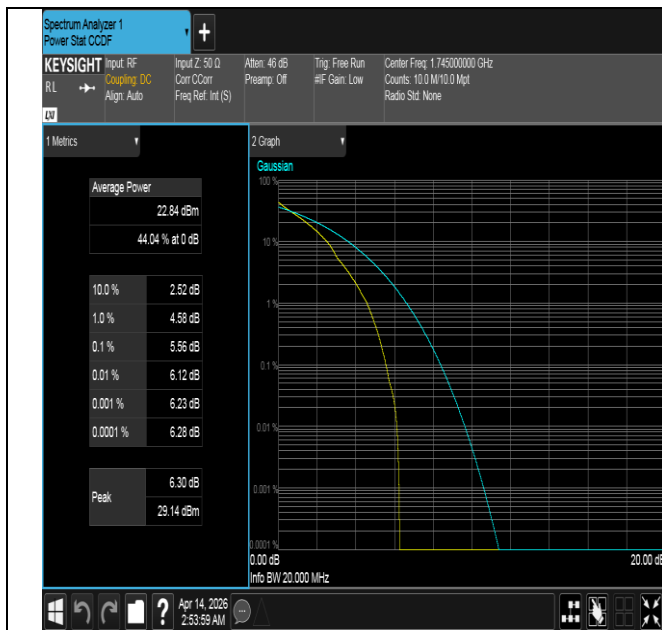
Band66-20MHz-QPSK-132322-1RB#0-PASS
