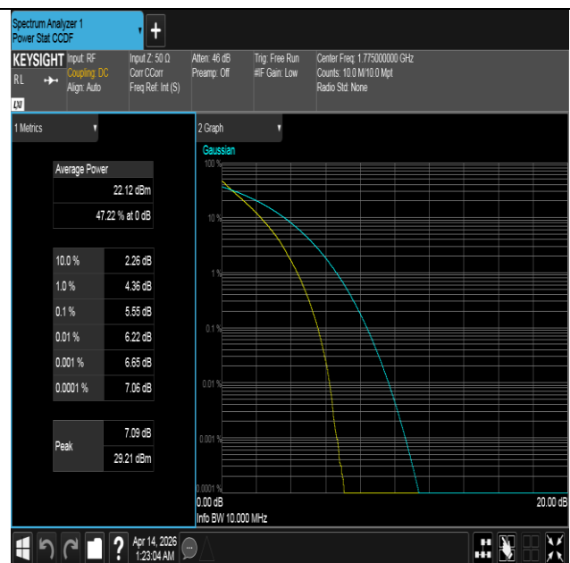
Band66-10MHz-QPSK-132622-50RB#0-PASS
