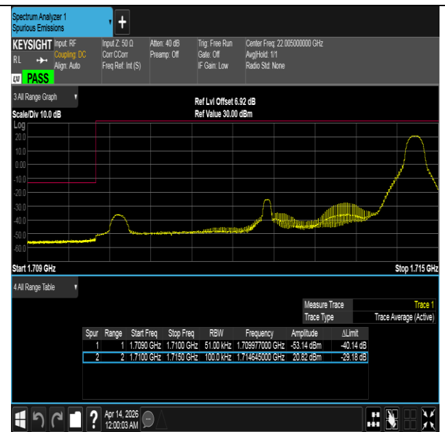
Band66-5MHz-QPSK-131997-1RB#24-PASS
