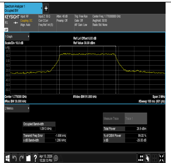
Band66-1.4MHz-16QAM-132665-6RB#0-PASS
