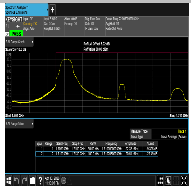
Band66-3MHz-16QAM-131987-1RB#0-PASS
