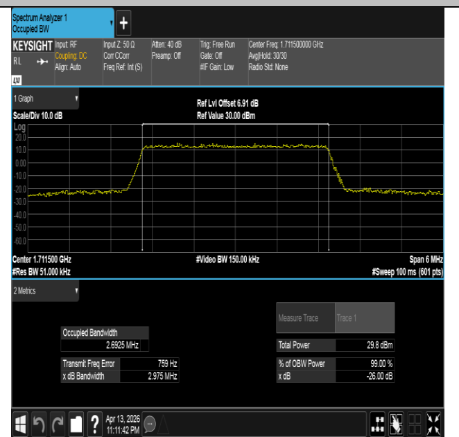
Band66-3MHz-16QAM-131987-15RB#0-PASS
