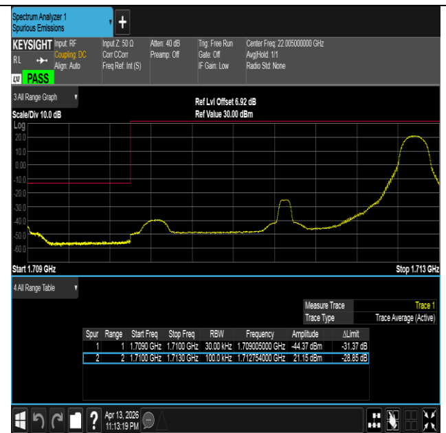
Band66-3MHz-QPSK-131987-1RB#14-PASS
