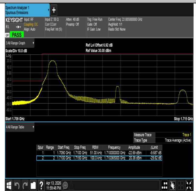
Band66-5MHz-16QAM-131997-1RB#0-PASS
