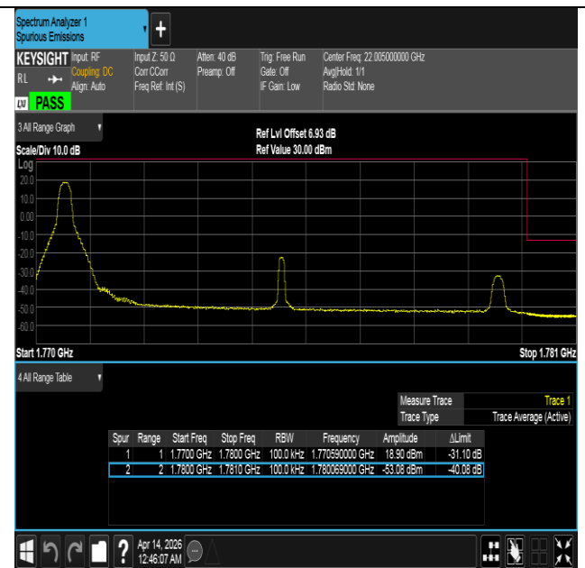
Band66-10MHz-16QAM-132622-1RB#0-PASS
