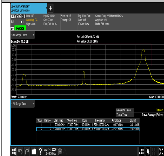
Band66-10MHz-16QAM-132622-1RB#49-PASS
