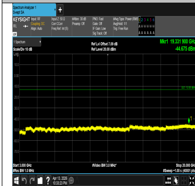
Band66-1.4MHz-QPSK-131979-6RB#0-3000~20000-PASS
