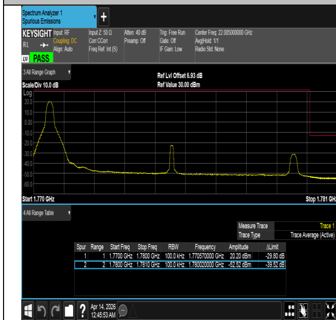
Band66-10MHz-QPSK-132622-1RB#0-PASS
