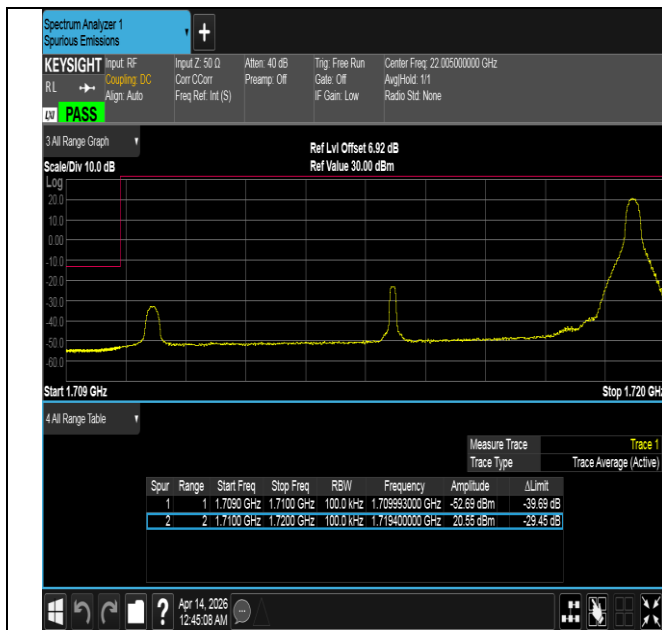
Band66-10MHz-16QAM-132022-1RB#49-PASS
