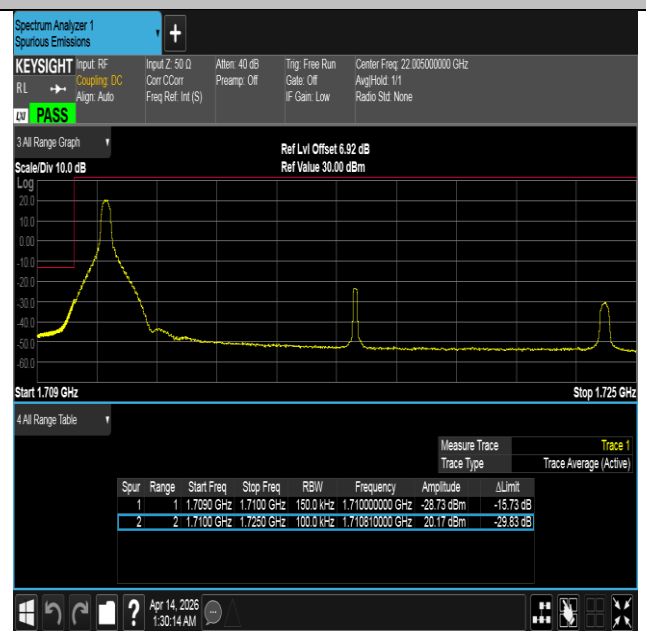
Band66-15MHz-16QAM-132047-1RB#0-PASS
