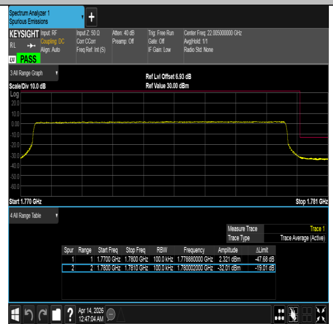
Band66-10MHz-16QAM-132622-50RB#0-PASS
