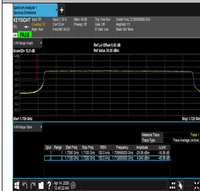
Band66-10MHz-QPSK-132022-50RB#0-PASS
