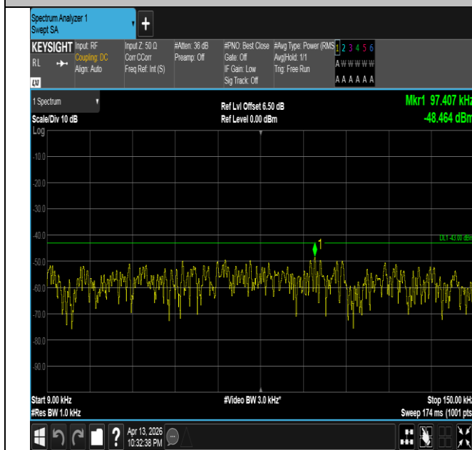
Band66-1.4MHz-QPSK-131979-6RB#0-0.009~0.15-PASS
