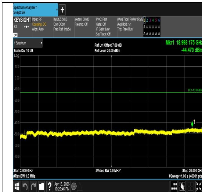
Band66-1.4MHz-QPSK-131979-1RB#0-3000~20000-PASS
