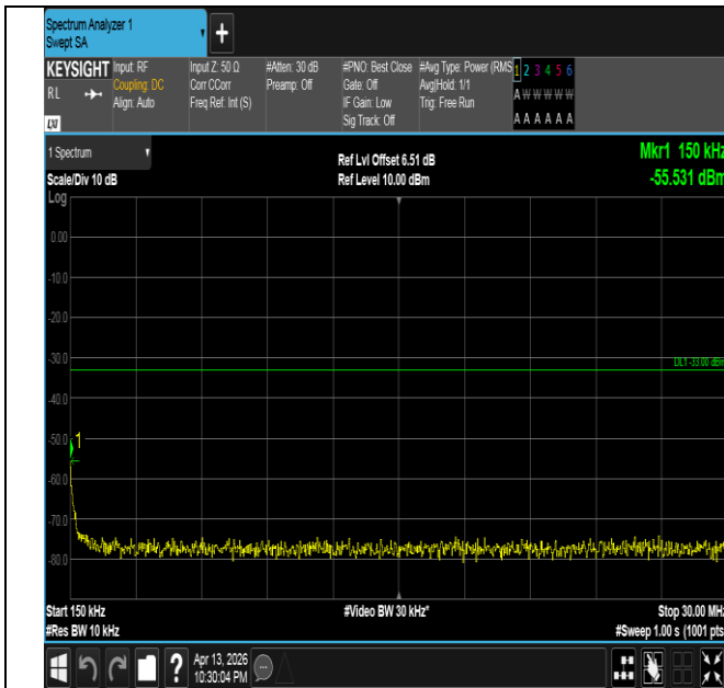
Band66-1.4MHz-16QAM-131979-1RB#0-0.15~30-PASS
