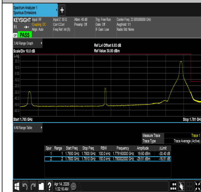
Band66-15MHz-16QAM-132597-1RB#74-PASS
