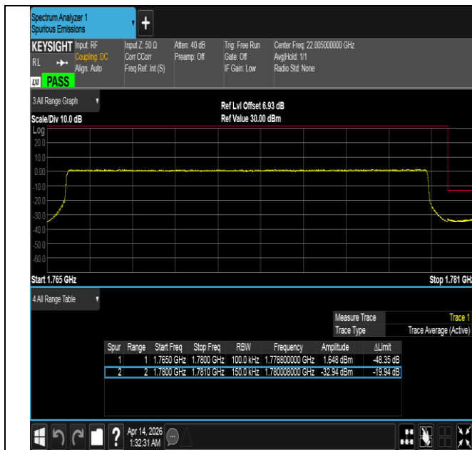
Band66-15MHz-QPSK-132597-75RB#0-PASS
