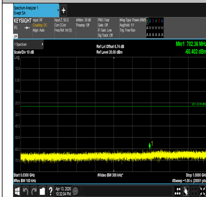
Band66-1.4MHz-16QAM-131979-1RB#5-30~1000-PASS
