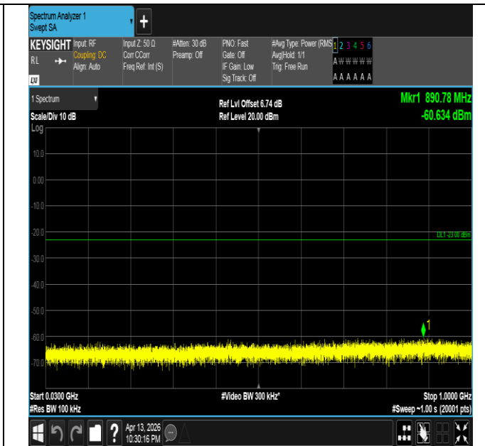
Band66-1.4MHz-16QAM-131979-1RB#0-30~1000-PASS
