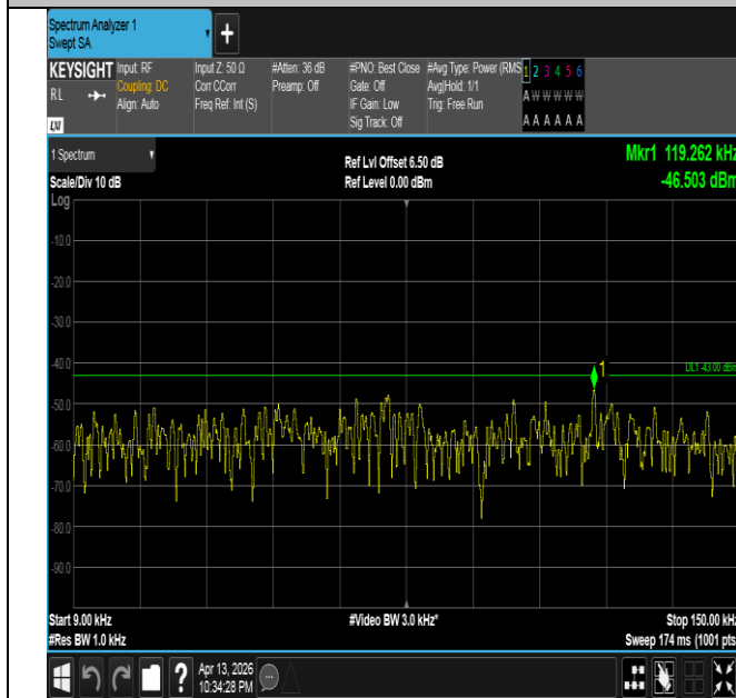
Band66-1.4MHz-QPSK-132322-1RB#0-0.009~0.15-PASS
