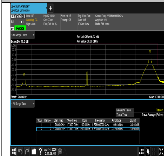
Band66-20MHz-16QAM-132572-1RB#99-PASS
