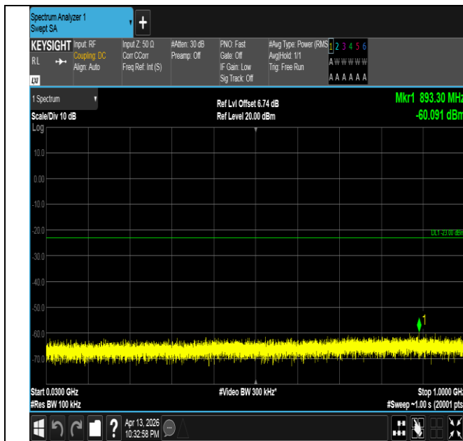
Band66-1.4MHz-QPSK-131979-6RB#0-30~1000-PASS
