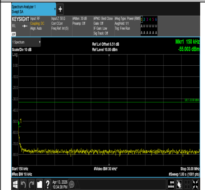
Band66-1.4MHz-QPSK-132322-1RB#0-0.15~30-PASS
