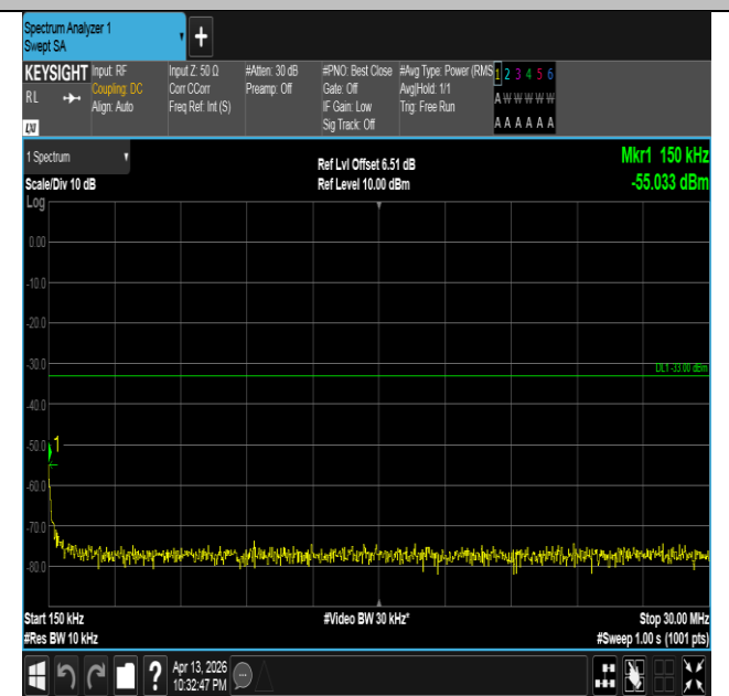
Band66-1.4MHz-QPSK-131979-6RB#0-0.15~30-PASS
