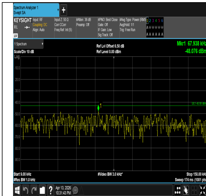
Band66-1.4MHz-16QAM-131979-1RB#5-0.009~0.15-PASS
