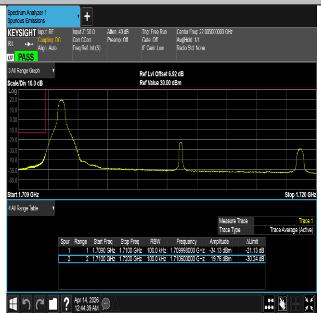
Band66-10MHz-16QAM-132022-1RB#0-PASS
