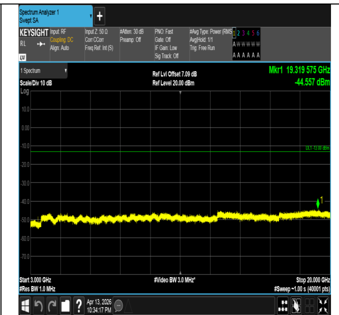
Band66-1.4MHz-16QAM-131979-6RB#0-3000~20000-PASS
