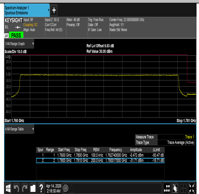
Band66-20MHz-16QAM-132572-100RB#0-PASS
