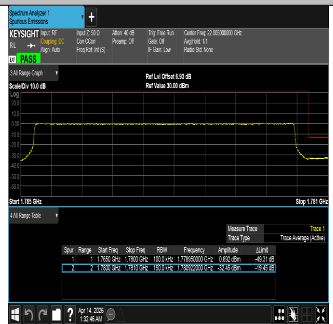
Band66-15MHz-16QAM-132597-75RB#0-PASS
