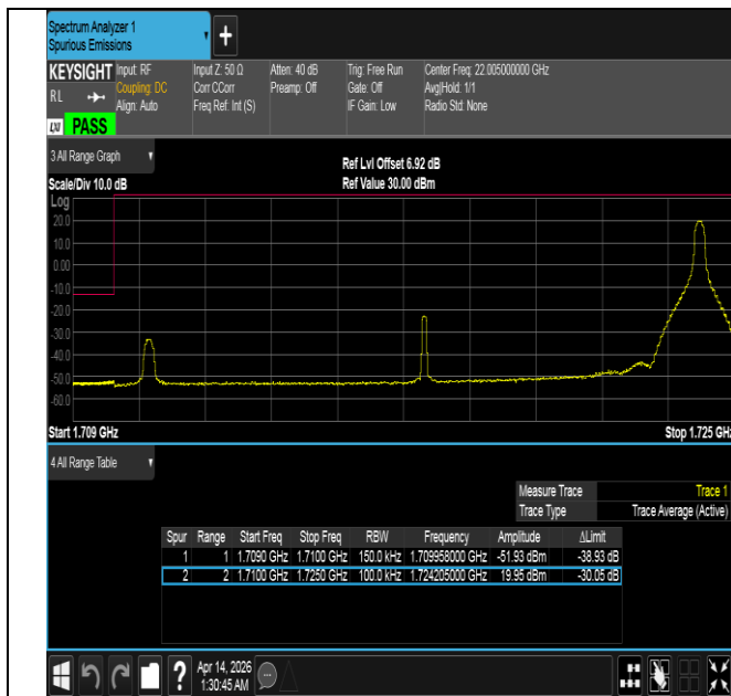
Band66-15MHz-16QAM-132047-1RB#74-PASS
