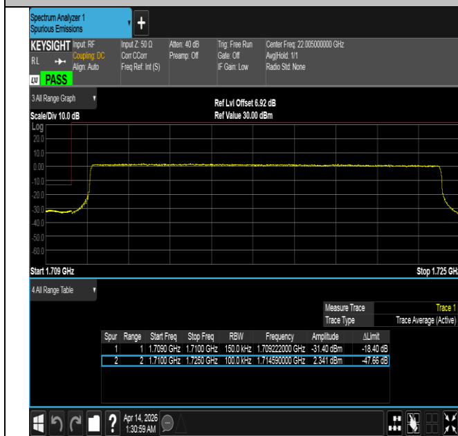
Band66-15MHz-QPSK-132047-75RB#0-PASS
