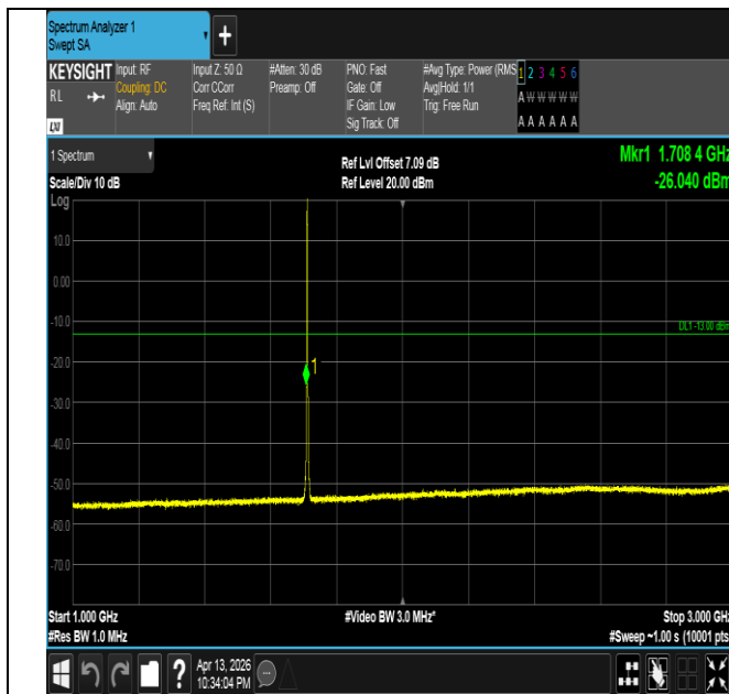
Band66-1.4MHz-16QAM-131979-6RB#0-1000~3000-PASS
