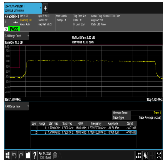
Band66-15MHz-16QAM-132047-75RB#0-PASS
