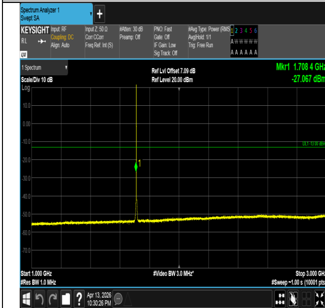
Band66-1.4MHz-16QAM-131979-1RB#0-1000~3000-PASS
