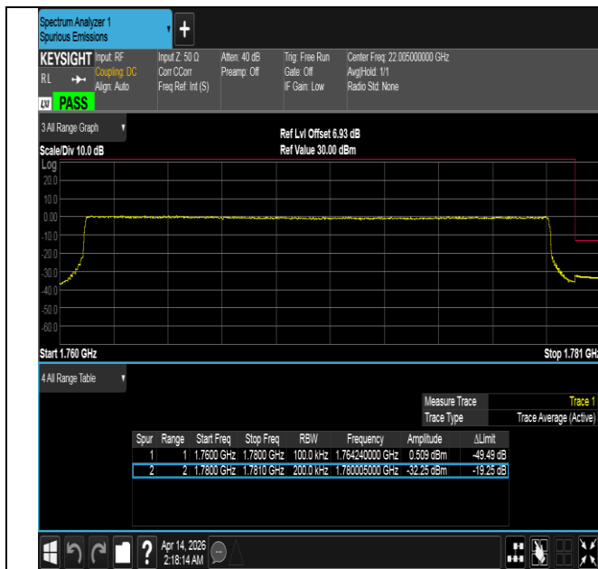
Band66-20MHz-QPSK-132572-100RB#0-PASS
