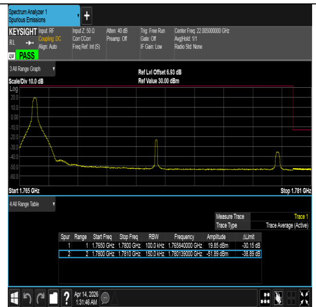
Band66-15MHz-16QAM-132597-1RB#0-PASS
