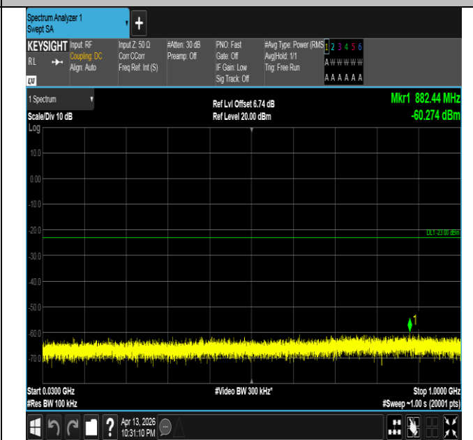
Band66-1.4MHz-QPSK-131979-1RB#5-30~1000-PASS
