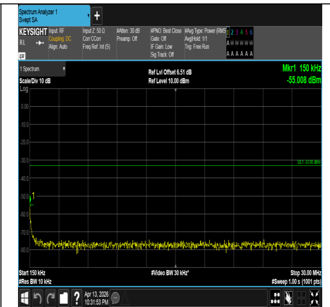
Band66-1.4MHz-16QAM-131979-1RB#5-0.15~30-PASS
