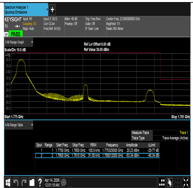
Band66-5MHz-16QAM-132647-1RB#0-PASS
