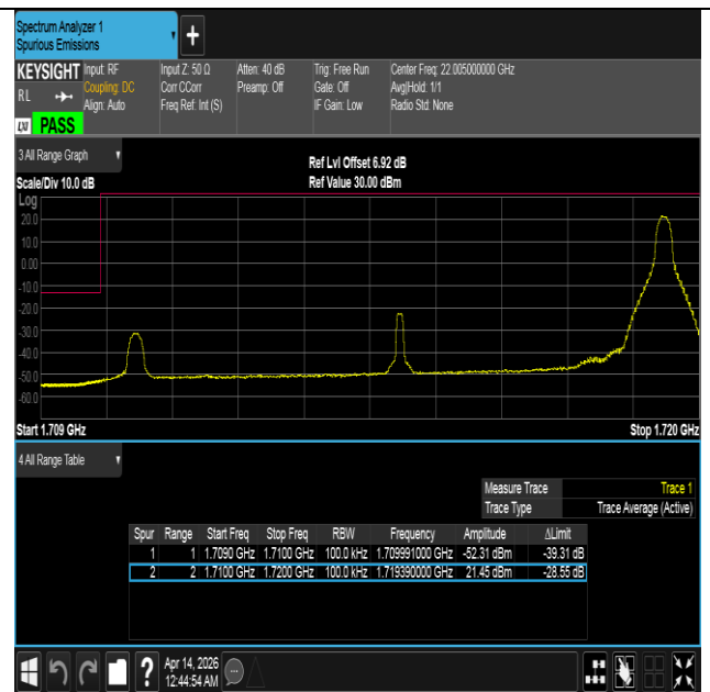
Band66-10MHz-QPSK-132022-1RB#49-PASS
