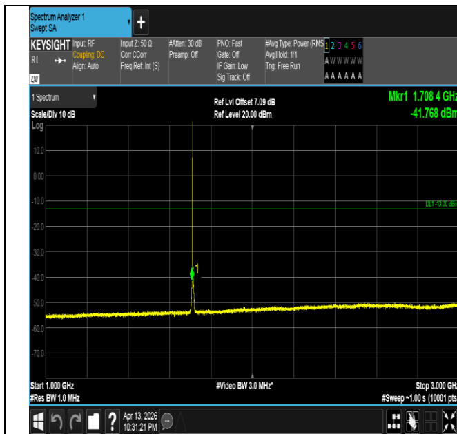
Band66-1.4MHz-QPSK-131979-1RB#5-1000~3000-PASS
