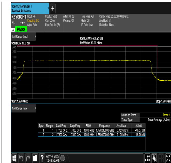
Band66-10MHz-QPSK-132622-50RB#0-PASS
