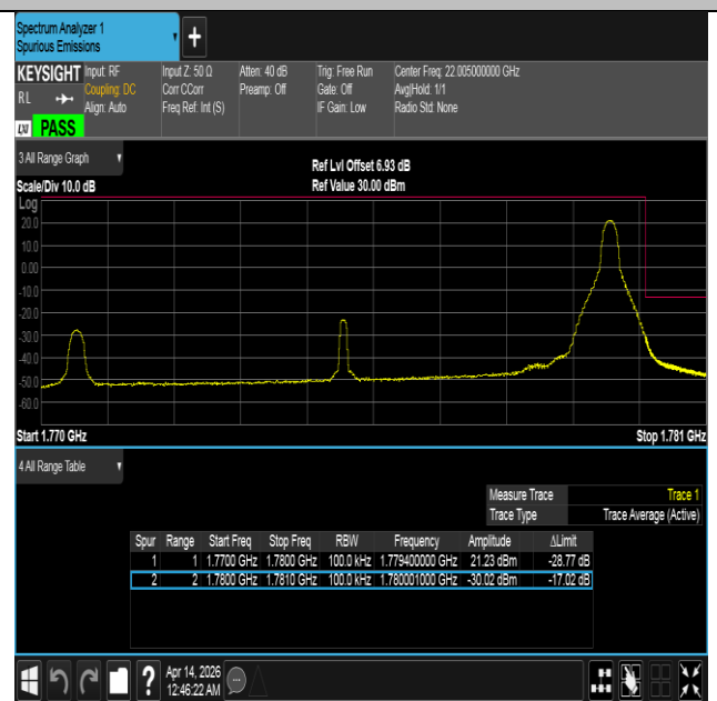
Band66-10MHz-QPSK-132622-1RB#49-PASS
