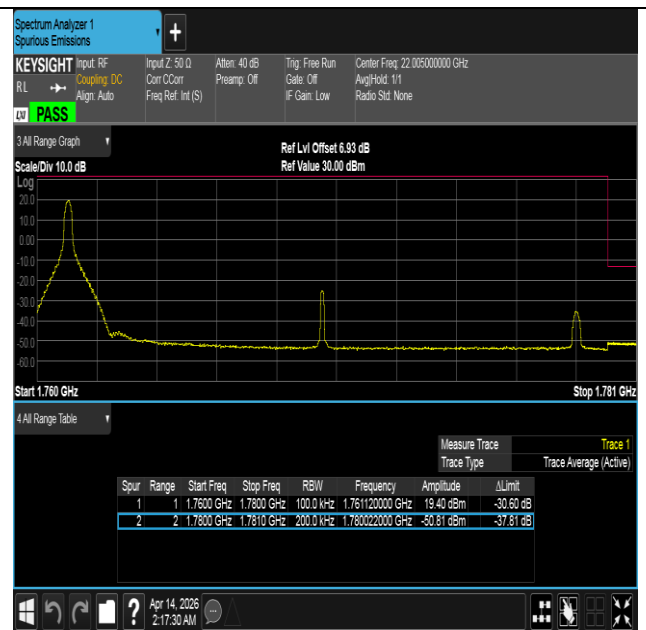
Band66-20MHz-16QAM-132572-1RB#0-PASS
