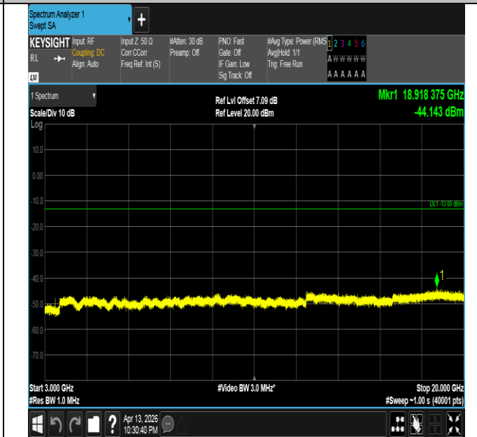
Band66-1.4MHz-16QAM-131979-1RB#0-3000~20000-PASS
