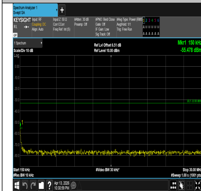
Band66-1.4MHz-QPSK-131979-1RB#5-0.15~30-PASS
