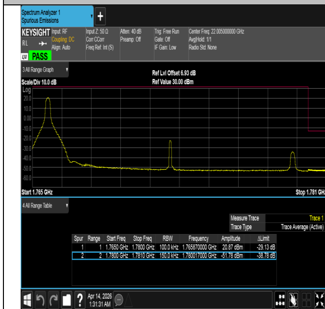
Band66-15MHz-QPSK-132597-1RB#0-PASS
