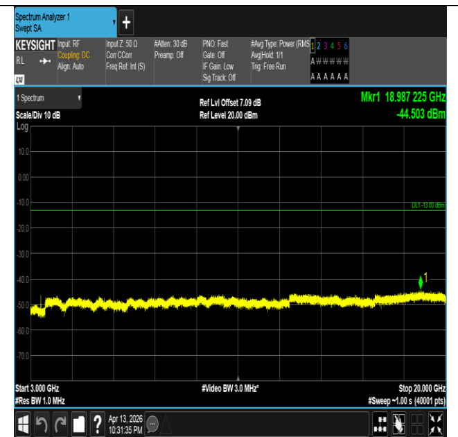
Band66-1.4MHz-QPSK-131979-1RB#5-3000~20000-PASS
