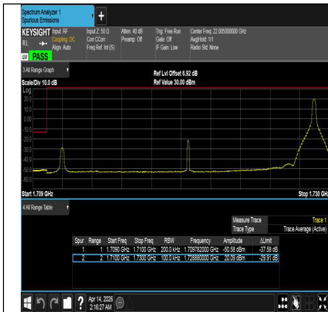
Band66-20MHz-16QAM-132072-1RB#99-PASS
