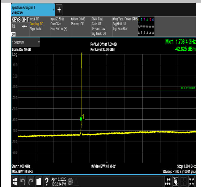
Band66-1.4MHz-16QAM-131979-1RB#5-1000~3000-PASS
