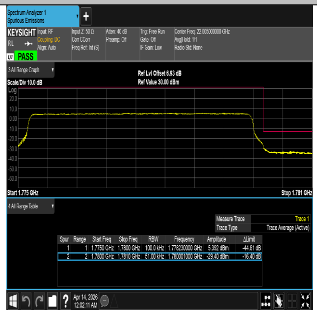
Band66-5MHz-16QAM-132647-25RB#0-PASS
