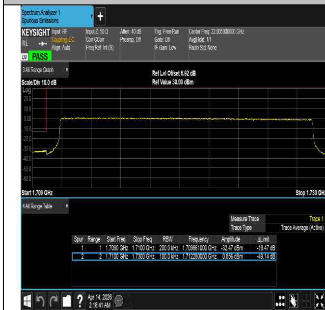
Band66-20MHz-QPSK-132072-100RB#0-PASS
