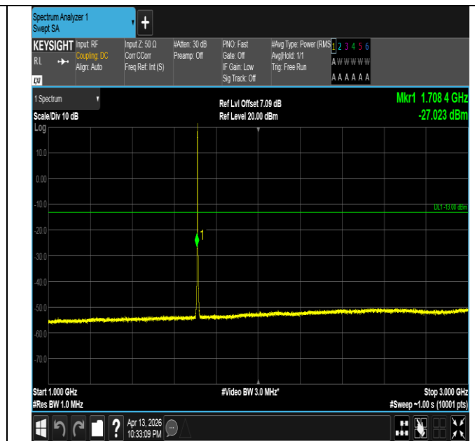
Band66-1.4MHz-QPSK-131979-6RB#0-1000~3000-PASS
