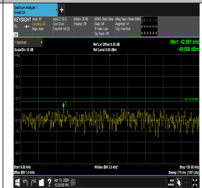
Band66-1.4MHz-16QAM-131979-1RB#0-0.009~0.15-PASS
