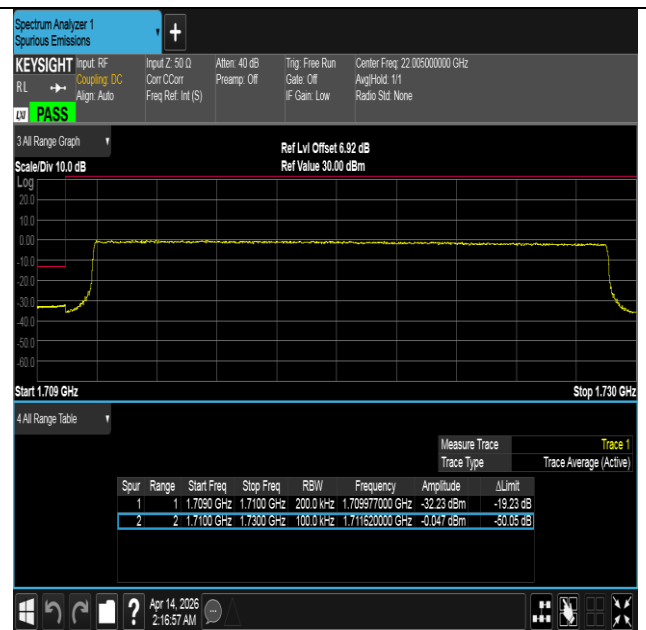
Band66-20MHz-16QAM-132072-100RB#0-PASS
