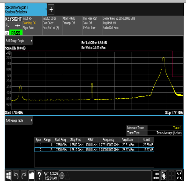
Band66-15MHz-QPSK-132597-1RB#74-PASS
