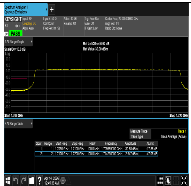
Band66-10MHz-16QAM-132022-50RB#0-PASS
