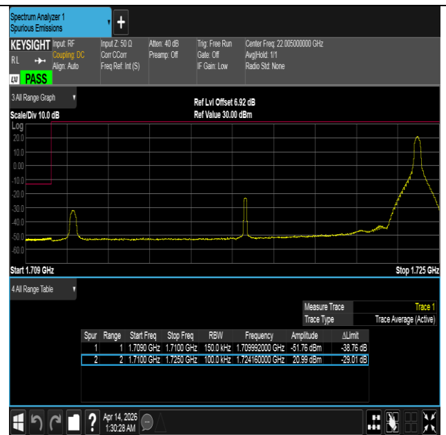
Band66-15MHz-QPSK-132047-1RB#74-PASS
