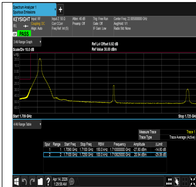
Band66-15MHz-QPSK-132047-1RB#0-PASS
