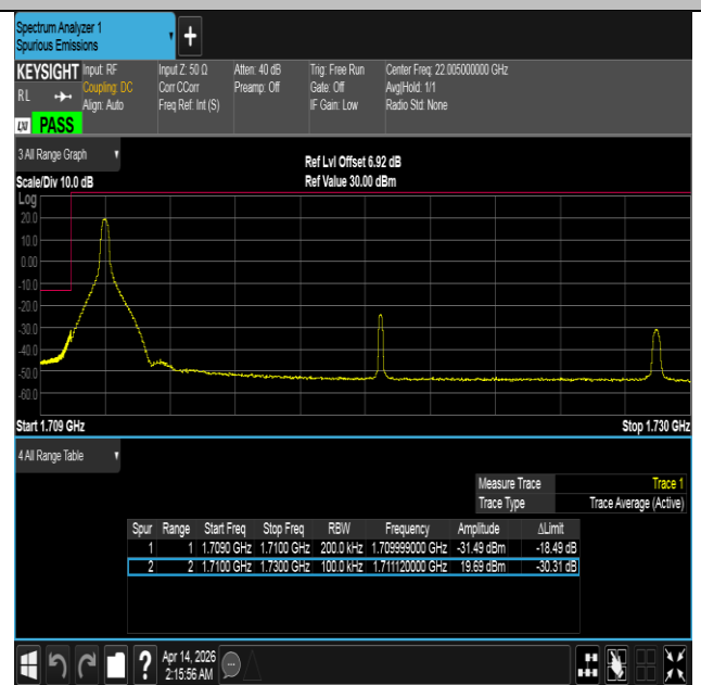
Band66-20MHz-16QAM-132072-1RB#0-PASS
