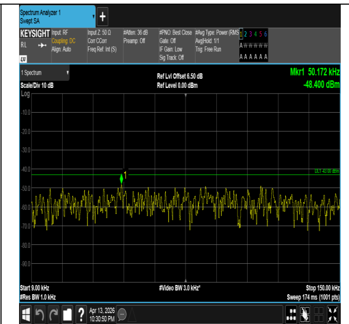
Band66-1.4MHz-QPSK-131979-1RB#5-0.009~0.15-PASS
