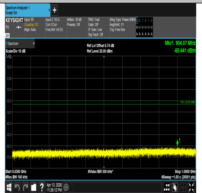
Band66-3MHz-16QAM-132322-15RB#0-30~1000-PASS
