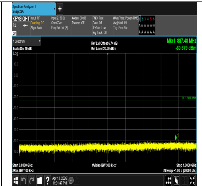
Band66-3MHz-16QAM-132657-15RB#0-30~1000-PASS
