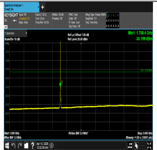
Band66-5MHz-QPSK-131997-1RB#0-1000~3000-PASS
