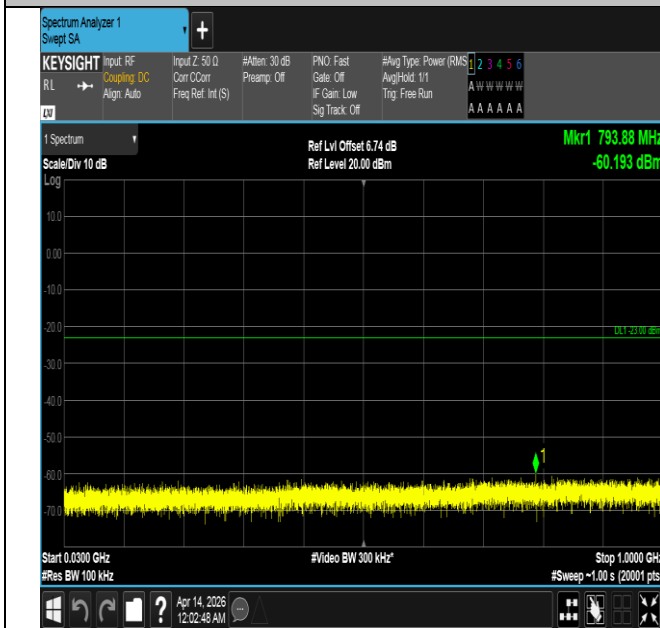
Band66-5MHz-QPSK-131997-1RB#0-30~1000-PASS
