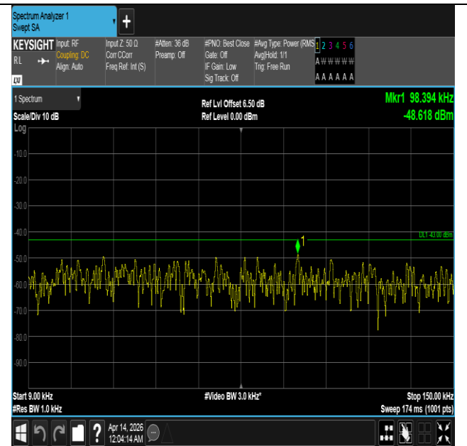
Band66-5MHz-QPSK-131997-1RB#24-0.009~0.15-PASS
