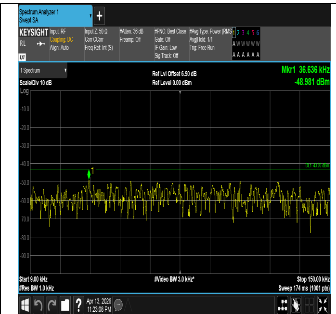
Band66-3MHz-QPSK-132322-1RB#14-0.009~0.15-PASS
