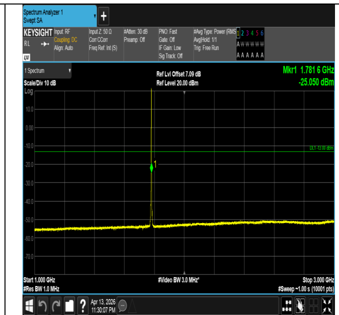
Band66-3MHz-16QAM-132657-1RB#14-1000~3000-PASS
