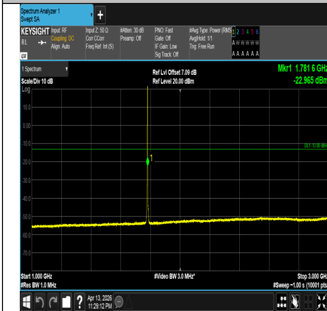
Band66-3MHz-QPSK-132657-1RB#14-1000~3000-PASS
