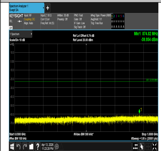
Band66-3MHz-QPSK-132322-1RB#14-30~1000-PASS
