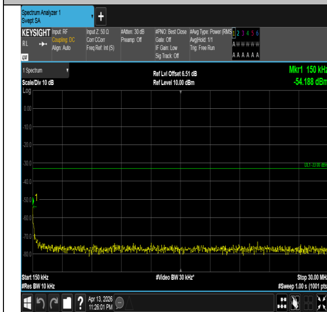
Band66-3MHz-16QAM-132322-15RB#0-0.15~30-PASS
