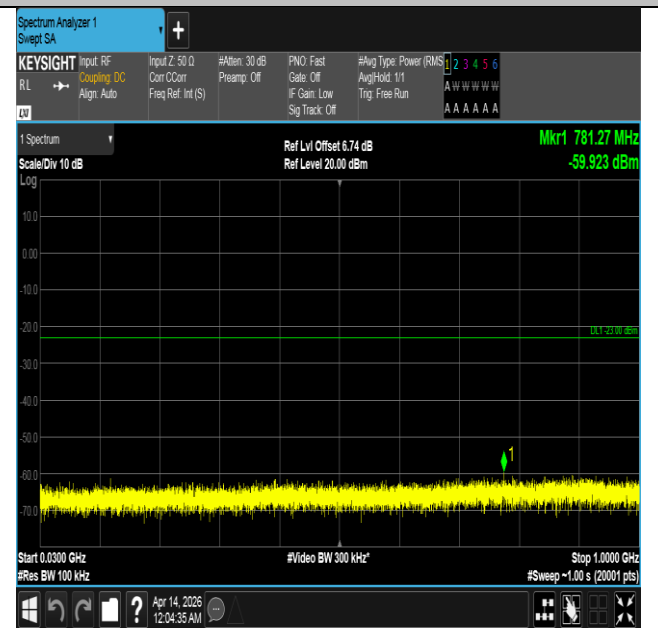
Band66-5MHz-QPSK-131997-1RB#24-30~1000-PASS
