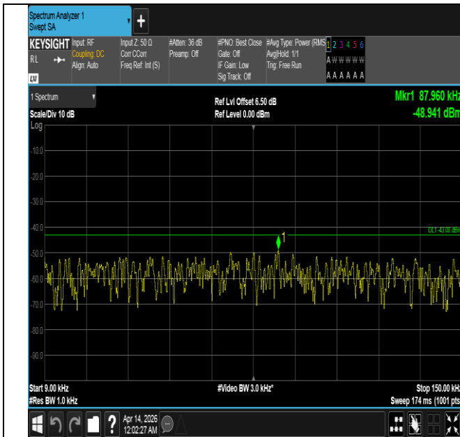
Band66-5MHz-QPSK-131997-1RB#0-0.009~0.15-PASS
