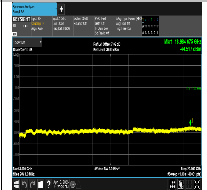
Band66-3MHz-QPSK-132657-1RB#14-3000~20000-PASS
