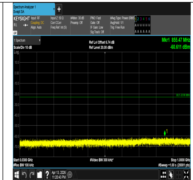
Band66-3MHz-16QAM-131987-15RB#0-30~1000-PASS
