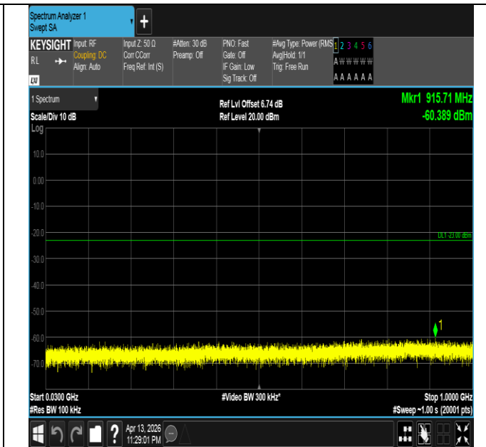
Band66-3MHz-QPSK-132657-1RB#14-30~1000-PASS
