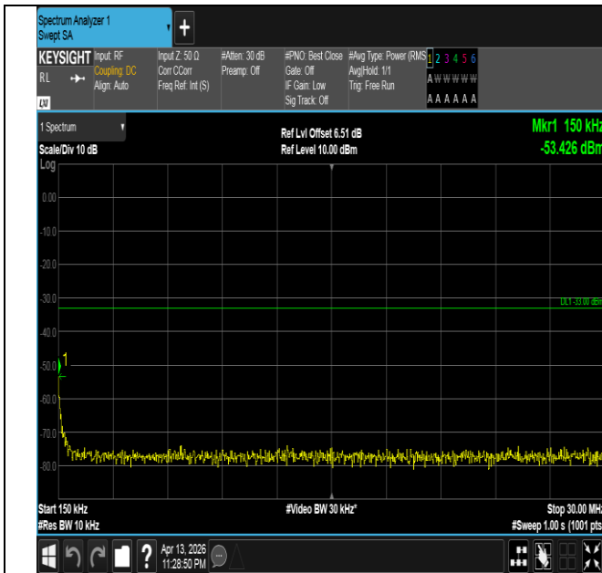
Band66-3MHz-QPSK-132657-1RB#14-0.15~30-PASS
