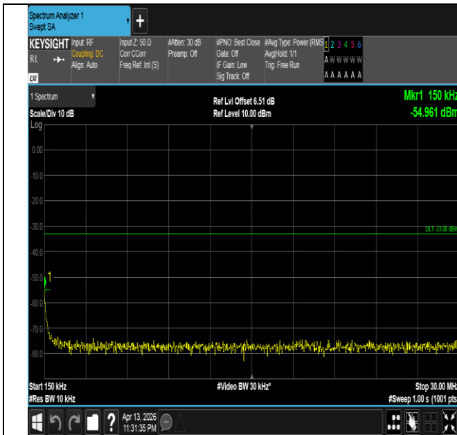
Band66-3MHz-16QAM-132657-15RB#0-0.15~30-PASS
