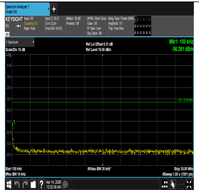
Band66-5MHz-QPSK-131997-1RB#0-0.15~30-PASS
