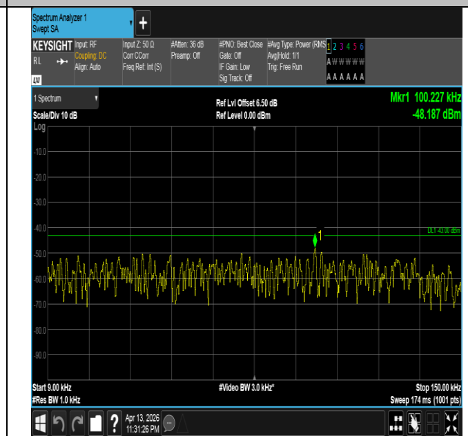
Band66-3MHz-16QAM-132657-15RB#0-0.009~0.15-PASS
