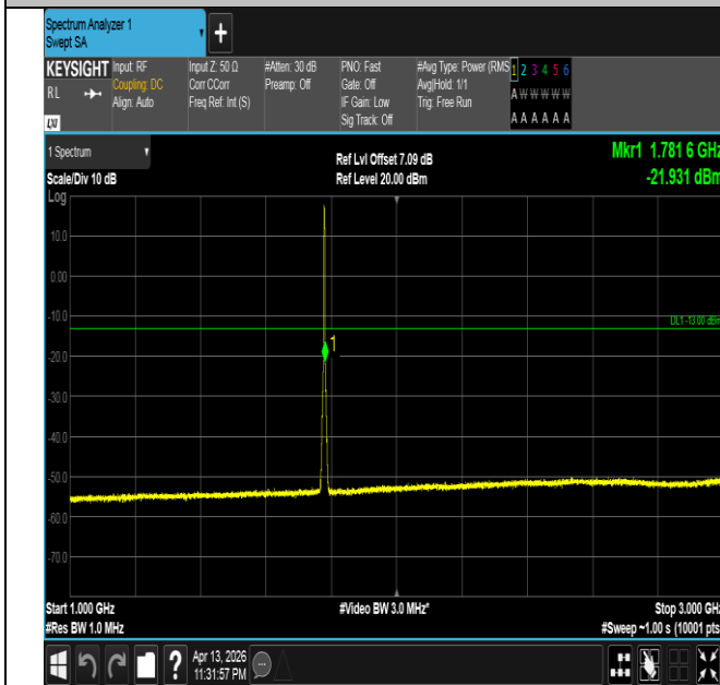
Band66-3MHz-16QAM-132657-15RB#0-1000~3000-PASS
