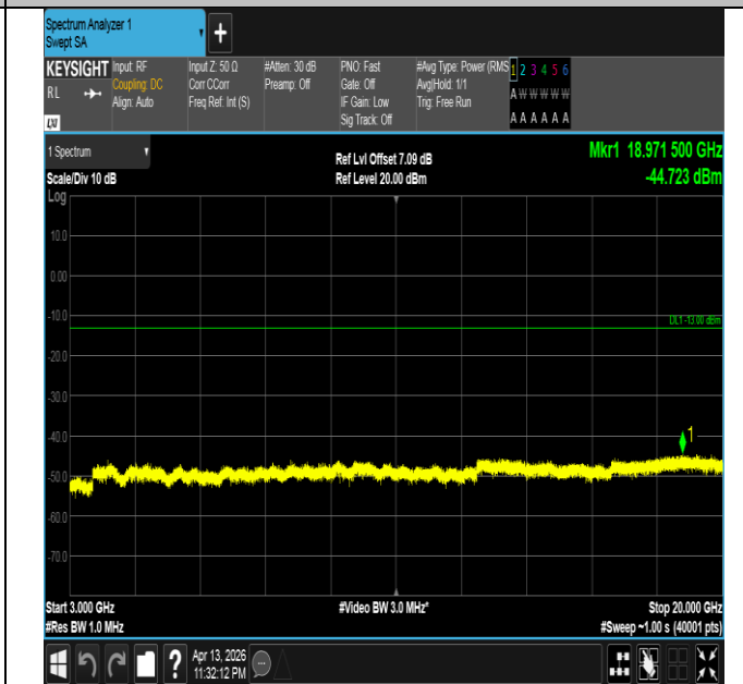
Band66-3MHz-16QAM-132657-15RB#0-3000~20000-PASS
