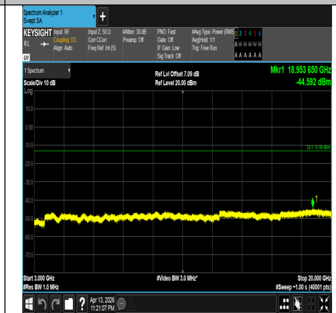
Band66-3MHz-16QAM-131987-15RB#0-3000~20000-PASS
