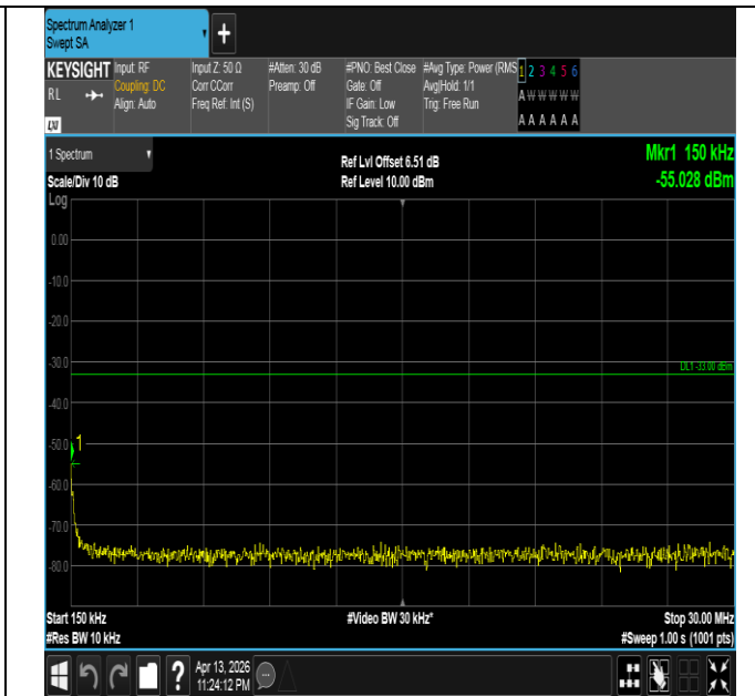
Band66-3MHz-16QAM-132322-1RB#14-0.15~30-PASS
