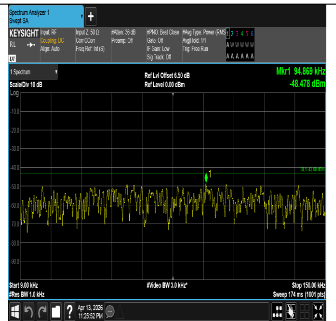
Band66-3MHz-16QAM-132322-15RB#0-0.009~0.15-PASS
