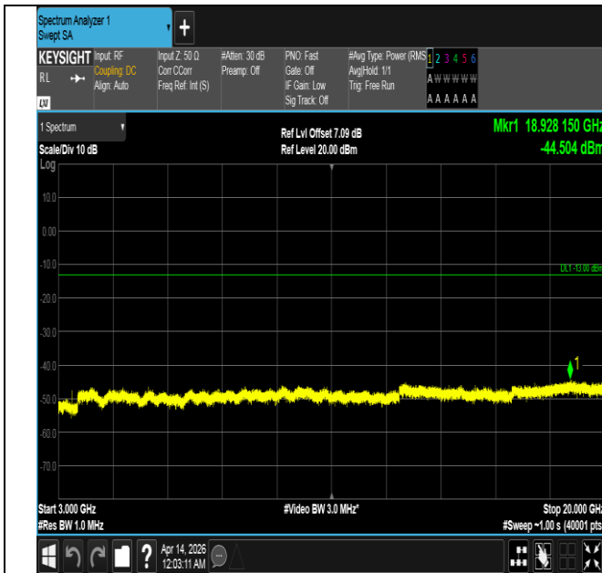
Band66-5MHz-QPSK-131997-1RB#0-3000~20000-PASS
