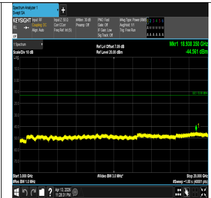
Band66-3MHz-16QAM-132657-1RB#0-3000~20000-PASS
