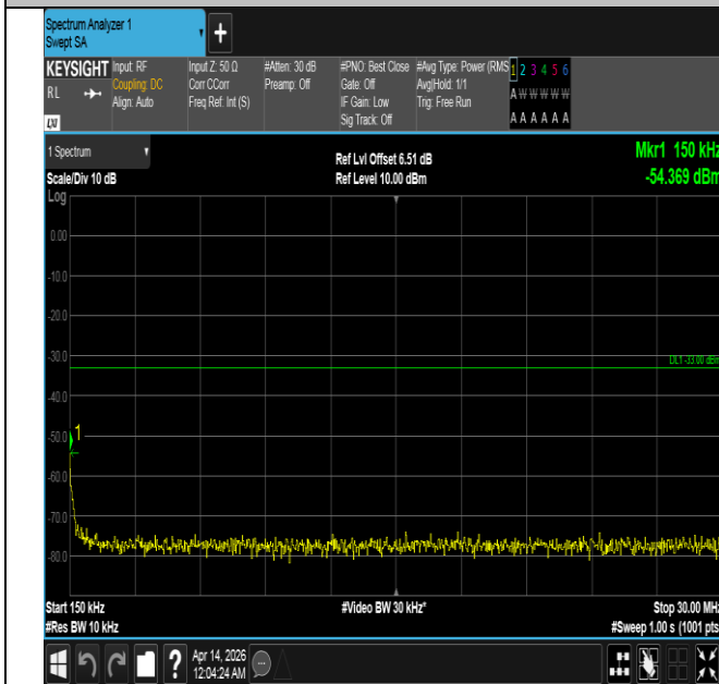
Band66-5MHz-QPSK-131997-1RB#24-0.15~30-PASS
