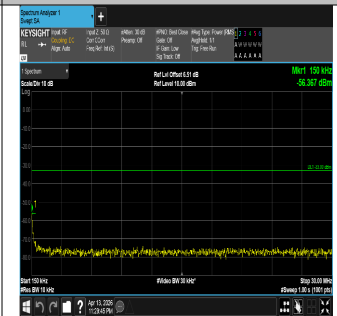
Band66-3MHz-16QAM-132657-1RB#14-0.15~30-PASS
