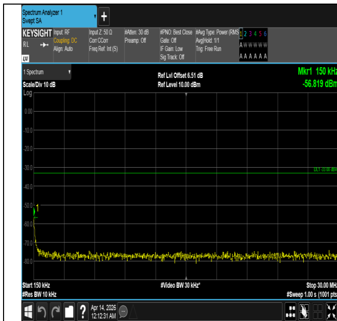
Band66-5MHz-16QAM-132322-25RB#0-0.15~30-PASS
