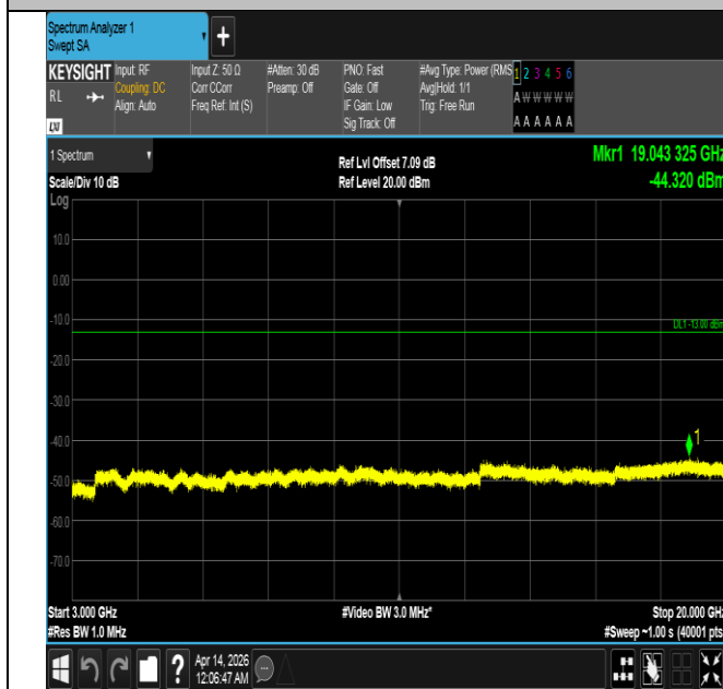
Band66-5MHz-QPSK-131997-25RB#0-3000~20000-PASS
