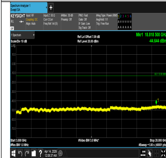
Band66-5MHz-QPSK-132322-1RB#0-3000~20000-PASS
