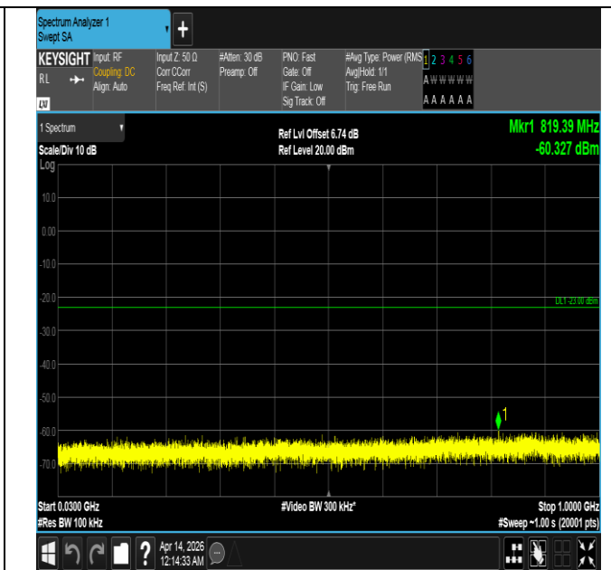
Band66-5MHz-16QAM-132647-1RB#0-30~1000-PASS
