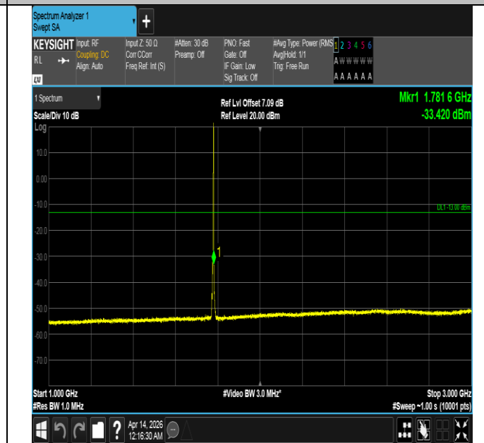
Band66-5MHz-16QAM-132647-1RB#24-1000~3000-PASS
