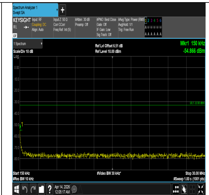
Band66-5MHz-16QAM-131997-1RB#24-0.15~30-PASS
