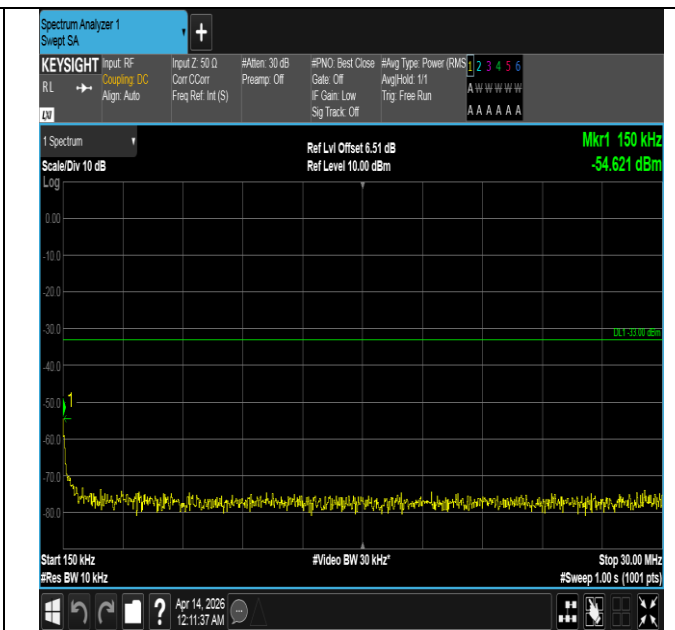
Band66-5MHz-QPSK-132322-25RB#0-0.15~30-PASS
