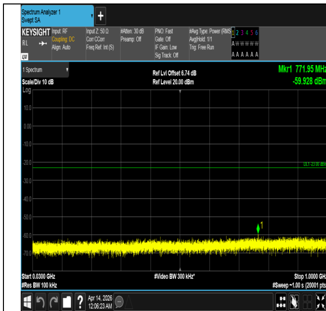
Band66-5MHz-QPSK-131997-25RB#0-30~1000-PASS
