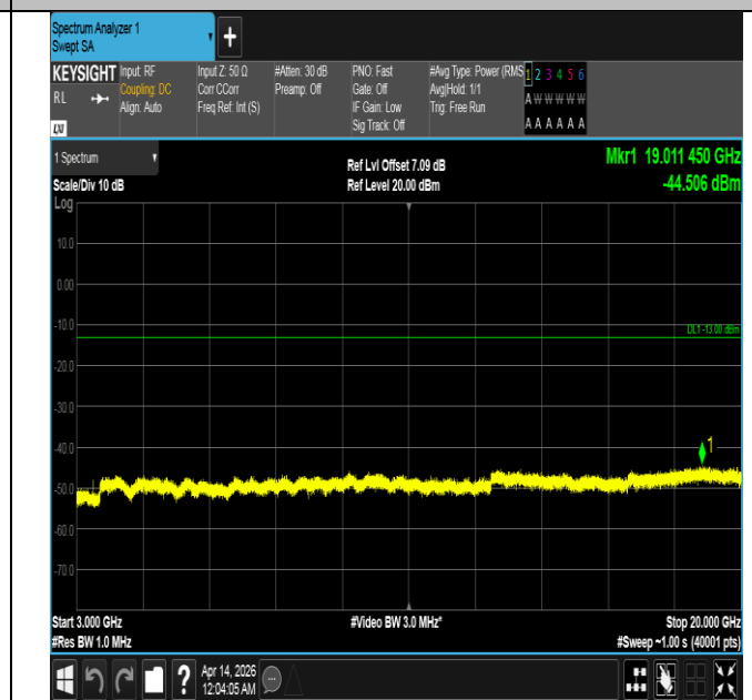
Band66-5MHz-16QAM-131997-1RB#0-3000~20000-PASS
