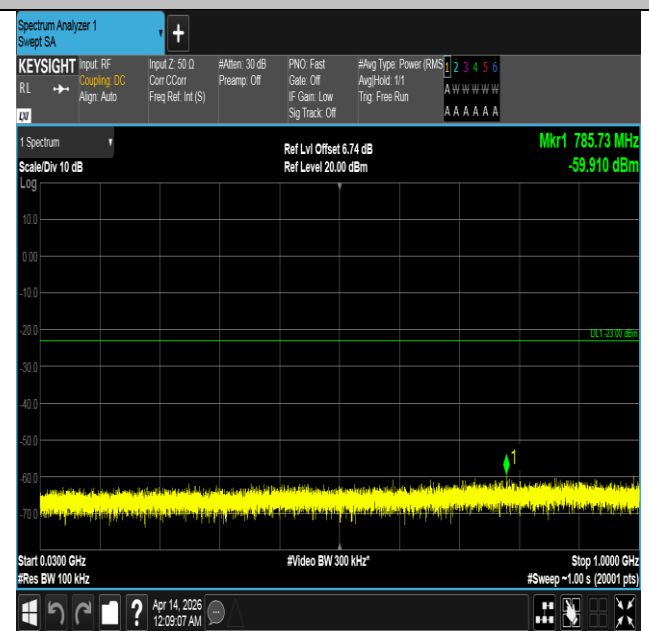
Band66-5MHz-16QAM-132322-1RB#0-30~1000-PASS
