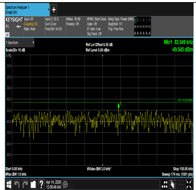
Band66-5MHz-16QAM-132322-1RB#0-0.009~0.15-PASS
