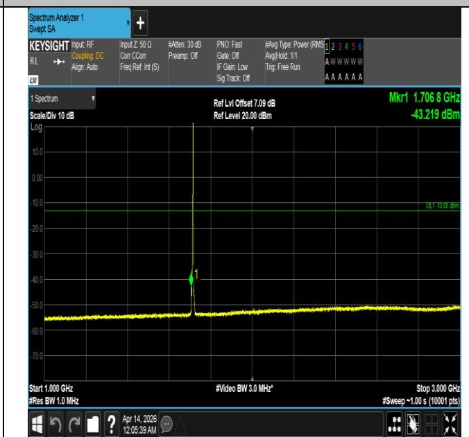
Band66-5MHz-16QAM-131997-1RB#24-1000~3000-PASS
