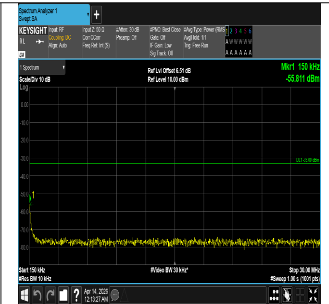
Band66-5MHz-QPSK-132647-1RB#0-0.15~30-PASS
