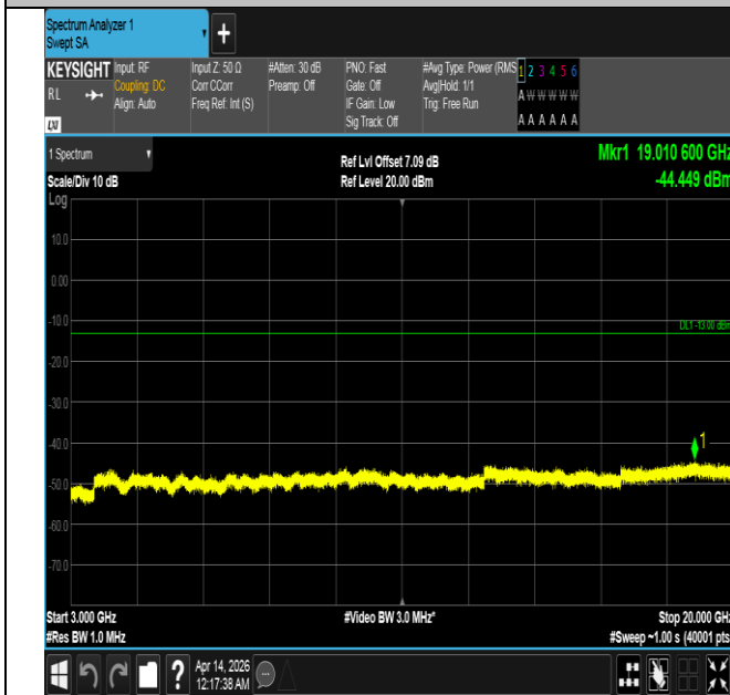
Band66-5MHz-QPSK-132647-25RB#0-3000~20000-PASS
