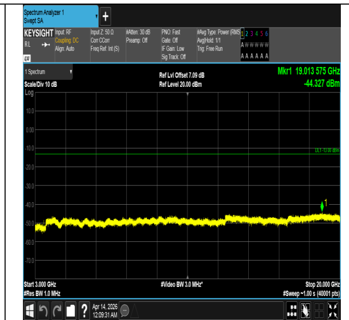
Band66-5MHz-16QAM-132322-1RB#0-3000~20000-PASS
