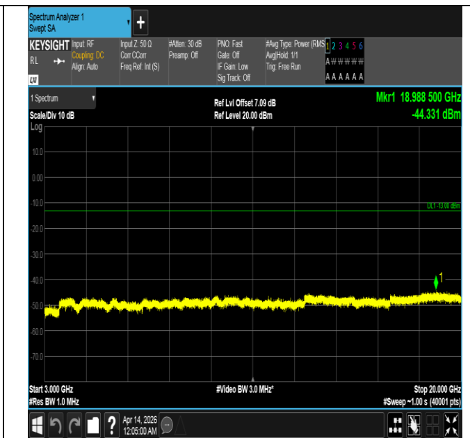
Band66-5MHz-QPSK-131997-1RB#24-3000~20000-PASS
