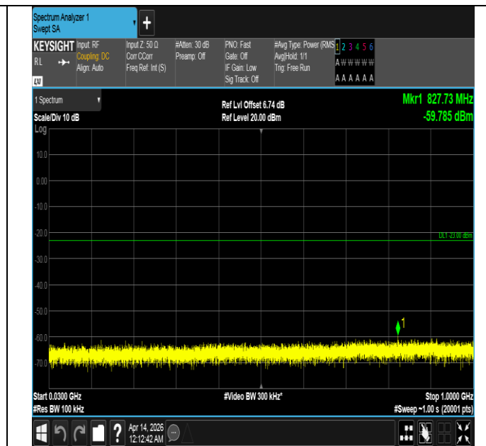
Band66-5MHz-16QAM-132322-25RB#0-30~1000-PASS
