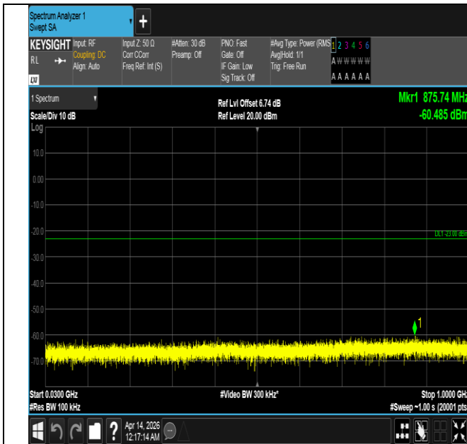
Band66-5MHz-QPSK-132647-25RB#0-30~1000-PASS
