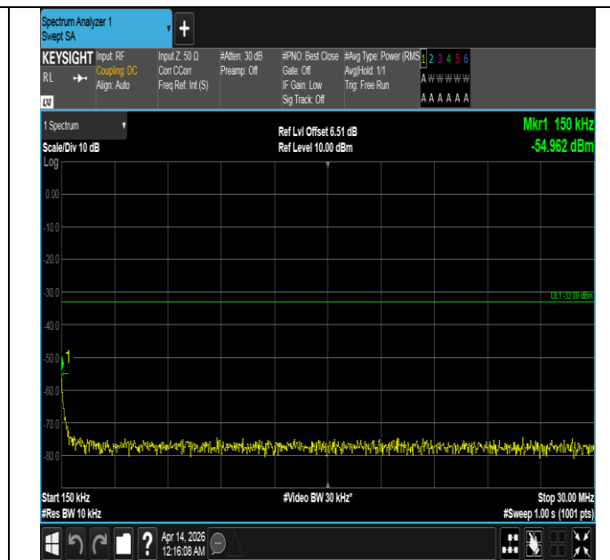
Band66-5MHz-16QAM-132647-1RB#24-0.15~30-PASS
