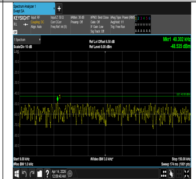
Band66-5MHz-QPSK-132322-1RB#24-0.009~0.15-PASS
