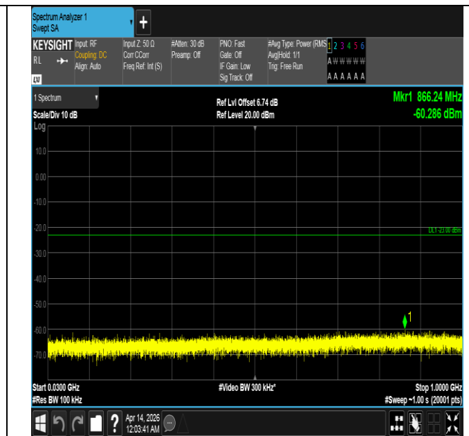
Band66-5MHz-16QAM-131997-1RB#0-30~1000-PASS
