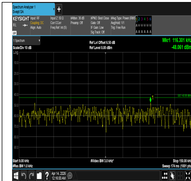
Band66-5MHz-16QAM-132647-1RB#24-0.009~0.15-PASS
