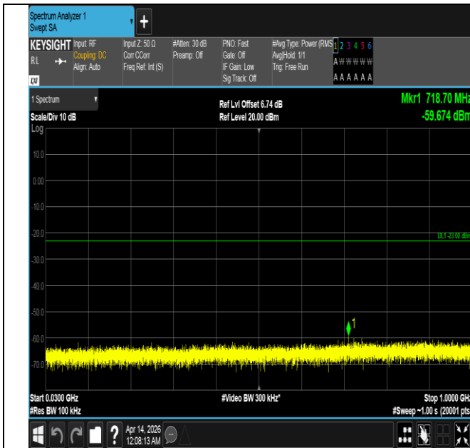
Band66-5MHz-QPSK-132322-1RB#0-30~1000-PASS
