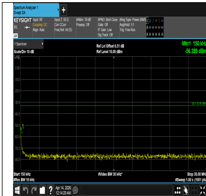
Band66-5MHz-16QAM-132647-1RB#0-0.15~30-PASS
