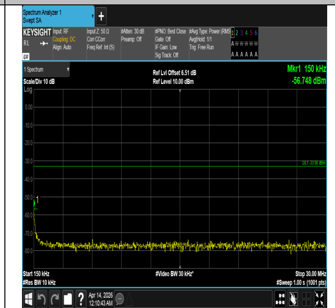
Band66-5MHz-16QAM-132322-1RB#24-0.15~30-PASS
