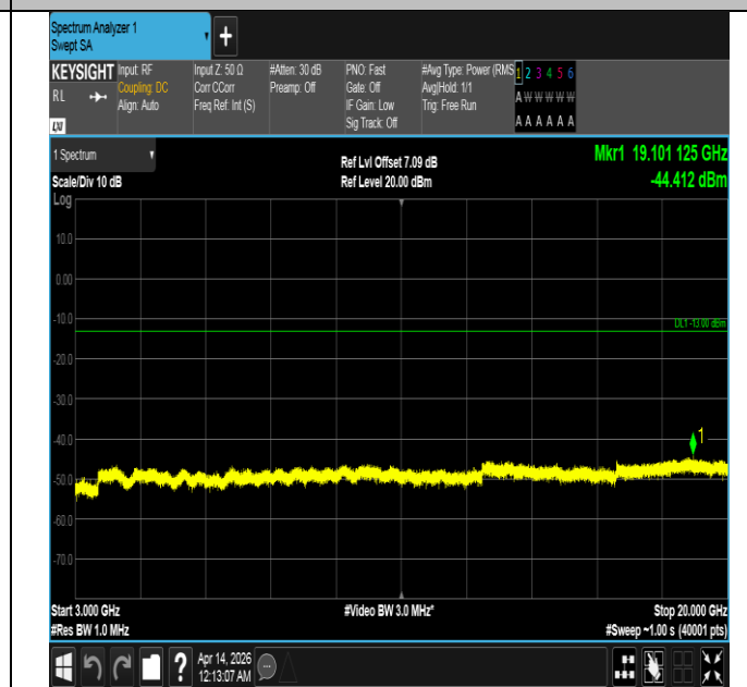
Band66-5MHz-16QAM-132322-25RB#0-3000~20000-PASS
