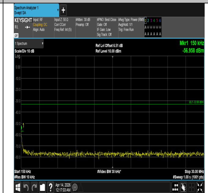
Band66-5MHz-QPSK-132647-25RB#0-0.15~30-PASS
