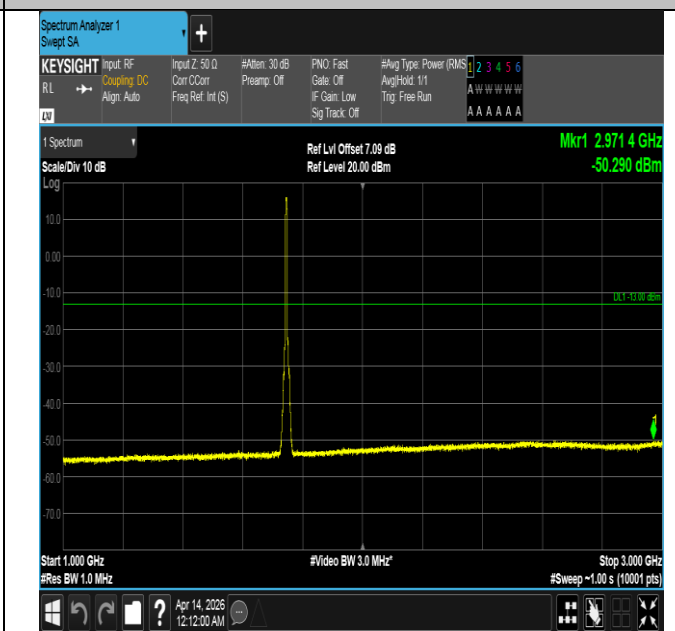
Band66-5MHz-QPSK-132322-25RB#0-1000~3000-PASS
