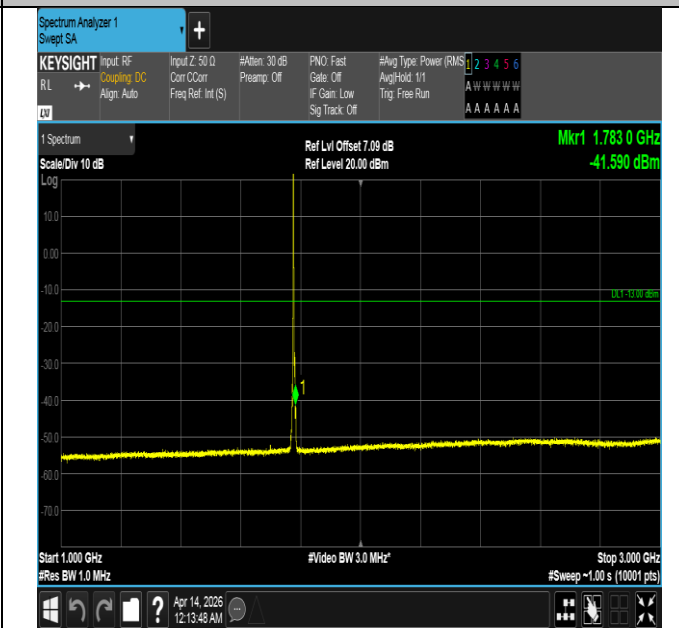
Band66-5MHz-QPSK-132647-1RB#0-1000~3000-PASS
