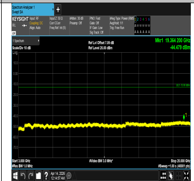
Band66-5MHz-16QAM-132647-1RB#0-3000~20000-PASS
