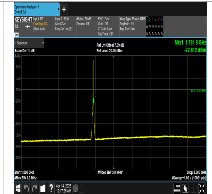
Band66-5MHz-QPSK-132647-25RB#0-1000~3000-PASS
