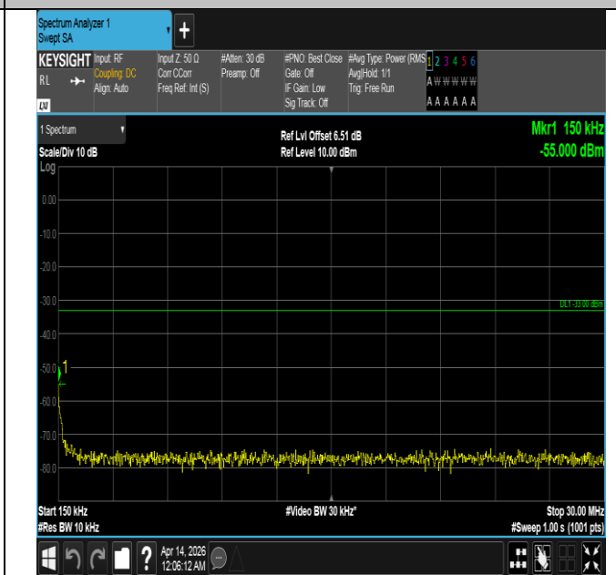
Band66-5MHz-QPSK-131997-25RB#0-0.15~30-PASS
