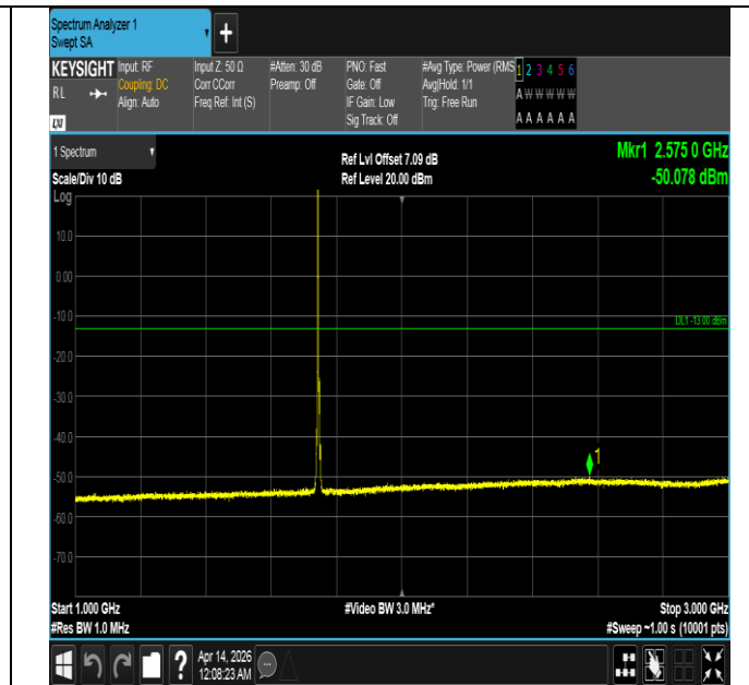
Band66-5MHz-QPSK-132322-1RB#0-1000~3000-PASS
