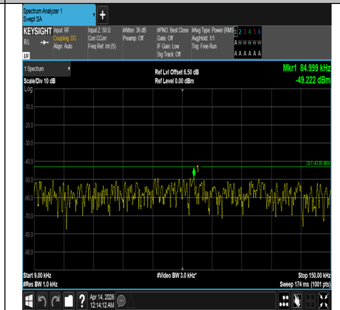
Band66-5MHz-16QAM-132647-1RB#0-0.009~0.15-PASS
