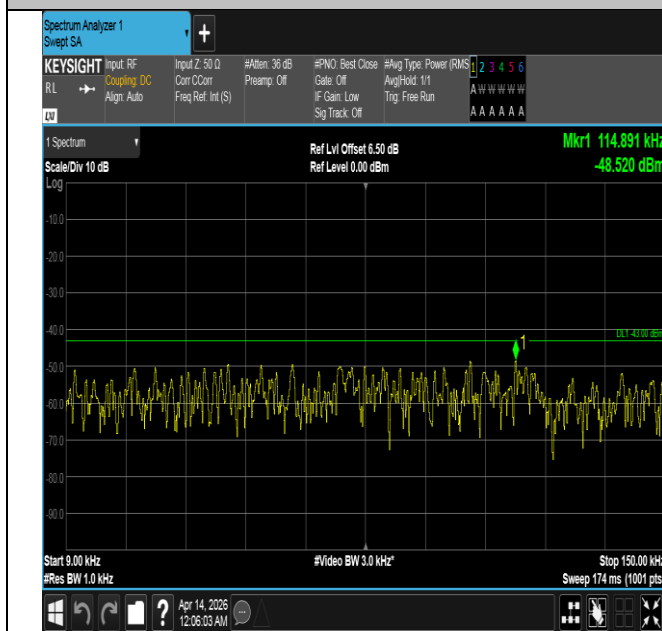
Band66-5MHz-QPSK-131997-25RB#0-0.009~0.15-PASS
