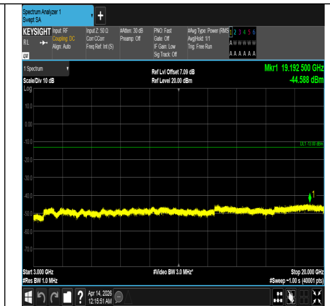
Band66-5MHz-QPSK-132647-1RB#24-3000~20000-PASS
