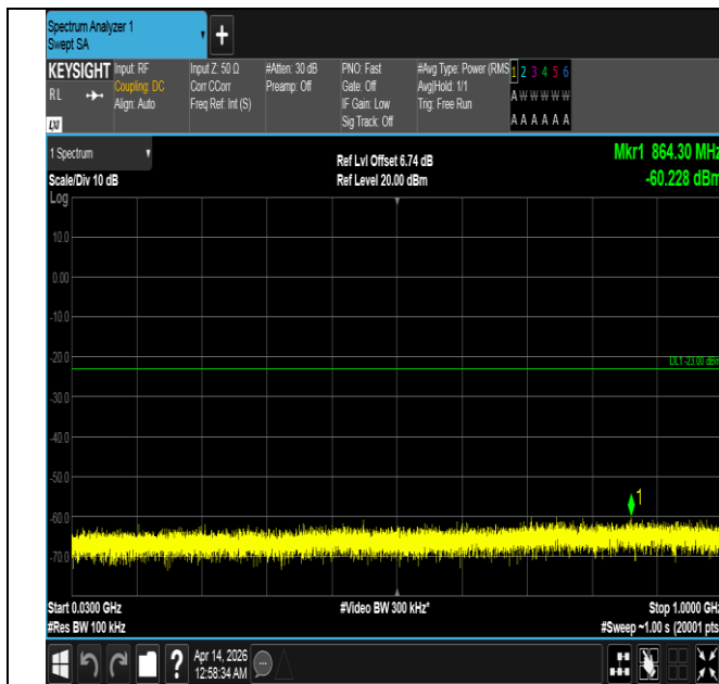
Band66-10MHz-QPSK-132622-1RB#0-30~1000-PASS
