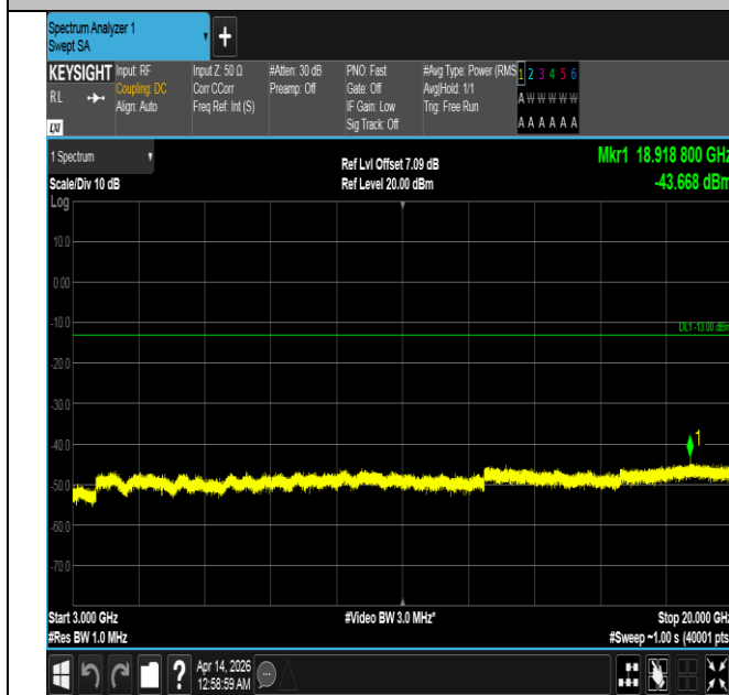
Band66-10MHz-QPSK-132622-1RB#0-3000~20000-PASS
