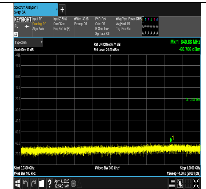
Band66-10MHz-16QAM-132322-1RB#0-30~1000-PASS
