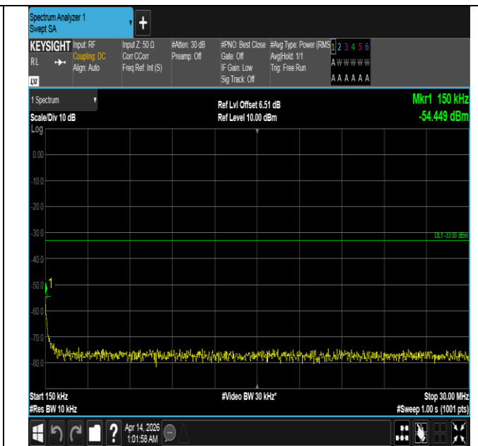
Band66-10MHz-QPSK-132622-50RB#0-0.15~30-PASS
