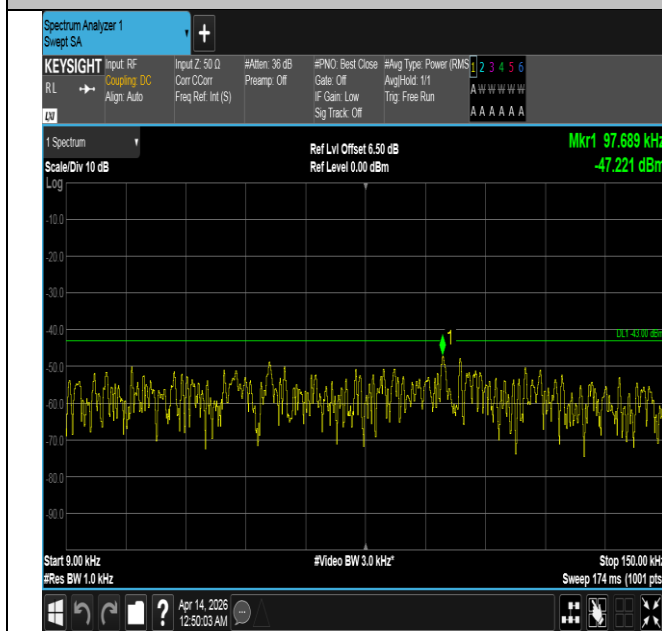
Band66-10MHz-16QAM-132022-1RB#49-0.009~0.15-PASS
