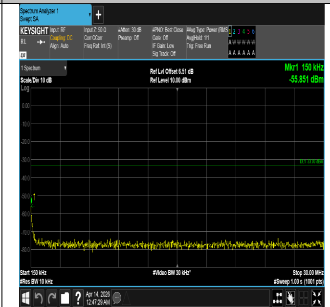
Band66-10MHz-QPSK-132022-1RB#0-0.15~30-PASS
