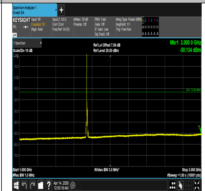
Band66-10MHz-QPSK-132322-1RB#0-1000~3000-PASS
