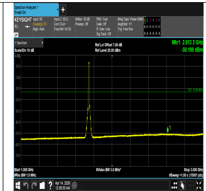
Band66-10MHz-QPSK-132322-50RB#0-1000~3000-PASS
