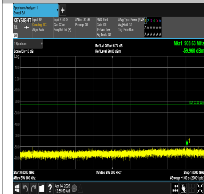
Band66-10MHz-16QAM-132322-1RB#49-30~1000-PASS
