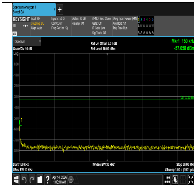
Band66-10MHz-QPSK-132622-1RB#49-0.15~30-PASS
