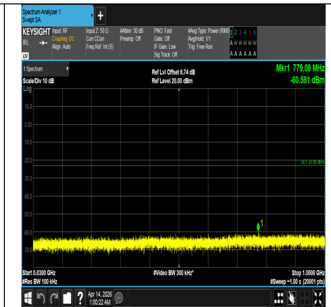
Band66-10MHz-QPSK-132622-1RB#49-30~1000-PASS
