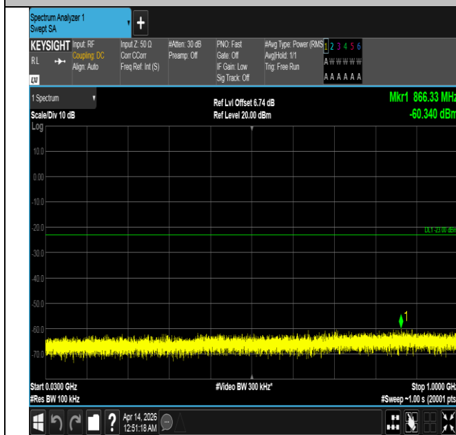
Band66-10MHz-QPSK-132022-50RB#0-30~1000-PASS
