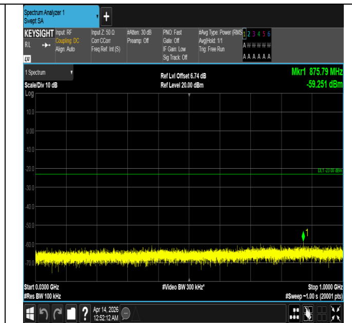
Band66-10MHz-16QAM-132022-50RB#0-30~1000-PASS
