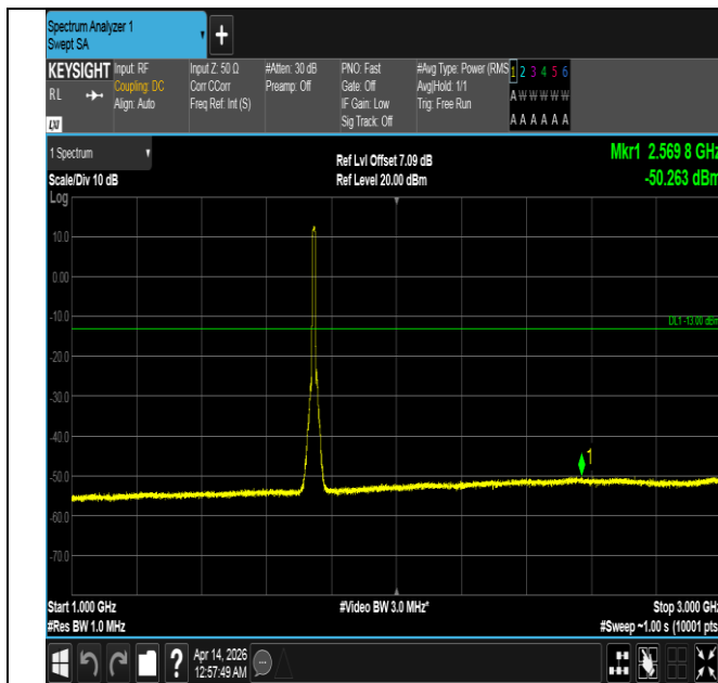
Band66-10MHz-16QAM-132322-50RB#0-1000~3000-PASS
