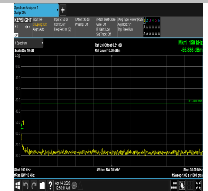
Band66-10MHz-16QAM-132022-1RB#49-0.15~30-PASS
