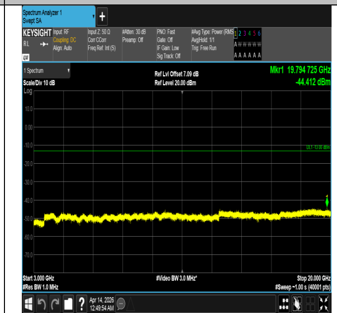
Band66-10MHz-QPSK-132022-1RB#49-3000~20000-PASS
