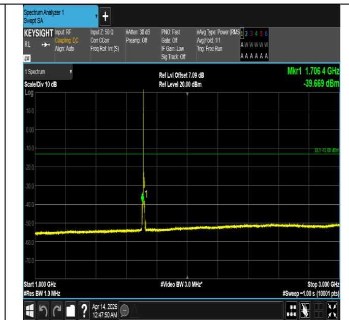
Band66-10MHz-QPSK-132022-1RB#0-1000~3000-PASS
