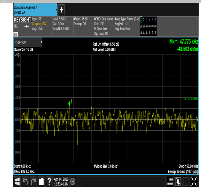
Band66-10MHz-16QAM-132322-1RB#0-0.009~0.15-PASS
