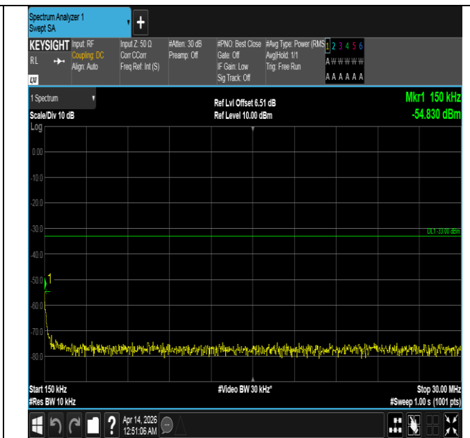
Band66-10MHz-QPSK-132022-50RB#0-0.15~30-PASS
