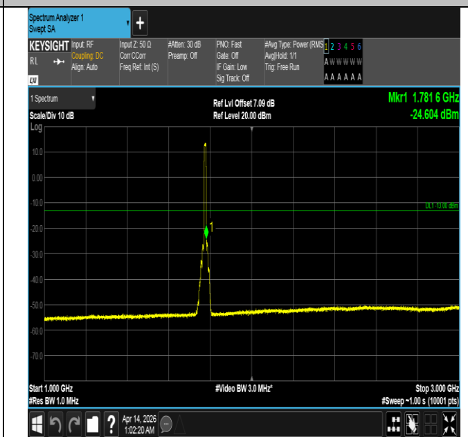
Band66-10MHz-QPSK-132622-50RB#0-1000~3000-PASS
