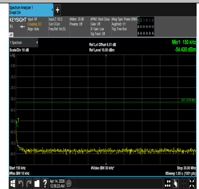
Band66-10MHz-QPSK-132622-1RB#0-0.15~30-PASS
