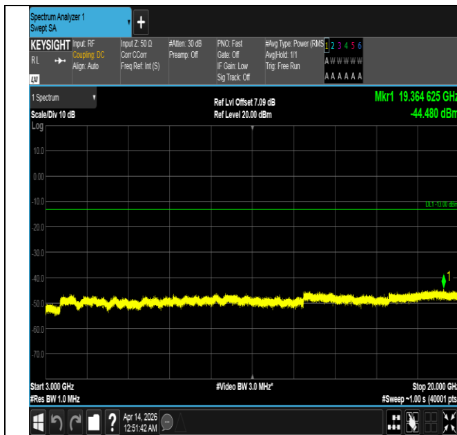
Band66-10MHz-QPSK-132022-50RB#0-3000~20000-PASS
