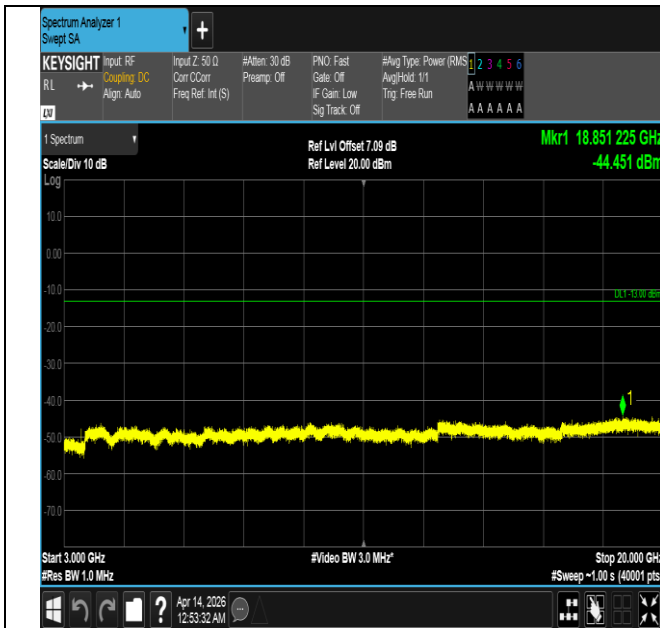
Band66-10MHz-QPSK-132322-1RB#0-3000~20000-PASS
