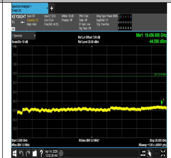
Band66-10MHz-16QAM-132022-50RB#0-3000~20000-PASS
