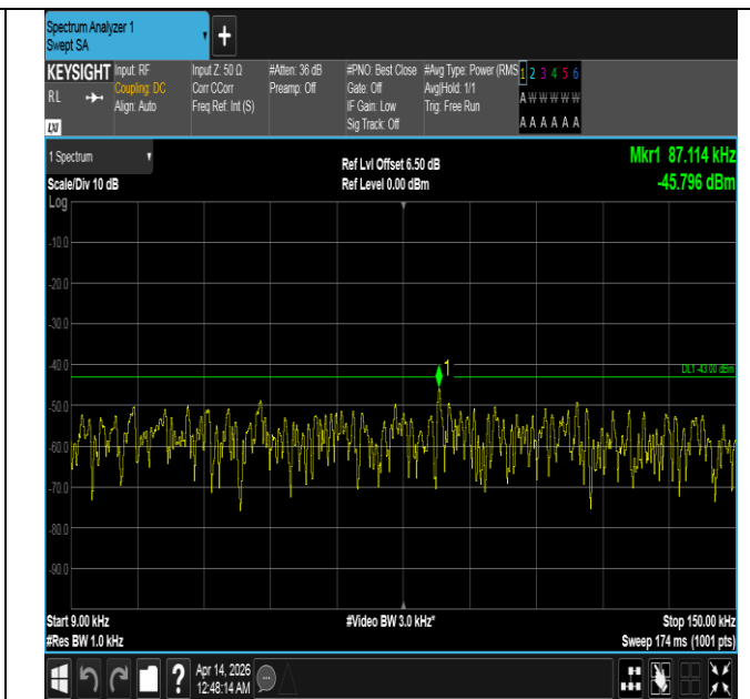
Band66-10MHz-16QAM-132022-1RB#0-0.009~0.15-PASS
