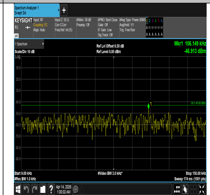
Band66-10MHz-QPSK-132622-1RB#49-0.009~0.15-PASS
