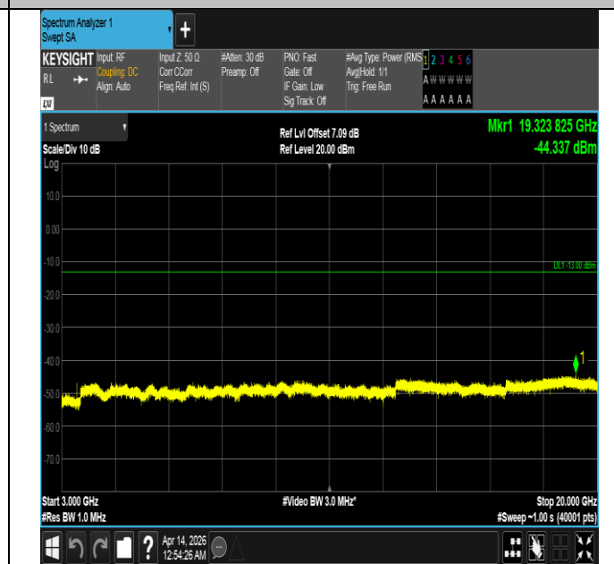
Band66-10MHz-16QAM-132322-1RB#0-3000~20000-PASS
