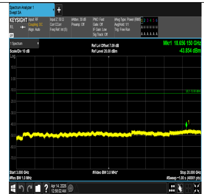
Band66-10MHz-16QAM-132322-50RB#0-3000~20000-PASS
