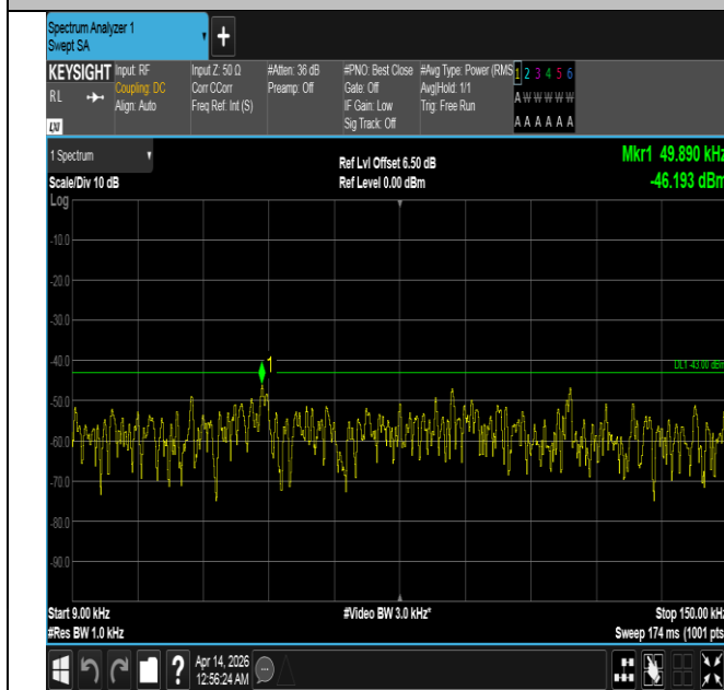
Band66-10MHz-QPSK-132322-50RB#0-0.009~0.15-PASS
