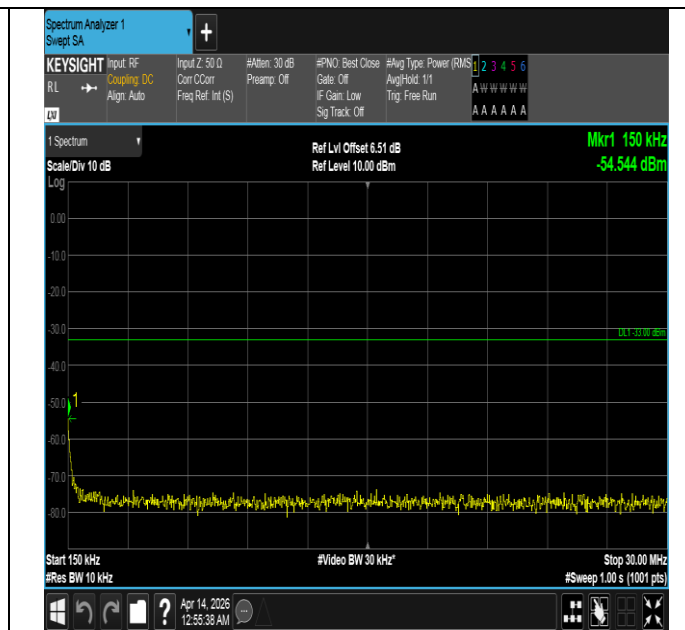
Band66-10MHz-16QAM-132322-1RB#49-0.15~30-PASS
