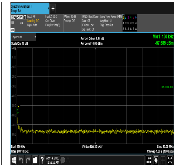
Band66-10MHz-QPSK-132322-1RB#0-0.15~30-PASS
