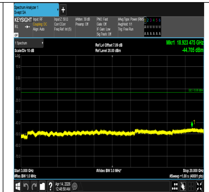
Band66-10MHz-16QAM-132022-1RB#0-3000~20000-PASS
