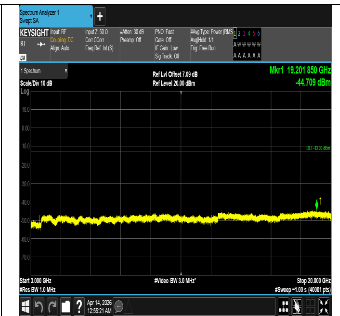
Band66-10MHz-QPSK-132322-1RB#49-3000~20000-PASS
