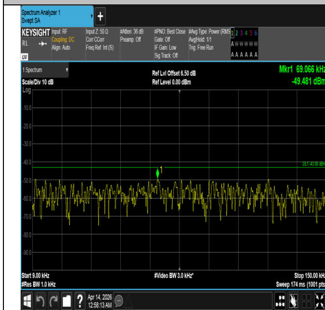
Band66-10MHz-QPSK-132622-1RB#0-0.009~0.15-PASS
