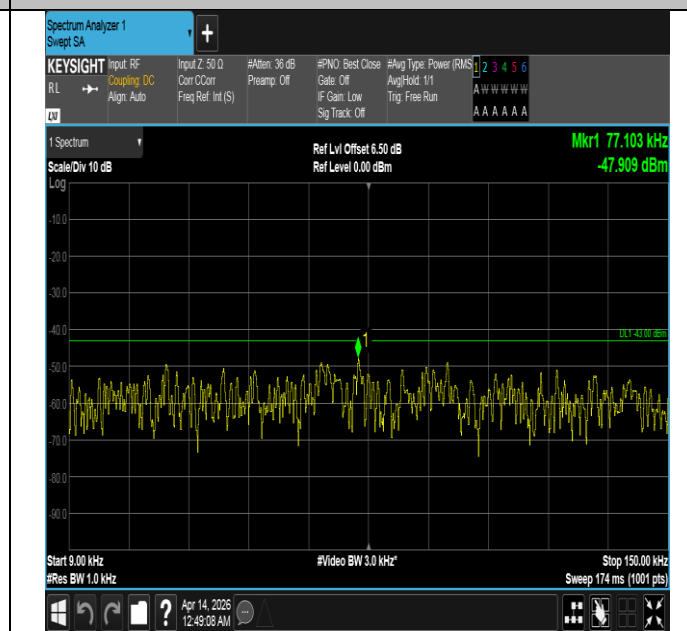
Band66-10MHz-QPSK-132022-1RB#49-0.009~0.15-PASS
