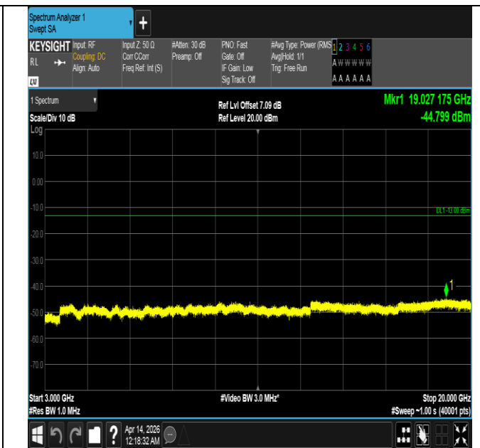
Band66-5MHz-16QAM-132647-25RB#0-3000~20000-PASS
