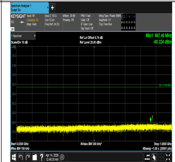
Band66-10MHz-16QAM-132022-1RB#0-30~1000-PASS
