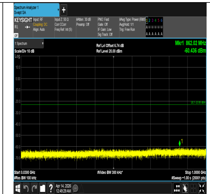
Band66-10MHz-QPSK-132022-1RB#49-30~1000-PASS
