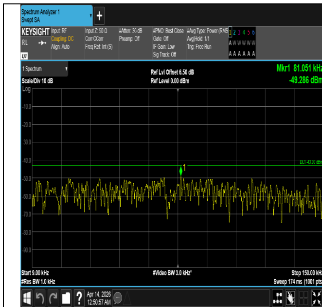
Band66-10MHz-QPSK-132022-50RB#0-0.009~0.15-PASS
