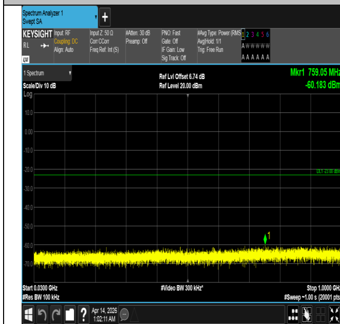
Band66-10MHz-QPSK-132622-50RB#0-30~1000-PASS
