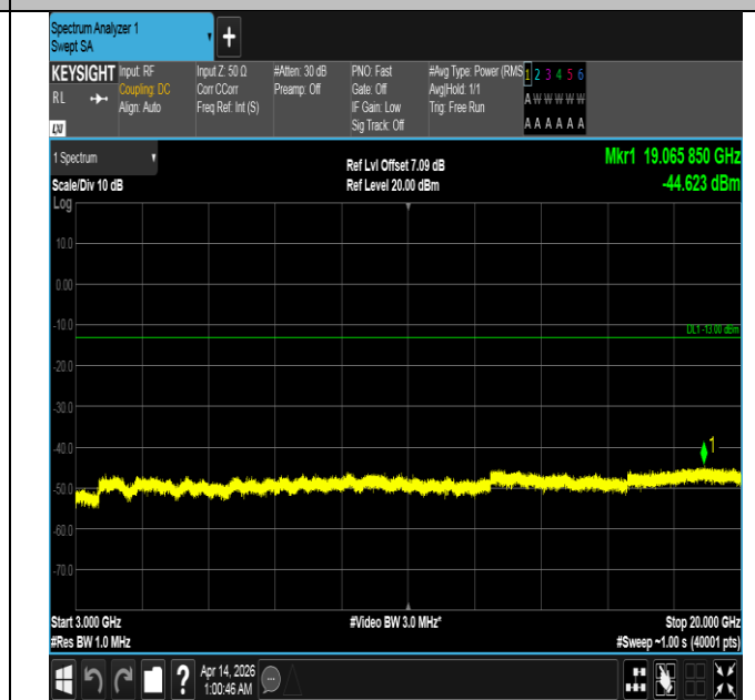
Band66-10MHz-QPSK-132622-1RB#49-3000~20000-PASS
