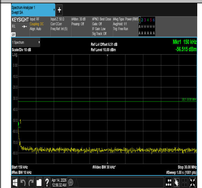
Band66-10MHz-QPSK-132322-50RB#0-0.15~30-PASS
