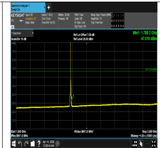
Band66-10MHz-QPSK-132622-1RB#0-1000~3000-PASS
