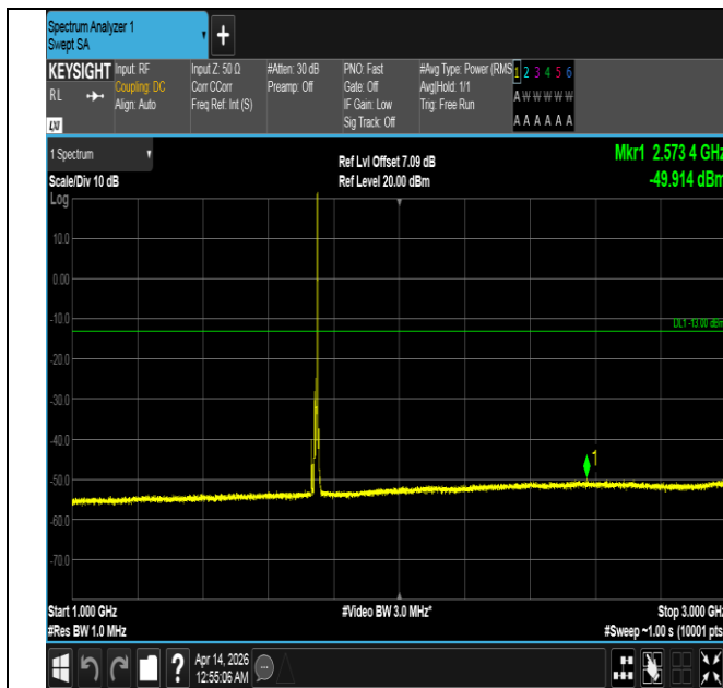
Band66-10MHz-QPSK-132322-1RB#49-1000~3000-PASS
