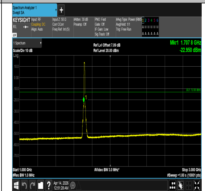
Band66-10MHz-QPSK-132022-50RB#0-1000~3000-PASS
