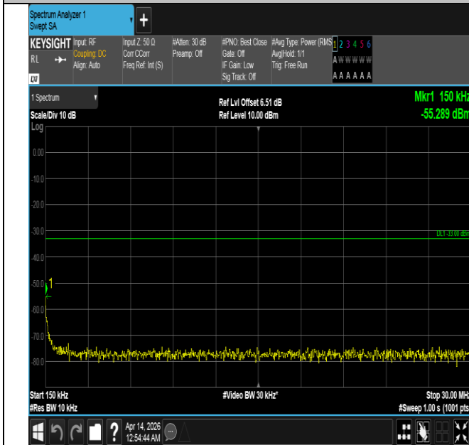
Band66-10MHz-QPSK-132322-1RB#49-0.15~30-PASS
