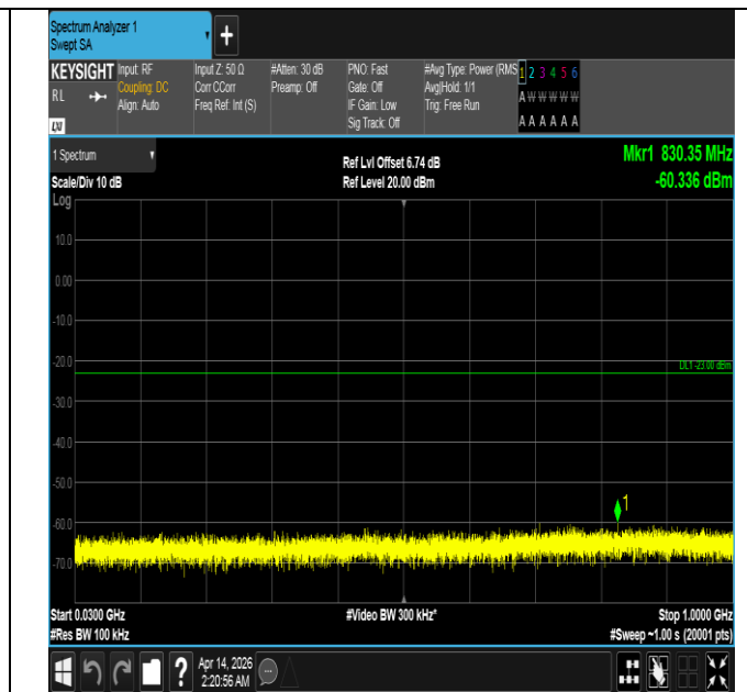
Band66-20MHz-QPSK-132072-1RB#99-30~1000-PASS
