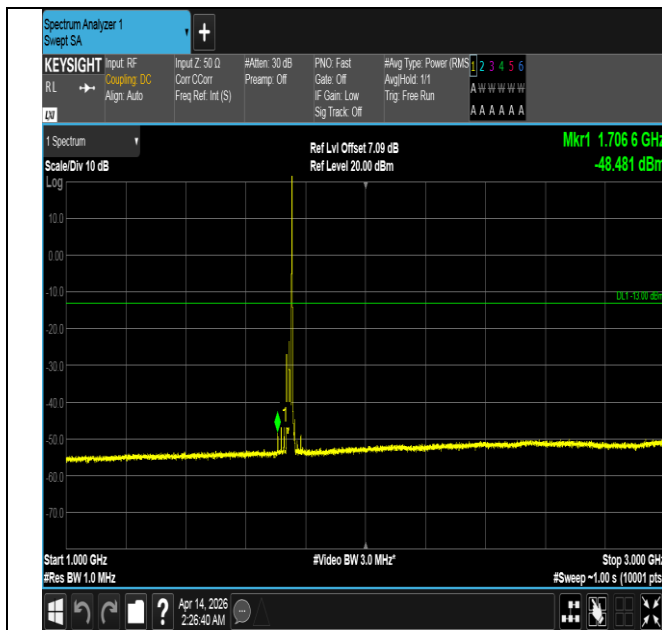
Band66-20MHz-QPSK-132322-1RB#99-1000~3000-PASS
