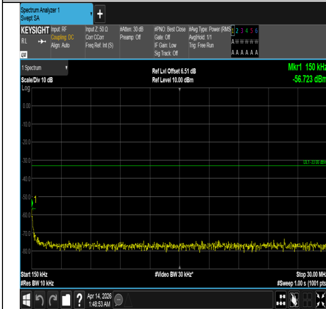
Band66-15MHz-16QAM-132597-75RB#0-0.15~30-PASS
