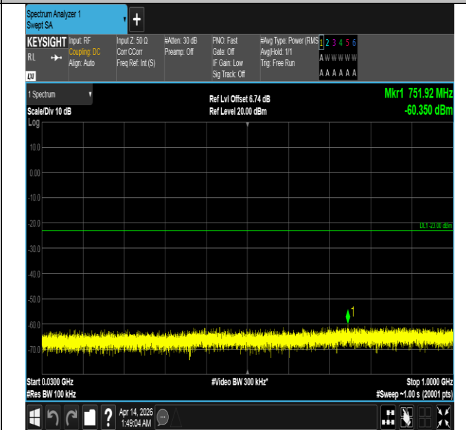
Band66-15MHz-16QAM-132597-75RB#0-30~1000-PASS
