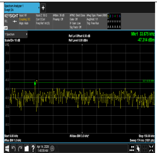
Band66-15MHz-QPSK-132597-1RB#74-0.009~0.15-PASS
