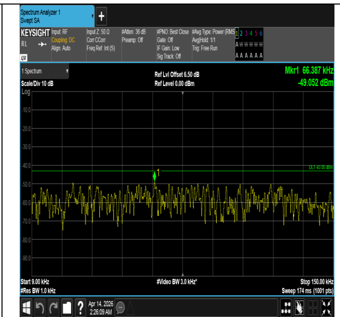
Band66-20MHz-QPSK-132322-1RB#99-0.009~0.15-PASS
