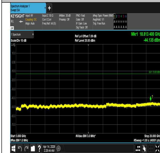
Band66-20MHz-QPSK-132322-100RB#0-3000~20000-PASS
