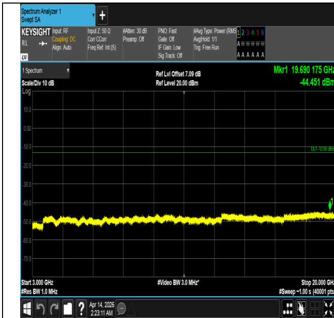
Band66-20MHz-QPSK-132072-100RB#0-3000~20000-PASS
