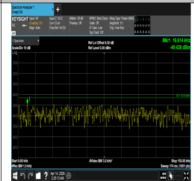
Band66-20MHz-16QAM-132322-1RB#0-0.009~0.15-PASS
