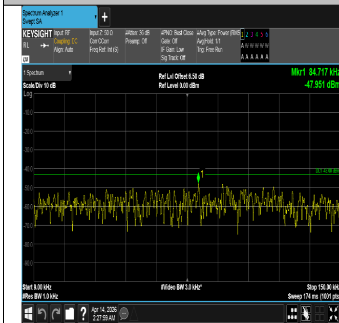
Band66-20MHz-QPSK-132322-100RB#0-0.009~0.15-PASS
