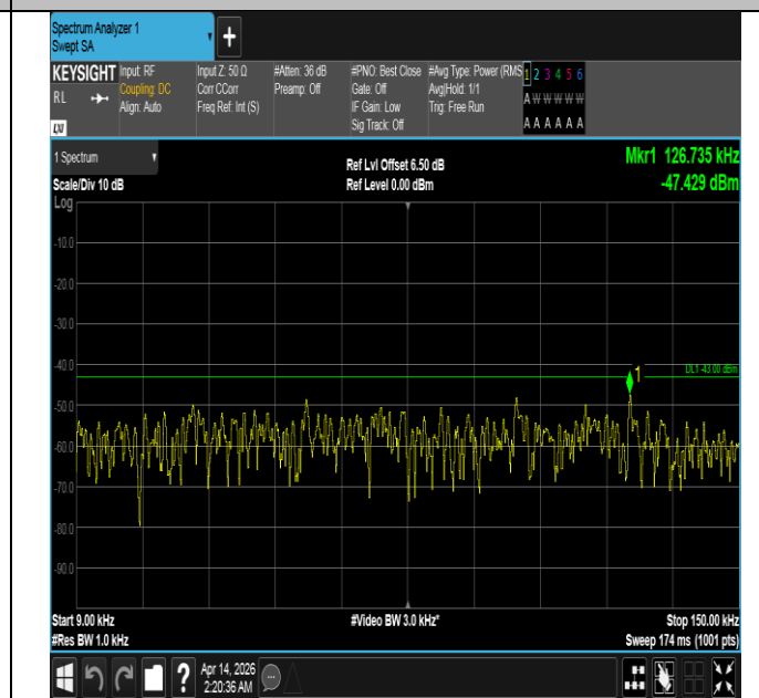
Band66-20MHz-QPSK-132072-1RB#99-0.009~0.15-PASS
