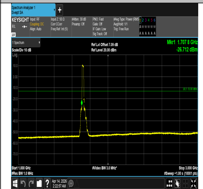
Band66-20MHz-QPSK-132072-100RB#0-1000~3000-PASS
