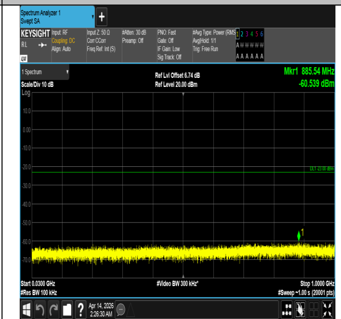
Band66-20MHz-QPSK-132322-1RB#99-30~1000-PASS
