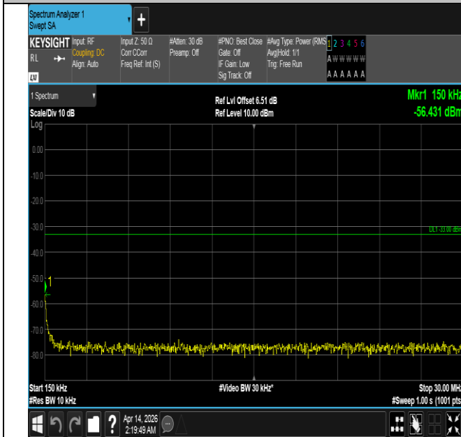
Band66-20MHz-16QAM-132072-1RB#0-0.15~30-PASS
