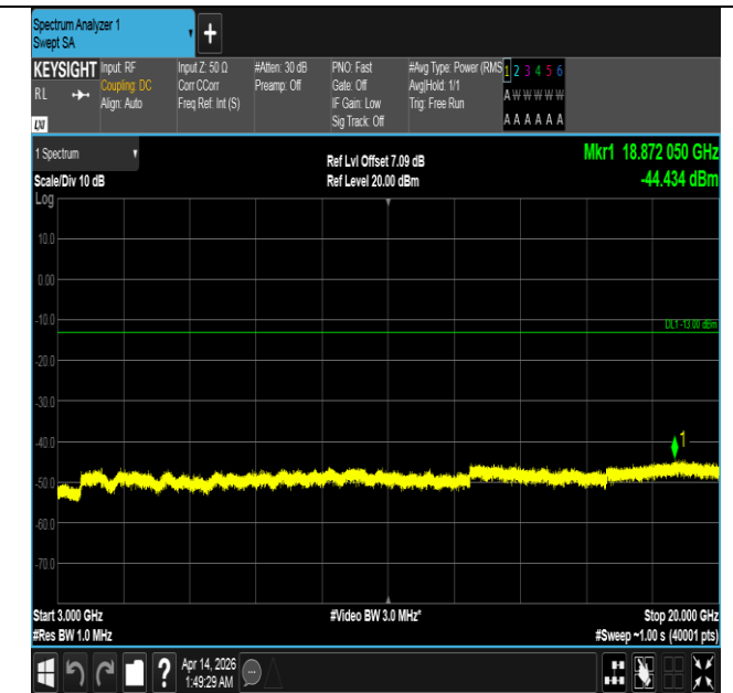
Band66-15MHz-16QAM-132597-75RB#0-3000~20000-PASS
