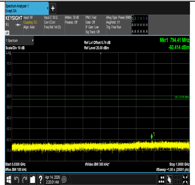
Band66-20MHz-16QAM-132072-1RB#0-30~1000-PASS
