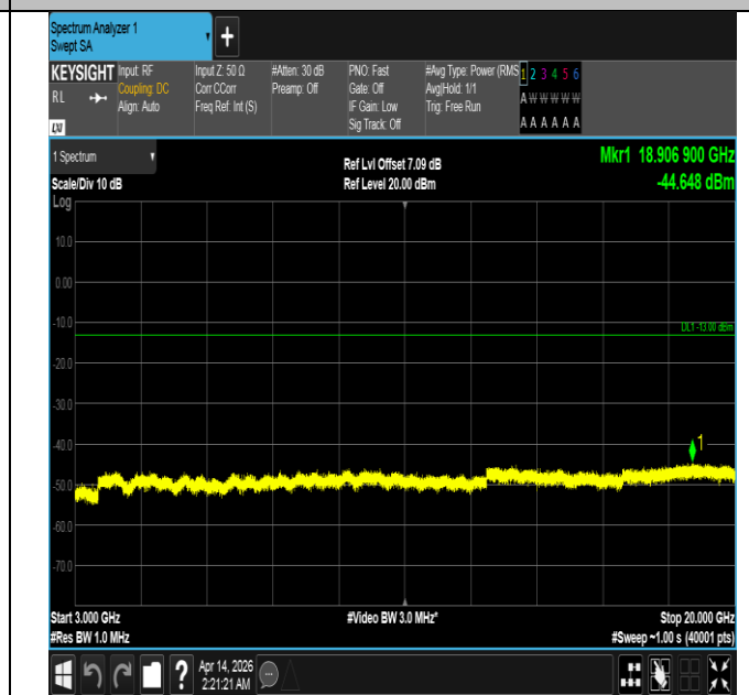
Band66-20MHz-QPSK-132072-1RB#99-3000~20000-PASS
