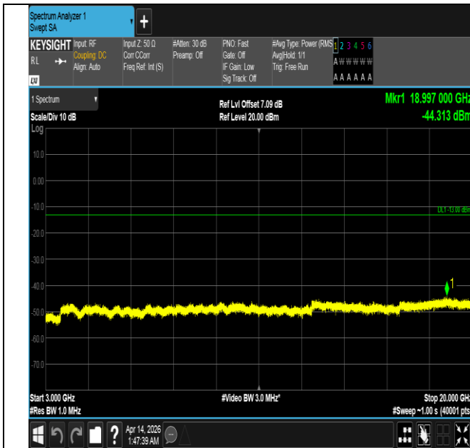
Band66-15MHz-16QAM-132597-1RB#74-3000~20000-PASS
