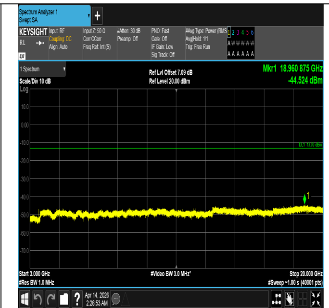
Band66-20MHz-QPSK-132322-1RB#99-3000~20000-PASS
