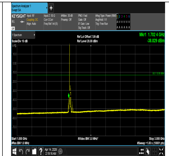
Band66-20MHz-QPSK-132072-1RB#0-1000~3000-PASS
