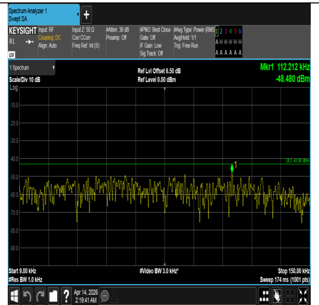
Band66-20MHz-16QAM-132072-1RB#0-0.009~0.15-PASS
