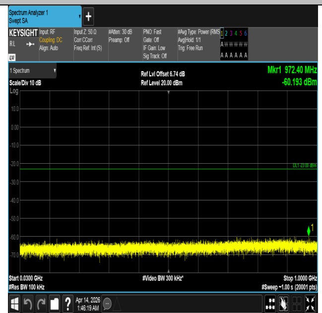
Band66-15MHz-QPSK-132597-1RB#74-30~1000-PASS
