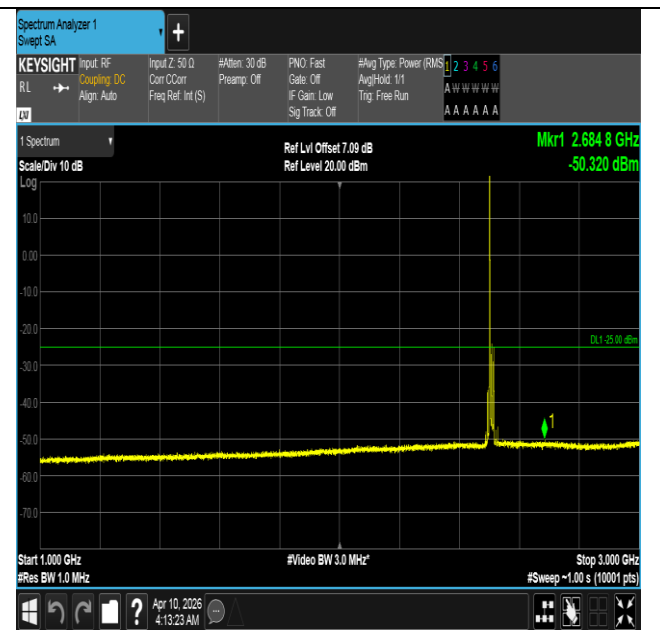
Band7-15MHz-QPSK-20825-1RB#0-1000~3000-PASS
