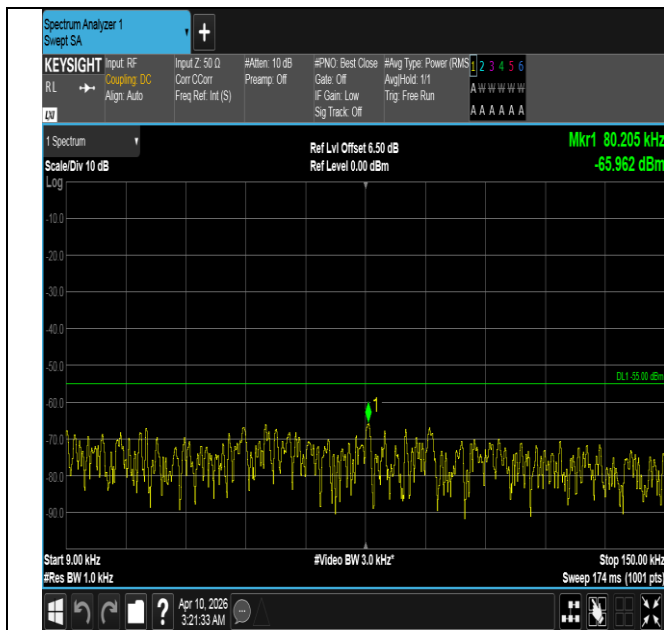
Band7-10MHz-16QAM-21400-1RB#0-0.009~0.15-PASS
