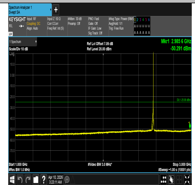
Band7-10MHz-QPSK-21400-1RB#49-1000~3000-PASS
