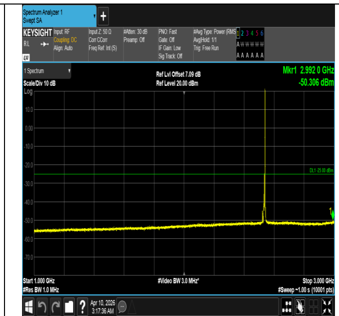
Band7-10MHz-16QAM-21100-1RB#49-1000~3000-PASS
