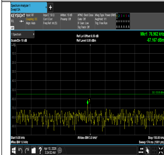
Band7-10MHz-QPSK-21400-50RB#0-0.009~0.15-PASS
