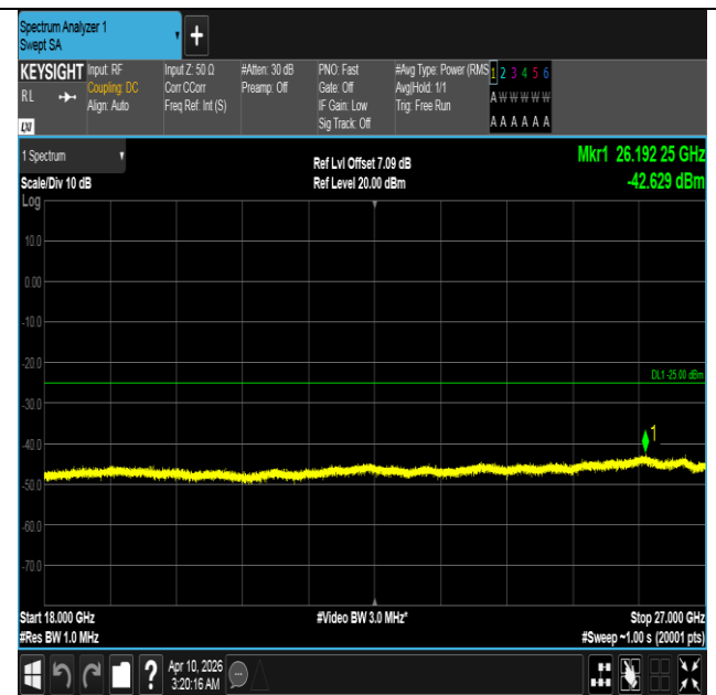
Band7-10MHz-16QAM-21100-50RB#0-18000~27000-PASS
