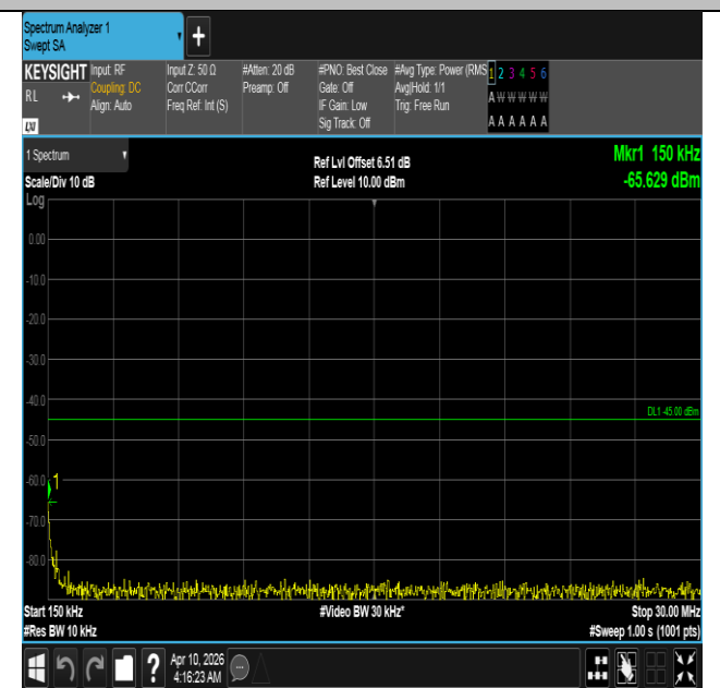
Band7-15MHz-16QAM-20825-1RB#74-0.15~30-PASS
