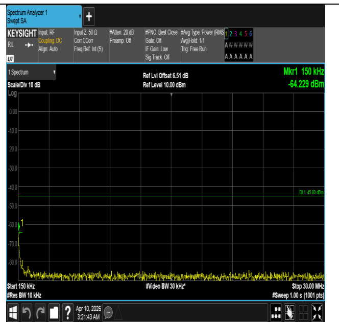
Band7-10MHz-16QAM-21400-1RB#0-0.15~30-PASS
