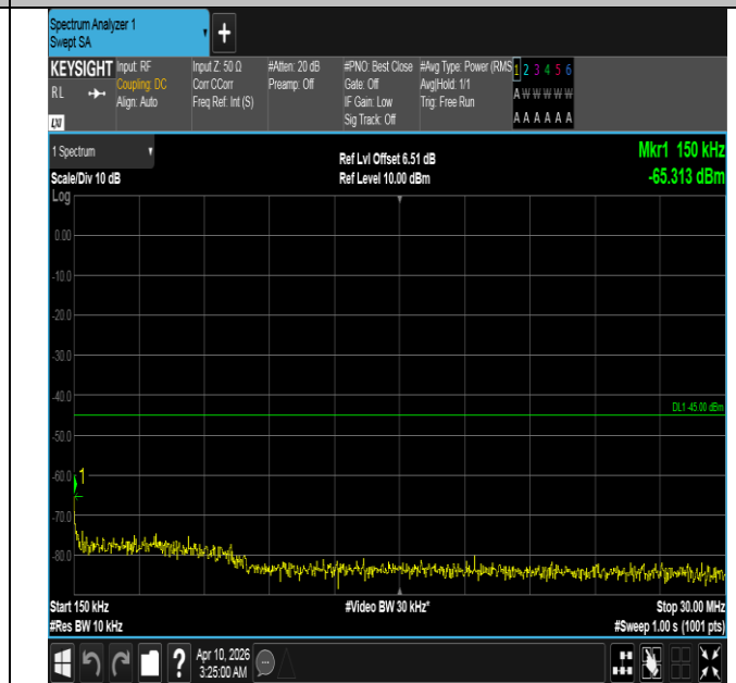
Band7-10MHz-QPSK-21400-50RB#0-0.15~30-PASS
