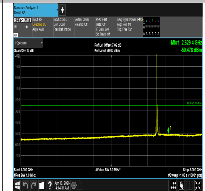
Band7-15MHz-16QAM-20825-1RB#0-1000~3000-PASS
