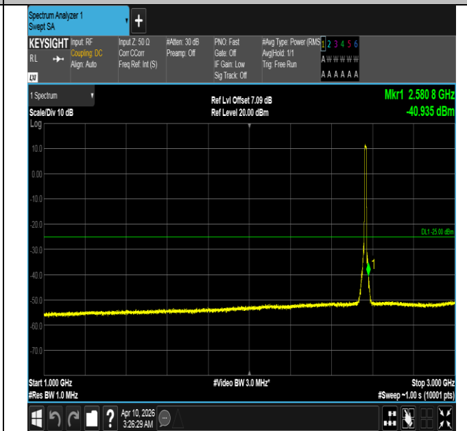
Band7-10MHz-16QAM-21400-50RB#0-1000~3000-PASS
