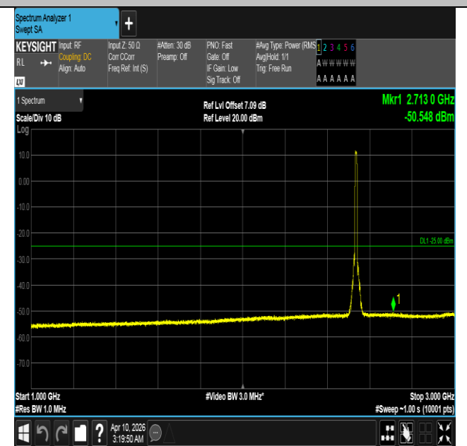
Band7-10MHz-16QAM-21100-50RB#0-1000~3000-PASS
