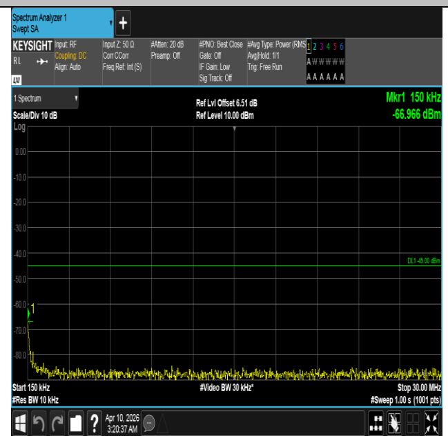
Band7-10MHz-QPSK-21400-1RB#0-0.15~30-PASS
