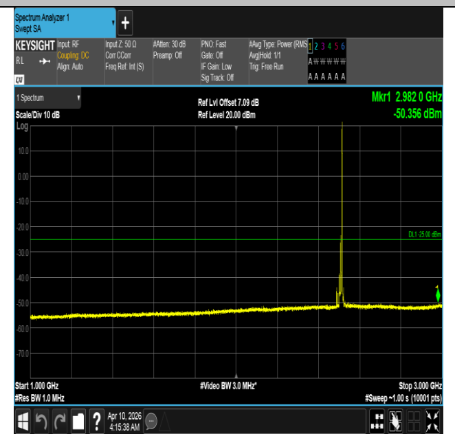
Band7-15MHz-QPSK-20825-1RB#74-1000~3000-PASS
