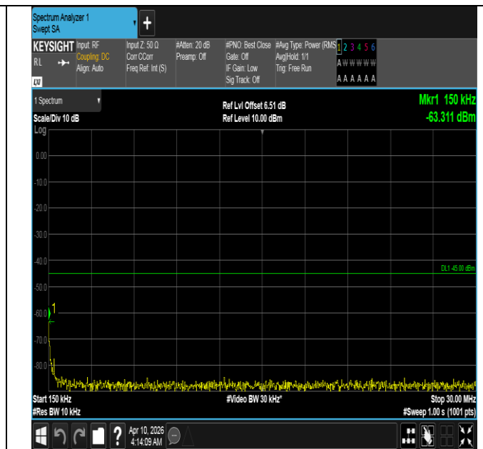
Band7-15MHz-16QAM-20825-1RB#0-0.15~30-PASS
