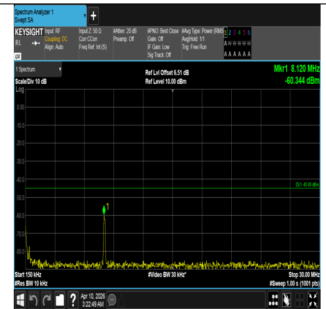
Band7-10MHz-QPSK-21400-1RB#49-0.15~30-PASS
