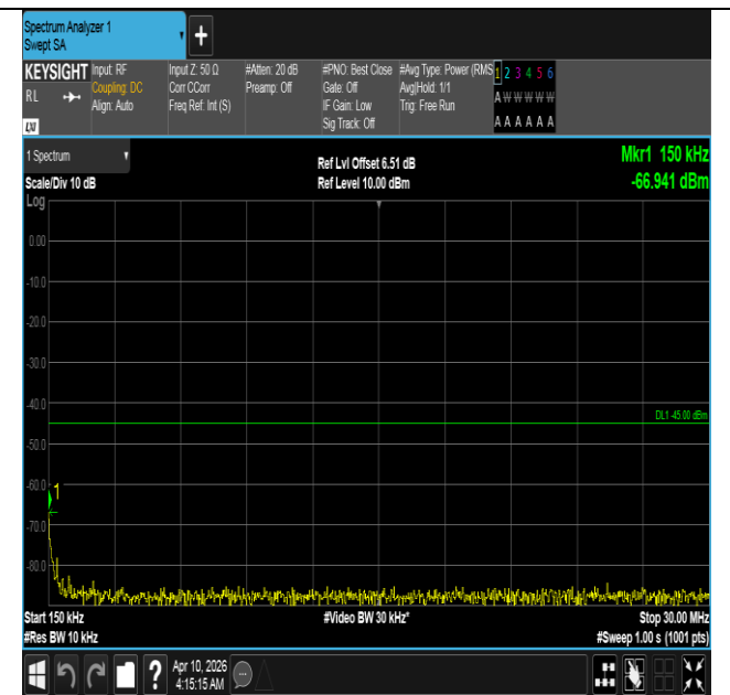
Band7-15MHz-QPSK-20825-1RB#74-0.15~30-PASS
