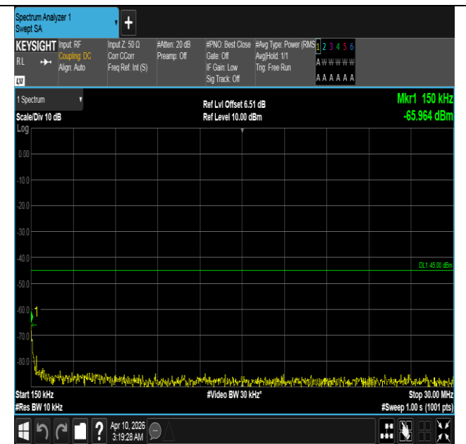
Band7-10MHz-16QAM-21100-50RB#0-0.15~30-PASS
