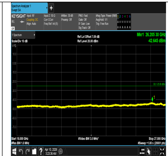
Band7-10MHz-QPSK-21400-1RB#49-18000~27000-PASS
