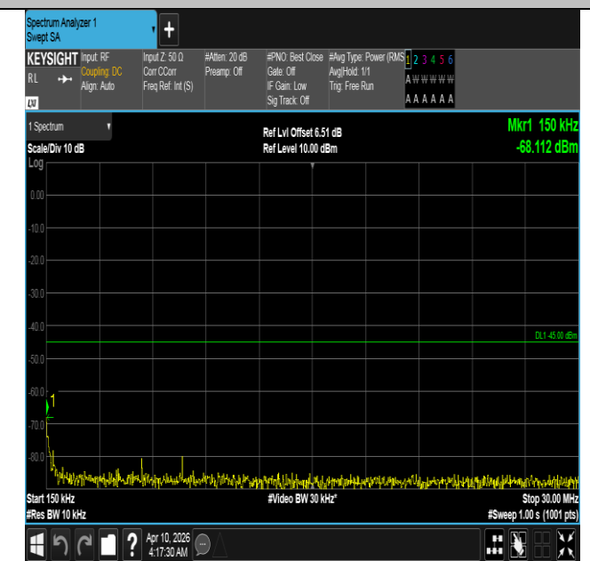
Band7-15MHz-QPSK-20825-75RB#0-0.15~30-PASS
