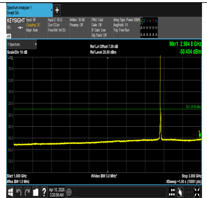
Band7-10MHz-QPSK-21400-1RB#0-1000~3000-PASS
