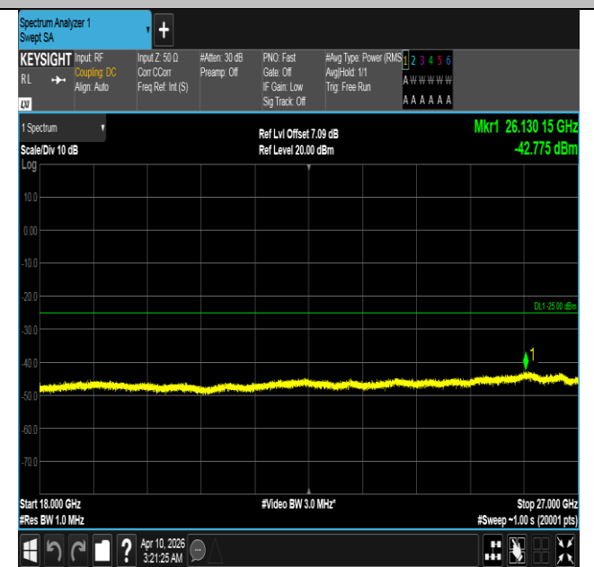
Band7-10MHz-QPSK-21400-1RB#0-18000~27000-PASS
