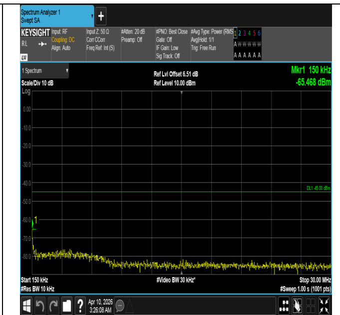
Band7-10MHz-16QAM-21400-50RB#0-0.15~30-PASS
