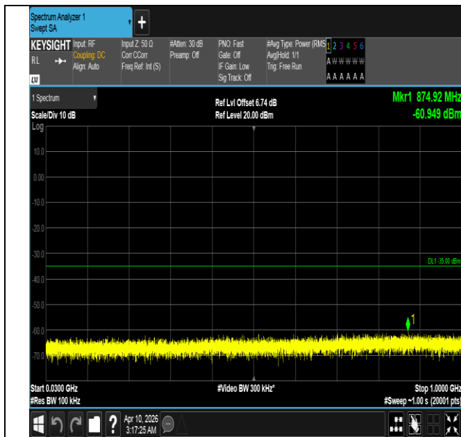
Band7-10MHz-16QAM-21100-1RB#49-30~1000-PASS
