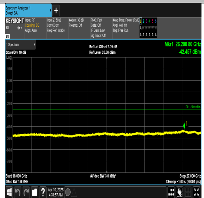
Band7-15MHz-QPSK-21375-75RB#0-18000~27000-PASS
