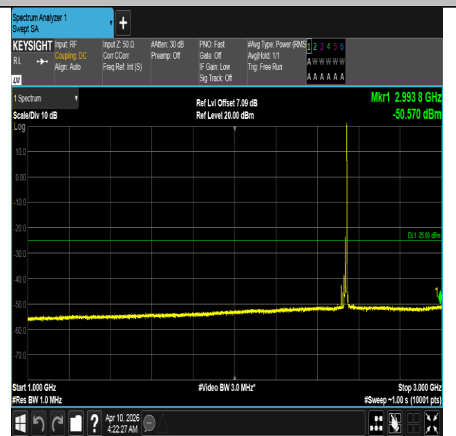
Band7-15MHz-QPSK-21100-1RB#74-1000~3000-PASS
