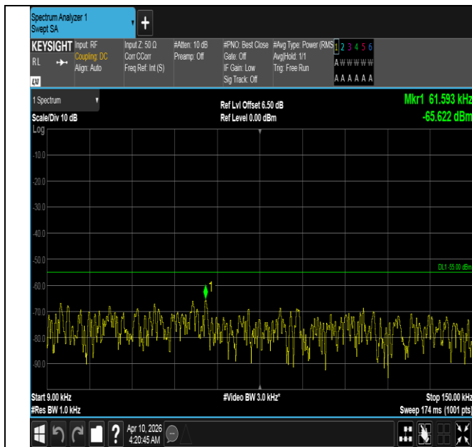
Band7-15MHz-16QAM-21100-1RB#0-0.009~0.15-PASS
