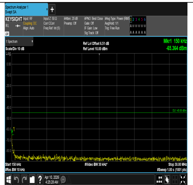
Band7-15MHz-16QAM-21100-75RB#0-0.15~30-PASS
