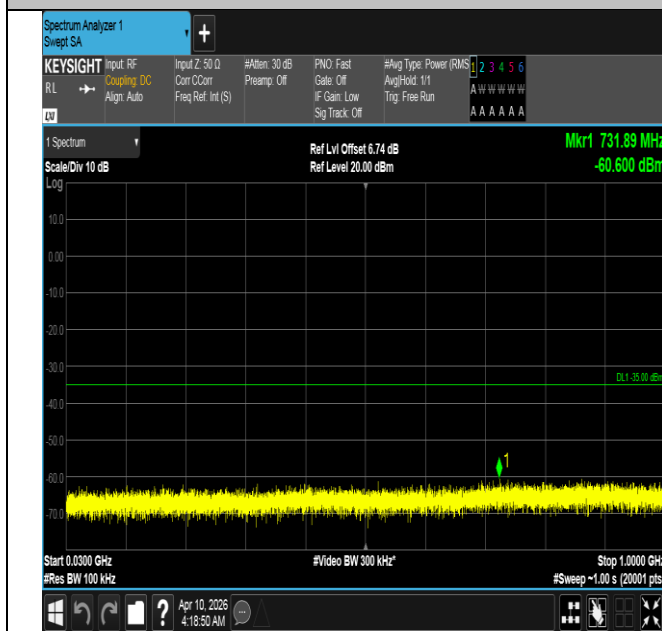
Band7-15MHz-16QAM-20825-75RB#0-30~1000-PASS
