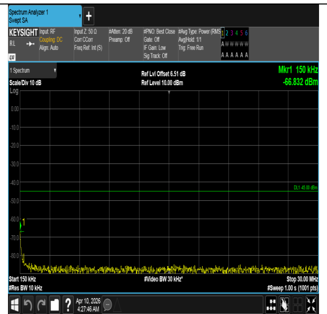
Band7-15MHz-16QAM-21375-1RB#0-0.15~30-PASS
