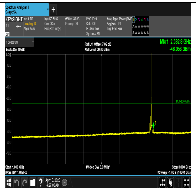
Band7-15MHz-QPSK-21375-1RB#0-1000~3000-PASS
