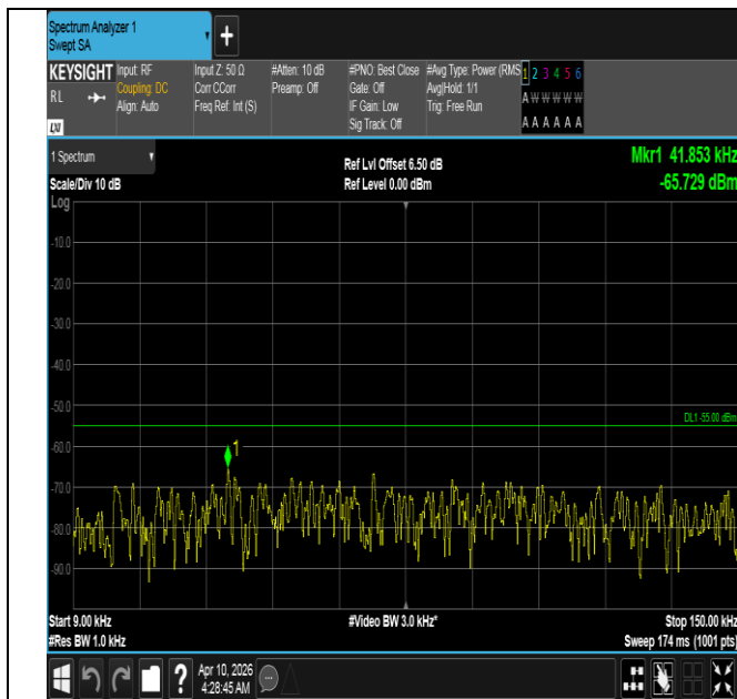
Band7-15MHz-QPSK-21375-1RB#74-0.009~0.15-PASS
