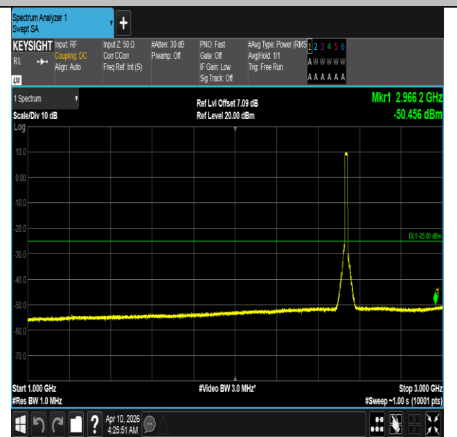
Band7-15MHz-16QAM-21100-75RB#0-1000~3000-PASS
