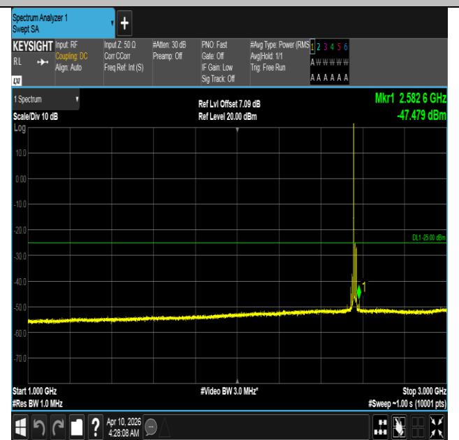
Band7-15MHz-16QAM-21375-1RB#0-1000~3000-PASS
