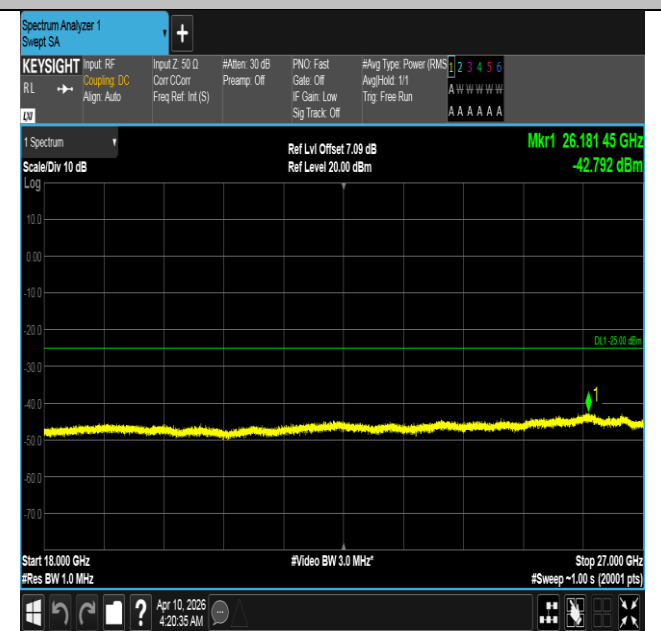
Band7-15MHz-QPSK-21100-1RB#0-18000~27000-PASS
