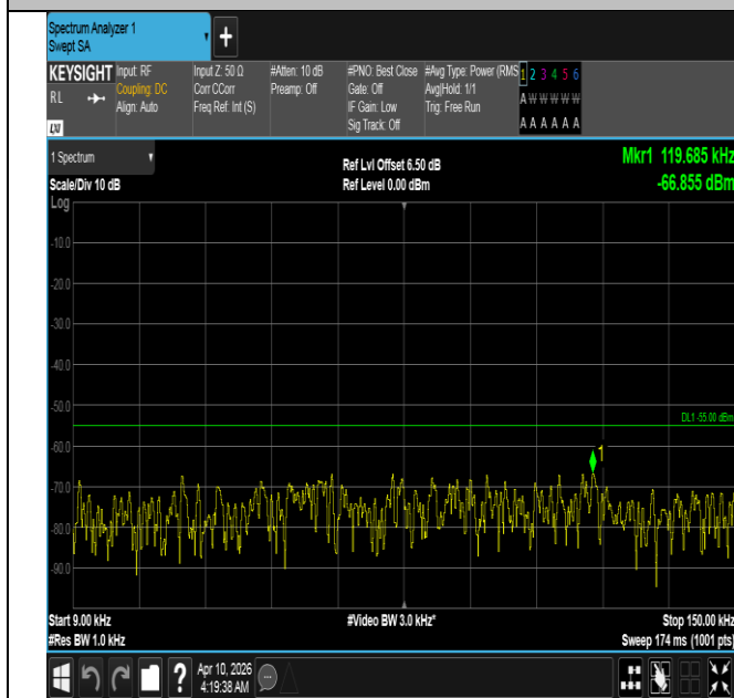
Band7-15MHz-QPSK-21100-1RB#0-0.009~0.15-PASS
