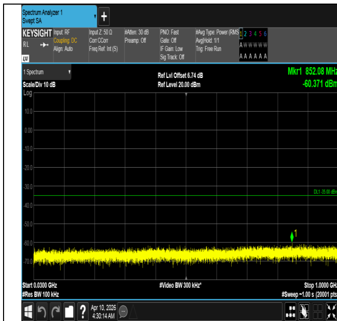
Band7-15MHz-16QAM-21375-1RB#74-30~1000-PASS
