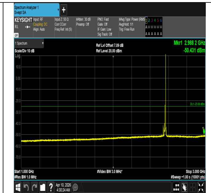
Band7-15MHz-16QAM-21375-1RB#74-1000~3000-PASS
