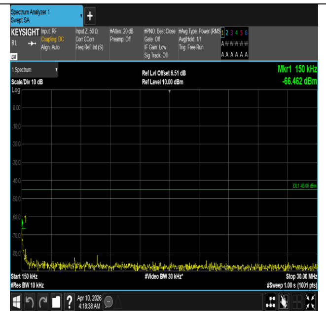
Band7-15MHz-16QAM-20825-75RB#0-0.15~30-PASS
