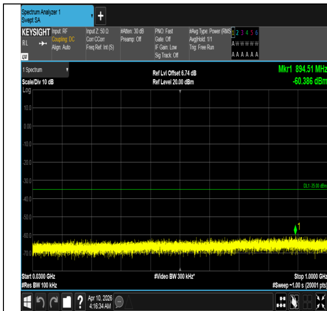
Band7-15MHz-16QAM-20825-1RB#74-30~1000-PASS
