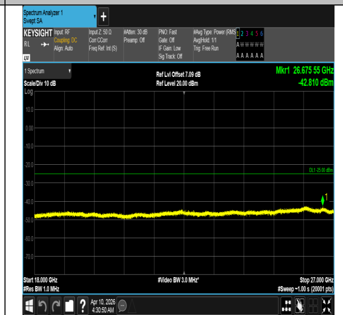
Band7-15MHz-16QAM-21375-1RB#74-18000~27000-PASS
