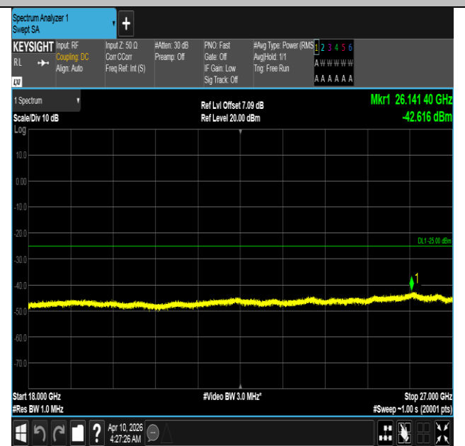
Band7-15MHz-QPSK-21375-1RB#0-18000~27000-PASS
