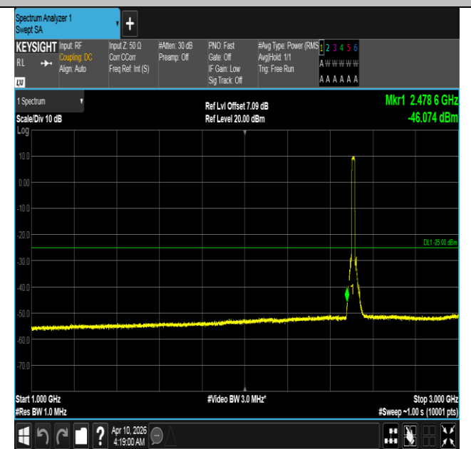
Band7-15MHz-16QAM-20825-75RB#0-1000~3000-PASS
