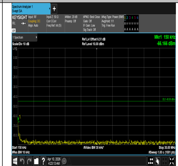
Band7-15MHz-16QAM-21100-1RB#74-0.15~30-PASS
