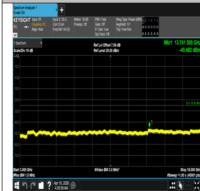
Band7-15MHz-16QAM-21375-1RB#74-3000~18000-PASS
