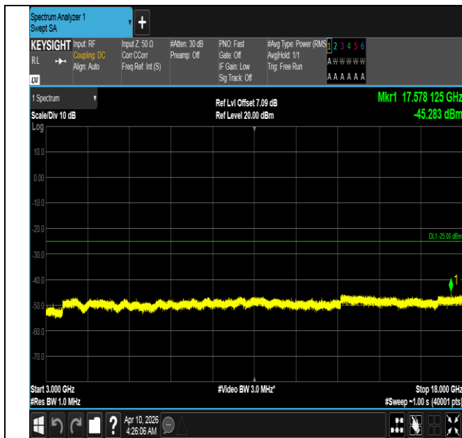
Band7-15MHz-16QAM-21100-75RB#0-3000~18000-PASS
