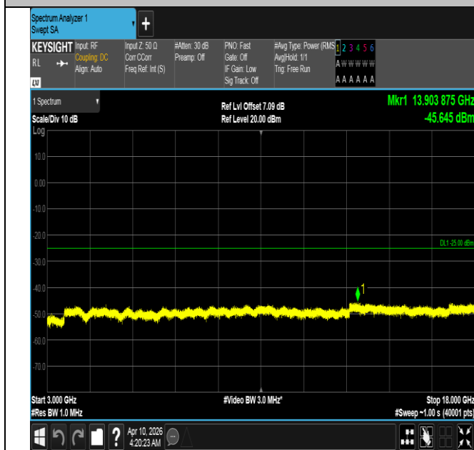
Band7-15MHz-QPSK-21100-1RB#0-3000~18000-PASS
