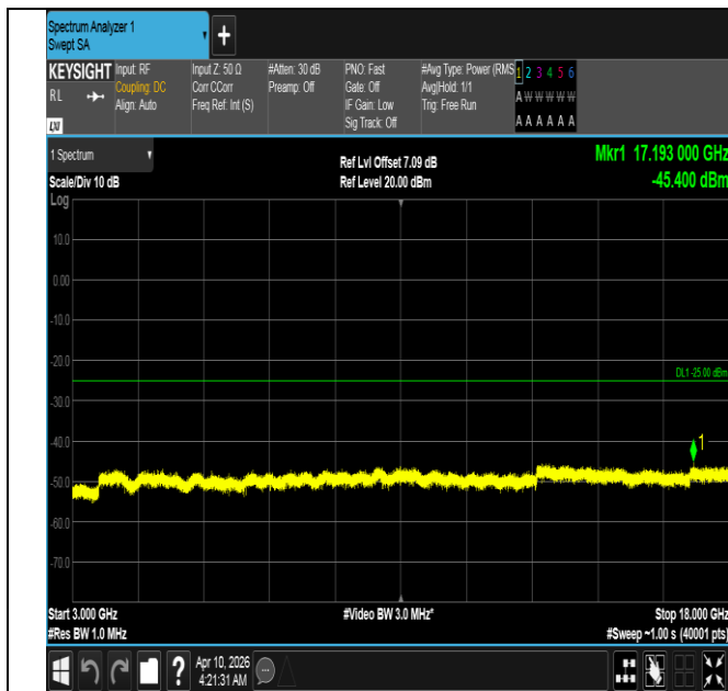
Band7-15MHz-16QAM-21100-1RB#0-3000~18000-PASS
