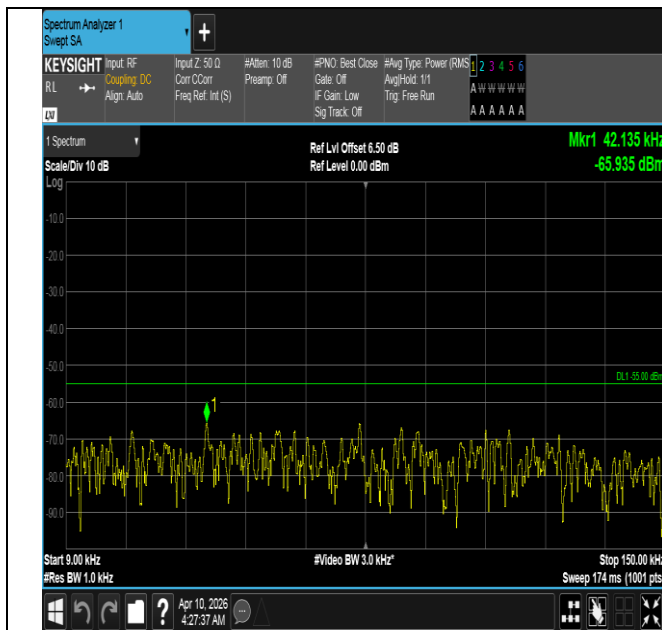
Band7-15MHz-16QAM-21375-1RB#0-0.009~0.15-PASS
