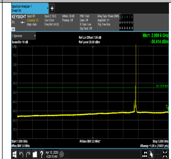
Band7-15MHz-QPSK-21375-1RB#74-1000~3000-PASS
