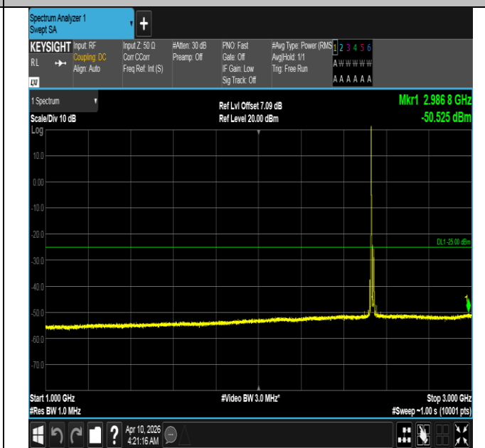
Band7-15MHz-16QAM-21100-1RB#0-1000~3000-PASS
