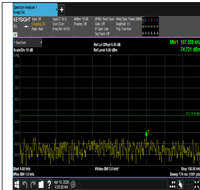
Band7-15MHz-16QAM-21100-75RB#0-0.009~0.15-PASS
