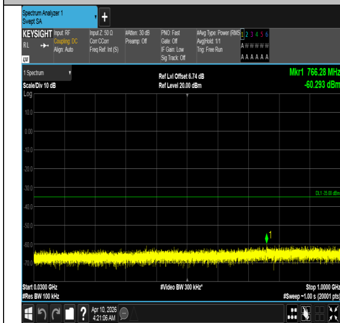
Band7-15MHz-16QAM-21100-1RB#0-30~1000-PASS
