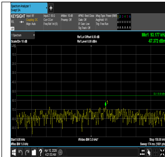
Band7-15MHz-QPSK-21100-1RB#74-0.009~0.15-PASS
