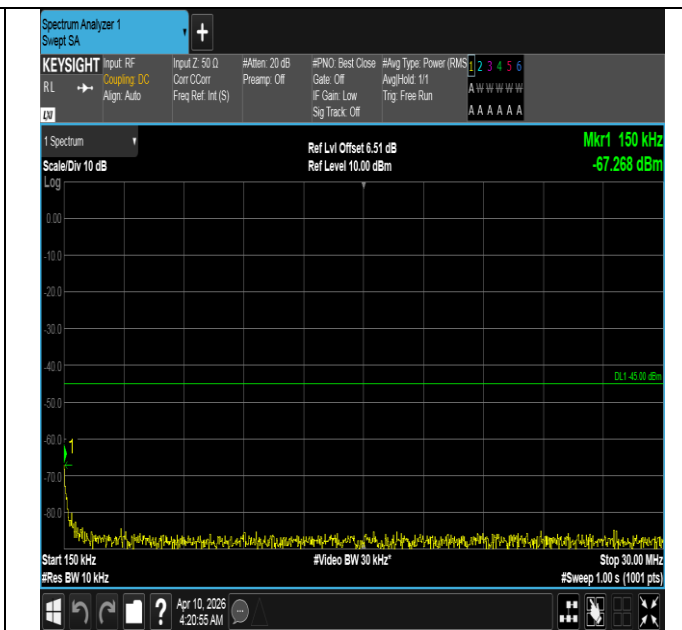
Band7-15MHz-16QAM-21100-1RB#0-0.15~30-PASS
