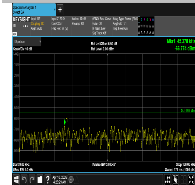
Band7-15MHz-QPSK-21375-1RB#0-0.009~0.15-PASS
