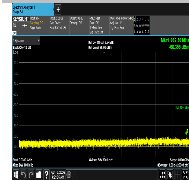
Band7-15MHz-QPSK-21375-1RB#74-30~1000-PASS
