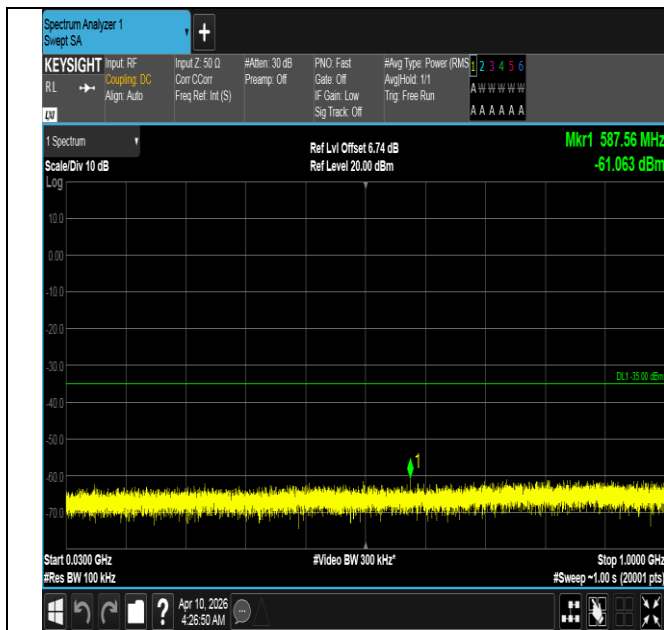
Band7-15MHz-QPSK-21375-1RB#0-30~1000-PASS
