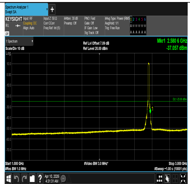
Band7-15MHz-QPSK-21375-75RB#0-1000~3000-PASS
