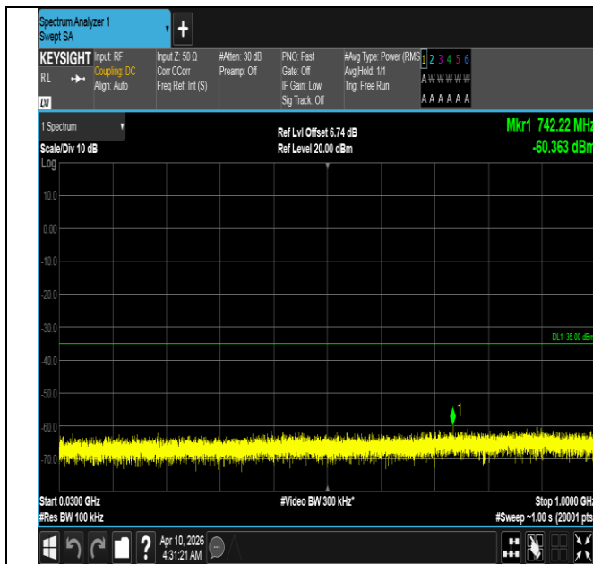
Band7-15MHz-QPSK-21375-75RB#0-30~1000-PASS
