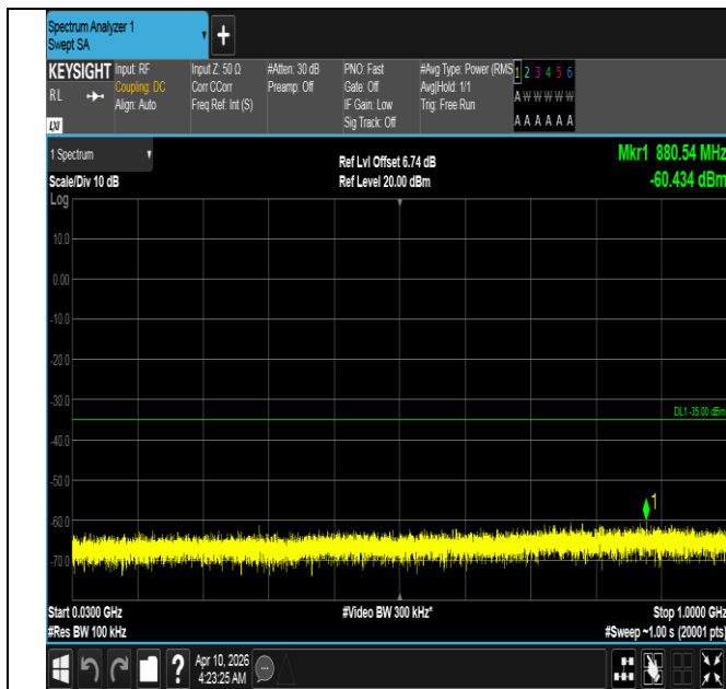
Band7-15MHz-16QAM-21100-1RB#74-30~1000-PASS
