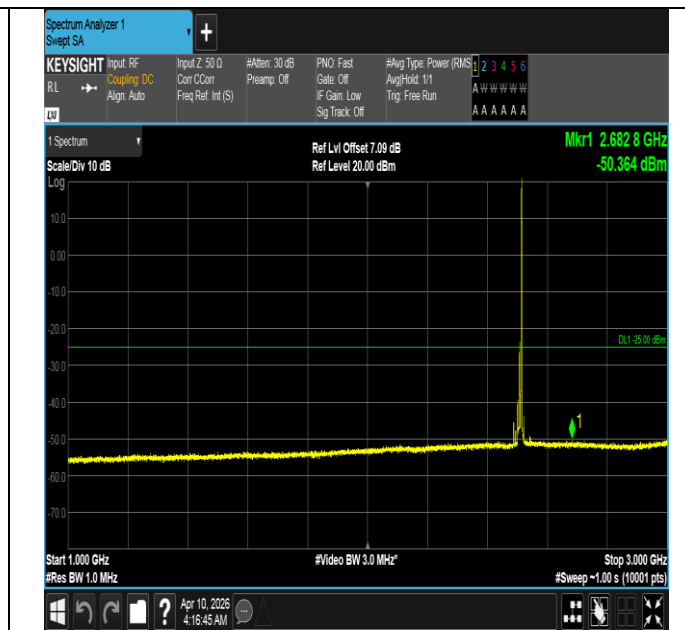
Band7-15MHz-16QAM-20825-1RB#74-1000~3000-PASS
