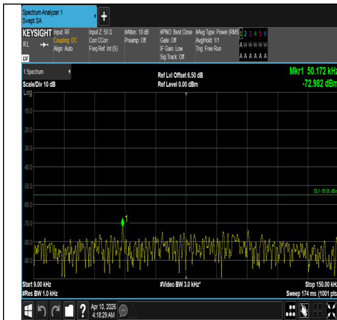
Band7-15MHz-16QAM-20825-75RB#0-0.009~0.15-PASS
