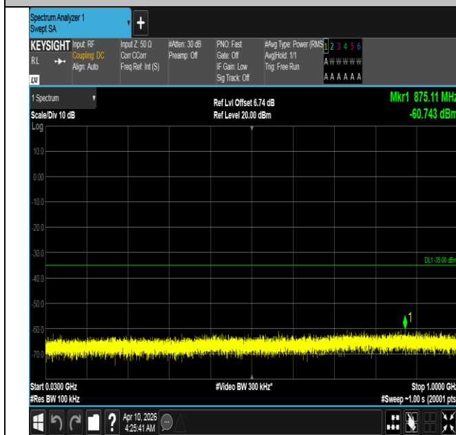
Band7-15MHz-16QAM-21100-75RB#0-30~1000-PASS
