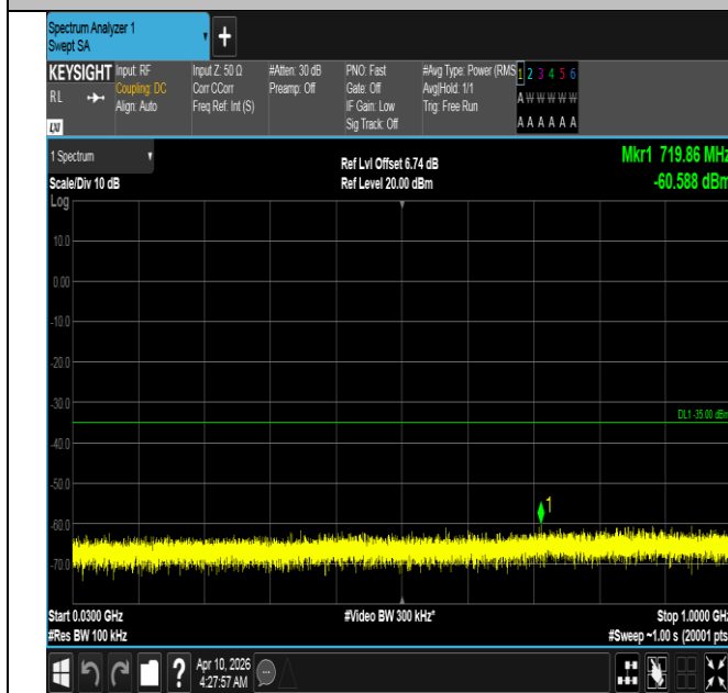
Band7-15MHz-16QAM-21375-1RB#0-30~1000-PASS
