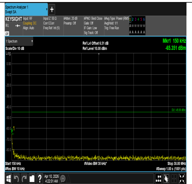
Band7-15MHz-QPSK-21100-1RB#74-0.15~30-PASS
