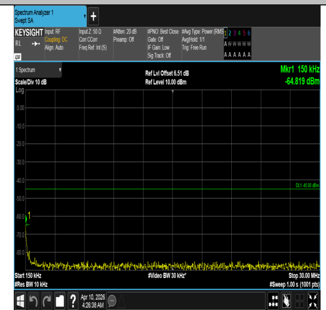
Band7-15MHz-QPSK-21375-1RB#0-0.15~30-PASS
