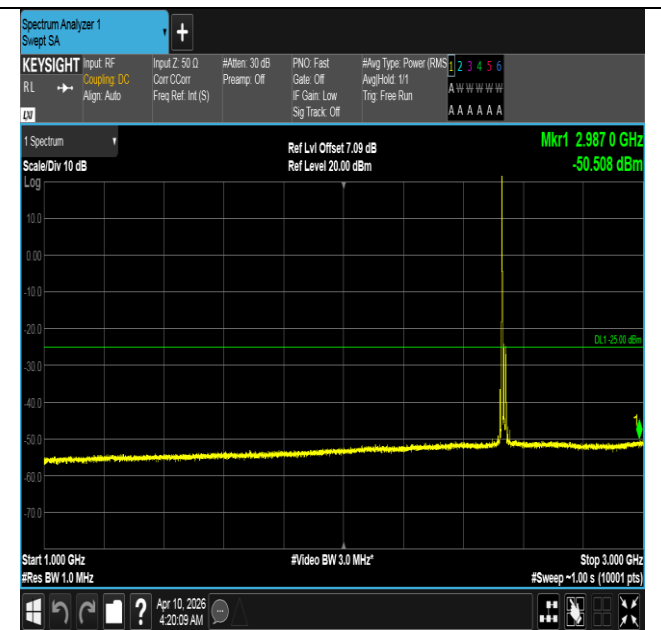
Band7-15MHz-QPSK-21100-1RB#0-1000~3000-PASS
