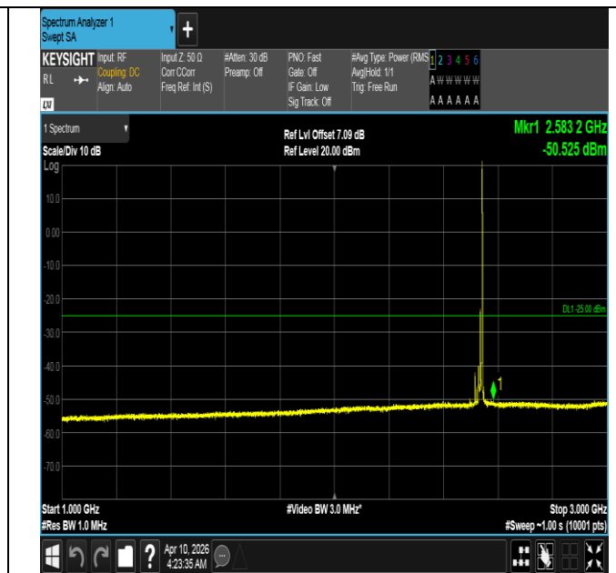
Band7-15MHz-16QAM-21100-1RB#74-1000~3000-PASS
