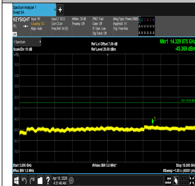
Band7-15MHz-QPSK-21375-75RB#0-3000~18000-PASS
