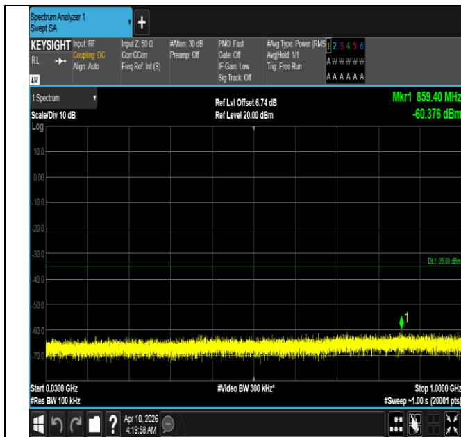
Band7-15MHz-QPSK-21100-1RB#0-30~1000-PASS
