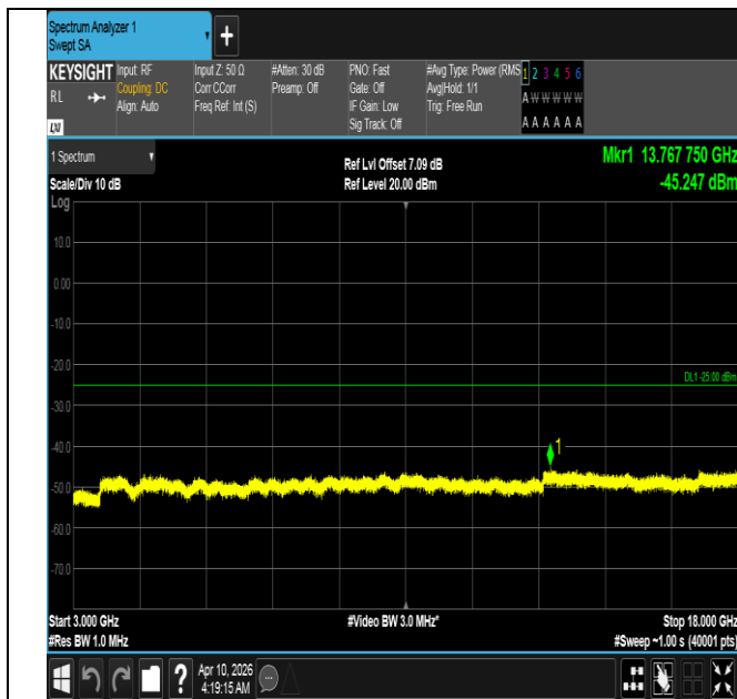
Band7-15MHz-16QAM-20825-75RB#0-3000~18000-PASS
