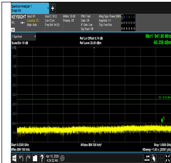
Band7-15MHz-QPSK-21100-75RB#0-30~1000-PASS
