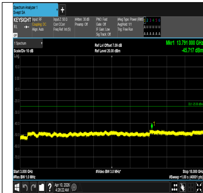
Band7-15MHz-16QAM-21375-1RB#0-3000~18000-PASS
