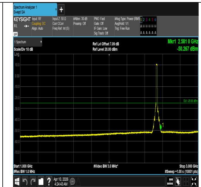
Band7-15MHz-QPSK-21100-75RB#0-1000~3000-PASS
