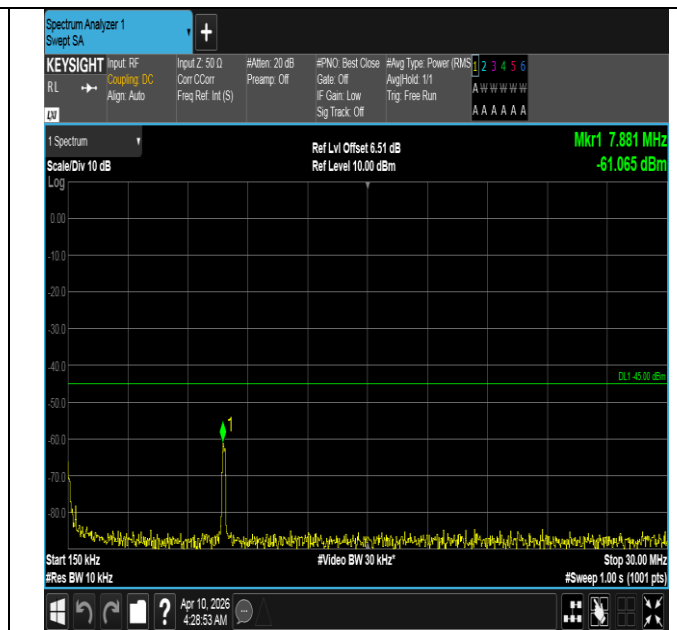
Band7-15MHz-QPSK-21375-1RB#74-0.15~30-PASS
