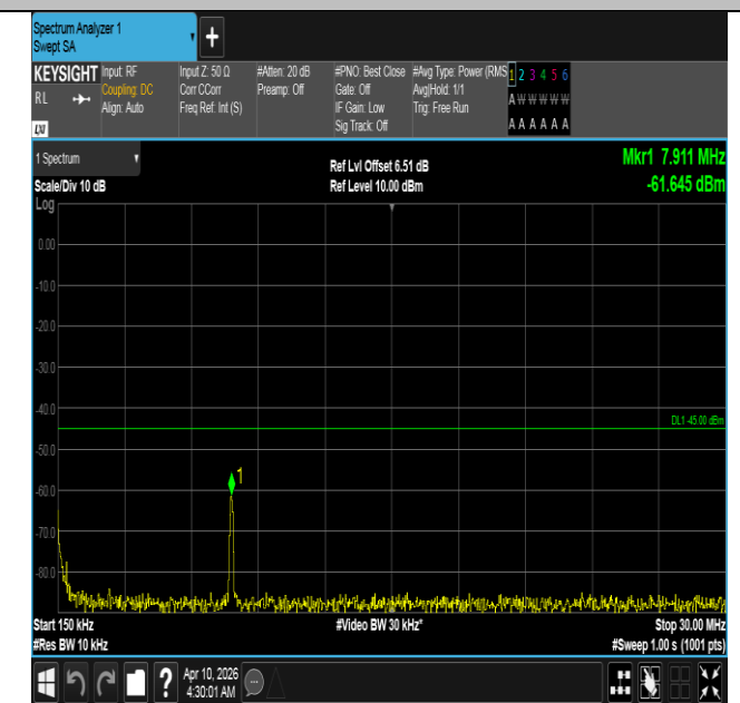
Band7-15MHz-16QAM-21375-1RB#74-0.15~30-PASS
