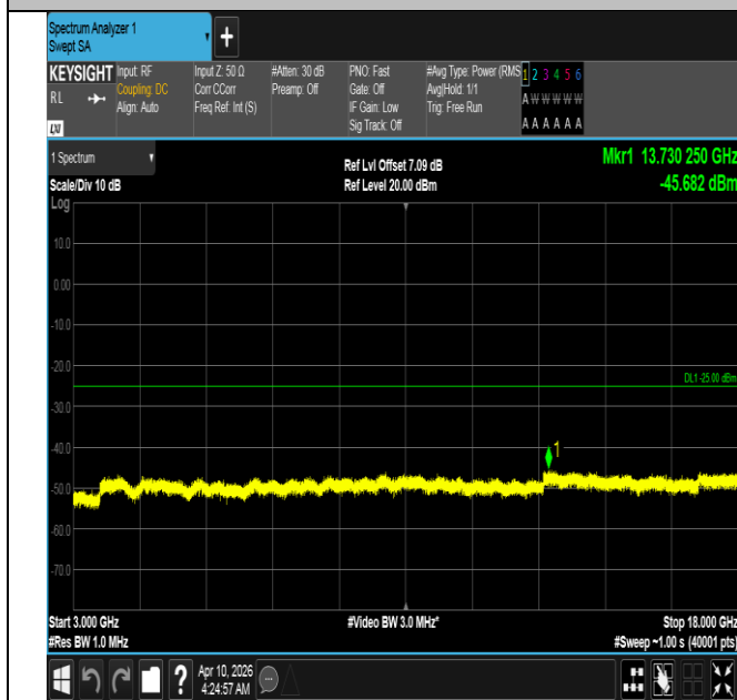
Band7-15MHz-QPSK-21100-75RB#0-3000~18000-PASS
