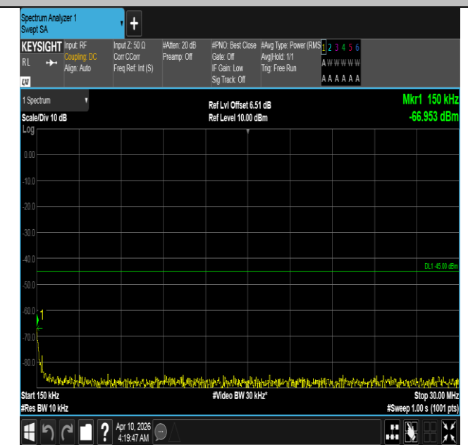
Band7-15MHz-QPSK-21100-1RB#0-0.15~30-PASS
