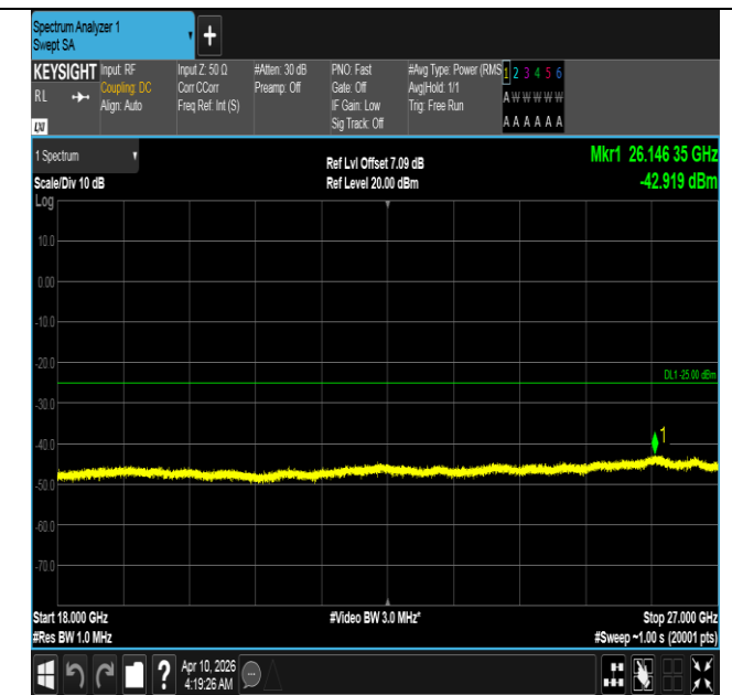
Band7-15MHz-16QAM-20825-75RB#0-18000~27000-PASS
