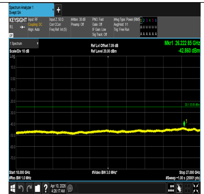
Band7-15MHz-16QAM-21100-75RB#0-18000~27000-PASS
