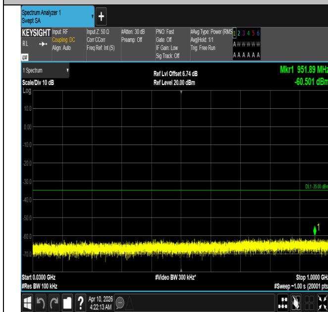
Band7-15MHz-QPSK-21100-1RB#74-30~1000-PASS
