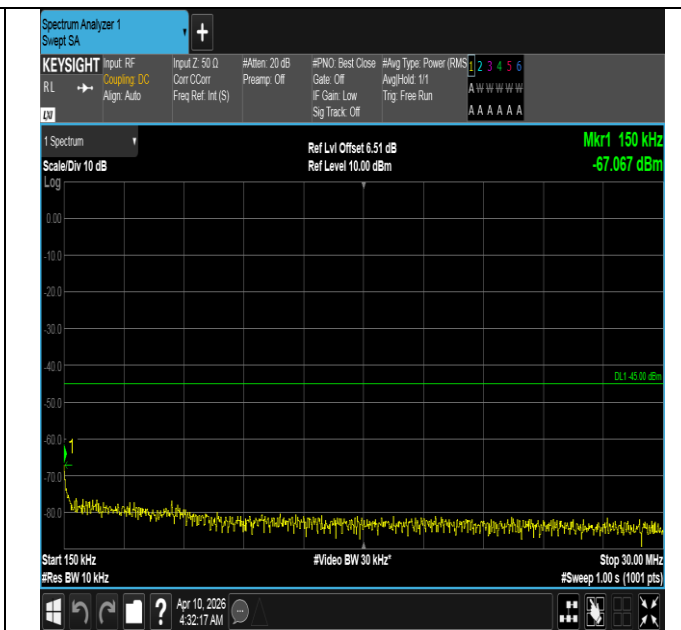
Band7-15MHz-16QAM-21375-75RB#0-0.15~30-PASS
