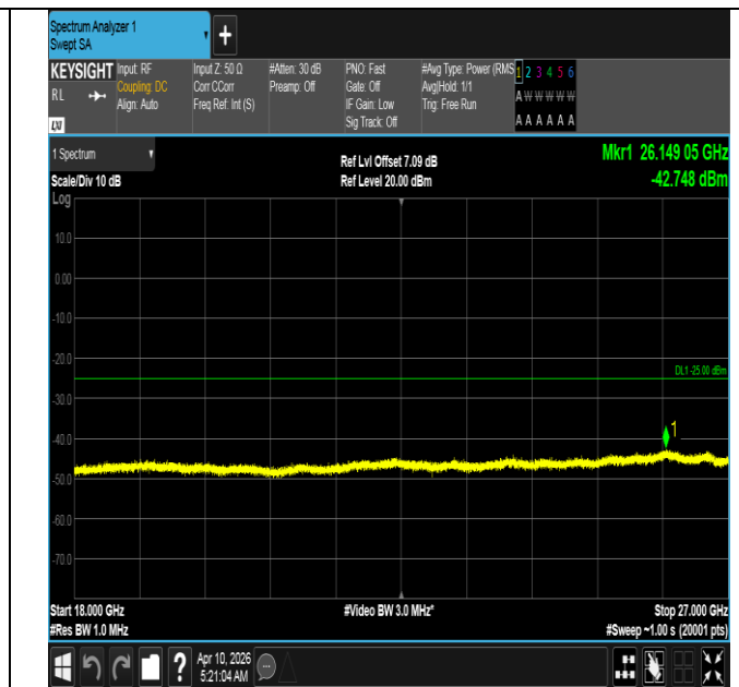
Band7-20MHz-16QAM-20850-1RB#0-18000~27000-PASS
