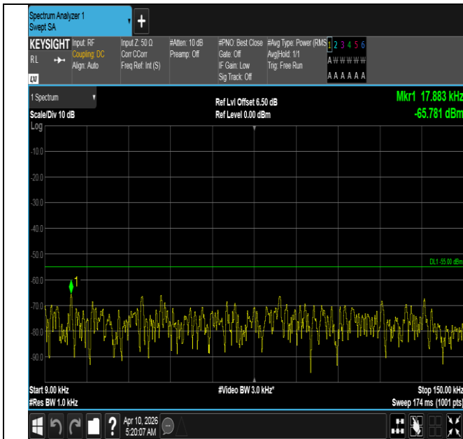
Band7-20MHz-16QAM-20850-1RB#0-0.009~0.15-PASS
