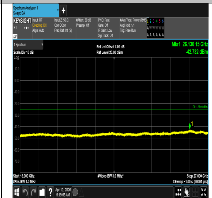
Band7-20MHz-QPSK-20850-1RB#0-18000~27000-PASS
