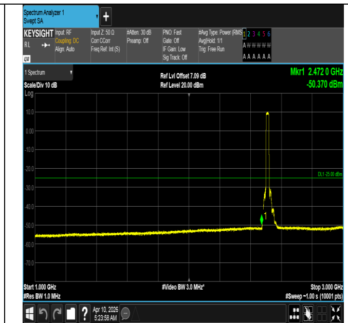
Band7-20MHz-QPSK-20850-100RB#0-1000~3000-PASS
