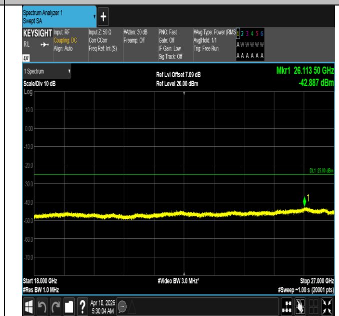
Band7-20MHz-16QAM-21100-1RB#99-18000~27000-PASS
