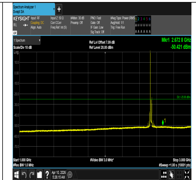
Band7-20MHz-QPSK-21100-1RB#0-1000~3000-PASS
