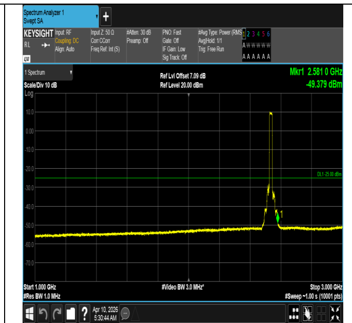
Band7-20MHz-QPSK-21100-100RB#0-1000~3000-PASS
