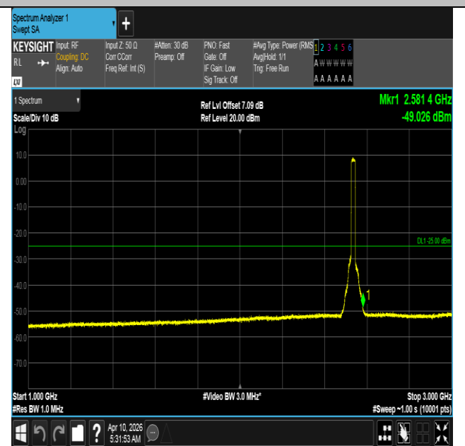
Band7-20MHz-16QAM-21100-100RB#0-1000~3000-PASS
