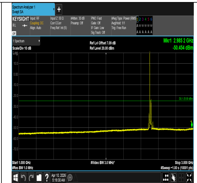
Band7-20MHz-QPSK-20850-1RB#0-1000~3000-PASS
