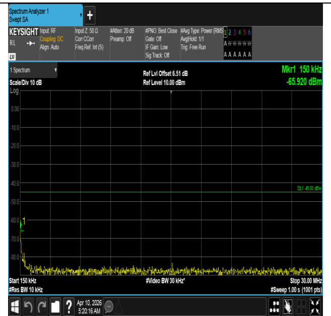
Band7-20MHz-16QAM-20850-1RB#0-0.15~30-PASS
