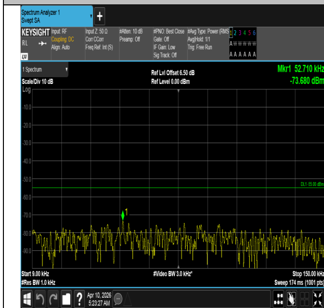
Band7-20MHz-QPSK-20850-100RB#0-0.009~0.15-PASS
