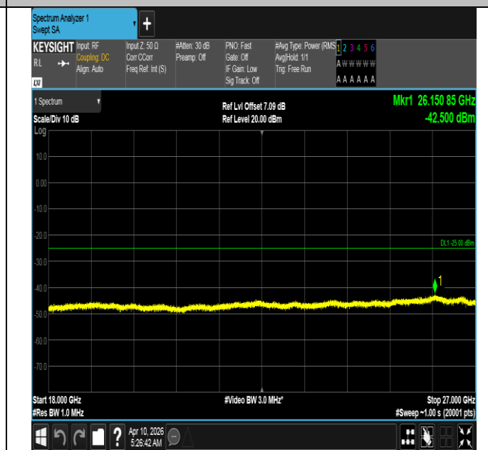
Band7-20MHz-QPSK-21100-1RB#0-18000~27000-PASS
