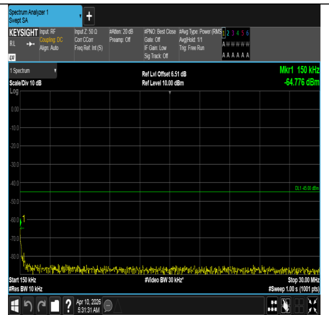
Band7-20MHz-16QAM-21100-100RB#0-0.15~30-PASS
