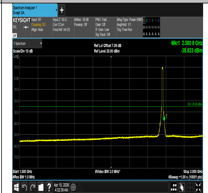
Band7-15MHz-16QAM-21375-75RB#0-1000~3000-PASS
