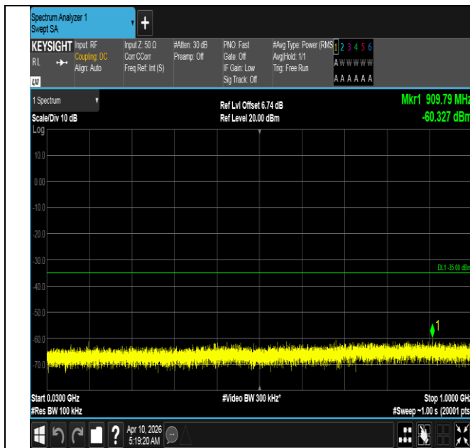
Band7-20MHz-QPSK-20850-1RB#0-30~1000-PASS
