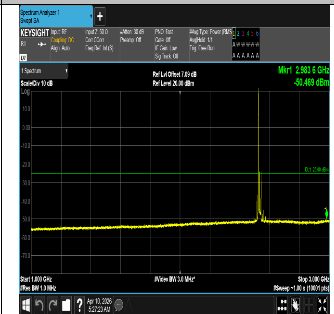
Band7-20MHz-16QAM-21100-1RB#0-1000~3000-PASS
