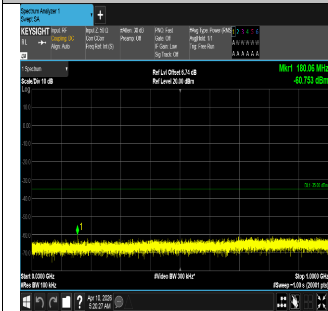
Band7-20MHz-16QAM-20850-1RB#0-30~1000-PASS
