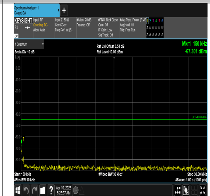
Band7-20MHz-QPSK-20850-100RB#0-0.15~30-PASS
