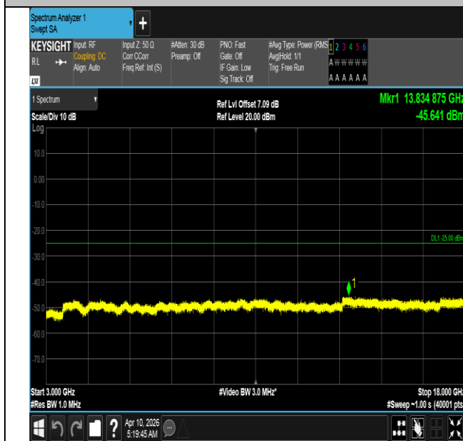
Band7-20MHz-QPSK-20850-1RB#0-3000~18000-PASS
