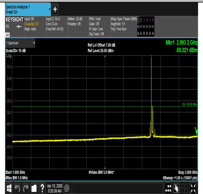
Band7-20MHz-16QAM-20850-1RB#0-1000~3000-PASS
