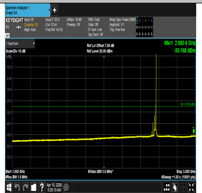
Band7-20MHz-QPSK-21350-1RB#99-1000~3000-PASS
