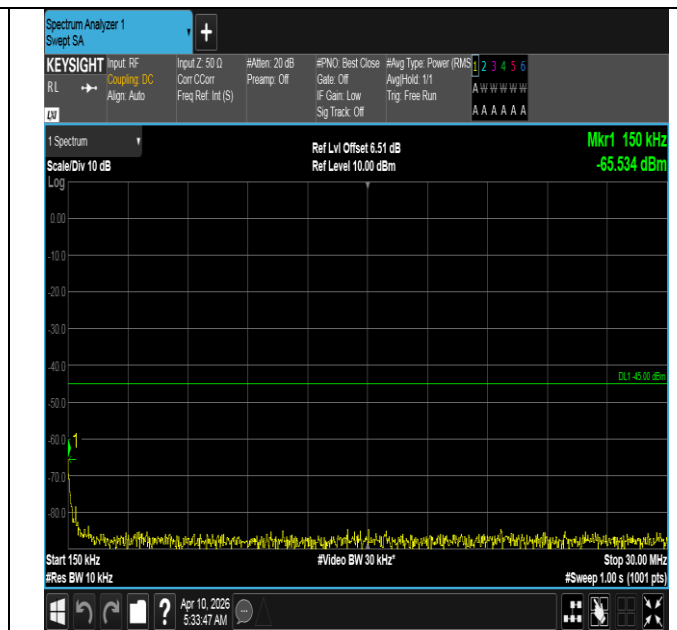
Band7-20MHz-16QAM-21350-1RB#0-0.15~30-PASS
