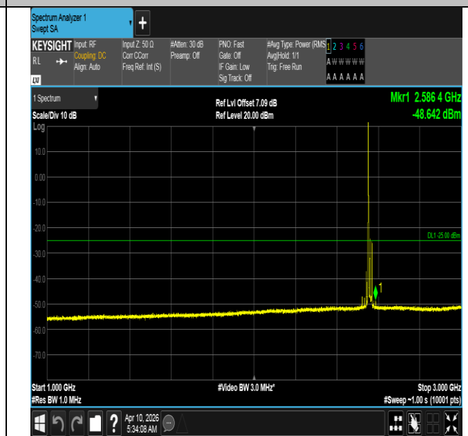
Band7-20MHz-16QAM-21350-1RB#0-1000~3000-PASS
