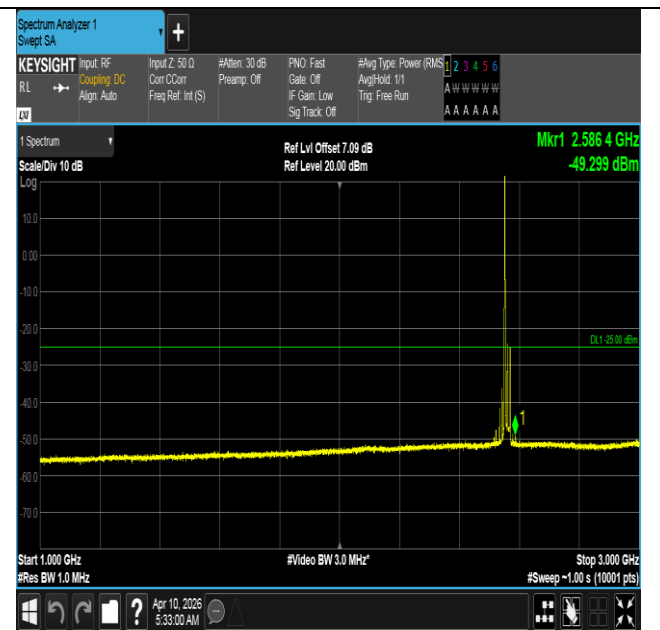
Band7-20MHz-QPSK-21350-1RB#0-1000~3000-PASS
