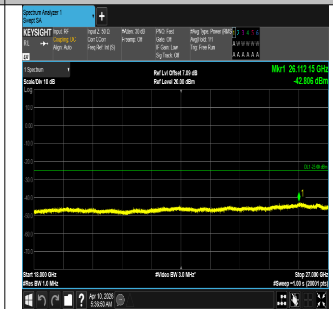
Band7-20MHz-16QAM-21350-1RB#99-18000~27000-PASS
