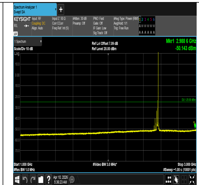
Band7-20MHz-16QAM-21350-1RB#99-1000~3000-PASS
