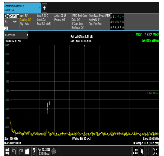
Band7-20MHz-QPSK-21350-1RB#99-0.15~30-PASS
