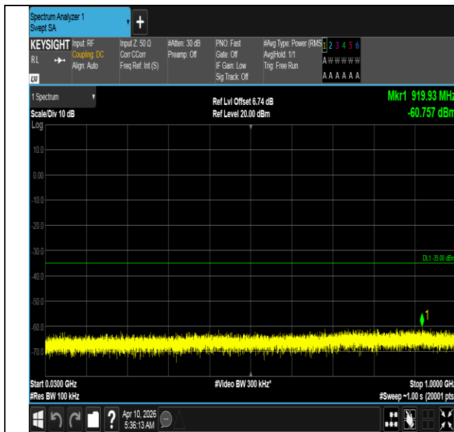
Band7-20MHz-16QAM-21350-1RB#99-30~1000-PASS
