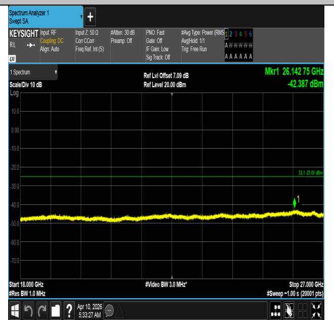
Band7-20MHz-QPSK-21350-1RB#0-18000~27000-PASS
