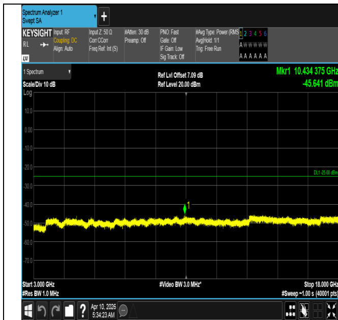
Band7-20MHz-16QAM-21350-1RB#0-3000~18000-PASS
