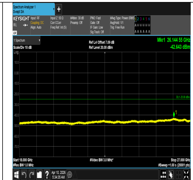
Band7-20MHz-16QAM-21350-1RB#0-18000~27000-PASS
