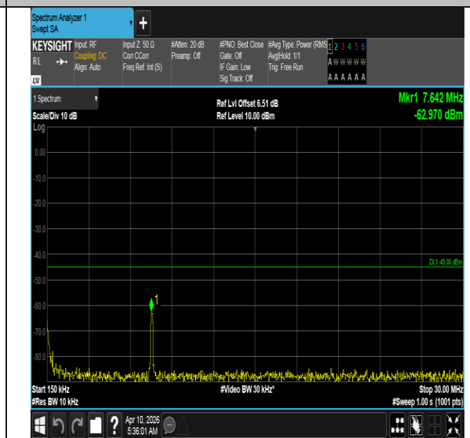
Band7-20MHz-16QAM-21350-1RB#99-0.15~30-PASS
