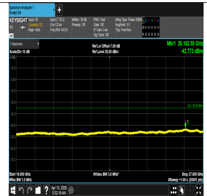
Band7-20MHz-16QAM-21100-100RB#0-18000~27000-PASS
