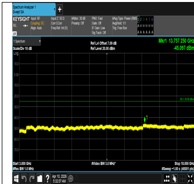
Band7-20MHz-16QAM-21100-100RB#0-3000~18000-PASS
