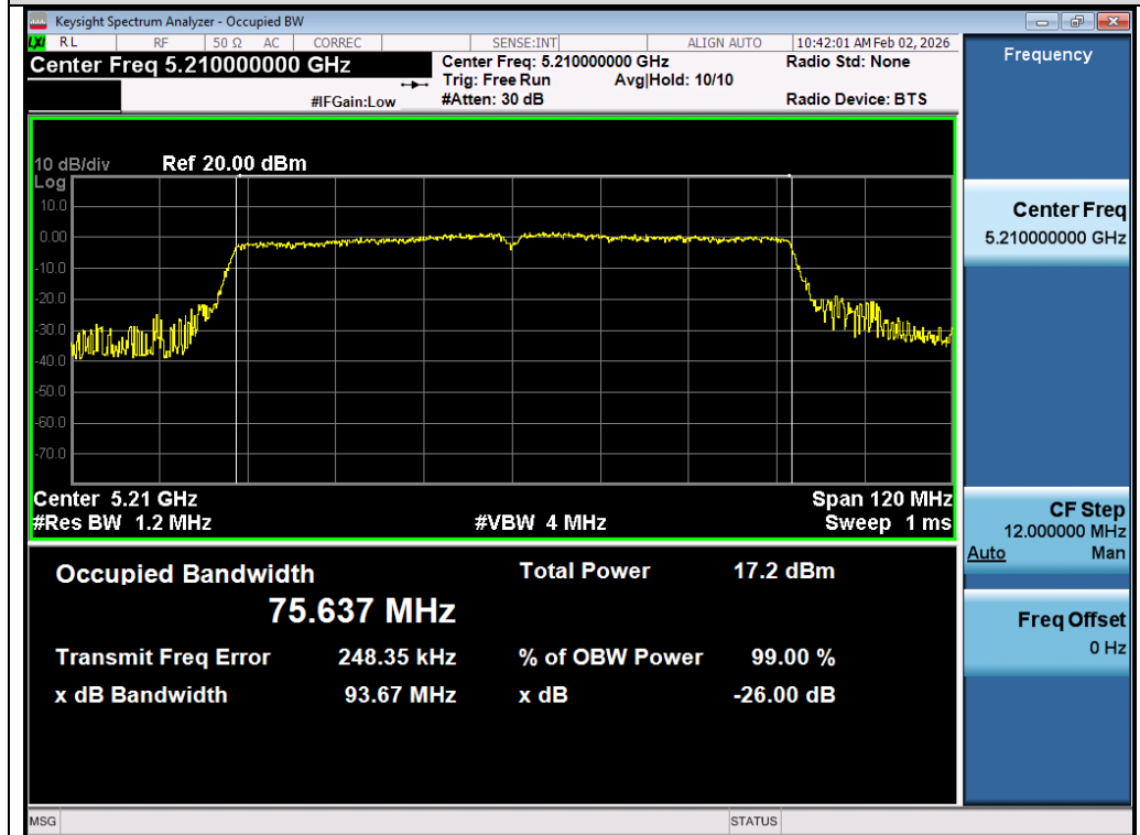
Test_Graph_802.11ac80_Chain A_5210_MCS0_OBW
