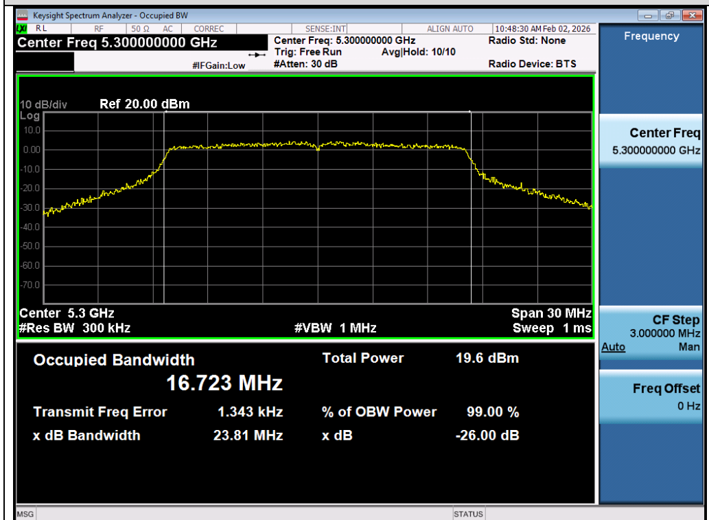
Test_Graph_802.11a_Chain A_5300_6Mbps_OBW
