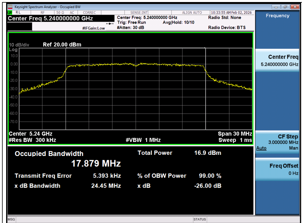
Test_Graph_802.11ac20_Chain A_5240_MCS0_OBW
