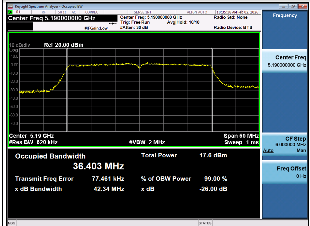
Test_Graph_802.11ac40_Chain A_5190_MCS0_OBW
