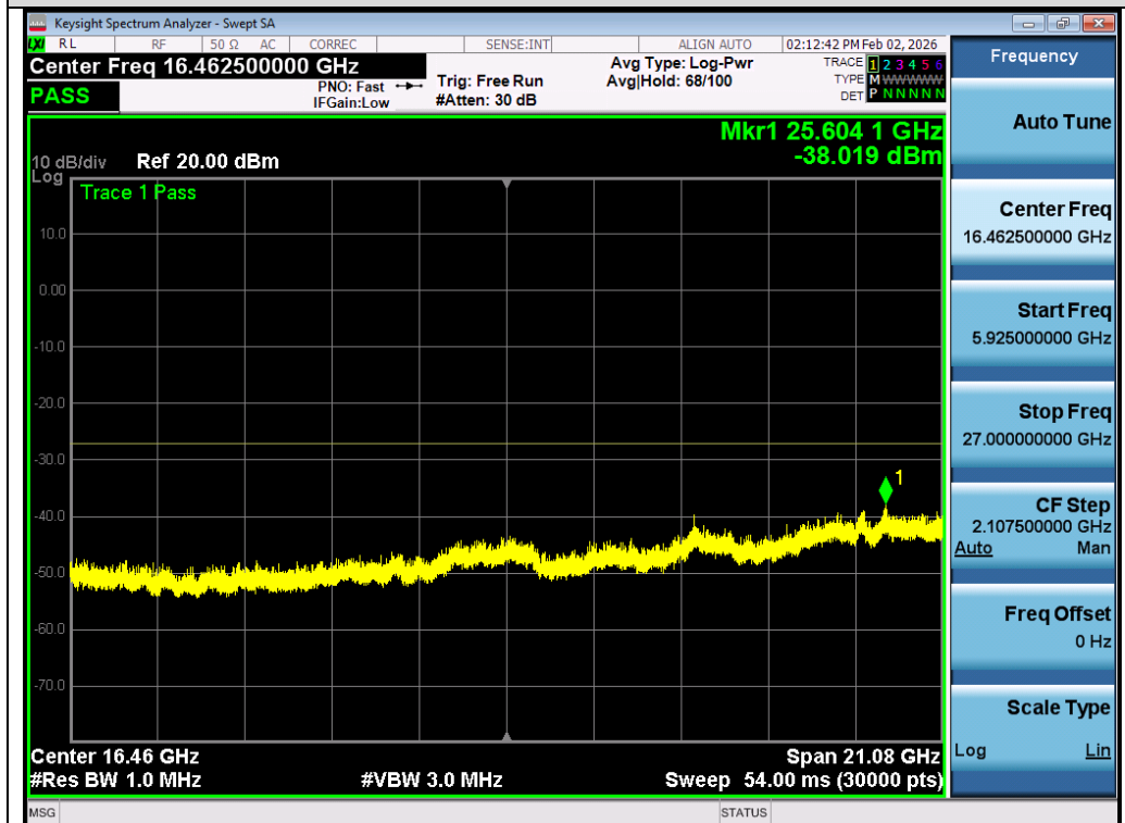
Test_Graph_802.11a_Chain A_5825_6Mbps_Frequency Band4
