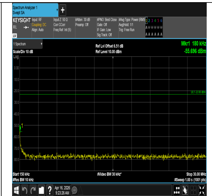
Band12-1.4MHz-QPSK-23017-6RB#0-0.15~30-PASS
