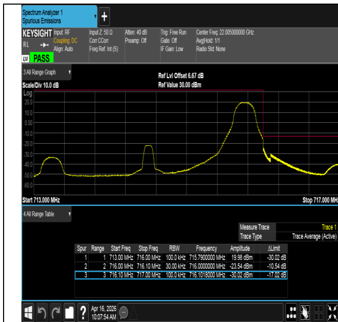
Band12-3MHz-16QAM-23165-1RB#14-PASS
