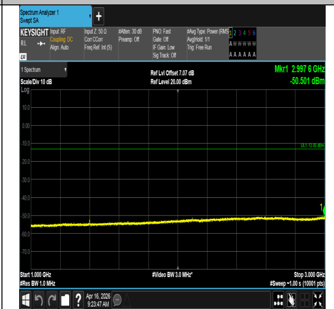
Band12-1.4MHz-QPSK-23017-6RB#0-1000~3000-PASS
