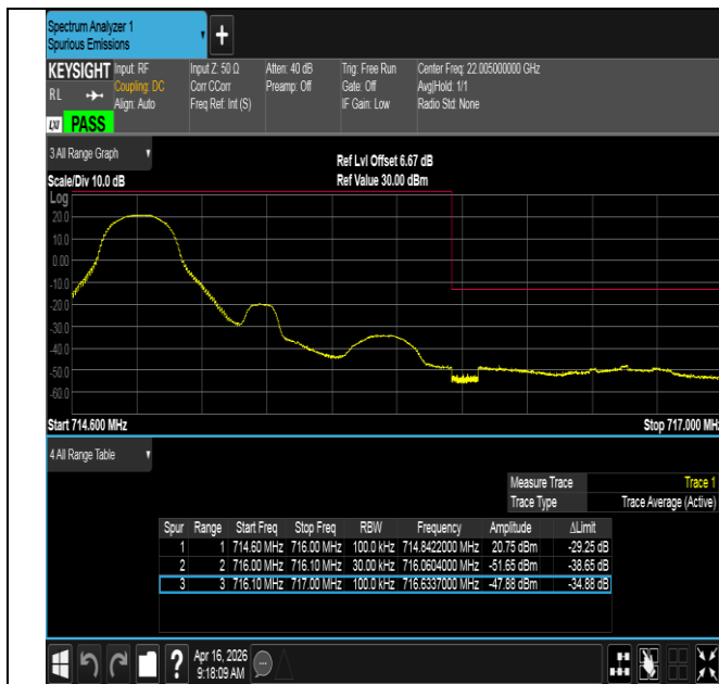
Band12-1.4MHz-QPSK-23173-1RB#0-PASS
