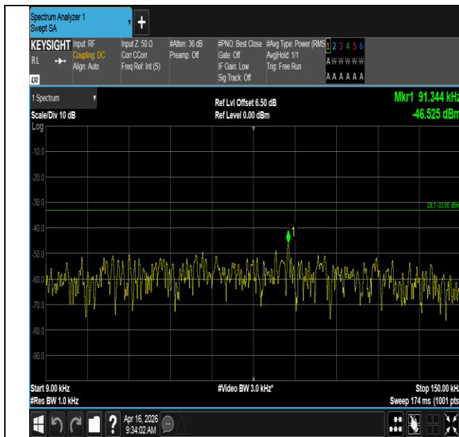
Band12-1.4MHz-QPSK-23173-6RB#0-0.009~0.15-PASS
