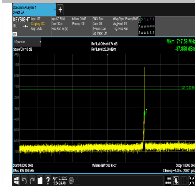
Band12-1.4MHz-QPSK-23173-6RB#0-30~1000-PASS
