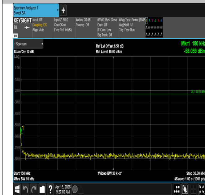
Band12-1.4MHz-QPSK-23095-1RB#5-0.15~30-PASS
