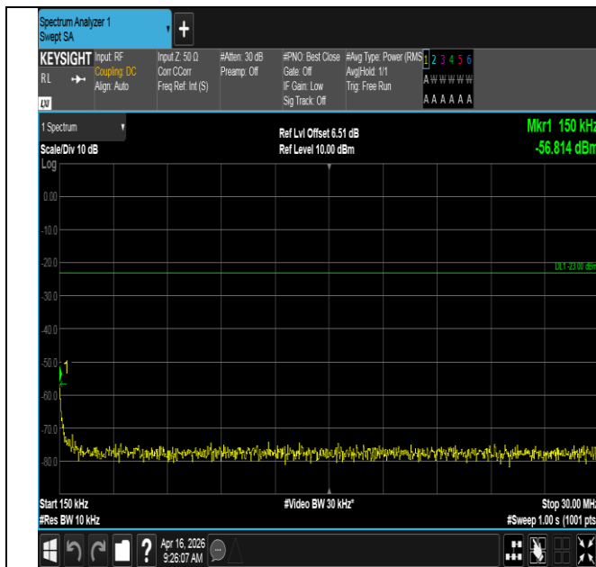
Band12-1.4MHz-16QAM-23095-1RB#0-0.15~30-PASS
