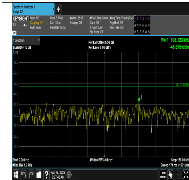
Band12-1.4MHz-16QAM-23095-1RB#5-0.009~0.15-PASS
