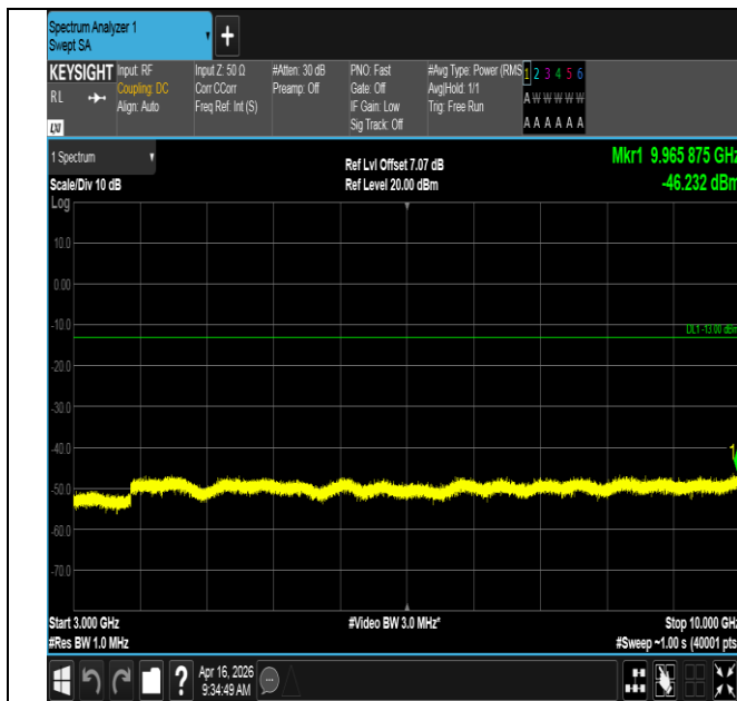
Band12-1.4MHz-QPSK-23173-6RB#0-3000~10000-PASS
