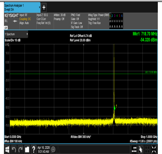
Band12-1.4MHz-16QAM-23173-1RB#0-30~1000-PASS
