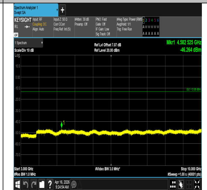
Band12-1.4MHz-16QAM-23017-6RB#0-3000~10000-PASS
