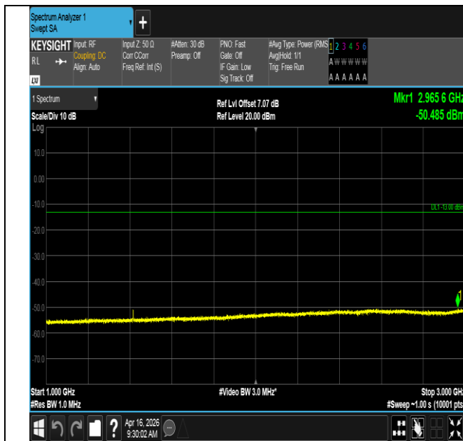
Band12-1.4MHz-16QAM-23095-6RB#0-1000~3000-PASS
