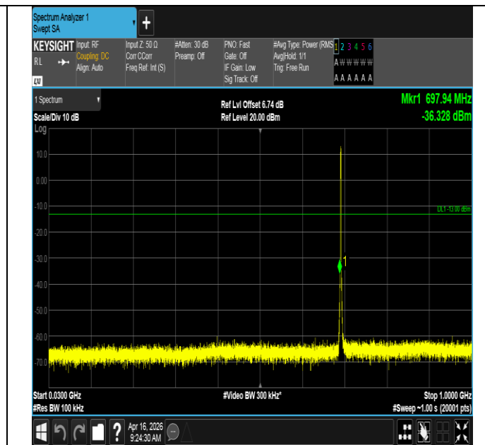
Band12-1.4MHz-16QAM-23017-6RB#0-30~1000-PASS
