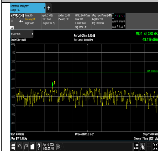
Band12-1.4MHz-QPSK-23173-1RB#0-0.009~0.15-PASS
