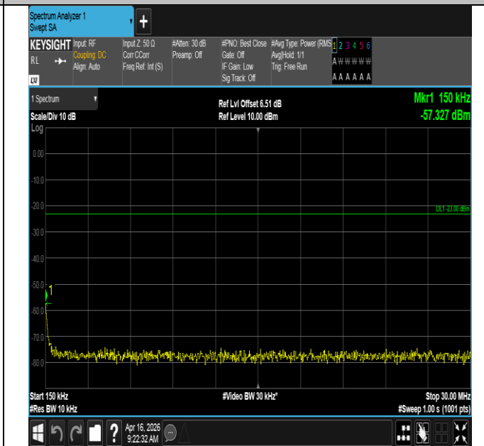
Band12-1.4MHz-16QAM-23017-1RB#5-0.15~30-PASS
