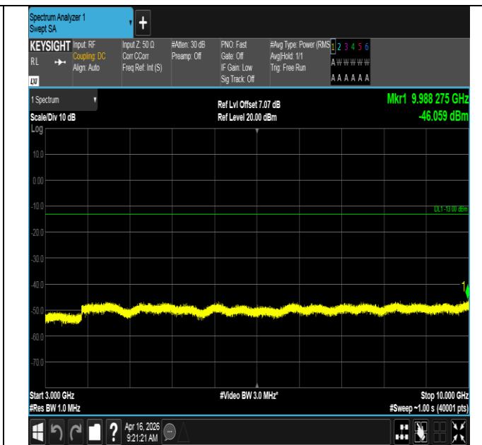
Band12-1.4MHz-16QAM-23017-1RB#0-3000~10000-PASS
