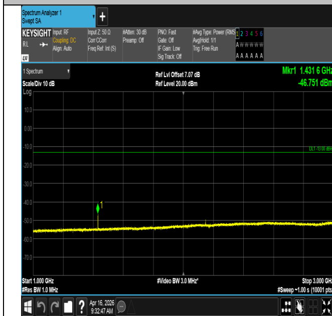
Band12-1.4MHz-QPSK-23173-1RB#5-1000~3000-PASS
