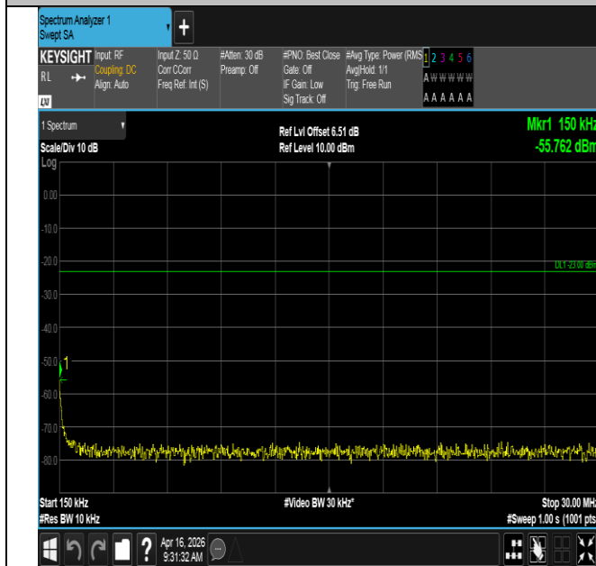
Band12-1.4MHz-16QAM-23173-1RB#0-0.15~30-PASS
