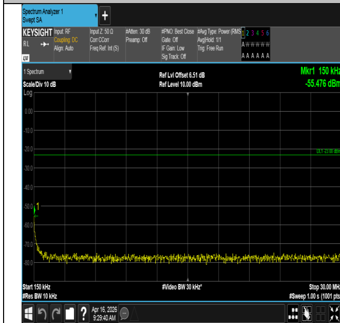
Band12-1.4MHz-16QAM-23095-6RB#0-0.15~30-PASS
