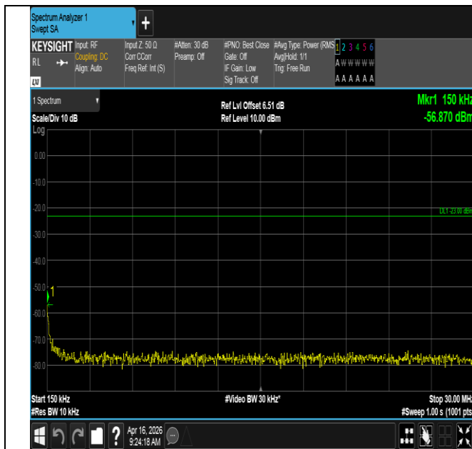
Band12-1.4MHz-16QAM-23017-6RB#0-0.15~30-PASS
