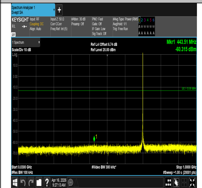
Band12-1.4MHz-QPSK-23095-1RB#5-30~1000-PASS
