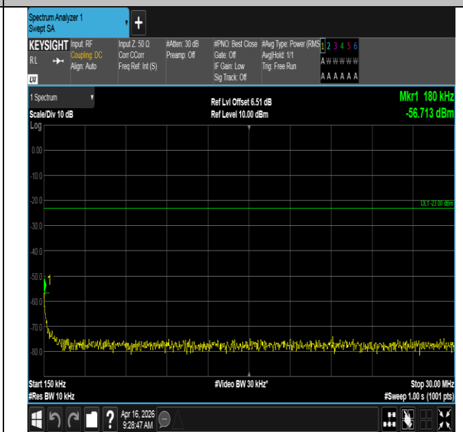
Band12-1.4MHz-QPSK-23095-6RB#0-0.15~30-PASS
