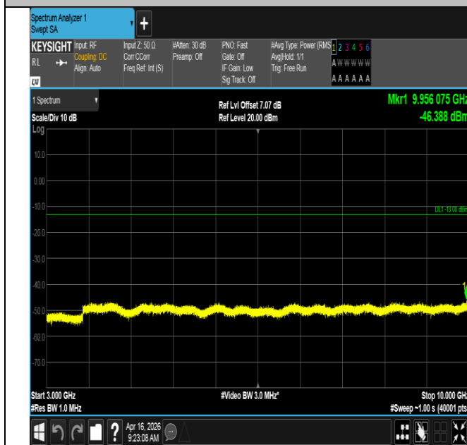
Band12-1.4MHz-16QAM-23017-1RB#5-3000~10000-PASS
