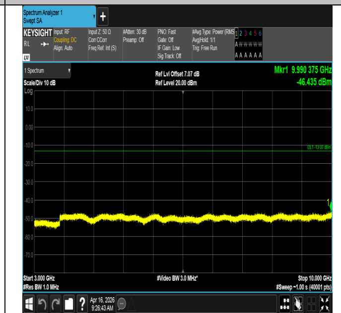
Band12-1.4MHz-16QAM-23095-1RB#0-3000~10000-PASS
