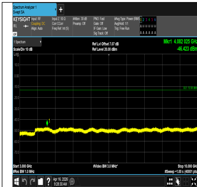
Band12-1.4MHz-16QAM-23095-1RB#5-3000~10000-PASS
