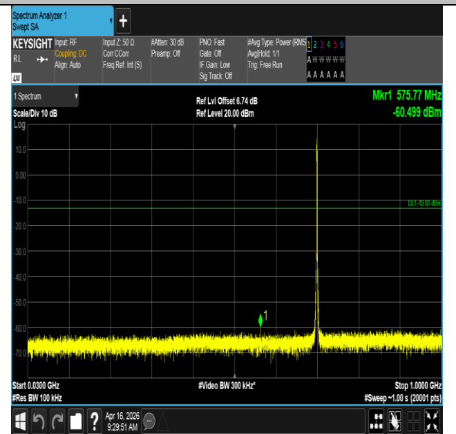
Band12-1.4MHz-16QAM-23095-6RB#0-30~1000-PASS
