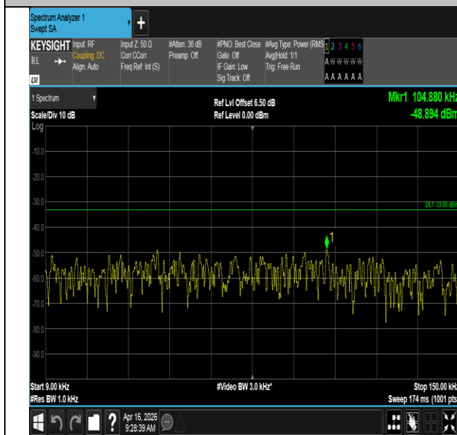
Band12-1.4MHz-QPSK-23095-6RB#0-0.009~0.15-PASS
