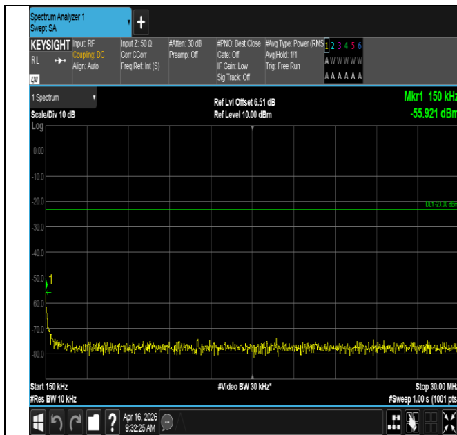
Band12-1.4MHz-QPSK-23173-1RB#5-0.15~30-PASS
