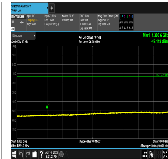
Band12-1.4MHz-16QAM-23017-1RB#0-1000~3000-PASS
