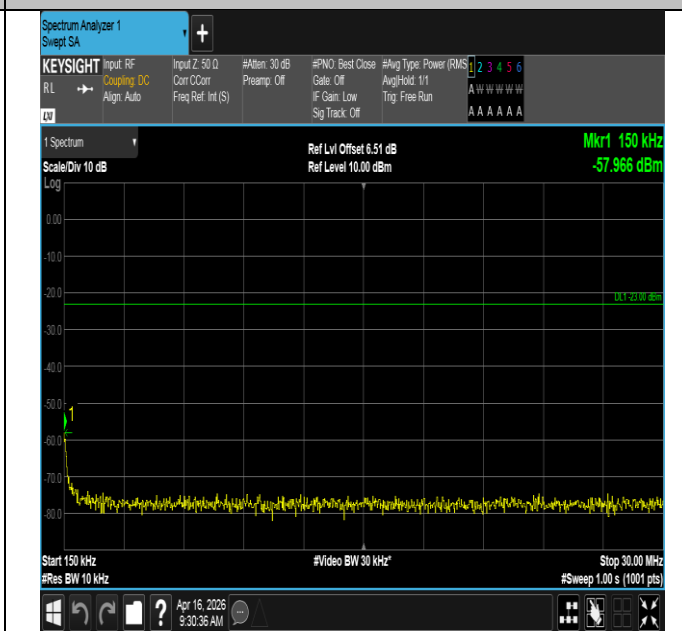
Band12-1.4MHz-QPSK-23173-1RB#0-0.15~30-PASS
