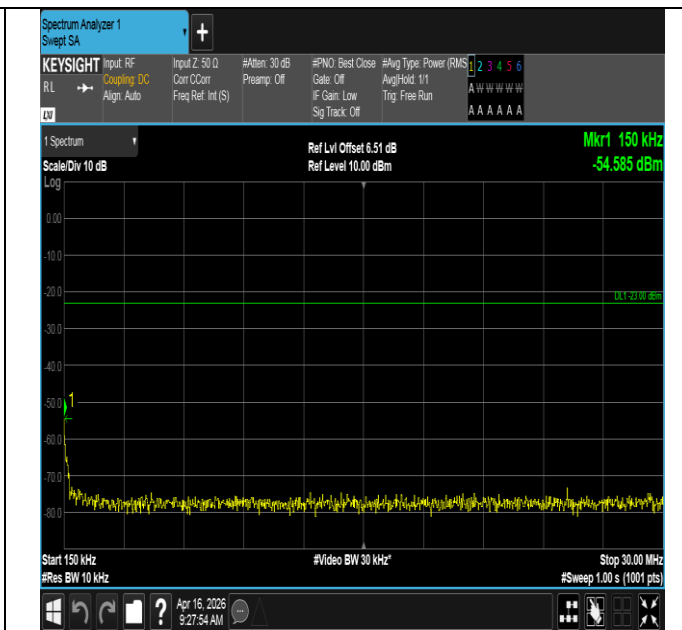
Band12-1.4MHz-16QAM-23095-1RB#5-0.15~30-PASS
