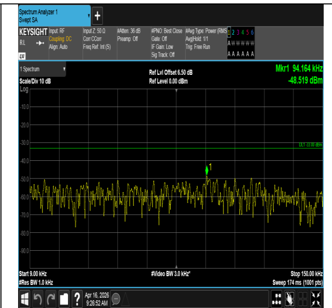
Band12-1.4MHz-QPSK-23095-1RB#5-0.009~0.15-PASS
