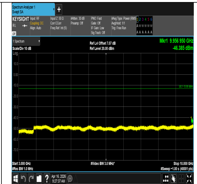
Band12-1.4MHz-QPSK-23095-1RB#5-3000~10000-PASS
