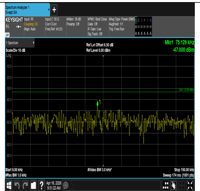
Band12-1.4MHz-16QAM-23173-1RB#0-0.009~0.15-PASS
