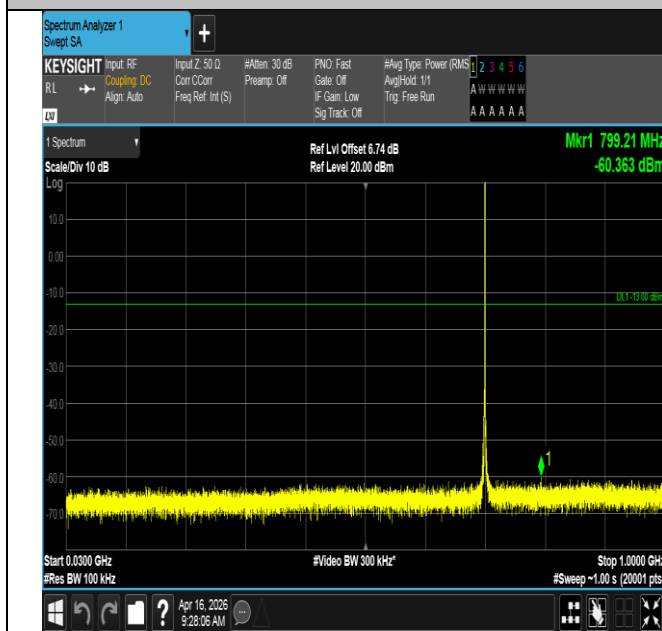
Band12-1.4MHz-16QAM-23095-1RB#5-30~1000-PASS
