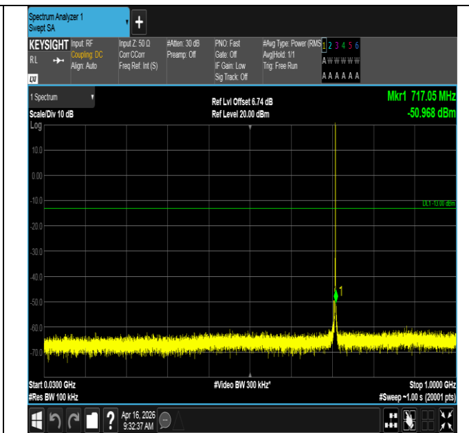
Band12-1.4MHz-QPSK-23173-1RB#5-30~1000-PASS
