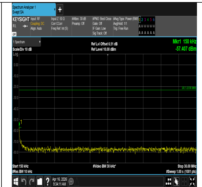
Band12-1.4MHz-QPSK-23173-6RB#0-0.15~30-PASS
