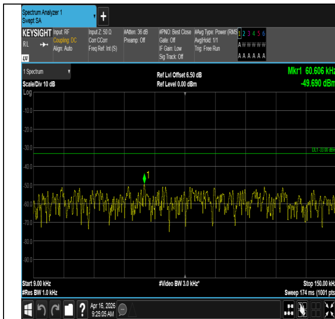
Band12-1.4MHz-QPSK-23095-1RB#0-0.009~0.15-PASS
