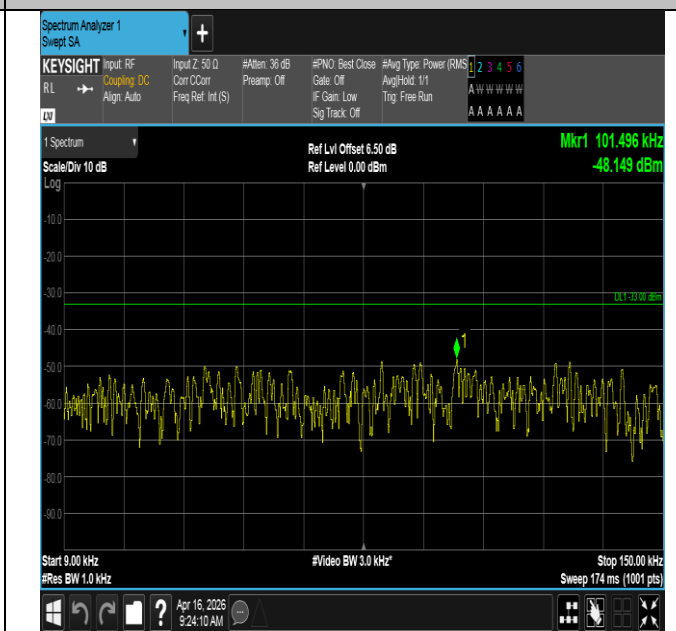
Band12-1.4MHz-16QAM-23017-6RB#0-0.009~0.15-PASS
