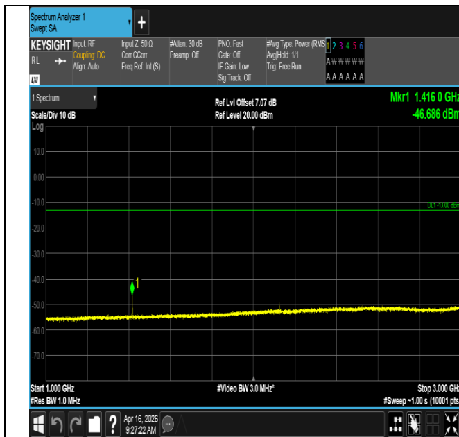
Band12-1.4MHz-QPSK-23095-1RB#5-1000~3000-PASS
