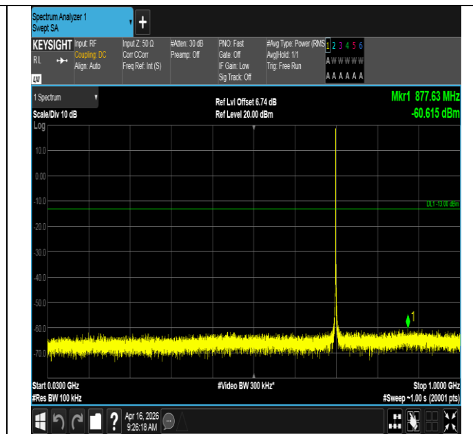
Band12-1.4MHz-16QAM-23095-1RB#0-30~1000-PASS
