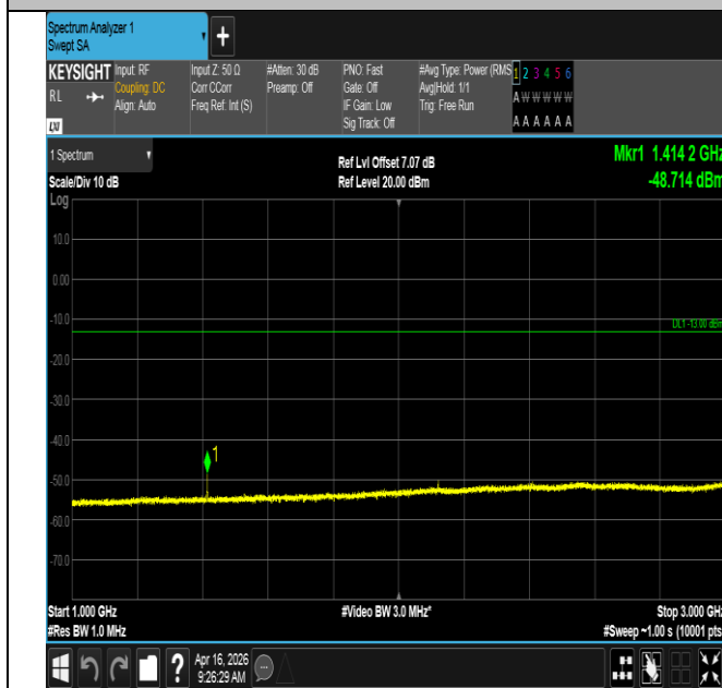
Band12-1.4MHz-16QAM-23095-1RB#0-1000~3000-PASS
