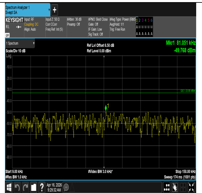
Band12-1.4MHz-16QAM-23095-6RB#0-0.009~0.15-PASS
