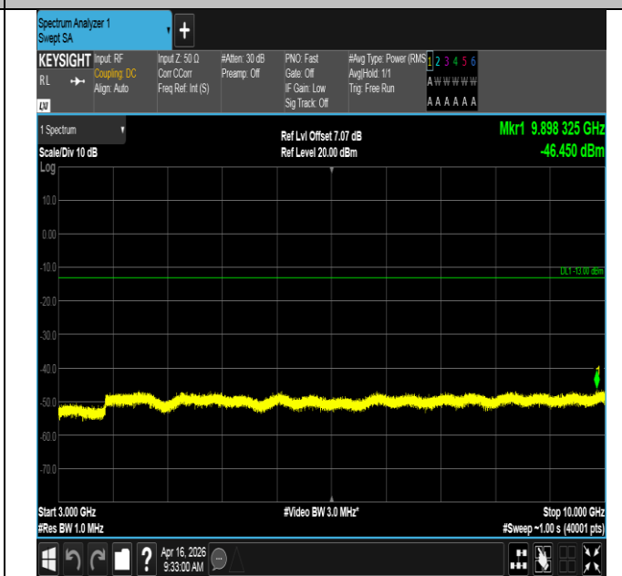
Band12-1.4MHz-QPSK-23173-1RB#5-3000~10000-PASS
