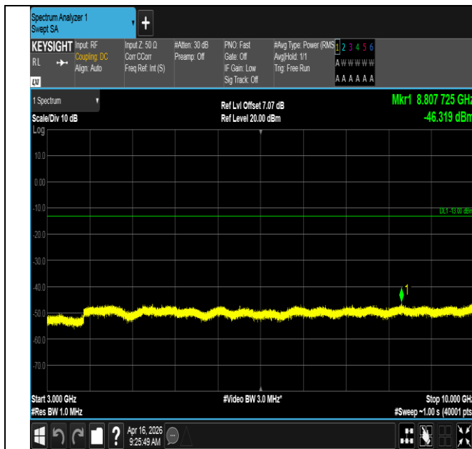
Band12-1.4MHz-QPSK-23095-1RB#0-3000~10000-PASS
