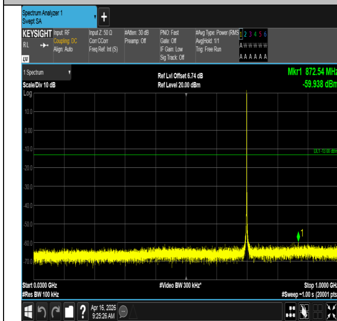
Band12-1.4MHz-QPSK-23095-1RB#0-30~1000-PASS
