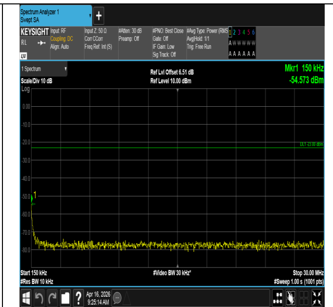
Band12-1.4MHz-QPSK-23095-1RB#0-0.15~30-PASS
