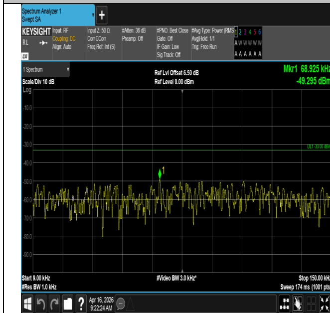
Band12-1.4MHz-16QAM-23017-1RB#5-0.009~0.15-PASS
