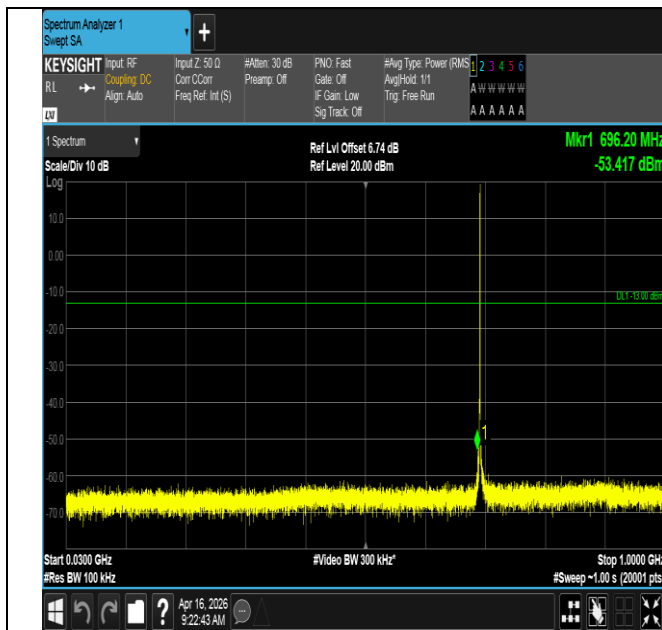
Band12-1.4MHz-16QAM-23017-1RB#5-30~1000-PASS
