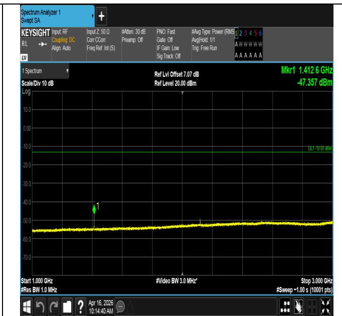
Band12-3MHz-QPSK-23095-1RB#0-1000~3000-PASS
