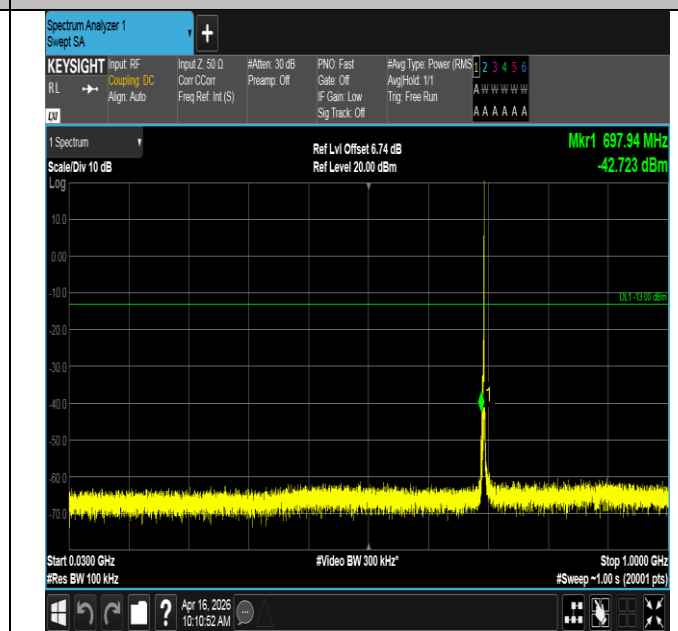
Band12-3MHz-QPSK-23025-1RB#14-30~1000-PASS
