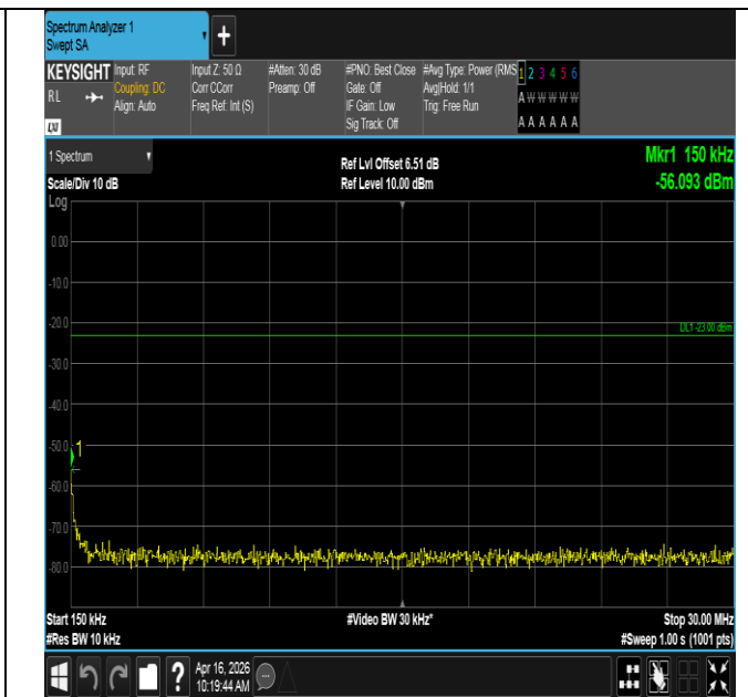
Band12-3MHz-QPSK-23165-1RB#0-0.15~30-PASS
