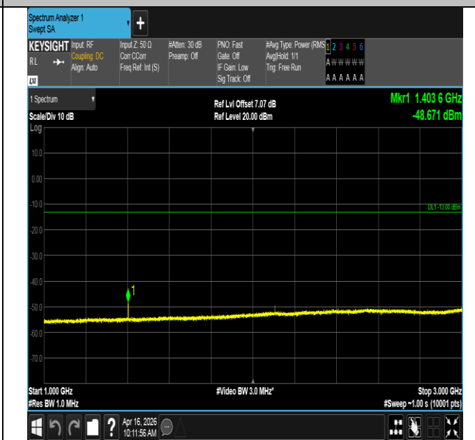
Band12-3MHz-16QAM-23025-1RB#14-1000~3000-PASS
