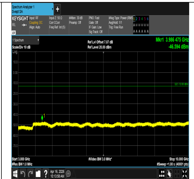
Band12-3MHz-16QAM-23025-15RB#0-3000~10000-PASS
