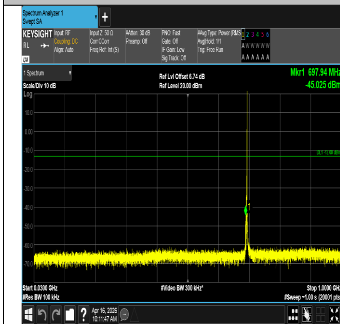
Band12-3MHz-16QAM-23025-1RB#14-30~1000-PASS
