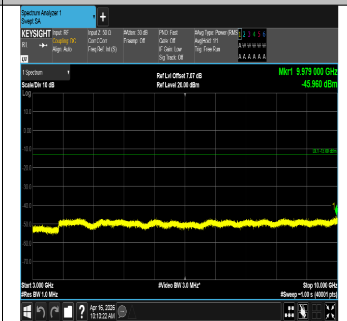
Band12-3MHz-16QAM-23025-1RB#0-3000~10000-PASS
