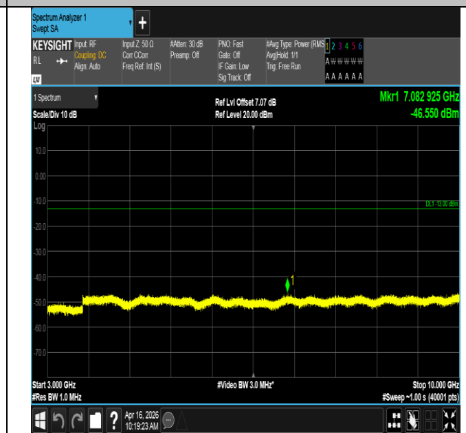
Band12-3MHz-16QAM-23095-15RB#0-3000~10000-PASS
