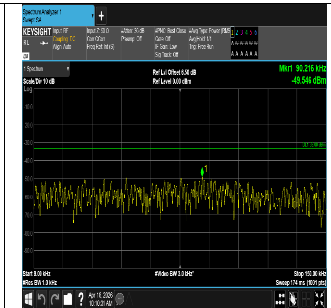
Band12-3MHz-QPSK-23025-1RB#14-0.009~0.15-PASS
