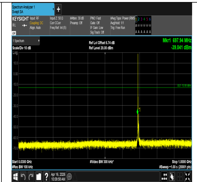
Band12-3MHz-16QAM-23025-1RB#0-30~1000-PASS
