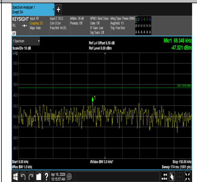
Band12-3MHz-QPSK-23095-1RB#14-0.009~0.15-PASS
