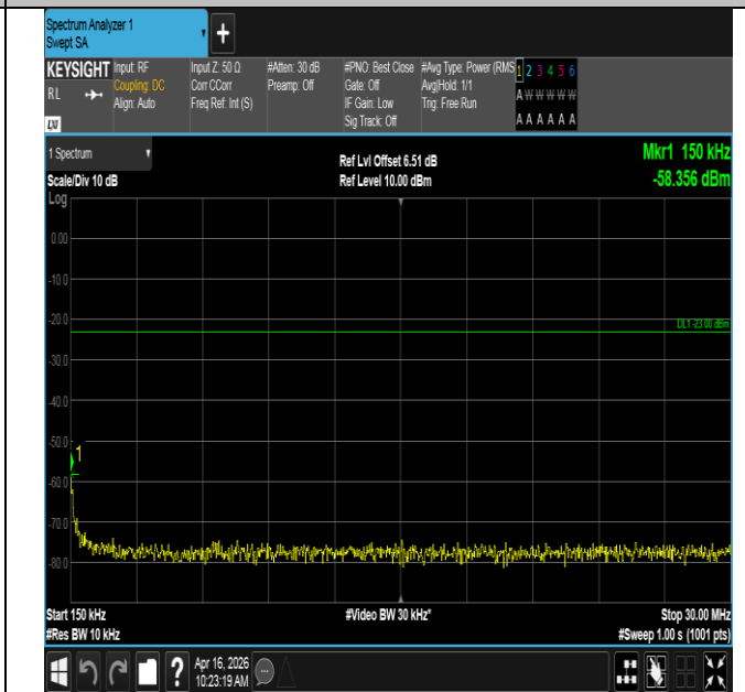
Band12-3MHz-QPSK-23165-15RB#0-0.15~30-PASS
