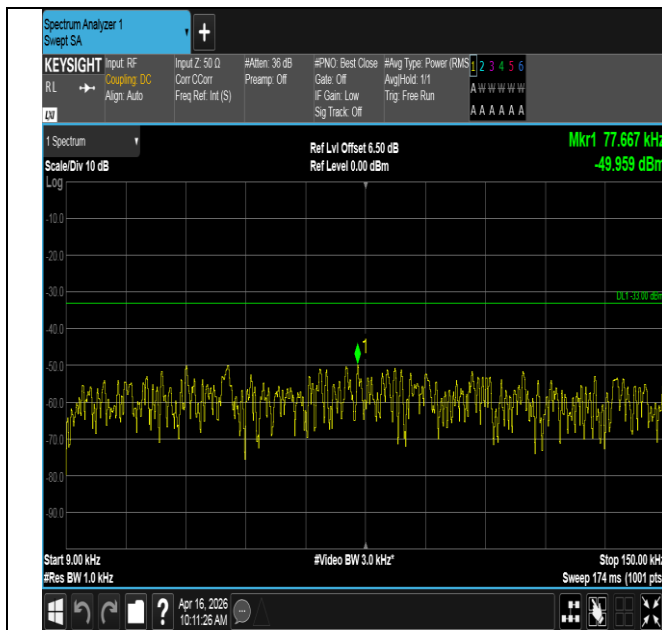
Band12-3MHz-16QAM-23025-1RB#14-0.009~0.15-PASS
