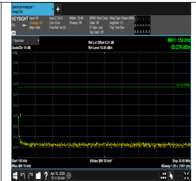
Band12-3MHz-16QAM-23025-1RB#14-0.15~30-PASS
