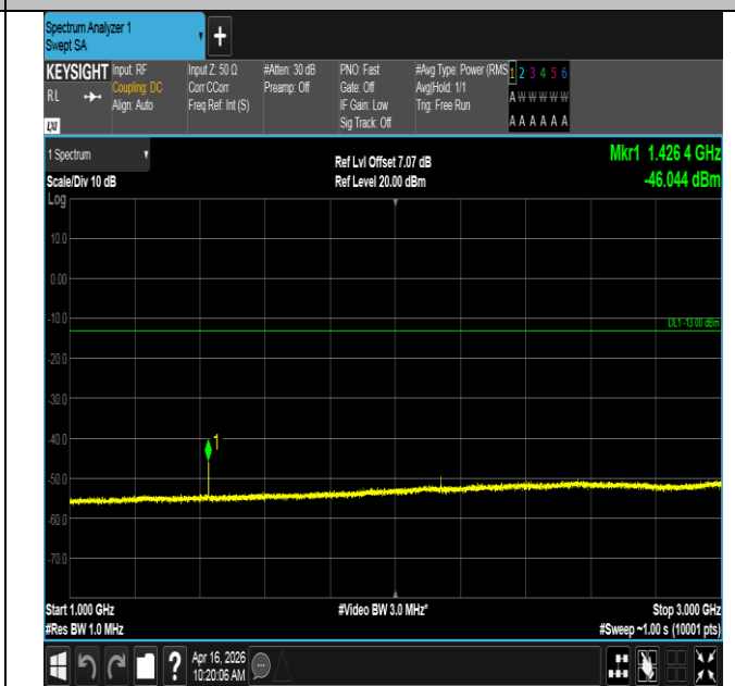
Band12-3MHz-QPSK-23165-1RB#0-1000~3000-PASS
