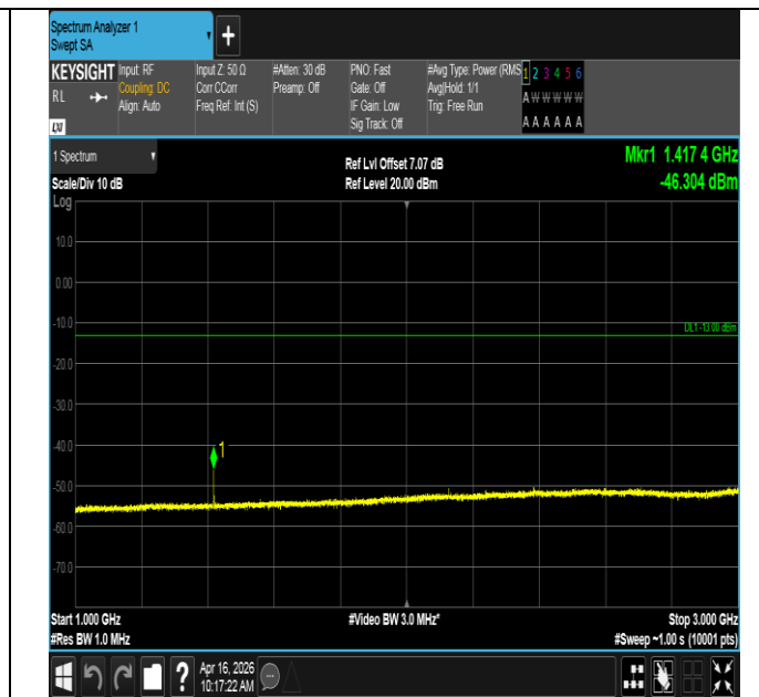
Band12-3MHz-16QAM-23095-1RB#14-1000~3000-PASS
