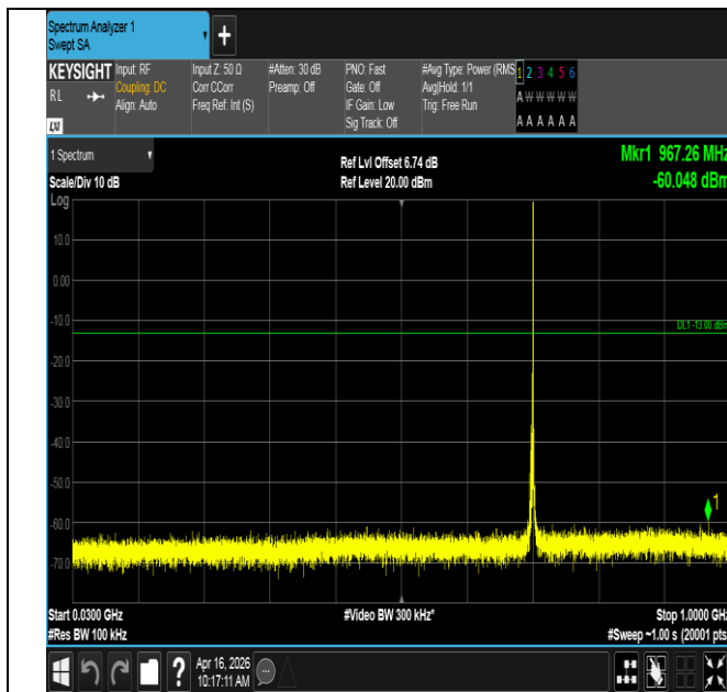
Band12-3MHz-16QAM-23095-1RB#14-30~1000-PASS
