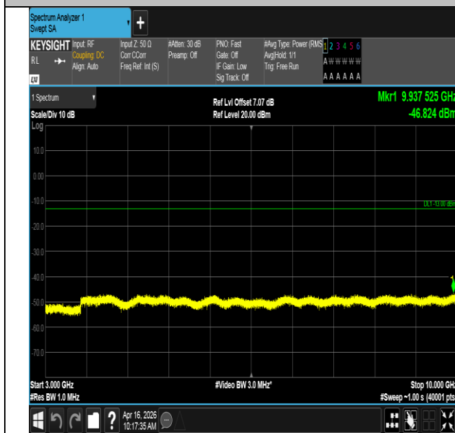
Band12-3MHz-16QAM-23095-1RB#14-3000~10000-PASS
