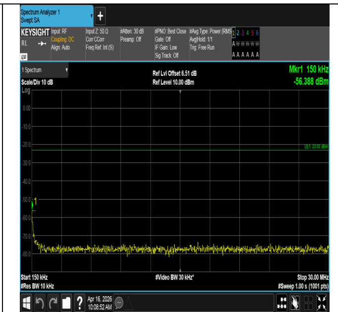
Band12-3MHz-QPSK-23025-1RB#0-0.15~30-PASS
