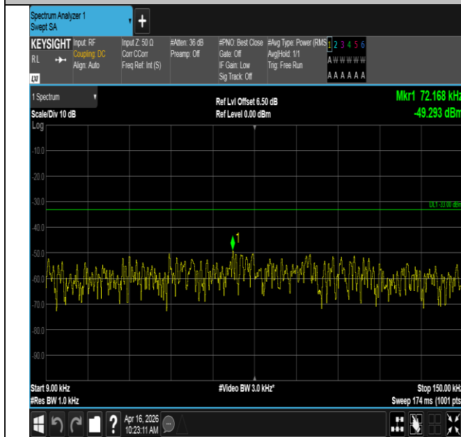
Band12-3MHz-QPSK-23165-15RB#0-0.009~0.15-PASS
