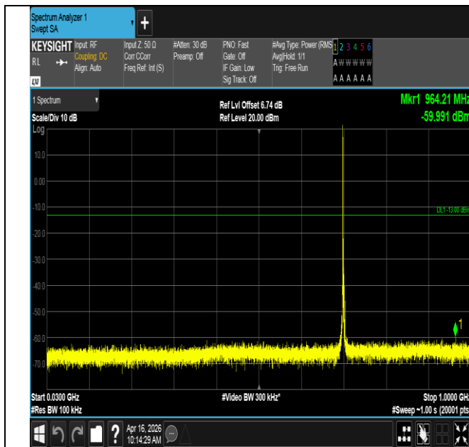
Band12-3MHz-QPSK-23095-1RB#0-30~1000-PASS
