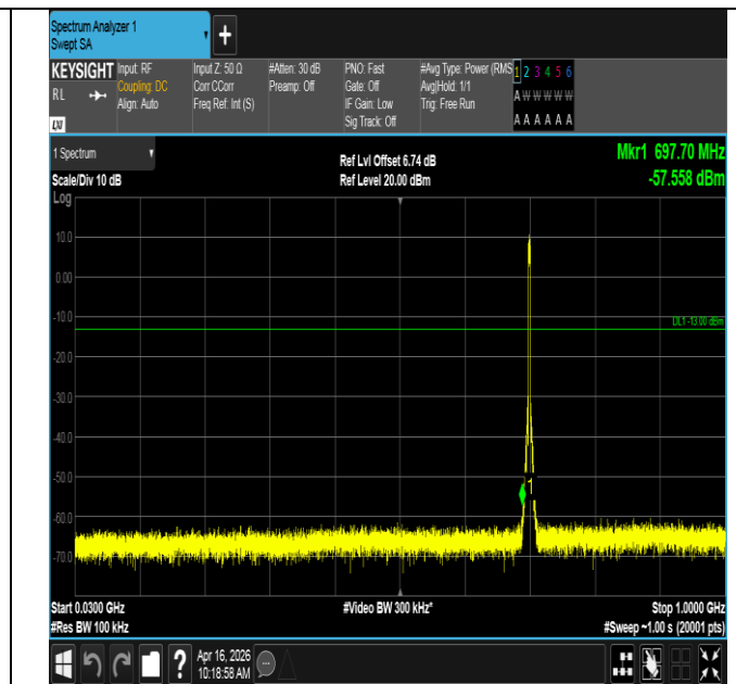
Band12-3MHz-16QAM-23095-15RB#0-30~1000-PASS
