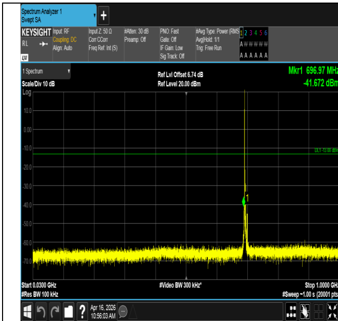
Band12-5MHz-QPSK-23035-1RB#0-30~1000-PASS
