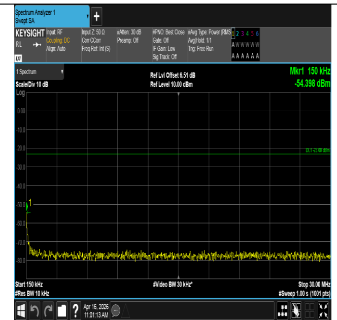
Band12-5MHz-QPSK-23095-1RB#0-0.15~30-PASS
