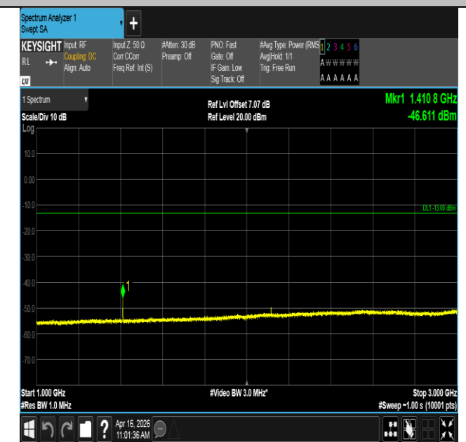
Band12-5MHz-QPSK-23095-1RB#0-1000~3000-PASS
