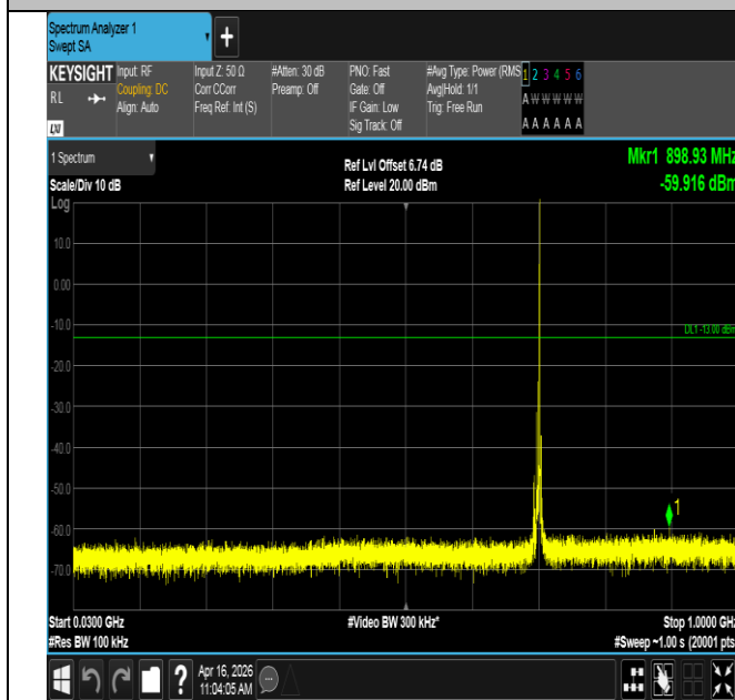
Band12-5MHz-16QAM-23095-1RB#24-30~1000-PASS
