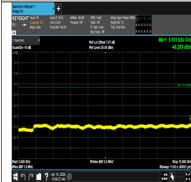
Band12-5MHz-QPSK-23035-1RB#0-3000~10000-PASS
