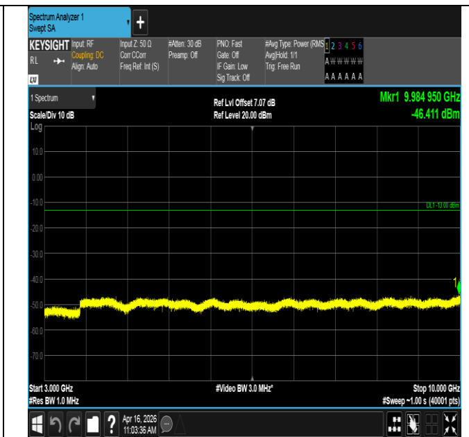
Band12-5MHz-QPSK-23095-1RB#24-3000~10000-PASS
