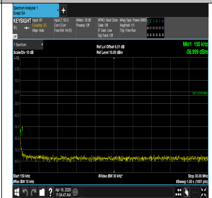
Band12-5MHz-QPSK-23095-25RB#0-0.15~30-PASS
