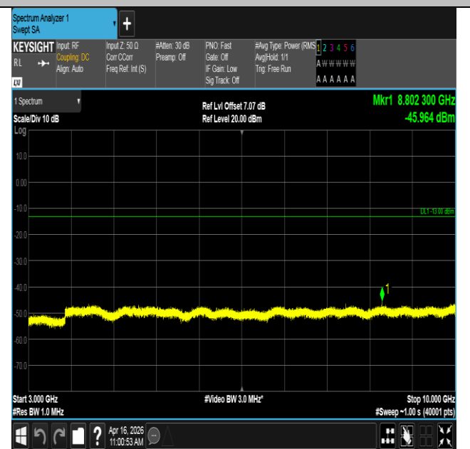
Band12-5MHz-16QAM-23035-25RB#0-3000~10000-PASS
