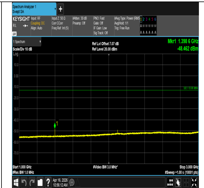
Band12-5MHz-QPSK-23035-1RB#0-1000~3000-PASS
