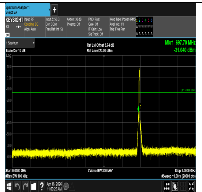
Band12-5MHz-16QAM-23035-25RB#0-30~1000-PASS
