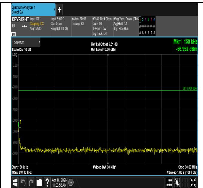
Band12-5MHz-16QAM-23095-1RB#24-0.15~30-PASS
