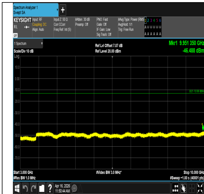
Band12-10MHz-QPSK-23095-50RB#0-3000~10000-PASS
