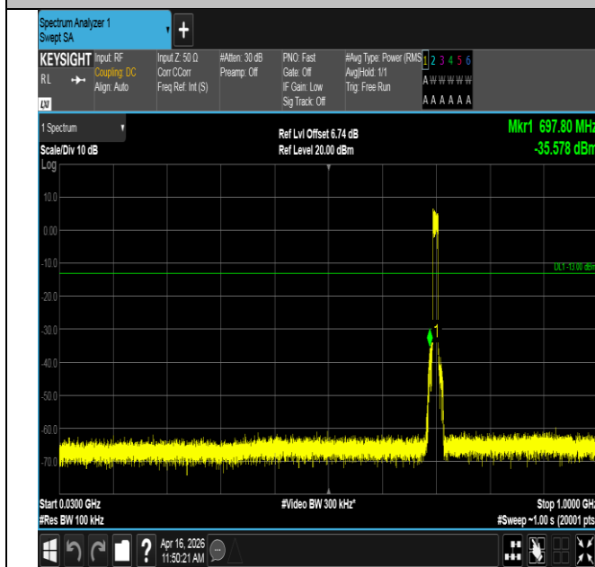
Band12-10MHz-QPSK-23095-50RB#0-30~1000-PASS
