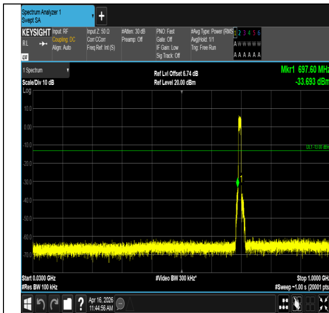
Band12-10MHz-QPSK-23060-50RB#0-30~1000-PASS
