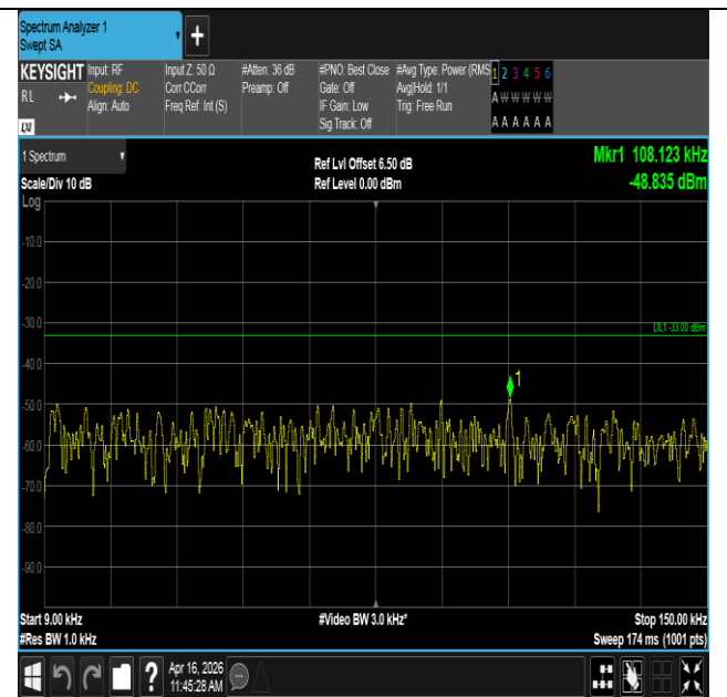
Band12-10MHz-16QAM-23060-50RB#0-0.009~0.15-PASS
