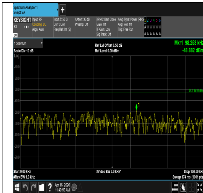
Band12-10MHz-QPSK-23060-1RB#0-0.009~0.15-PASS
