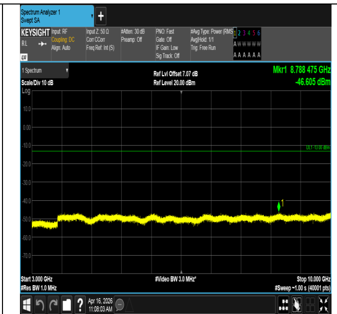
Band12-5MHz-16QAM-23155-1RB#0-3000~10000-PASS
