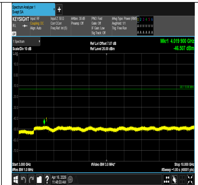
Band12-10MHz-16QAM-23095-1RB#0-3000~10000-PASS
