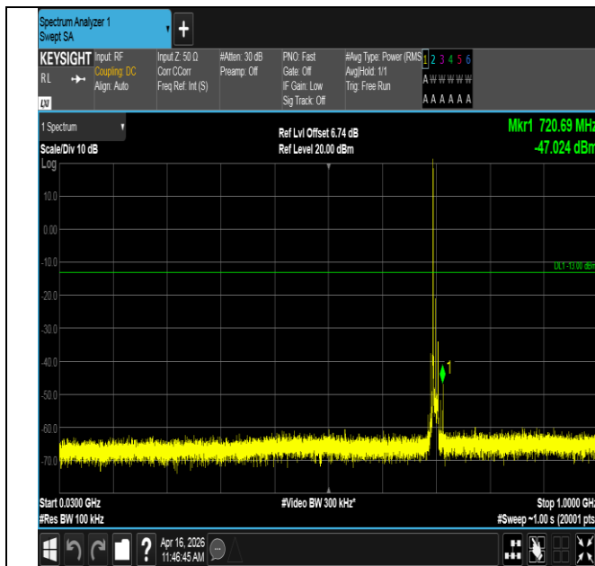
Band12-10MHz-QPSK-23095-1RB#0-30~1000-PASS
