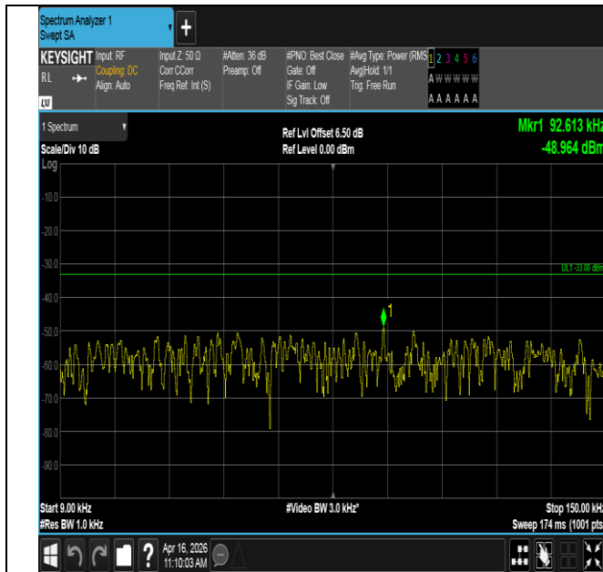
Band12-5MHz-QPSK-23155-25RB#0-0.009~0.15-PASS
