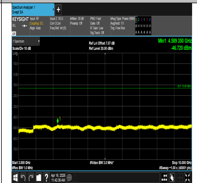
Band12-10MHz-16QAM-23060-1RB#0-3000~10000-PASS
