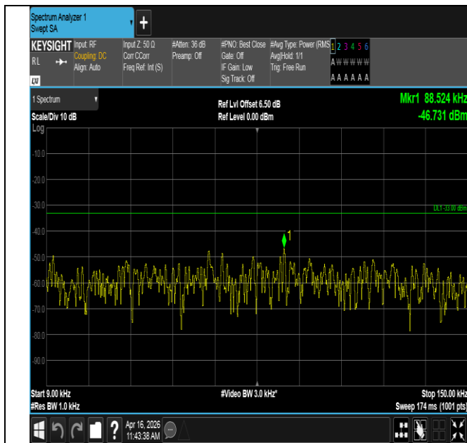
Band12-10MHz-16QAM-23060-1RB#49-0.009~0.15-PASS
