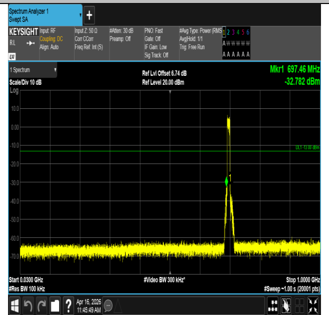
Band12-10MHz-16QAM-23060-50RB#0-30~1000-PASS
