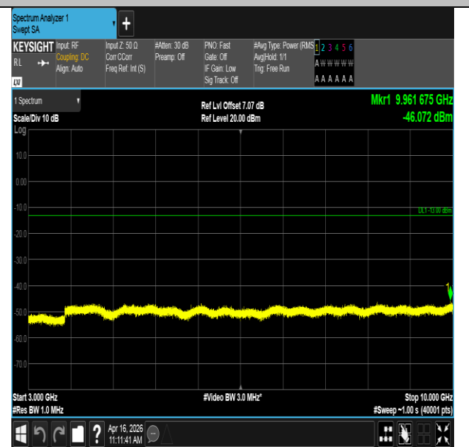
Band12-5MHz-16QAM-23155-25RB#0-3000~10000-PASS
