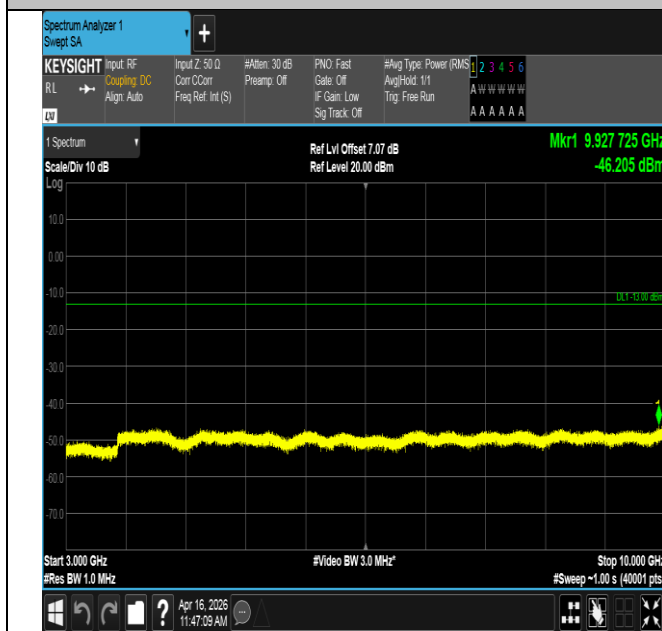
Band12-10MHz-QPSK-23095-1RB#0-3000~10000-PASS
