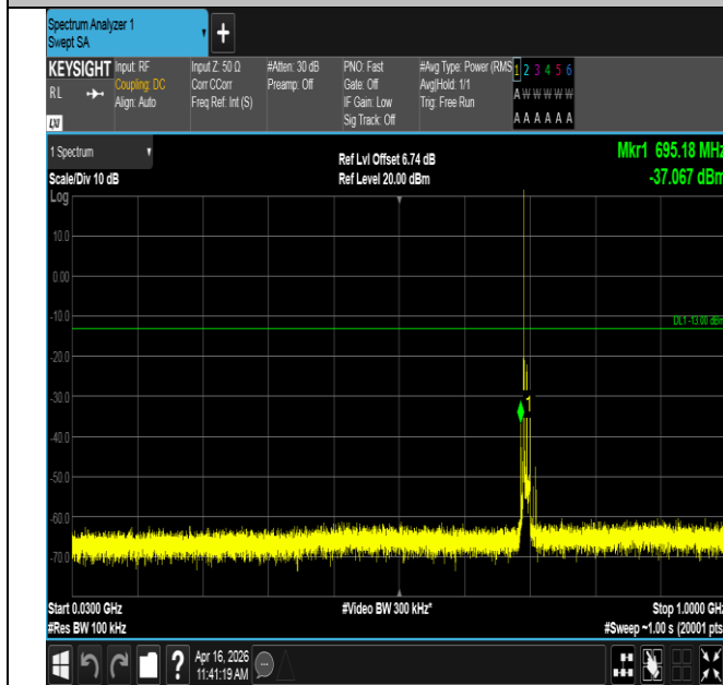
Band12-10MHz-QPSK-23060-1RB#0-30~1000-PASS
