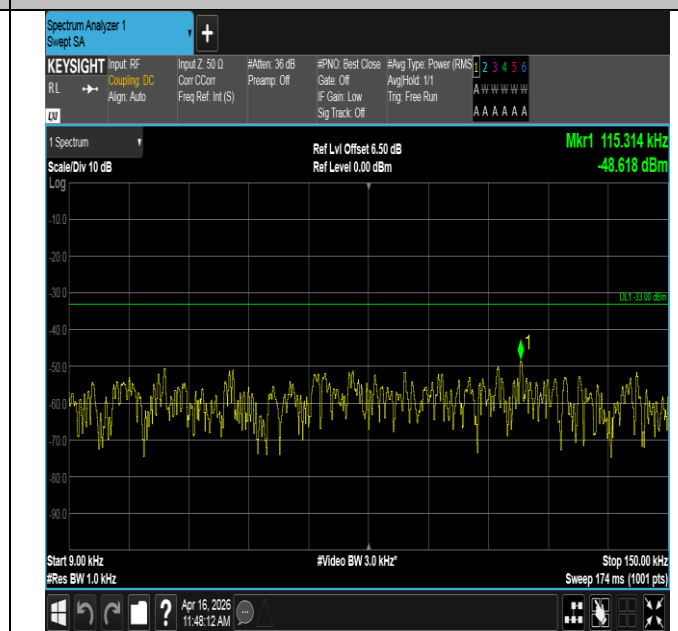
Band12-10MHz-QPSK-23095-1RB#49-0.009~0.15-PASS
