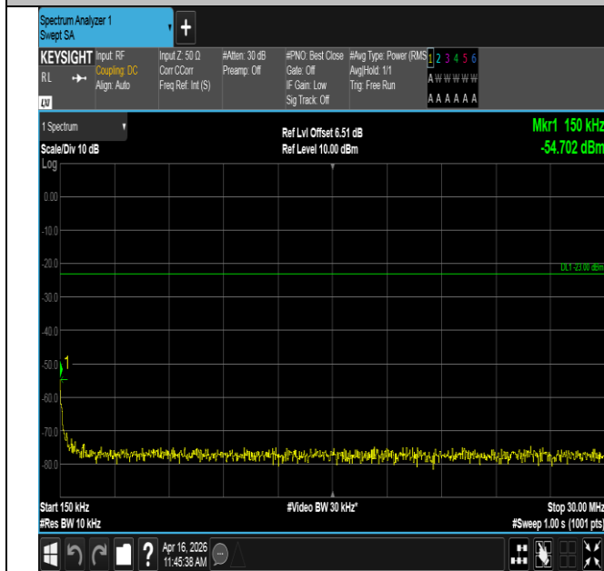
Band12-10MHz-16QAM-23060-50RB#0-0.15~30-PASS
