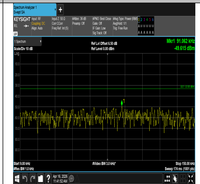
Band12-10MHz-16QAM-23060-1RB#0-0.009~0.15-PASS
