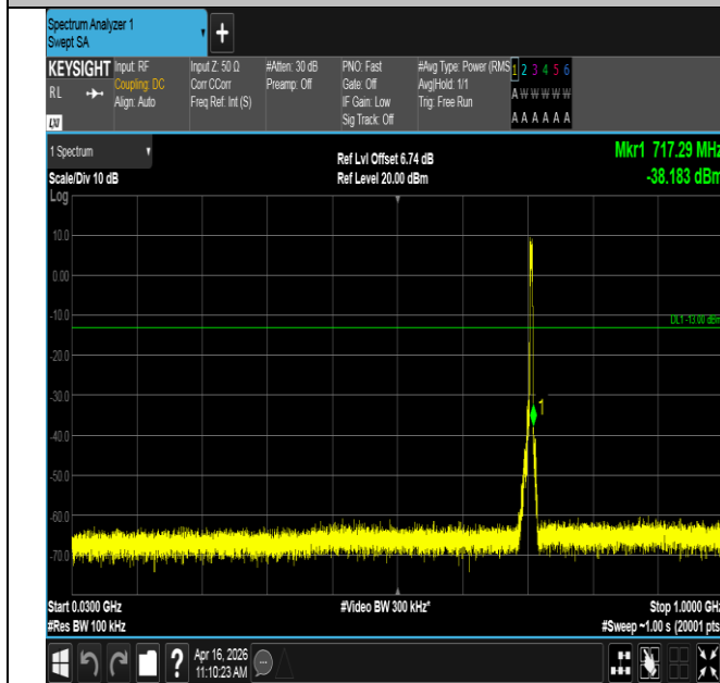
Band12-5MHz-QPSK-23155-25RB#0-30~1000-PASS
