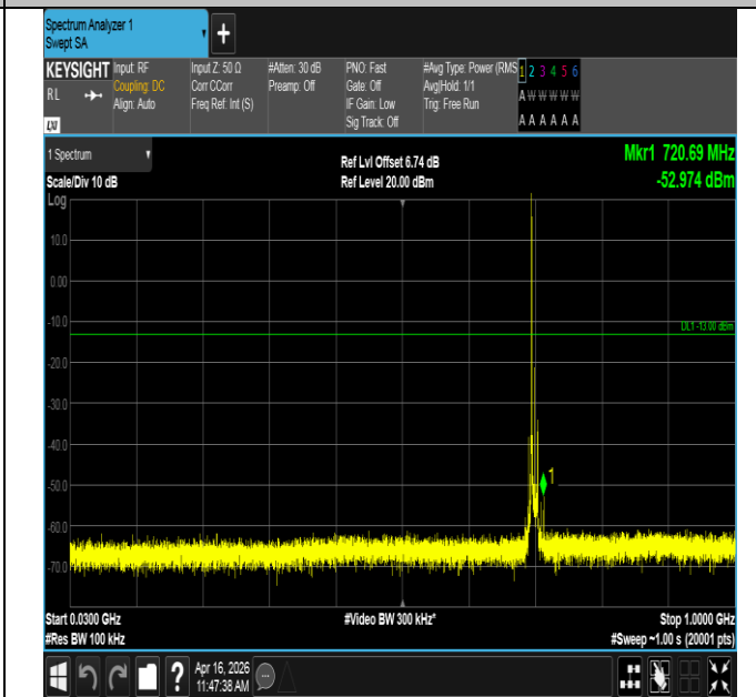
Band12-10MHz-16QAM-23095-1RB#0-30~1000-PASS
