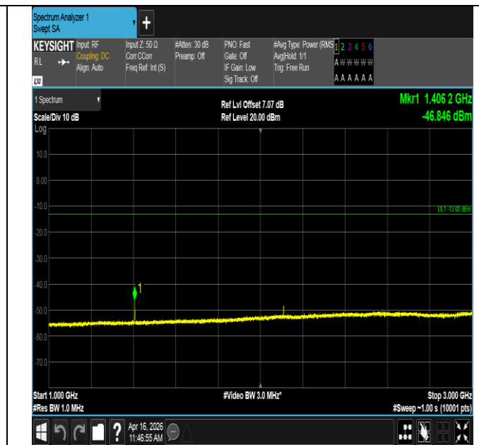
Band12-10MHz-QPSK-23095-1RB#0-1000~3000-PASS
