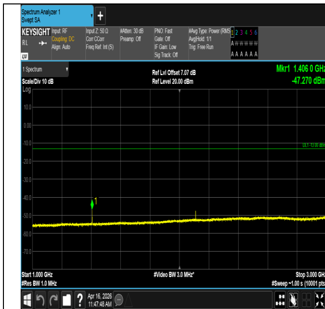
Band12-10MHz-16QAM-23095-1RB#0-1000~3000-PASS
