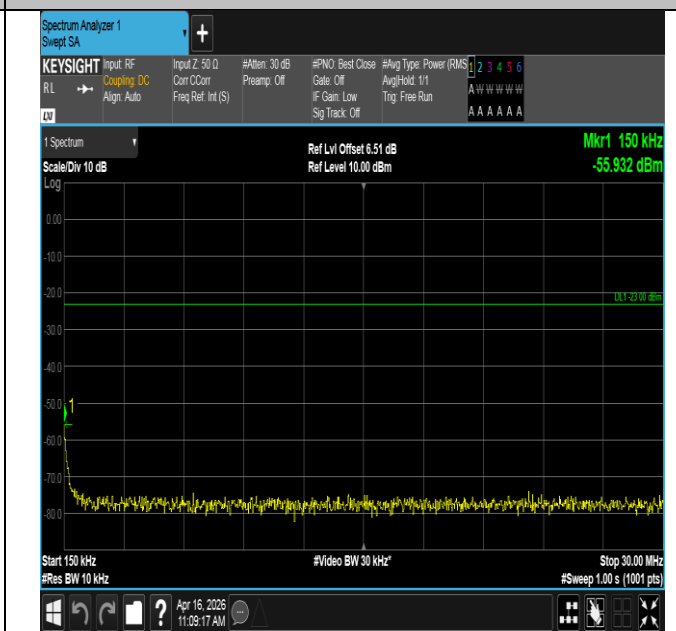
Band12-5MHz-16QAM-23155-1RB#24-0.15~30-PASS
