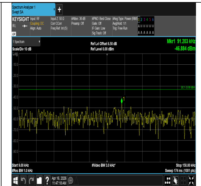
Band12-10MHz-16QAM-23095-1RB#0-0.009~0.15-PASS
