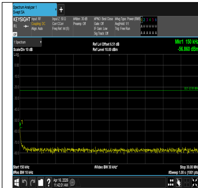
Band12-10MHz-16QAM-23060-1RB#0-0.15~30-PASS
