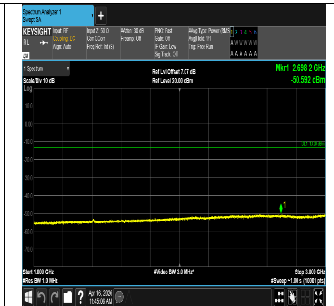
Band12-10MHz-QPSK-23060-50RB#0-1000~3000-PASS
