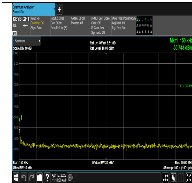
Band12-5MHz-16QAM-23155-25RB#0-0.15~30-PASS
