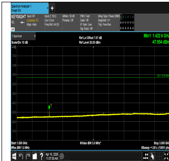
Band12-5MHz-16QAM-23155-1RB#0-1000~3000-PASS
