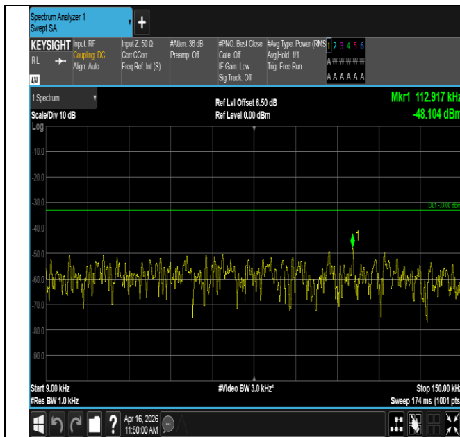
Band12-10MHz-QPSK-23095-50RB#0-0.009~0.15-PASS
