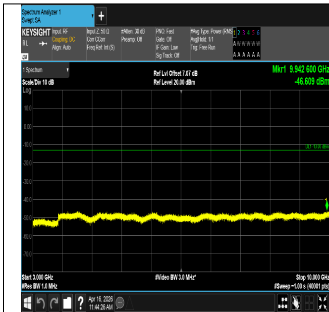
Band12-10MHz-16QAM-23060-1RB#49-3000~10000-PASS
