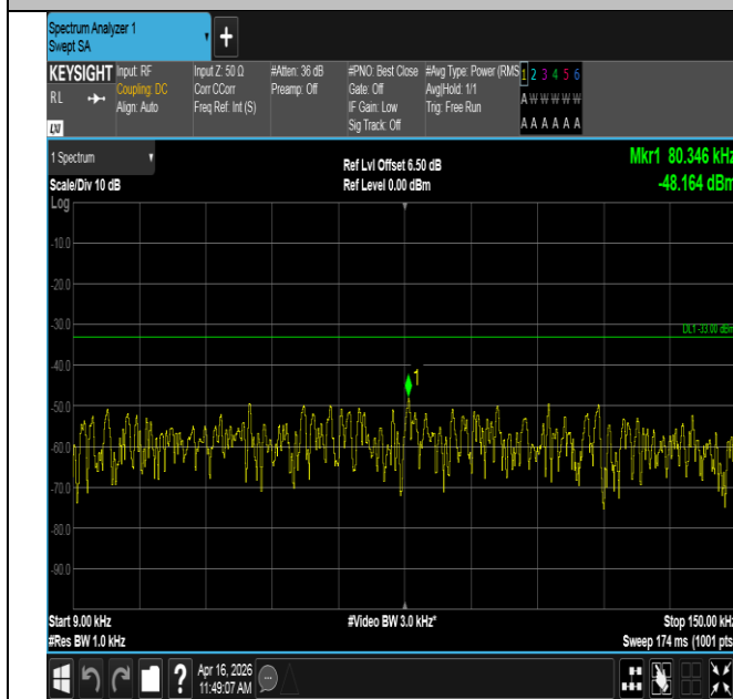
Band12-10MHz-16QAM-23095-1RB#49-0.009~0.15-PASS
