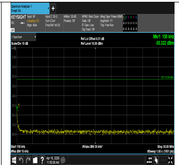
Band12-10MHz-QPSK-23095-50RB#0-0.15~30-PASS
