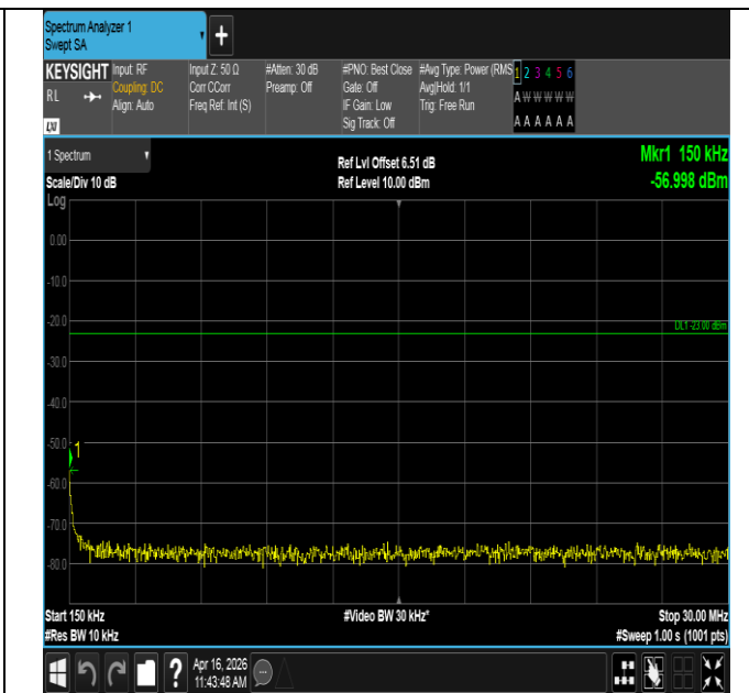
Band12-10MHz-16QAM-23060-1RB#49-0.15~30-PASS
