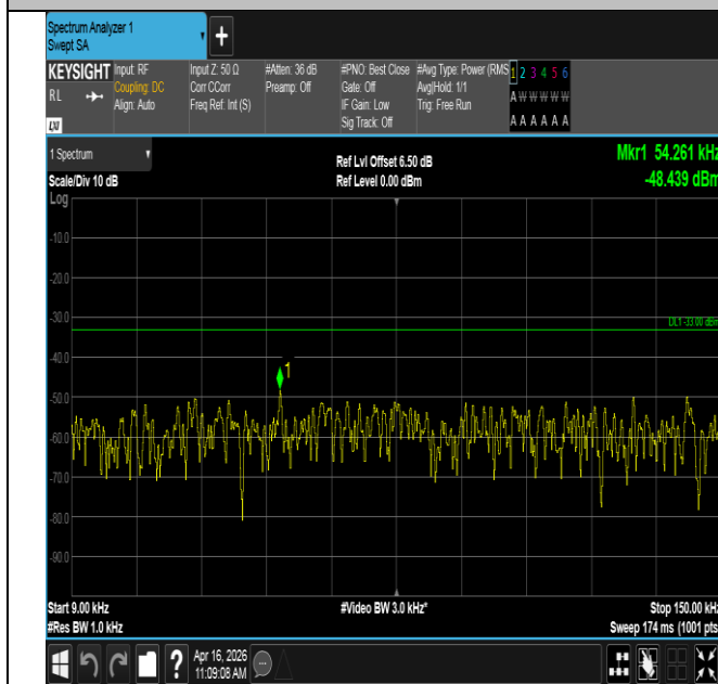
Band12-5MHz-16QAM-23155-1RB#24-0.009~0.15-PASS
