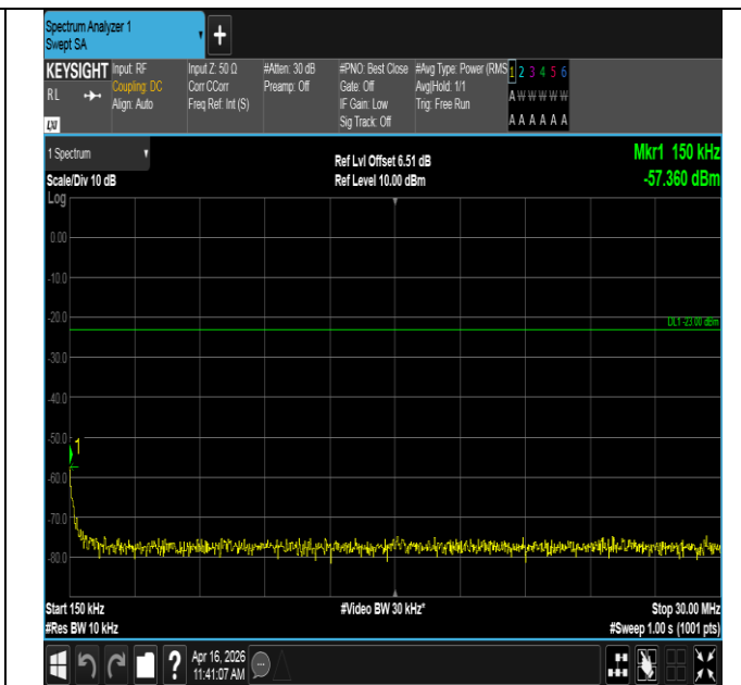
Band12-10MHz-QPSK-23060-1RB#0-0.15~30-PASS
