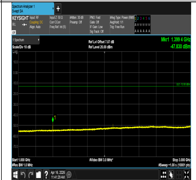
Band12-10MHz-QPSK-23060-1RB#0-1000~3000-PASS
