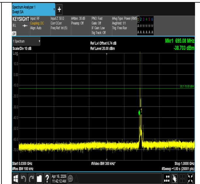
Band12-10MHz-16QAM-23060-1RB#0-30~1000-PASS
