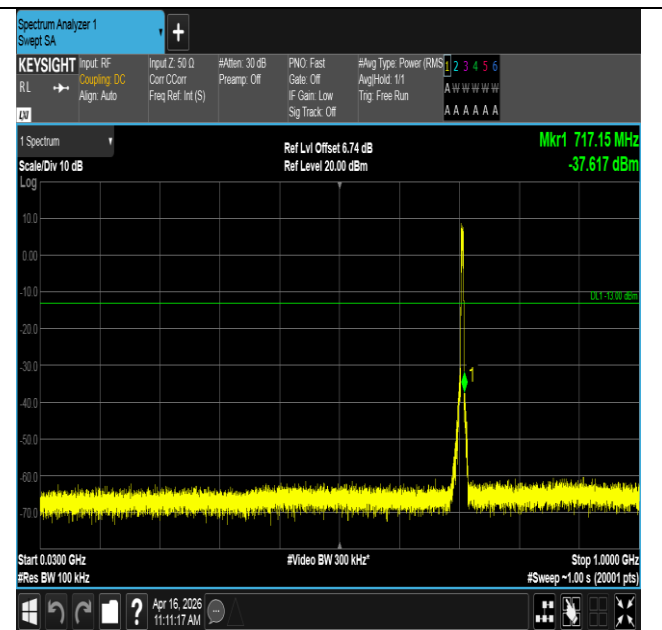
Band12-5MHz-16QAM-23155-25RB#0-30~1000-PASS
