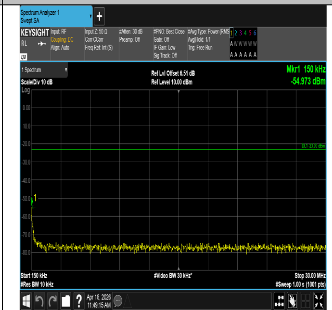
Band12-10MHz-16QAM-23095-1RB#49-0.15~30-PASS
