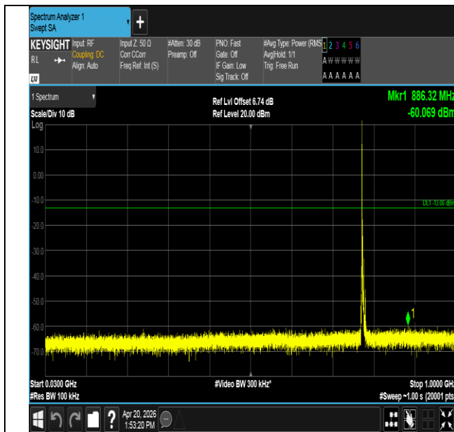
Band13-5MHz-QPSK-23205-1RB#0-30~1000-PASS
