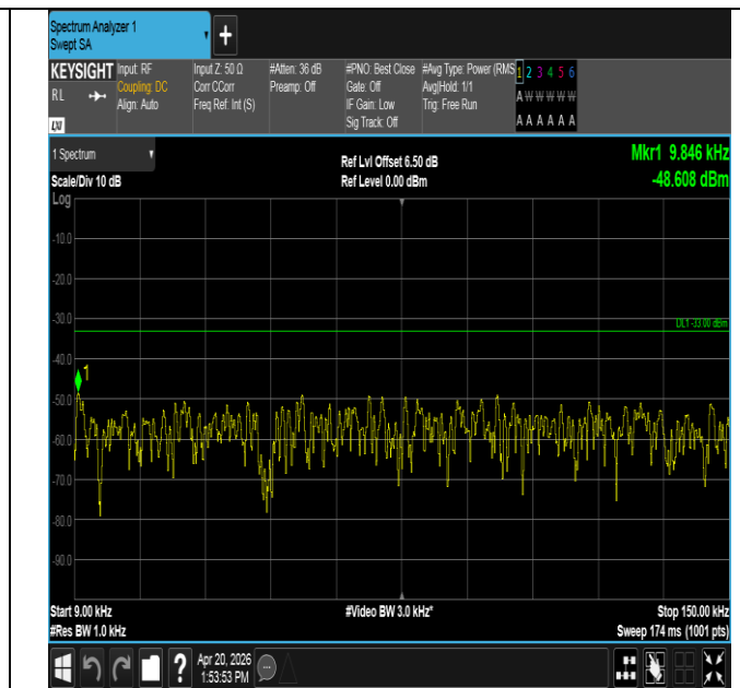
Band13-5MHz-16QAM-23205-1RB#0-0.009~0.15-PASS
