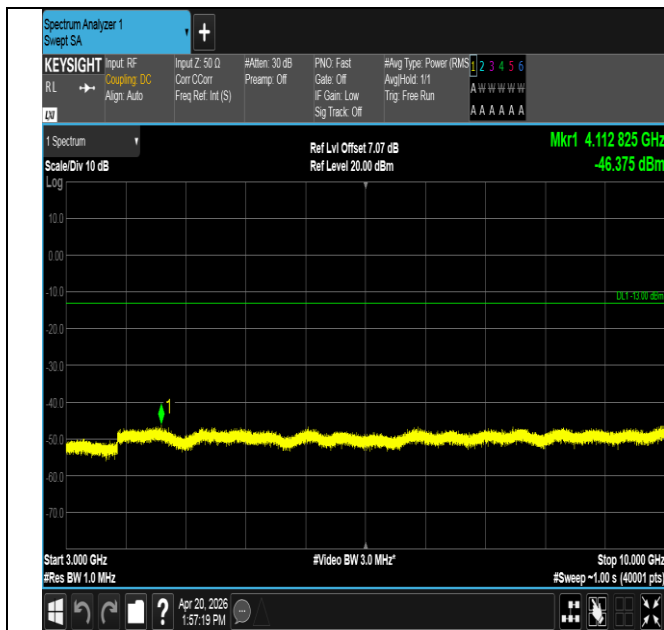
Band13-5MHz-QPSK-23205-25RB#0-3000~10000-PASS
