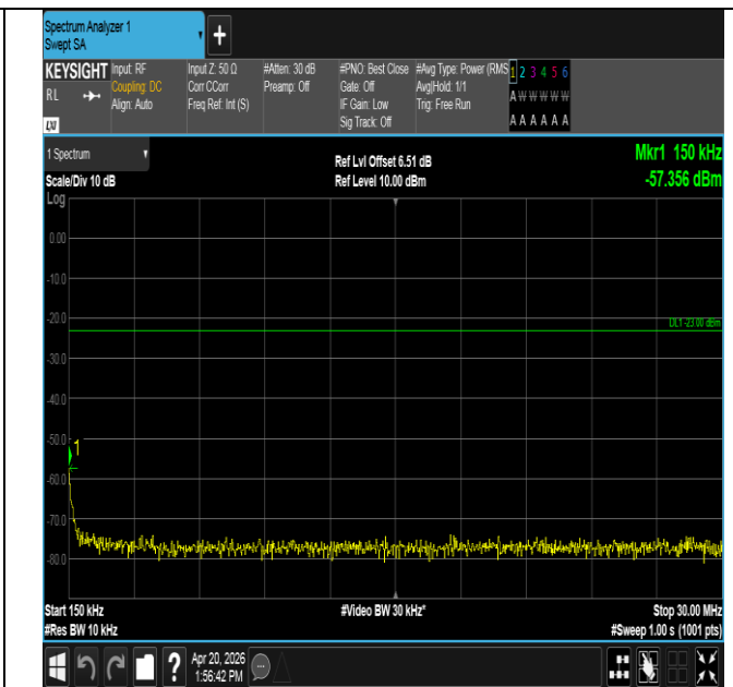
Band13-5MHz-QPSK-23205-25RB#0-0.15~30-PASS
