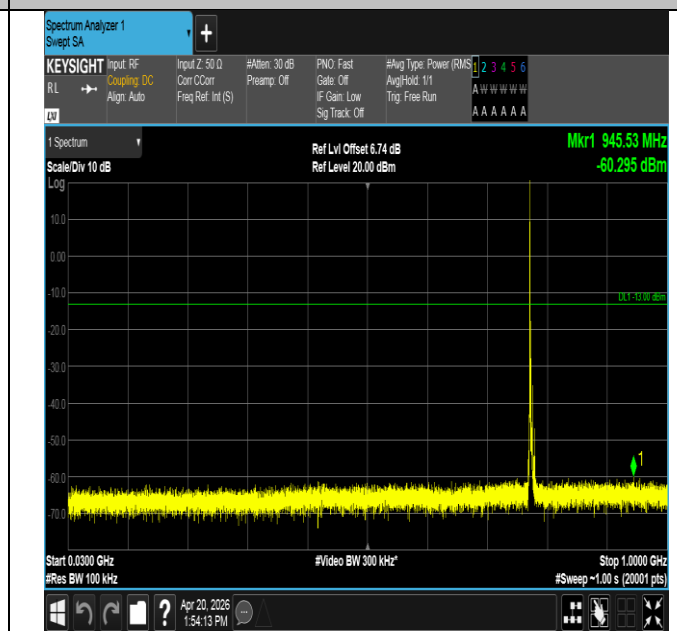
Band13-5MHz-16QAM-23205-1RB#0-30~1000-PASS
