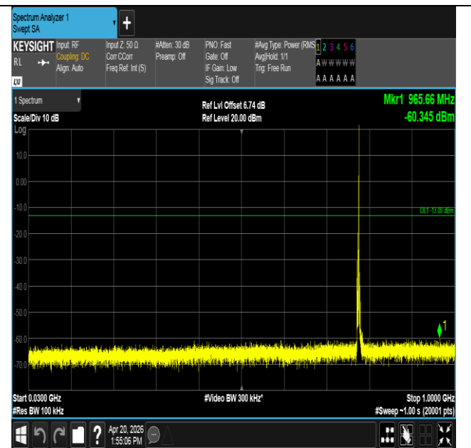
Band13-5MHz-QPSK-23205-1RB#24-30~1000-PASS
