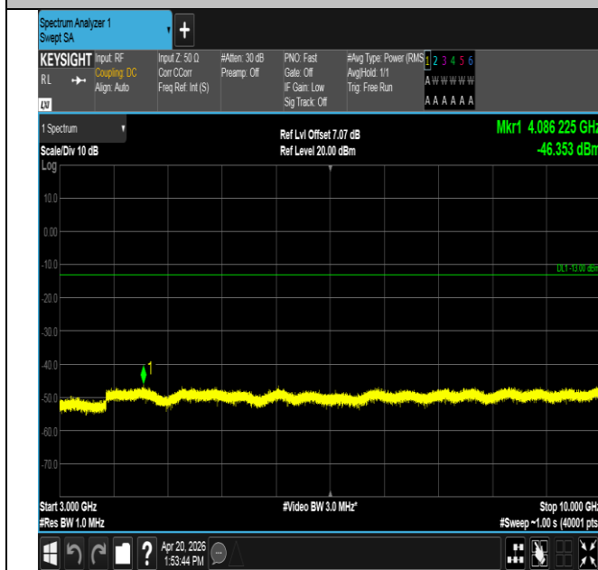
Band13-5MHz-QPSK-23205-1RB#0-3000~10000-PASS
