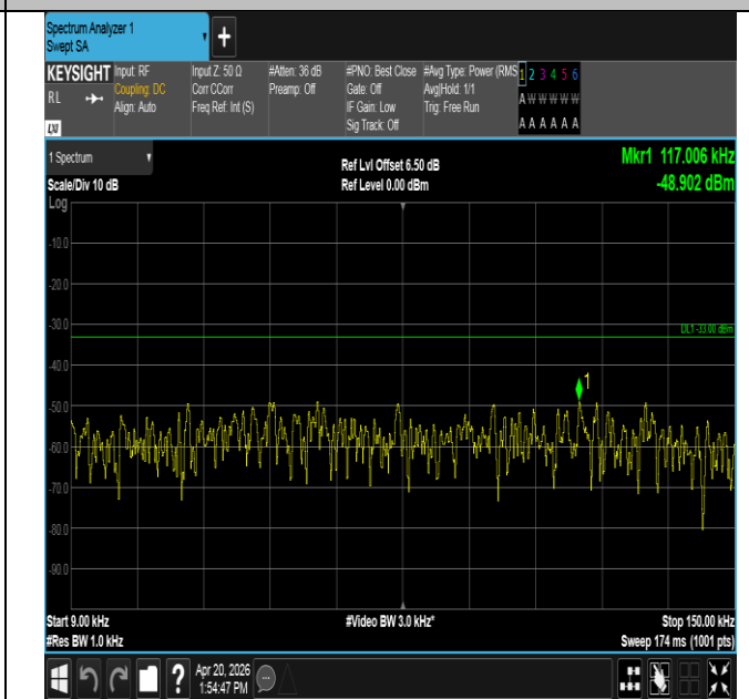
Band13-5MHz-QPSK-23205-1RB#24-0.009~0.15-PASS
