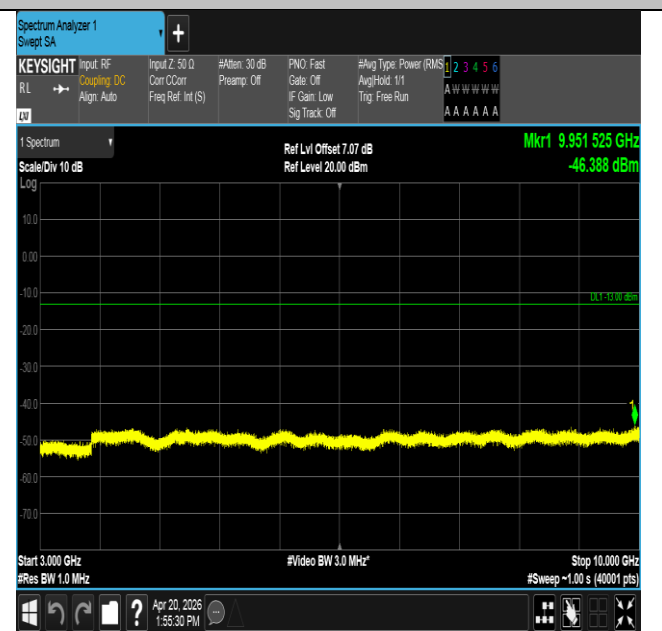
Band13-5MHz-QPSK-23205-1RB#24-3000~10000-PASS
