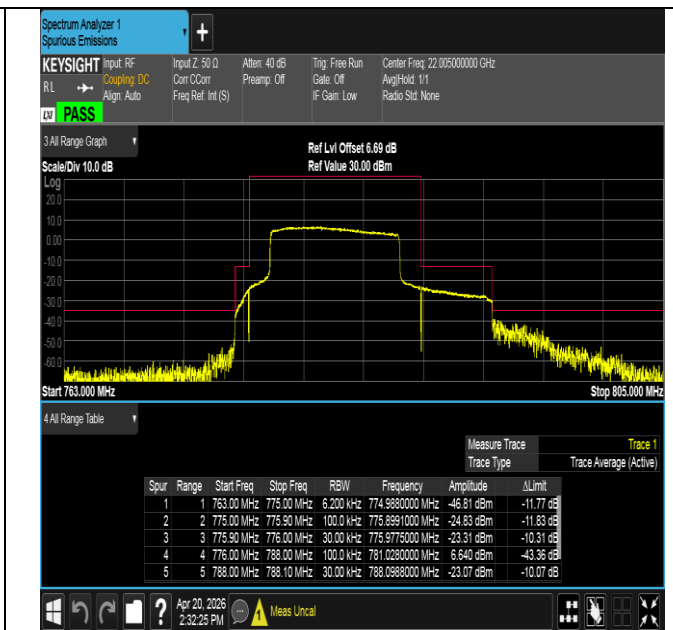
Band13-10MHz-16QAM-23230-50RB#0-PASS
