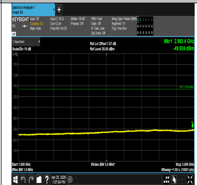
Band13-5MHz-QPSK-23205-25RB#0-1000~3000-PASS
