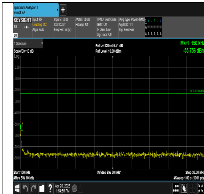
Band13-5MHz-QPSK-23205-1RB#24-0.15~30-PASS
