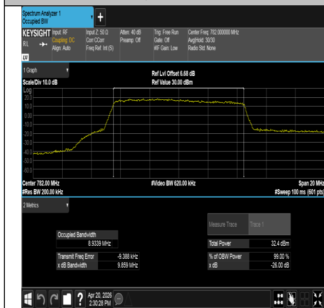
Band13-10MHz-QPSK-23230-50RB#0-PASS
