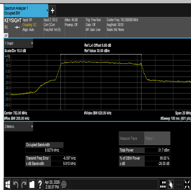
Band13-10MHz-16QAM-23230-50RB#0-PASS
