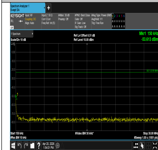
Band13-5MHz-16QAM-23205-1RB#0-0.15~30-PASS
