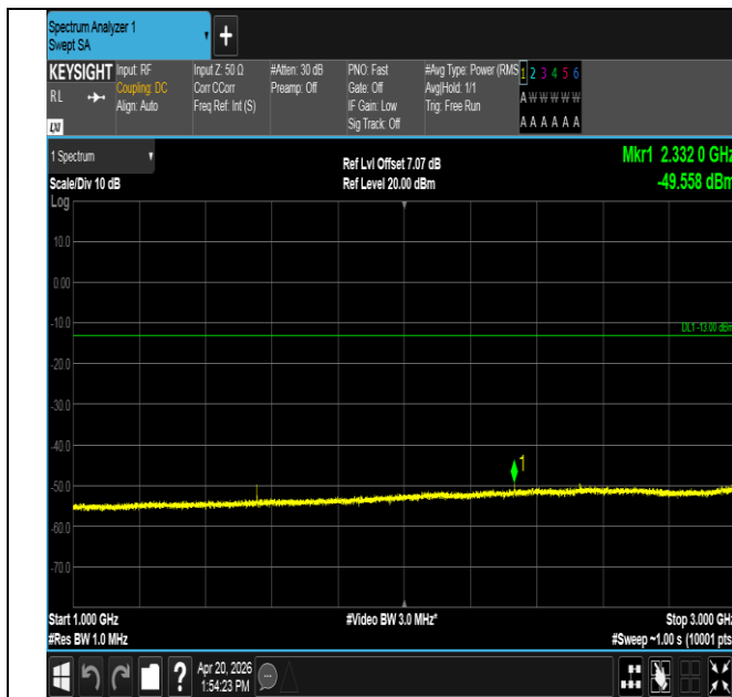
Band13-5MHz-16QAM-23205-1RB#0-1000~3000-PASS
