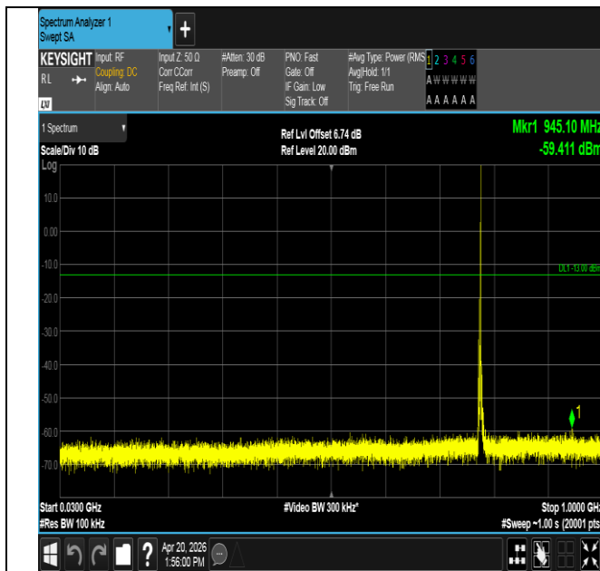
Band13-5MHz-16QAM-23205-1RB#24-30~1000-PASS
