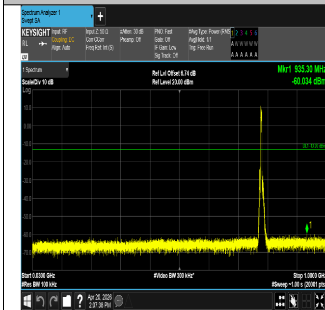
Band13-5MHz-QPSK-23255-25RB#0-30~1000-PASS
