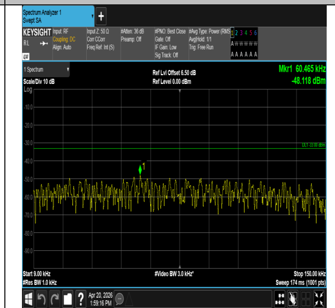
Band13-5MHz-16QAM-23230-1RB#0-0.009~0.15-PASS
