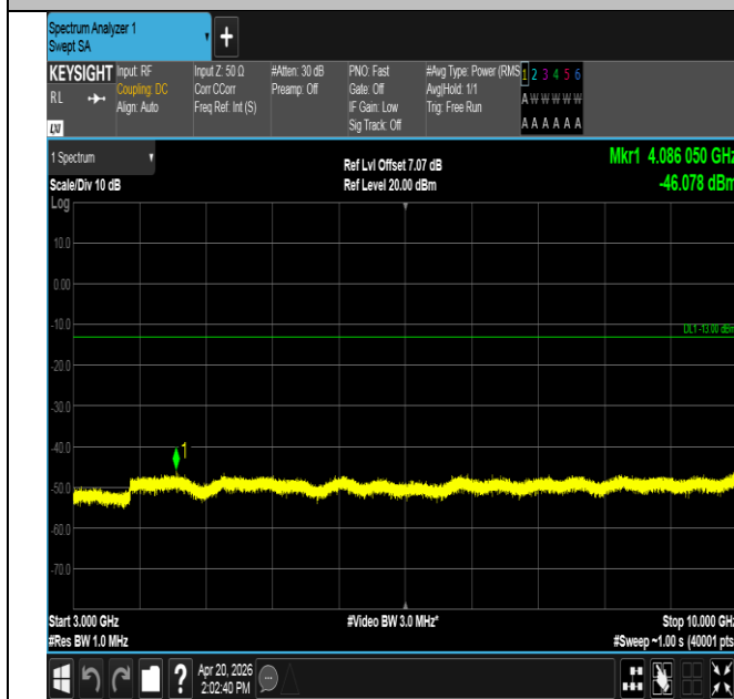
Band13-5MHz-QPSK-23230-25RB#0-3000~10000-PASS
