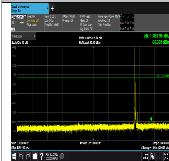
Band13-10MHz-QPSK-23230-1RB#0-30~1000-PASS
