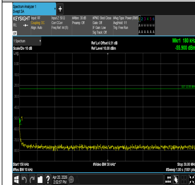
Band13-5MHz-16QAM-23230-25RB#0-0.15~30-PASS
