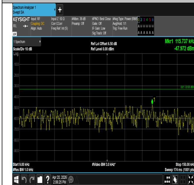
Band13-5MHz-16QAM-23255-1RB#24-0.009~0.15-PASS
