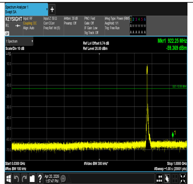
Band13-5MHz-16QAM-23205-25RB#0-30~1000-PASS
