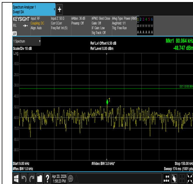
Band13-5MHz-QPSK-23230-1RB#0-0.009~0.15-PASS
