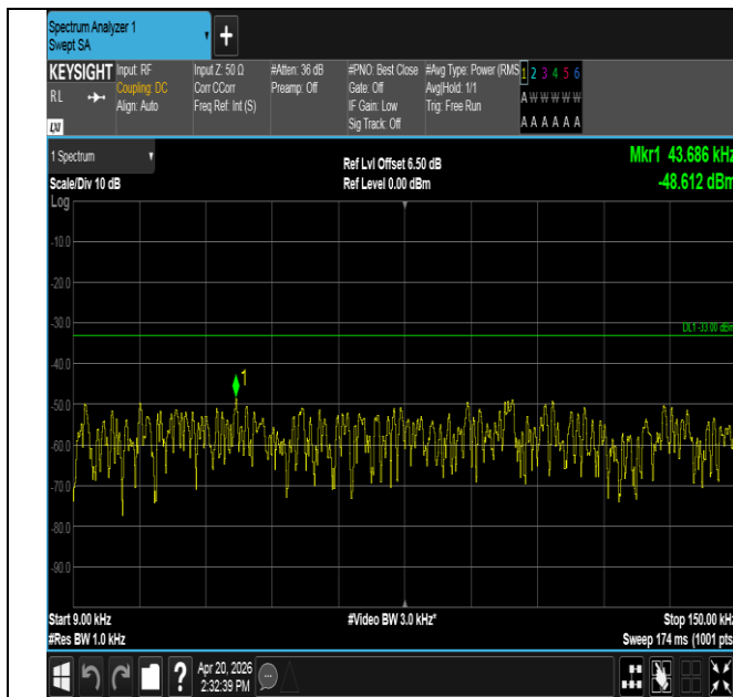
Band13-10MHz-QPSK-23230-1RB#0-0.009~0.15-PASS
