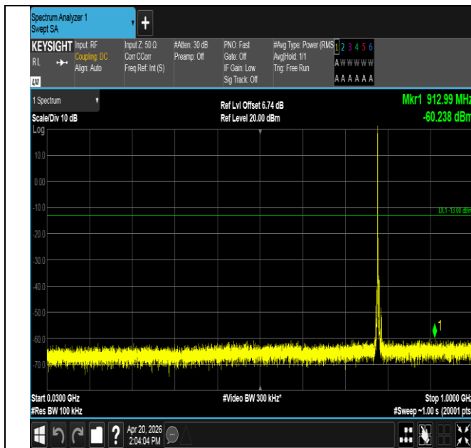
Band13-5MHz-QPSK-23255-1RB#0-30~1000-PASS
