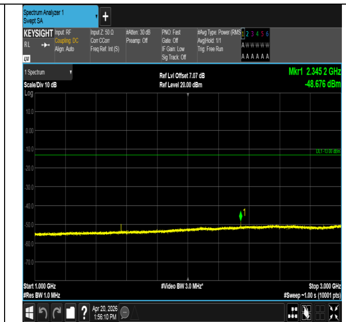
Band13-5MHz-16QAM-23205-1RB#24-1000~3000-PASS
