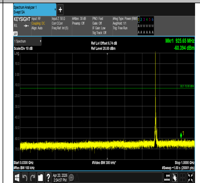
Band13-5MHz-16QAM-23255-1RB#0-30~1000-PASS
