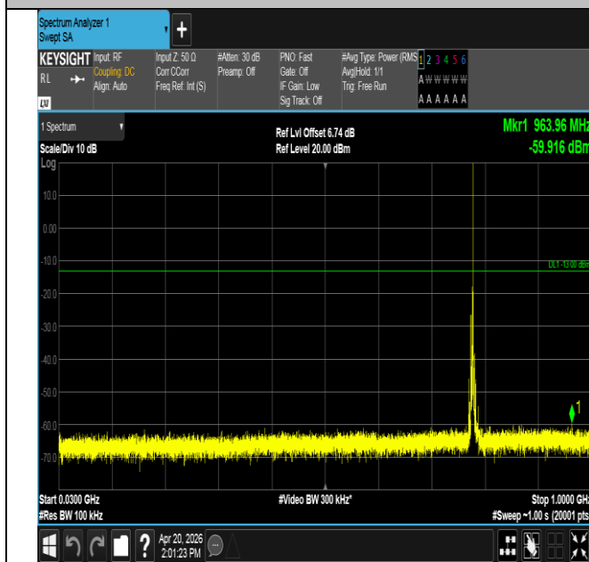
Band13-5MHz-16QAM-23230-1RB#24-30~1000-PASS
