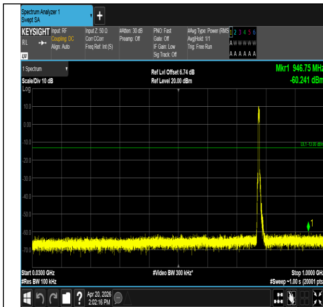
Band13-5MHz-QPSK-23230-25RB#0-30~1000-PASS
