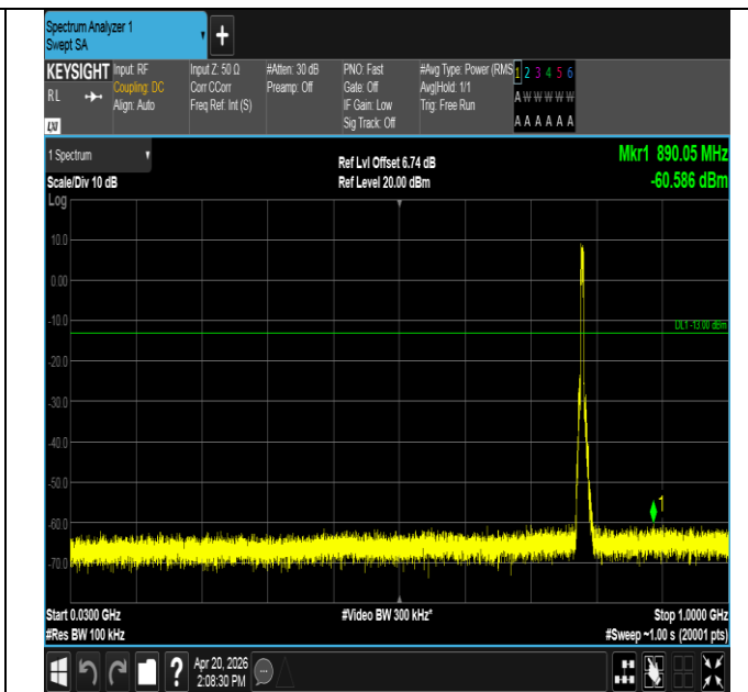
Band13-5MHz-16QAM-23255-25RB#0-30~1000-PASS
