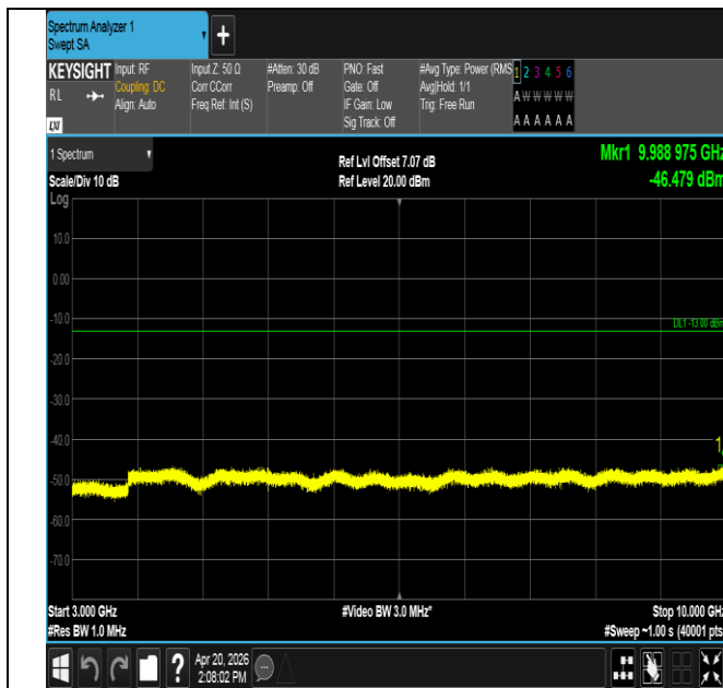
Band13-5MHz-QPSK-23255-25RB#0-3000~10000-PASS
