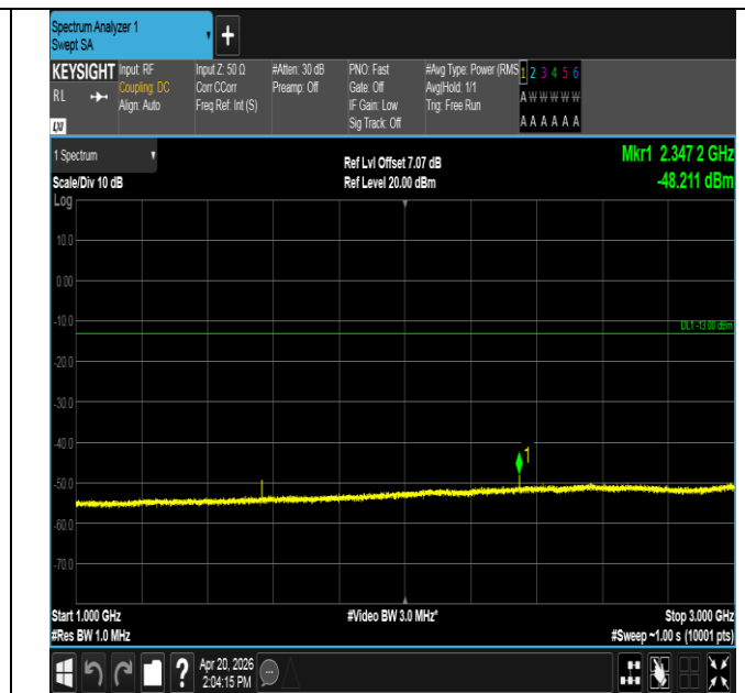
Band13-5MHz-QPSK-23255-1RB#0-1000~3000-PASS
