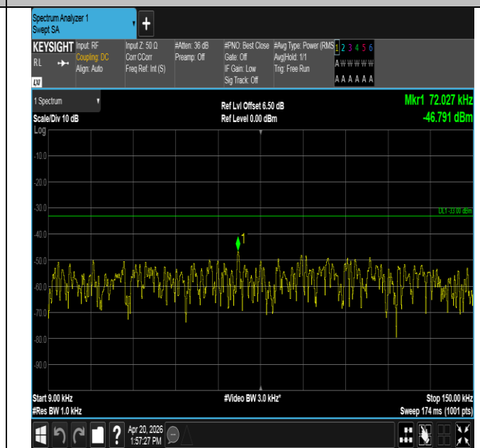
Band13-5MHz-16QAM-23205-25RB#0-0.009~0.15-PASS
