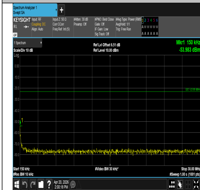
Band13-5MHz-QPSK-23230-1RB#24-0.15~30-PASS
