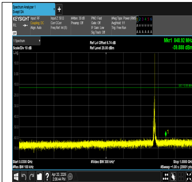
Band13-5MHz-16QAM-23255-1RB#24-30~1000-PASS
