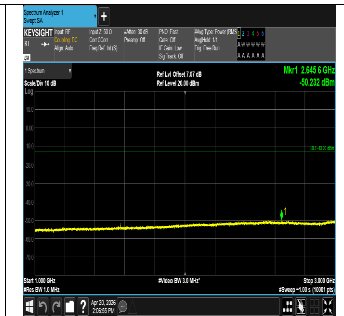
Band13-5MHz-16QAM-23255-1RB#24-1000~3000-PASS
