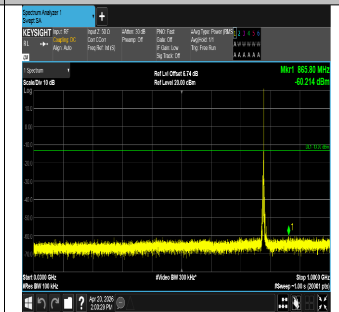
Band13-5MHz-QPSK-23230-1RB#24-30~1000-PASS
