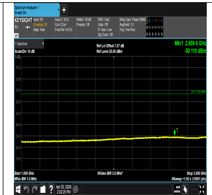
Band13-5MHz-QPSK-23230-25RB#0-1000~3000-PASS
