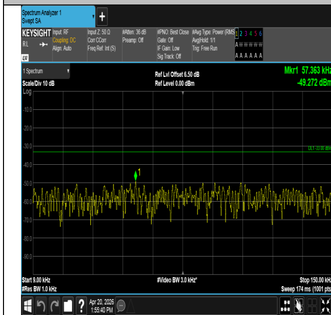
Band13-5MHz-16QAM-23205-1RB#24-0.009~0.15-PASS
