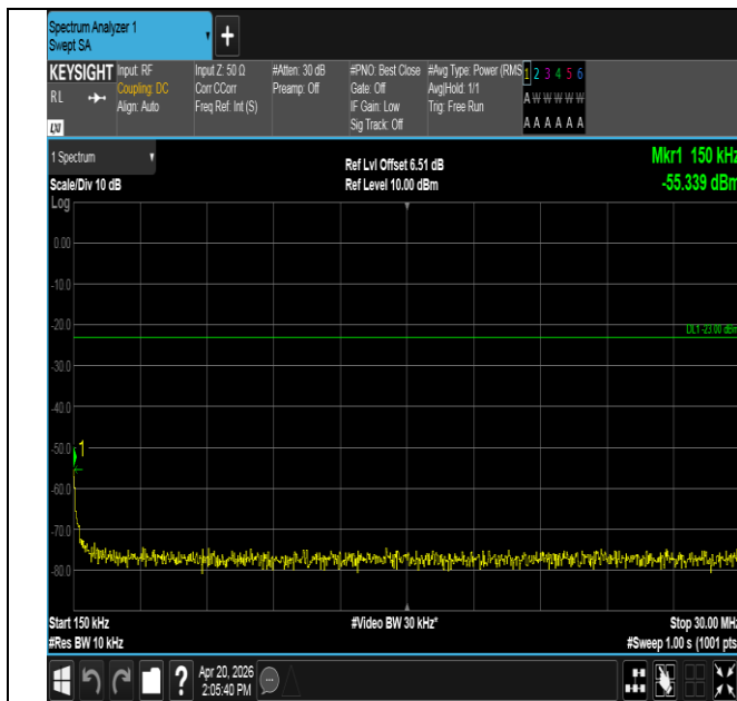
Band13-5MHz-QPSK-23255-1RB#24-0.15~30-PASS
