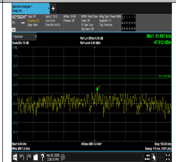
Band13-5MHz-16QAM-23255-25RB#0-0.009~0.15-PASS
