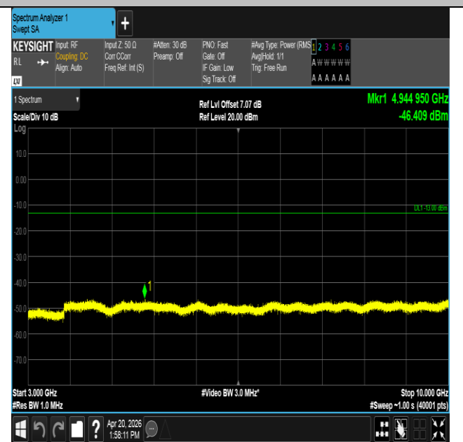
Band13-5MHz-16QAM-23205-25RB#0-3000~10000-PASS
