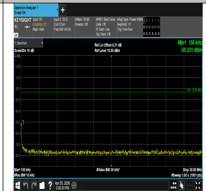
Band13-5MHz-16QAM-23255-1RB#24-0.15~30-PASS
