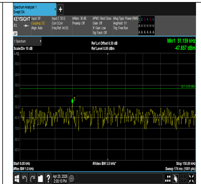
Band13-5MHz-QPSK-23230-1RB#24-0.009~0.15-PASS
