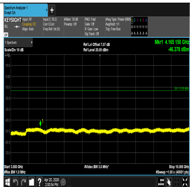
Band13-5MHz-QPSK-23230-1RB#24-3000~10000-PASS
