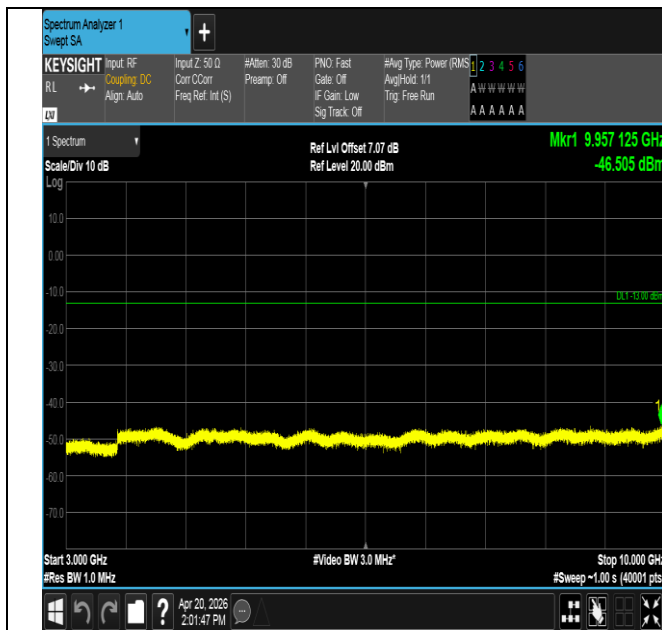
Band13-5MHz-16QAM-23230-1RB#24-3000~10000-PASS
