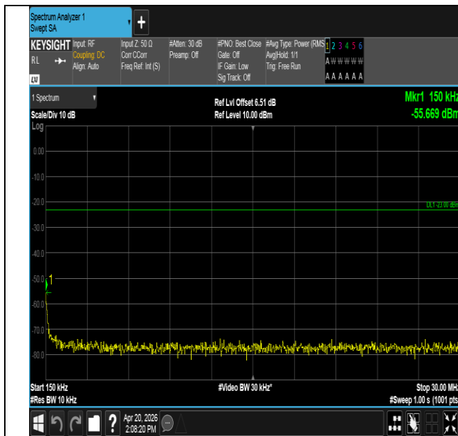
Band13-5MHz-16QAM-23255-25RB#0-0.15~30-PASS
