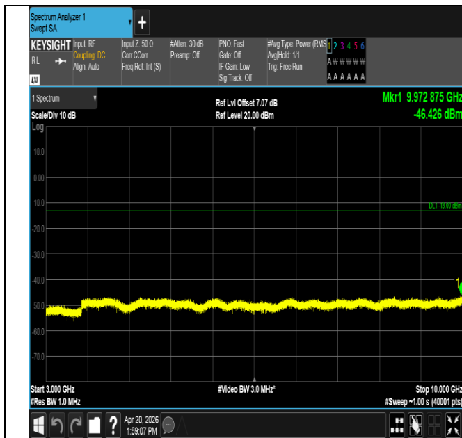
Band13-5MHz-QPSK-23230-1RB#0-3000~10000-PASS
