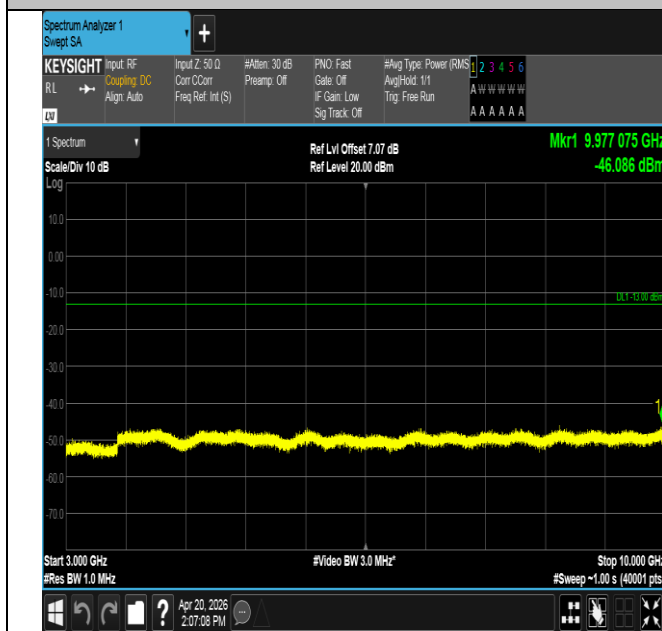
Band13-5MHz-16QAM-23255-1RB#24-3000~10000-PASS
