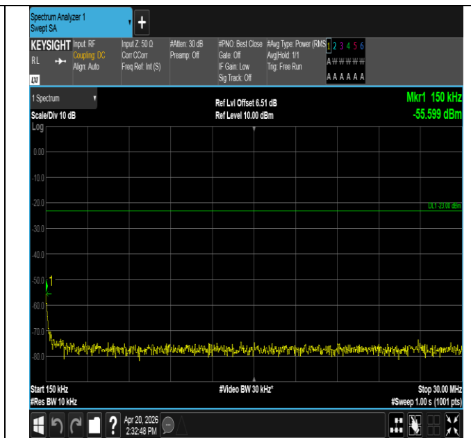
Band13-10MHz-QPSK-23230-1RB#0-0.15~30-PASS
