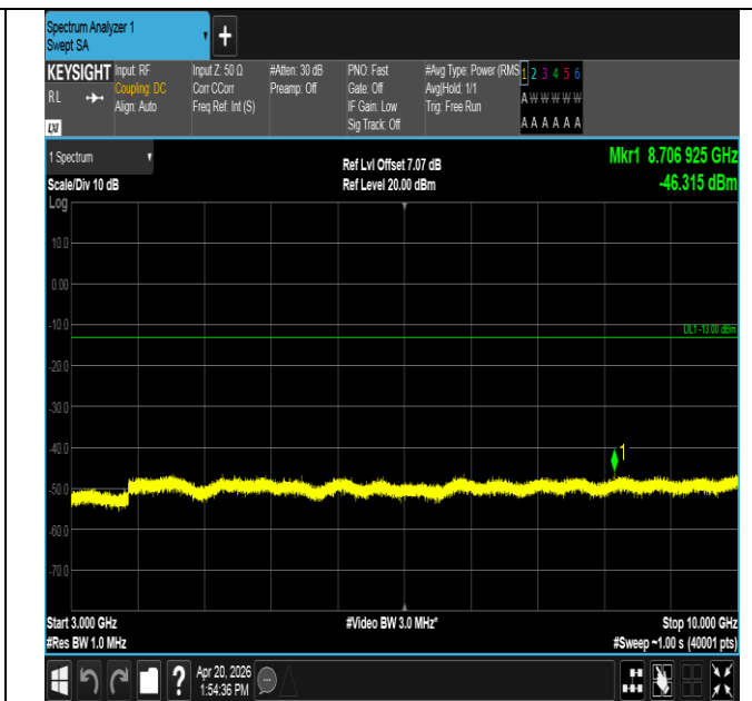
Band13-5MHz-16QAM-23205-1RB#0-3000~10000-PASS
