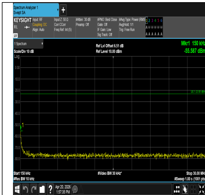
Band13-5MHz-16QAM-23205-25RB#0-0.15~30-PASS
