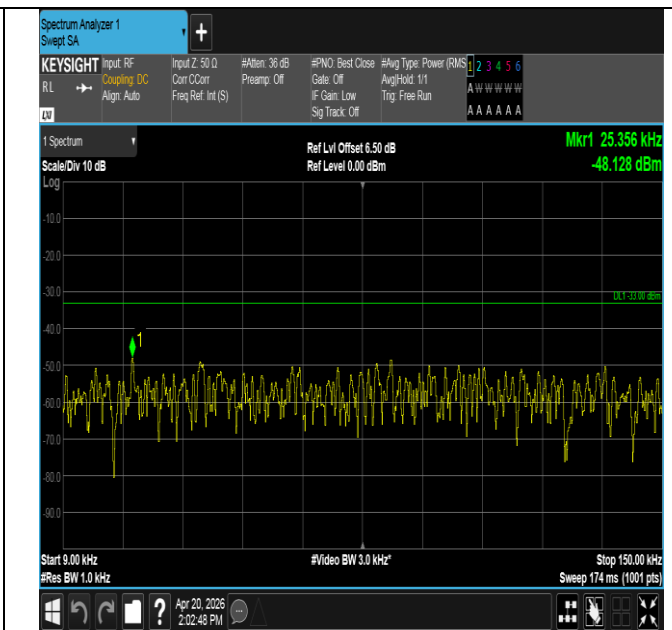
Band13-5MHz-16QAM-23230-25RB#0-0.009~0.15-PASS
