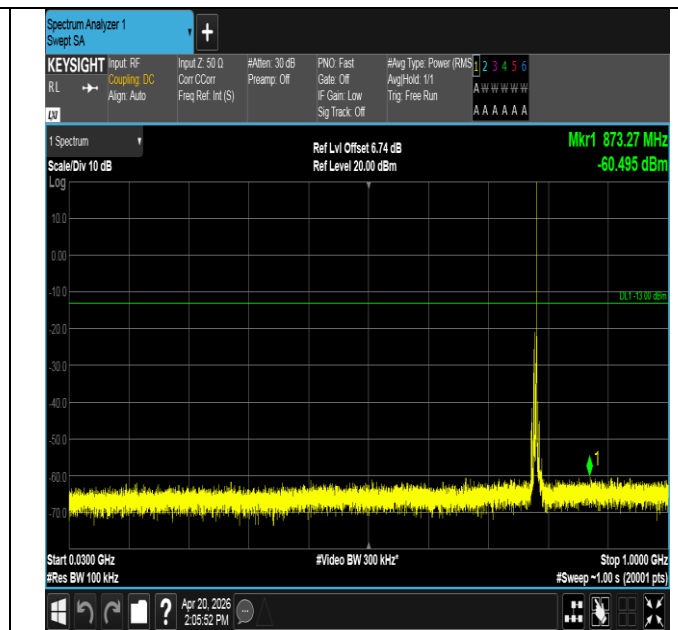
Band13-5MHz-QPSK-23255-1RB#24-30~1000-PASS
