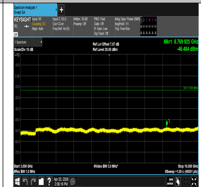
Band13-5MHz-QPSK-23255-1RB#24-3000~10000-PASS
