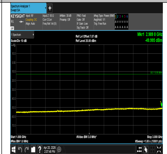
Band13-5MHz-QPSK-23255-25RB#0-1000~3000-PASS
