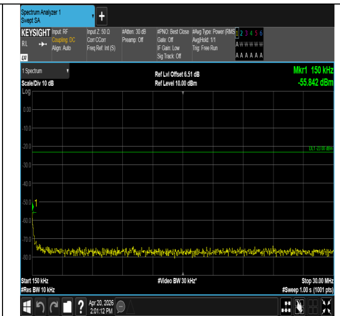
Band13-5MHz-16QAM-23230-1RB#24-0.15~30-PASS
