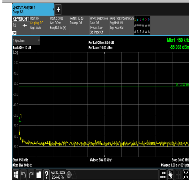
Band13-5MHz-16QAM-23255-1RB#0-0.15~30-PASS
