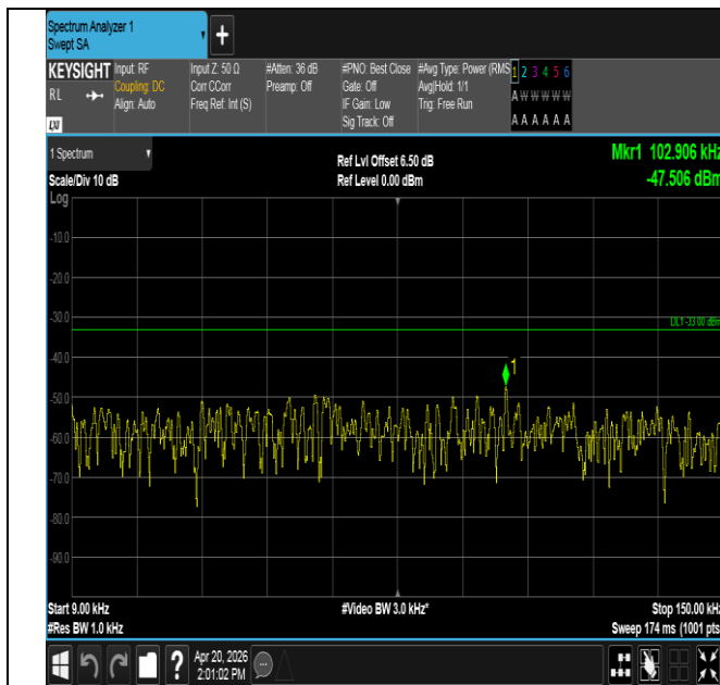
Band13-5MHz-16QAM-23230-1RB#24-0.009~0.15-PASS
