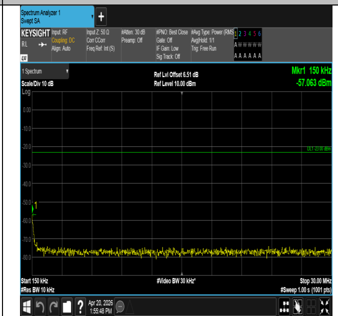
Band13-5MHz-16QAM-23205-1RB#24-0.15~30-PASS
