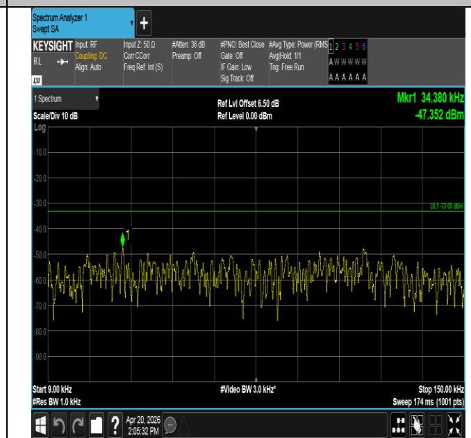
Band13-5MHz-QPSK-23255-1RB#24-0.009~0.15-PASS
