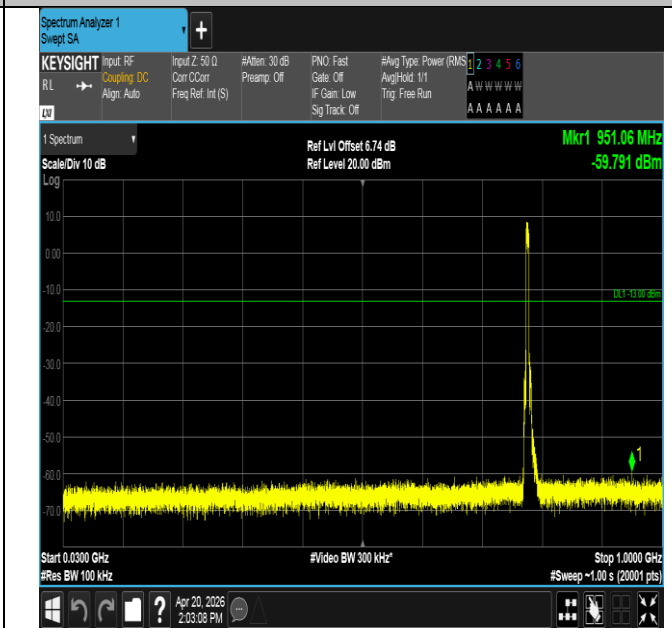
Band13-5MHz-16QAM-23230-25RB#0-30~1000-PASS
