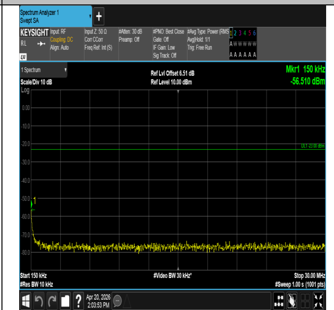
Band13-5MHz-QPSK-23255-1RB#0-0.15~30-PASS
