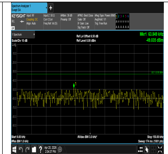
Band13-5MHz-16QAM-23255-1RB#0-0.009~0.15-PASS
