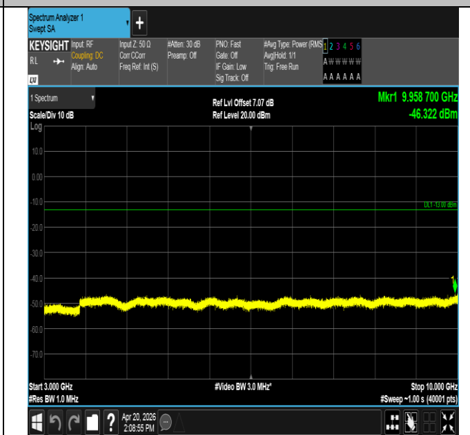
Band13-5MHz-16QAM-23255-25RB#0-3000~10000-PASS
