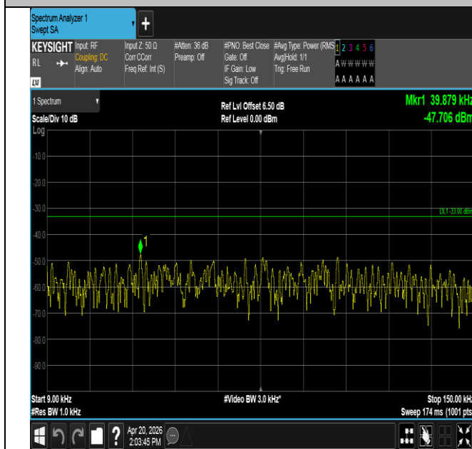
Band13-5MHz-QPSK-23255-1RB#0-0.009~0.15-PASS
