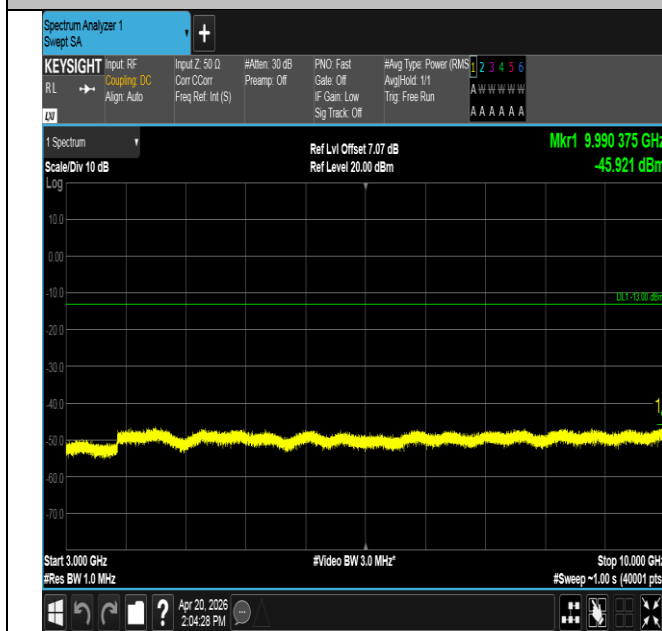
Band13-5MHz-QPSK-23255-1RB#0-3000~10000-PASS
