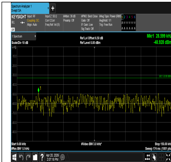
Band13-5MHz-QPSK-23255-25RB#0-0.009~0.15-PASS
