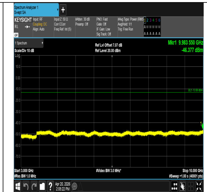
Band13-5MHz-16QAM-23255-1RB#0-3000~10000-PASS
