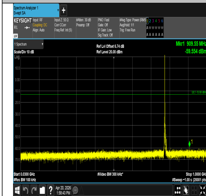
Band13-5MHz-QPSK-23230-1RB#0-30~1000-PASS
