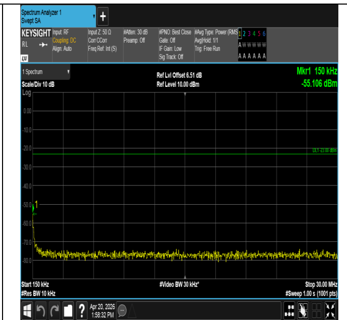
Band13-5MHz-QPSK-23230-1RB#0-0.15~30-PASS
