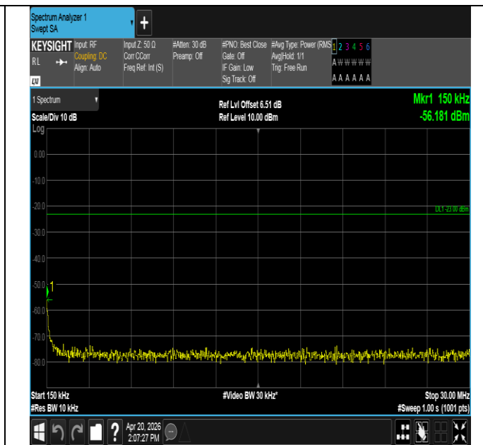
Band13-5MHz-QPSK-23255-25RB#0-0.15~30-PASS
