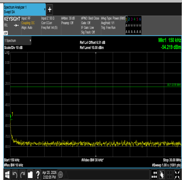
Band13-5MHz-QPSK-23230-25RB#0-0.15~30-PASS
