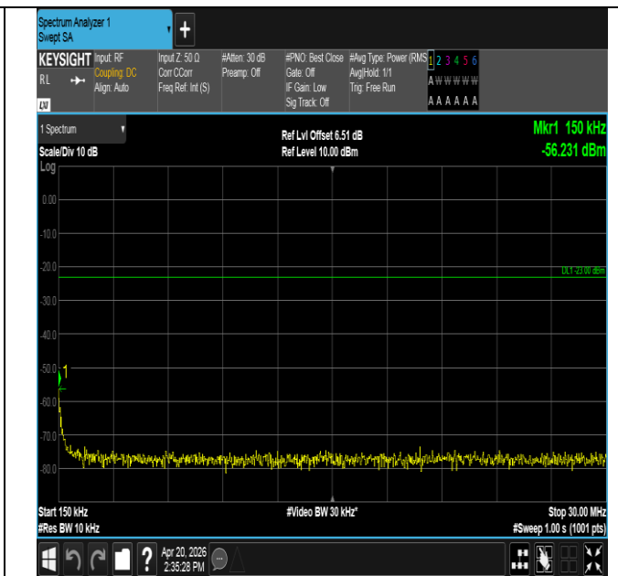
Band13-10MHz-16QAM-23230-1RB#49-0.15~30-PASS
