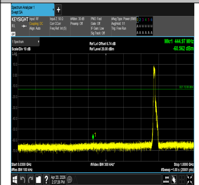
Band13-10MHz-16QAM-23230-50RB#0-30~1000-PASS
