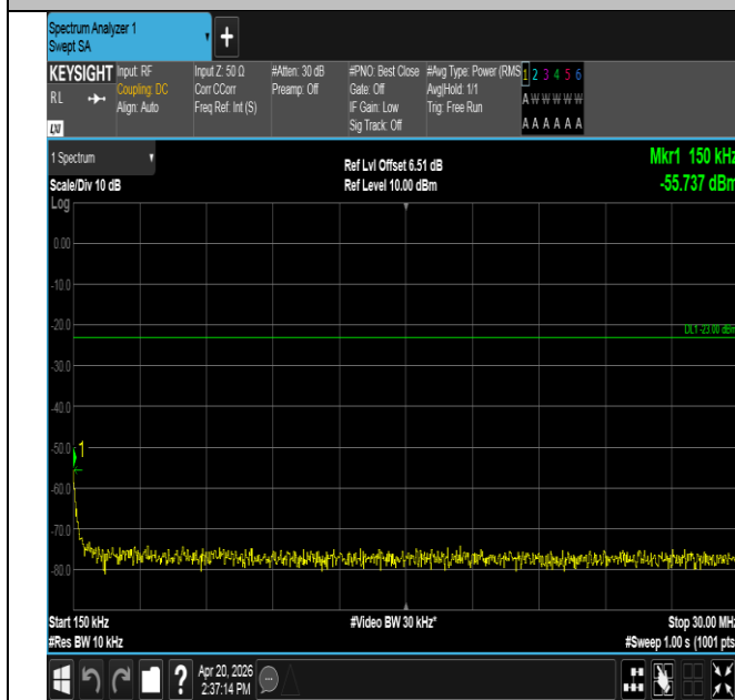
Band13-10MHz-16QAM-23230-50RB#0-0.15~30-PASS
