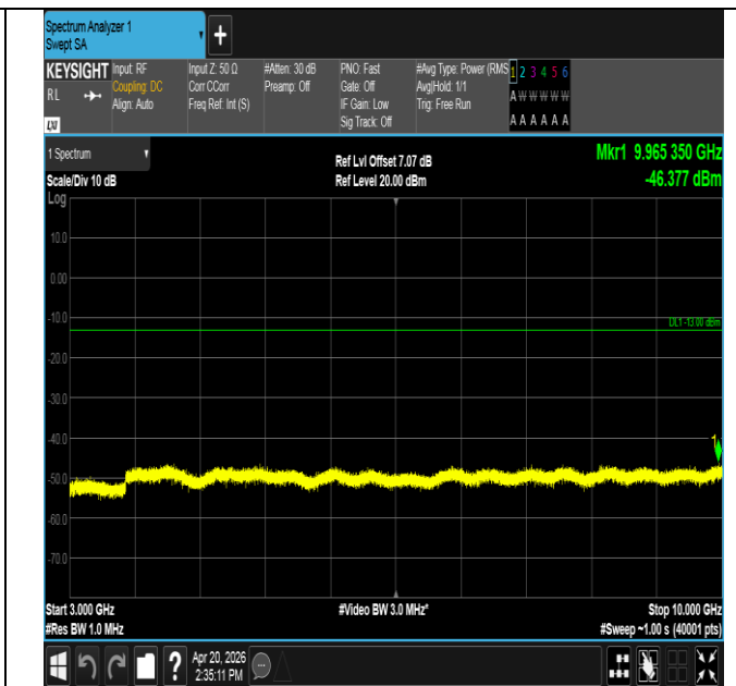
Band13-10MHz-QPSK-23230-1RB#49-3000~10000-PASS
