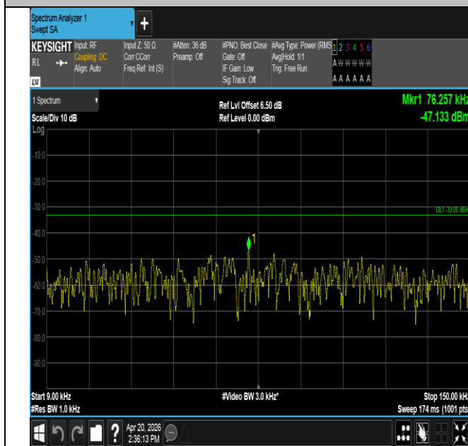
Band13-10MHz-QPSK-23230-50RB#0-0.009~0.15-PASS
