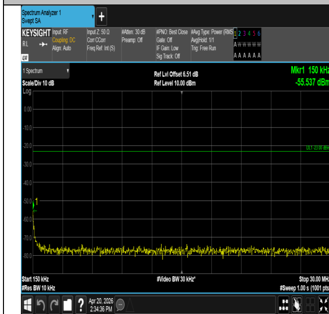
Band13-10MHz-QPSK-23230-1RB#49-0.15~30-PASS
