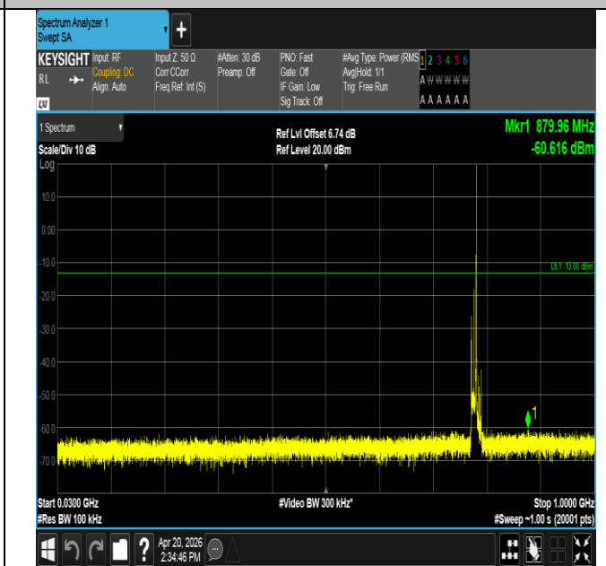
Band13-10MHz-QPSK-23230-1RB#49-30~1000-PASS
