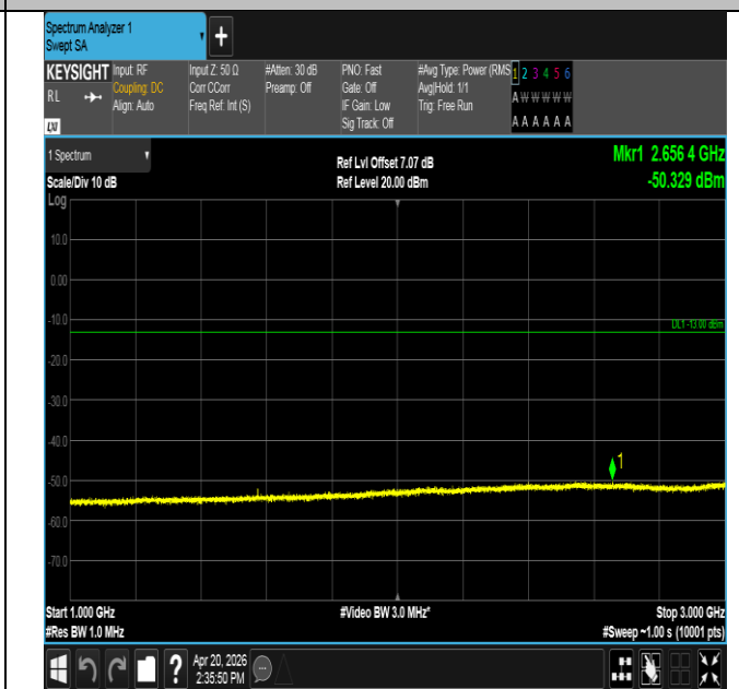
Band13-10MHz-16QAM-23230-1RB#49-1000~3000-PASS
