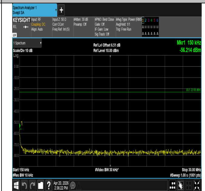
Band13-10MHz-QPSK-23230-50RB#0-0.15~30-PASS
