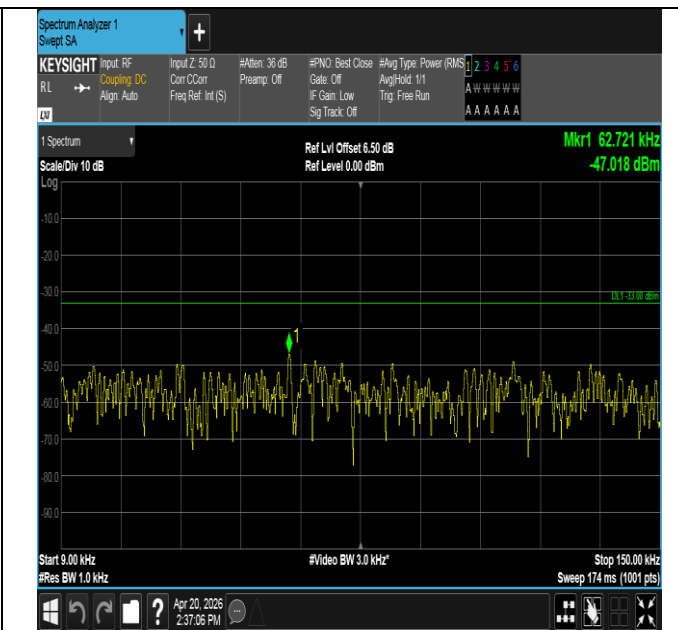
Band13-10MHz-16QAM-23230-50RB#0-0.009~0.15-PASS
