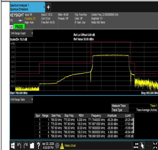
Band14-10MHz-QPSK-23330-50RB#0-PASS
