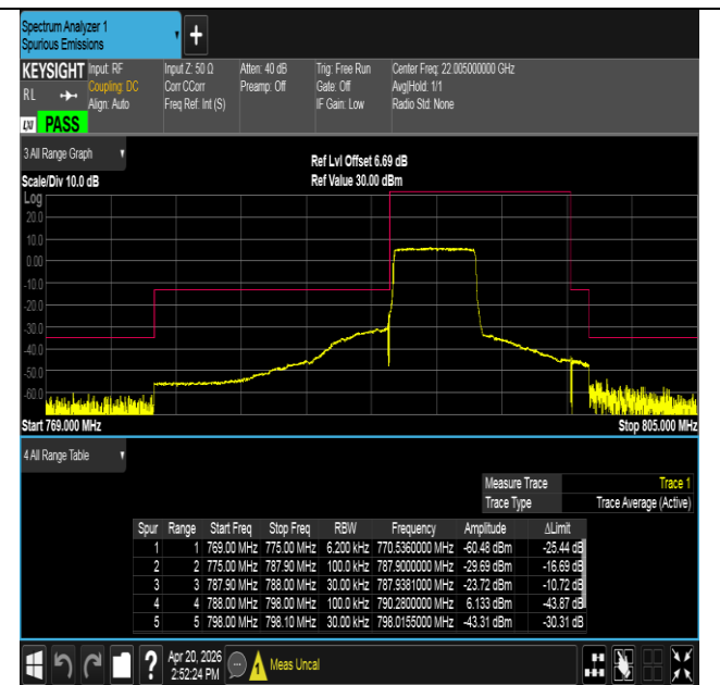
Band14-5MHz-16QAM-23305-25RB#0-PASS
