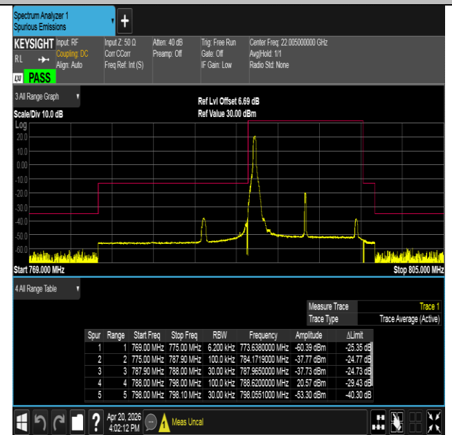
Band14-10MHz-16QAM-23330-1RB#0-PASS
