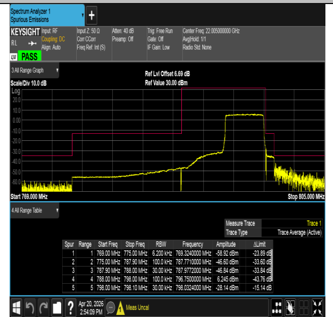
Band14-5MHz-16QAM-23355-25RB#0-PASS
