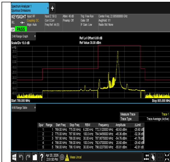
Band14-5MHz-16QAM-23305-1RB#24-PASS
