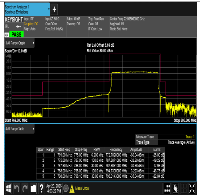
Band14-10MHz-16QAM-23330-50RB#0-PASS
