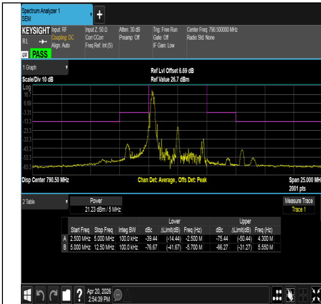
NTNV-Band14-5MHz-16QAM-23305-1RB#0--12.50--5.00-PAS
