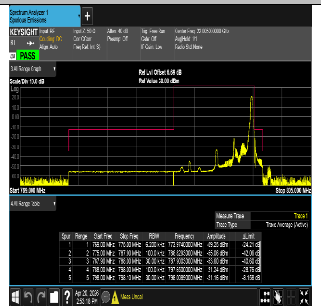
Band14-5MHz-QPSK-23355-1RB#24-PASS
