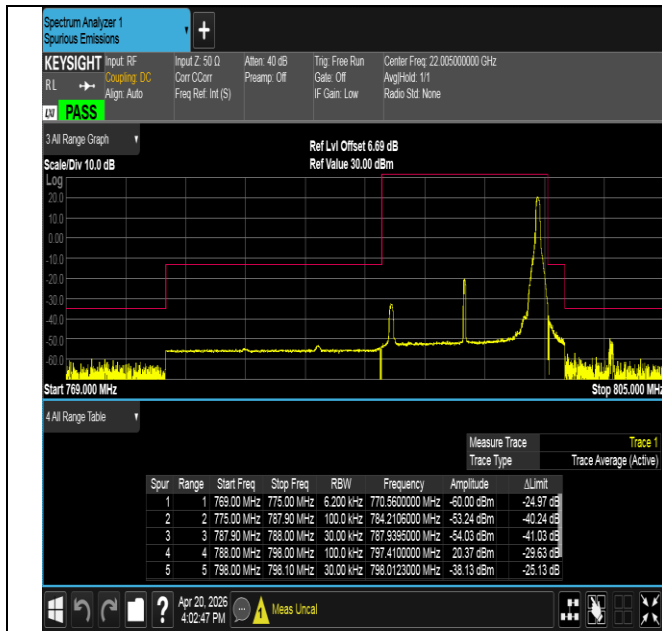
Band14-10MHz-16QAM-23330-1RB#49-PASS
