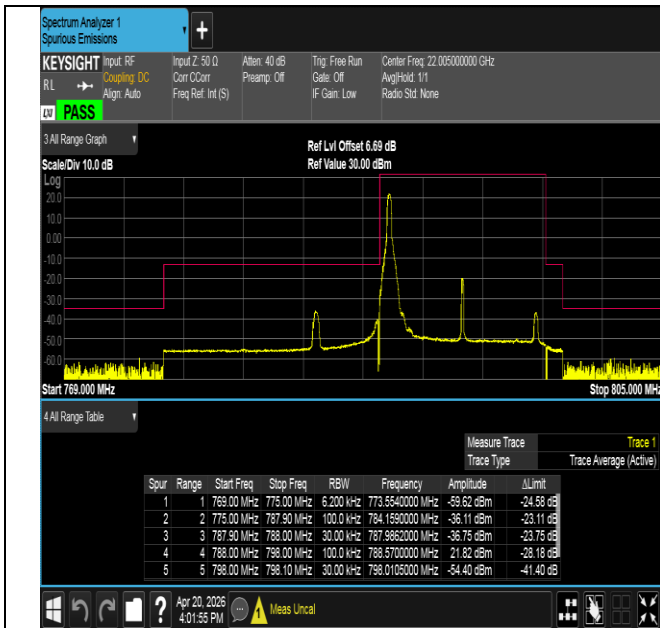
Band14-10MHz-QPSK-23330-1RB#0-PASS
