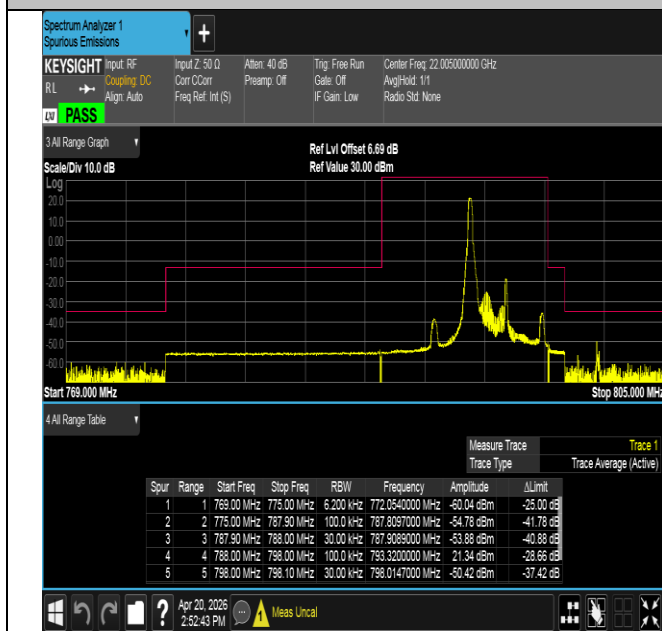
Band14-5MHz-QPSK-23355-1RB#0-PASS
