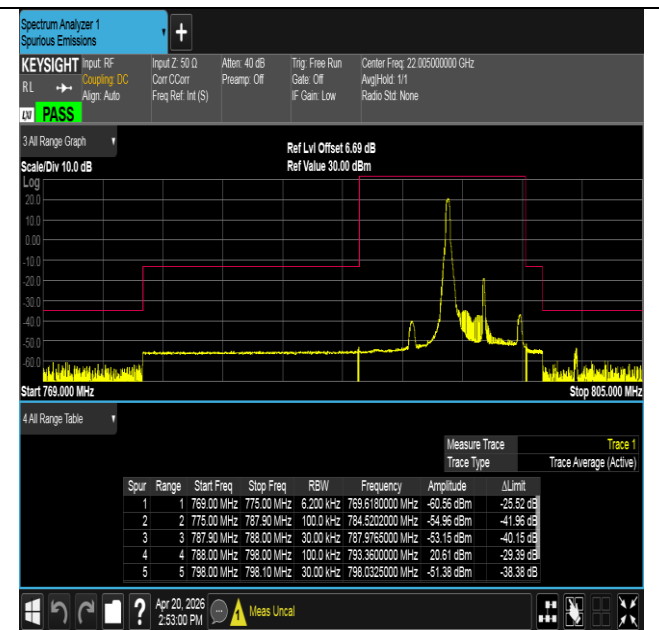
Band14-5MHz-16QAM-23355-1RB#0-PASS
