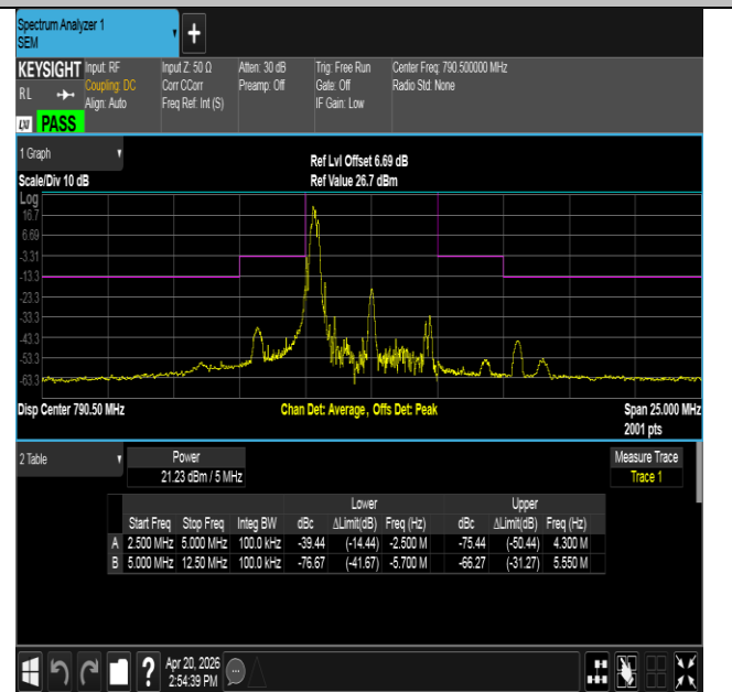
NTNV-Band14-5MHz-16QAM-23305-1RB#0-5.00-12.50-PAS
