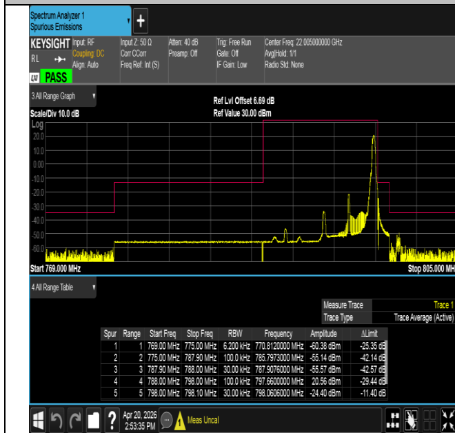
Band14-5MHz-16QAM-23355-1RB#24-PASS
