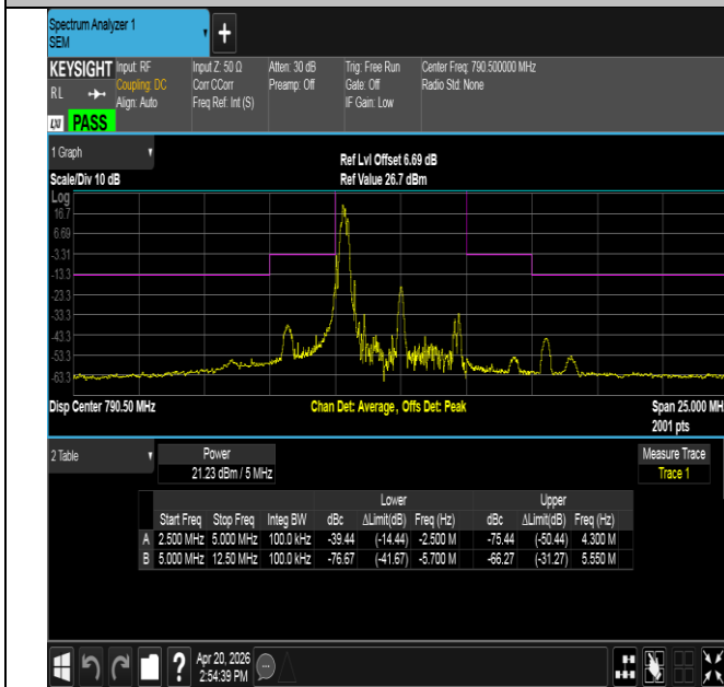
NTNV-Band14-5MHz-16QAM-23305-1RB#0-2.50-5.00-PASS
