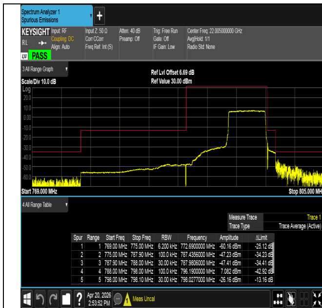
Band14-5MHz-QPSK-23355-25RB#0-PASS
