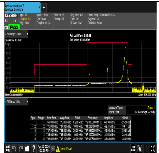
Band14-10MHz-QPSK-23330-1RB#49-PASS
