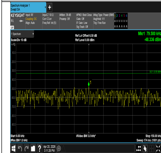
Band14-5MHz-QPSK-23330-25RB#0-0.009~0.15-PASS
