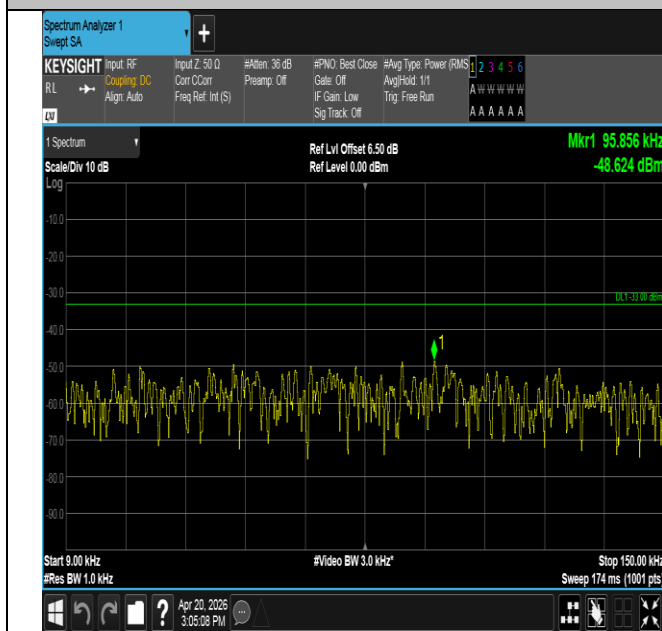
Band14-5MHz-16QAM-23305-1RB#24-0.009~0.15-PASS
