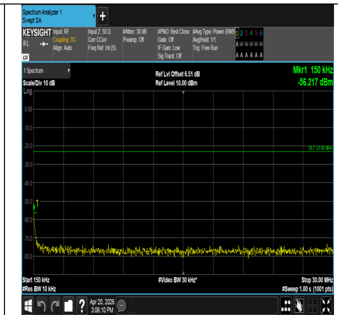
Band14-5MHz-QPSK-23305-25RB#0-0.15~30-PASS
