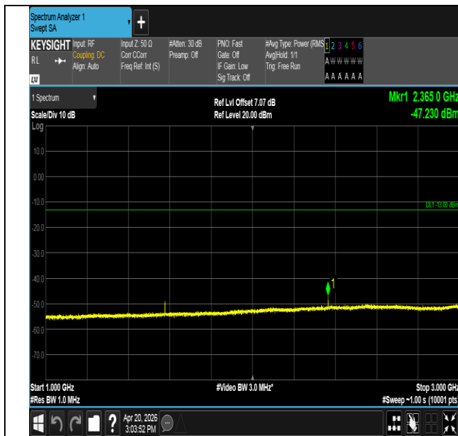
Band14-5MHz-16QAM-23305-1RB#0-1000~3000-PASS
