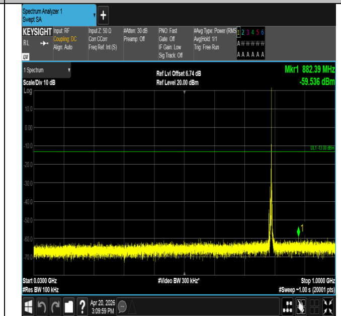
Band14-5MHz-QPSK-23330-1RB#24-30~1000-PASS
