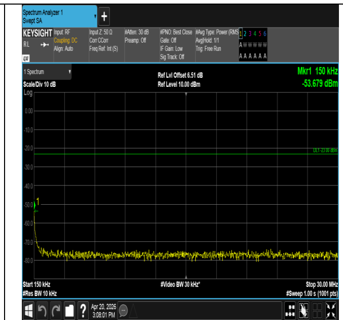
Band14-5MHz-QPSK-23330-1RB#0-0.15~30-PASS
