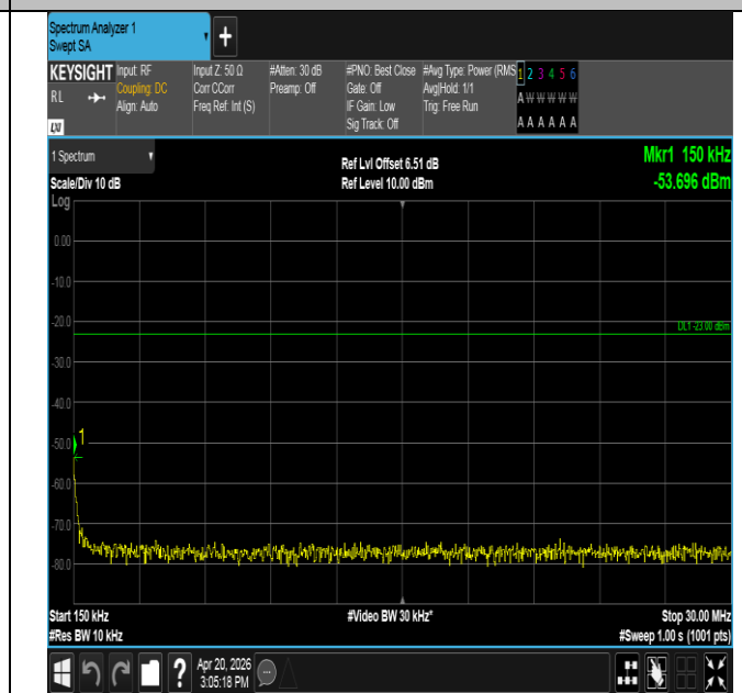
Band14-5MHz-16QAM-23305-1RB#24-0.15~30-PASS
