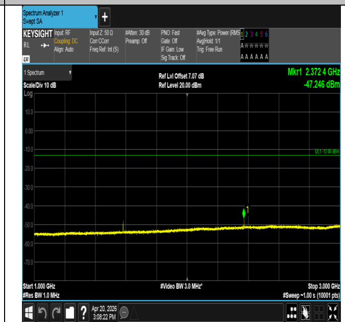
Band14-5MHz-QPSK-23330-1RB#0-1000~3000-PASS
