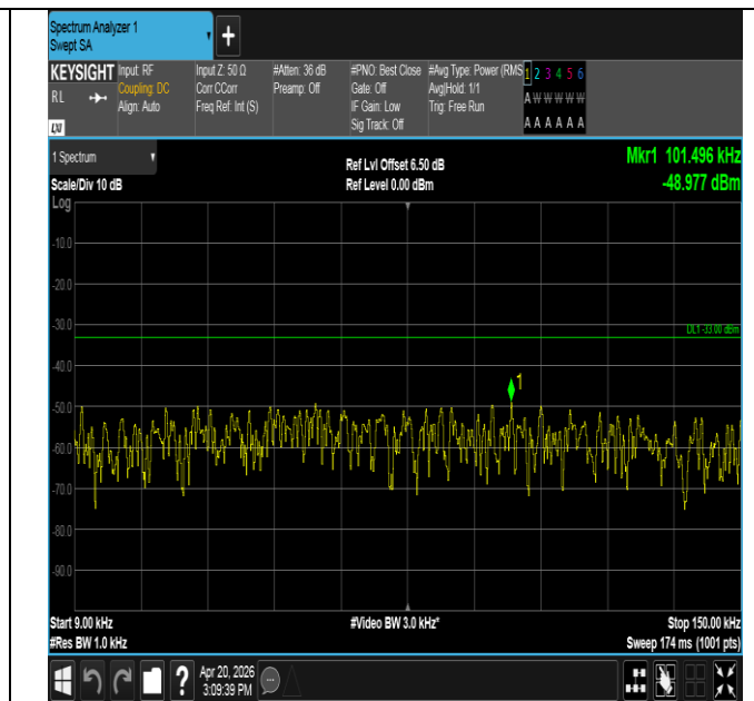
Band14-5MHz-QPSK-23330-1RB#24-0.009~0.15-PASS
