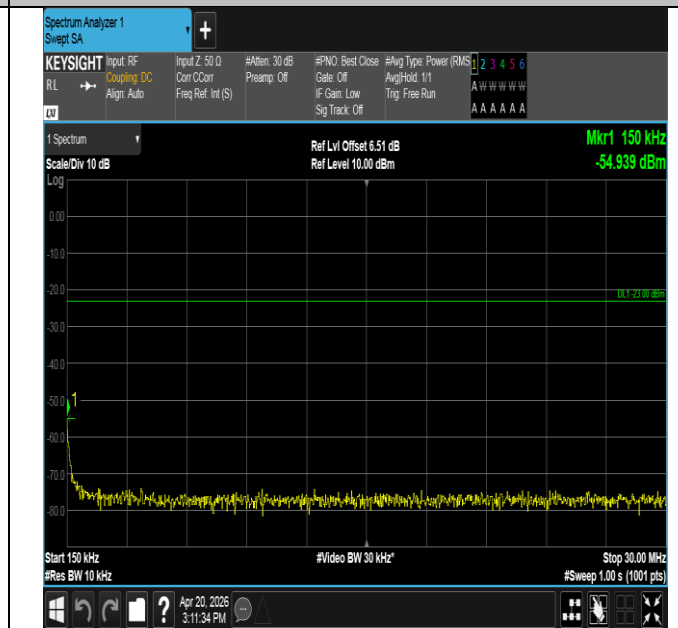
Band14-5MHz-QPSK-23330-25RB#0-0.15~30-PASS
