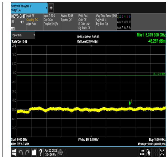
Band14-5MHz-16QAM-23305-1RB#0-3000~10000-PASS
