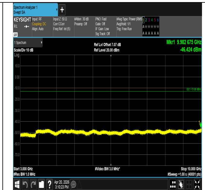
Band14-5MHz-QPSK-23330-1RB#24-3000~10000-PASS
