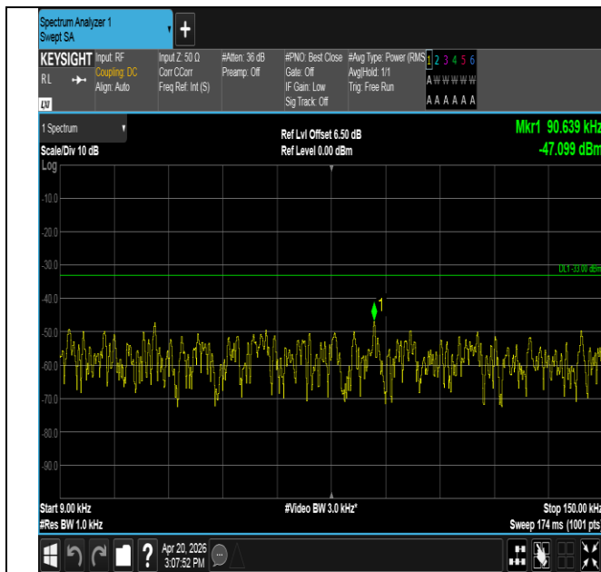
Band14-5MHz-QPSK-23330-1RB#0-0.009~0.15-PASS
