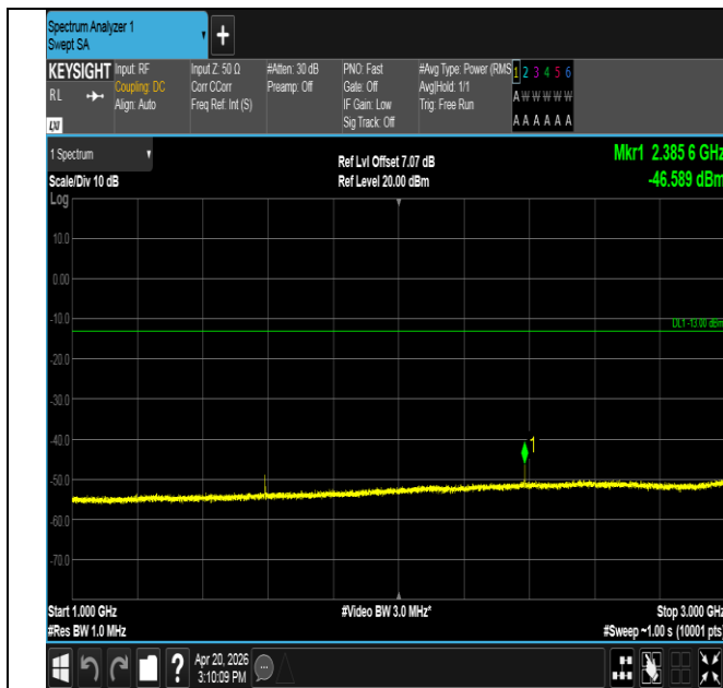
Band14-5MHz-QPSK-23330-1RB#24-1000~3000-PASS
