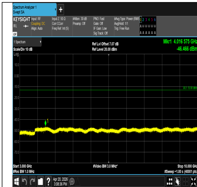
Band14-5MHz-QPSK-23330-1RB#0-3000~10000-PASS
