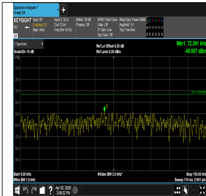
Band14-5MHz-QPSK-23305-25RB#0-0.009~0.15-PASS
