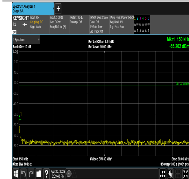
Band14-5MHz-QPSK-23330-1RB#24-0.15~30-PASS
