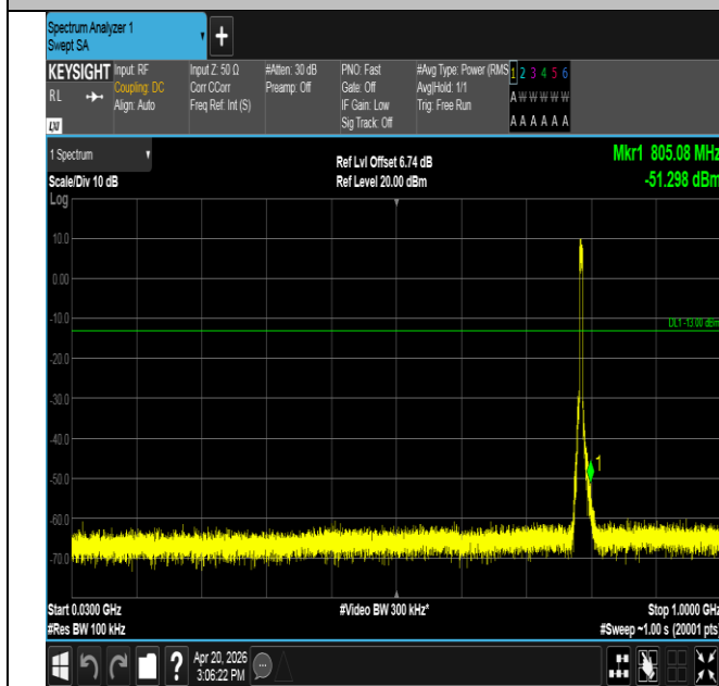
Band14-5MHz-QPSK-23305-25RB#0-30~1000-PASS
