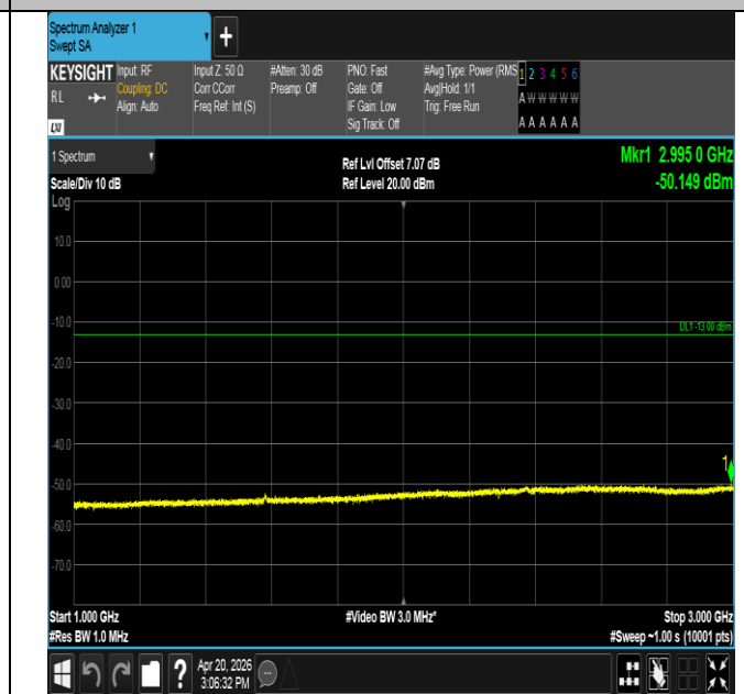
Band14-5MHz-QPSK-23305-25RB#0-1000~3000-PASS
