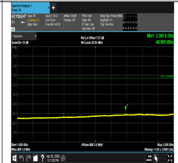
Band14-5MHz-16QAM-23330-1RB#24-1000~3000-PASS
