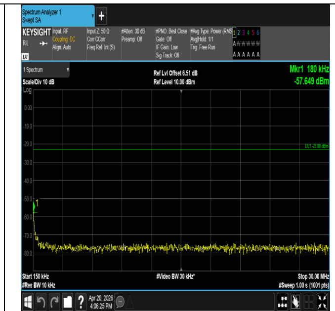
Band14-10MHz-16QAM-23330-1RB#49-0.15~30-PASS
