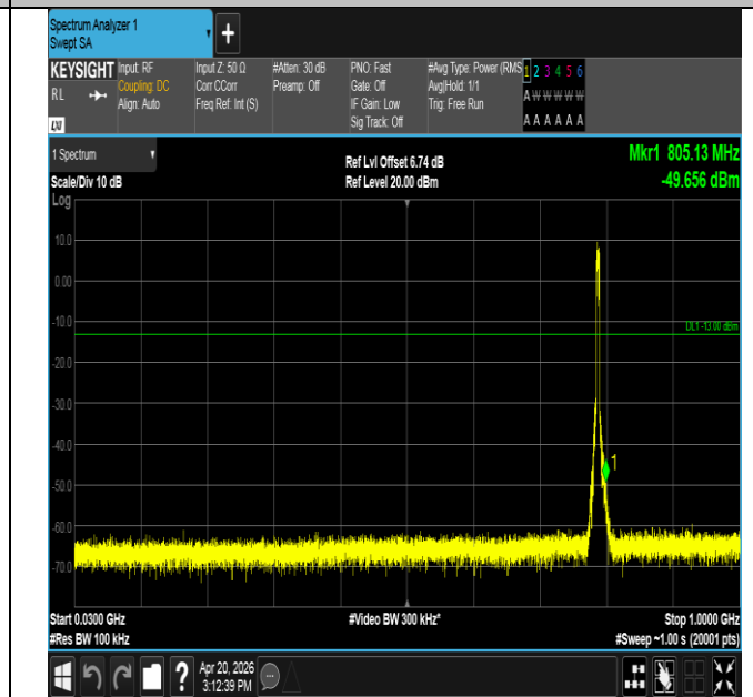
Band14-5MHz-16QAM-23330-25RB#0-30~1000-PASS
