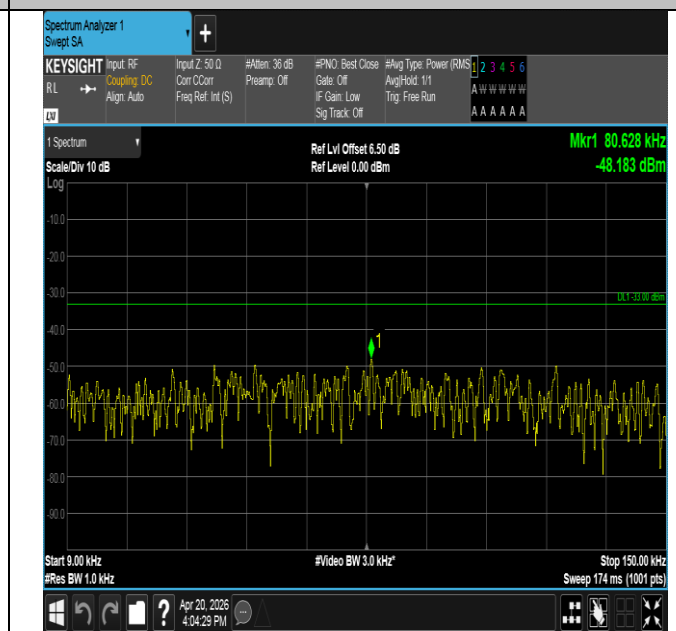
Band14-10MHz-16QAM-23330-1RB#0-0.009~0.15-PASS
