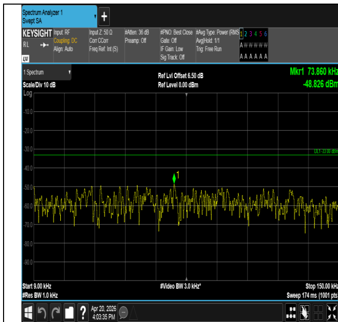
Band14-10MHz-QPSK-23330-1RB#0-0.009~0.15-PASS
