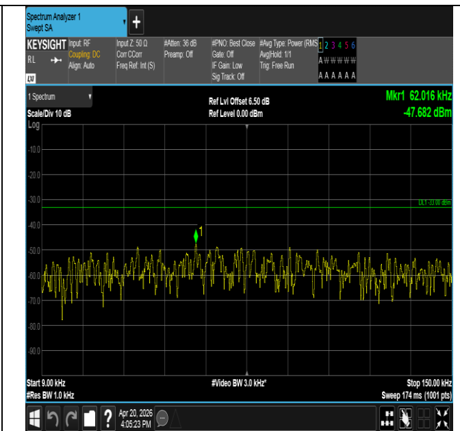
Band14-10MHz-QPSK-23330-1RB#49-0.009~0.15-PASS
