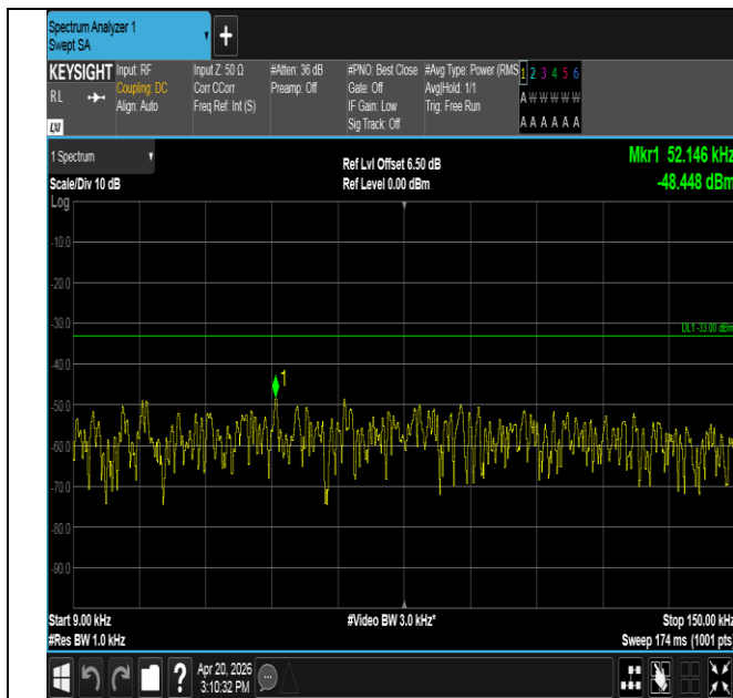
Band14-5MHz-16QAM-23330-1RB#24-0.009~0.15-PASS
