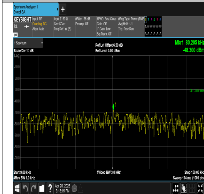
Band14-5MHz-QPSK-23355-1RB#0-0.009~0.15-PASS
