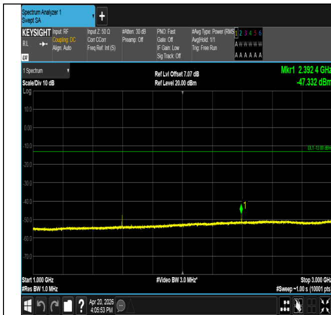
Band14-10MHz-QPSK-23330-1RB#49-1000~3000-PASS
