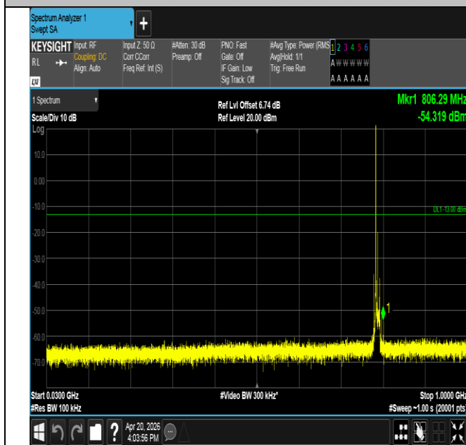
Band14-10MHz-QPSK-23330-1RB#0-30~1000-PASS
