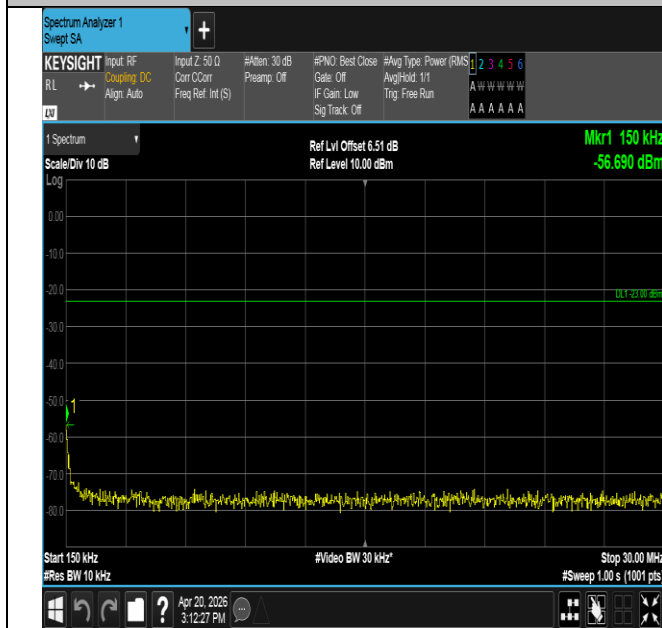
Band14-5MHz-16QAM-23330-25RB#0-0.15~30-PASS
