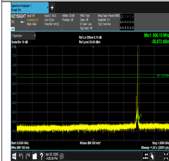
Band14-10MHz-16QAM-23330-1RB#49-30~1000-PASS
