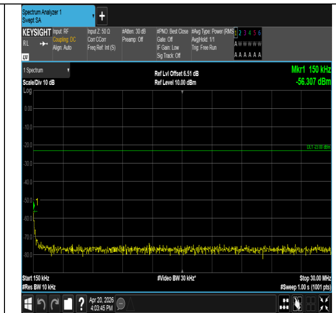
Band14-10MHz-QPSK-23330-1RB#0-0.15~30-PASS
