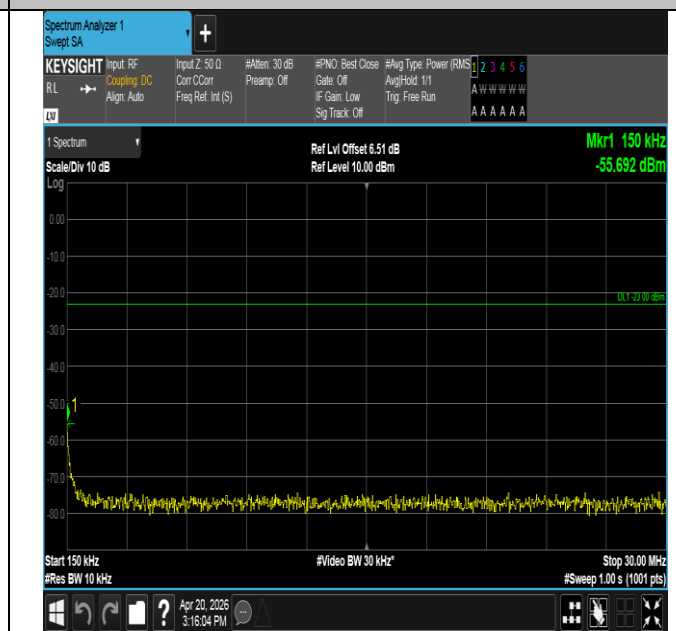
Band14-5MHz-16QAM-23355-1RB#24-0.15~30-PASS
