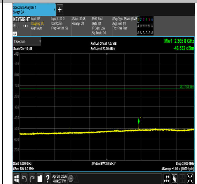
Band14-10MHz-QPSK-23330-1RB#0-1000~3000-PASS
