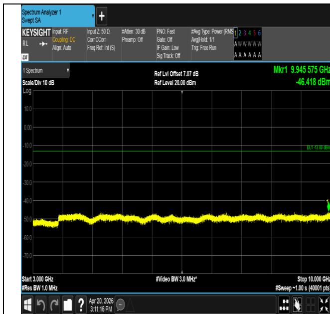
Band14-5MHz-16QAM-23330-1RB#24-3000~10000-PASS
