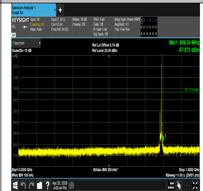
Band14-10MHz-QPSK-23330-1RB#49-30~1000-PASS
