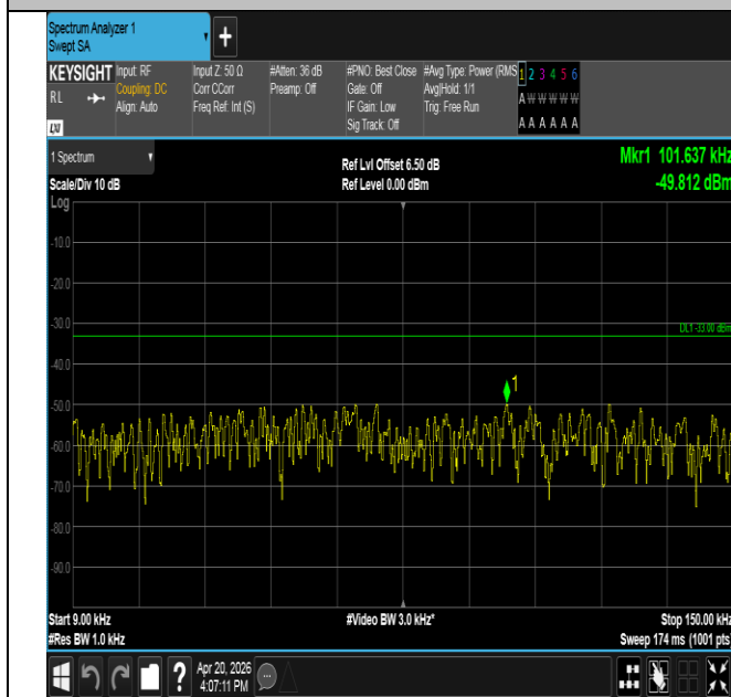
Band14-10MHz-QPSK-23330-50RB#0-0.009~0.15-PASS
