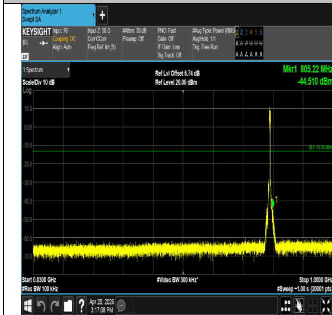
Band14-5MHz-QPSK-23355-25RB#0-30~1000-PASS
