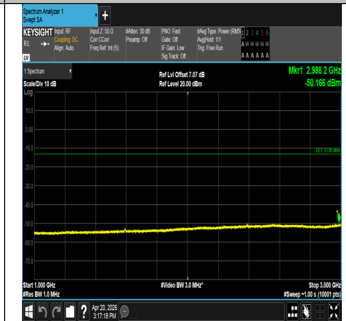
Band14-5MHz-QPSK-23355-25RB#0-1000~3000-PASS
