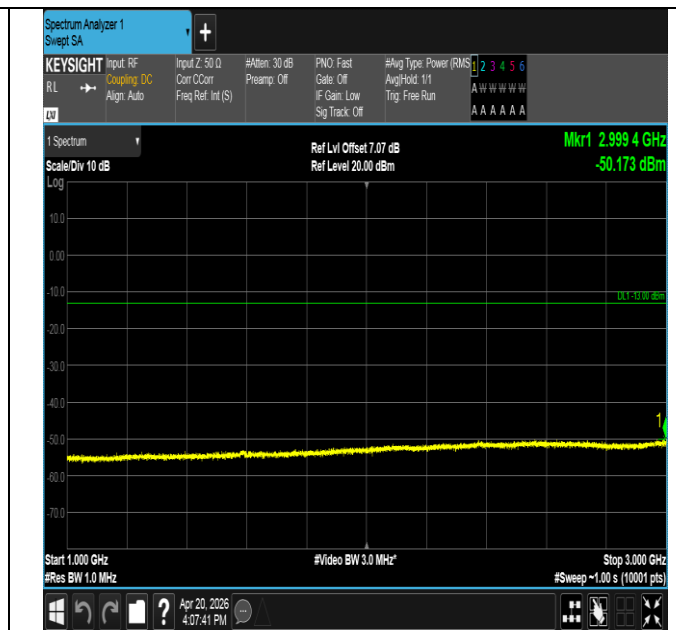
Band14-10MHz-QPSK-23330-50RB#0-1000~3000-PASS
