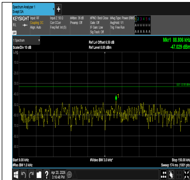
Band14-5MHz-QPSK-23355-25RB#0-0.009~0.15-PASS
