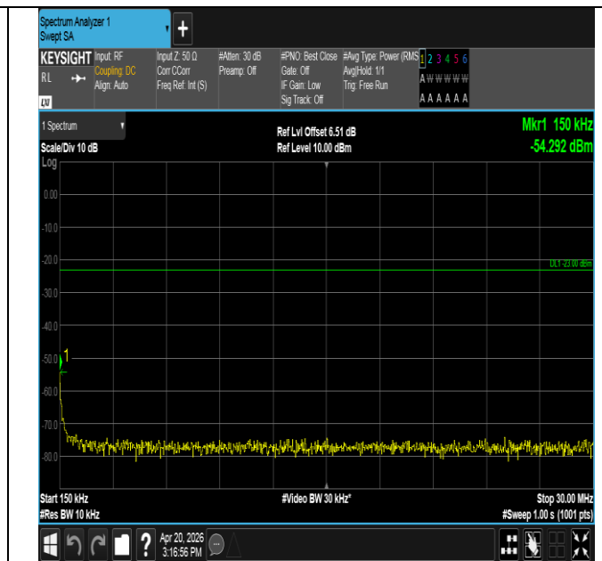
Band14-5MHz-QPSK-23355-25RB#0-0.15~30-PASS
