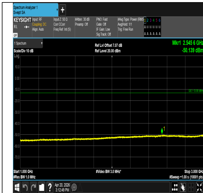
Band14-5MHz-16QAM-23330-25RB#0-1000~3000-PASS
