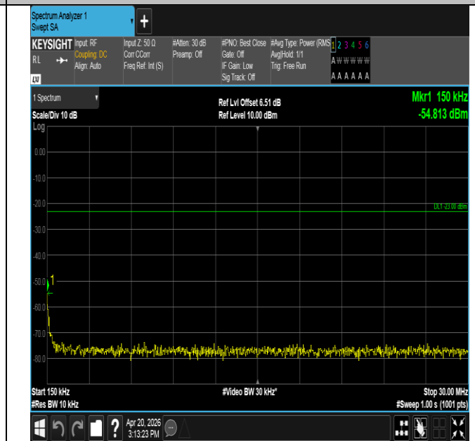
Band14-5MHz-QPSK-23355-1RB#0-0.15~30-PASS
