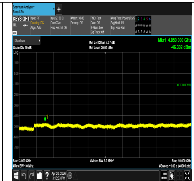
Band14-5MHz-16QAM-23330-25RB#0-3000~10000-PASS
