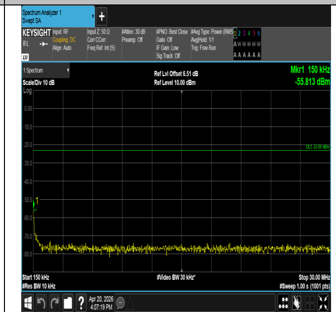
Band14-10MHz-QPSK-23330-50RB#0-0.15~30-PASS
