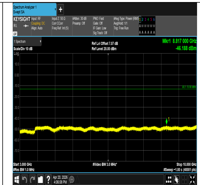
Band14-10MHz-QPSK-23330-1RB#49-3000~10000-PASS
