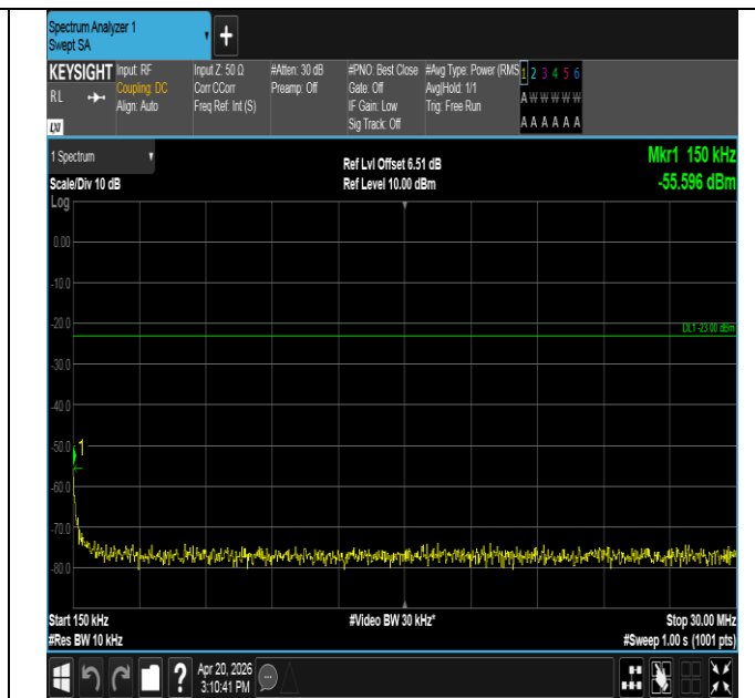
Band14-5MHz-16QAM-23330-1RB#24-0.15~30-PASS
