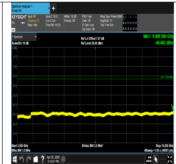
Band14-5MHz-16QAM-23355-1RB#0-3000~10000-PASS
