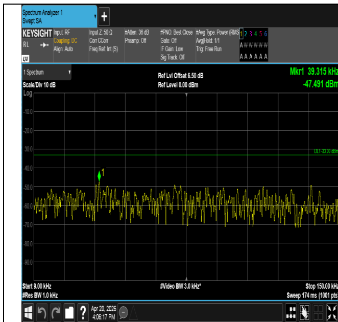
Band14-10MHz-16QAM-23330-1RB#49-0.009~0.15-PASS
