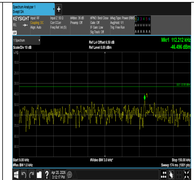
Band14-5MHz-16QAM-23330-25RB#0-0.009~0.15-PASS
