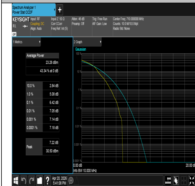
Band17-10MHz-16QAM-23790-1RB#0-PASS
