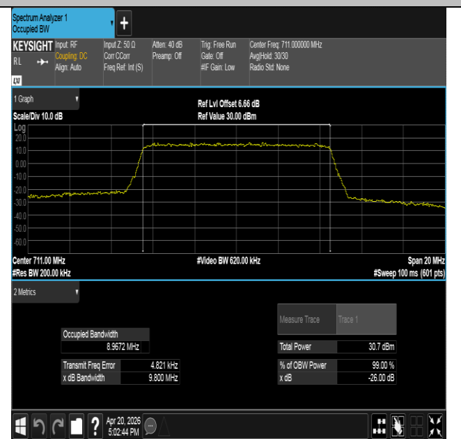
Band17-10MHz-16QAM-23800-50RB#0-PASS
