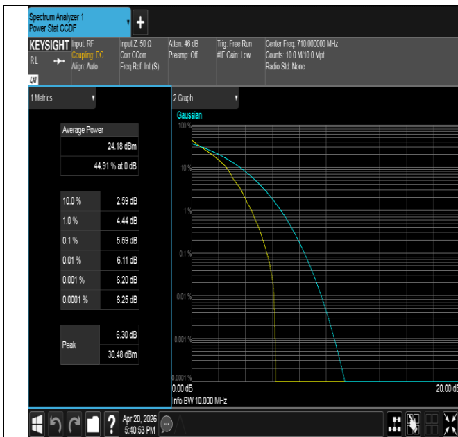
Band17-10MHz-QPSK-23790-1RB#0-PASS
