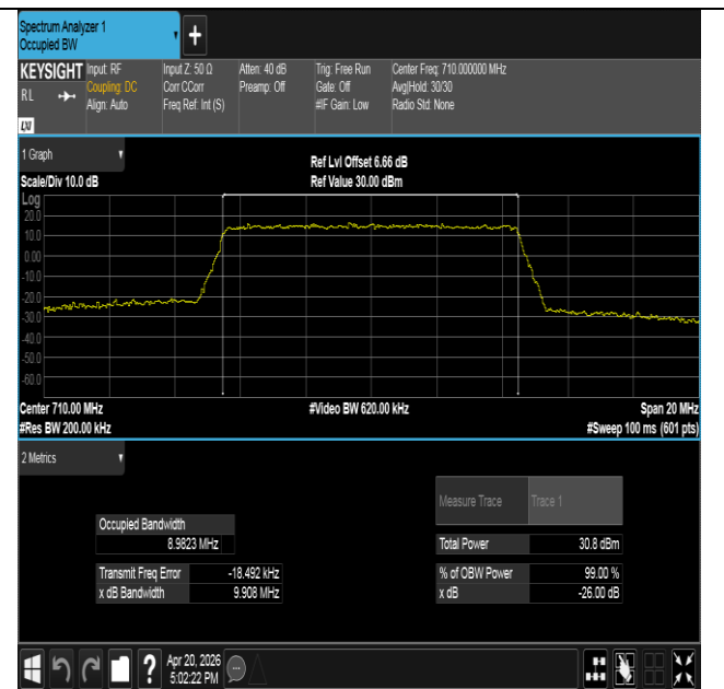
Band17-10MHz-16QAM-23790-50RB#0-PASS
