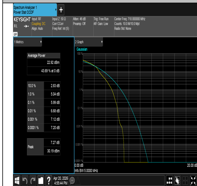
Band17-5MHz-16QAM-23790-1RB#0-PASS
