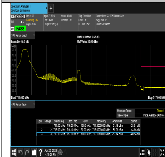
Band17-5MHz-QPSK-23825-1RB#0-PASS
