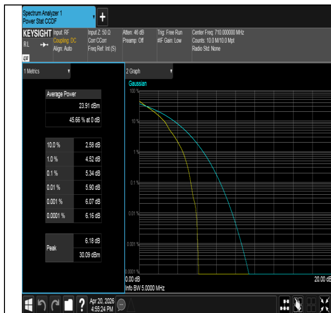
Band17-5MHz-QPSK-23790-1RB#0-PASS
