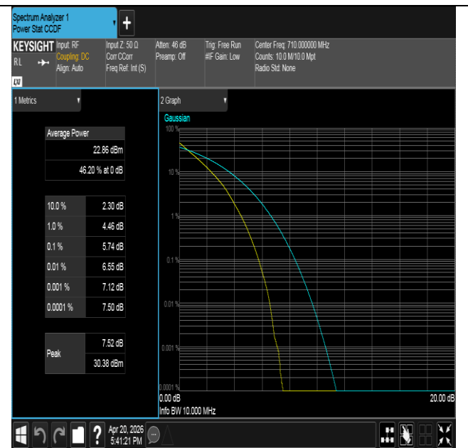
Band17-10MHz-QPSK-23790-50RB#0-PASS
