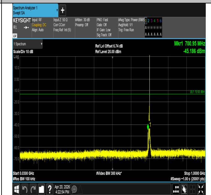
Band17-5MHz-QPSK-23755-1RB#24-30~1000-PASS
