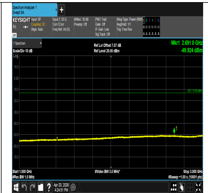
Band17-5MHz-QPSK-23755-25RB#0-1000~3000-PASS
