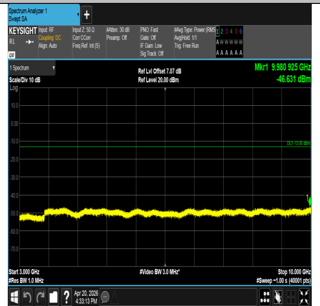
Band17-5MHz-16QAM-23825-1RB#0-3000~10000-PASS
