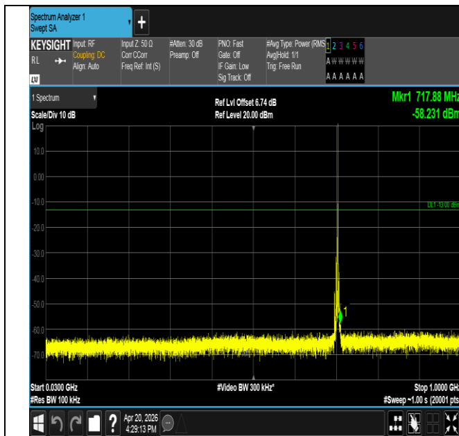
Band17-5MHz-16QAM-23790-1RB#24-30~1000-PASS
