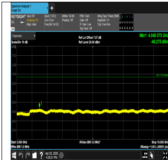
Band17-5MHz-QPSK-23790-25RB#0-3000~10000-PASS
