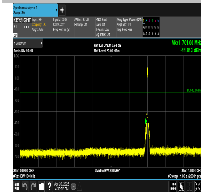
Band17-5MHz-QPSK-23790-25RB#0-30~1000-PASS
