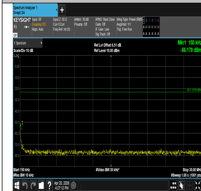
Band17-5MHz-16QAM-23790-1RB#0-0.15~30-PASS
