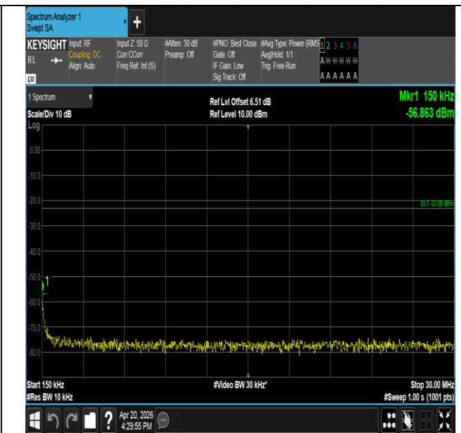
Band17-5MHz-QPSK-23790-25RB#0-0.15~30-PASS
