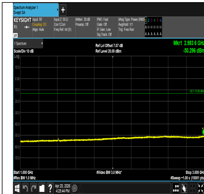
Band17-5MHz-16QAM-23755-25RB#0-1000~3000-PASS
