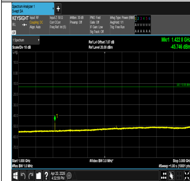
Band17-5MHz-16QAM-23825-1RB#0-1000~3000-PASS
