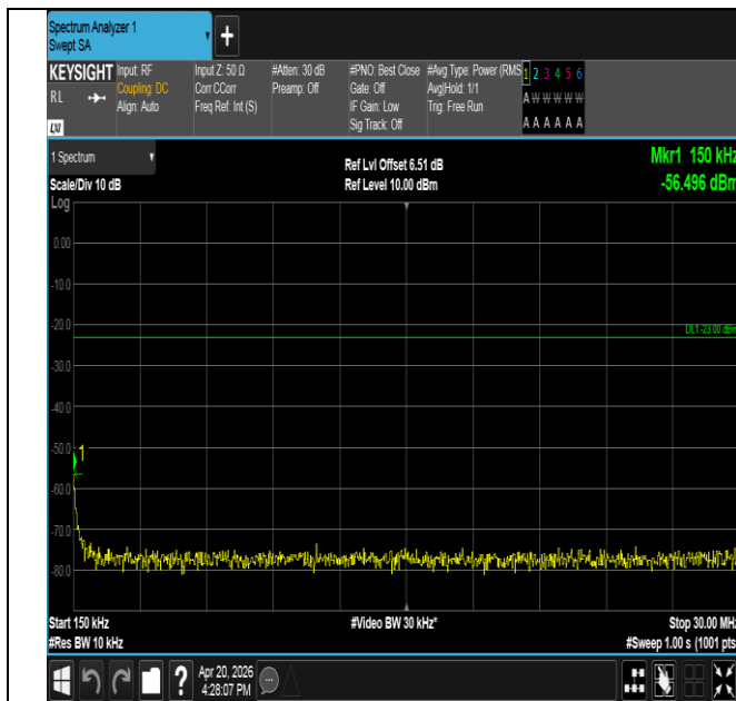
Band17-5MHz-QPSK-23790-1RB#24-0.15~30-PASS
