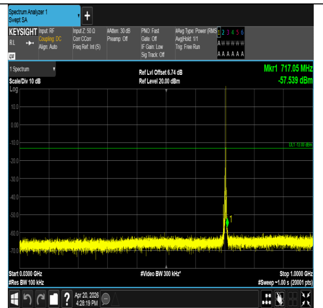
Band17-5MHz-QPSK-23790-1RB#24-30~1000-PASS
