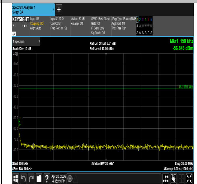
Band17-5MHz-QPSK-23825-25RB#0-0.15~30-PASS
