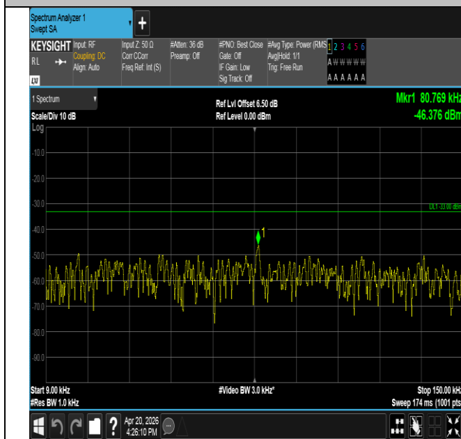
Band17-5MHz-QPSK-23790-1RB#0-0.009~0.15-PASS
