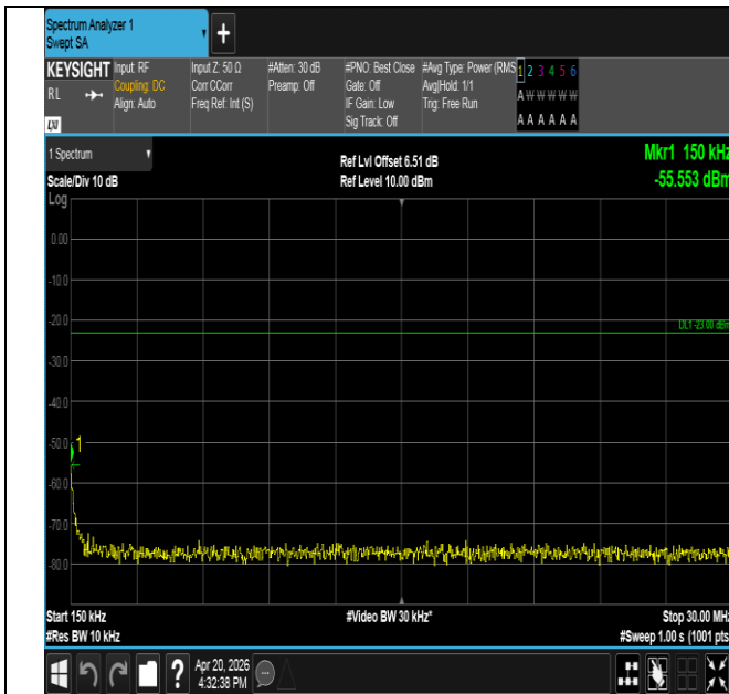
Band17-5MHz-16QAM-23825-1RB#0-0.15~30-PASS
