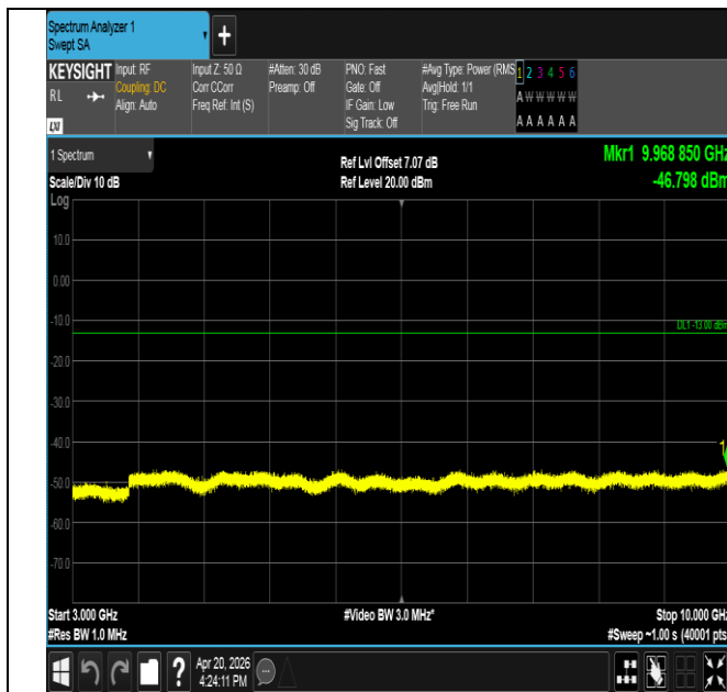
Band17-5MHz-16QAM-23755-1RB#24-3000~10000-PASS
