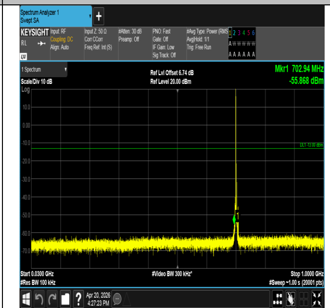
Band17-5MHz-16QAM-23790-1RB#0-30~1000-PASS
