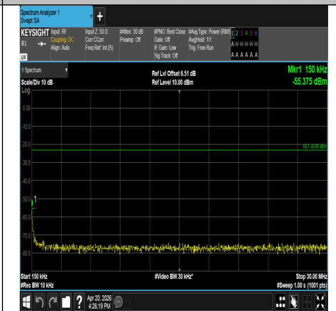
Band17-5MHz-QPSK-23790-1RB#0-0.15~30-PASS
