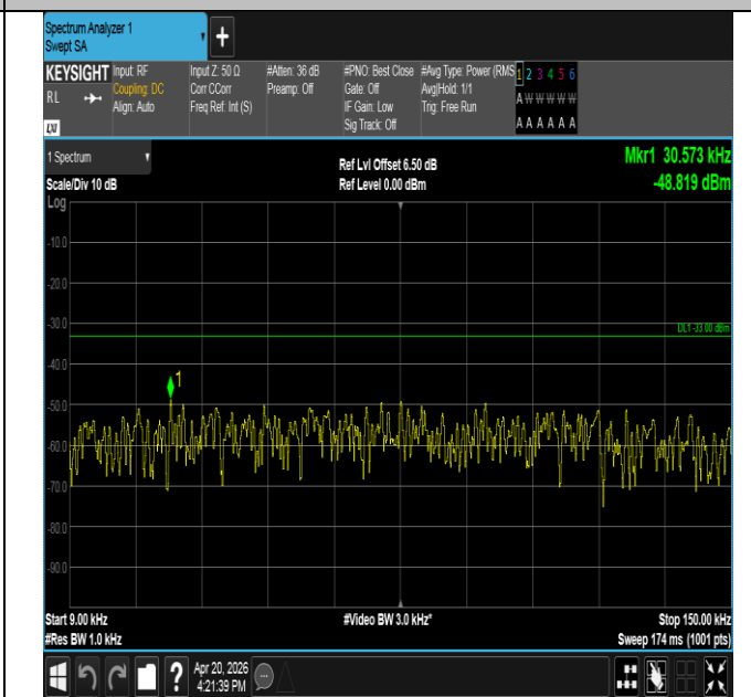
Band17-5MHz-16QAM-23755-1RB#0-0.009~0.15-PASS
