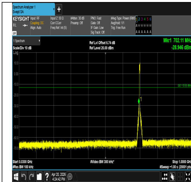
Band17-5MHz-QPSK-23755-25RB#0-30~1000-PASS
