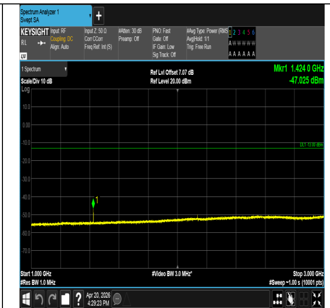
Band17-5MHz-16QAM-23790-1RB#24-1000~3000-PASS
