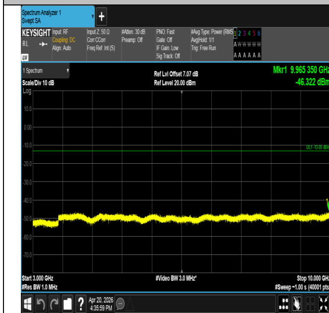
Band17-5MHz-QPSK-23825-25RB#0-3000~10000-PASS
