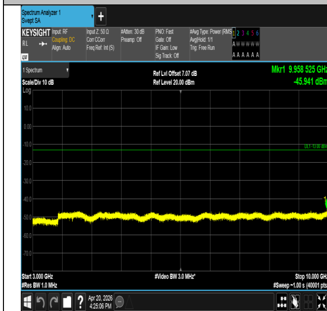
Band17-5MHz-QPSK-23755-25RB#0-3000~10000-PASS
