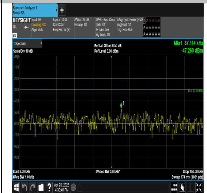
Band17-5MHz-16QAM-23790-25RB#0-0.009~0.15-PASS
