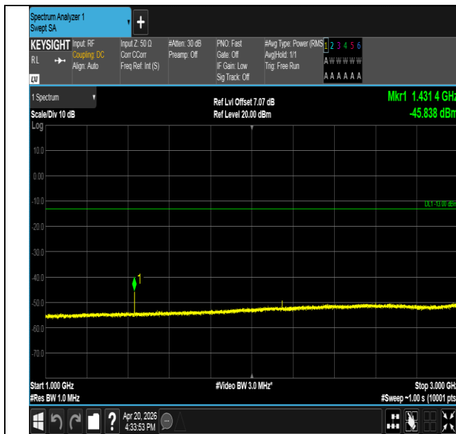
Band17-5MHz-QPSK-23825-1RB#24-1000~3000-PASS
