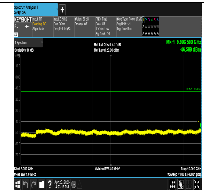
Band17-5MHz-QPSK-23755-1RB#24-3000~10000-PASS
