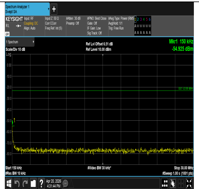
Band17-5MHz-QPSK-23825-1RB#0-0.15~30-PASS
