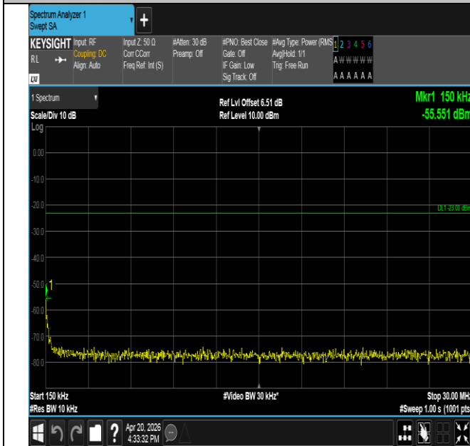
Band17-5MHz-QPSK-23825-1RB#24-0.15~30-PASS
