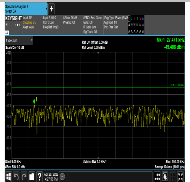
Band17-5MHz-QPSK-23790-1RB#24-0.009~0.15-PASS
