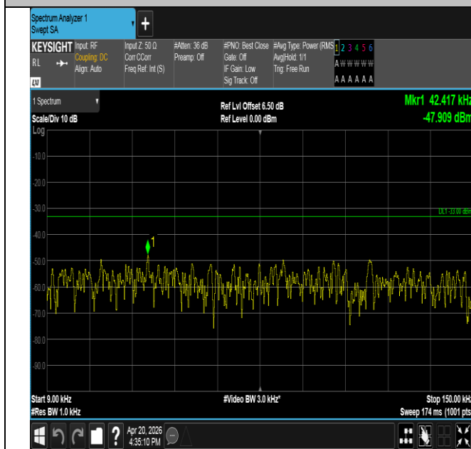
Band17-5MHz-QPSK-23825-25RB#0-0.009~0.15-PASS
