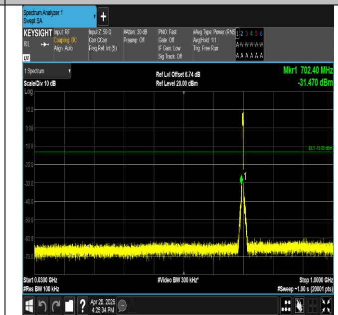
Band17-5MHz-16QAM-23755-25RB#0-30~1000-PASS
