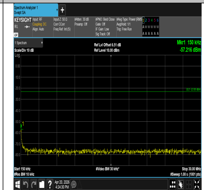
Band17-5MHz-QPSK-23755-25RB#0-0.15~30-PASS
