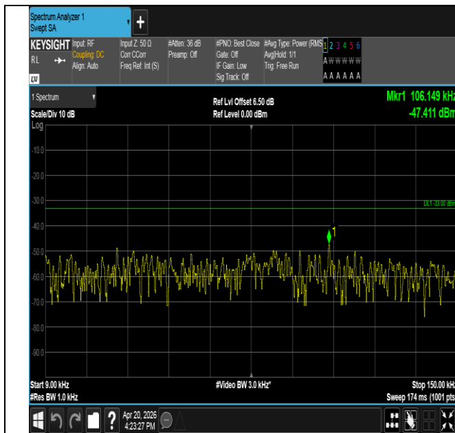
Band17-5MHz-16QAM-23755-1RB#24-0.009~0.15-PASS
