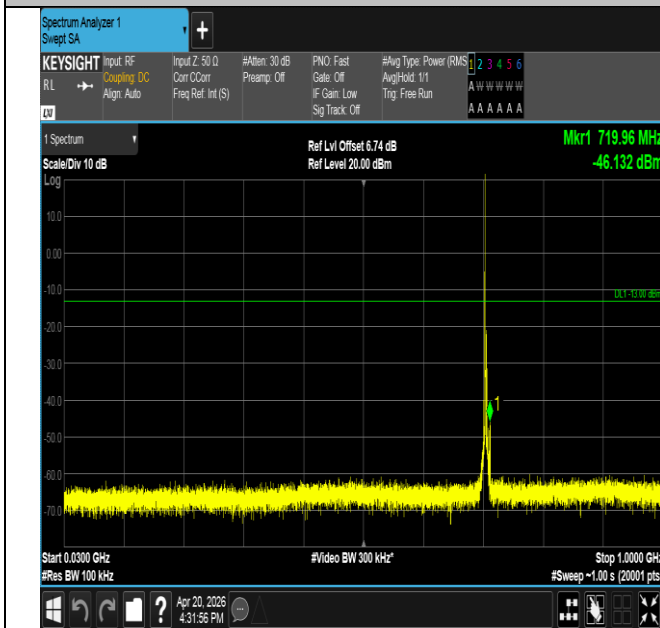
Band17-5MHz-QPSK-23825-1RB#0-30~1000-PASS
