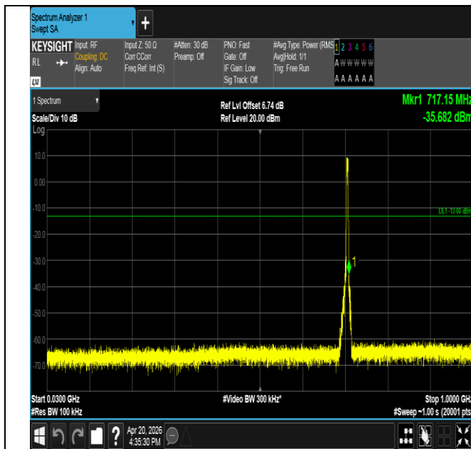
Band17-5MHz-QPSK-23825-25RB#0-30~1000-PASS
