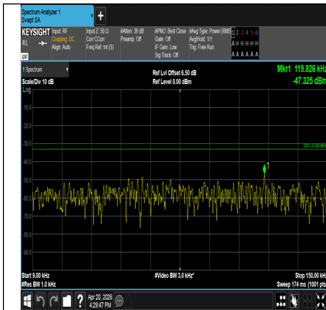
Band17-5MHz-QPSK-23790-25RB#0-0.009~0.15-PASS
