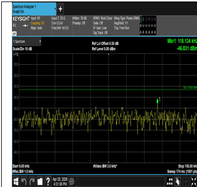
Band17-5MHz-QPSK-23825-1RB#0-0.009~0.15-PASS
