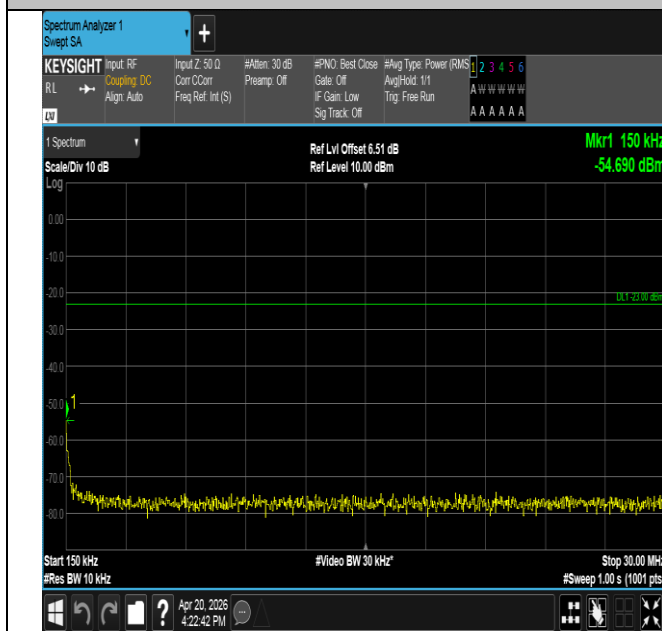
Band17-5MHz-QPSK-23755-1RB#24-0.15~30-PASS
