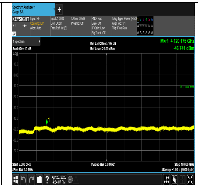
Band17-5MHz-QPSK-23825-1RB#24-3000~10000-PASS
