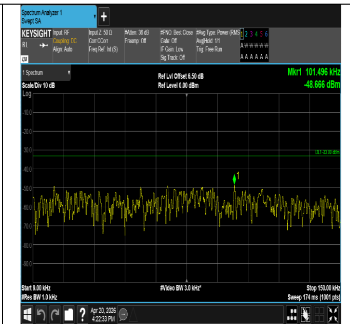
Band17-5MHz-QPSK-23755-1RB#24-0.009~0.15-PASS
