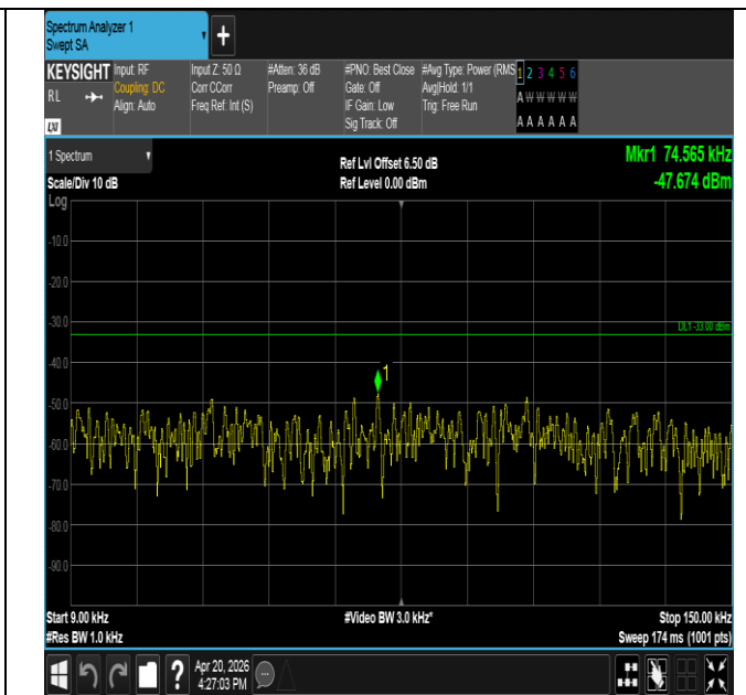
Band17-5MHz-16QAM-23790-1RB#0-0.009~0.15-PASS
