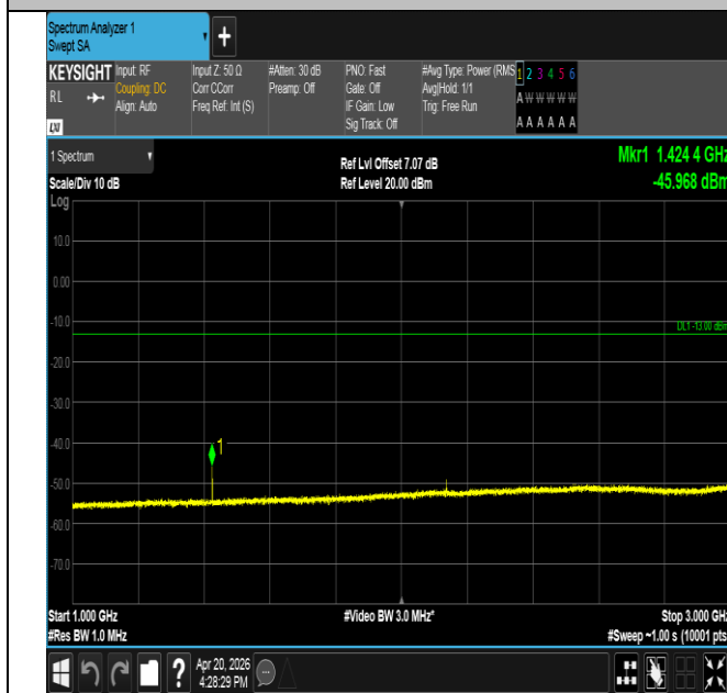
Band17-5MHz-QPSK-23790-1RB#24-1000~3000-PASS
