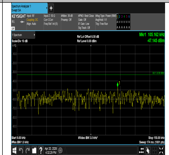
Band17-5MHz-16QAM-23825-1RB#0-0.009~0.15-PASS
