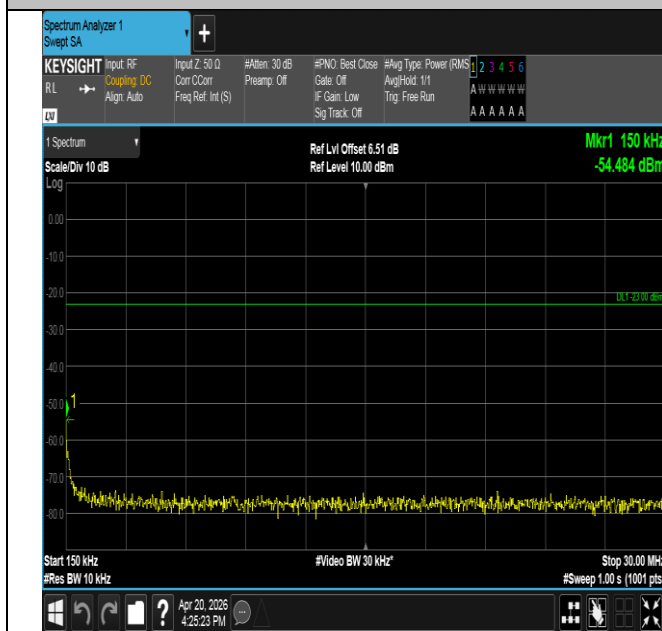
Band17-5MHz-16QAM-23755-25RB#0-0.15~30-PASS
