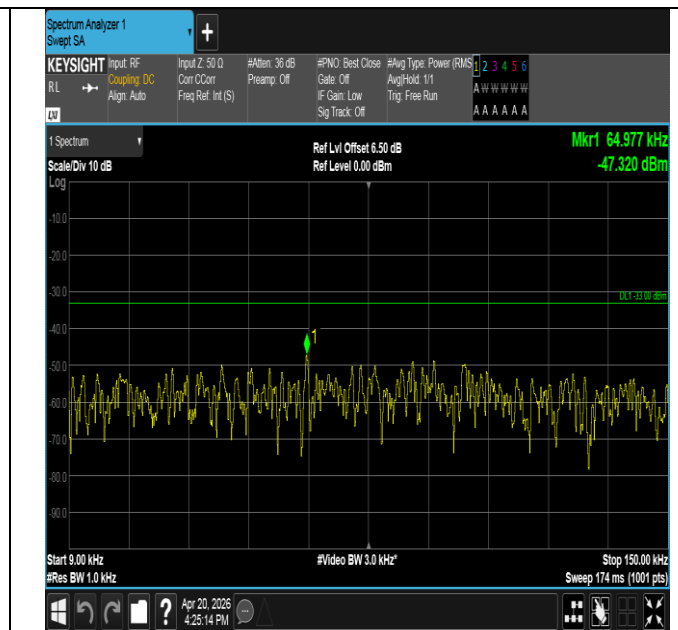
Band17-5MHz-16QAM-23755-25RB#0-0.009~0.15-PASS
