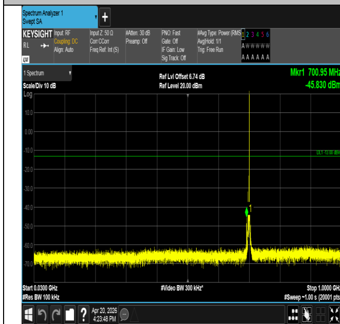
Band17-5MHz-16QAM-23755-1RB#24-30~1000-PASS
