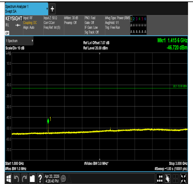
Band17-5MHz-QPSK-23790-1RB#0-1000~3000-PASS
