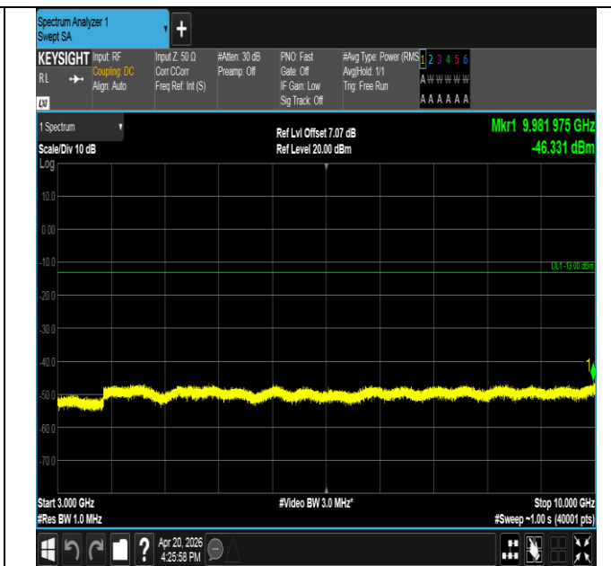
Band17-5MHz-16QAM-23755-25RB#0-3000~10000-PASS
