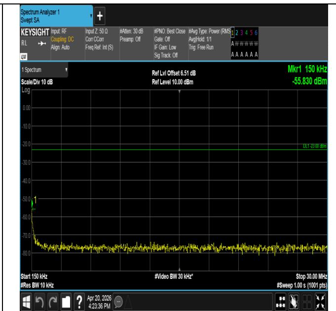
Band17-5MHz-16QAM-23755-1RB#24-0.15~30-PASS
