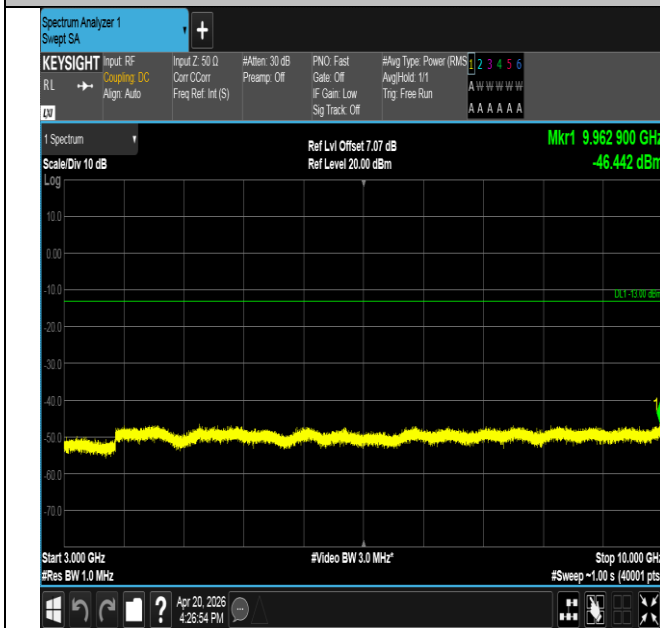
Band17-5MHz-QPSK-23790-1RB#0-3000~10000-PASS
