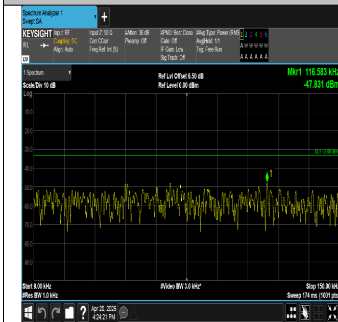
Band17-5MHz-QPSK-23755-25RB#0-0.009~0.15-PASS
