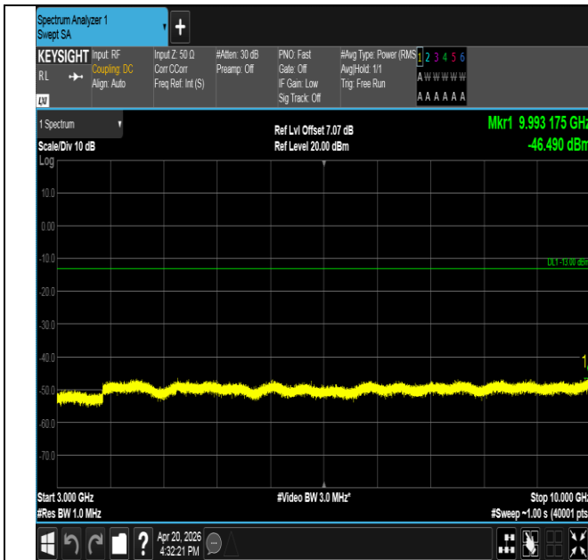
Band17-5MHz-QPSK-23825-1RB#0-3000~10000-PASS
