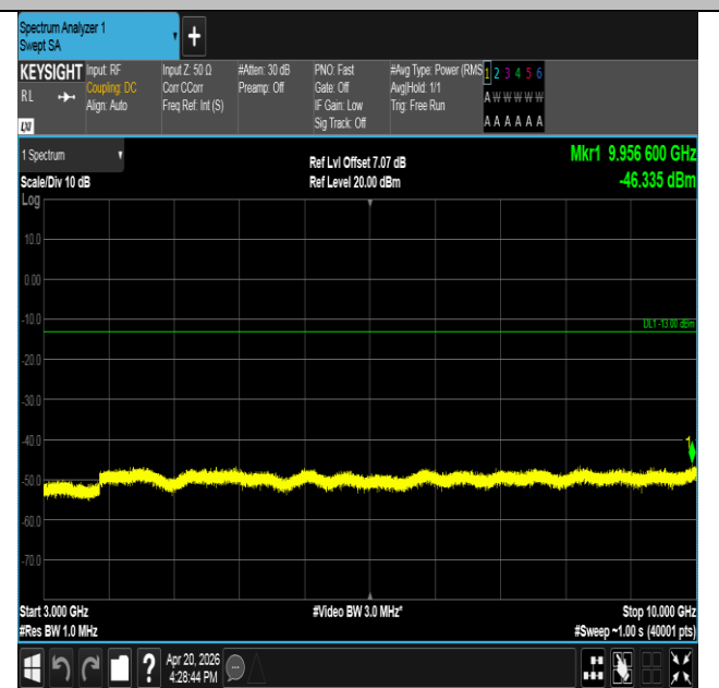
Band17-5MHz-QPSK-23790-1RB#24-3000~10000-PASS
