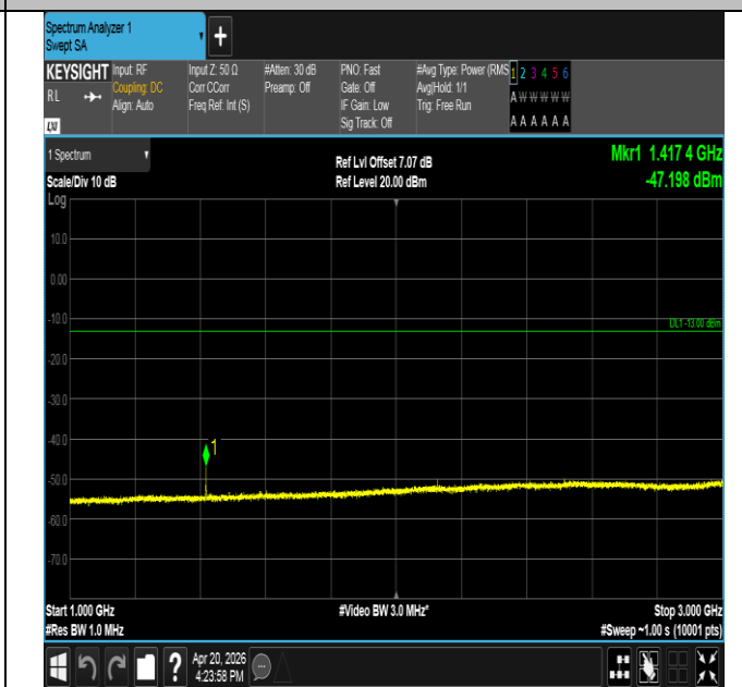
Band17-5MHz-16QAM-23755-1RB#24-1000~3000-PASS
