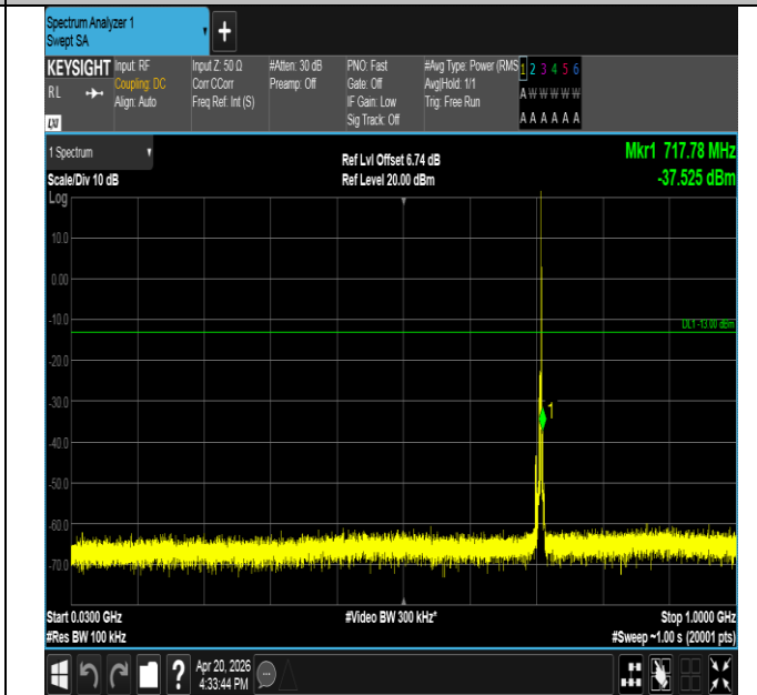
Band17-5MHz-QPSK-23825-1RB#24-30~1000-PASS
