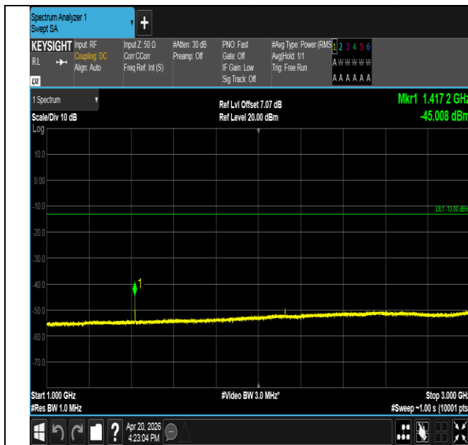
Band17-5MHz-QPSK-23755-1RB#24-1000~3000-PASS
