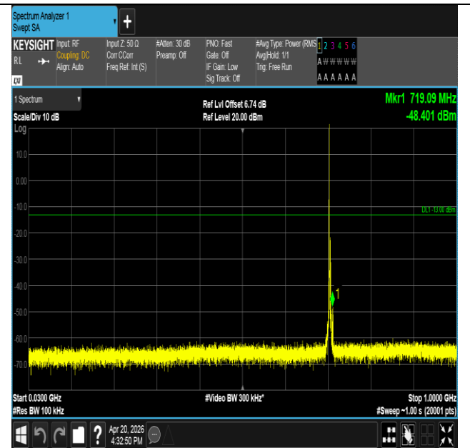
Band17-5MHz-16QAM-23825-1RB#0-30~1000-PASS
