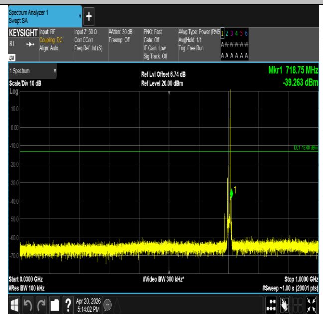
Band17-10MHz-QPSK-23790-1RB#49-30~1000-PASS
