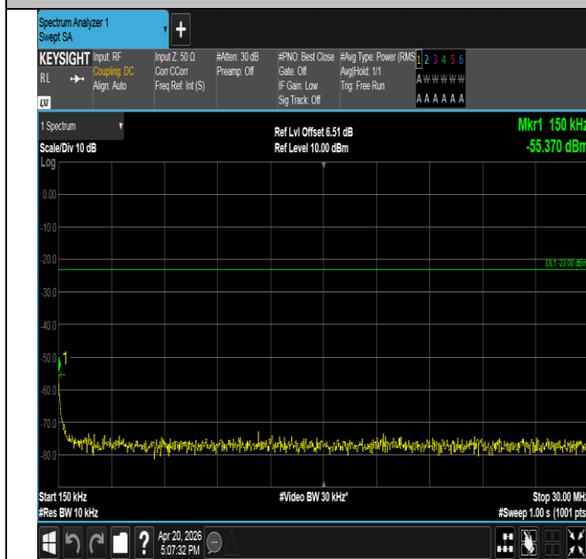
Band17-10MHz-16QAM-23780-1RB#0-0.15~30-PASS
