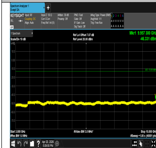
Band17-10MHz-16QAM-23780-1RB#49-3000~10000-PASS
