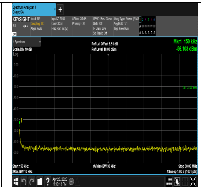
Band17-10MHz-QPSK-23780-50RB#0-0.15~30-PASS
