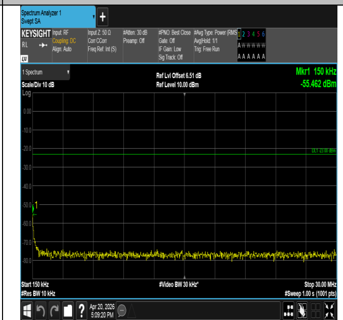
Band17-10MHz-16QAM-23780-1RB#49-0.15~30-PASS
