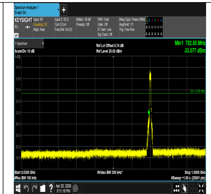
Band17-10MHz-16QAM-23780-50RB#0-30~1000-PASS
