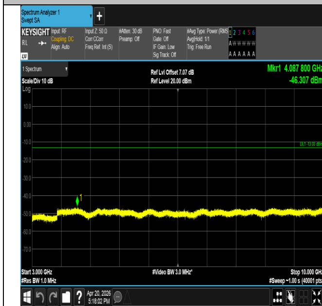
Band17-10MHz-QPSK-23800-1RB#0-3000~10000-PASS
