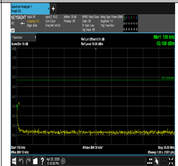
Band17-10MHz-QPSK-23790-50RB#0-0.15~30-PASS
