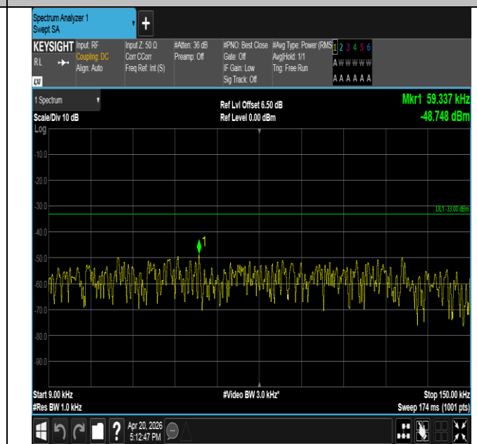
Band17-10MHz-16QAM-23790-1RB#0-0.009~0.15-PASS
