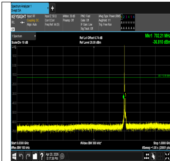
Band17-10MHz-QPSK-23800-1RB#0-30~1000-PASS
