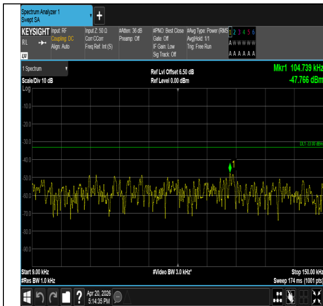
Band17-10MHz-16QAM-23790-1RB#49-0.009~0.15-PASS
