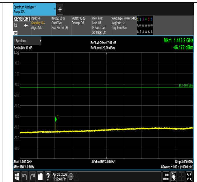
Band17-10MHz-QPSK-23800-1RB#0-1000~3000-PASS
