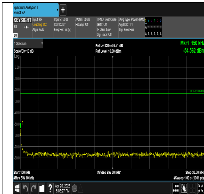
Band17-10MHz-QPSK-23780-1RB#49-0.15~30-PASS
