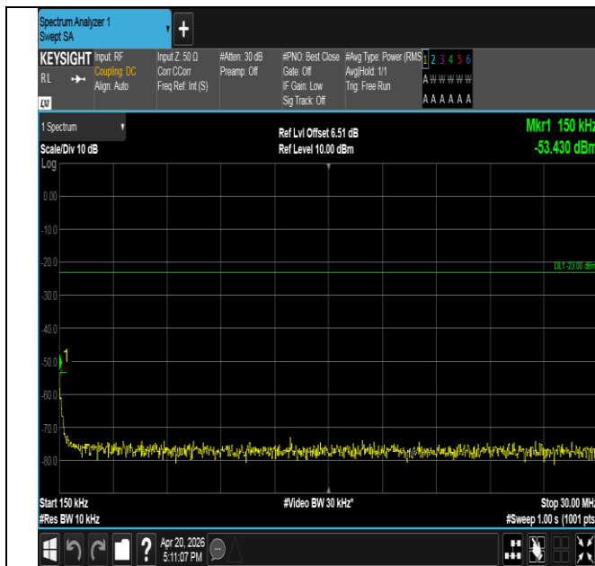
Band17-10MHz-16QAM-23780-50RB#0-0.15~30-PASS
