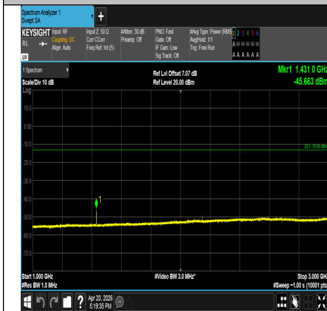
Band17-10MHz-QPSK-23800-1RB#49-1000~3000-PASS
