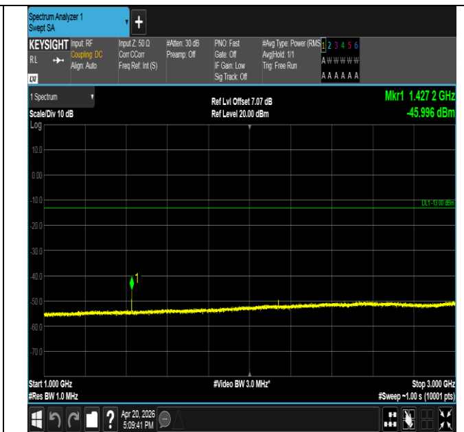
Band17-10MHz-16QAM-23780-1RB#49-1000~3000-PASS
