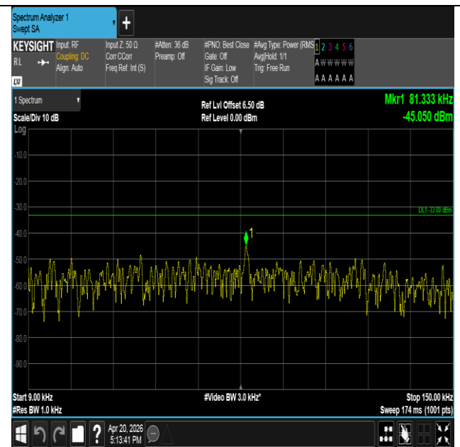
Band17-10MHz-QPSK-23790-1RB#49-0.009~0.15-PASS
