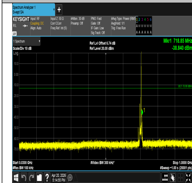
Band17-10MHz-16QAM-23790-1RB#49-30~1000-PASS
