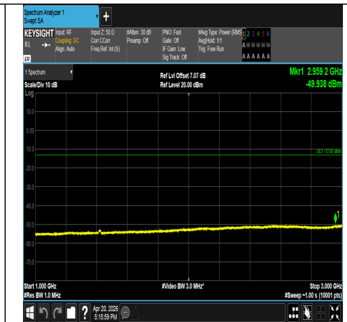
Band17-10MHz-QPSK-23790-50RB#0-1000~3000-PASS
