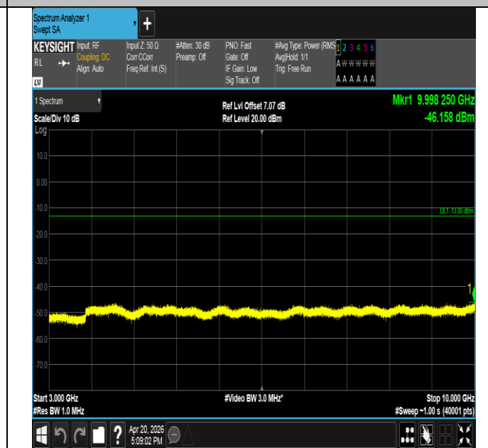
Band17-10MHz-QPSK-23780-1RB#49-3000~10000-PASS
