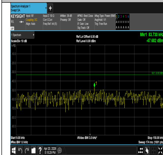
Band17-10MHz-QPSK-23790-50RB#0-0.009~0.15-PASS
