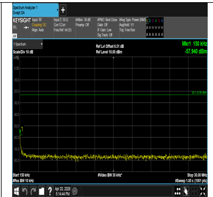
Band17-10MHz-16QAM-23790-1RB#49-0.15~30-PASS
