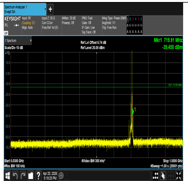
Band17-10MHz-QPSK-23800-1RB#49-30~1000-PASS
