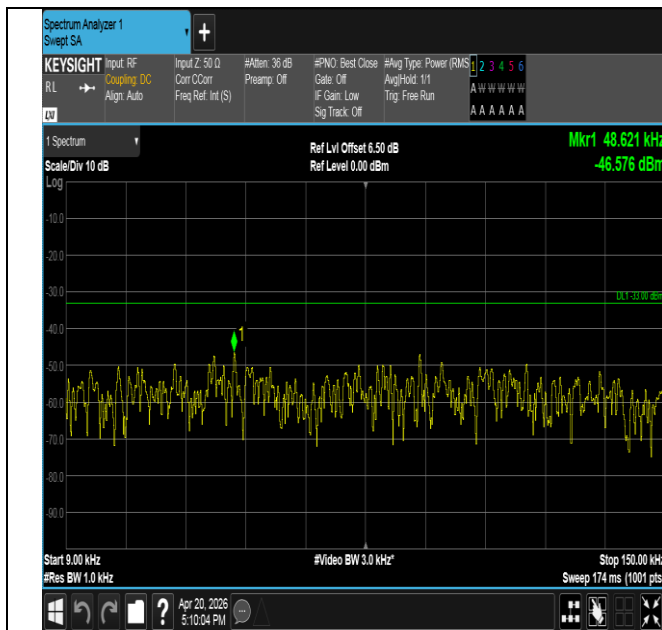
Band17-10MHz-QPSK-23780-50RB#0-0.009~0.15-PASS
