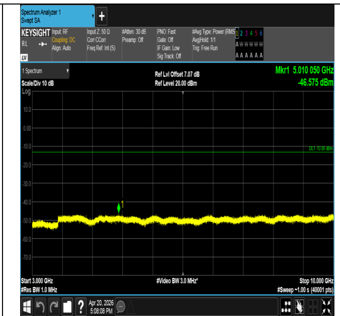
Band17-10MHz-16QAM-23780-1RB#0-3000~10000-PASS
