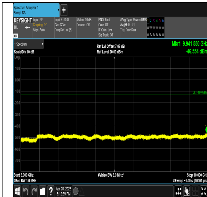
Band17-10MHz-QPSK-23790-1RB#0-3000~10000-PASS
