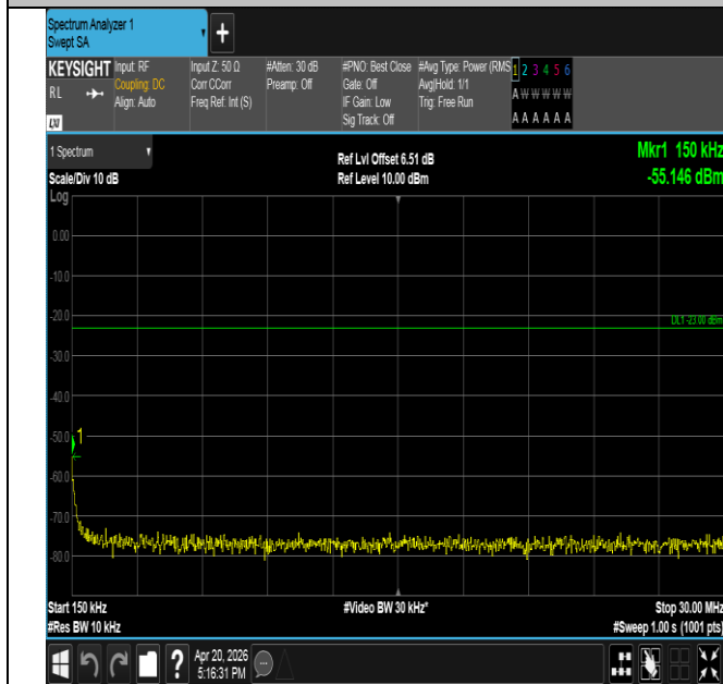
Band17-10MHz-16QAM-23790-50RB#0-0.15~30-PASS
