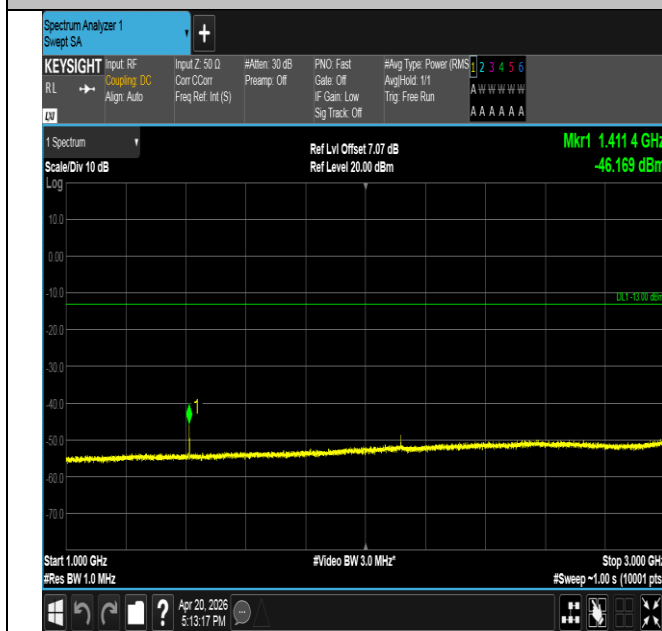
Band17-10MHz-16QAM-23790-1RB#0-1000~3000-PASS
