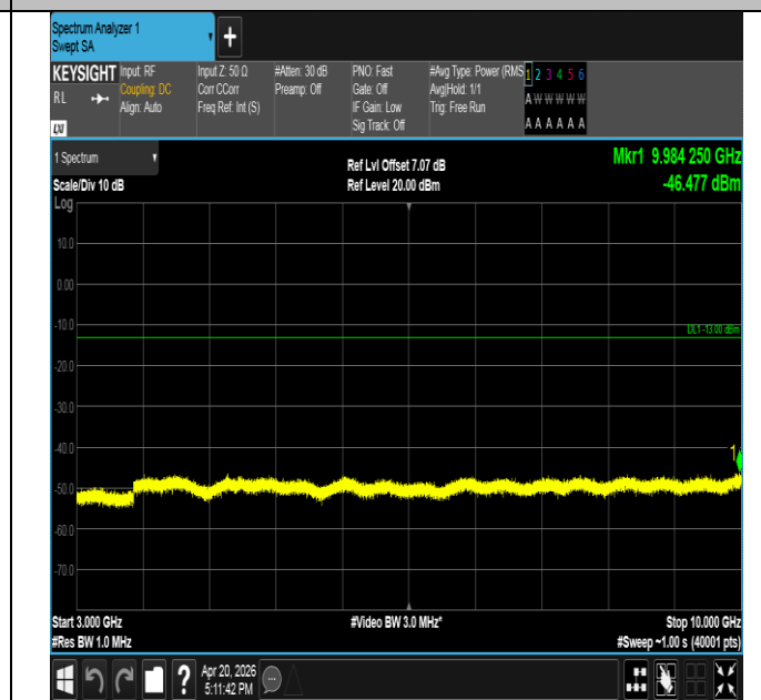
Band17-10MHz-16QAM-23780-50RB#0-3000~10000-PASS
