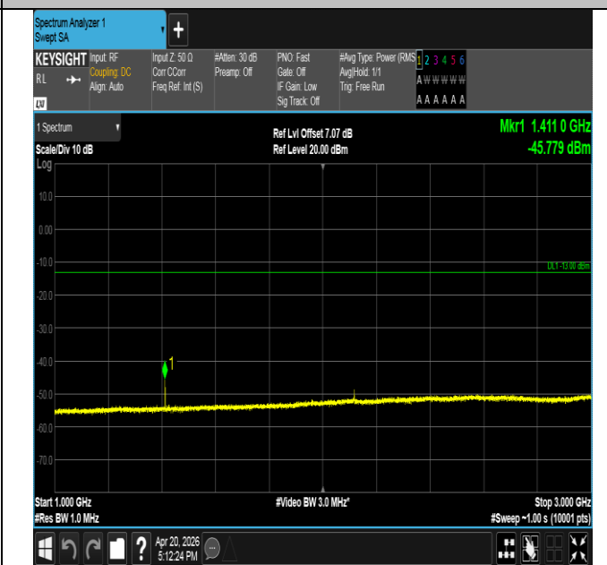
Band17-10MHz-QPSK-23790-1RB#0-1000~3000-PASS
