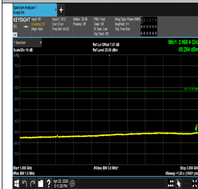
Band17-10MHz-16QAM-23780-50RB#0-1000~3000-PASS
