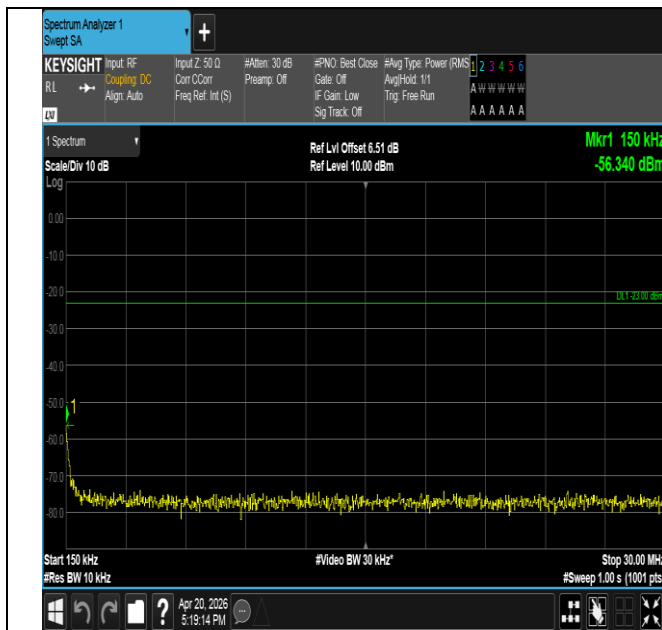
Band17-10MHz-QPSK-23800-1RB#49-0.15~30-PASS
