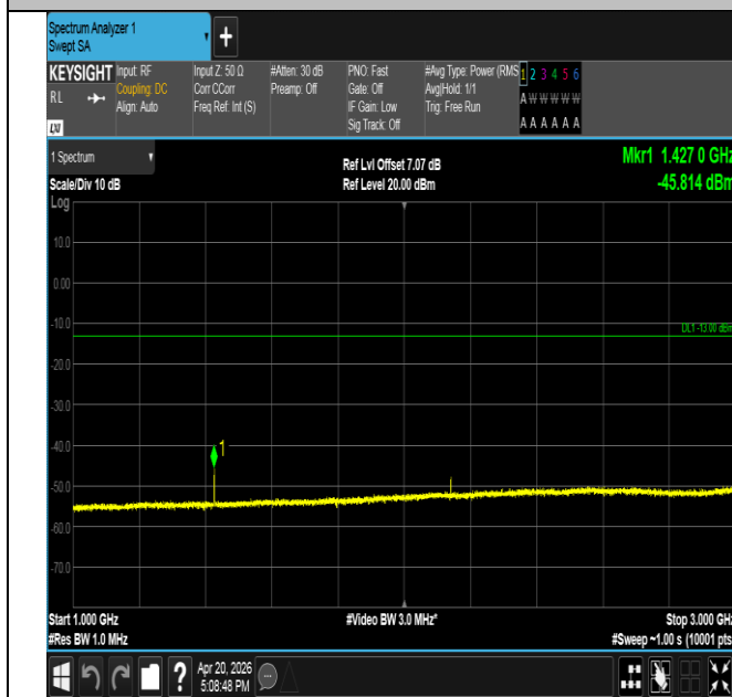
Band17-10MHz-QPSK-23780-1RB#49-1000~3000-PASS
