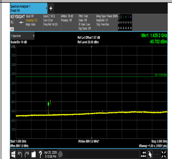
Band17-10MHz-16QAM-23790-1RB#49-1000~3000-PASS
