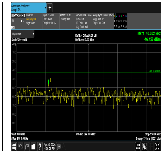
Band17-5MHz-16QAM-23825-25RB#0-0.009~0.15-PASS
