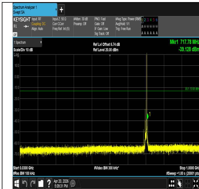
Band17-10MHz-16QAM-23780-1RB#49-30~1000-PASS
