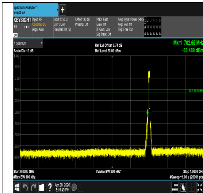
Band17-10MHz-QPSK-23790-50RB#0-30~1000-PASS
