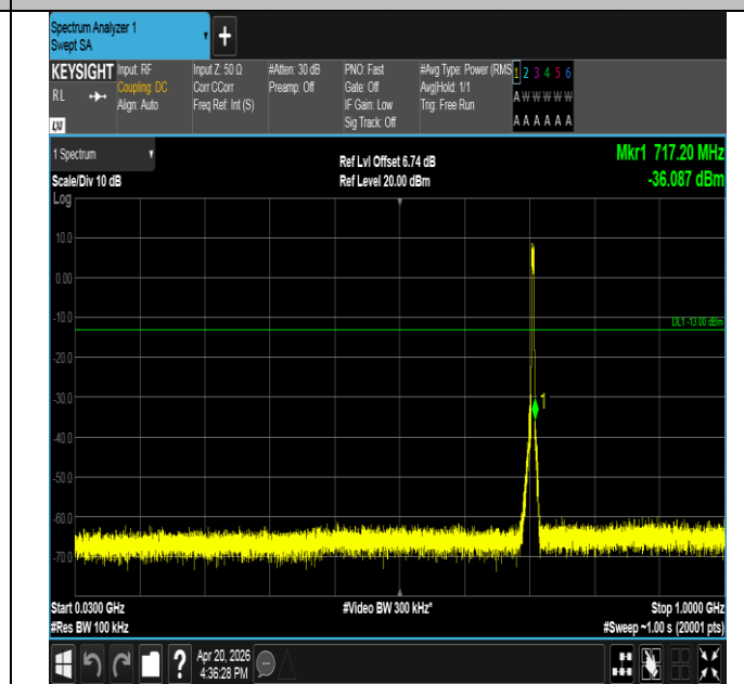
Band17-5MHz-16QAM-23825-25RB#0-30~1000-PASS
