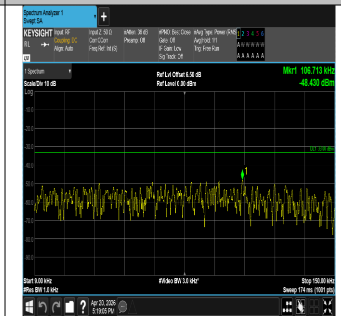
Band17-10MHz-QPSK-23800-1RB#49-0.009~0.15-PASS
