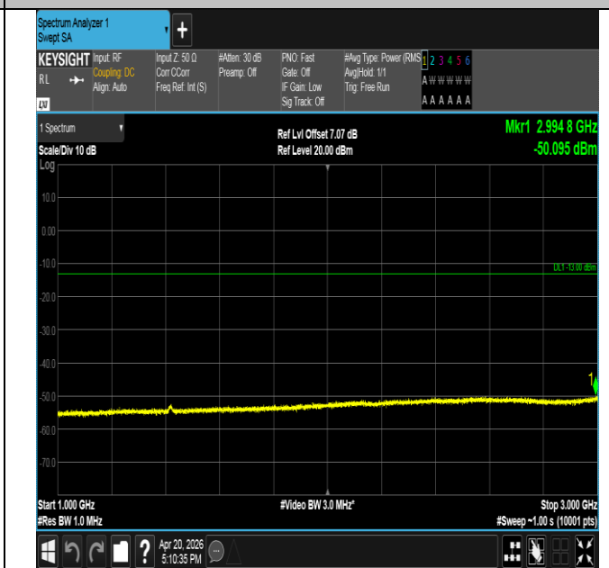
Band17-10MHz-QPSK-23780-50RB#0-1000~3000-PASS
