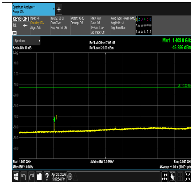
Band17-10MHz-16QAM-23780-1RB#0-1000~3000-PASS
