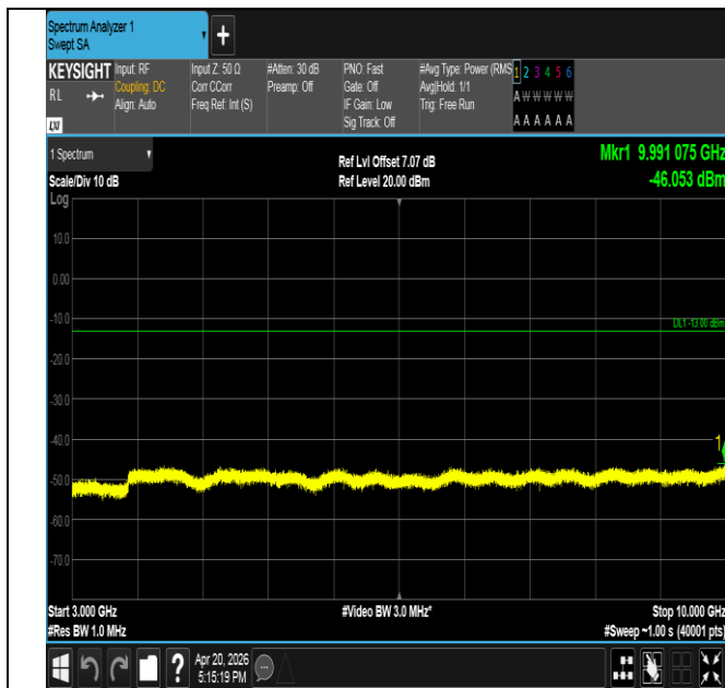
Band17-10MHz-16QAM-23790-1RB#49-3000~10000-PASS
