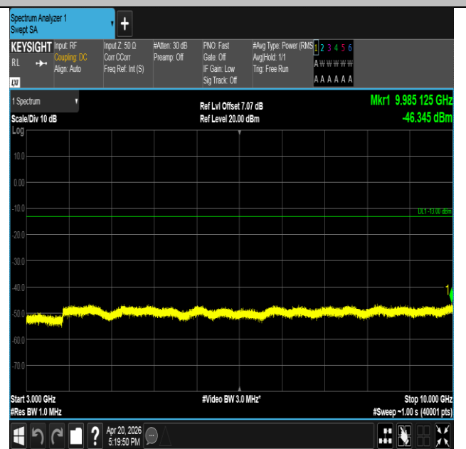
Band17-10MHz-QPSK-23800-1RB#49-3000~10000-PASS
