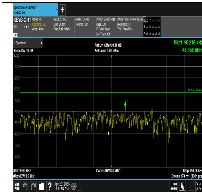
Band17-10MHz-QPSK-23790-1RB#0-0.009~0.15-PASS
