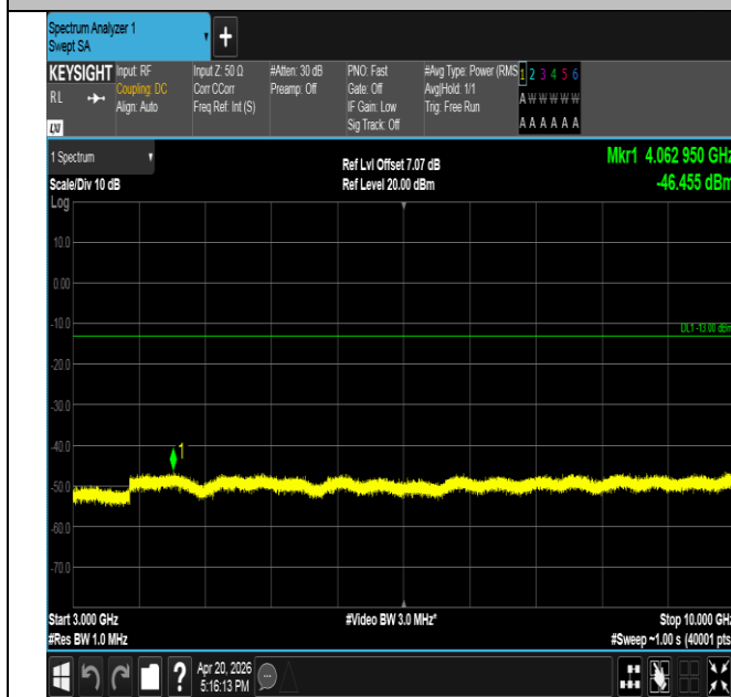
Band17-10MHz-QPSK-23790-50RB#0-3000~10000-PASS
