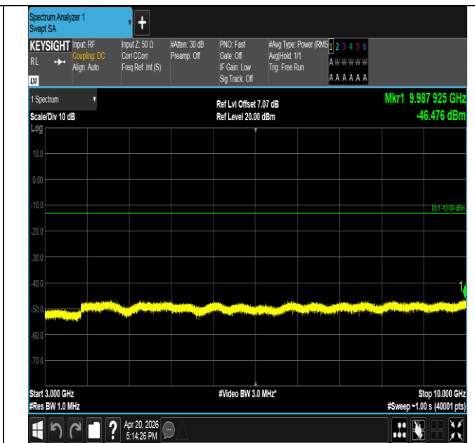
Band17-10MHz-QPSK-23790-1RB#49-3000~10000-PASS
