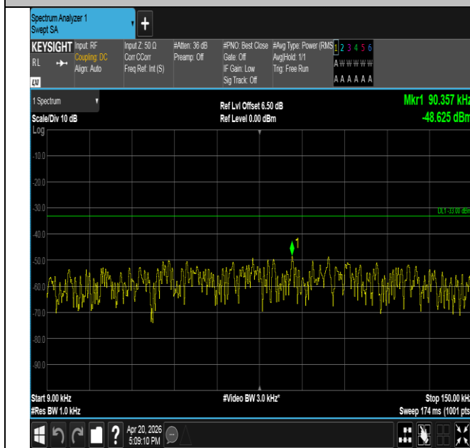
Band17-10MHz-16QAM-23780-1RB#49-0.009~0.15-PASS
