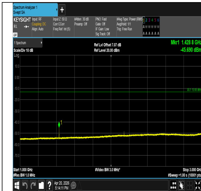
Band17-10MHz-QPSK-23790-1RB#49-1000~3000-PASS
