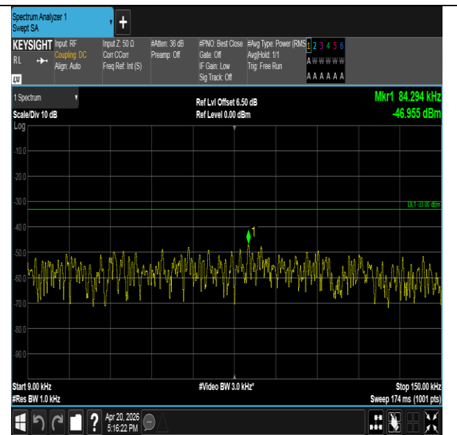
Band17-10MHz-16QAM-23790-50RB#0-0.009~0.15-PASS
