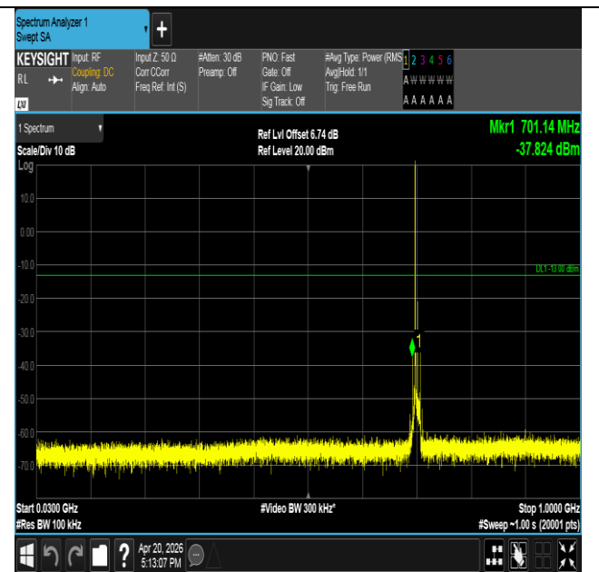
Band17-10MHz-16QAM-23790-1RB#0-30~1000-PASS
