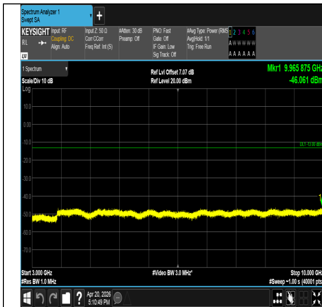
Band17-10MHz-QPSK-23780-50RB#0-3000~10000-PASS
