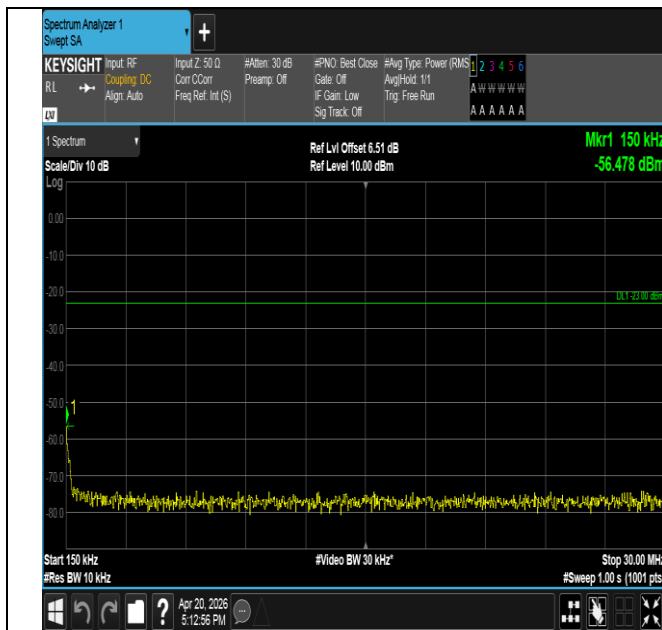
Band17-10MHz-16QAM-23790-1RB#0-0.15~30-PASS
