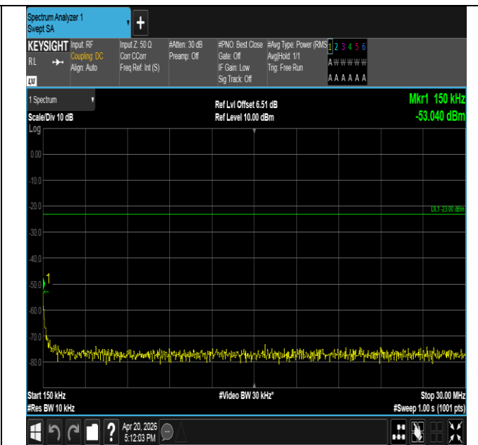
Band17-10MHz-QPSK-23790-1RB#0-0.15~30-PASS
