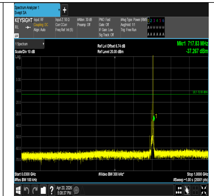
Band17-10MHz-QPSK-23780-1RB#49-30~1000-PASS
