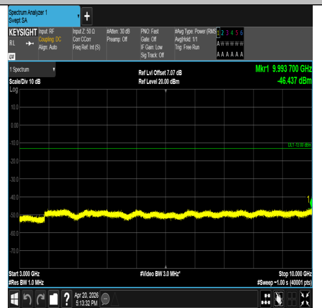
Band17-10MHz-16QAM-23790-1RB#0-3000~10000-PASS
