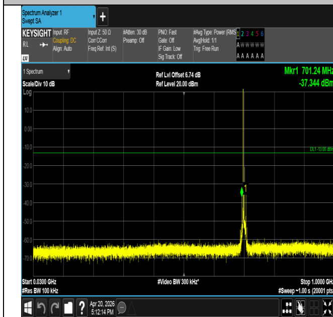
Band17-10MHz-QPSK-23790-1RB#0-30~1000-PASS
