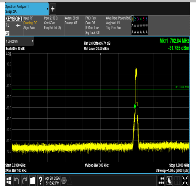
Band17-10MHz-16QAM-23790-50RB#0-30~1000-PASS
