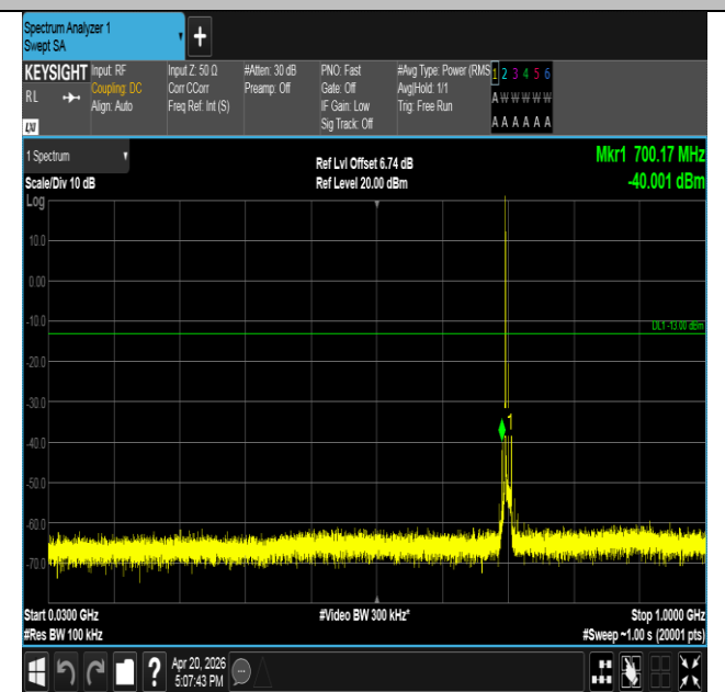
Band17-10MHz-16QAM-23780-1RB#0-30~1000-PASS
