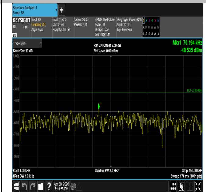
Band17-10MHz-16QAM-23780-50RB#0-0.009~0.15-PASS
