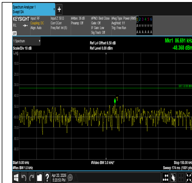
Band17-10MHz-QPSK-23800-50RB#0-0.009~0.15-PASS
