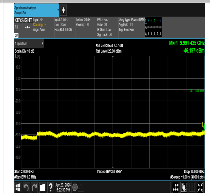
Band17-10MHz-16QAM-23800-50RB#0-3000~10000-PASS
