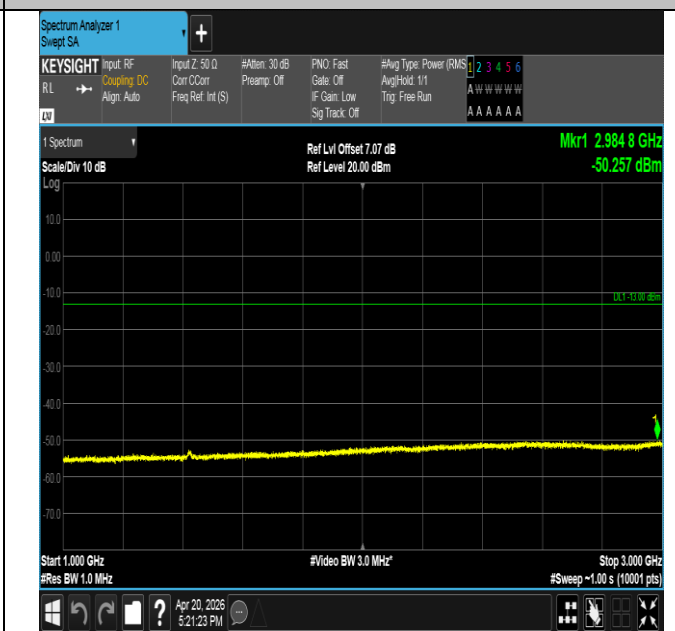
Band17-10MHz-QPSK-23800-50RB#0-1000~3000-PASS
