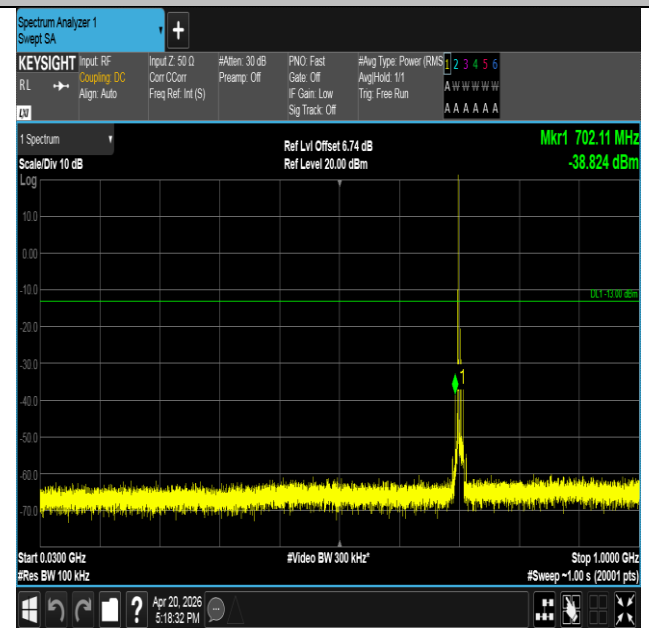
Band17-10MHz-16QAM-23800-1RB#0-30~1000-PASS
