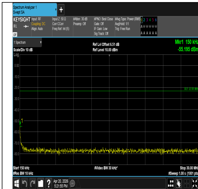
Band17-10MHz-16QAM-23800-50RB#0-0.15~30-PASS
