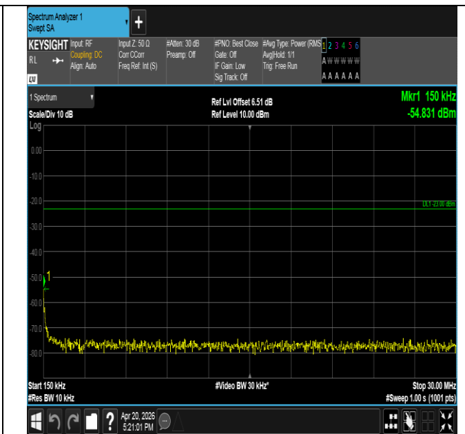
Band17-10MHz-QPSK-23800-50RB#0-0.15~30-PASS
