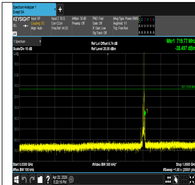
Band17-10MHz-16QAM-23800-1RB#49-30~1000-PASS
