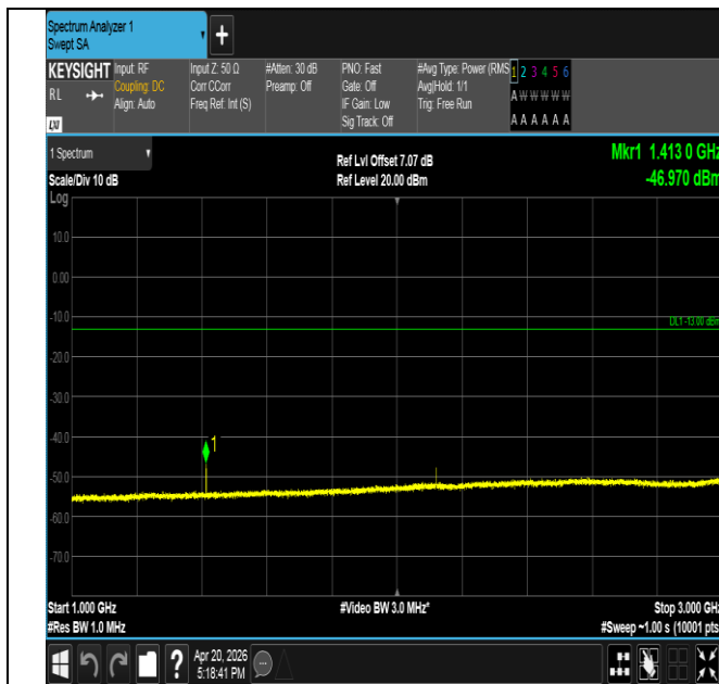
Band17-10MHz-16QAM-23800-1RB#0-1000~3000-PASS
