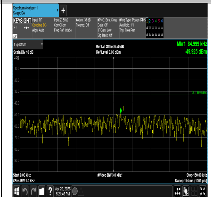
Band17-10MHz-16QAM-23800-50RB#0-0.009~0.15-PASS
