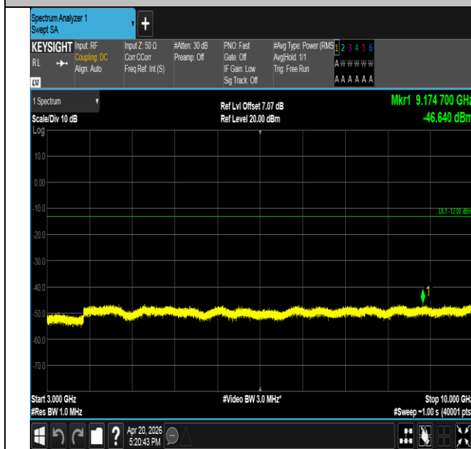
Band17-10MHz-16QAM-23800-1RB#49-3000~10000-PASS
