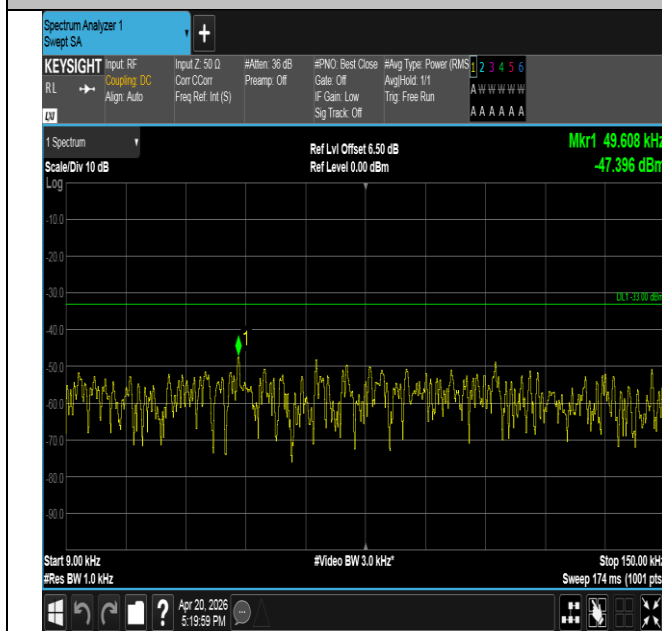
Band17-10MHz-16QAM-23800-1RB#49-0.009~0.15-PASS
