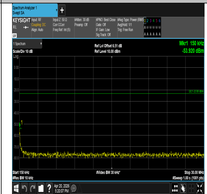
Band17-10MHz-16QAM-23800-1RB#49-0.15~30-PASS
