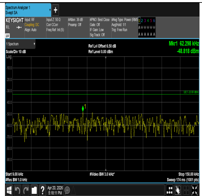
Band17-10MHz-16QAM-23800-1RB#0-0.009~0.15-PASS
