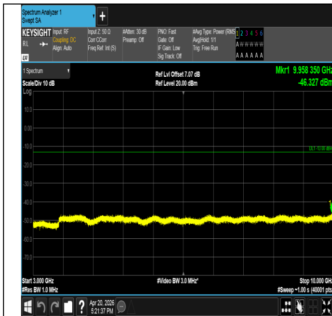
Band17-10MHz-QPSK-23800-50RB#0-3000~10000-PASS
