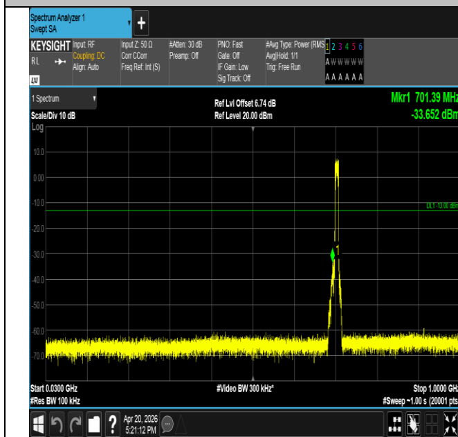
Band17-10MHz-QPSK-23800-50RB#0-30~1000-PASS
