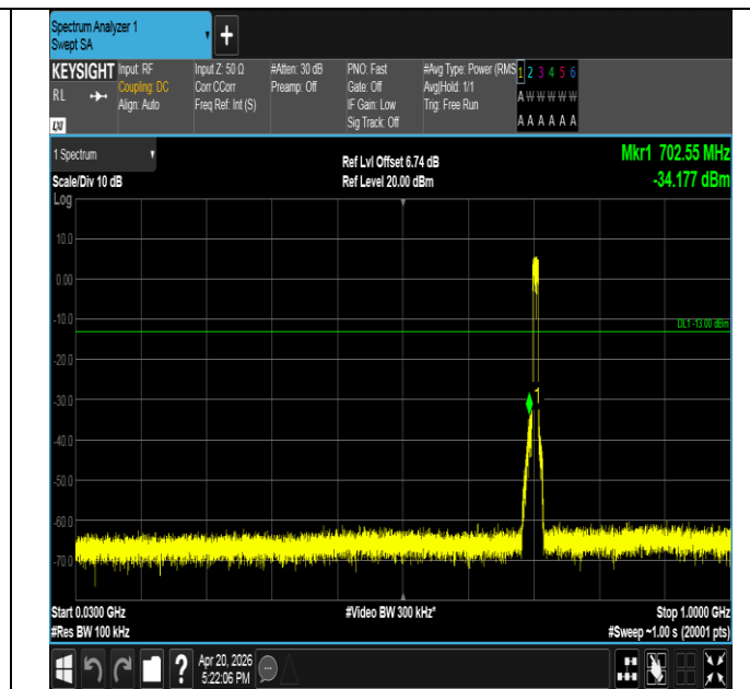
Band17-10MHz-16QAM-23800-50RB#0-30~1000-PASS
