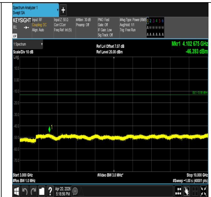
Band17-10MHz-16QAM-23800-1RB#0-3000~10000-PASS
