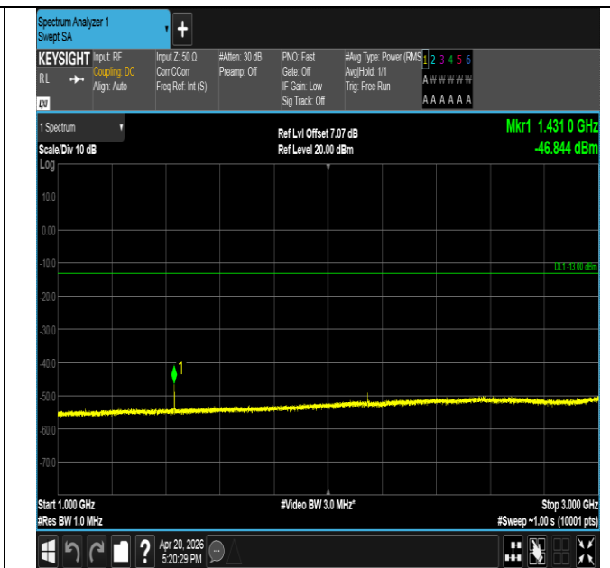
Band17-10MHz-16QAM-23800-1RB#49-1000~3000-PASS
