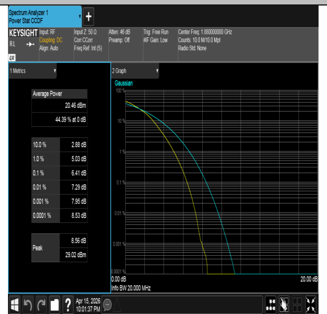
Band2-20MHz-16QAM-18900-100RB#0-PASS
