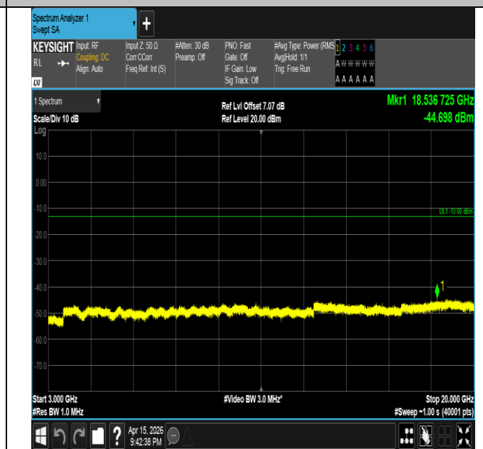
Band2-20MHz-16QAM-19100-100RB#0-3000~20000-PASS
