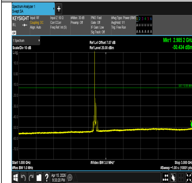
Band2-20MHz-16QAM-18900-1RB#0-1000~3000-PASS
