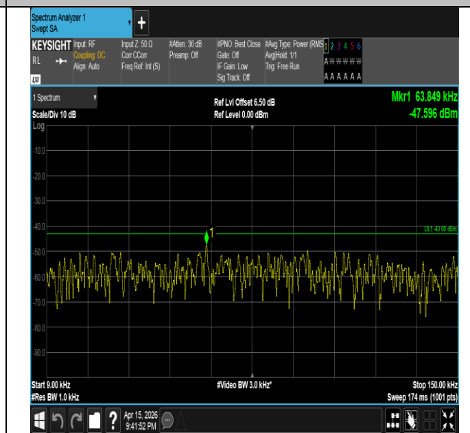
Band2-20MHz-16QAM-19100-100RB#0-0.009~0.15-PASS
