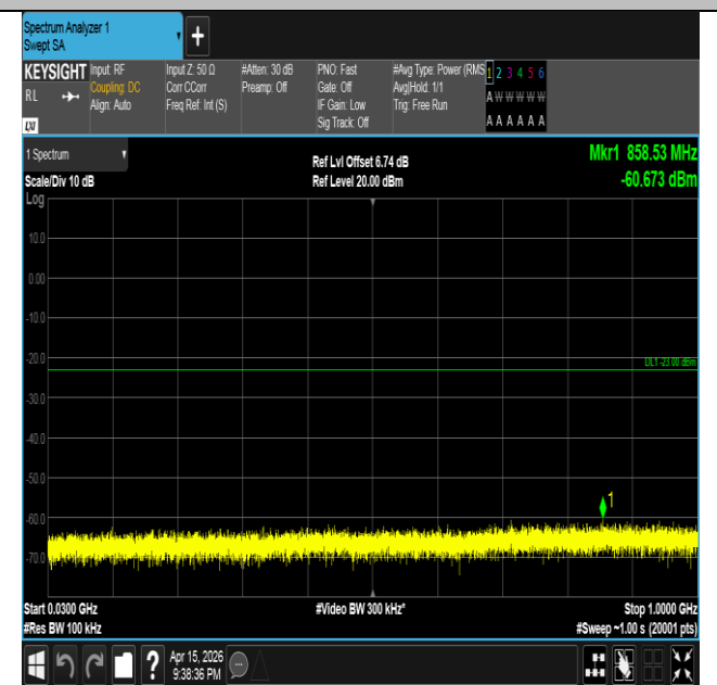
Band2-20MHz-16QAM-19100-1RB#0-30~1000-PASS
