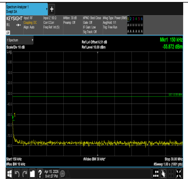
Band2-20MHz-QPSK-19100-100RB#0-0.15~30-PASS
