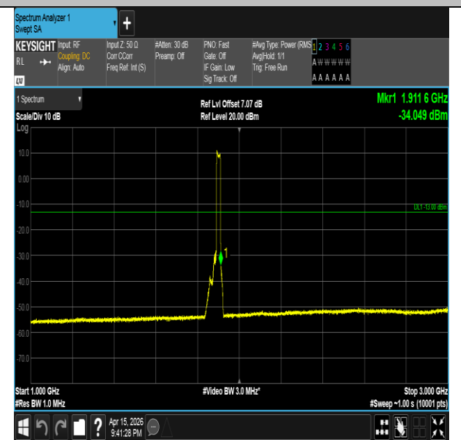
Band2-20MHz-QPSK-19100-100RB#0-1000~3000-PASS
