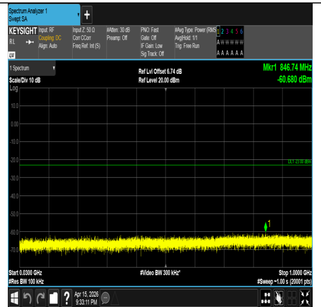
Band2-20MHz-16QAM-18900-1RB#0-30~1000-PASS
