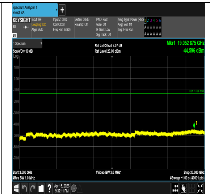
Band2-20MHz-16QAM-18900-100RB#0-3000~20000-PASS
