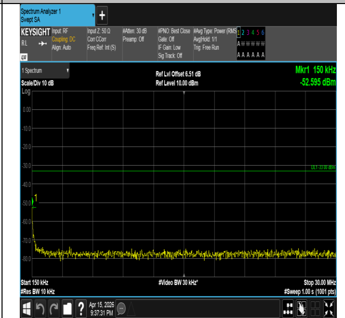
Band2-20MHz-QPSK-19100-1RB#0-0.15~30-PASS
