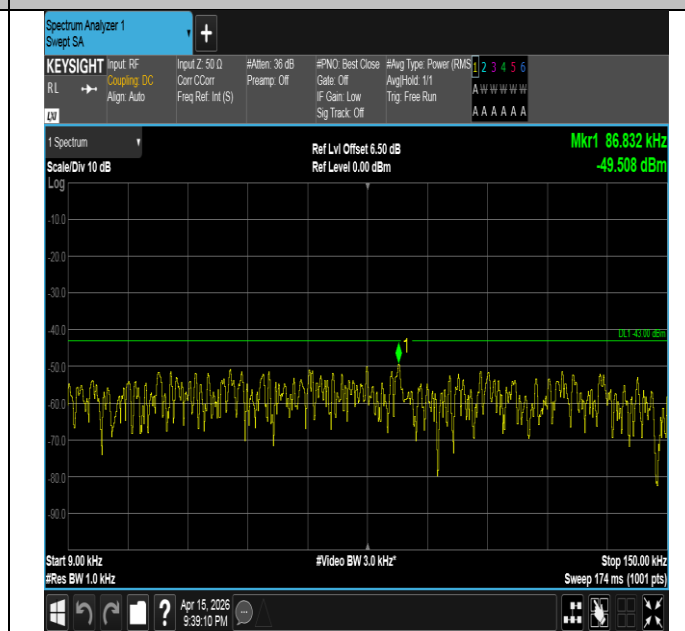
Band2-20MHz-QPSK-19100-1RB#99-0.009~0.15-PASS
