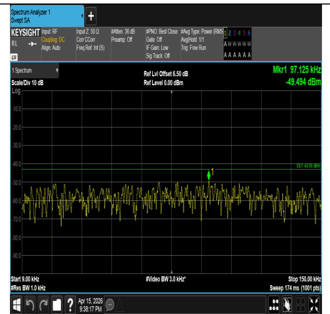
Band2-20MHz-16QAM-19100-1RB#0-0.009~0.15-PASS
