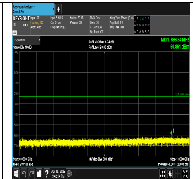
Band2-20MHz-16QAM-19100-100RB#0-30~1000-PASS
