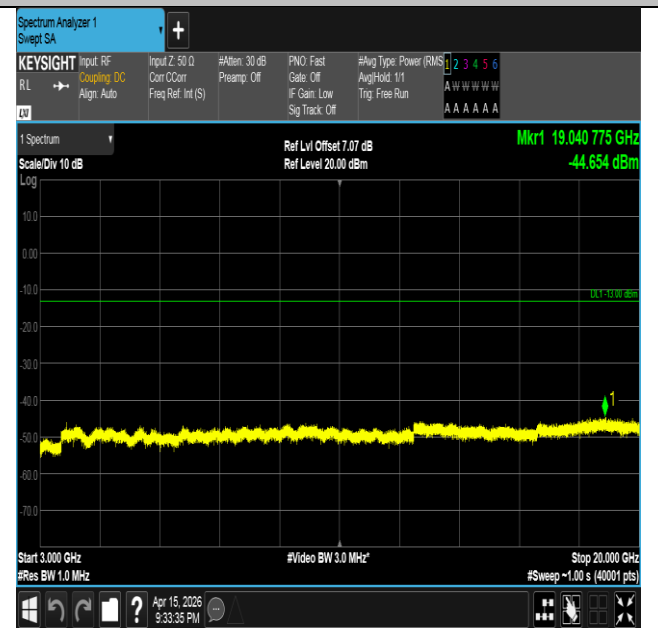
Band2-20MHz-16QAM-18900-1RB#0-3000~20000-PASS
