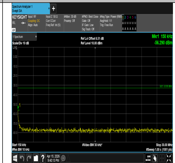
Band2-20MHz-16QAM-19100-1RB#99-0.15~30-PASS
