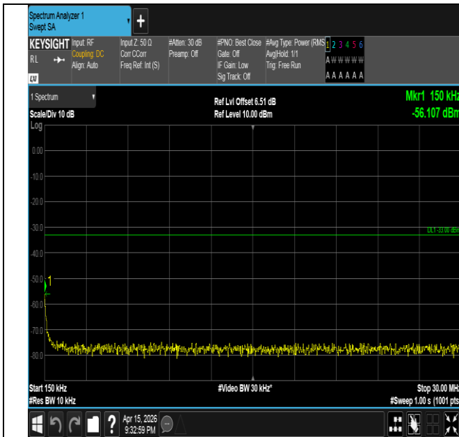
Band2-20MHz-16QAM-18900-1RB#0-0.15~30-PASS
