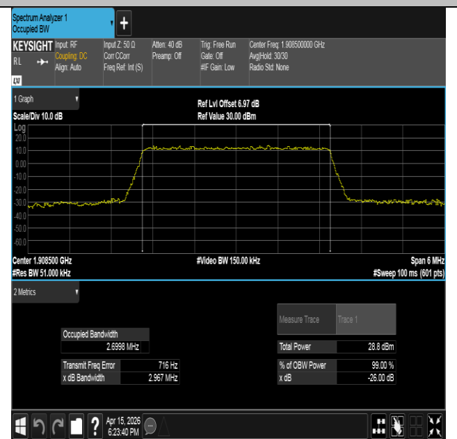
Band2-3MHz-16QAM-19185-15RB#0-PASS
