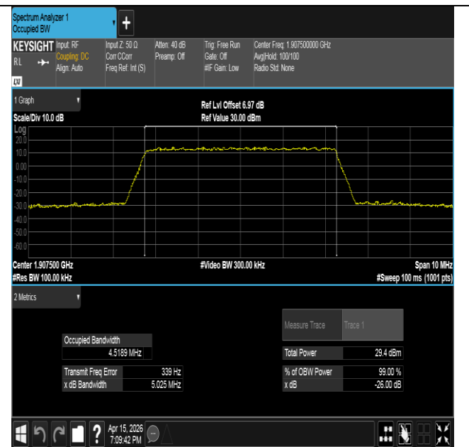
Band2-5MHz-16QAM-19175-25RB#0-PASS
