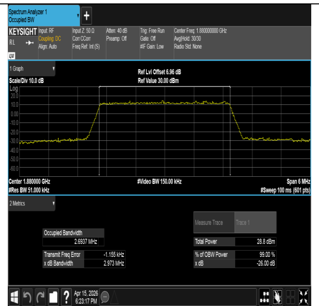
Band2-3MHz-16QAM-18900-15RB#0-PASS
