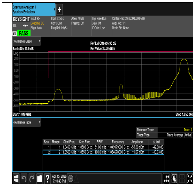
Band2-5MHz-16QAM-18625-1RB#24-PASS
