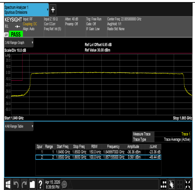
Band2-15MHz-16QAM-18675-75RB#0-PASS
