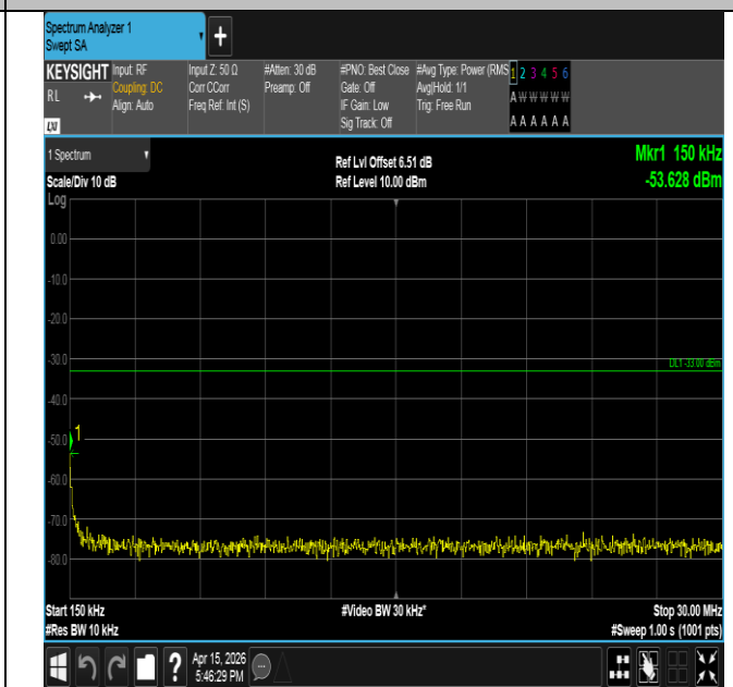
Band2-1.4MHz-QPSK-18900-1RB#0-0.15~30-PASS
