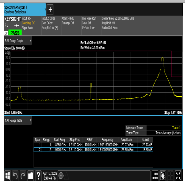
Band2-15MHz-QPSK-19125-1RB#74-PASS
