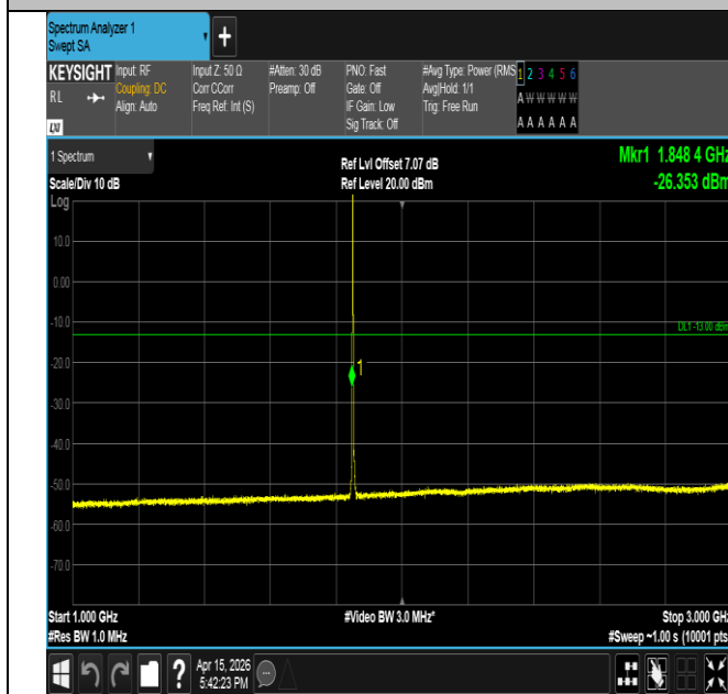
Band2-1.4MHz-16QAM-18607-1RB#0-1000~3000-PASS
