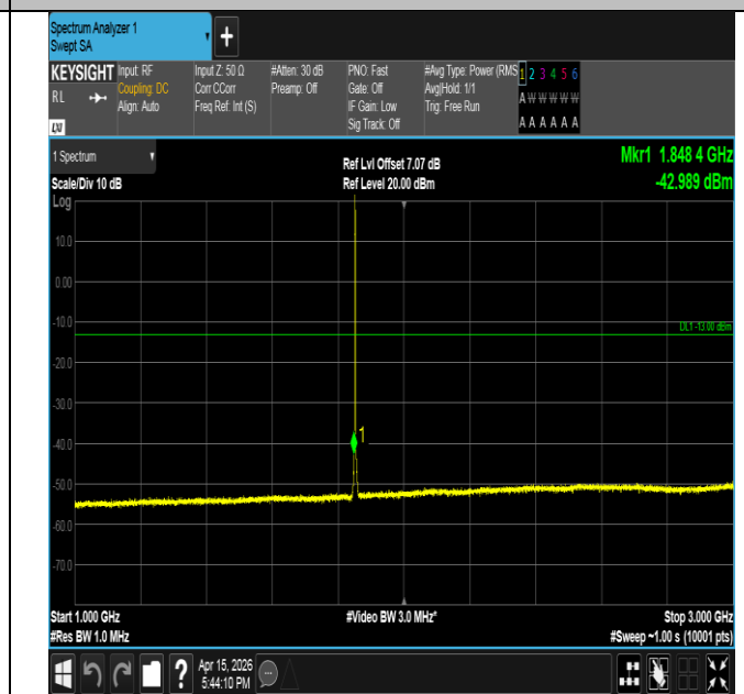
Band2-1.4MHz-16QAM-18607-1RB#5-1000~3000-PASS
