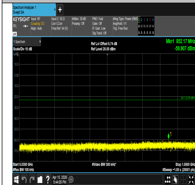
Band2-1.4MHz-16QAM-18607-1RB#5-30~1000-PASS
