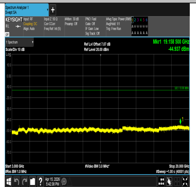
Band2-1.4MHz-16QAM-18607-1RB#0-3000~20000-PASS
