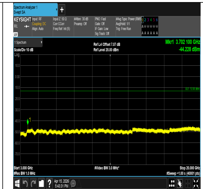
Band2-1.4MHz-QPSK-18607-1RB#5-3000~20000-PASS
