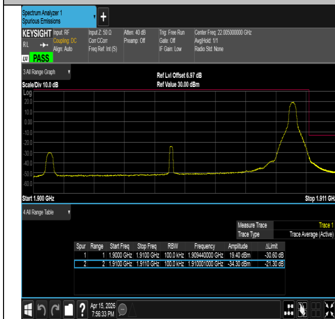
Band2-10MHz-16QAM-19150-1RB#49-PASS
