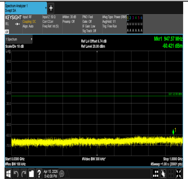
Band2-1.4MHz-QPSK-18607-1RB#5-30~1000-PASS
