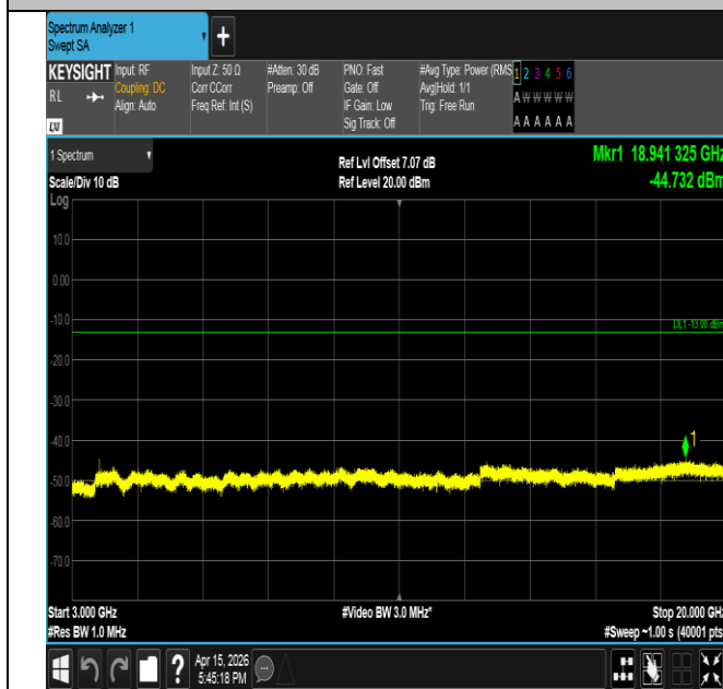
Band2-1.4MHz-QPSK-18607-6RB#0-3000~20000-PASS
