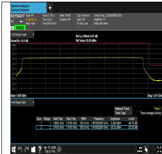
Band2-10MHz-QPSK-19150-50RB#0-PASS
