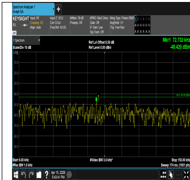
Band2-1.4MHz-16QAM-18607-1RB#5-0.009~0.15-PASS
