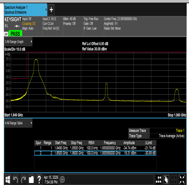
Band2-10MHz-16QAM-18650-1RB#0-PASS
