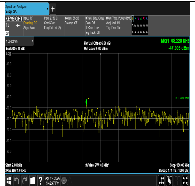
Band2-1.4MHz-QPSK-18607-1RB#5-0.009~0.15-PASS
