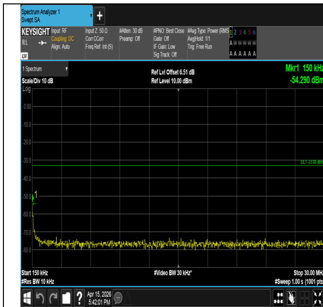
Band2-1.4MHz-16QAM-18607-1RB#0-0.15~30-PASS
