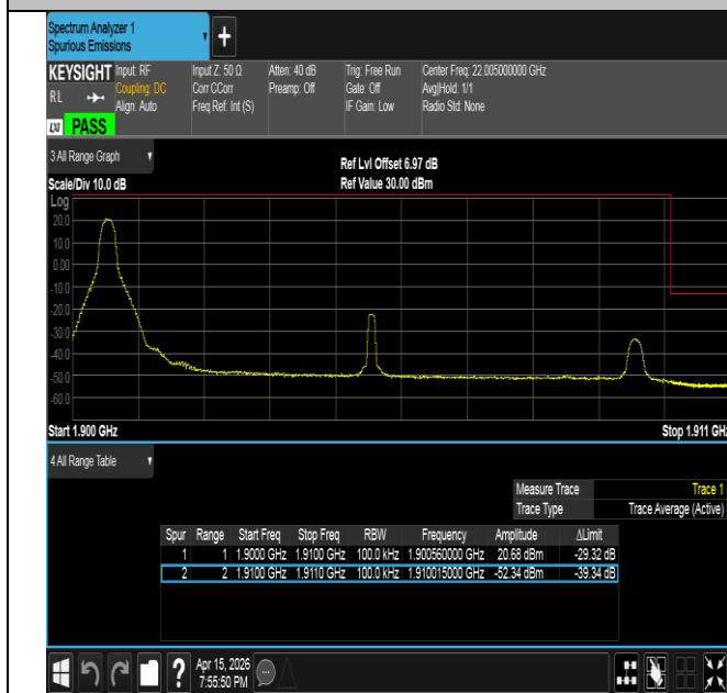
Band2-10MHz-QPSK-19150-1RB#0-PASS
