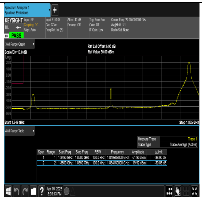
Band2-15MHz-QPSK-18675-1RB#74-PASS
