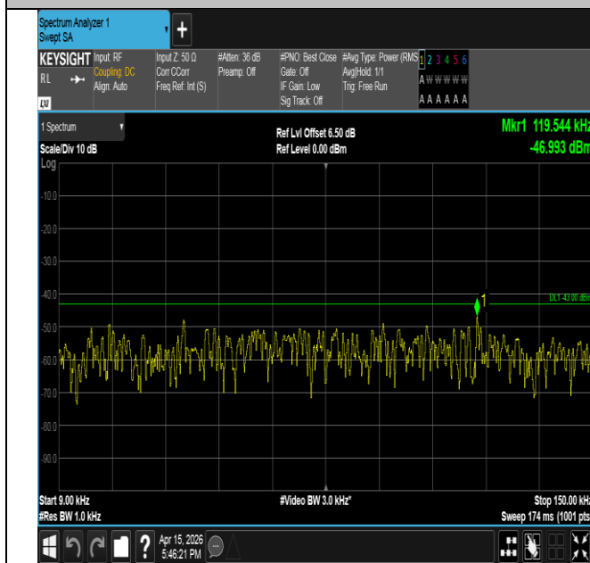
Band2-1.4MHz-QPSK-18900-1RB#0-0.009~0.15-PASS
