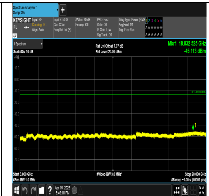
Band2-1.4MHz-16QAM-18607-6RB#0-3000~20000-PASS
