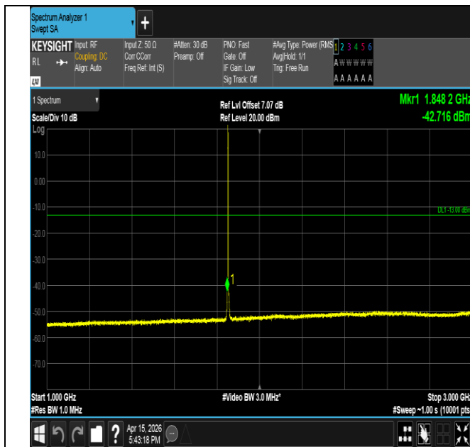
Band2-1.4MHz-QPSK-18607-1RB#5-1000~3000-PASS
