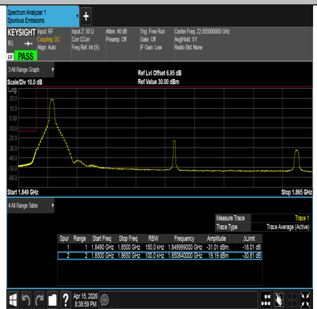
Band2-15MHz-16QAM-18675-1RB#0-PASS
