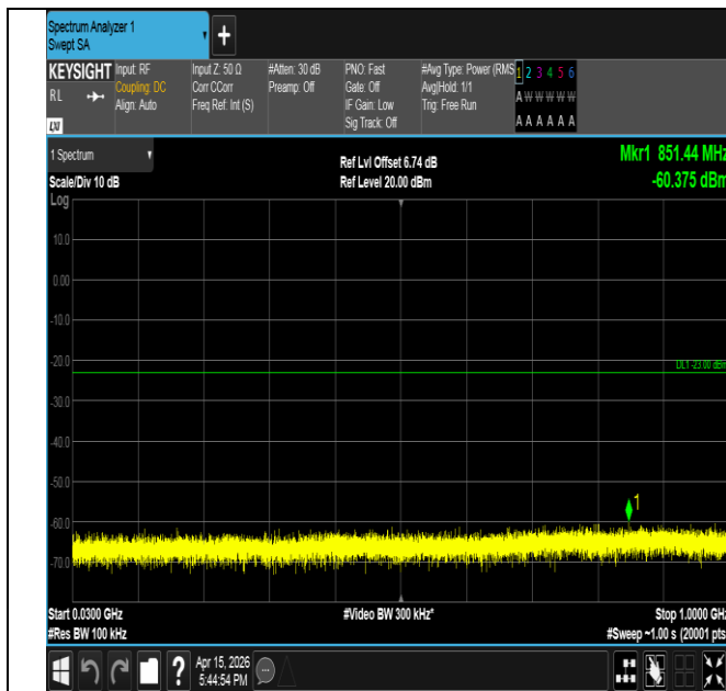
Band2-1.4MHz-QPSK-18607-6RB#0-30~1000-PASS
