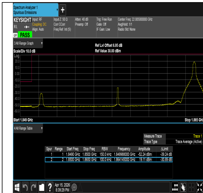
Band2-15MHz-16QAM-18675-1RB#74-PASS
