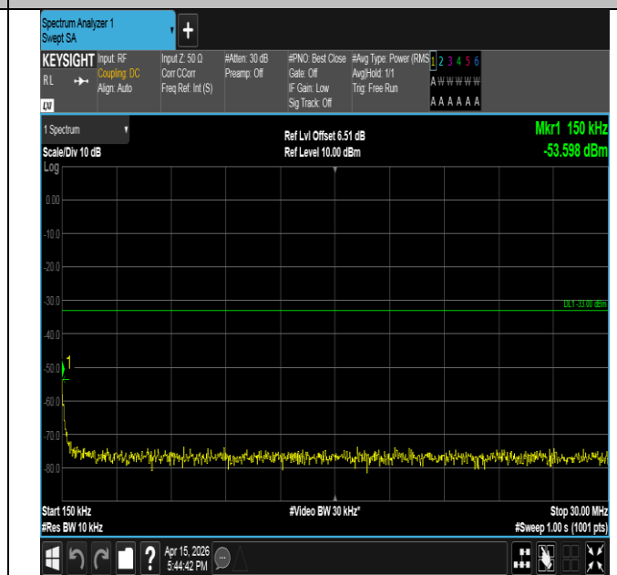
Band2-1.4MHz-QPSK-18607-6RB#0-0.15~30-PASS
