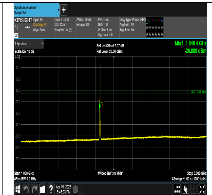
Band2-1.4MHz-QPSK-18607-6RB#0-1000~3000-PASS
