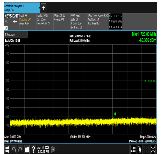
Band2-1.4MHz-16QAM-18607-1RB#0-30~1000-PASS
