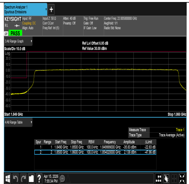
Band2-10MHz-16QAM-18650-50RB#0-PASS
