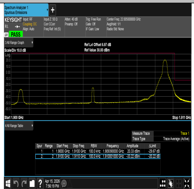
Band2-10MHz-QPSK-19150-1RB#49-PASS
