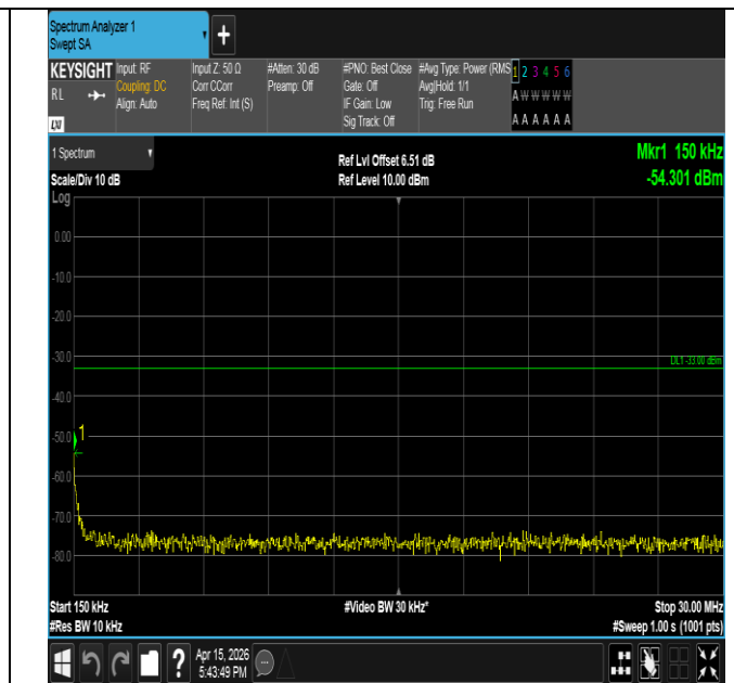
Band2-1.4MHz-16QAM-18607-1RB#5-0.15~30-PASS
