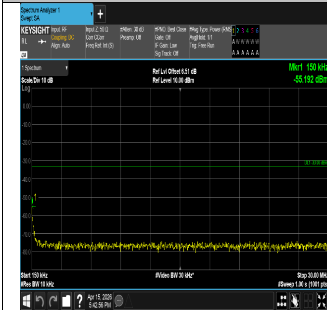
Band2-1.4MHz-QPSK-18607-1RB#5-0.15~30-PASS
