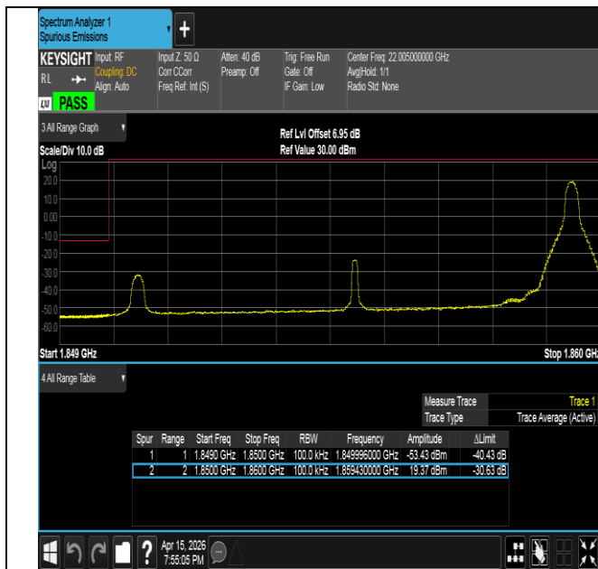
Band2-10MHz-16QAM-18650-1RB#49-PASS
