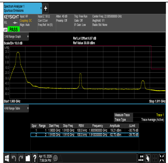
Band2-10MHz-16QAM-19150-1RB#0-PASS
