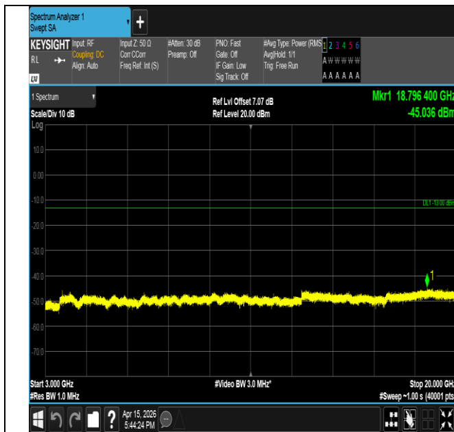
Band2-1.4MHz-16QAM-18607-1RB#5-3000~20000-PASS
