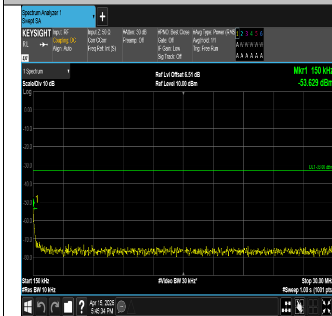
Band2-1.4MHz-16QAM-18607-6RB#0-0.15~30-PASS
