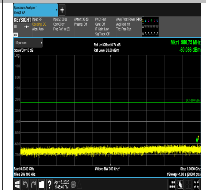
Band2-1.4MHz-16QAM-18607-6RB#0-30~1000-PASS
