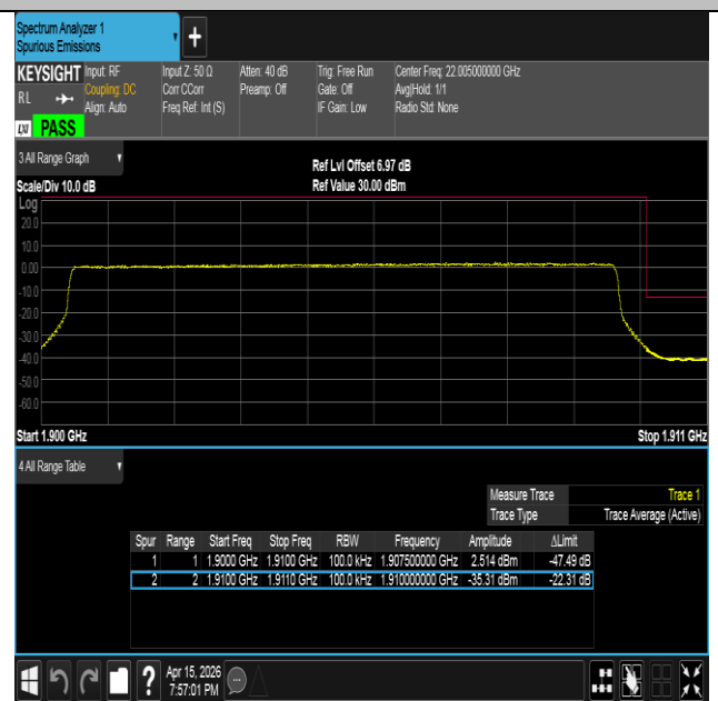
Band2-10MHz-16QAM-19150-50RB#0-PASS
