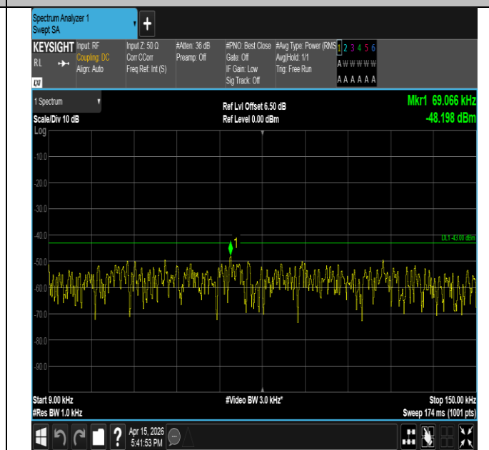
Band2-1.4MHz-16QAM-18607-1RB#0-0.009~0.15-PASS
