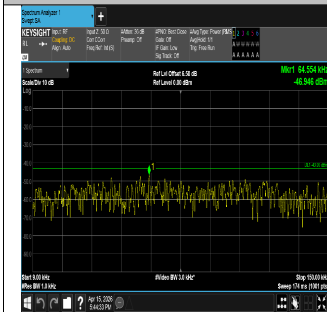
Band2-1.4MHz-QPSK-18607-6RB#0-0.009~0.15-PASS
