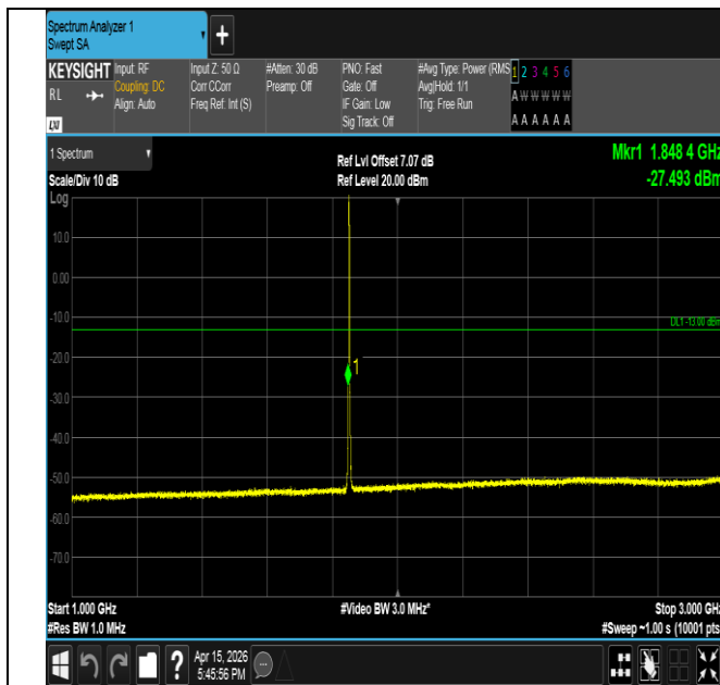
Band2-1.4MHz-16QAM-18607-6RB#0-1000~3000-PASS
