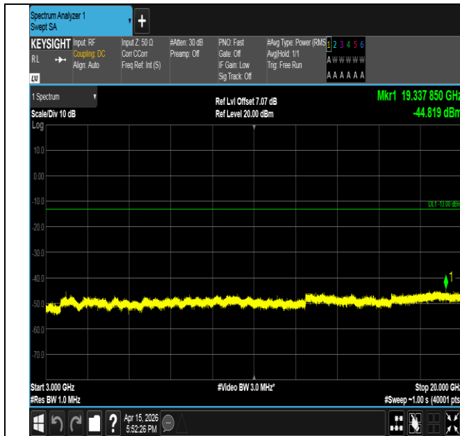
Band2-1.4MHz-QPSK-19193-1RB#0-3000~20000-PASS
