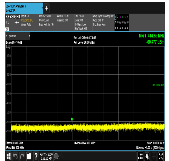
Band2-1.4MHz-16QAM-19193-1RB#0-30~1000-PASS
