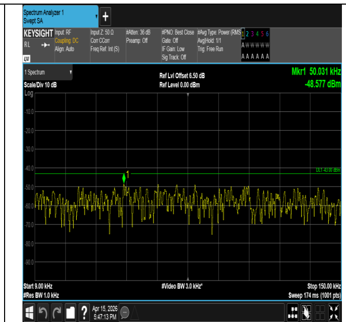
Band2-1.4MHz-16QAM-18900-1RB#0-0.009~0.15-PASS
