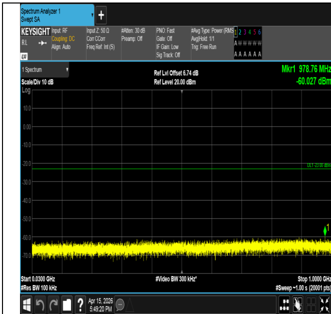
Band2-1.4MHz-16QAM-18900-1RB#5-30~1000-PASS
