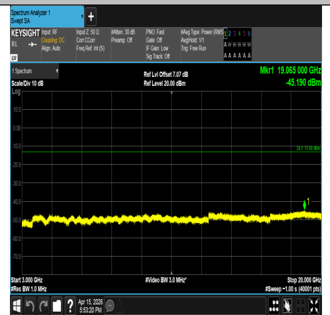
Band2-1.4MHz-16QAM-19193-1RB#0-3000~20000-PASS
