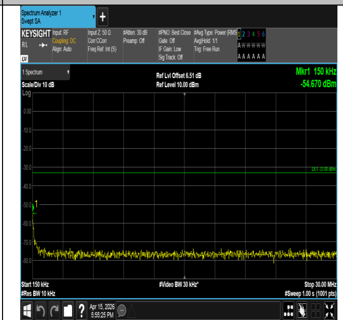
Band2-1.4MHz-QPSK-19193-6RB#0-0.15~30-PASS
