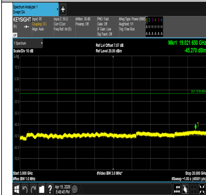
Band2-1.4MHz-16QAM-18900-1RB#5-3000~20000-PASS
