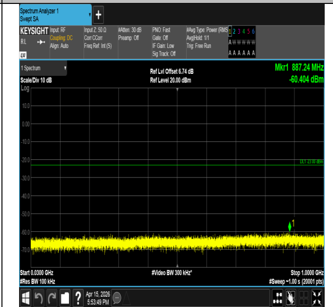
Band2-1.4MHz-QPSK-19193-1RB#5-30~1000-PASS
