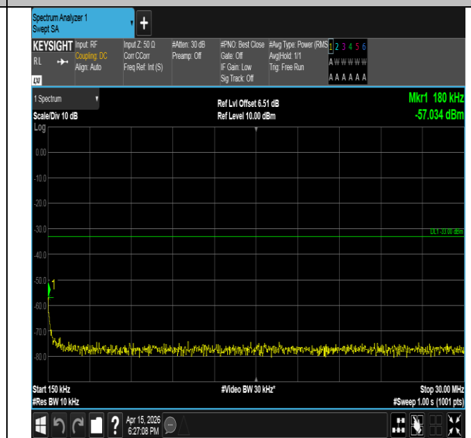
Band2-3MHz-QPSK-18615-1RB#0-0.15~30-PASS
