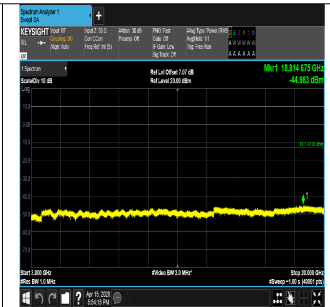
Band2-1.4MHz-QPSK-19193-1RB#5-3000~20000-PASS
