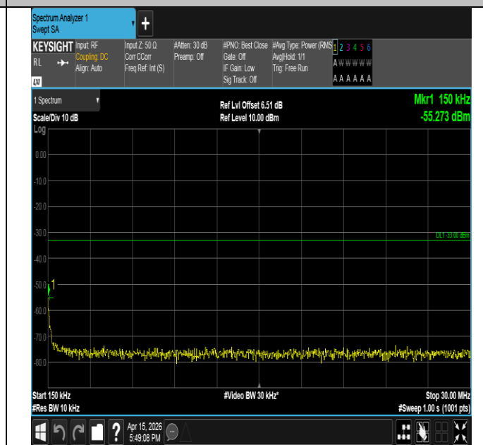
Band2-1.4MHz-16QAM-18900-1RB#5-0.15~30-PASS
