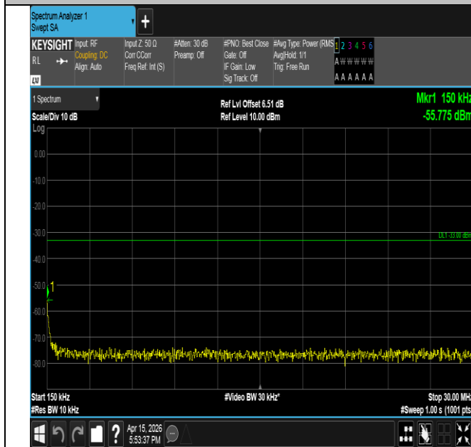
Band2-1.4MHz-QPSK-19193-1RB#5-0.15~30-PASS
