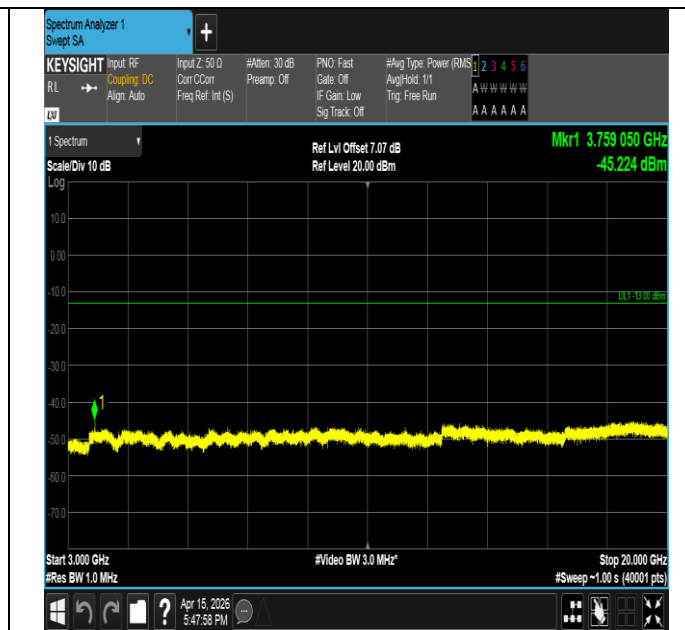
Band2-1.4MHz-16QAM-18900-1RB#0-3000~20000-PASS
