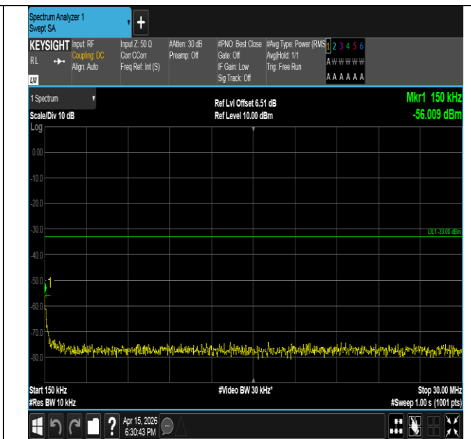
Band2-3MHz-QPSK-18615-15RB#0-0.15~30-PASS
