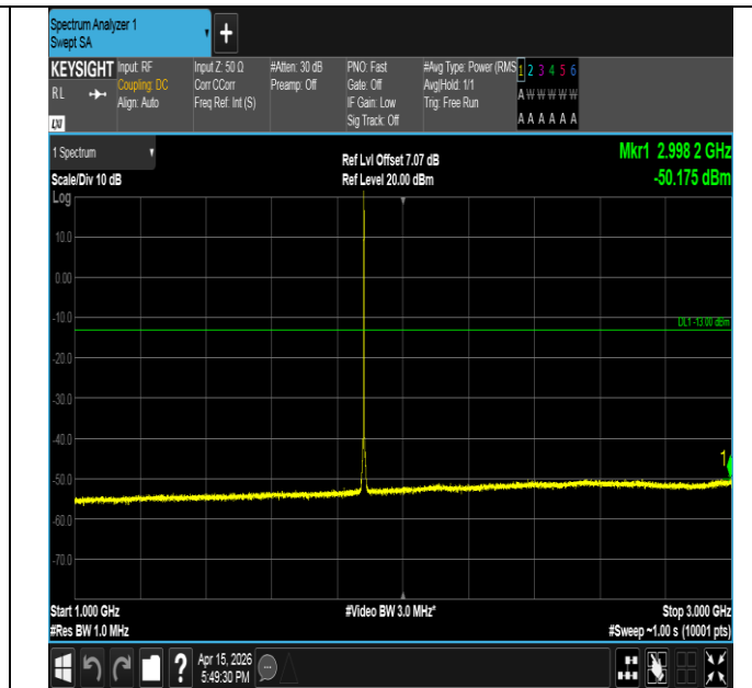
Band2-1.4MHz-16QAM-18900-1RB#5-1000~3000-PASS
