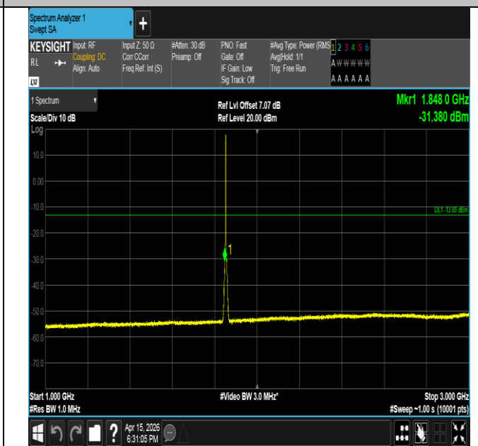
Band2-3MHz-QPSK-18615-15RB#0-1000~3000-PASS
