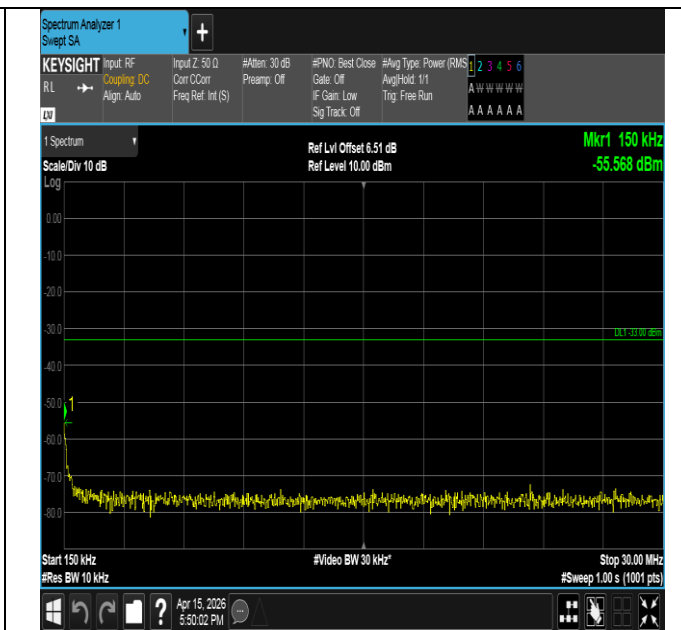
Band2-1.4MHz-QPSK-18900-6RB#0-0.15~30-PASS
