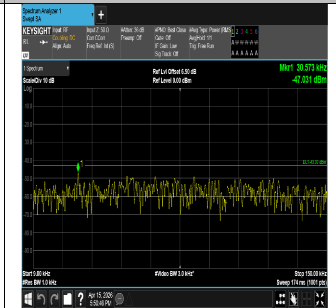
Band2-1.4MHz-16QAM-18900-6RB#0-0.009~0.15-PASS
