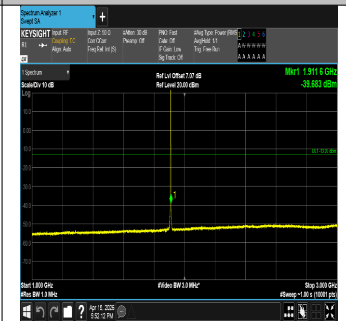
Band2-1.4MHz-QPSK-19193-1RB#0-1000~3000-PASS
