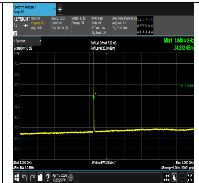
Band2-3MHz-QPSK-18615-1RB#0-1000~3000-PASS
