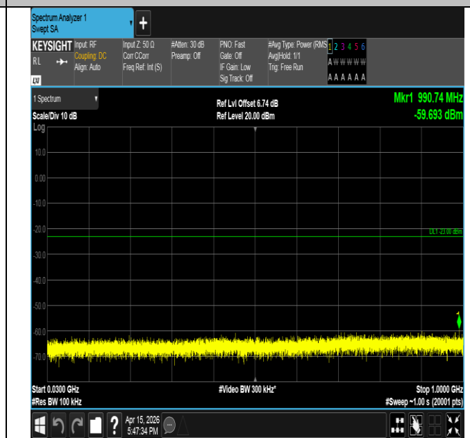
Band2-1.4MHz-16QAM-18900-1RB#0-30~1000-PASS
