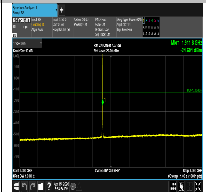
Band2-1.4MHz-16QAM-19193-1RB#5-1000~3000-PASS
