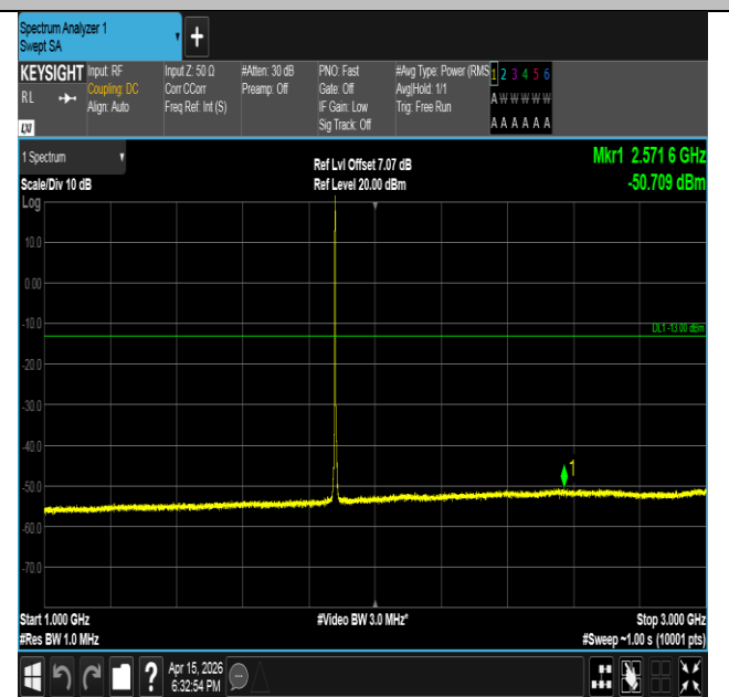
Band2-3MHz-QPSK-18900-1RB#0-1000~3000-PASS
