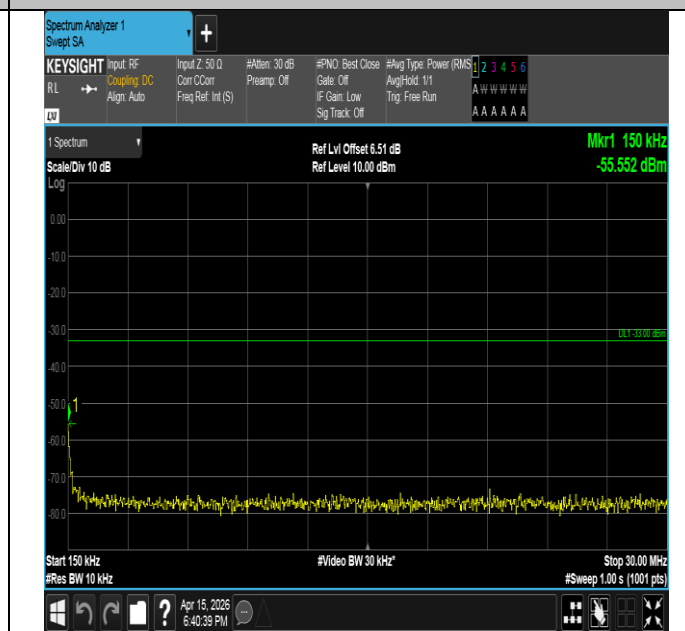
Band2-3MHz-16QAM-19185-1RB#14-0.15~30-PASS
