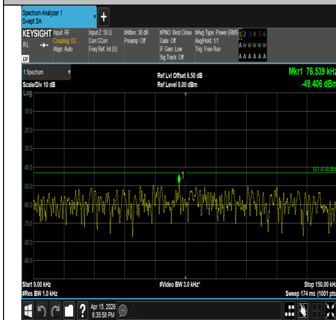
Band2-3MHz-QPSK-18900-15RB#0-0.009~0.15-PASS
