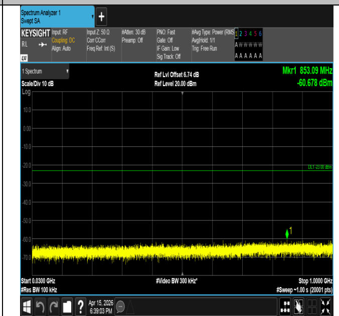
Band2-3MHz-16QAM-19185-1RB#0-30~1000-PASS
