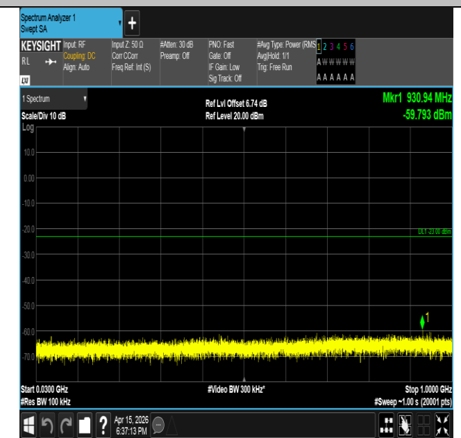
Band2-3MHz-16QAM-18900-15RB#0-30~1000-PASS
