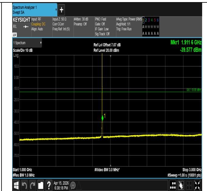
Band2-3MHz-QPSK-19185-1RB#0-1000~3000-PASS
