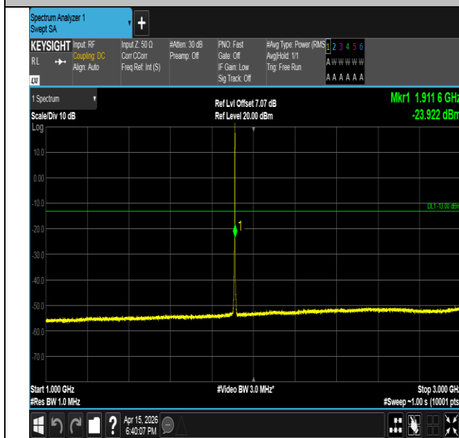
Band2-3MHz-QPSK-19185-1RB#14-1000~3000-PASS
