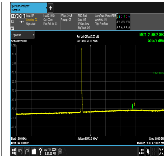
Band2-3MHz-16QAM-18900-15RB#0-1000~3000-PASS
