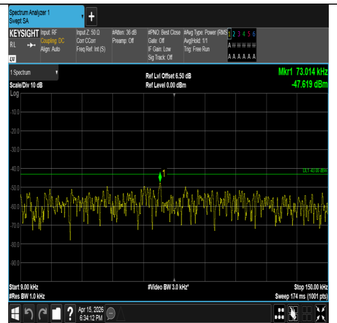
Band2-3MHz-QPSK-18900-1RB#14-0.009~0.15-PASS
