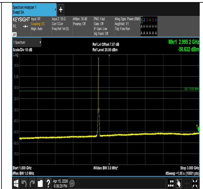
Band2-3MHz-QPSK-18900-15RB#0-1000~3000-PASS
