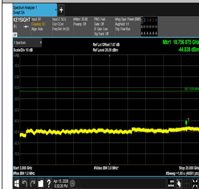
Band2-3MHz-16QAM-18615-1RB#14-3000~20000-PASS
