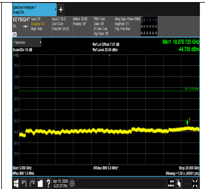
Band2-3MHz-16QAM-18900-15RB#0-3000~20000-PASS
