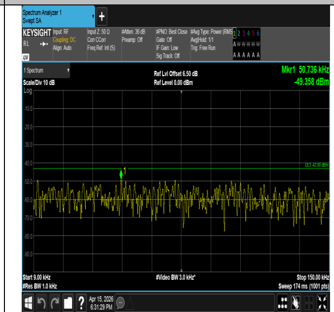
Band2-3MHz-16QAM-18615-15RB#0-0.009~0.15-PASS
