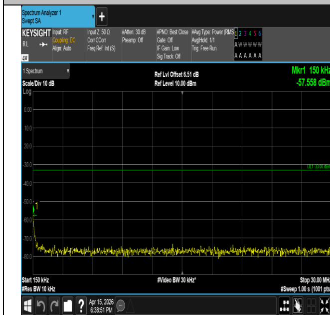
Band2-3MHz-16QAM-19185-1RB#0-0.15~30-PASS
