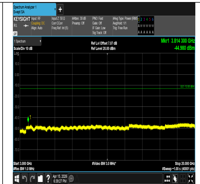
Band2-3MHz-16QAM-19185-1RB#0-3000~20000-PASS
