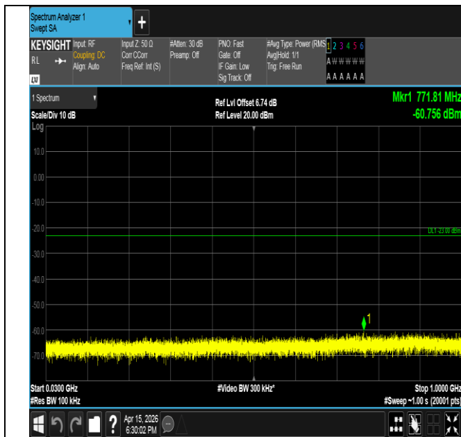
Band2-3MHz-16QAM-18615-1RB#14-30~1000-PASS
