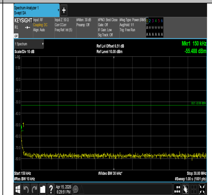
Band2-3MHz-16QAM-18615-1RB#14-0.15~30-PASS
