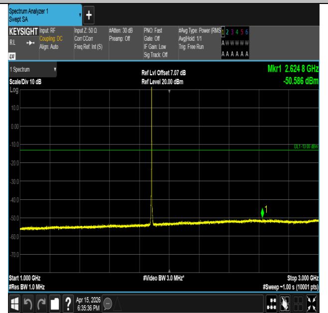
Band2-3MHz-16QAM-18900-1RB#14-1000~3000-PASS
