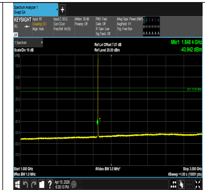
Band2-3MHz-16QAM-18615-1RB#14-1000~3000-PASS
