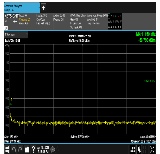
Band2-5MHz-QPSK-18625-1RB#0-0.15~30-PASS
