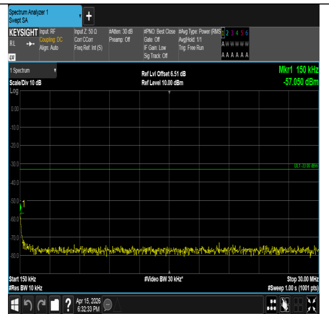
Band2-3MHz-QPSK-18900-1RB#0-0.15~30-PASS
