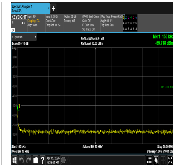
Band2-3MHz-QPSK-19185-1RB#14-0.15~30-PASS
