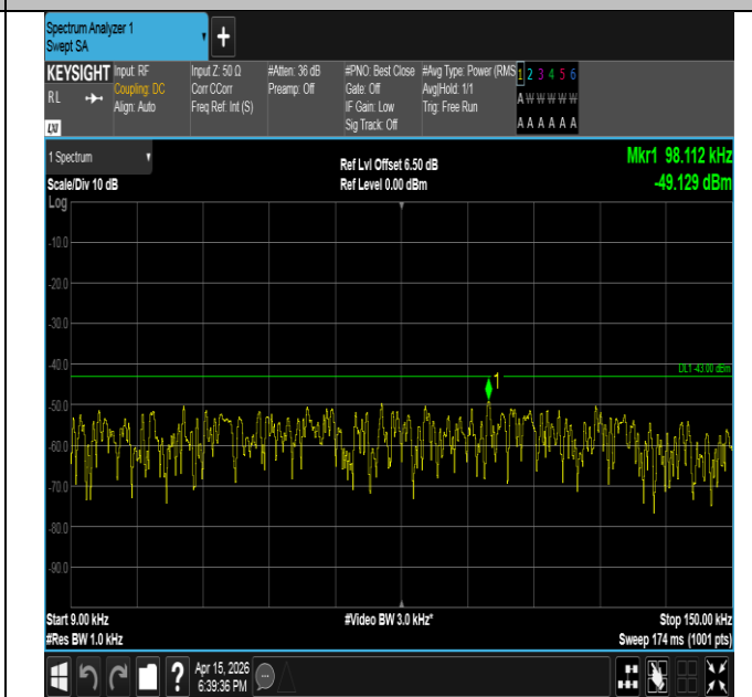
Band2-3MHz-QPSK-19185-1RB#14-0.009~0.15-PASS
