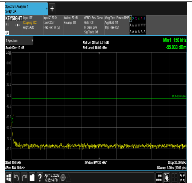
Band2-3MHz-16QAM-18900-1RB#14-0.15~30-PASS
