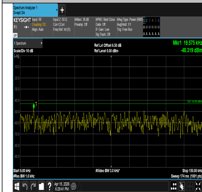
Band2-3MHz-16QAM-18615-1RB#14-0.009~0.15-PASS
