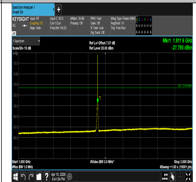
Band2-3MHz-QPSK-19185-15RB#0-1000~3000-PASS
