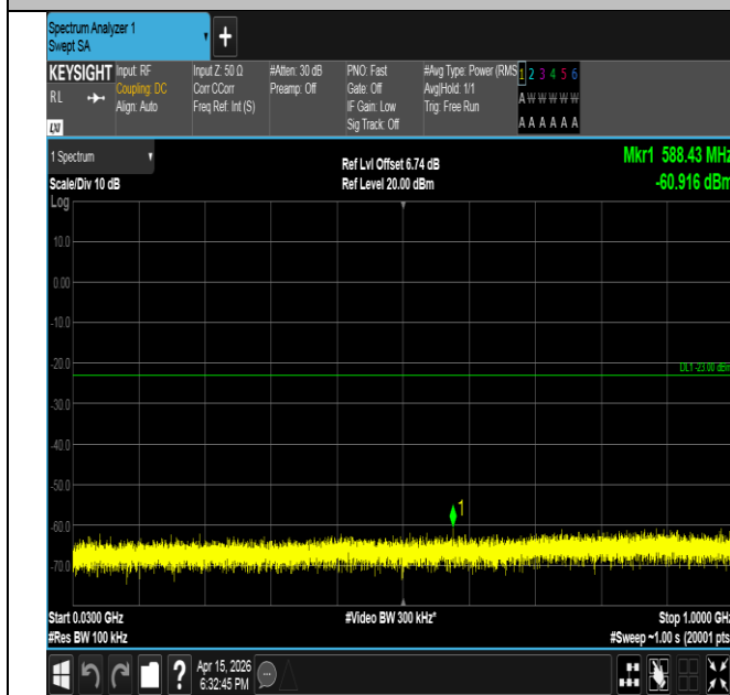
Band2-3MHz-QPSK-18900-1RB#0-30~1000-PASS
