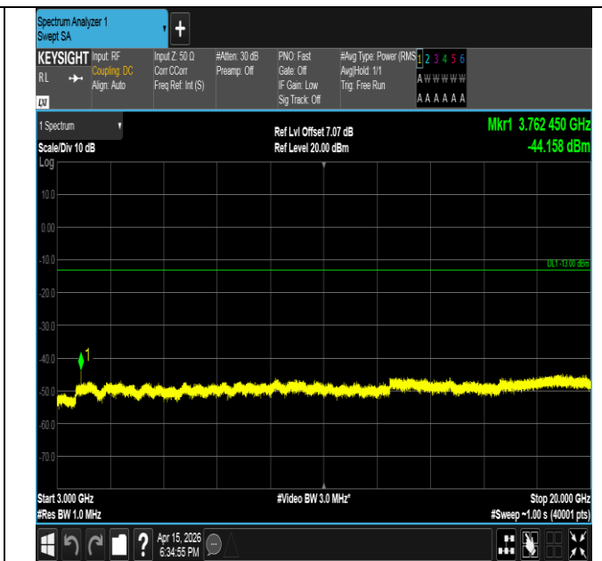
Band2-3MHz-QPSK-18900-1RB#14-3000~20000-PASS
