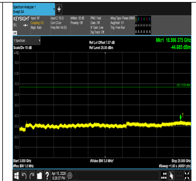
Band2-3MHz-16QAM-18615-1RB#0-3000~20000-PASS
