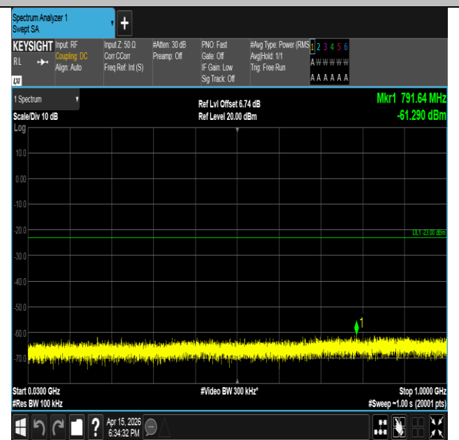
Band2-3MHz-QPSK-18900-1RB#14-30~1000-PASS
