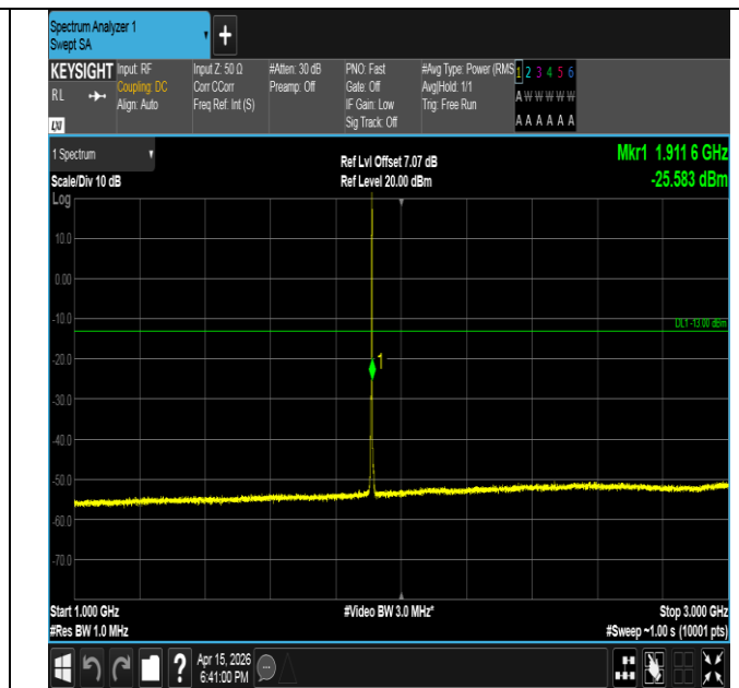
Band2-3MHz-16QAM-19185-1RB#14-1000~3000-PASS
