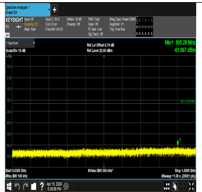
Band2-3MHz-QPSK-19185-1RB#14-30~1000-PASS
