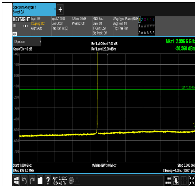
Band2-3MHz-QPSK-18900-1RB#14-1000~3000-PASS
