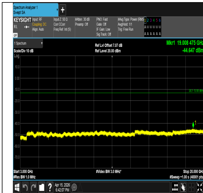
Band2-3MHz-QPSK-19185-15RB#0-3000~20000-PASS
