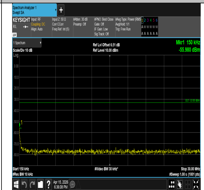
Band2-3MHz-QPSK-18900-15RB#0-0.15~30-PASS
