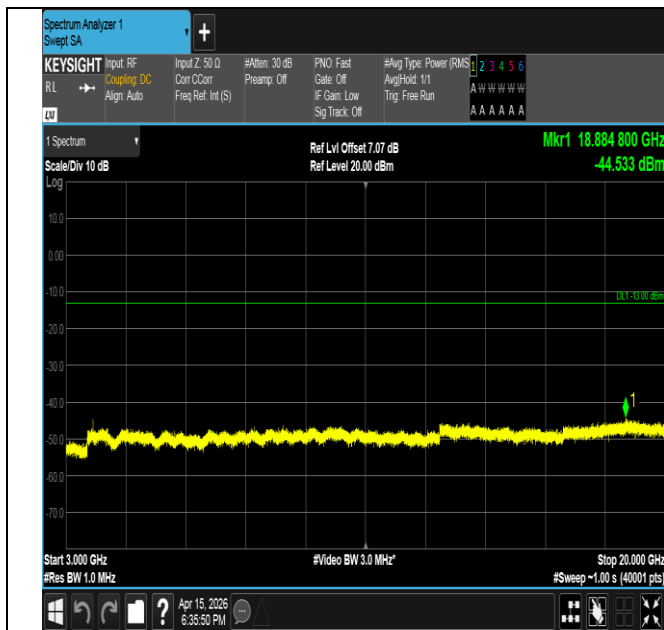
Band2-3MHz-16QAM-18900-1RB#14-3000~20000-PASS
