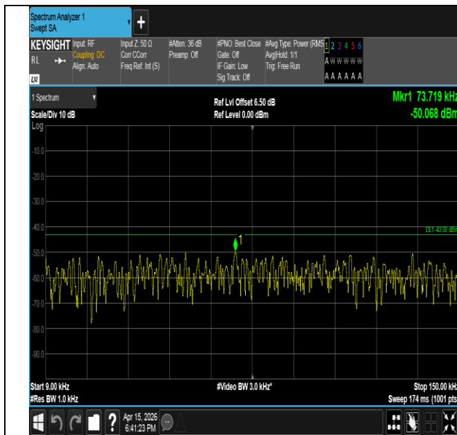
Band2-3MHz-QPSK-19185-15RB#0-0.009~0.15-PASS
