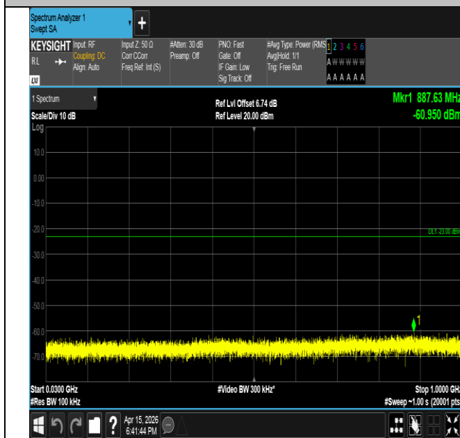
Band2-3MHz-QPSK-19185-15RB#0-30~1000-PASS
