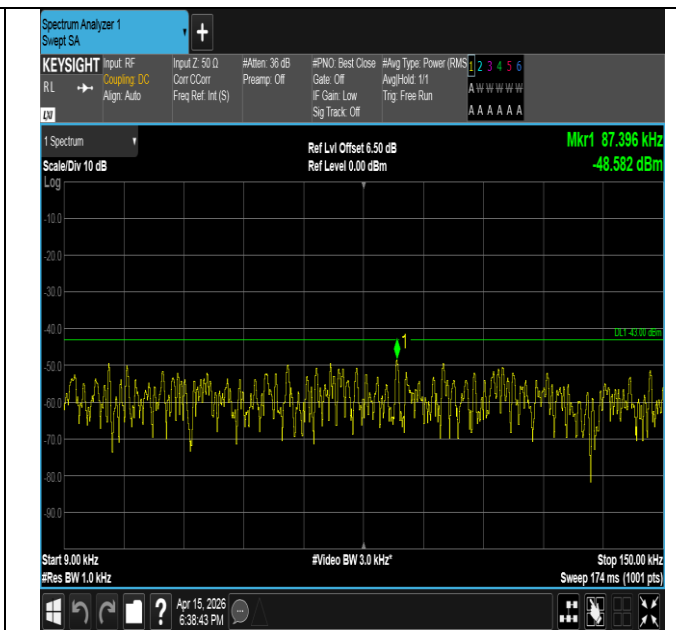
Band2-3MHz-16QAM-19185-1RB#0-0.009~0.15-PASS
