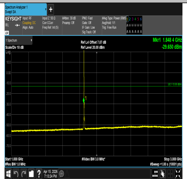
Band2-5MHz-QPSK-18625-1RB#0-1000~3000-PASS
