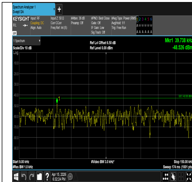
Band2-3MHz-QPSK-18900-1RB#0-0.009~0.15-PASS
