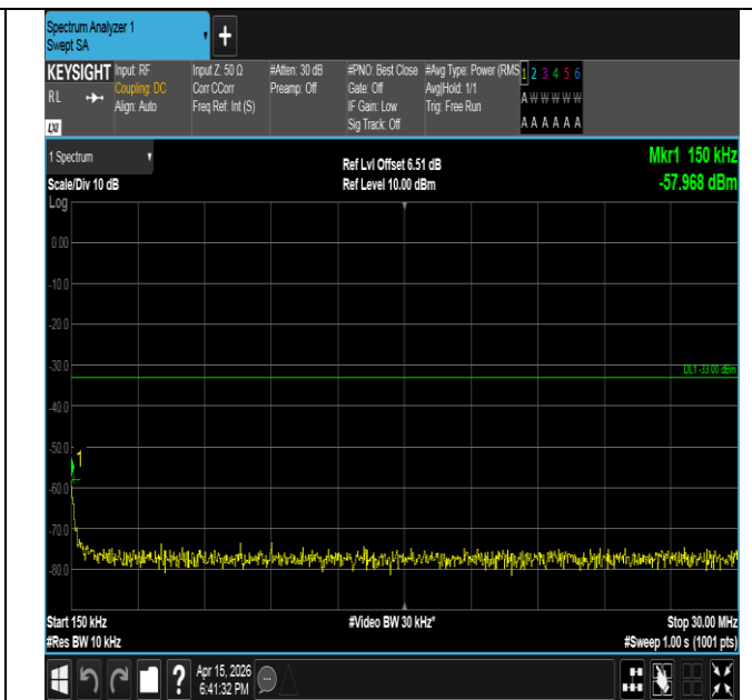
Band2-3MHz-QPSK-19185-15RB#0-0.15~30-PASS
