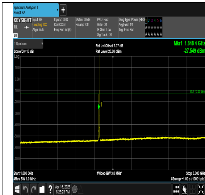
Band2-3MHz-16QAM-18615-1RB#0-1000~3000-PASS
