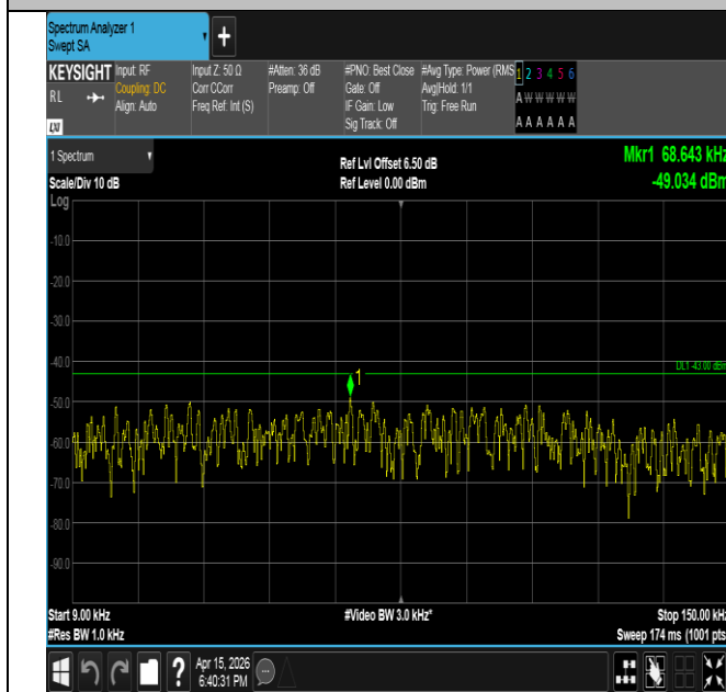
Band2-3MHz-16QAM-19185-1RB#14-0.009~0.15-PASS
