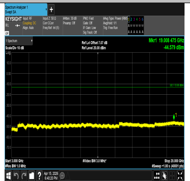
Band2-3MHz-QPSK-19185-1RB#14-3000~20000-PASS
