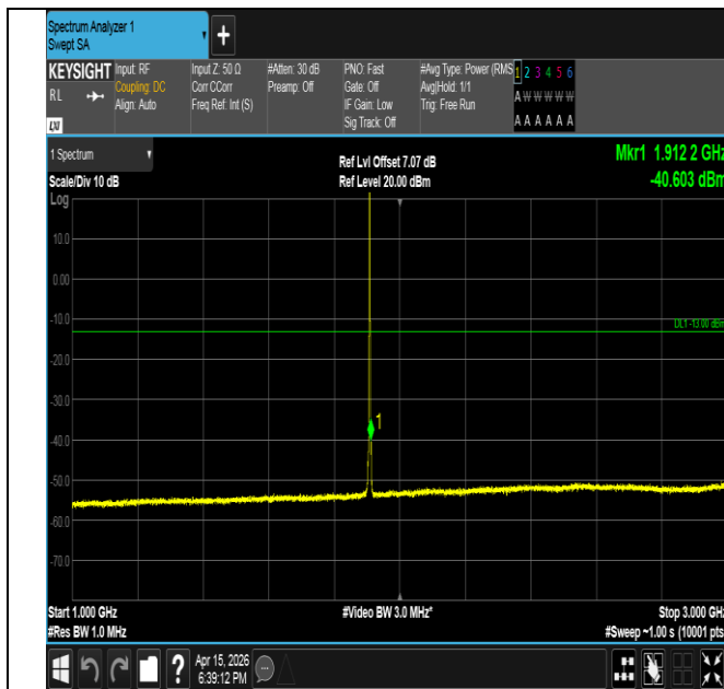
Band2-3MHz-16QAM-19185-1RB#0-1000~3000-PASS
