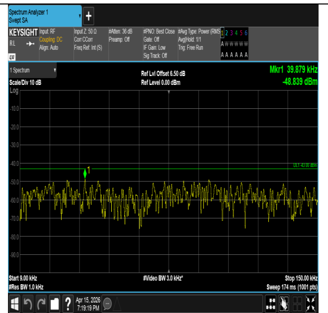
Band2-5MHz-16QAM-18900-1RB#0-0.009~0.15-PASS
