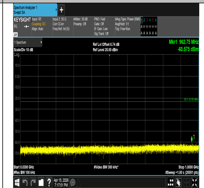
Band2-5MHz-16QAM-18625-25RB#0-30~1000-PASS
