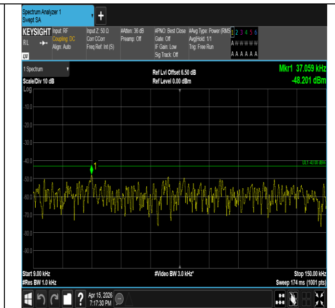
Band2-5MHz-16QAM-18625-25RB#0-0.009~0.15-PASS
