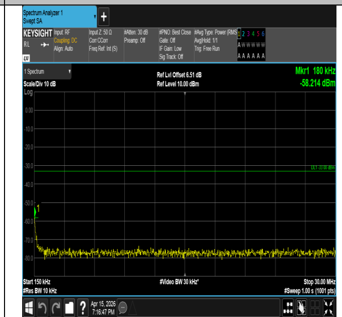
Band2-5MHz-QPSK-18625-25RB#0-0.15~30-PASS
