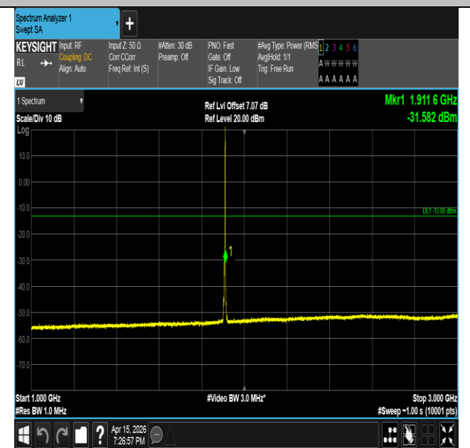
Band2-5MHz-16QAM-19175-1RB#24-1000~3000-PASS
