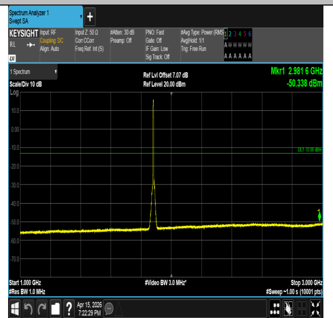
Band2-5MHz-QPSK-18900-25RB#0-1000~3000-PASS
