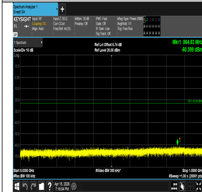
Band2-5MHz-16QAM-18625-1RB#24-30~1000-PASS
