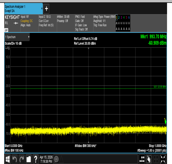
Band2-5MHz-16QAM-18900-1RB#0-30~1000-PASS
