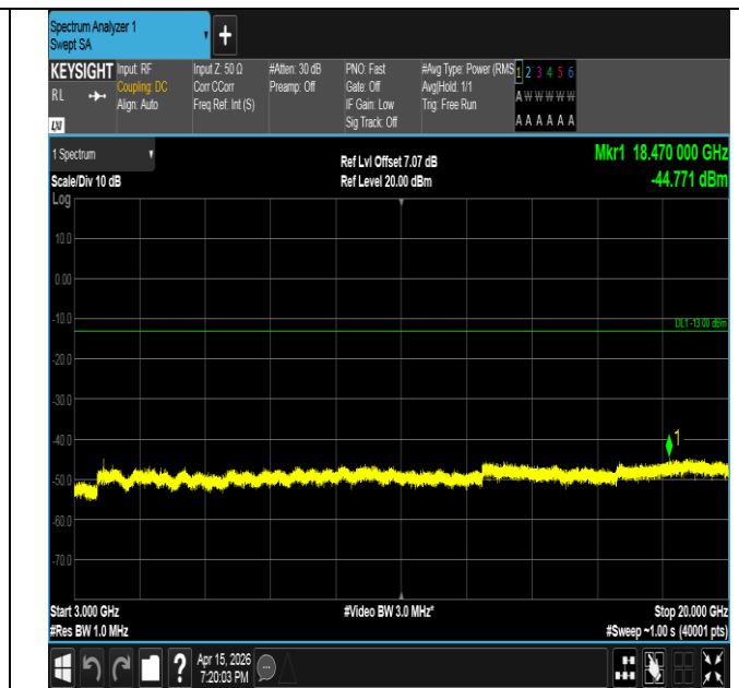
Band2-5MHz-16QAM-18900-1RB#0-3000~20000-PASS
