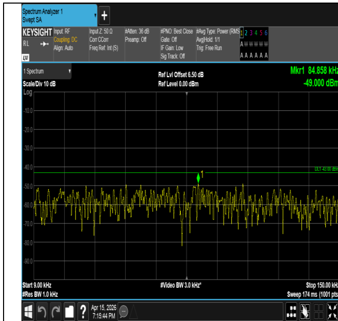
Band2-5MHz-16QAM-18625-1RB#24-0.009~0.15-PASS
