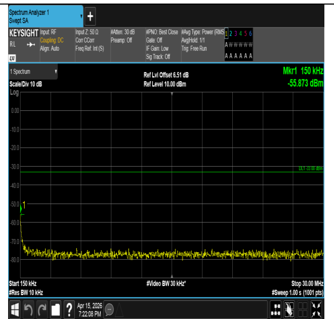
Band2-5MHz-QPSK-18900-25RB#0-0.15~30-PASS
