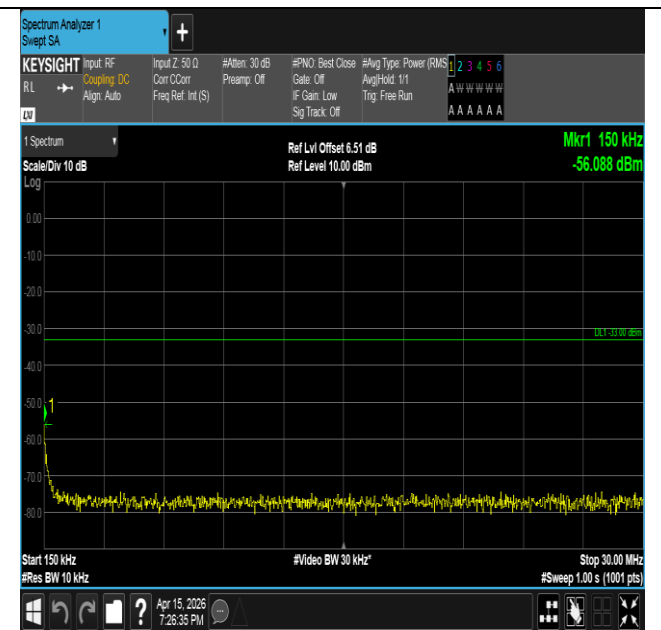
Band2-5MHz-16QAM-19175-1RB#24-0.15~30-PASS
