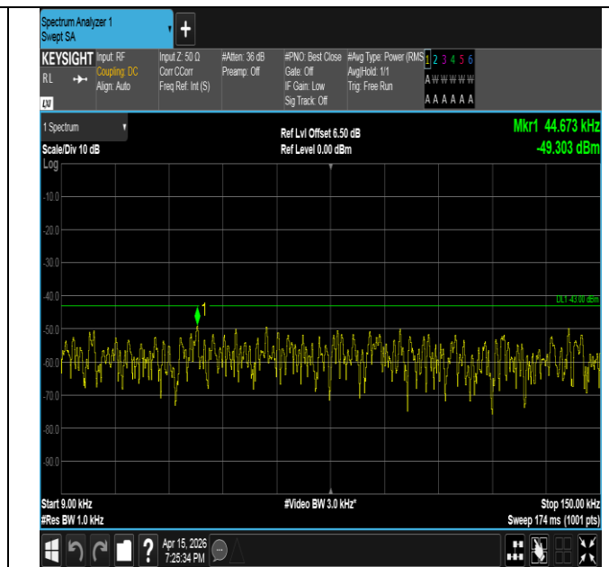
Band2-5MHz-QPSK-19175-1RB#24-0.009~0.15-PASS
