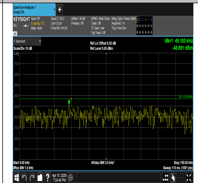
Band2-5MHz-16QAM-19175-1RB#0-0.009~0.15-PASS
