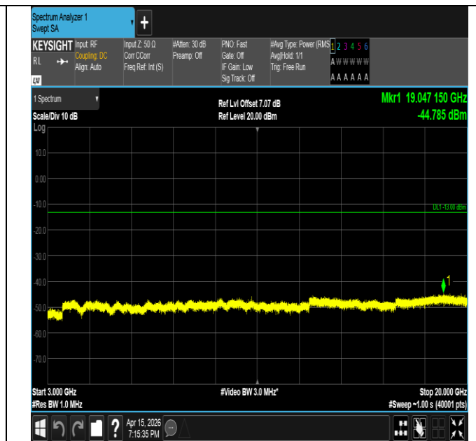
Band2-5MHz-QPSK-18625-1RB#24-3000~20000-PASS
