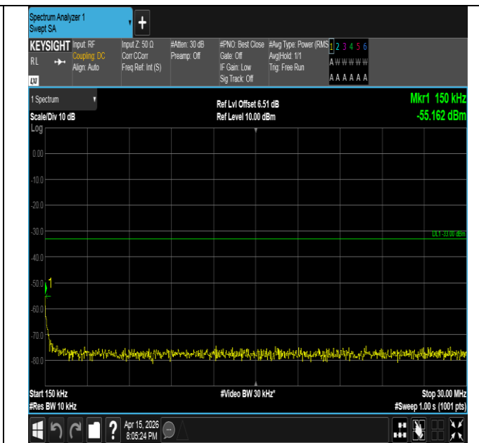
Band2-10MHz-16QAM-18900-1RB#49-0.15~30-PASS
