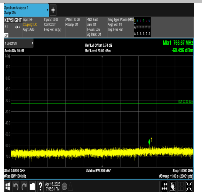
Band2-10MHz-16QAM-18650-1RB#0-30~1000-PASS
