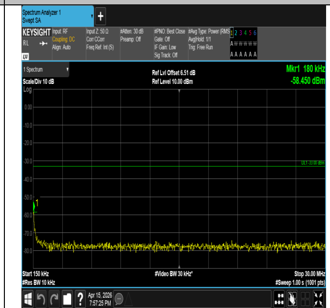
Band2-10MHz-QPSK-18650-1RB#0-0.15~30-PASS
