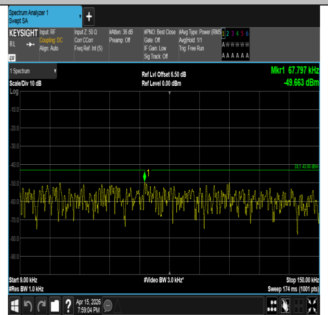
Band2-10MHz-QPSK-18650-1RB#49-0.009~0.15-PASS
