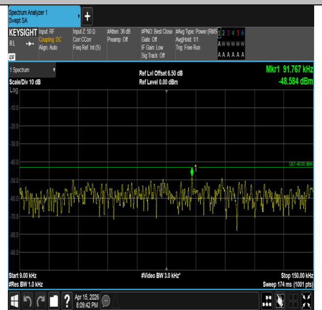
Band2-10MHz-QPSK-19150-1RB#49-0.009~0.15-PASS
