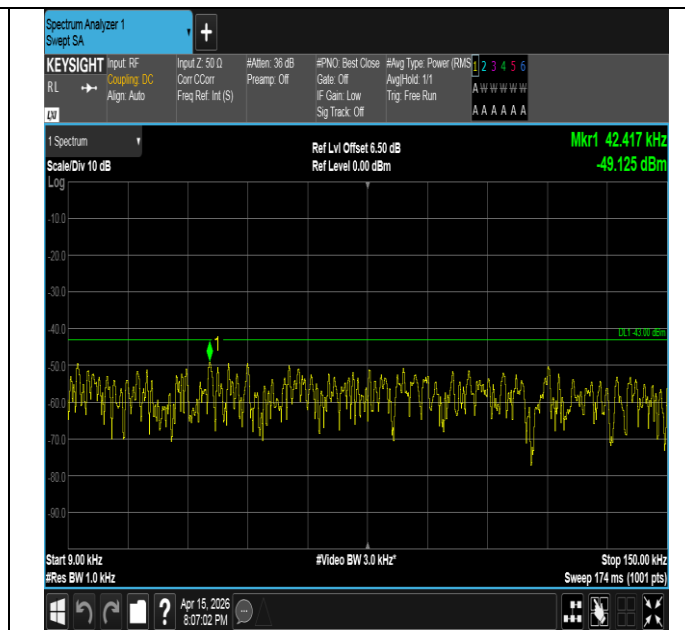
Band2-10MHz-16QAM-18900-50RB#0-0.009~0.15-PASS
