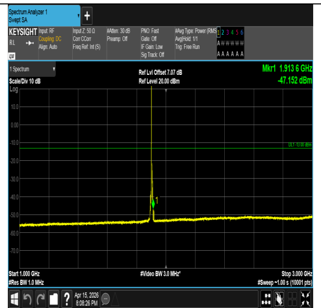
Band2-10MHz-QPSK-19150-1RB#0-1000~3000-PASS
