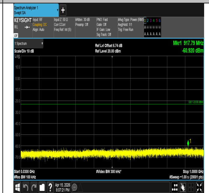
Band2-10MHz-16QAM-18900-50RB#0-30~1000-PASS
