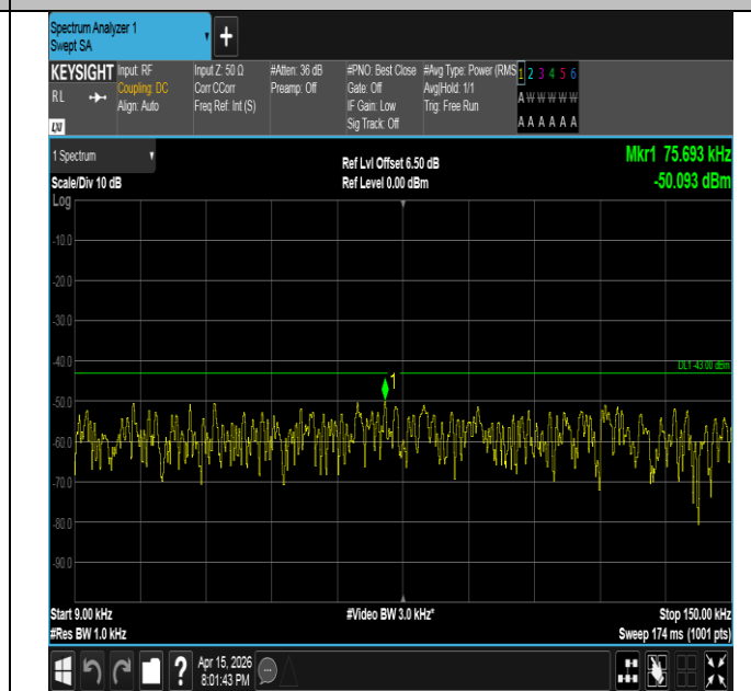
Band2-10MHz-16QAM-18650-50RB#0-0.009~0.15-PASS
