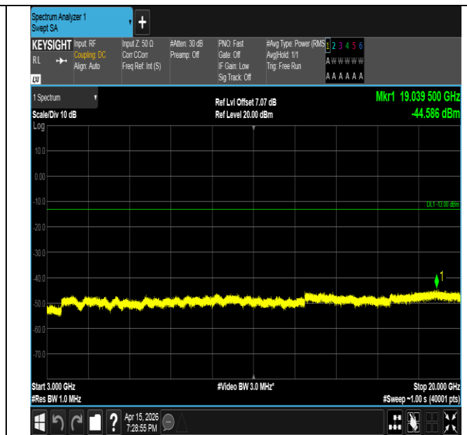
Band2-5MHz-16QAM-19175-25RB#0-3000~20000-PASS
