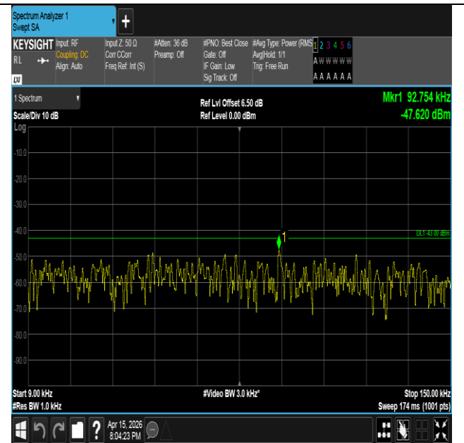
Band2-10MHz-QPSK-18900-1RB#49-0.009~0.15-PASS
