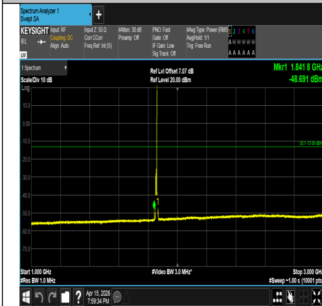
Band2-10MHz-QPSK-18650-1RB#49-1000~3000-PASS
