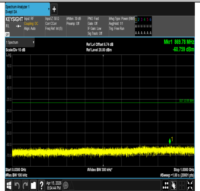
Band2-10MHz-QPSK-18900-1RB#49-30~1000-PASS
