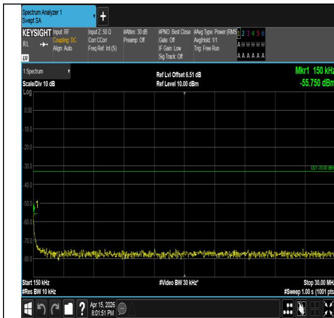
Band2-10MHz-16QAM-18650-50RB#0-0.15~30-PASS
