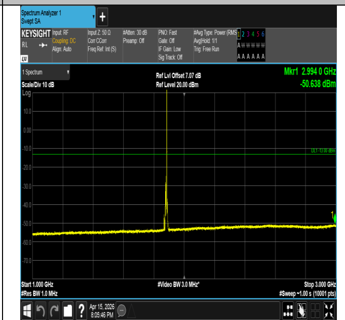
Band2-10MHz-16QAM-18900-1RB#49-1000~3000-PASS
