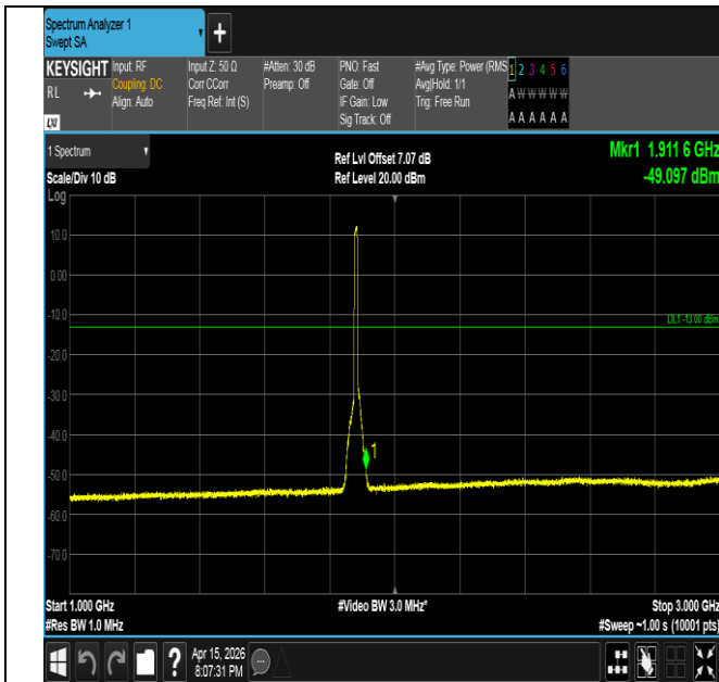
Band2-10MHz-16QAM-18900-50RB#0-1000~3000-PASS
