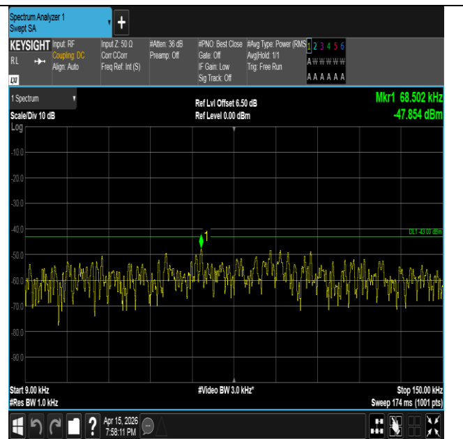
Band2-10MHz-16QAM-18650-1RB#0-0.009~0.15-PASS
