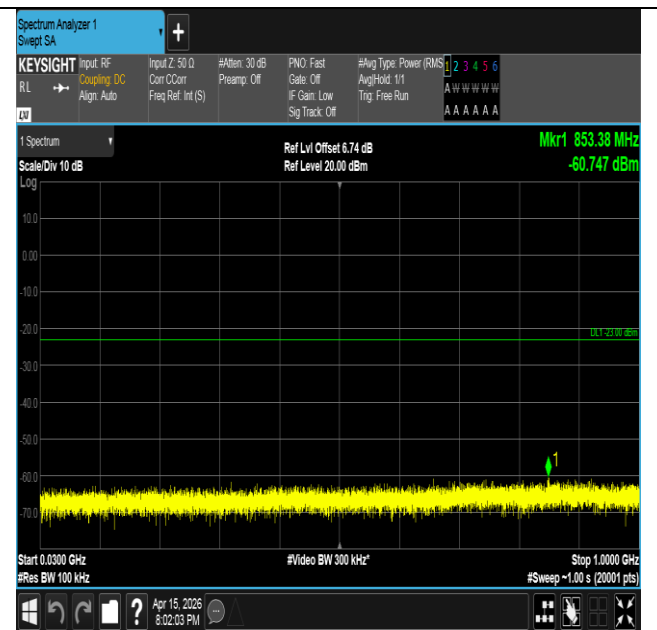
Band2-10MHz-16QAM-18650-50RB#0-30~1000-PASS
