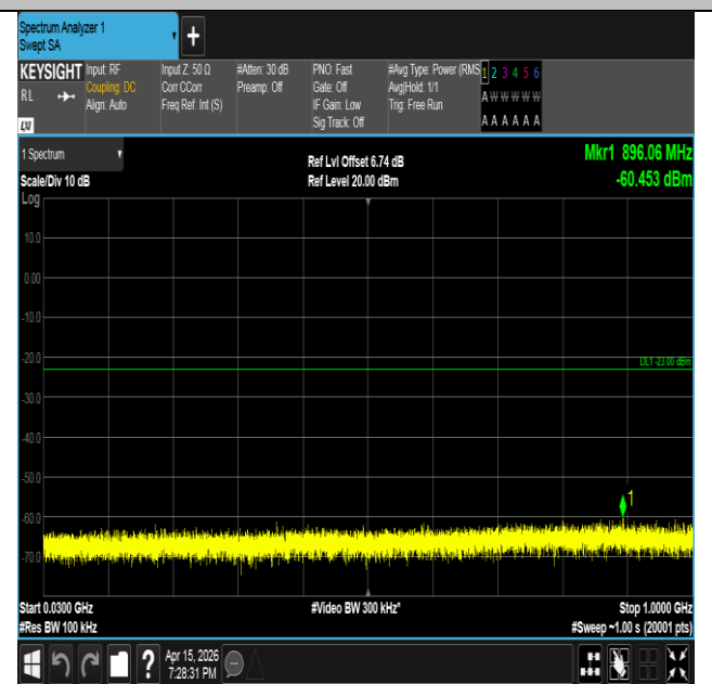
Band2-5MHz-16QAM-19175-25RB#0-30~1000-PASS
