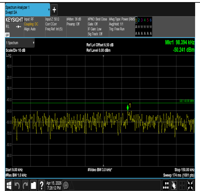
Band2-5MHz-16QAM-19175-25RB#0-0.009~0.15-PASS
