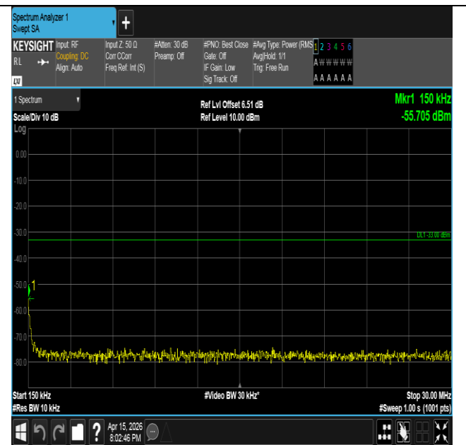
Band2-10MHz-QPSK-18900-1RB#0-0.15~30-PASS
