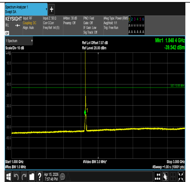
Band2-10MHz-QPSK-18650-1RB#0-1000~3000-PASS
