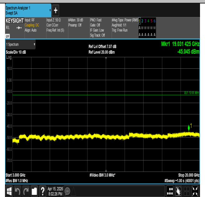
Band2-10MHz-16QAM-18650-50RB#0-3000~20000-PASS
