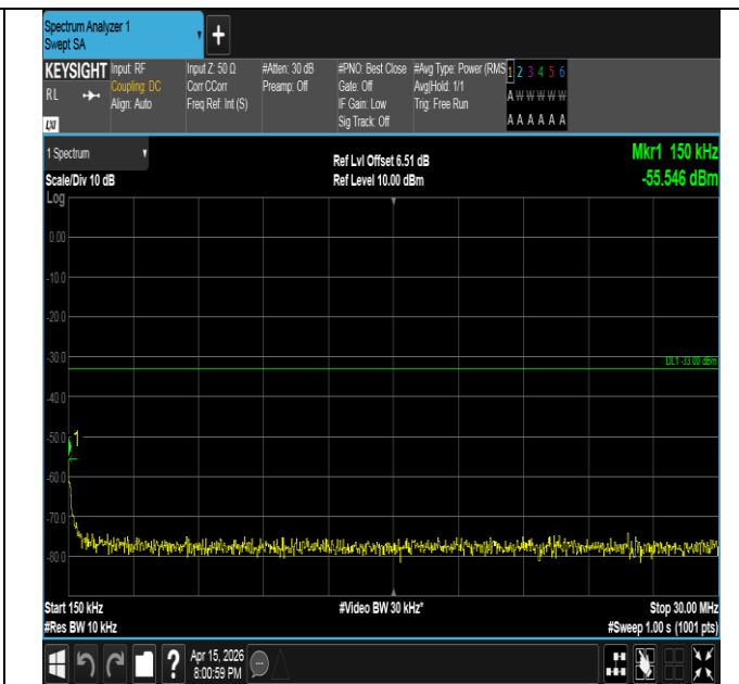
Band2-10MHz-QPSK-18650-50RB#0-0.15~30-PASS
