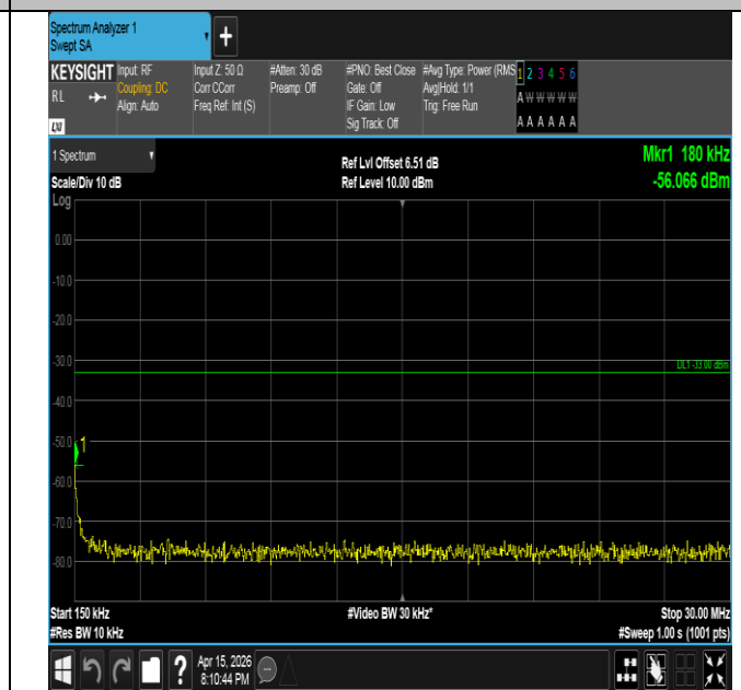
Band2-10MHz-16QAM-19150-1RB#49-0.15~30-PASS
