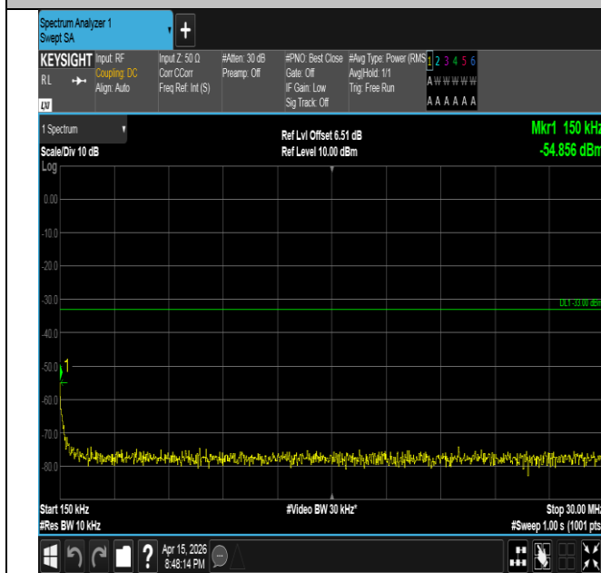
Band2-15MHz-16QAM-18900-1RB#0-0.15~30-PASS
