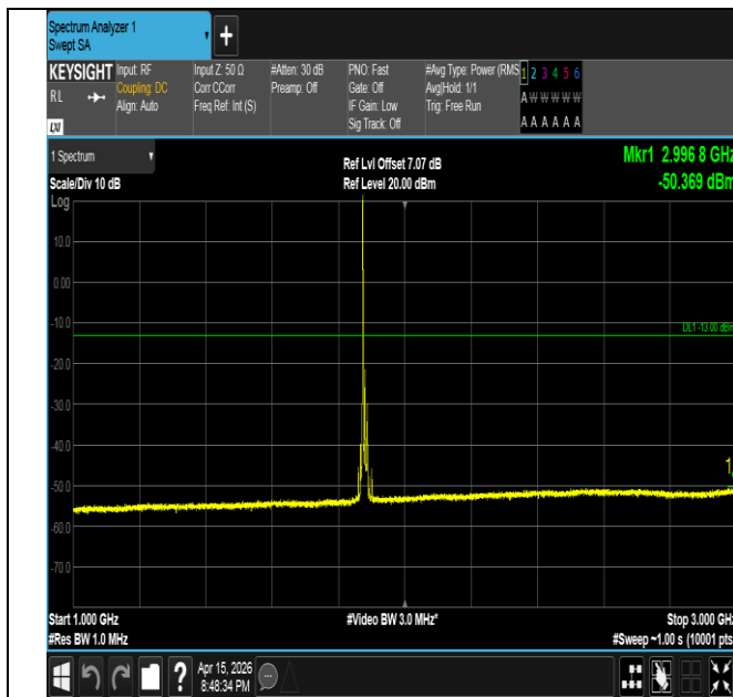
Band2-15MHz-16QAM-18900-1RB#0-1000~3000-PASS
