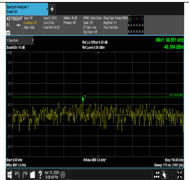
Band2-10MHz-16QAM-19150-1RB#0-0.009~0.15-PASS
