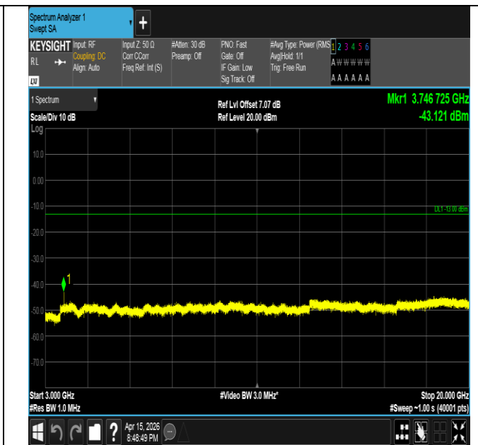
Band2-15MHz-16QAM-18900-1RB#0-3000~20000-PASS
