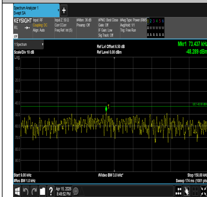
Band2-15MHz-16QAM-18900-1RB#74-0.009~0.15-PASS
