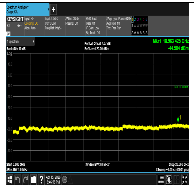
Band2-15MHz-16QAM-18675-75RB#0-3000~20000-PASS
