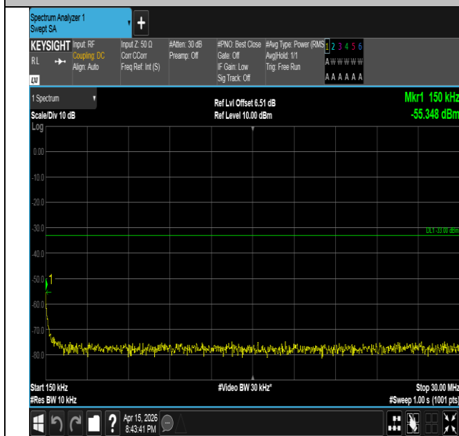
Band2-15MHz-QPSK-18675-1RB#74-0.15~30-PASS
