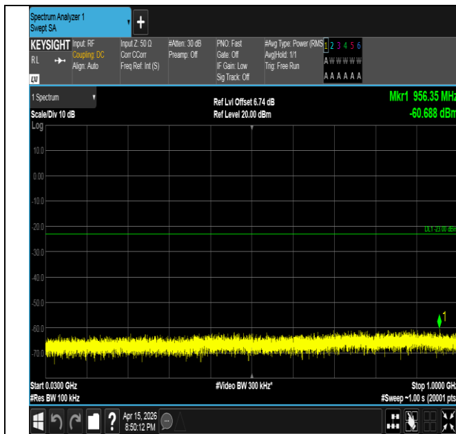
Band2-15MHz-16QAM-18900-1RB#74-30~1000-PASS
