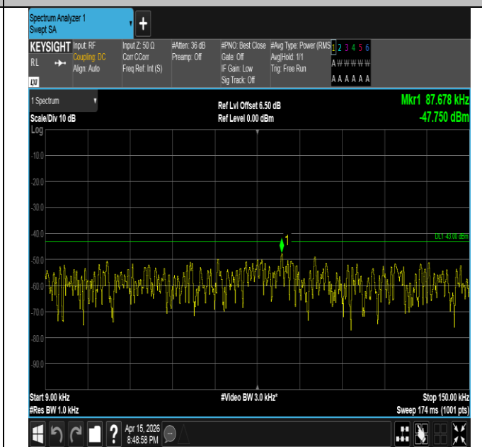
Band2-15MHz-QPSK-18900-1RB#74-0.009~0.15-PASS
