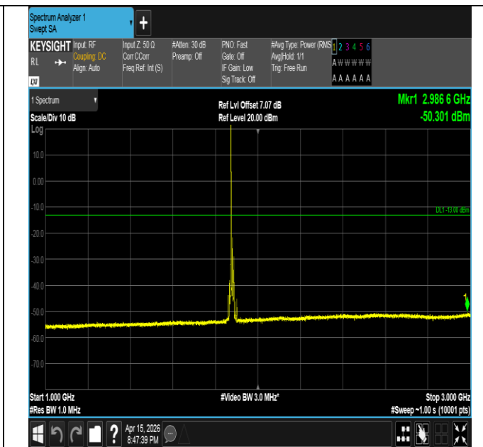
Band2-15MHz-QPSK-18900-1RB#0-1000~3000-PASS
