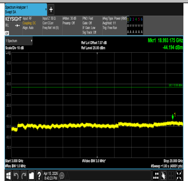
Band2-15MHz-16QAM-18675-1RB#0-3000~20000-PASS
