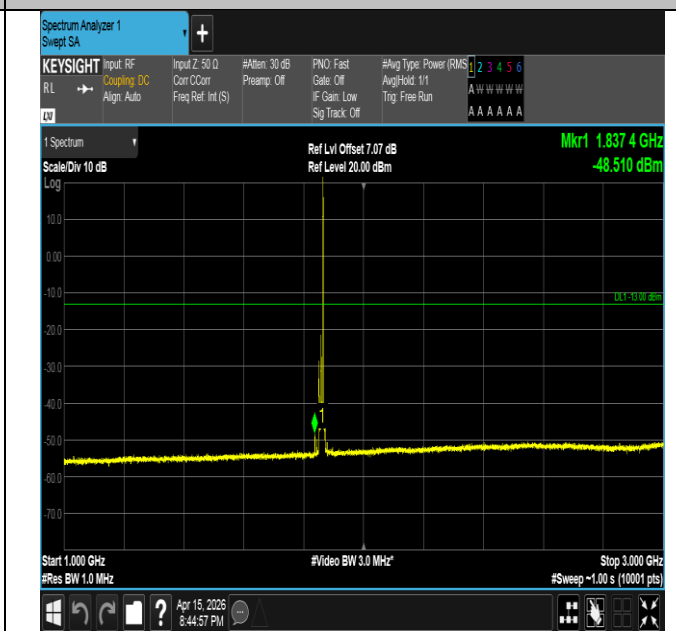
Band2-15MHz-16QAM-18675-1RB#74-1000~3000-PASS
