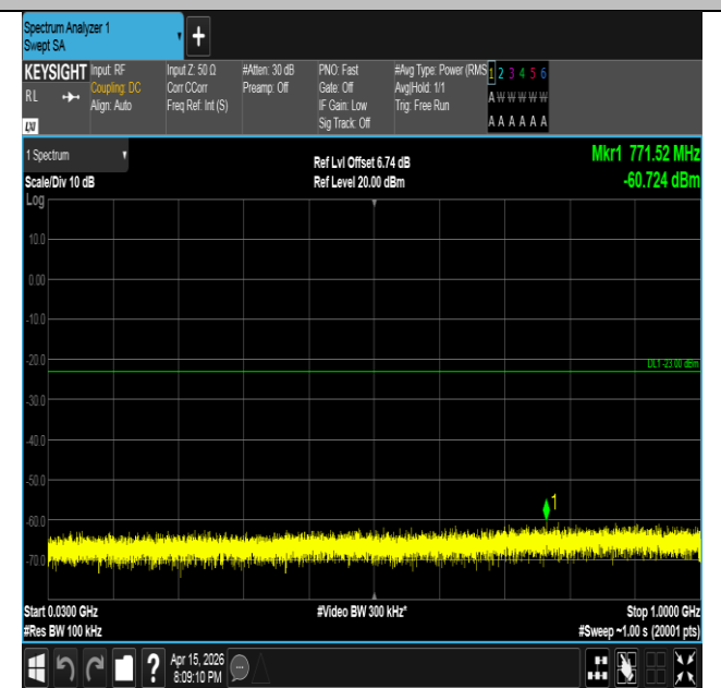
Band2-10MHz-16QAM-19150-1RB#0-30~1000-PASS
