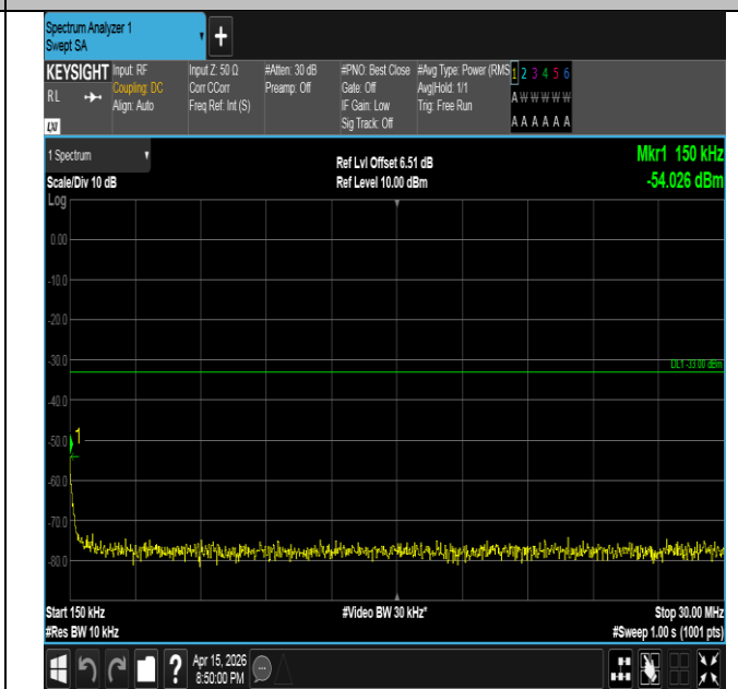
Band2-15MHz-16QAM-18900-1RB#74-0.15~30-PASS
