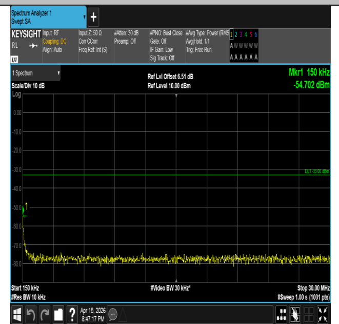
Band2-15MHz-QPSK-18900-1RB#0-0.15~30-PASS
