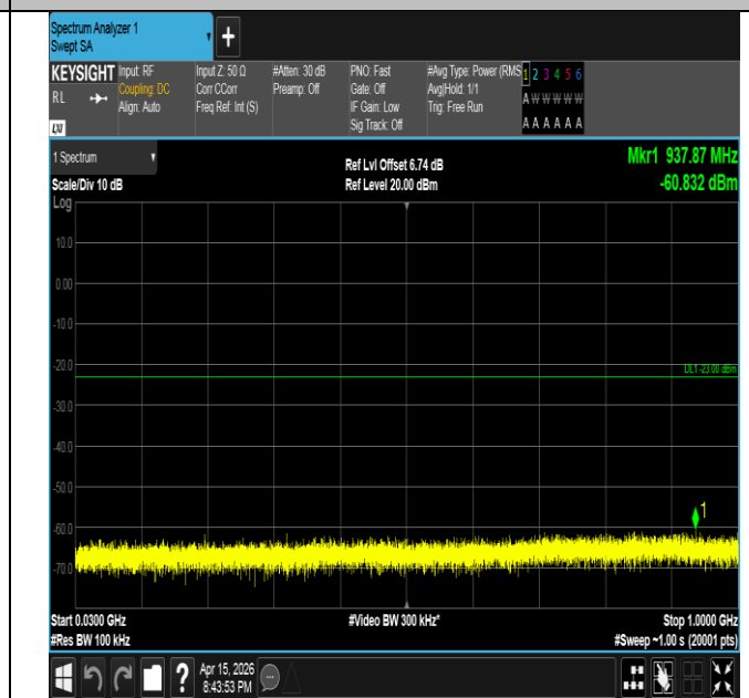
Band2-15MHz-QPSK-18675-1RB#74-30~1000-PASS
