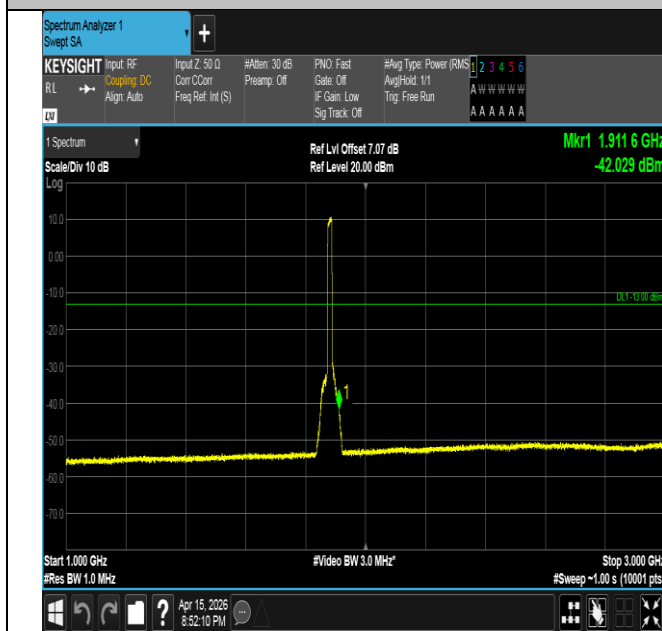
Band2-15MHz-16QAM-18900-75RB#0-1000~3000-PASS
