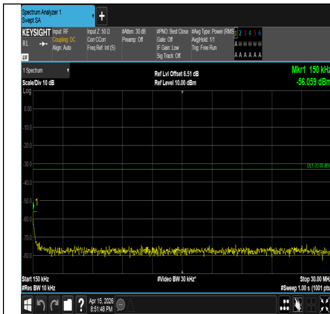
Band2-15MHz-16QAM-18900-75RB#0-0.15~30-PASS
