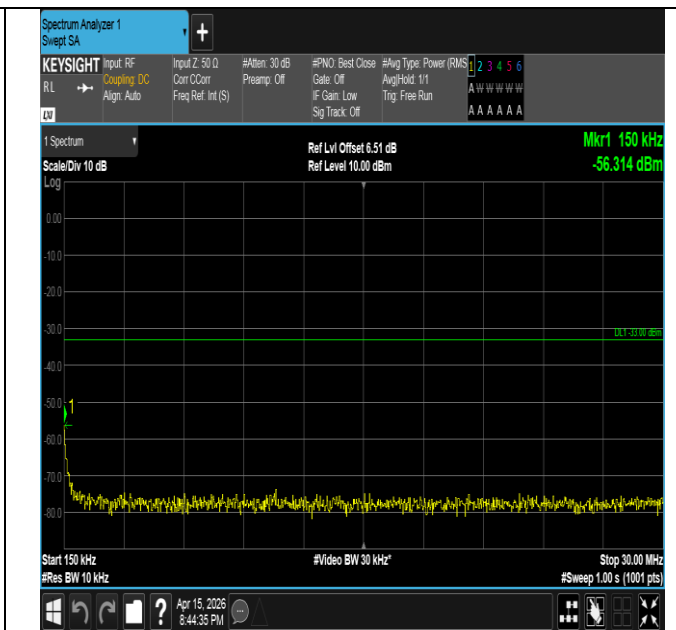
Band2-15MHz-16QAM-18675-1RB#74-0.15~30-PASS
