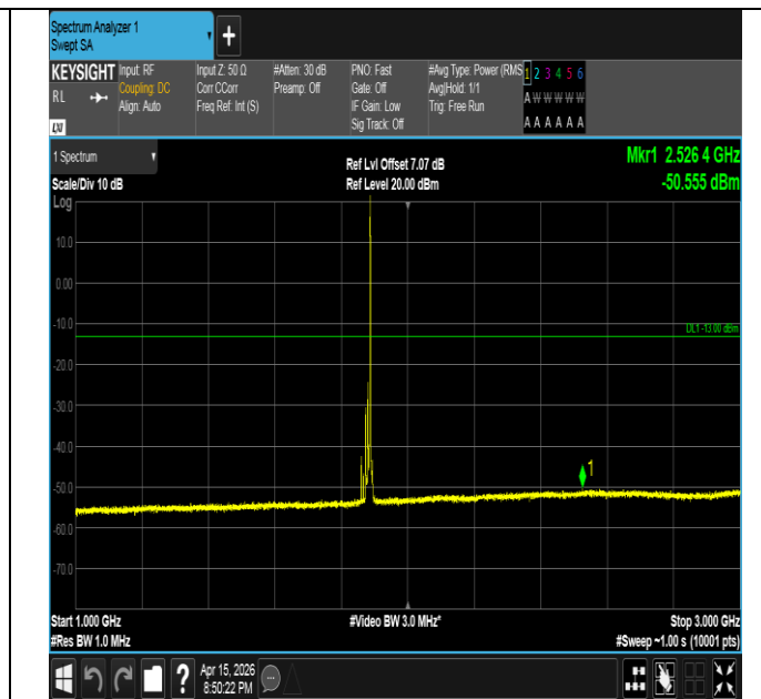
Band2-15MHz-16QAM-18900-1RB#74-1000~3000-PASS
