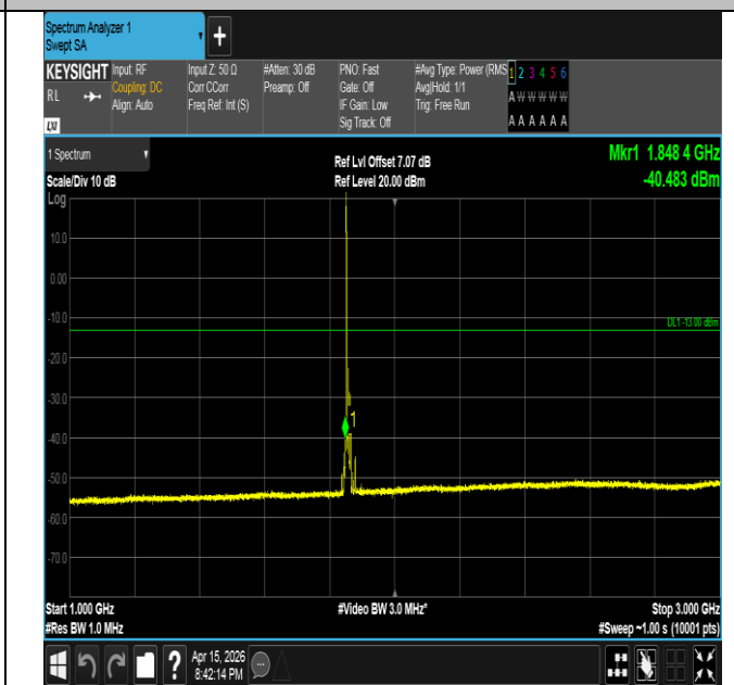
Band2-15MHz-QPSK-18675-1RB#0-1000~3000-PASS
