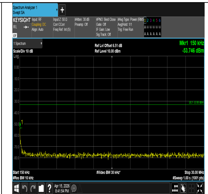
Band2-15MHz-QPSK-18675-1RB#0-0.15~30-PASS
