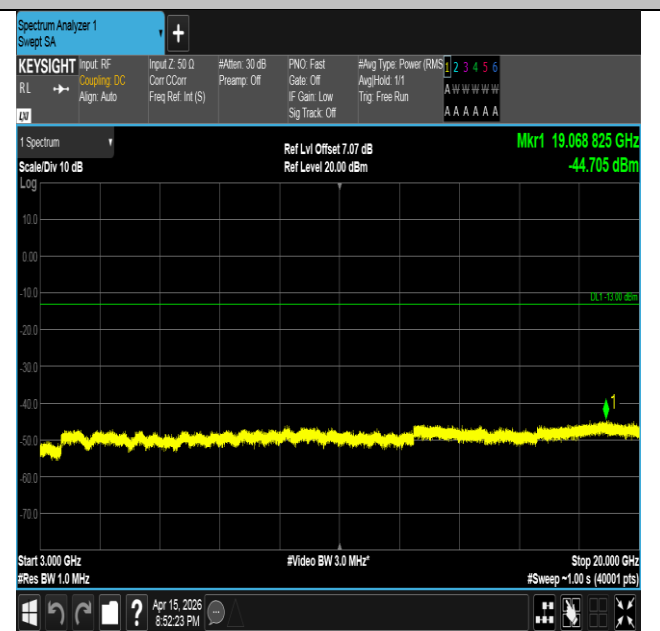
Band2-15MHz-16QAM-18900-75RB#0-3000~20000-PASS
