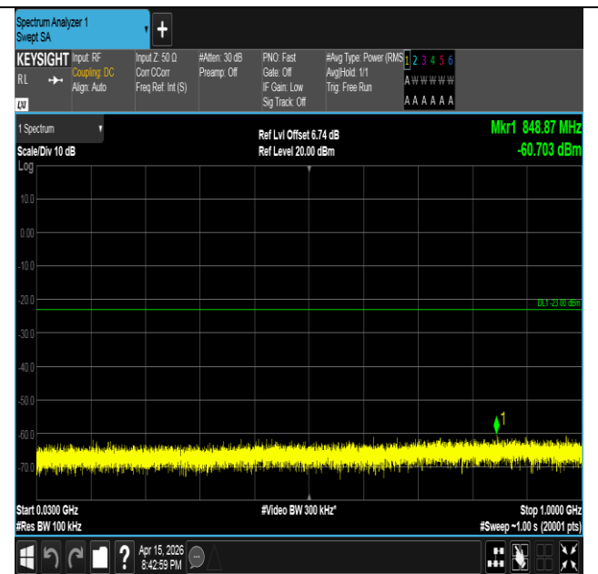
Band2-15MHz-16QAM-18675-1RB#0-30~1000-PASS
