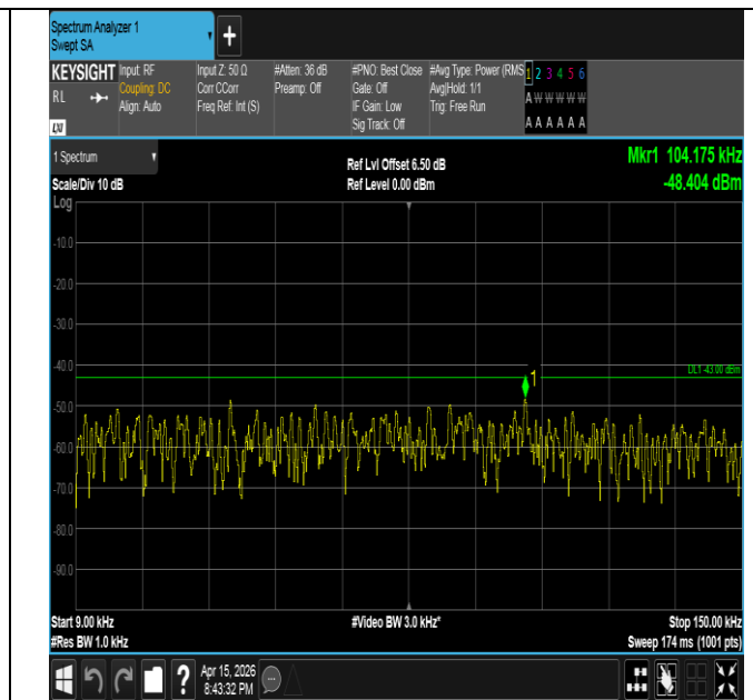
Band2-15MHz-QPSK-18675-1RB#74-0.009~0.15-PASS
