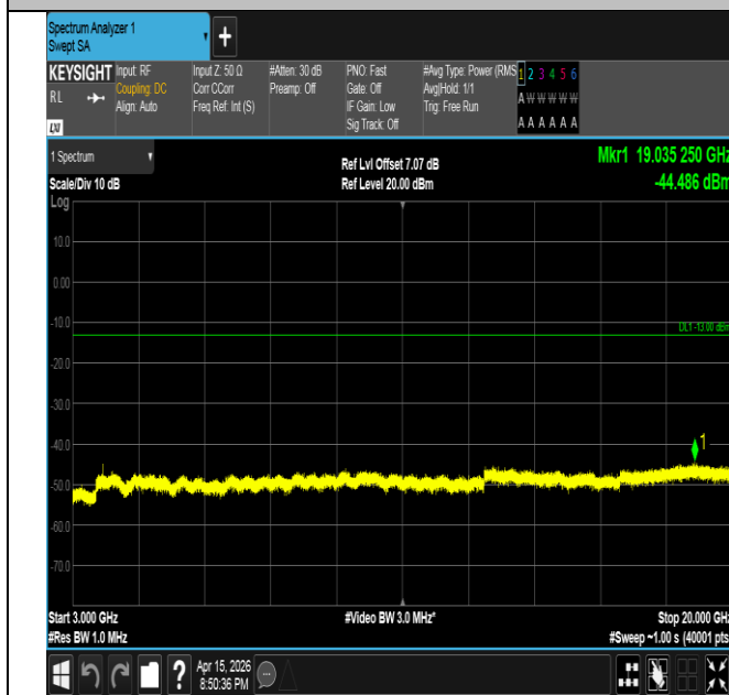
Band2-15MHz-16QAM-18900-1RB#74-3000~20000-PASS
