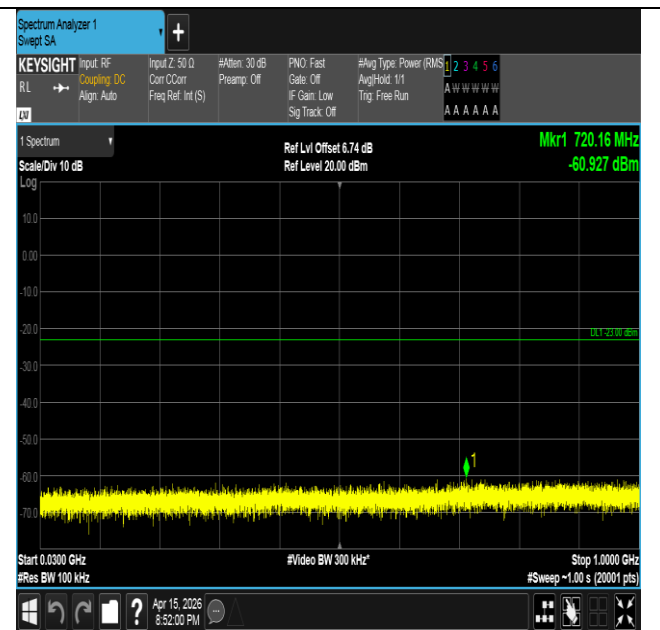
Band2-15MHz-16QAM-18900-75RB#0-30~1000-PASS
