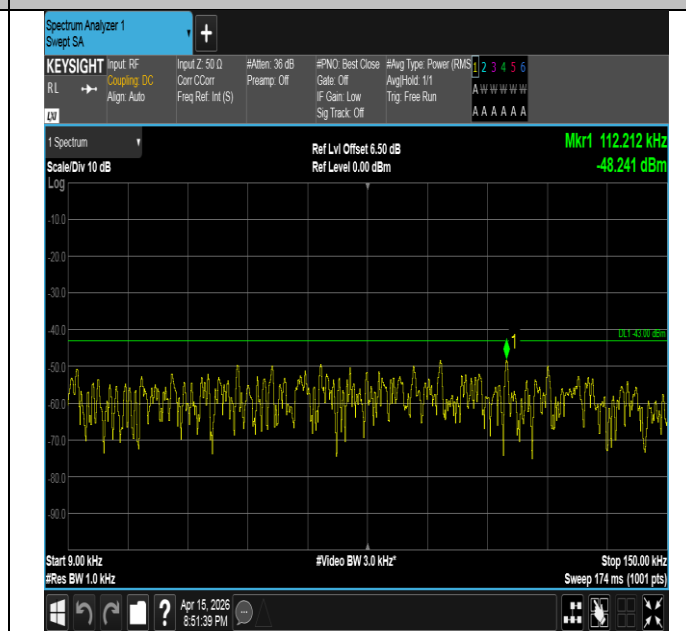
Band2-15MHz-16QAM-18900-75RB#0-0.009~0.15-PASS
