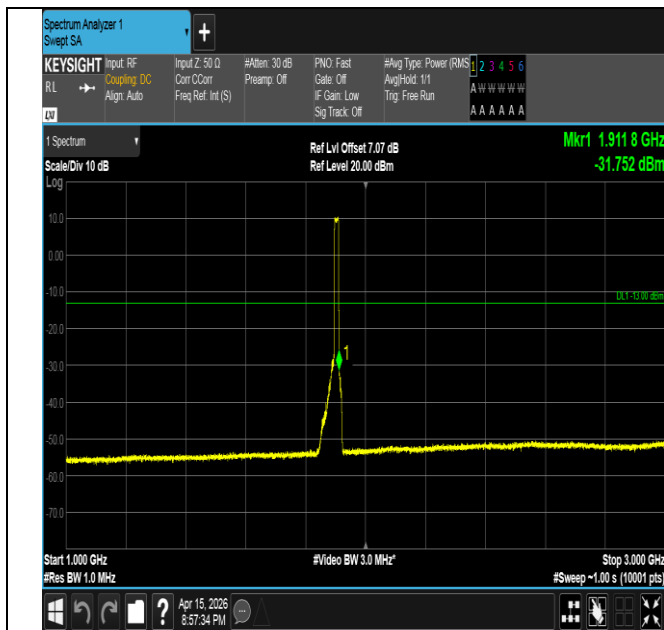
Band2-15MHz-16QAM-19125-75RB#0-1000~3000-PASS
