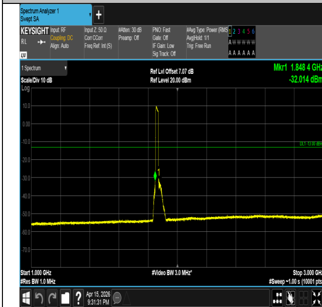
Band2-20MHz-16QAM-18700-100RB#0-1000~3000-PASS
