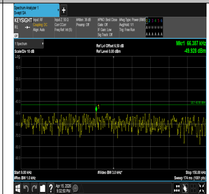
Band2-20MHz-16QAM-18900-1RB#0-0.009~0.15-PASS
