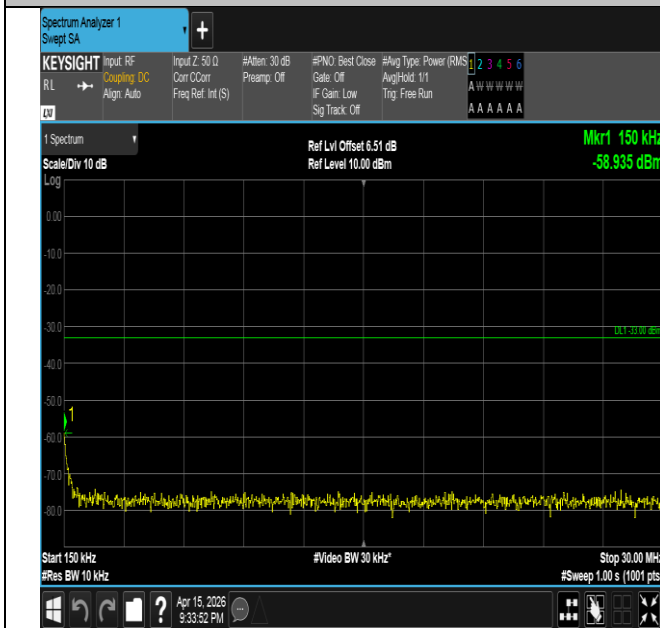
Band2-20MHz-QPSK-18900-1RB#99-0.15~30-PASS
