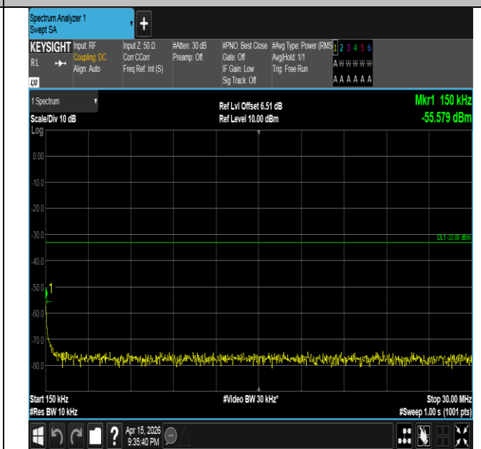
Band2-20MHz-QPSK-18900-100RB#0-0.15~30-PASS
