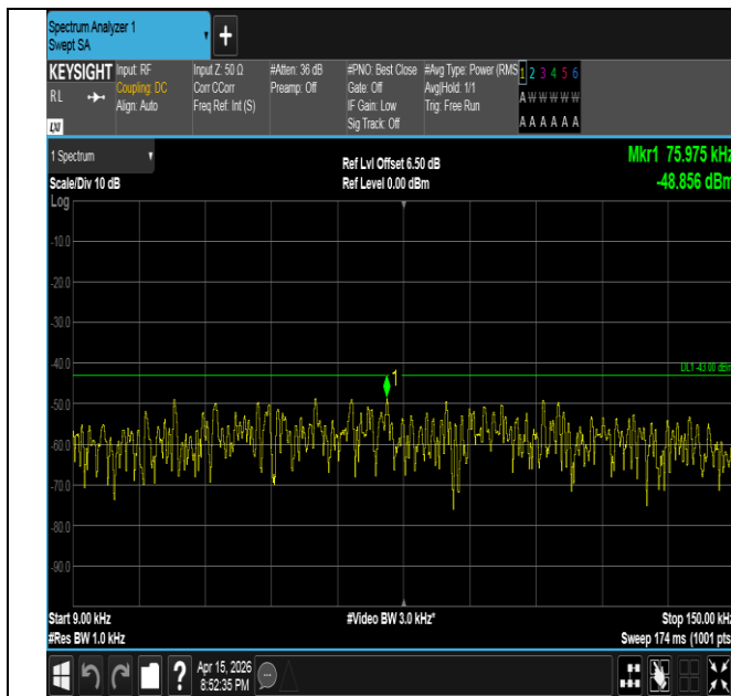
Band2-15MHz-QPSK-19125-1RB#0-0.009~0.15-PASS
