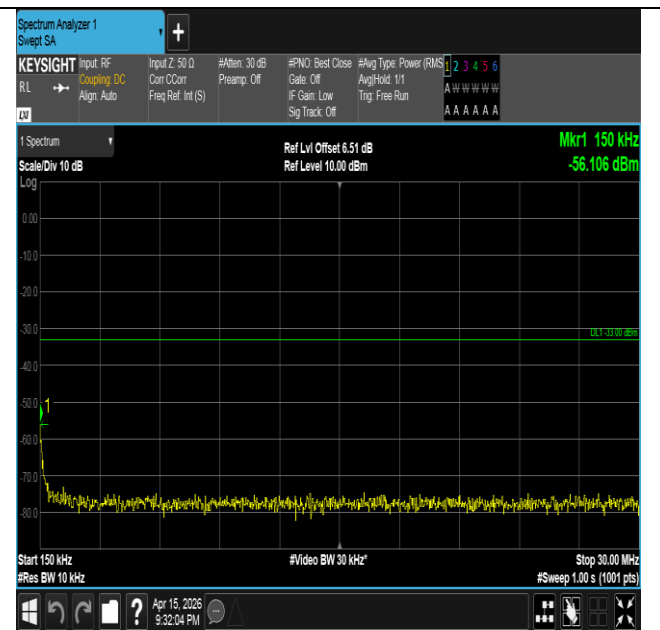
Band2-20MHz-QPSK-18900-1RB#0-0.15~30-PASS
