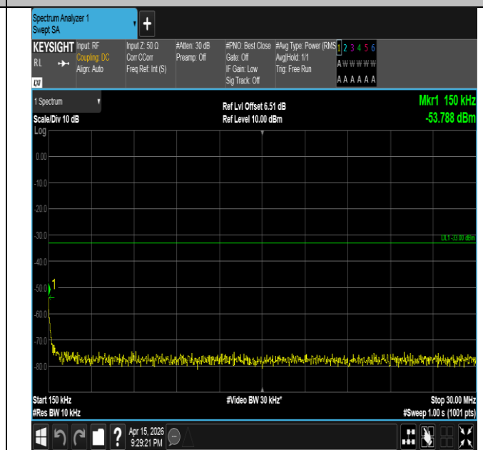
Band2-20MHz-16QAM-18700-1RB#99-0.15~30-PASS
