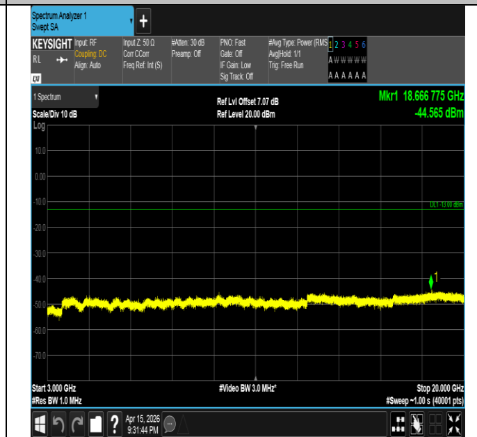
Band2-20MHz-16QAM-18700-100RB#0-3000~20000-PASS
