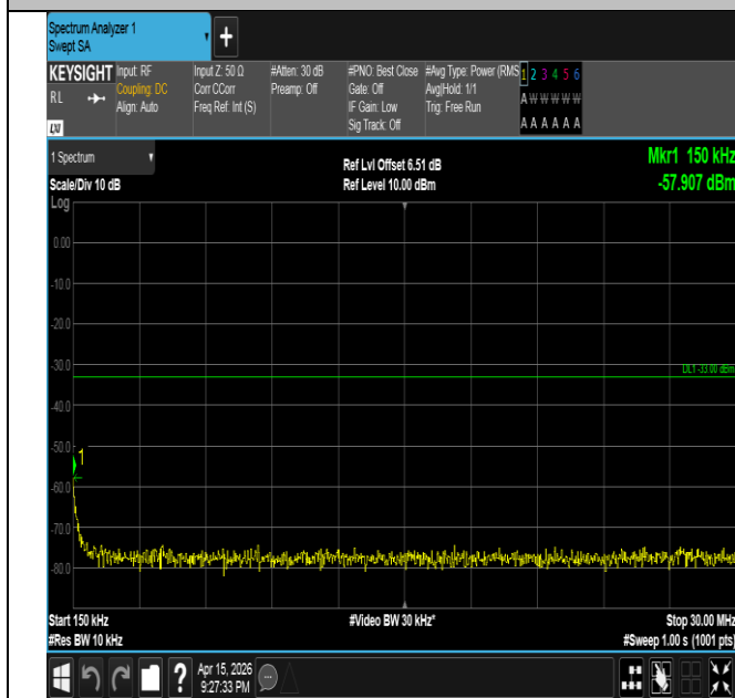
Band2-20MHz-16QAM-18700-1RB#0-0.15~30-PASS
