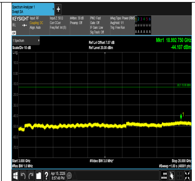
Band2-15MHz-16QAM-19125-75RB#0-3000~20000-PASS
