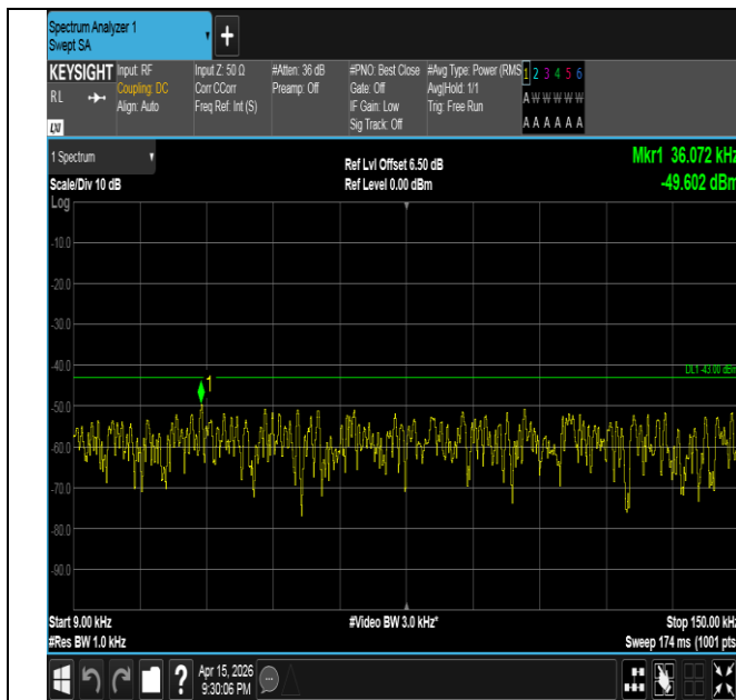
Band2-20MHz-QPSK-18700-100RB#0-0.009~0.15-PASS
