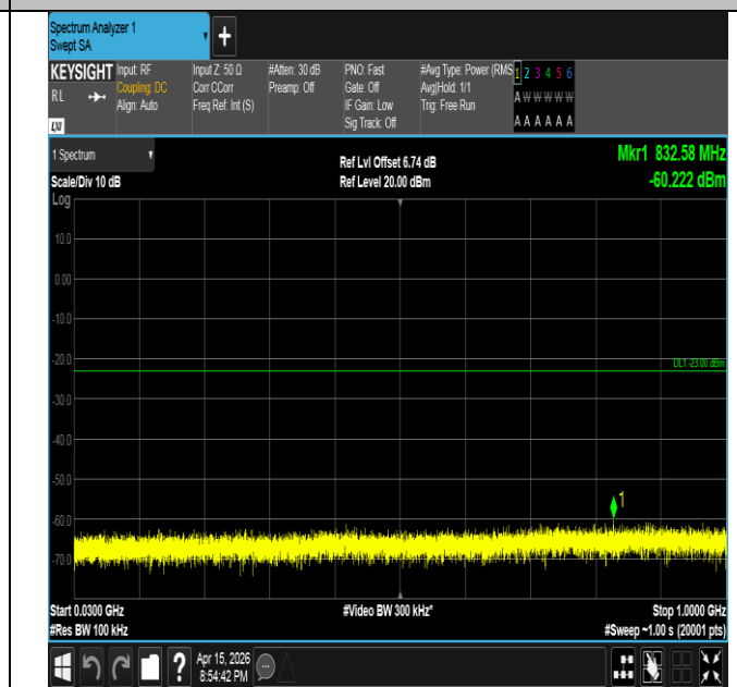
Band2-15MHz-QPSK-19125-1RB#74-30~1000-PASS
