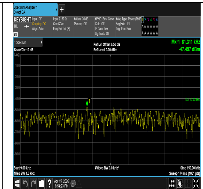
Band2-15MHz-QPSK-19125-1RB#74-0.009~0.15-PASS
