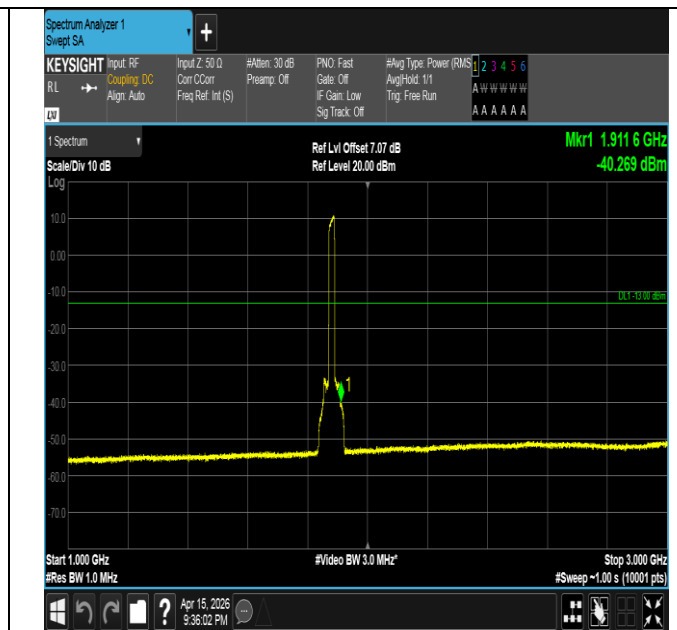
Band2-20MHz-QPSK-18900-100RB#0-1000~3000-PASS
