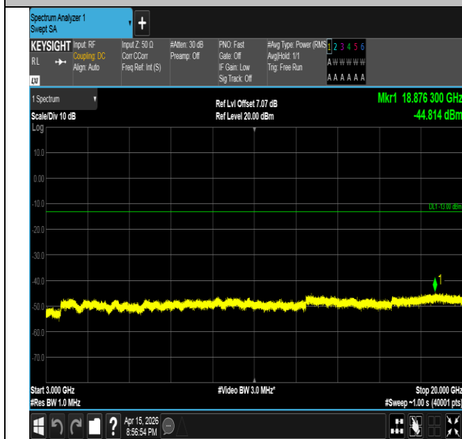
Band2-15MHz-QPSK-19125-75RB#0-3000~20000-PASS
