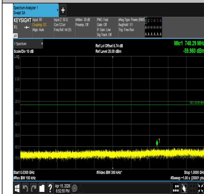
Band2-15MHz-QPSK-19125-1RB#0-30~1000-PASS
