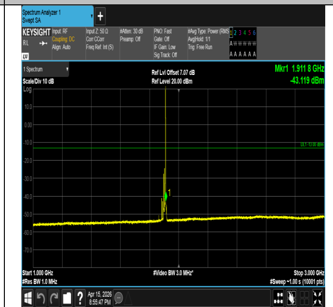
Band2-15MHz-16QAM-19125-1RB#74-1000~3000-PASS
