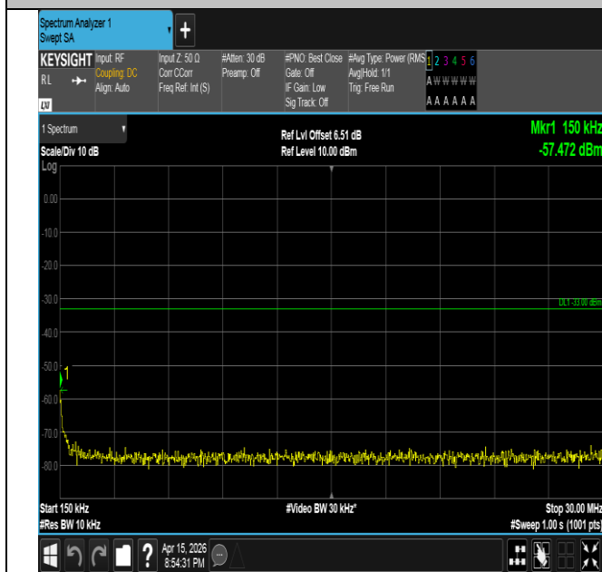
Band2-15MHz-QPSK-19125-1RB#74-0.15~30-PASS
