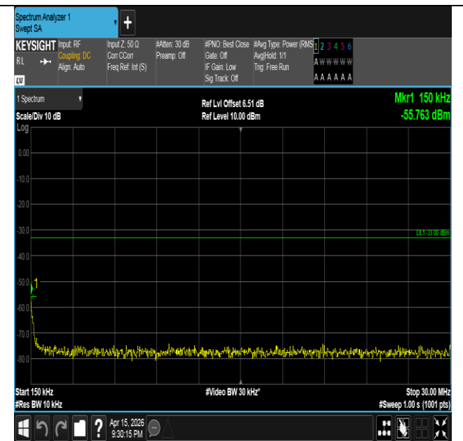
Band2-20MHz-QPSK-18700-100RB#0-0.15~30-PASS
