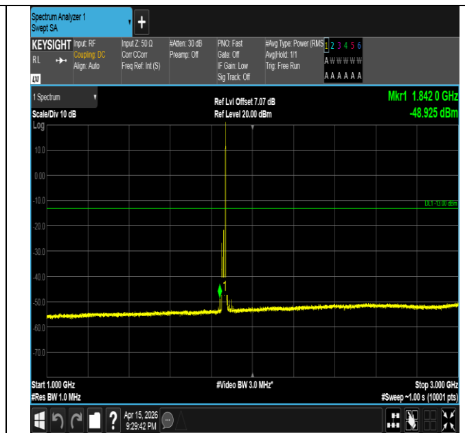
Band2-20MHz-16QAM-18700-1RB#99-1000~3000-PASS
