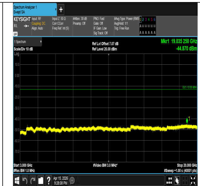
Band2-20MHz-16QAM-18700-1RB#0-3000~20000-PASS
