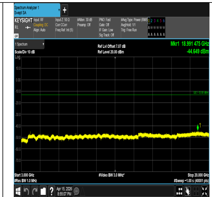
Band2-15MHz-QPSK-19125-1RB#74-3000~20000-PASS
