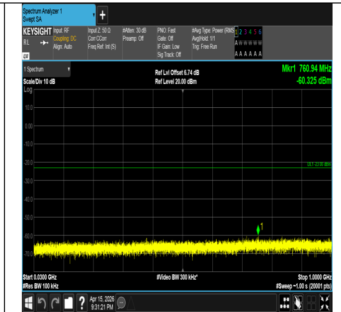
Band2-20MHz-16QAM-18700-100RB#0-30~1000-PASS
