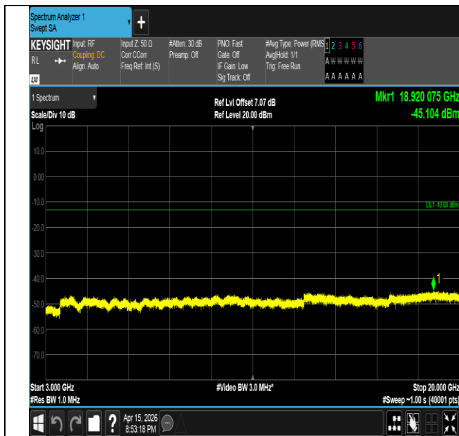
Band2-15MHz-QPSK-19125-1RB#0-3000~20000-PASS
