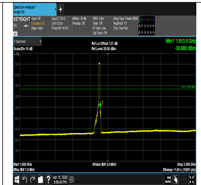
Band2-15MHz-QPSK-19125-75RB#0-1000~3000-PASS
