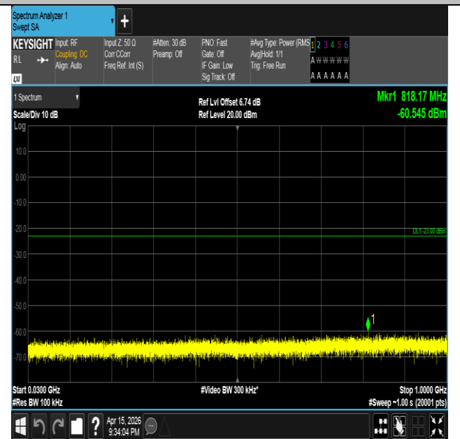
Band2-20MHz-QPSK-18900-1RB#99-30~1000-PASS
