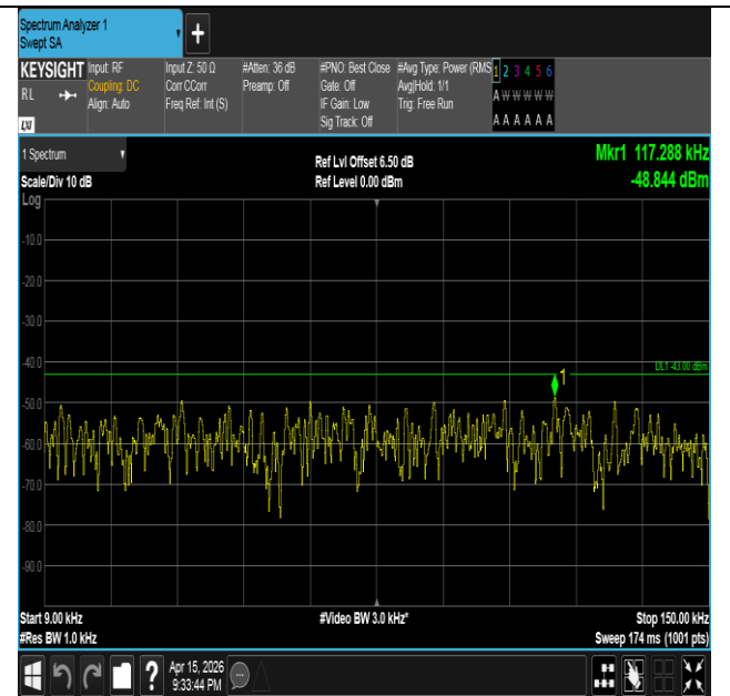
Band2-20MHz-QPSK-18900-1RB#99-0.009~0.15-PASS
