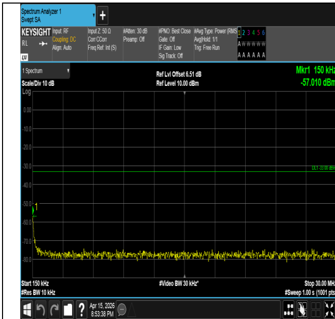
Band2-15MHz-16QAM-19125-1RB#0-0.15~30-PASS
