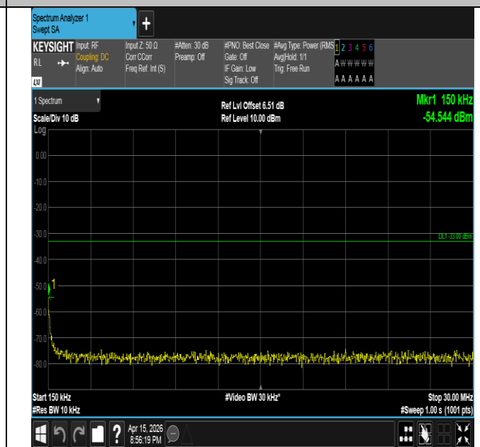
Band2-15MHz-QPSK-19125-75RB#0-0.15~30-PASS
