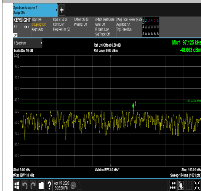
Band2-20MHz-QPSK-18700-1RB#0-0.009~0.15-PASS
