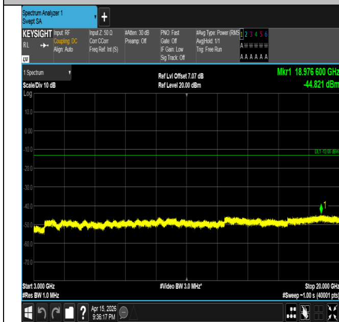
Band2-20MHz-QPSK-18900-100RB#0-3000~20000-PASS
