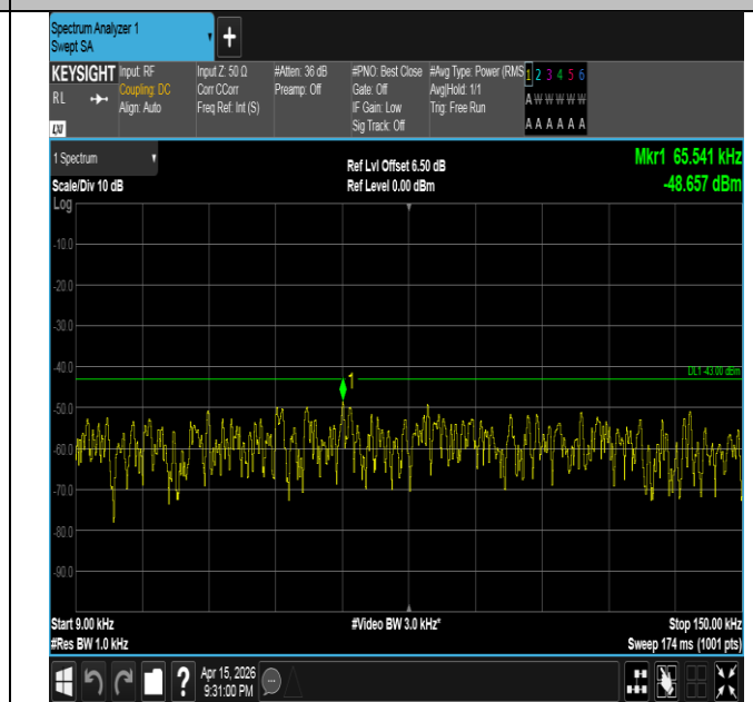
Band2-20MHz-16QAM-18700-100RB#0-0.009~0.15-PASS
