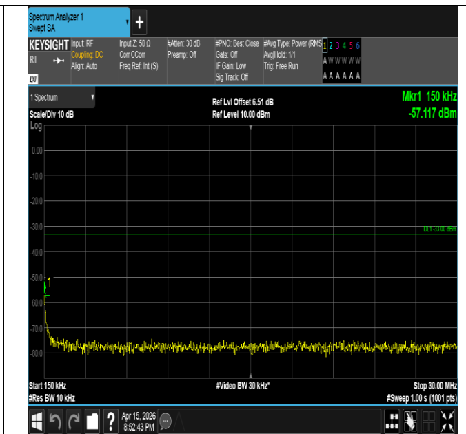
Band2-15MHz-QPSK-19125-1RB#0-0.15~30-PASS
