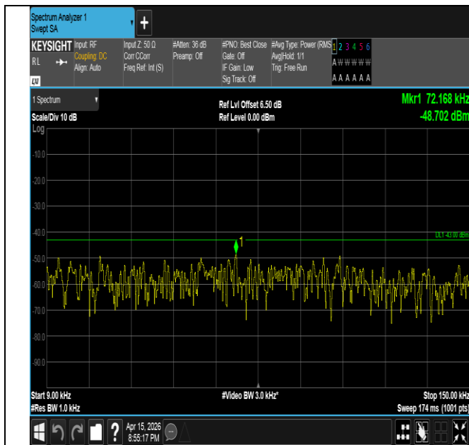
Band2-15MHz-16QAM-19125-1RB#74-0.009~0.15-PASS
