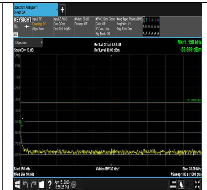
Band2-15MHz-16QAM-19125-1RB#74-0.15~30-PASS
