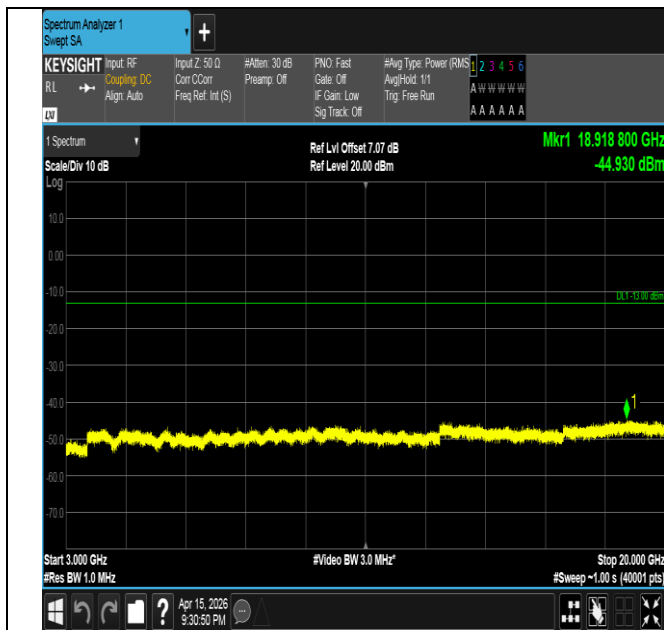
Band2-20MHz-QPSK-18700-100RB#0-3000~20000-PASS
