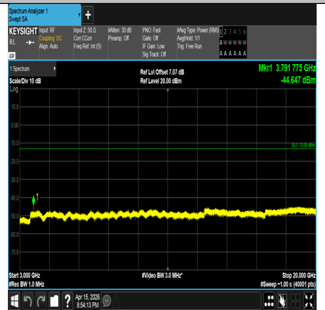
Band2-15MHz-16QAM-19125-1RB#0-3000~20000-PASS
