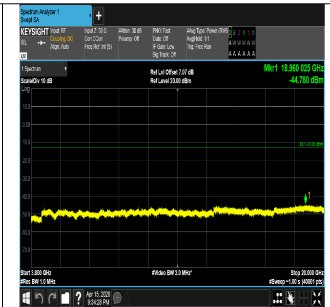
Band2-20MHz-QPSK-18900-1RB#99-3000~20000-PASS
