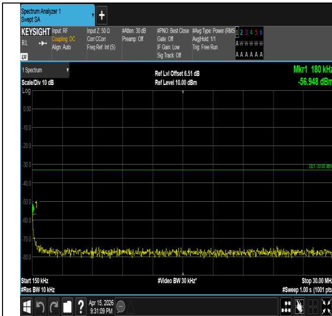
Band2-20MHz-16QAM-18700-100RB#0-0.15~30-PASS
