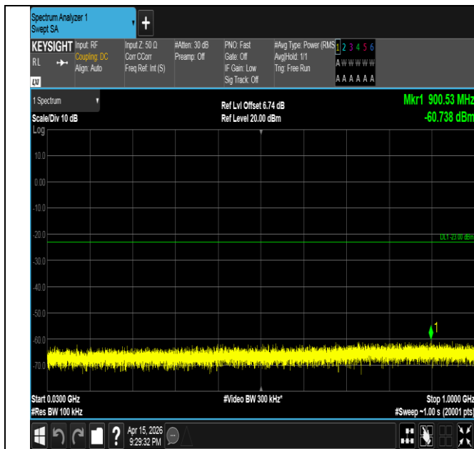
Band2-20MHz-16QAM-18700-1RB#99-30~1000-PASS
