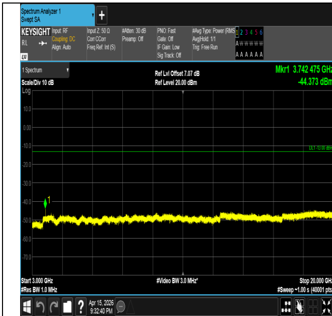
Band2-20MHz-QPSK-18900-1RB#0-3000~20000-PASS
