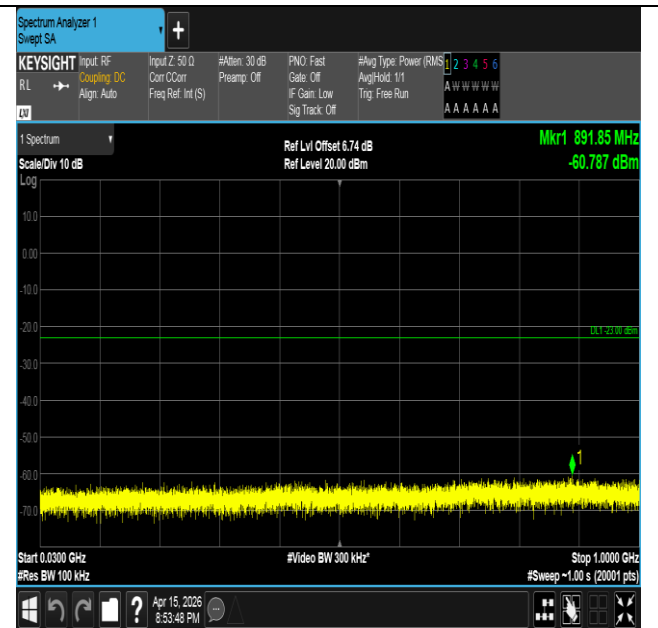
Band2-15MHz-16QAM-19125-1RB#0-30~1000-PASS
