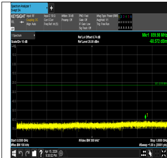
Band2-20MHz-QPSK-18900-100RB#0-30~1000-PASS
