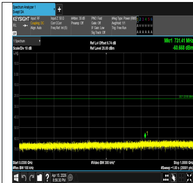
Band2-15MHz-QPSK-19125-75RB#0-30~1000-PASS
