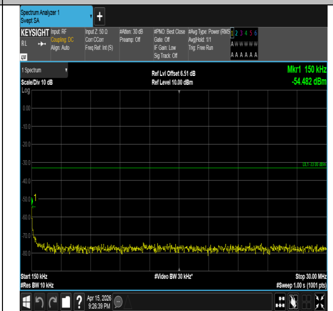
Band2-20MHz-QPSK-18700-1RB#0-0.15~30-PASS
