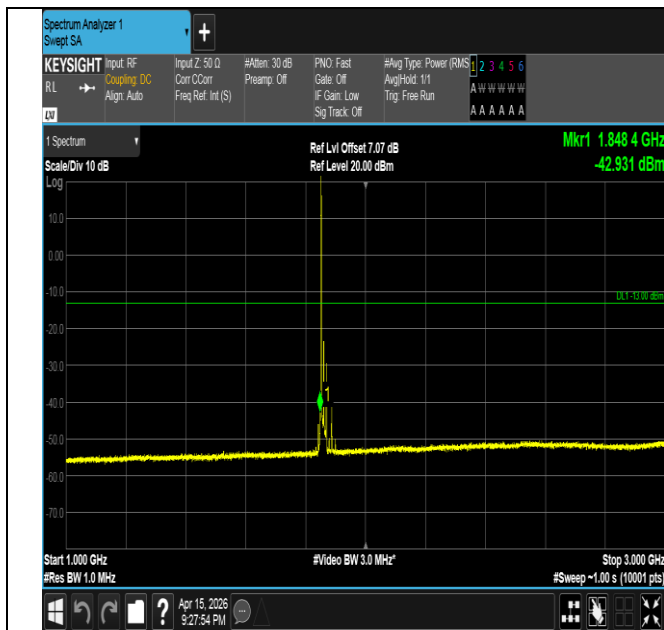
Band2-20MHz-16QAM-18700-1RB#0-1000~3000-PASS
