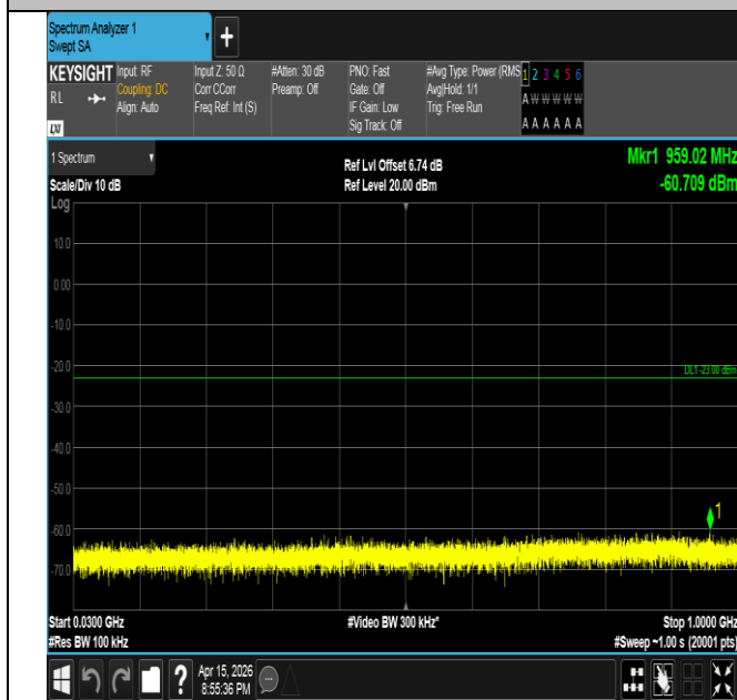
Band2-15MHz-16QAM-19125-1RB#74-30~1000-PASS
