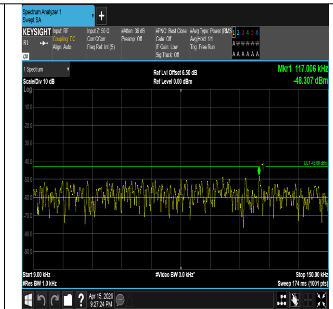
Band2-20MHz-16QAM-18700-1RB#0-0.009~0.15-PASS
