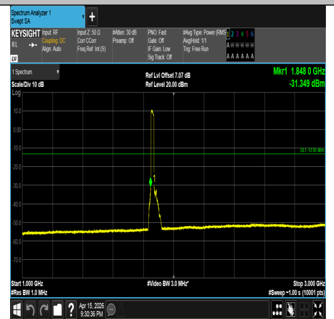
Band2-20MHz-QPSK-18700-100RB#0-1000~3000-PASS
