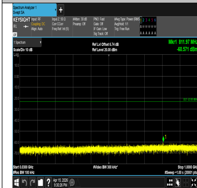
Band2-20MHz-QPSK-18700-100RB#0-30~1000-PASS
