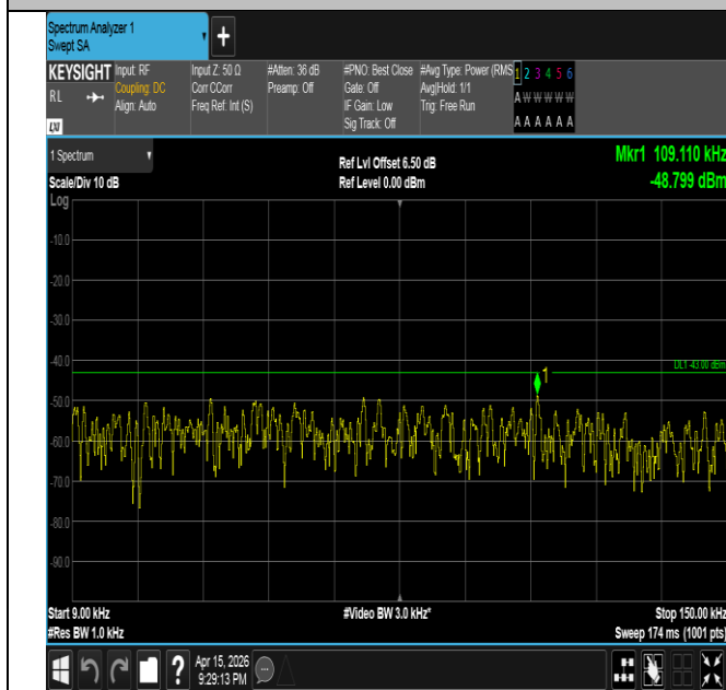
Band2-20MHz-16QAM-18700-1RB#99-0.009~0.15-PASS
