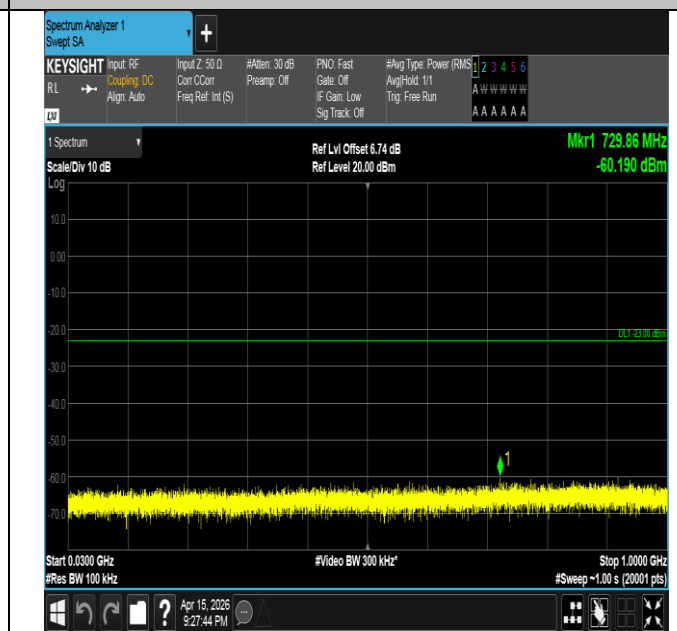
Band2-20MHz-16QAM-18700-1RB#0-30~1000-PASS
