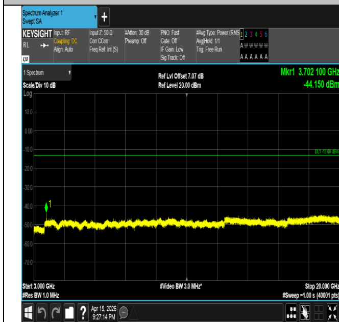
Band2-20MHz-QPSK-18700-1RB#0-3000~20000-PASS
