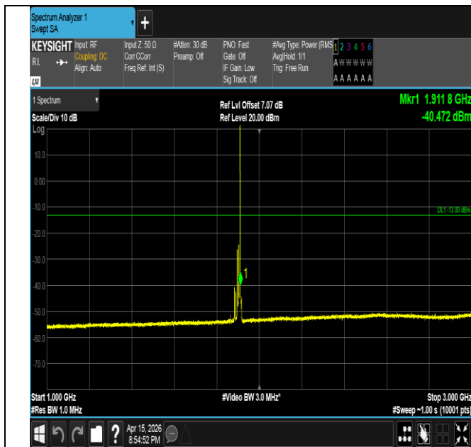
Band2-15MHz-QPSK-19125-1RB#74-1000~3000-PASS
