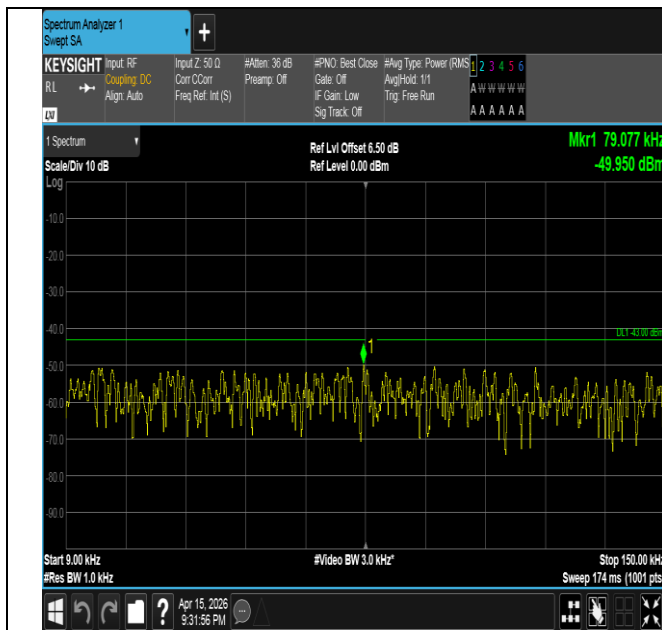
Band2-20MHz-QPSK-18900-1RB#0-0.009~0.15-PASS
