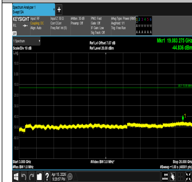
Band2-20MHz-16QAM-18700-1RB#99-3000~20000-PASS
