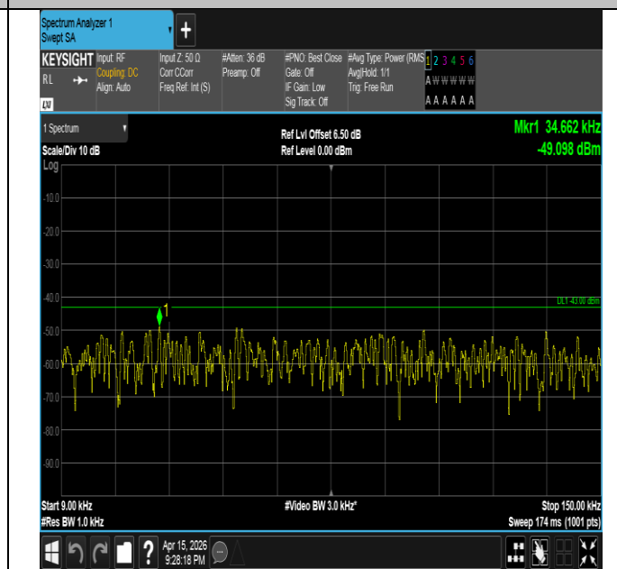
Band2-20MHz-QPSK-18700-1RB#99-0.009~0.15-PASS
