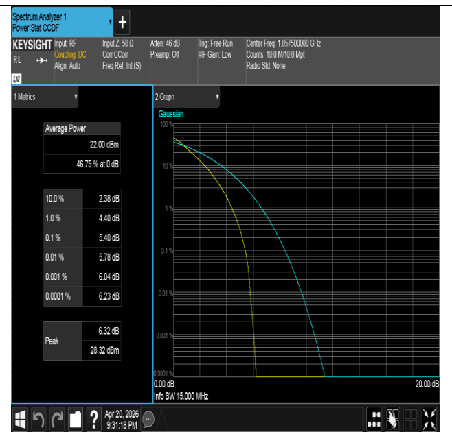
Band25-15MHz-QPSK-26115-75RB#0-PASS
