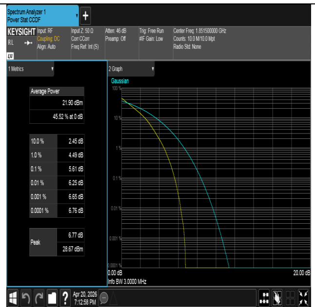
Band25-3MHz-QPSK-26055-15RB#0-PASS
