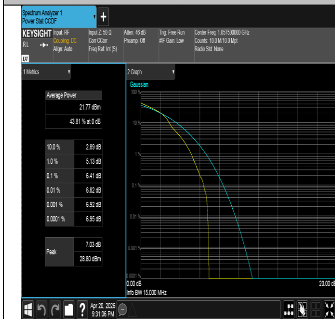
Band25-15MHz-16QAM-26115-1RB#0-PASS
