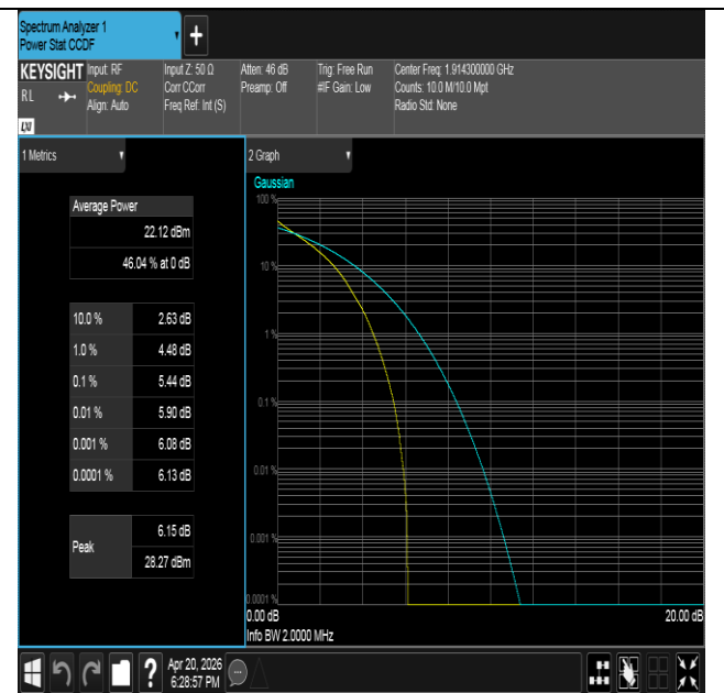
Band25-1.4MHz-QPSK-26683-6RB#0-PASS
