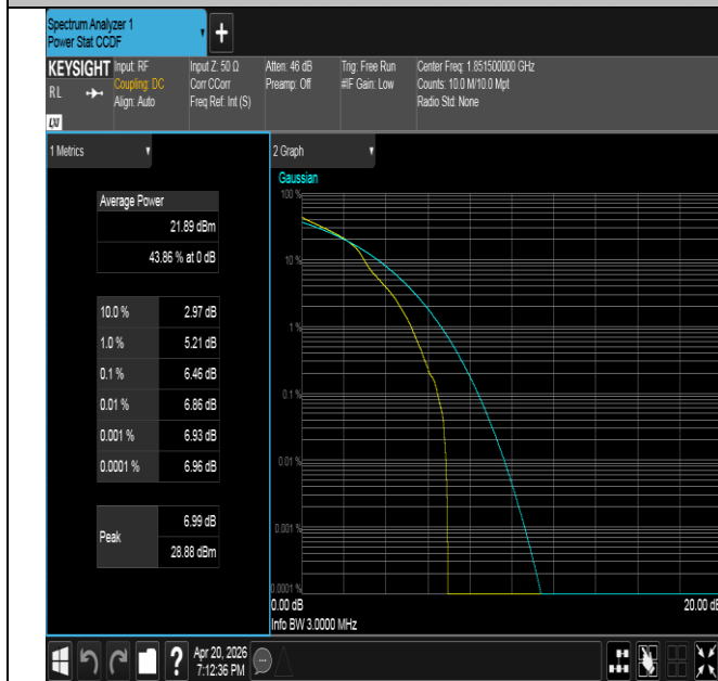
Band25-3MHz-16QAM-26055-1RB#0-PASS
