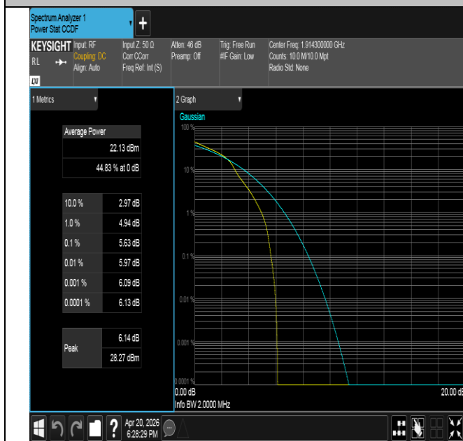
Band25-1.4MHz-16QAM-26683-1RB#0-PASS
