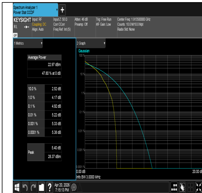
Band25-3MHz-QPSK-26675-1RB#0-PASS
