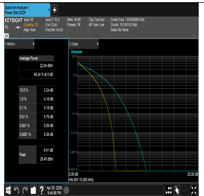
Band25-10MHz-QPSK-26090-50RB#0-PASS
