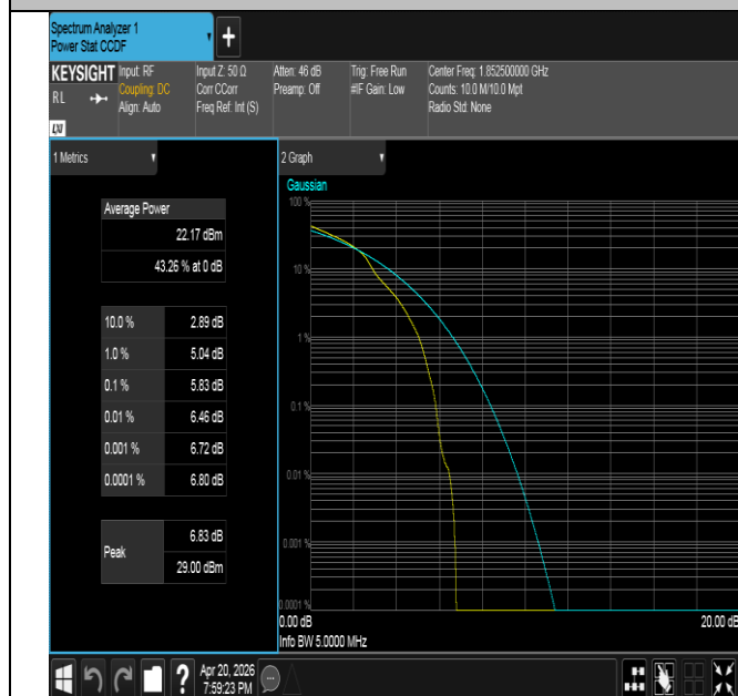
Band25-5MHz-16QAM-26065-1RB#0-PASS
