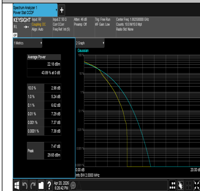
Band25-1.4MHz-16QAM-26365-1RB#0-PASS
