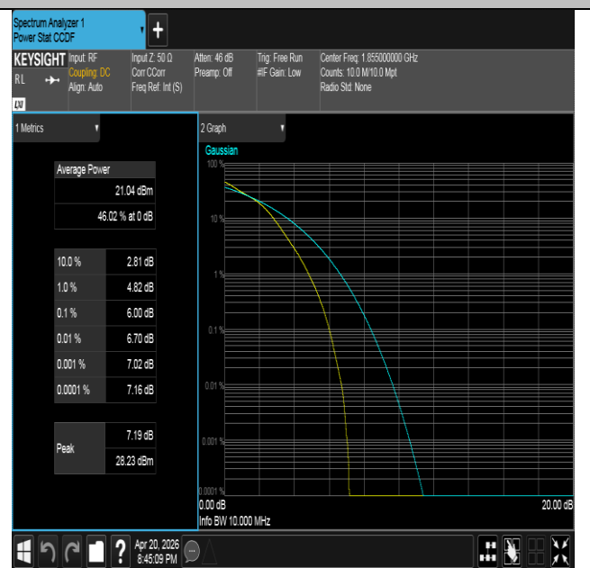
Band25-10MHz-16QAM-26090-50RB#0-PASS
