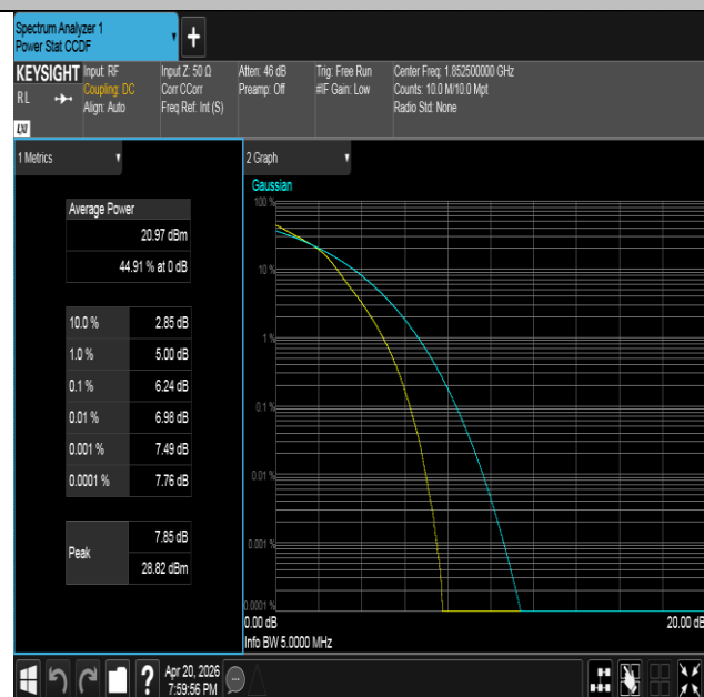
Band25-5MHz-16QAM-26065-25RB#0-PASS
