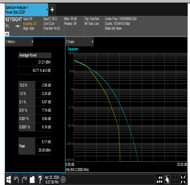
Band25-1.4MHz-16QAM-26365-6RB#0-PASS
