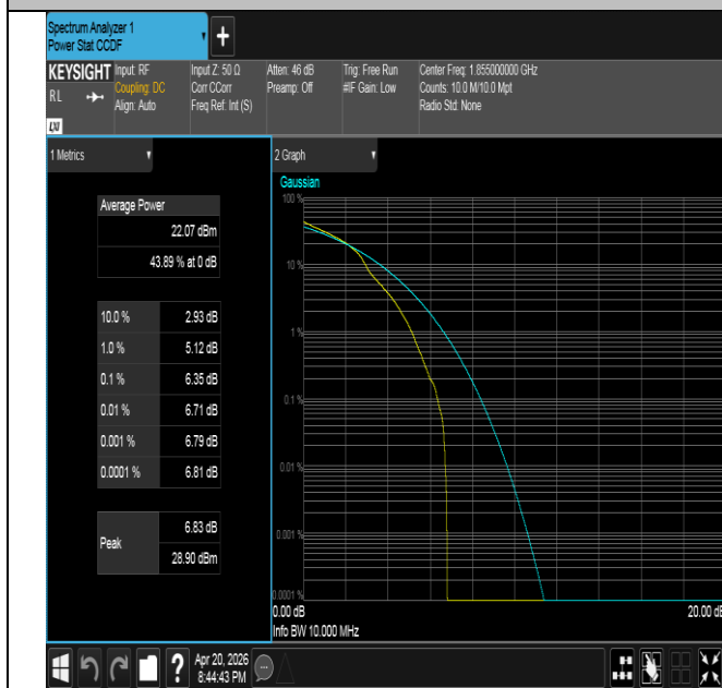
Band25-10MHz-16QAM-26090-1RB#0-PASS
