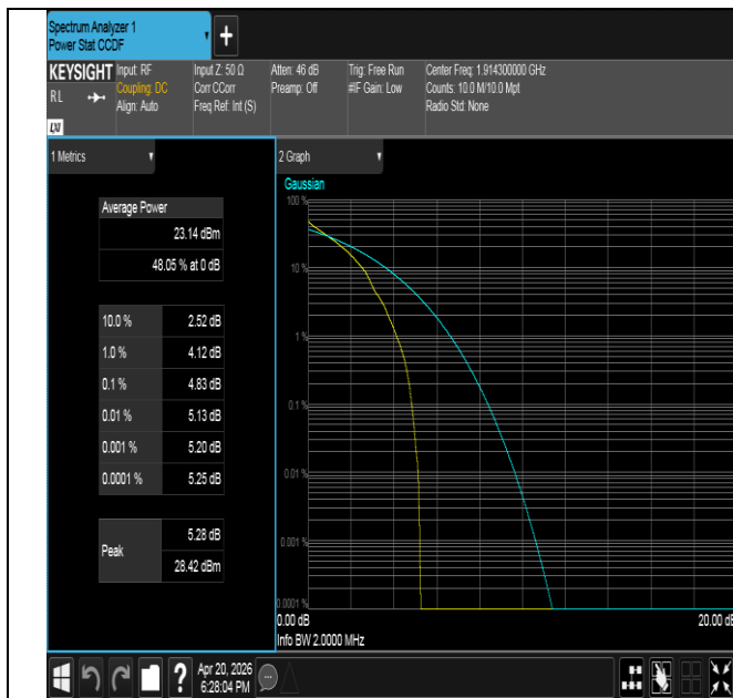
Band25-1.4MHz-QPSK-26683-1RB#0-PASS
