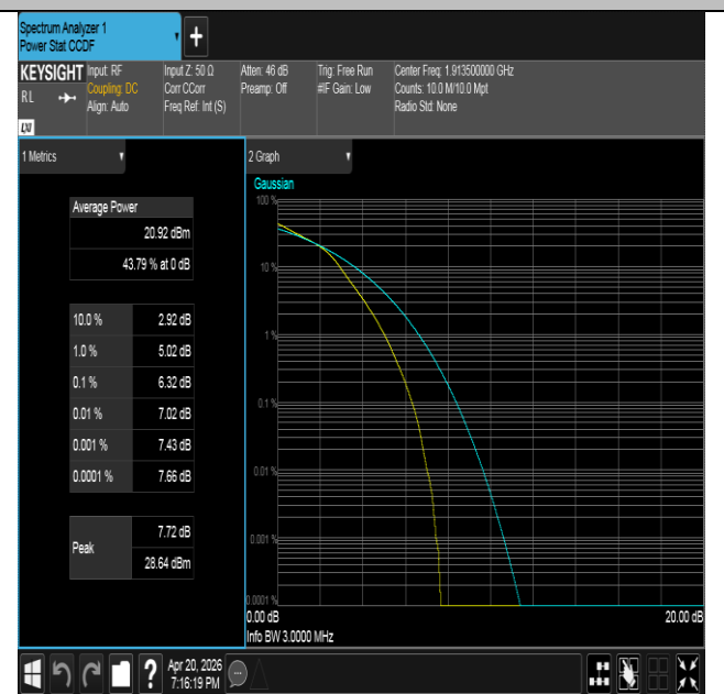
Band25-3MHz-16QAM-26675-15RB#0-PASS
