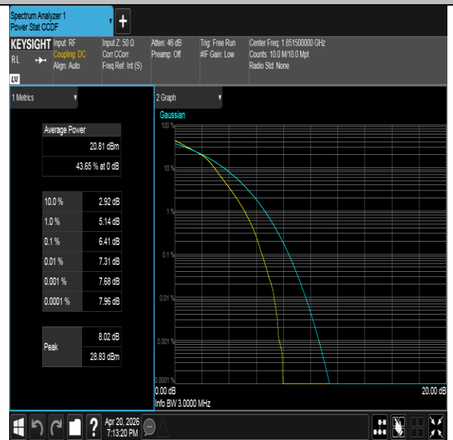
Band25-3MHz-16QAM-26055-15RB#0-PASS
