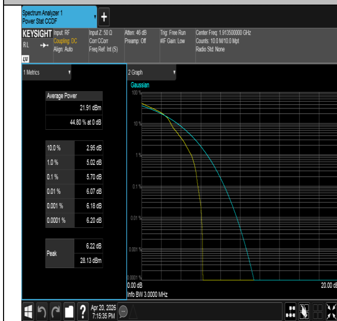
Band25-3MHz-16QAM-26675-1RB#0-PASS
