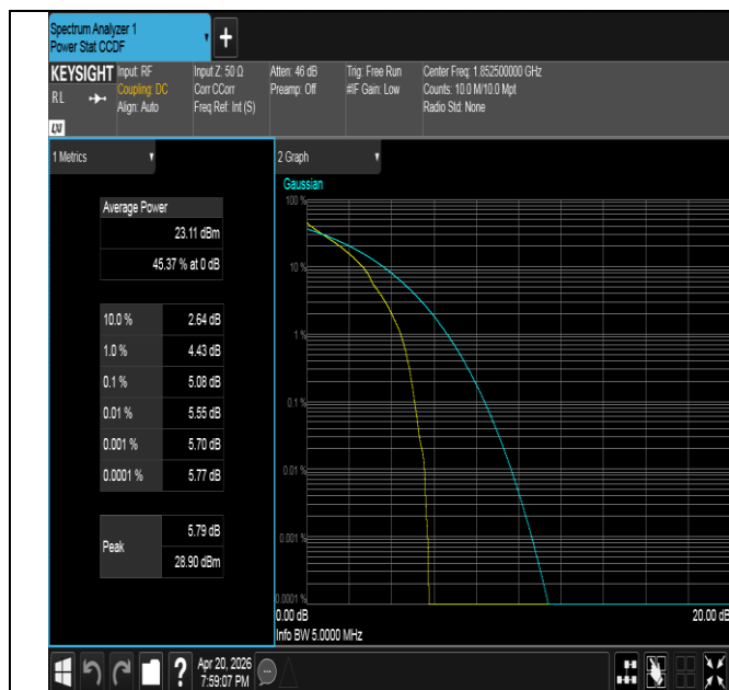
Band25-5MHz-QPSK-26065-1RB#0-PASS
