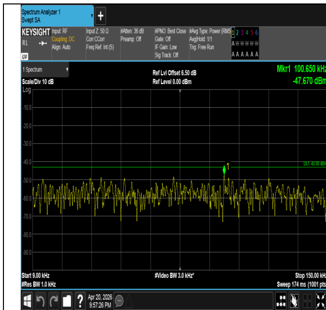
Band25-20MHz-QPSK-26590-100RB#0-0.009~0.15-PASS
