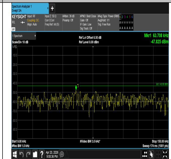
Band25-20MHz-QPSK-26590-1RB#99-0.009~0.15-PASS
