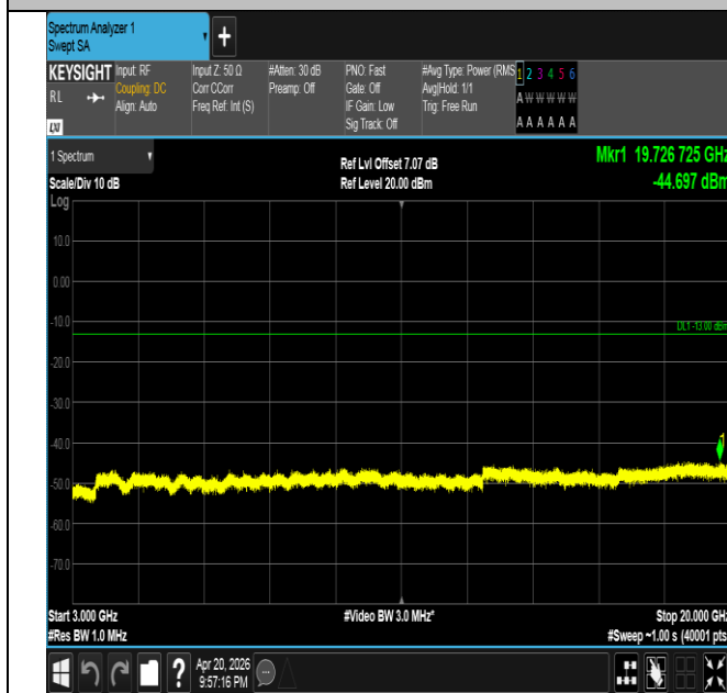
Band25-20MHz-16QAM-26590-1RB#99-3000~20000-PASS
