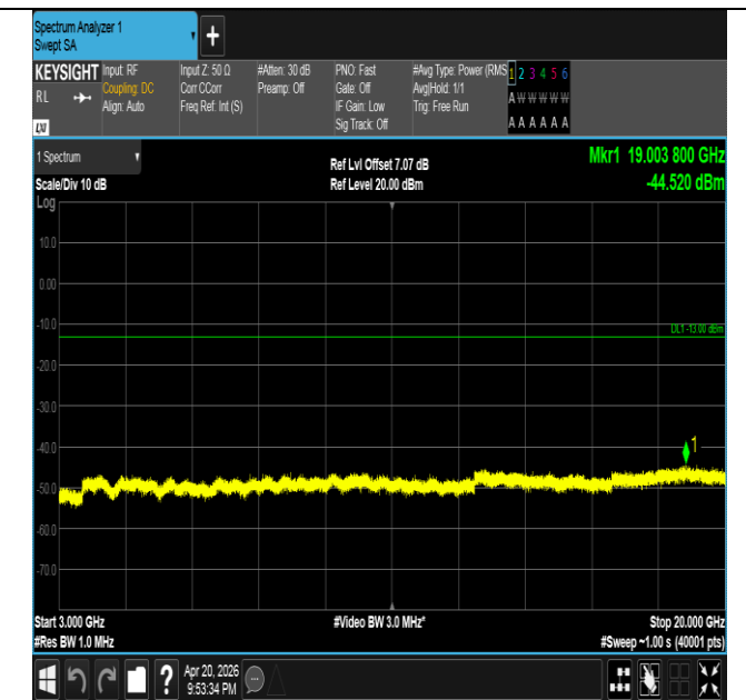
Band25-20MHz-16QAM-26365-100RB#0-3000~20000-PASS
