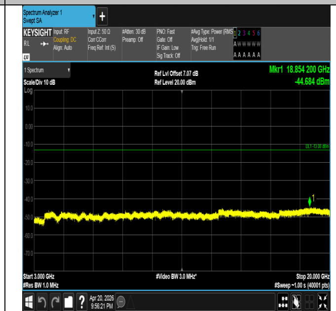
Band25-20MHz-QPSK-26590-1RB#99-3000~20000-PASS
