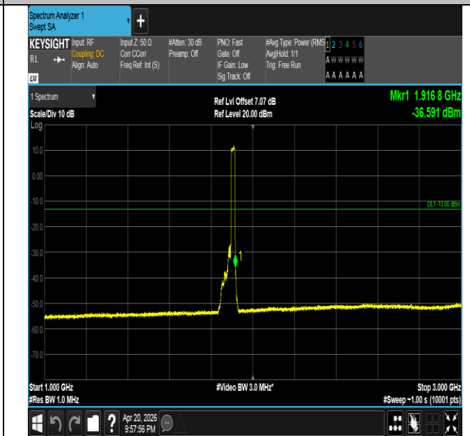
Band25-20MHz-QPSK-26590-100RB#0-1000~3000-PASS
