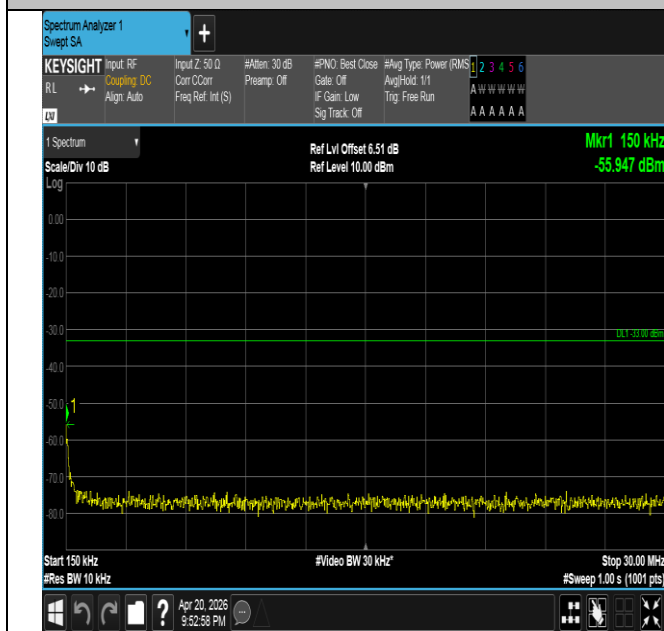
Band25-20MHz-16QAM-26365-100RB#0-0.15~30-PASS
