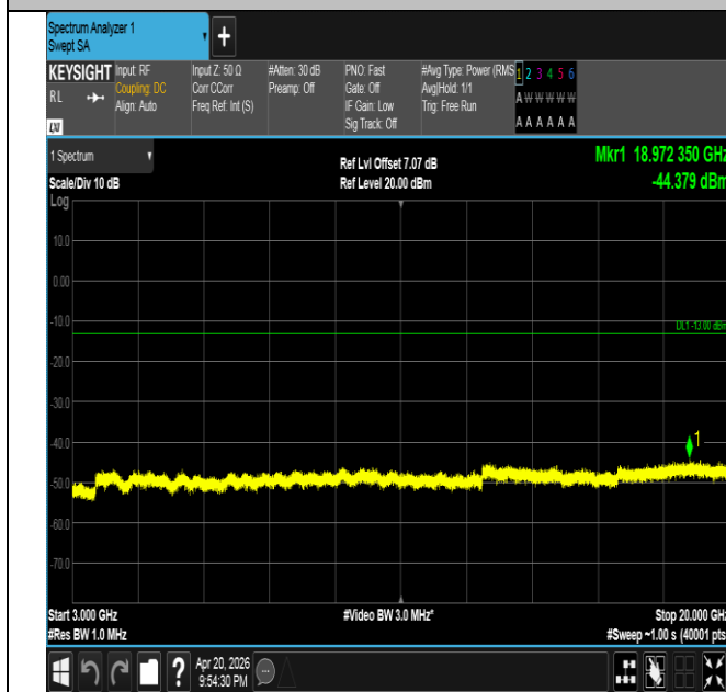
Band25-20MHz-QPSK-26590-1RB#0-3000~20000-PASS
