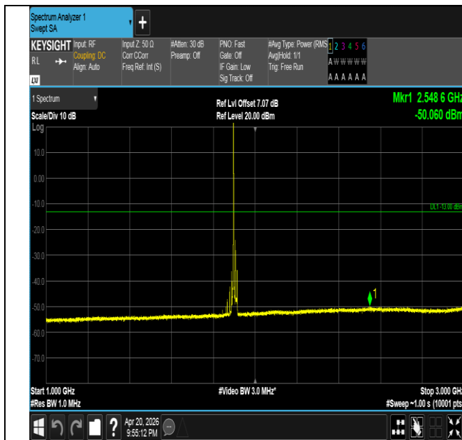
Band25-20MHz-16QAM-26590-1RB#0-1000~3000-PASS
