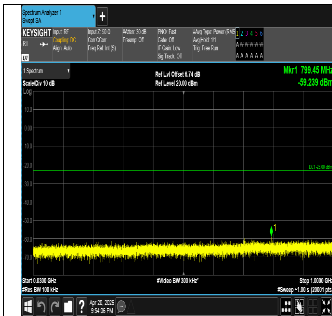
Band25-20MHz-QPSK-26590-1RB#0-30~1000-PASS
