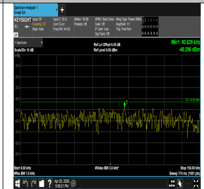
Band25-20MHz-16QAM-26590-100RB#0-0.009~0.15-PASS
