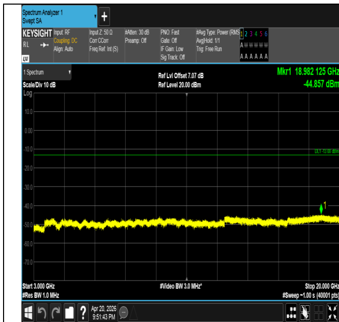
Band25-20MHz-16QAM-26365-1RB#99-3000~20000-PASS
