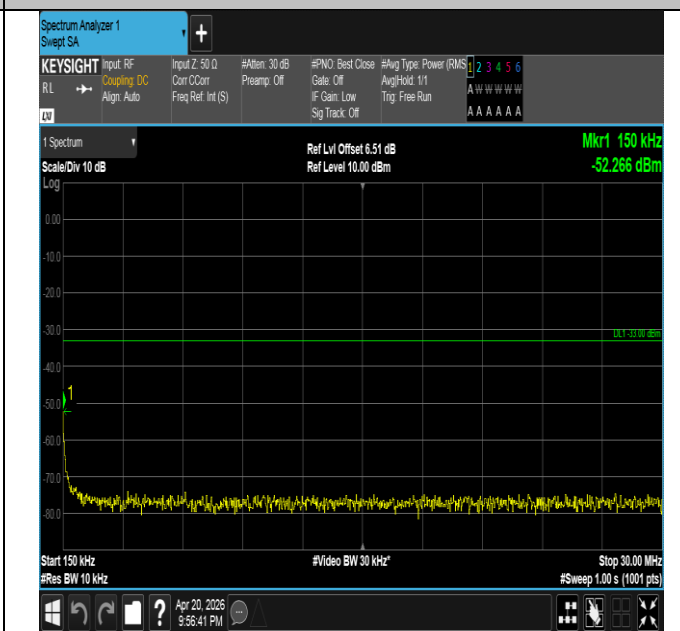
Band25-20MHz-16QAM-26590-1RB#99-0.15~30-PASS
