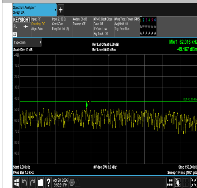
Band25-20MHz-16QAM-26590-1RB#99-0.009~0.15-PASS
