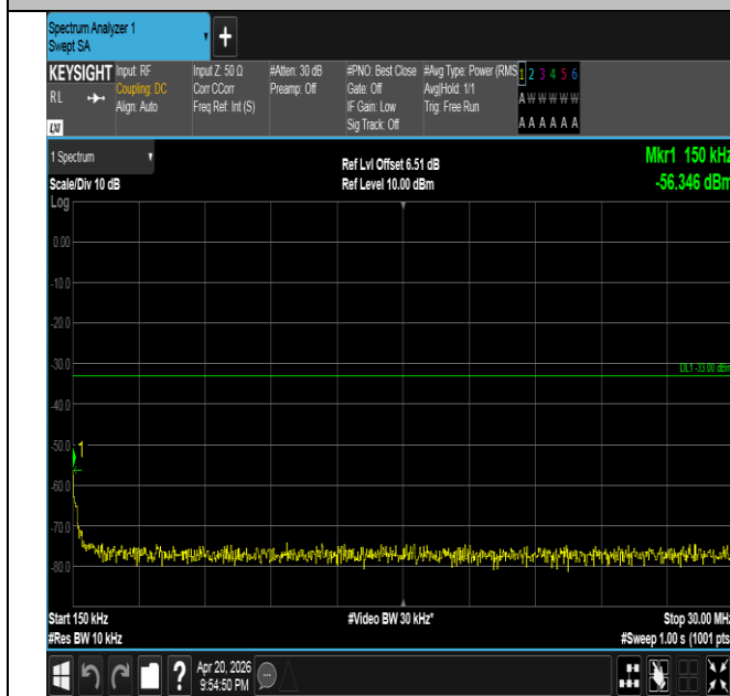
Band25-20MHz-16QAM-26590-1RB#0-0.15~30-PASS
