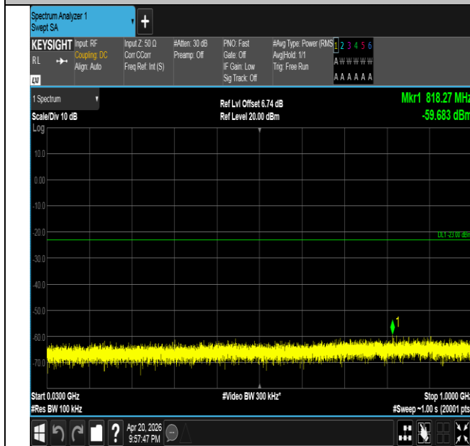
Band25-20MHz-QPSK-26590-100RB#0-30~1000-PASS
