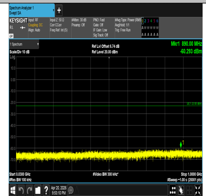
Band25-20MHz-16QAM-26365-100RB#0-30~1000-PASS
