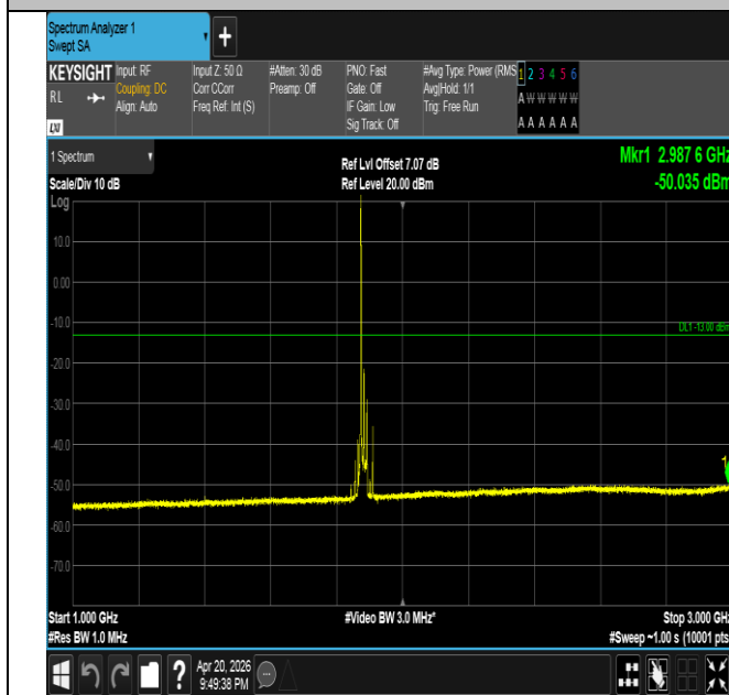
Band25-20MHz-16QAM-26365-1RB#0-1000~3000-PASS
