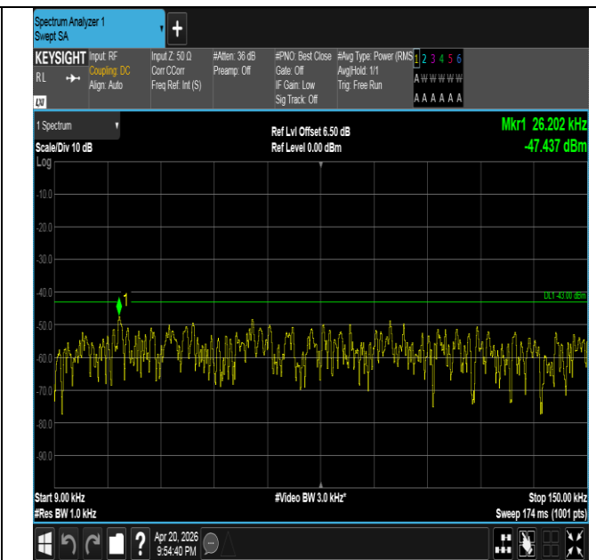
Band25-20MHz-16QAM-26590-1RB#0-0.009~0.15-PASS
