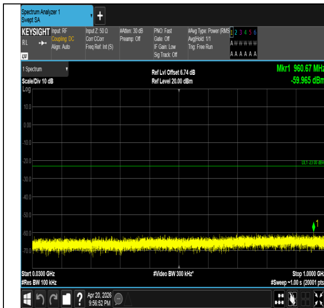
Band25-20MHz-16QAM-26590-1RB#99-30~1000-PASS
