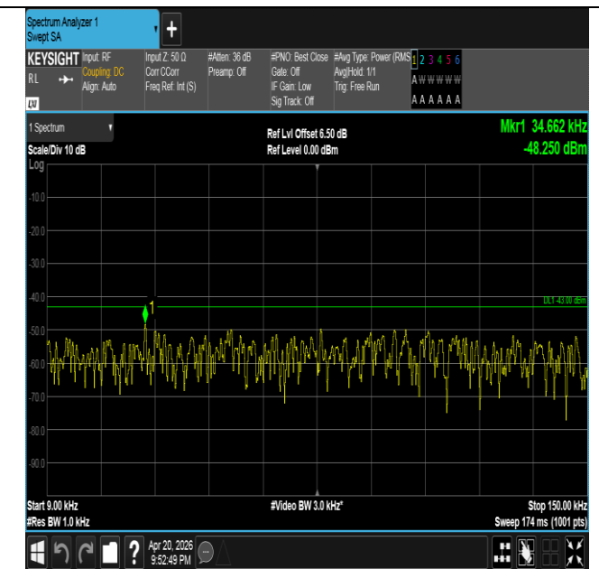
Band25-20MHz-16QAM-26365-100RB#0-0.009~0.15-PASS
