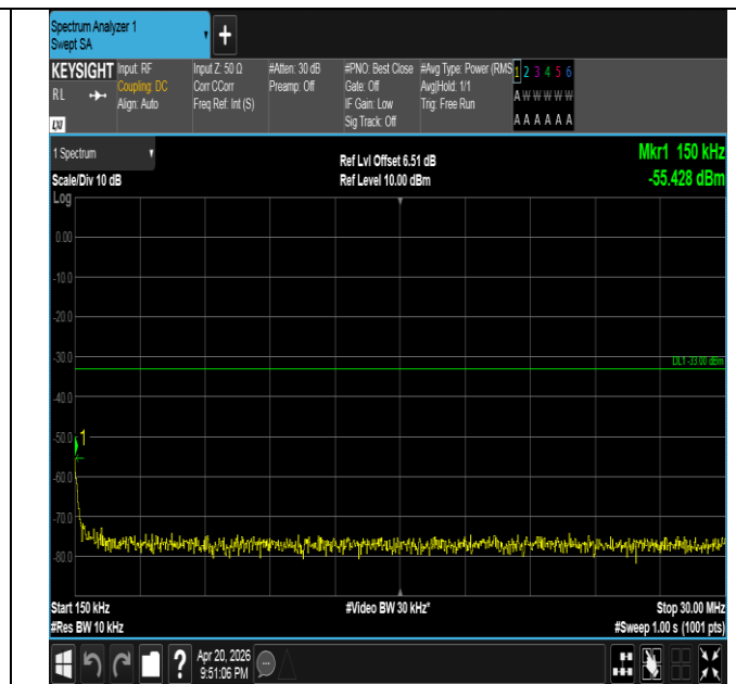
Band25-20MHz-16QAM-26365-1RB#99-0.15~30-PASS
