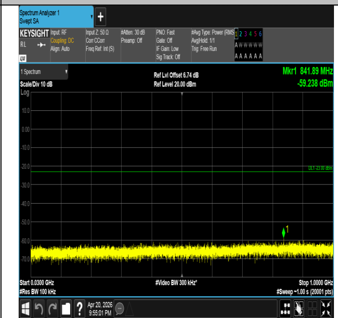
Band25-20MHz-16QAM-26590-1RB#0-30~1000-PASS
