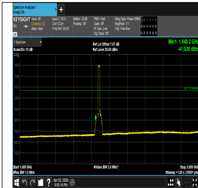
Band25-20MHz-16QAM-26365-100RB#0-1000~3000-PASS
