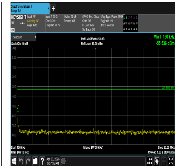
Band25-20MHz-QPSK-26590-100RB#0-0.15~30-PASS
