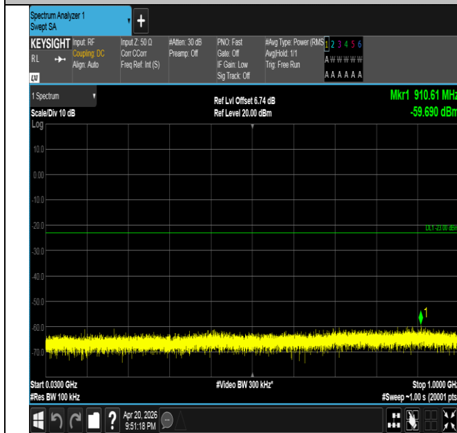
Band25-20MHz-16QAM-26365-1RB#99-30~1000-PASS
