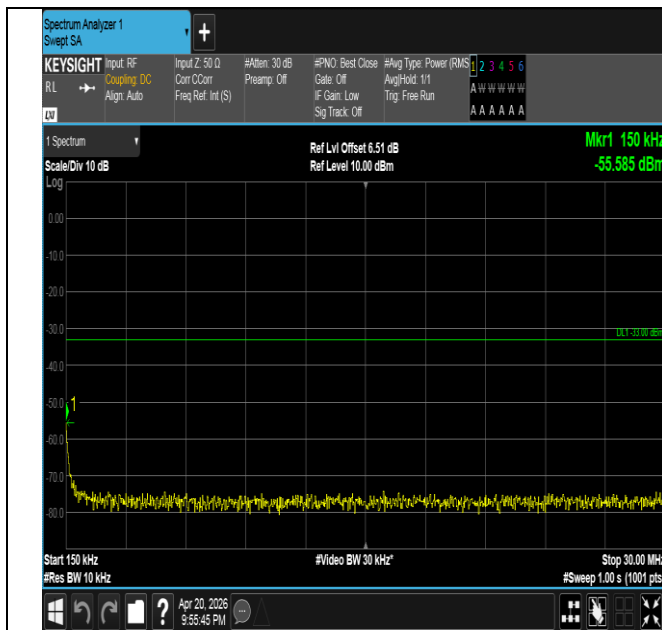
Band25-20MHz-QPSK-26590-1RB#99-0.15~30-PASS
