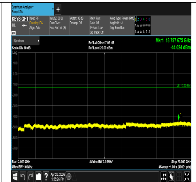
Band25-20MHz-16QAM-26590-1RB#0-3000~20000-PASS
