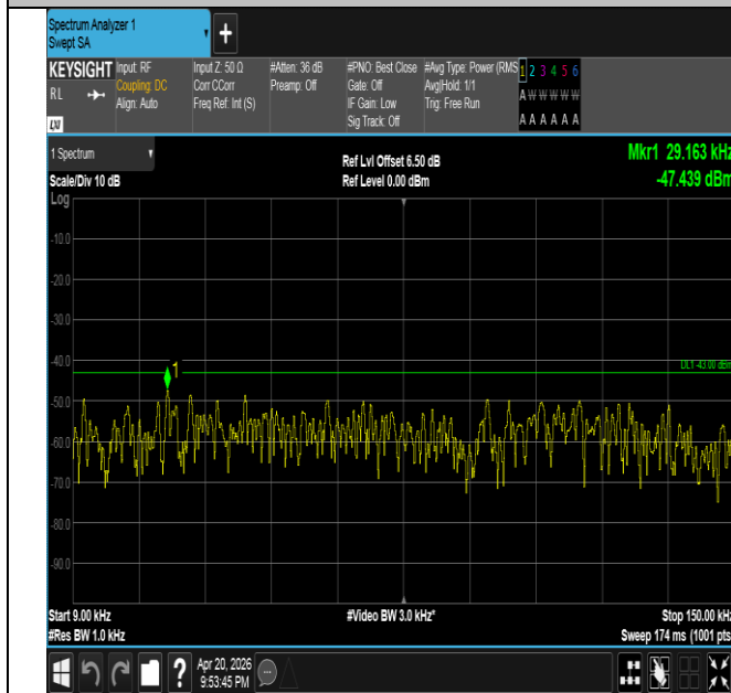
Band25-20MHz-QPSK-26590-1RB#0-0.009~0.15-PASS
