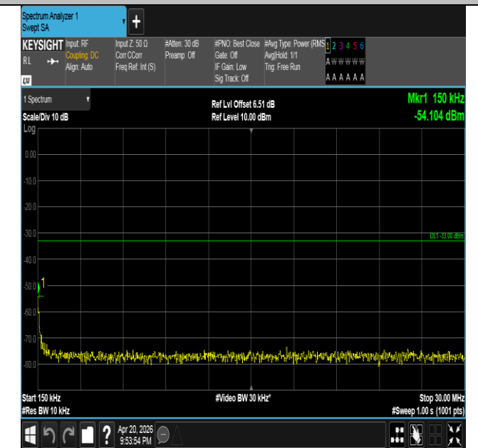
Band25-20MHz-QPSK-26590-1RB#0-0.15~30-PASS
