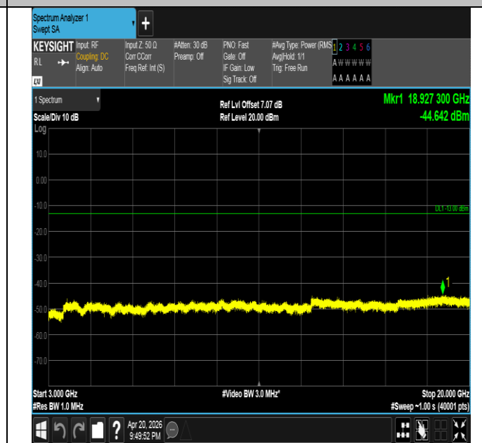
Band25-20MHz-16QAM-26365-1RB#0-3000~20000-PASS
