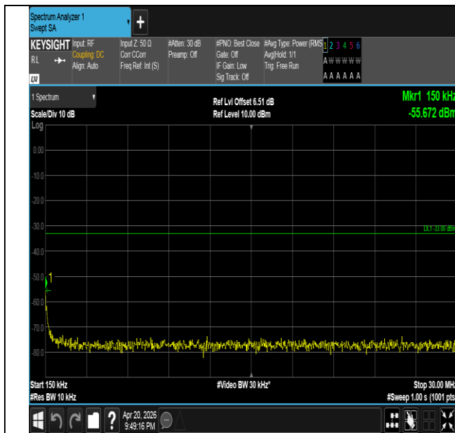
Band25-20MHz-16QAM-26365-1RB#0-0.15~30-PASS
