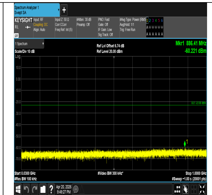
Band25-20MHz-16QAM-26365-1RB#0-30~1000-PASS
